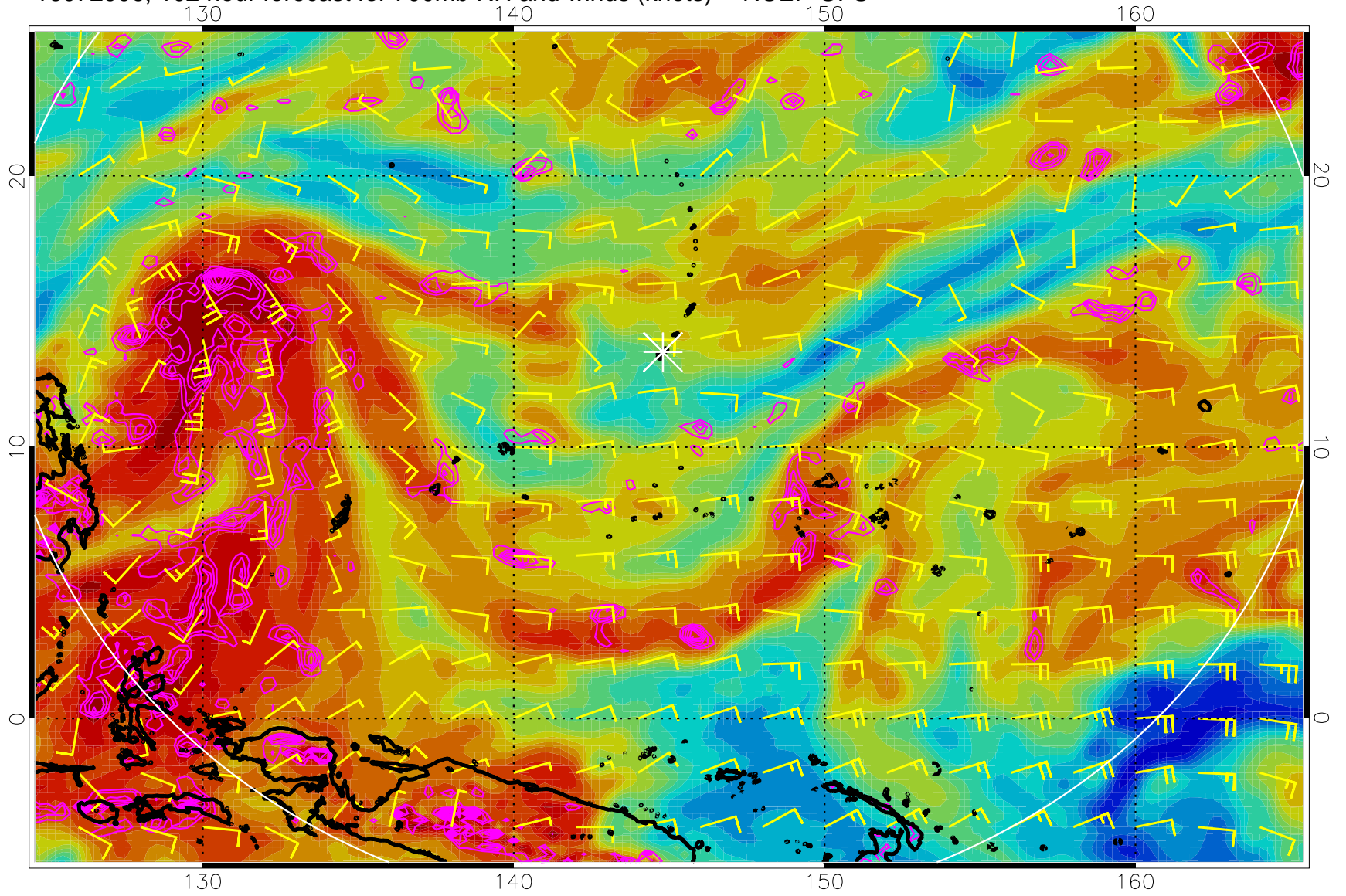
16072906, 102 hour forecast for 700mb RH and winds (knots) -- NCEP GFS
