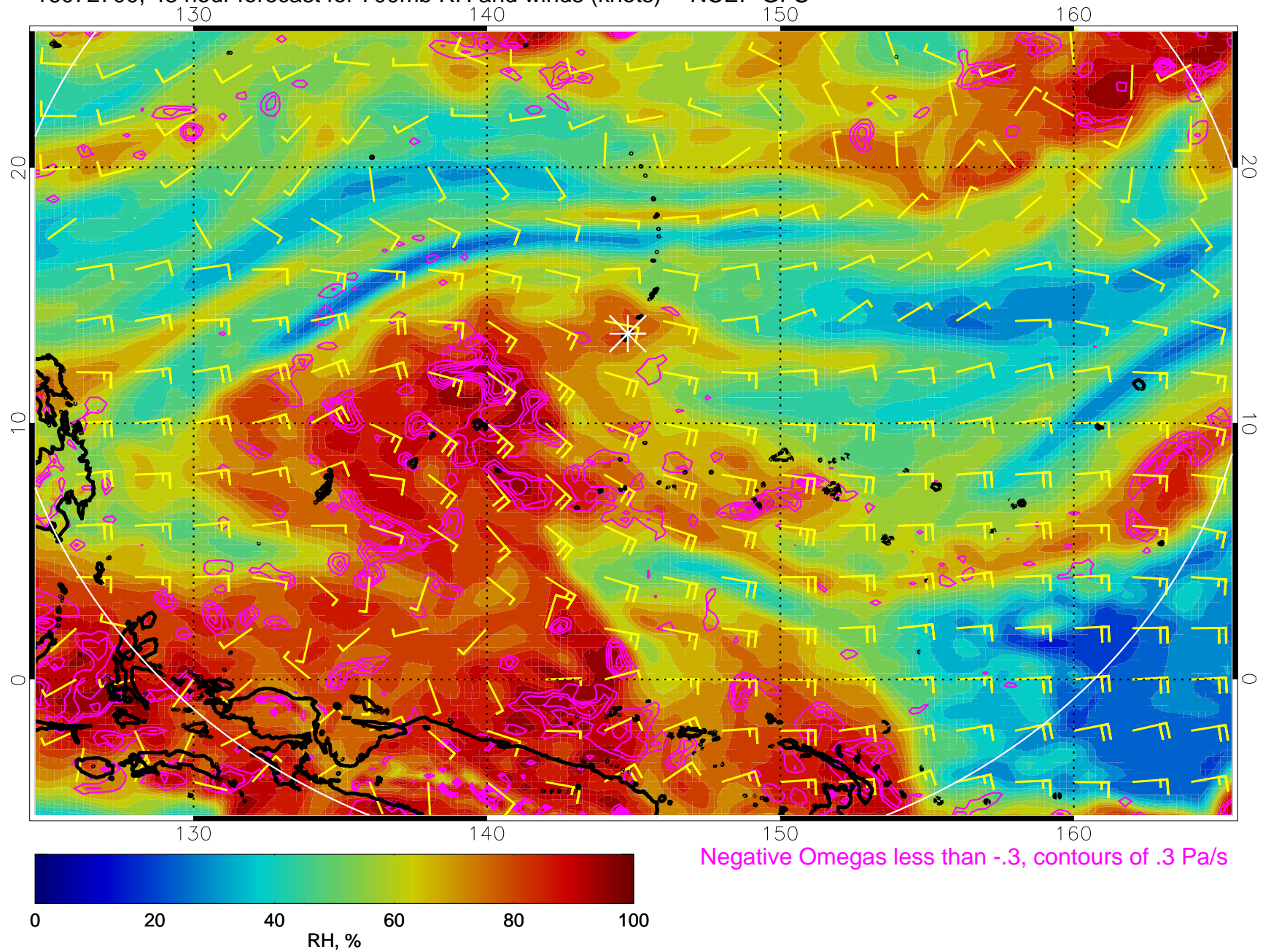
16072700, 48 hour forecast for 700mb RH and winds (knots) -- NCEP GFS
