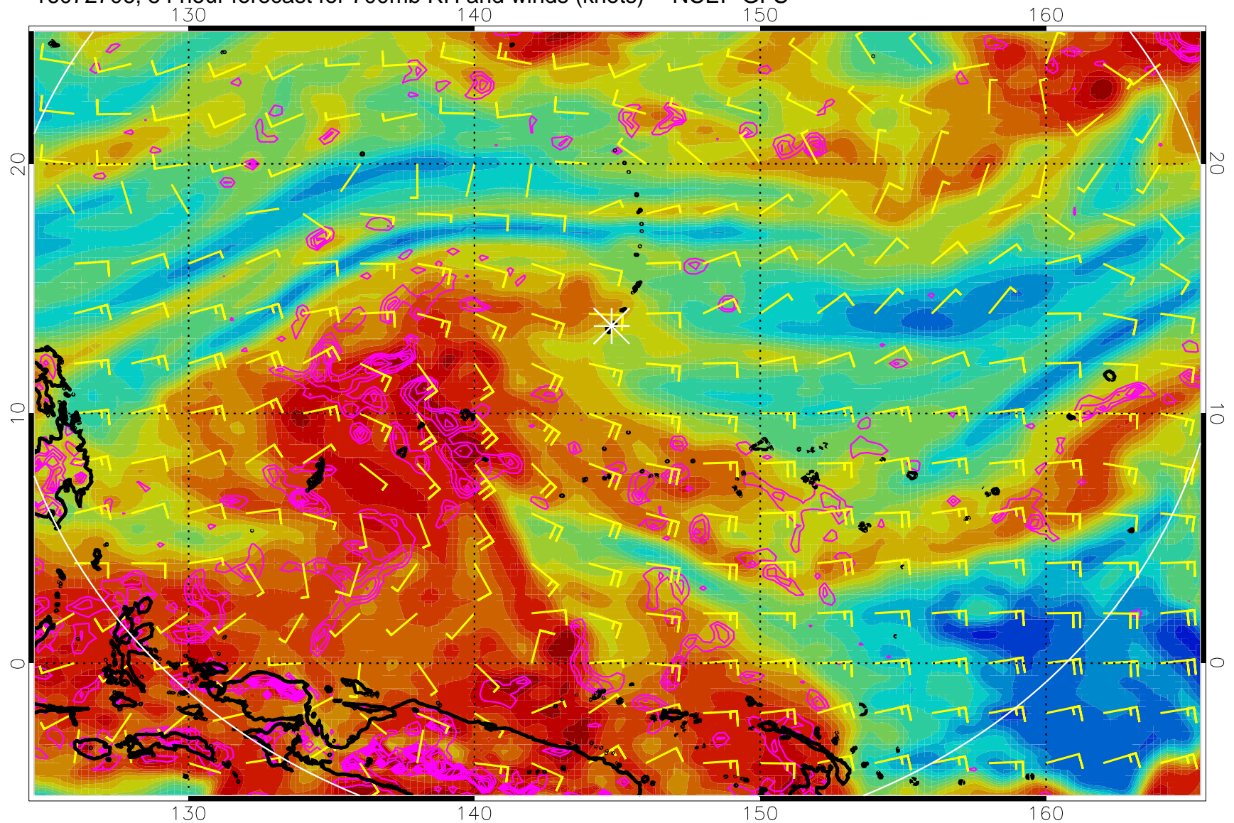
16072706, 54 hour forecast for 700mb RH and winds (knots) -- NCEP GFS
