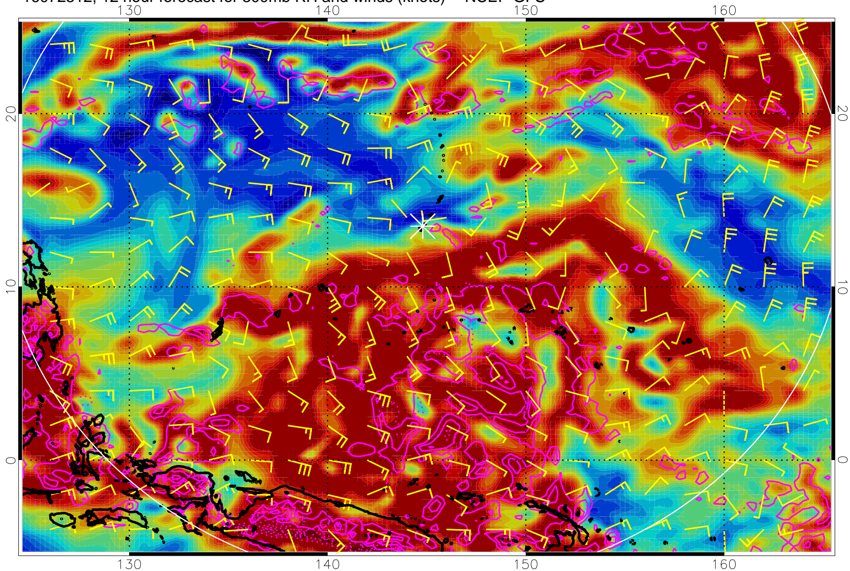
16072512, 12 hour forecast for 300mb RH and winds (knots) -- NCEP GFS
