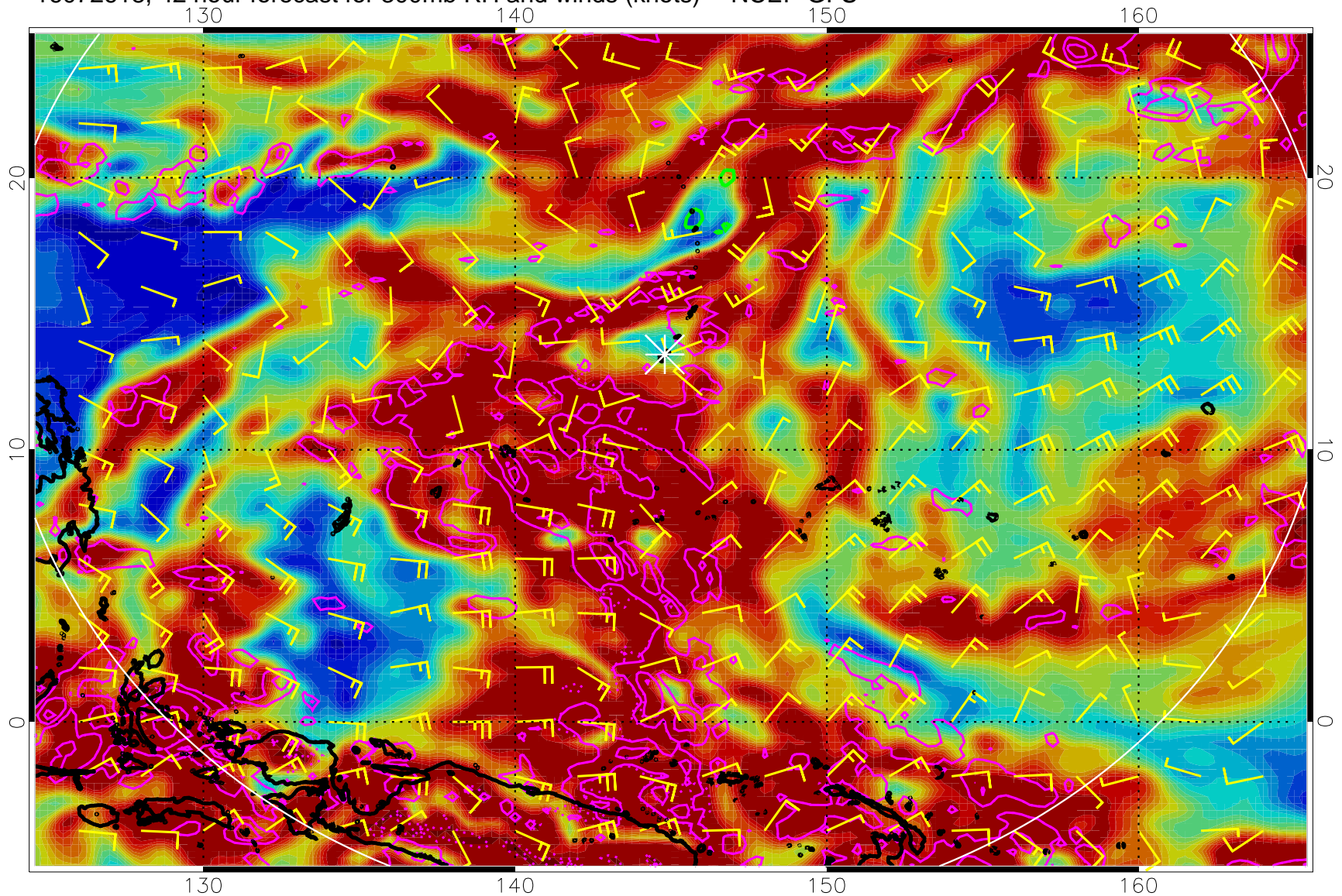
16072618, 42 hour forecast for 300mb RH and winds (knots) -- NCEP GFS
