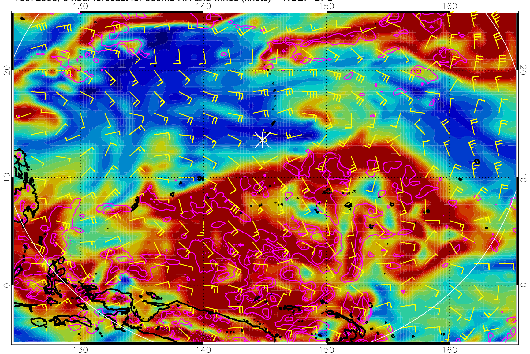
16072506, 6 hour forecast for 300mb RH and winds (knots) -- NCEP GFS
