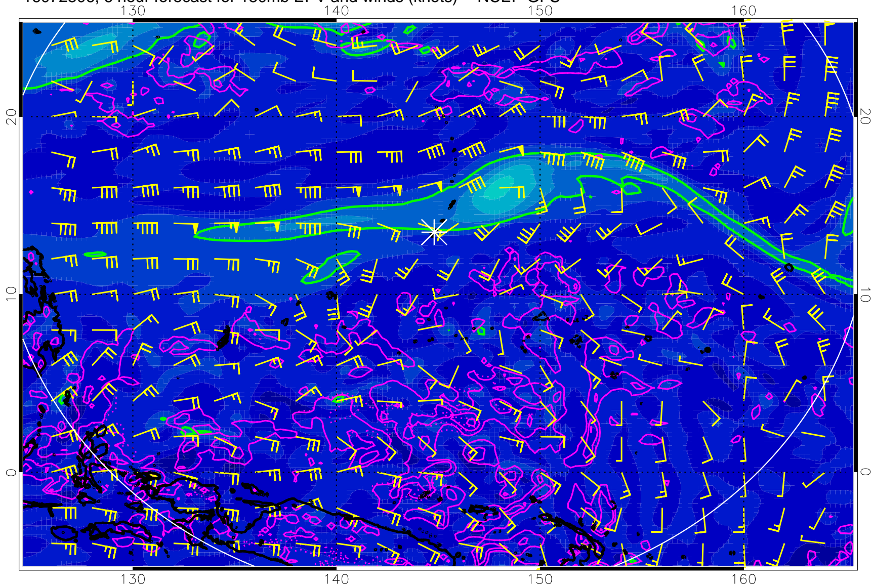
16072506, 6 hour forecast for 150mb EPV and winds (knots) -- NCEP GFS
