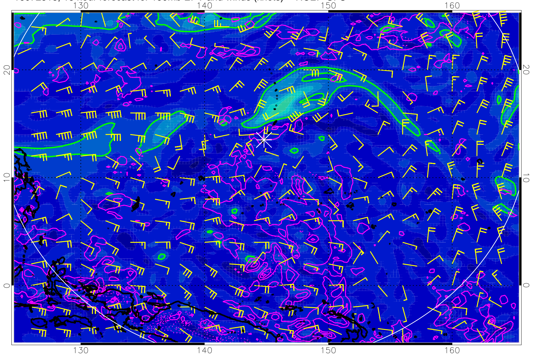
16072518, 18 hour forecast for 150mb EPV and winds (knots) -- NCEP GFS
