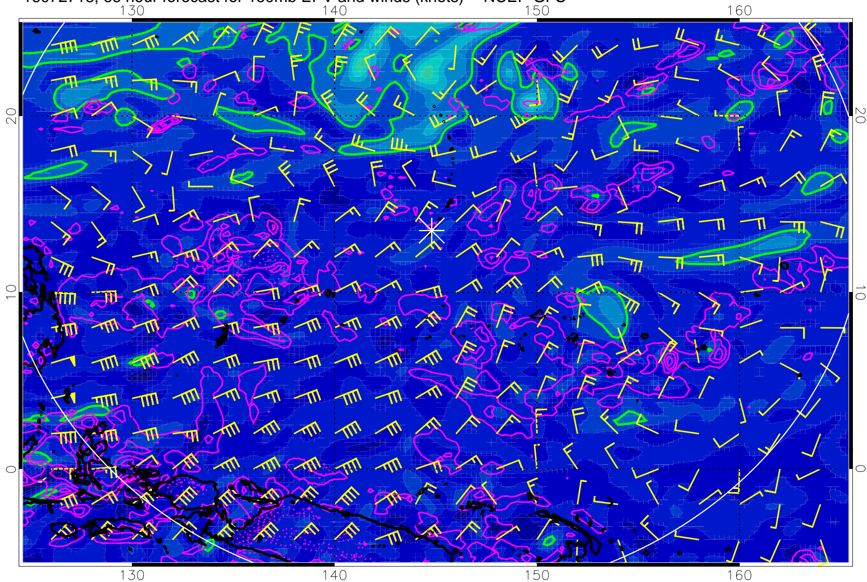
16072718, 66 hour forecast for 150mb EPV and winds (knots) -- NCEP GFS
