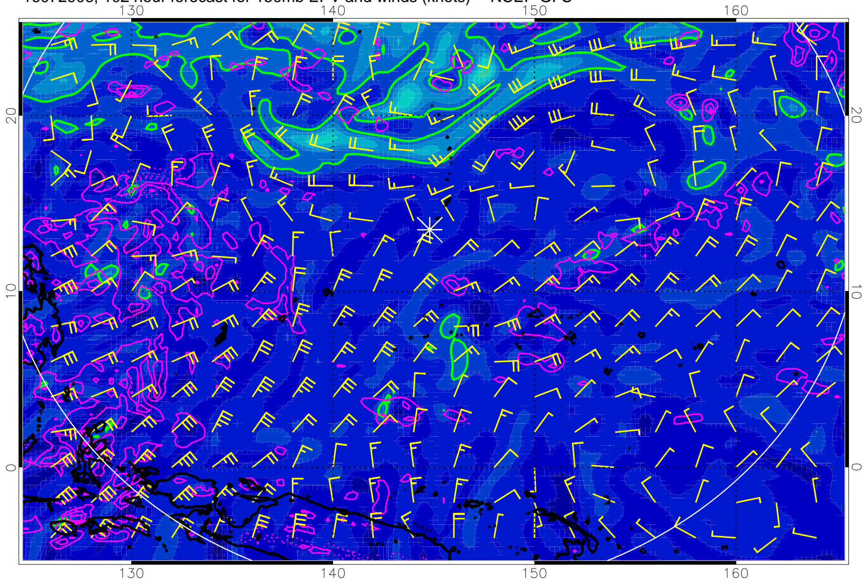
16072906, 102 hour forecast for 150mb EPV and winds (knots) -- NCEP GFS
