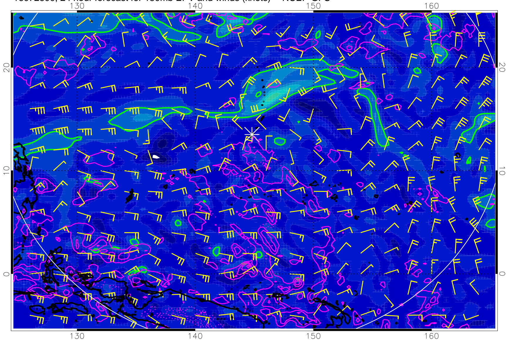
16072600, 24 hour forecast for 150mb EPV and winds (knots) -- NCEP GFS
