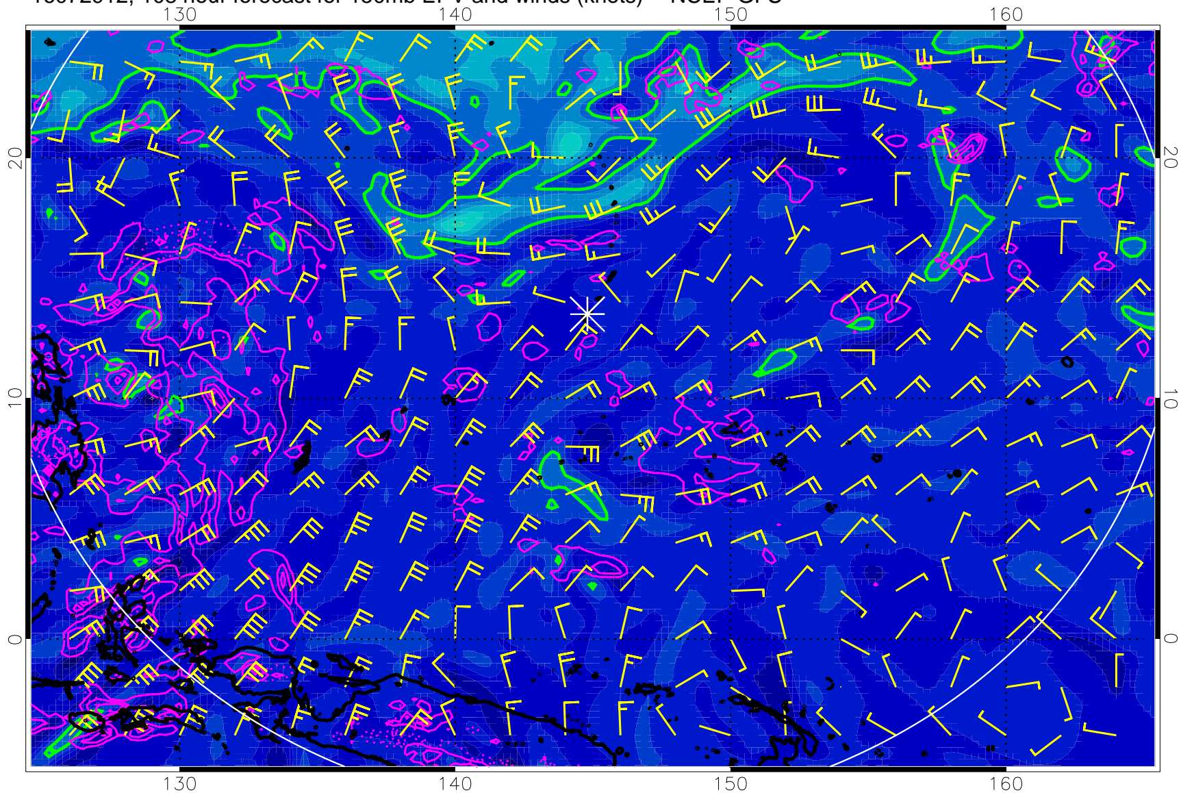
16072912, 108 hour forecast for 150mb EPV and winds (knots) -- NCEP GFS
