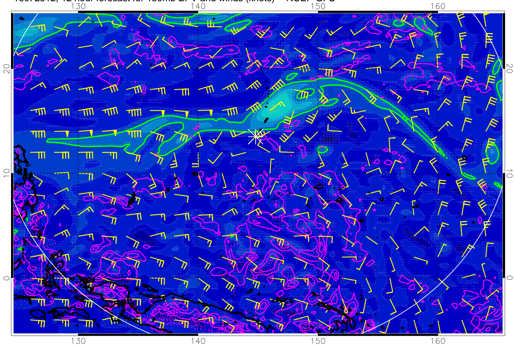
16072512, 12 hour forecast for 150mb EPV and winds (knots) -- NCEP GFS
