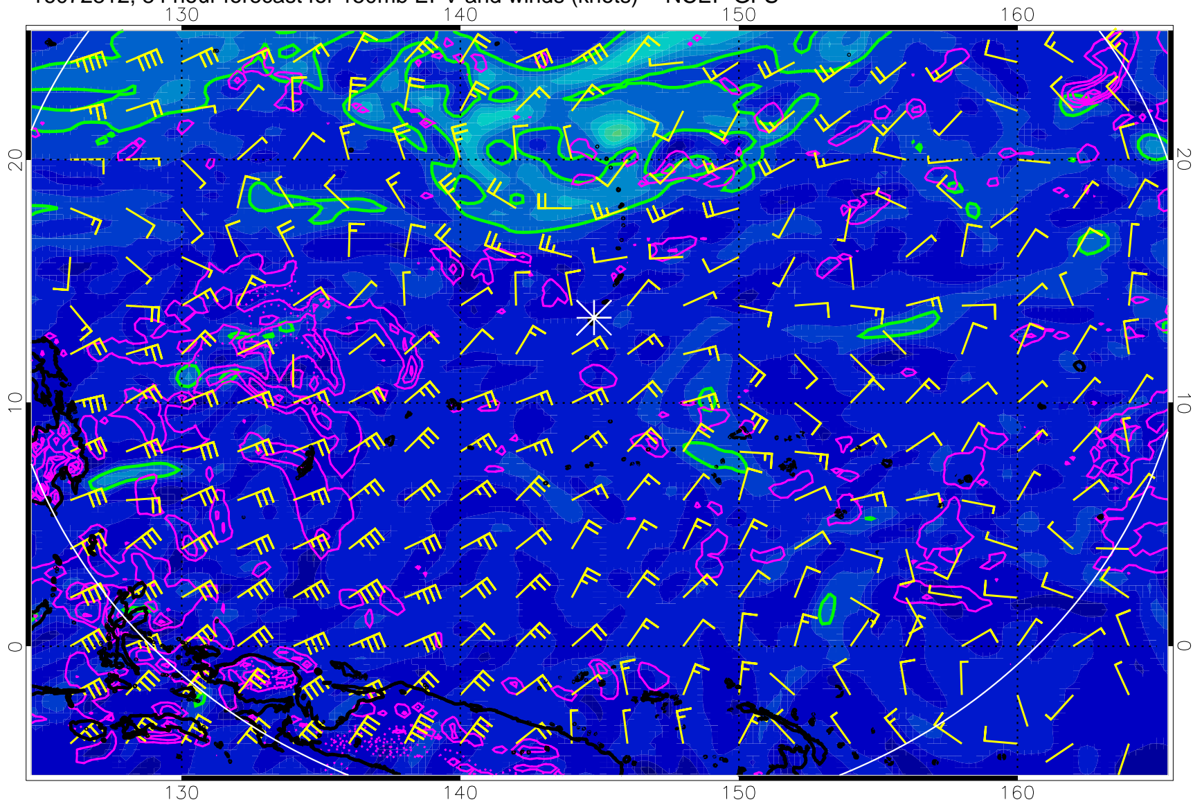
16072812, 84 hour forecast for 150mb EPV and winds (knots) -- NCEP GFS
