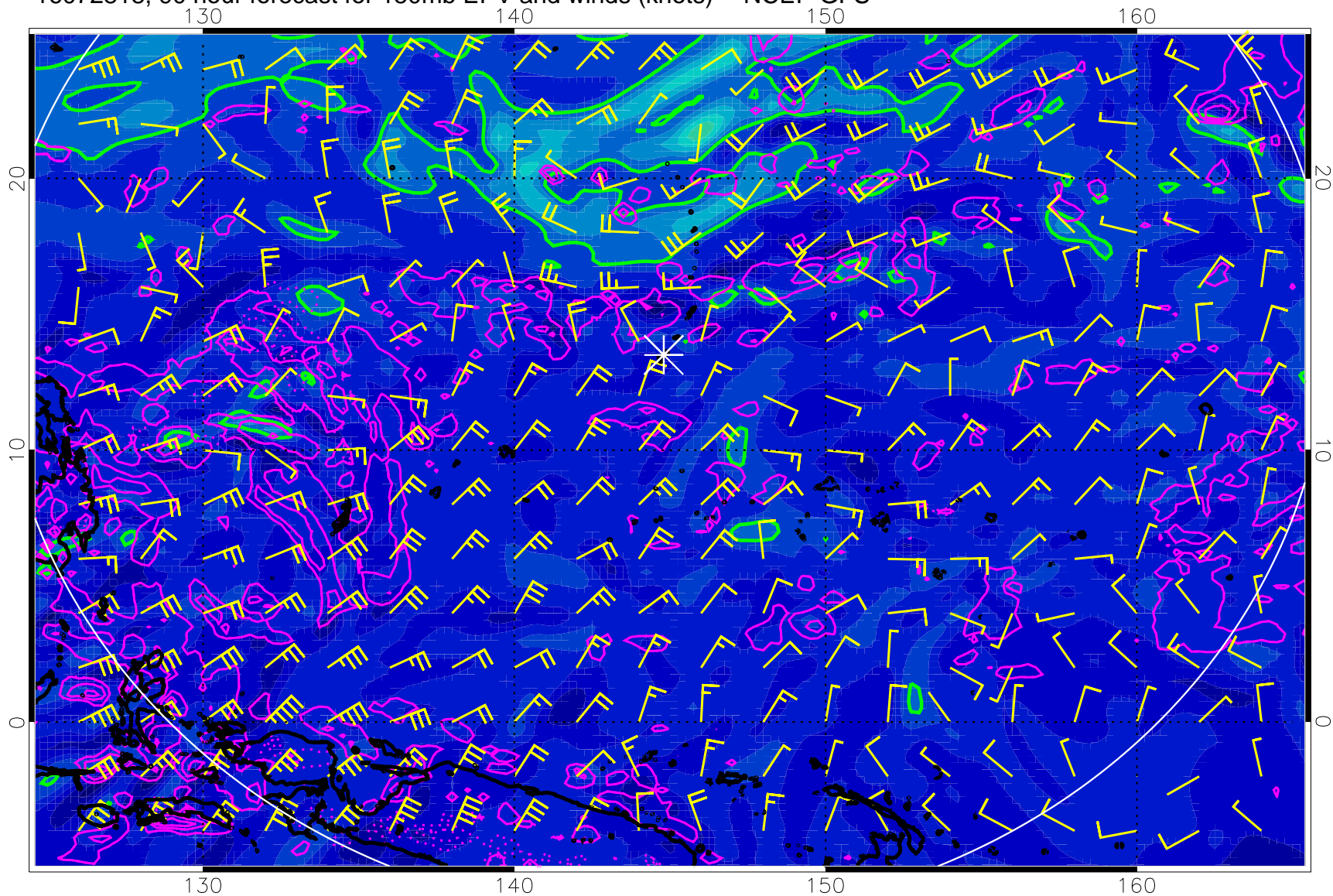
16072818, 90 hour forecast for 150mb EPV and winds (knots) -- NCEP GFS
