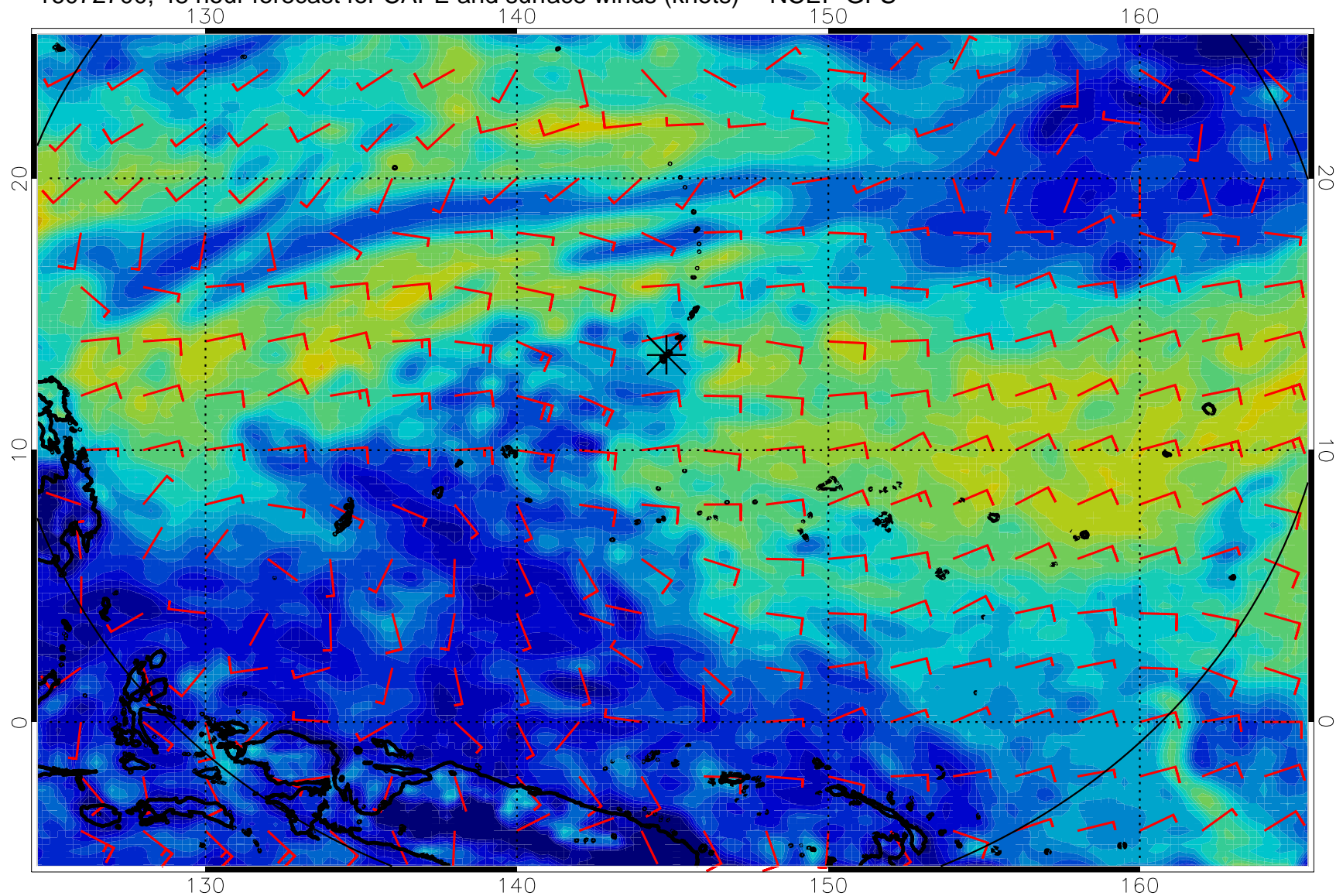
16072700, 48 hour forecast for CAPE and surface winds (knots) -- NCEP GFS
