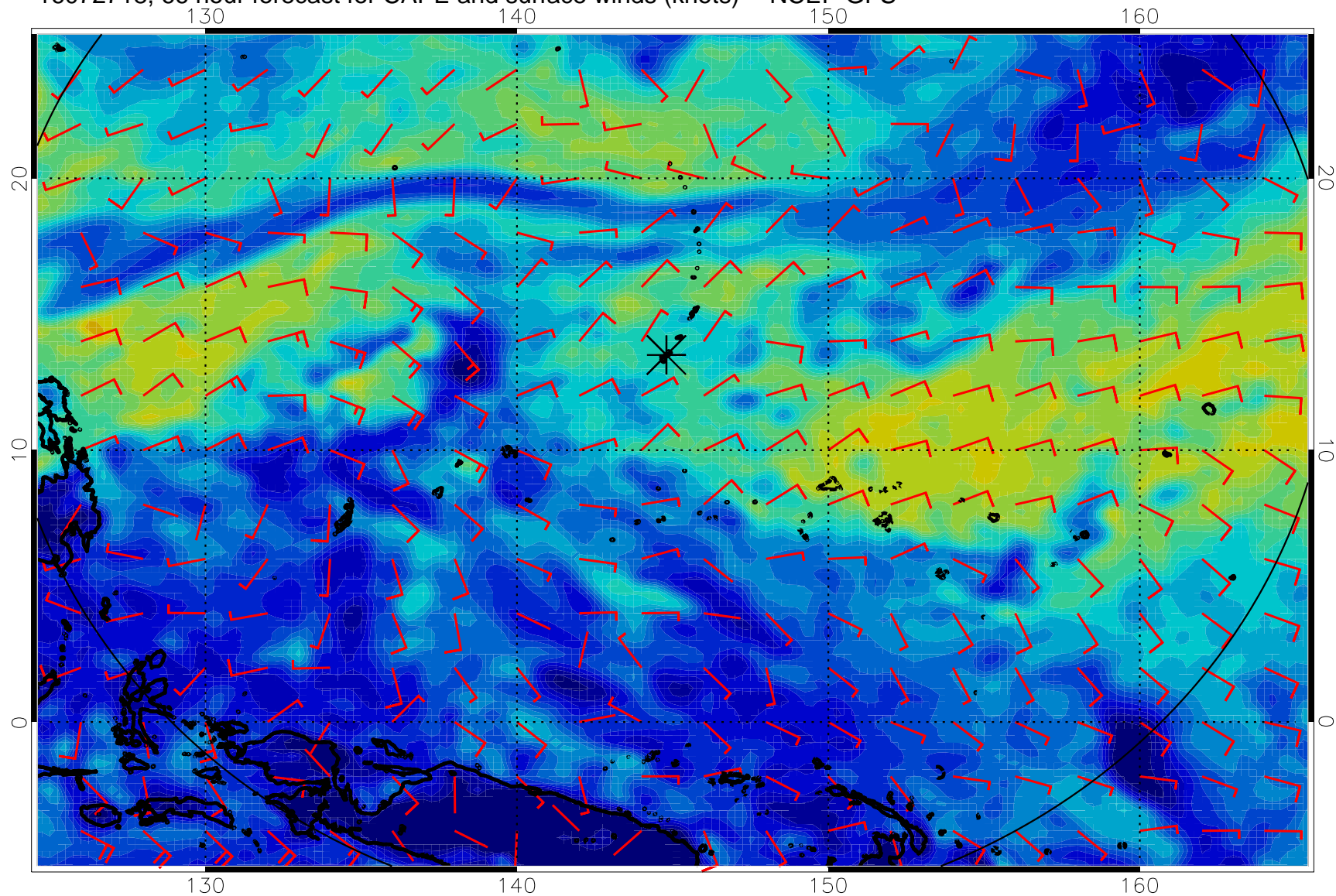
16072718, 66 hour forecast for CAPE and surface winds (knots) -- NCEP GFS
