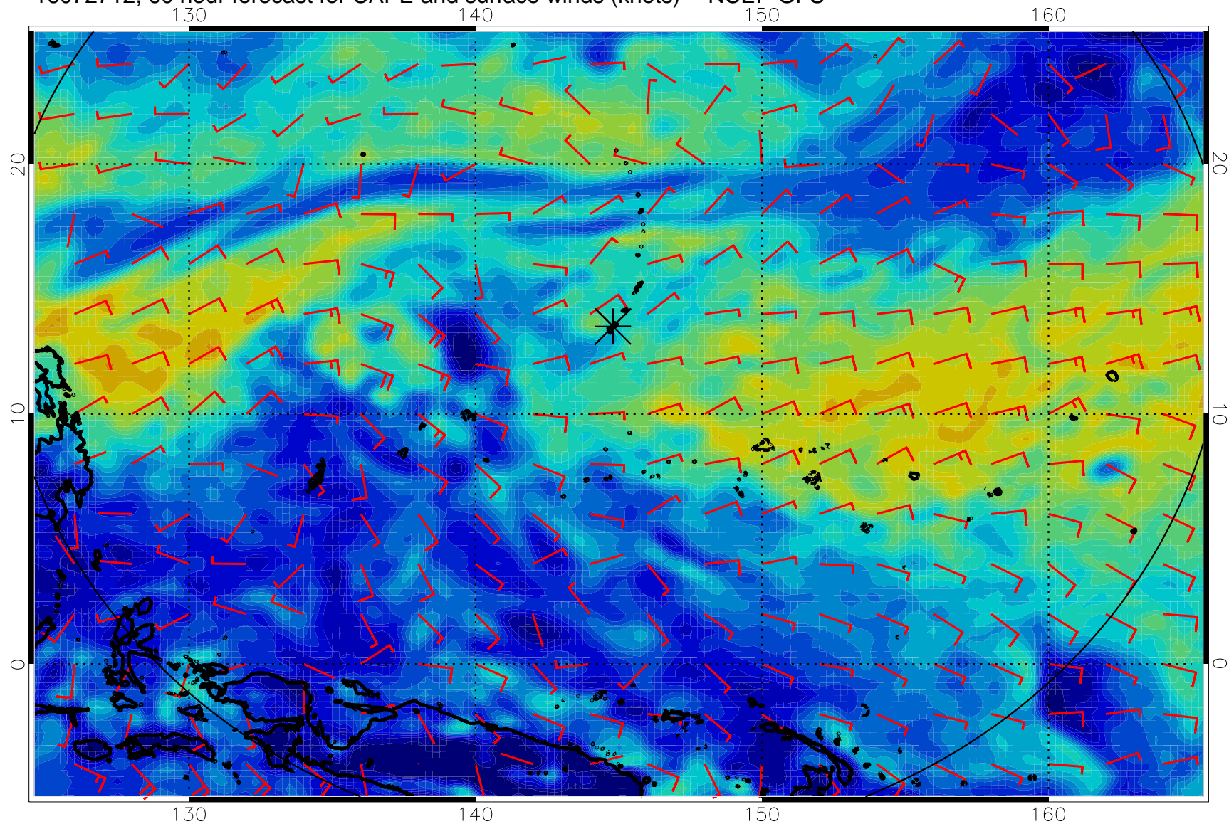
16072712, 60 hour forecast for CAPE and surface winds (knots) -- NCEP GFS
