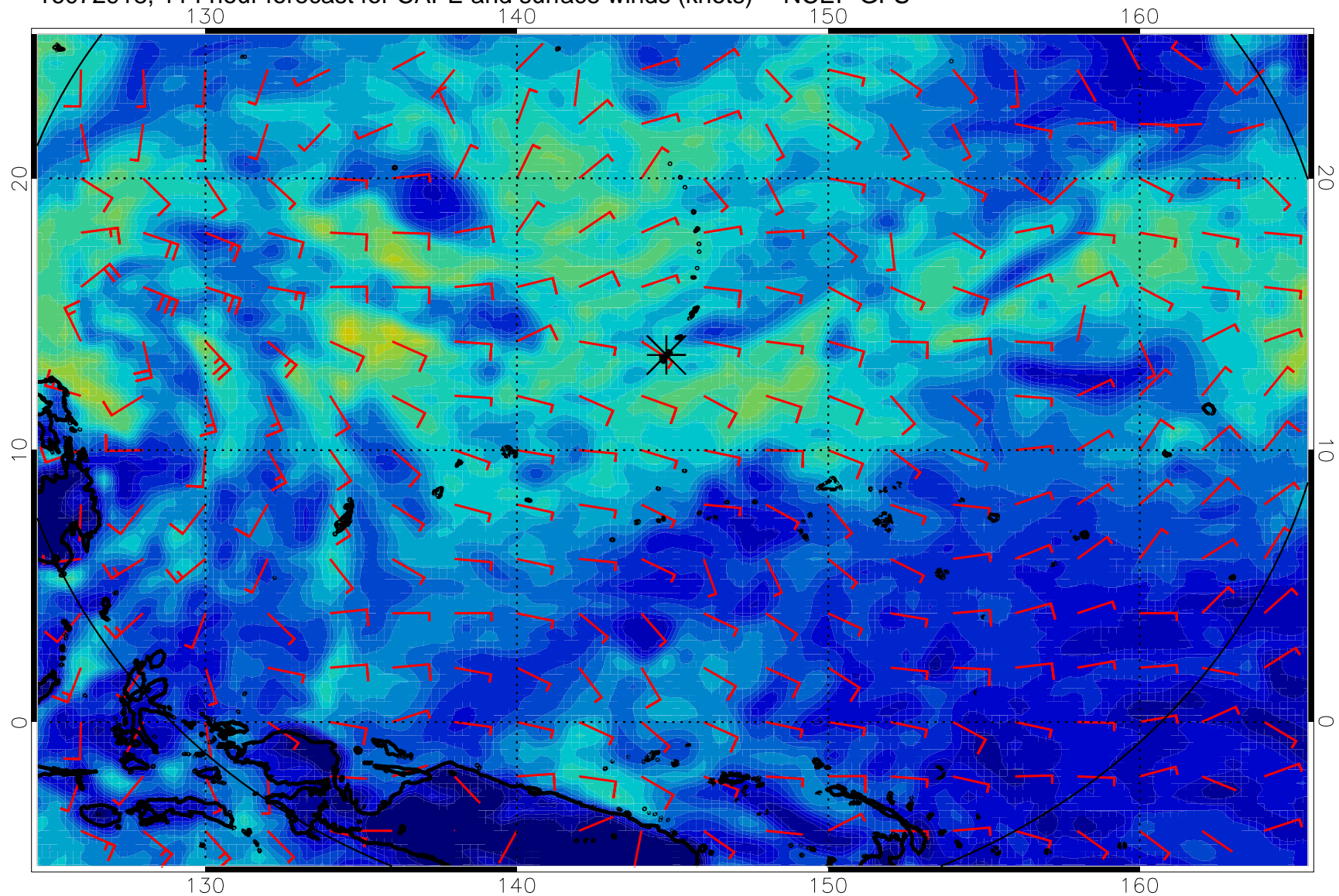
16072918, 114 hour forecast for CAPE and surface winds (knots) -- NCEP GFS
