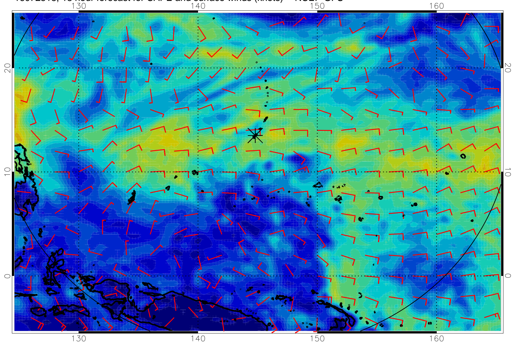
16072518, 18 hour forecast for CAPE and surface winds (knots) -- NCEP GFS
