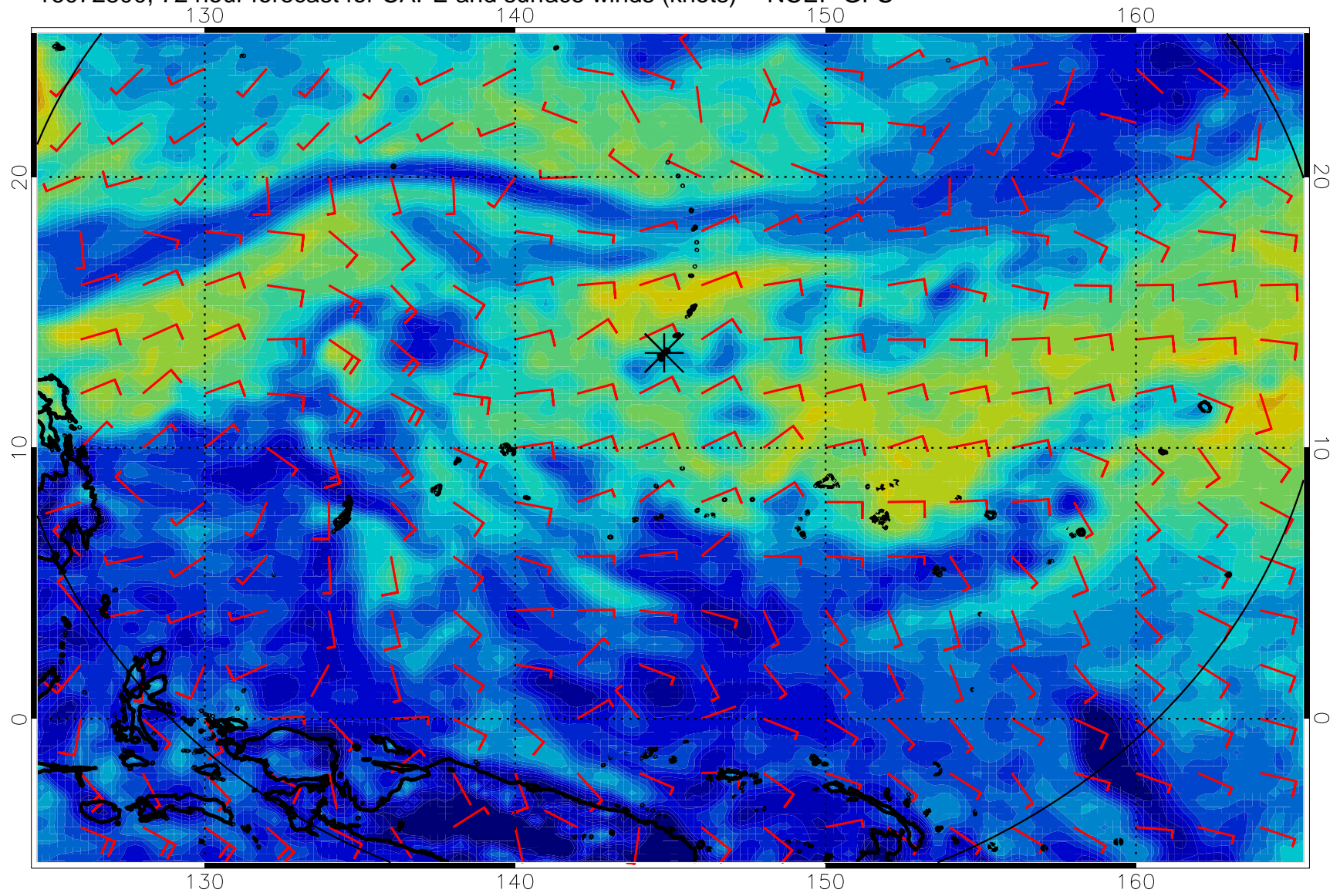
16072800, 72 hour forecast for CAPE and surface winds (knots) -- NCEP GFS
