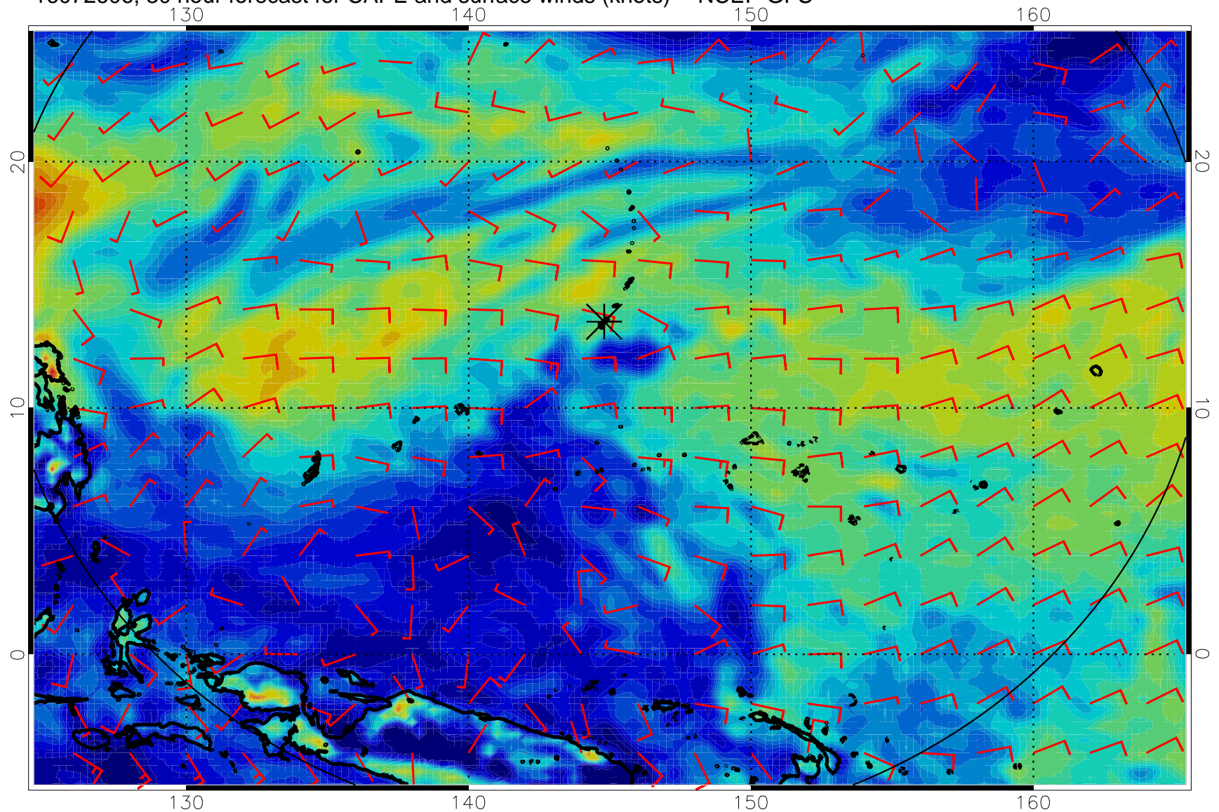
16072606, 30 hour forecast for CAPE and surface winds (knots) -- NCEP GFS
