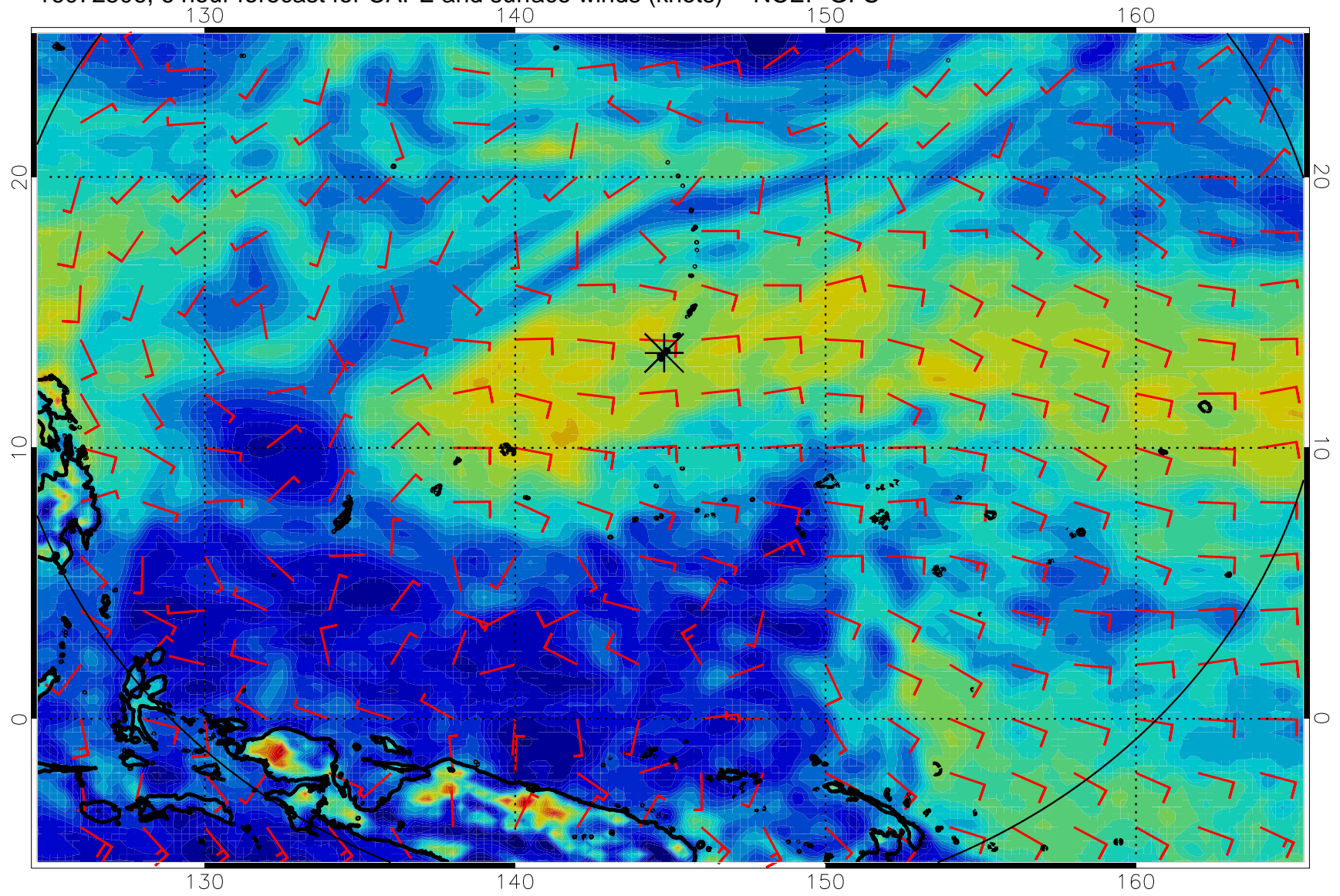
16072506, 6 hour forecast for CAPE and surface winds (knots) -- NCEP GFS
