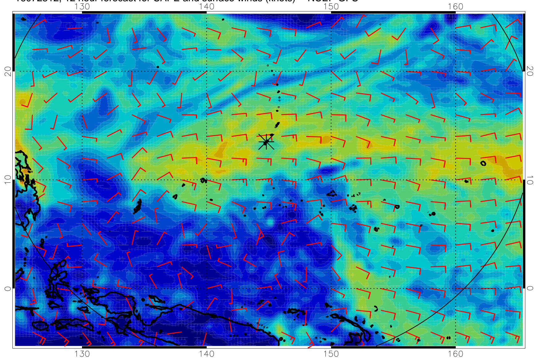
16072512, 12 hour forecast for CAPE and surface winds (knots) -- NCEP GFS
