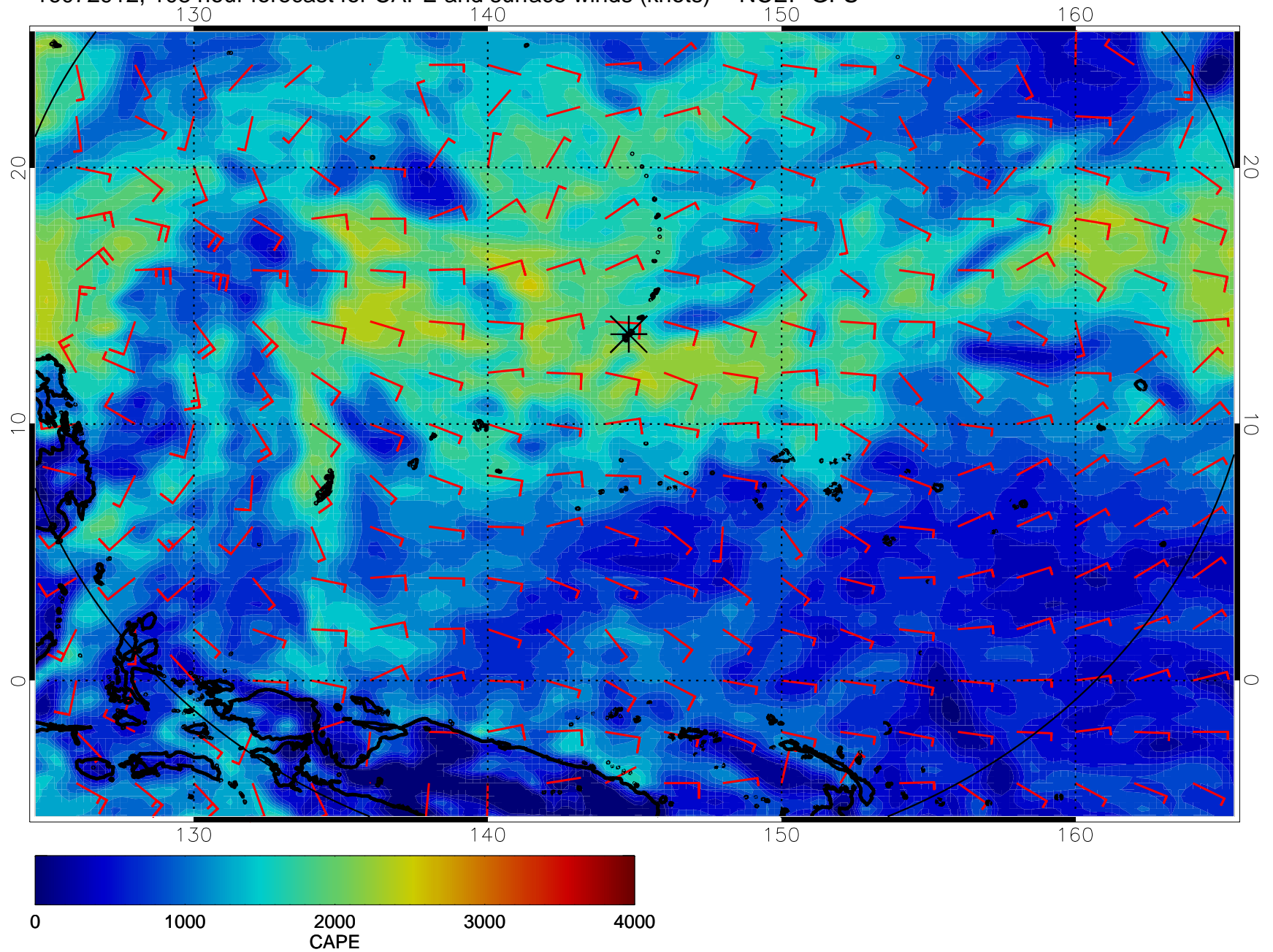
16072912, 108 hour forecast for CAPE and surface winds (knots) -- NCEP GFS
