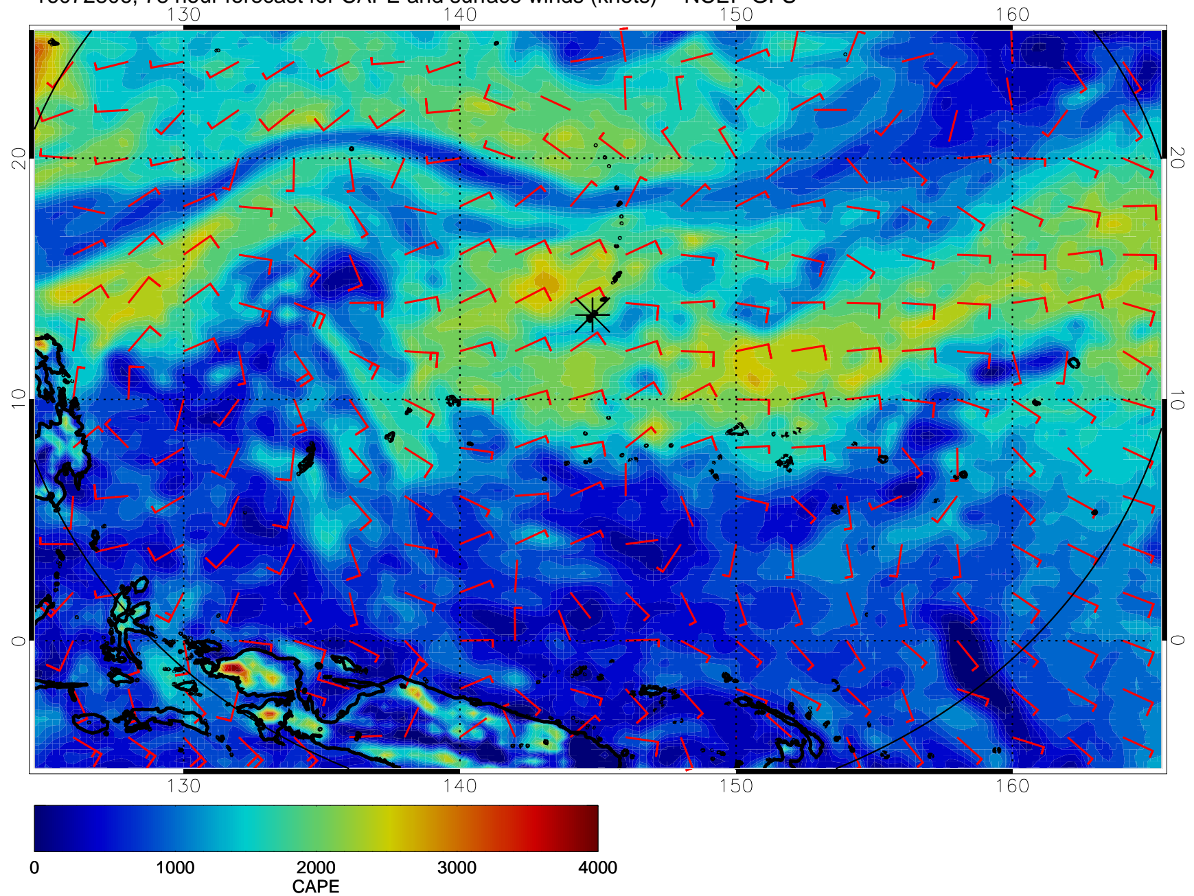
16072806, 78 hour forecast for CAPE and surface winds (knots) -- NCEP GFS
