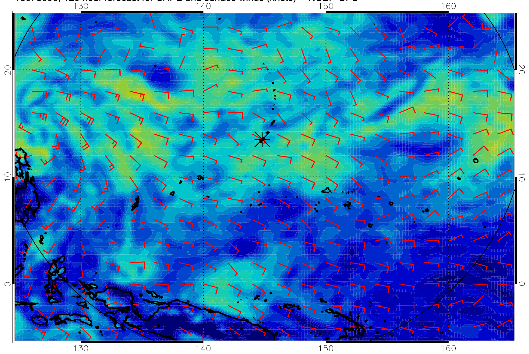
16073000, 120 hour forecast for CAPE and surface winds (knots) -- NCEP GFS
