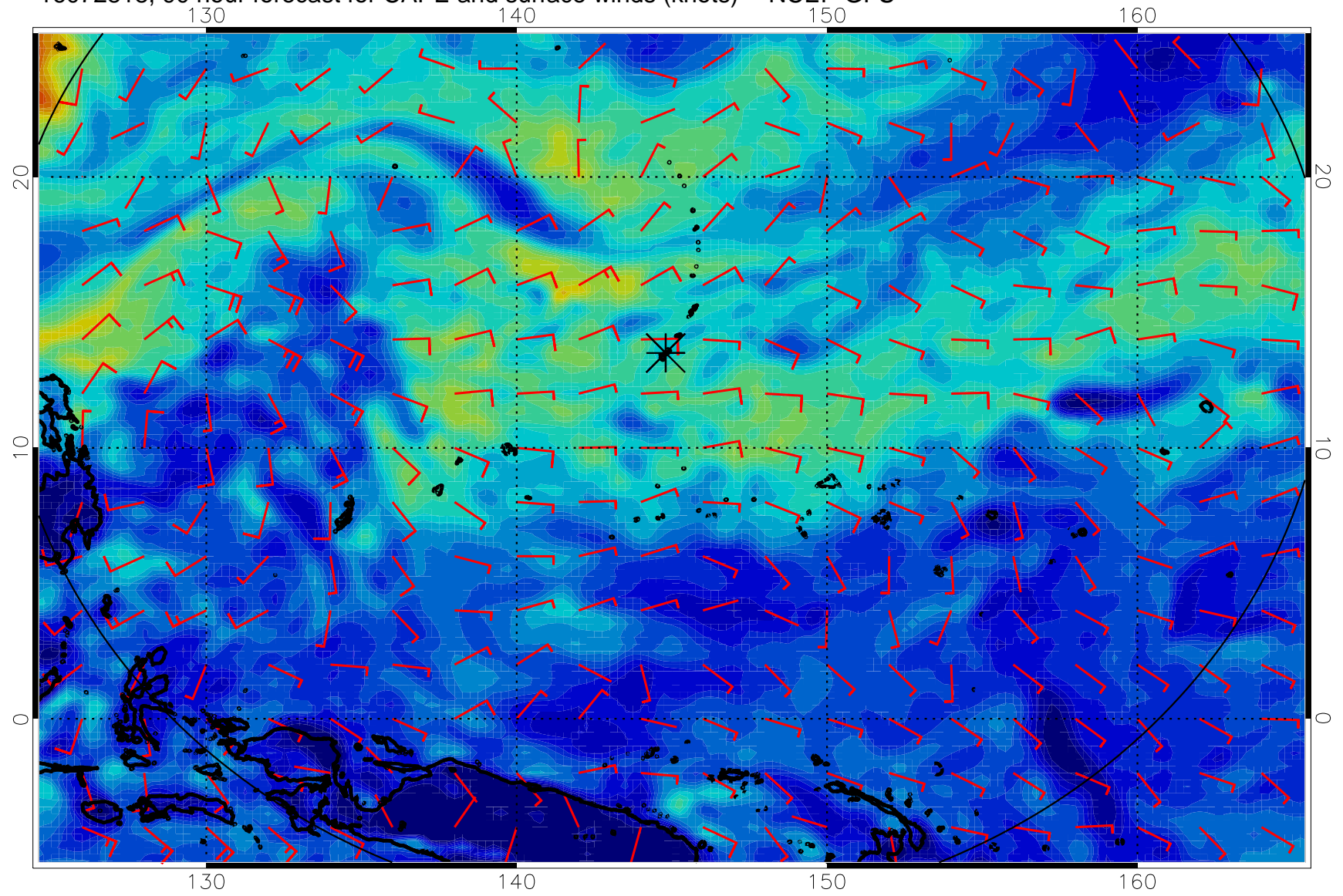
16072818, 90 hour forecast for CAPE and surface winds (knots) -- NCEP GFS
