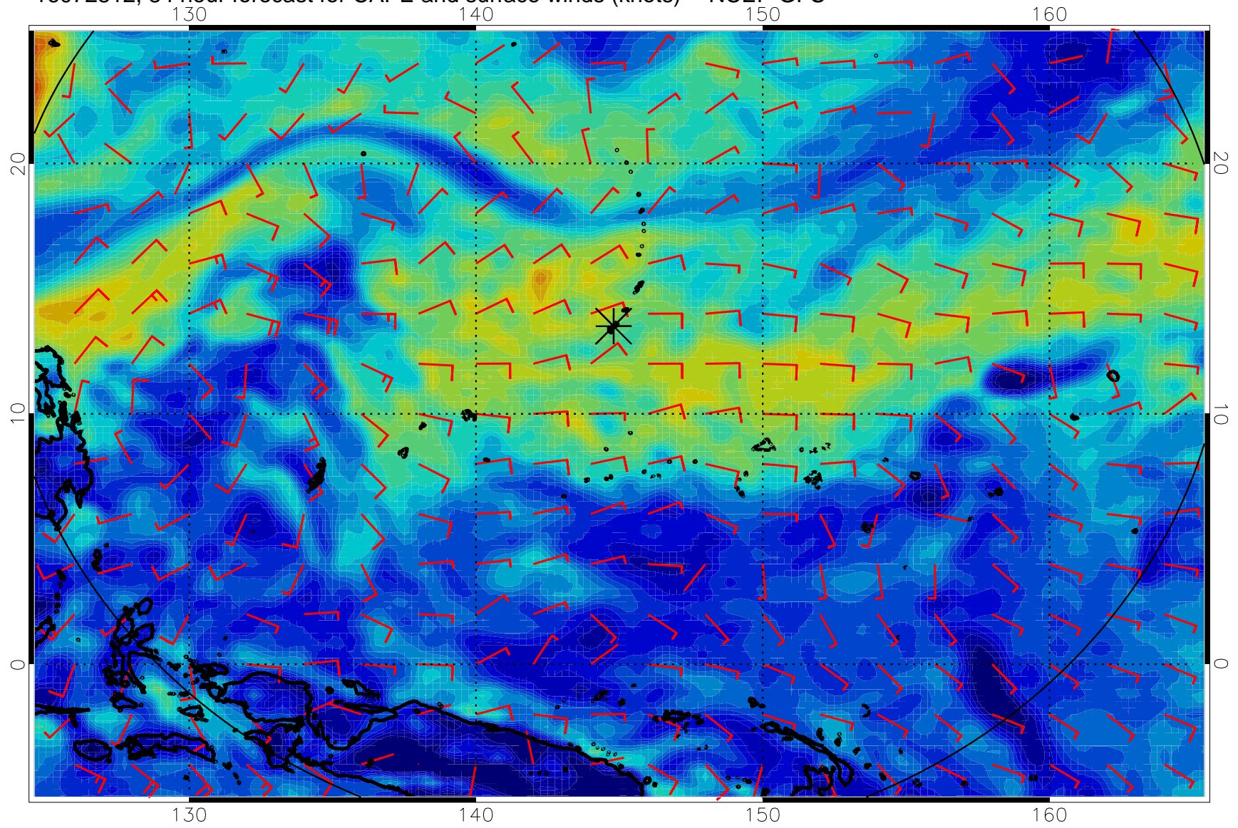
16072812, 84 hour forecast for CAPE and surface winds (knots) -- NCEP GFS
