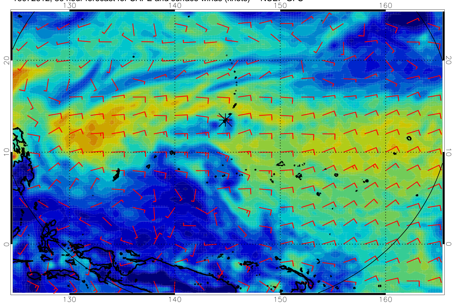
16072612, 36 hour forecast for CAPE and surface winds (knots) -- NCEP GFS
