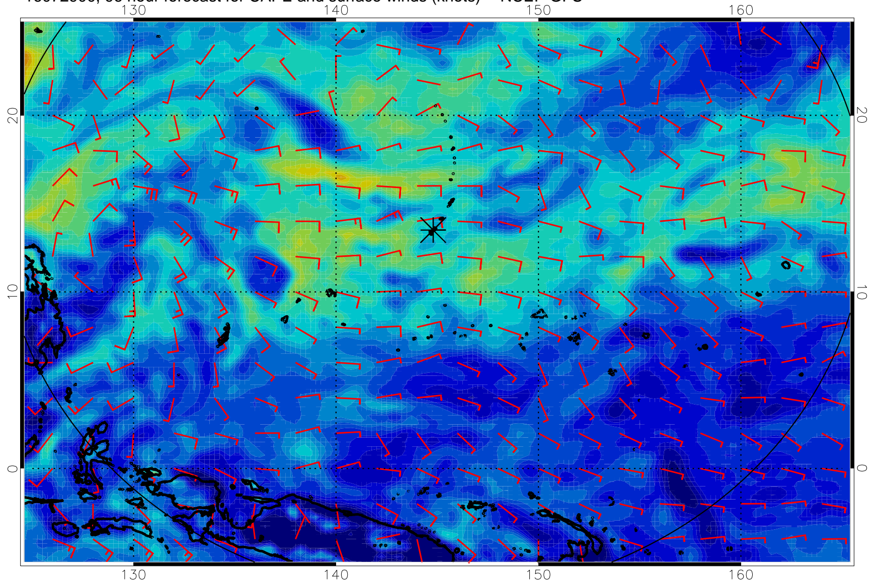
16072900, 96 hour forecast for CAPE and surface winds (knots) -- NCEP GFS
