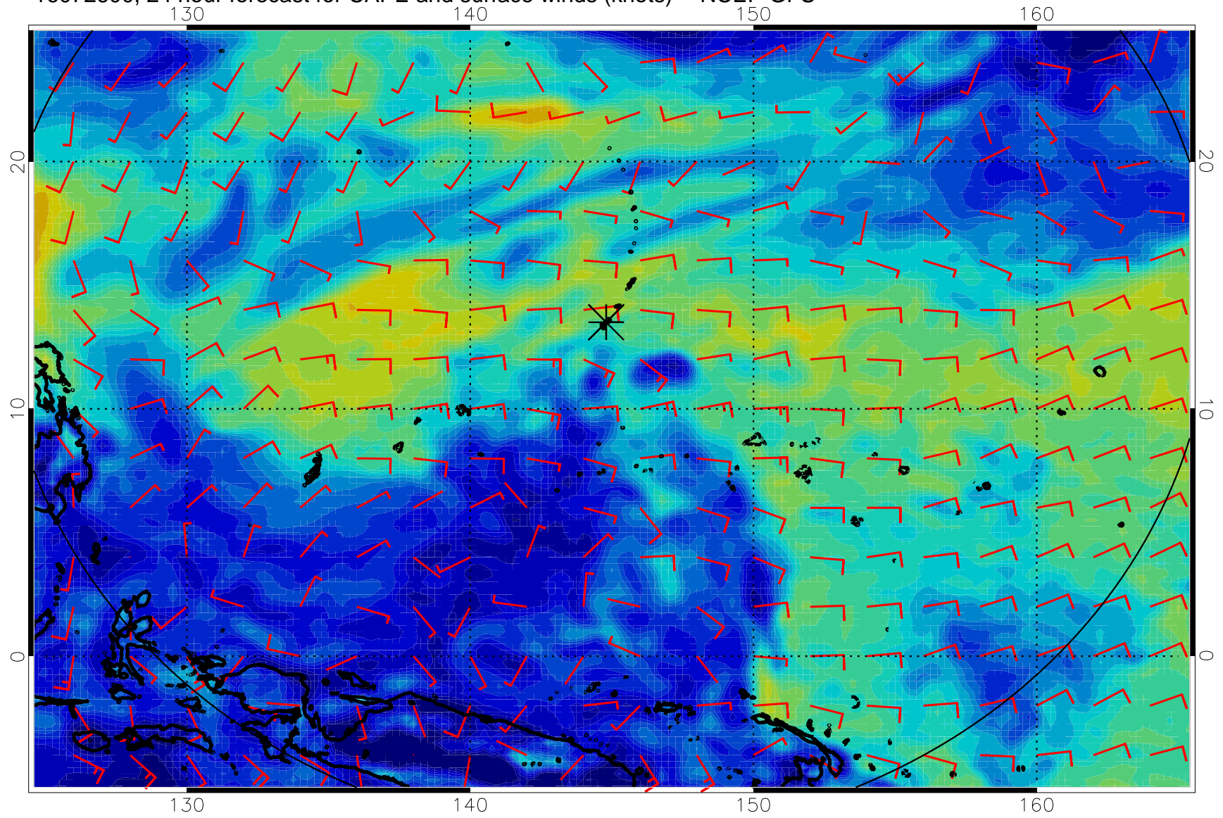
16072600, 24 hour forecast for CAPE and surface winds (knots) -- NCEP GFS
