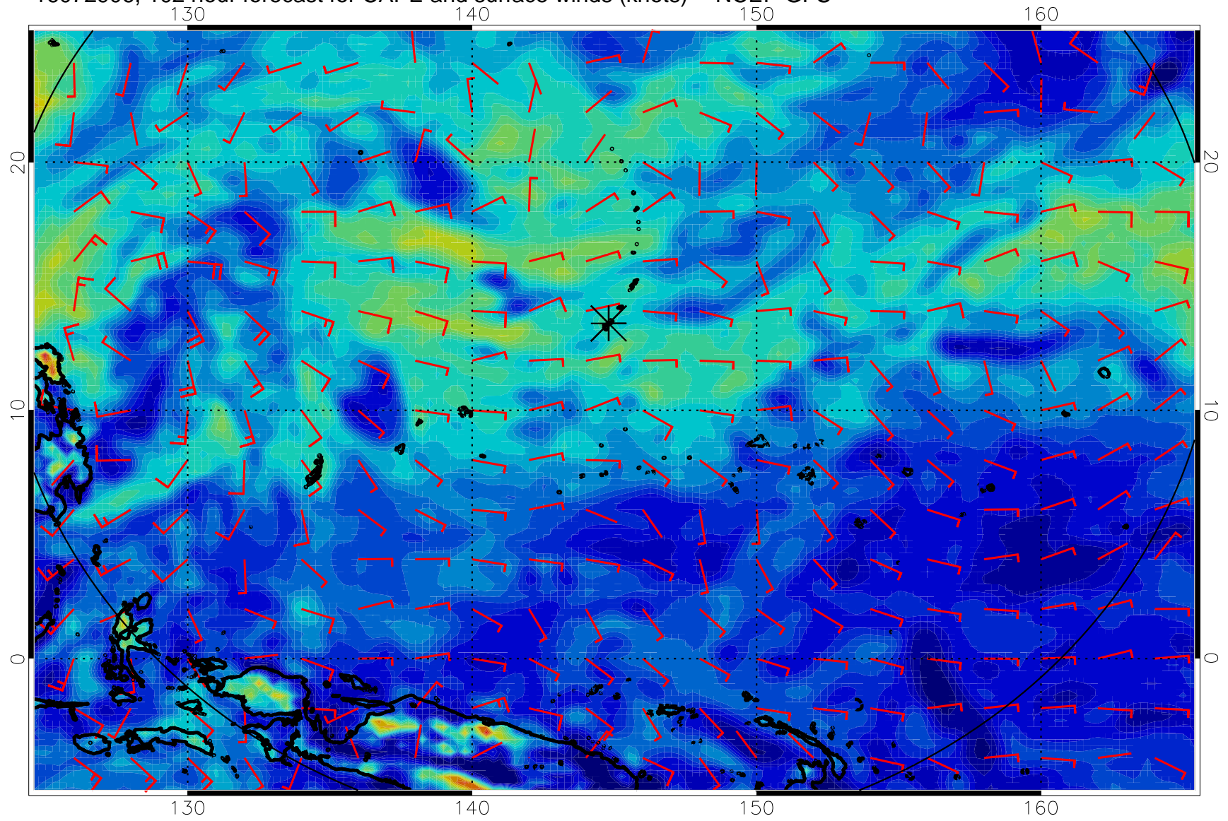
16072906, 102 hour forecast for CAPE and surface winds (knots) -- NCEP GFS
