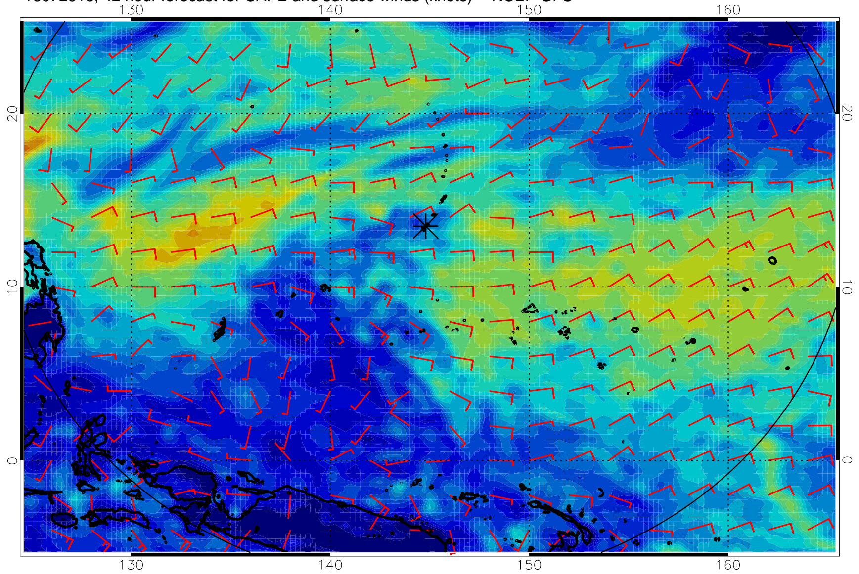
16072618, 42 hour forecast for CAPE and surface winds (knots) -- NCEP GFS
