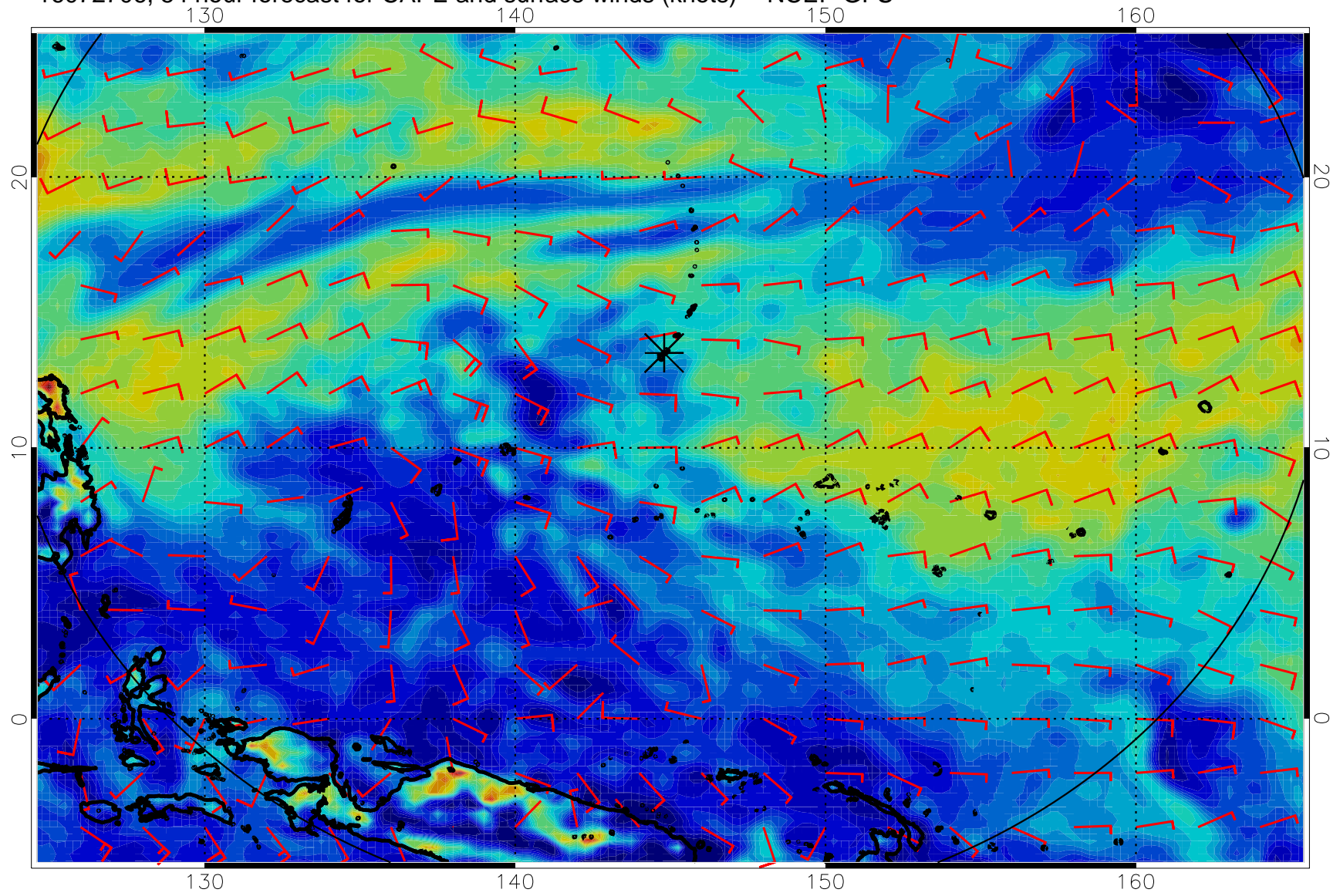
16072706, 54 hour forecast for CAPE and surface winds (knots) -- NCEP GFS
