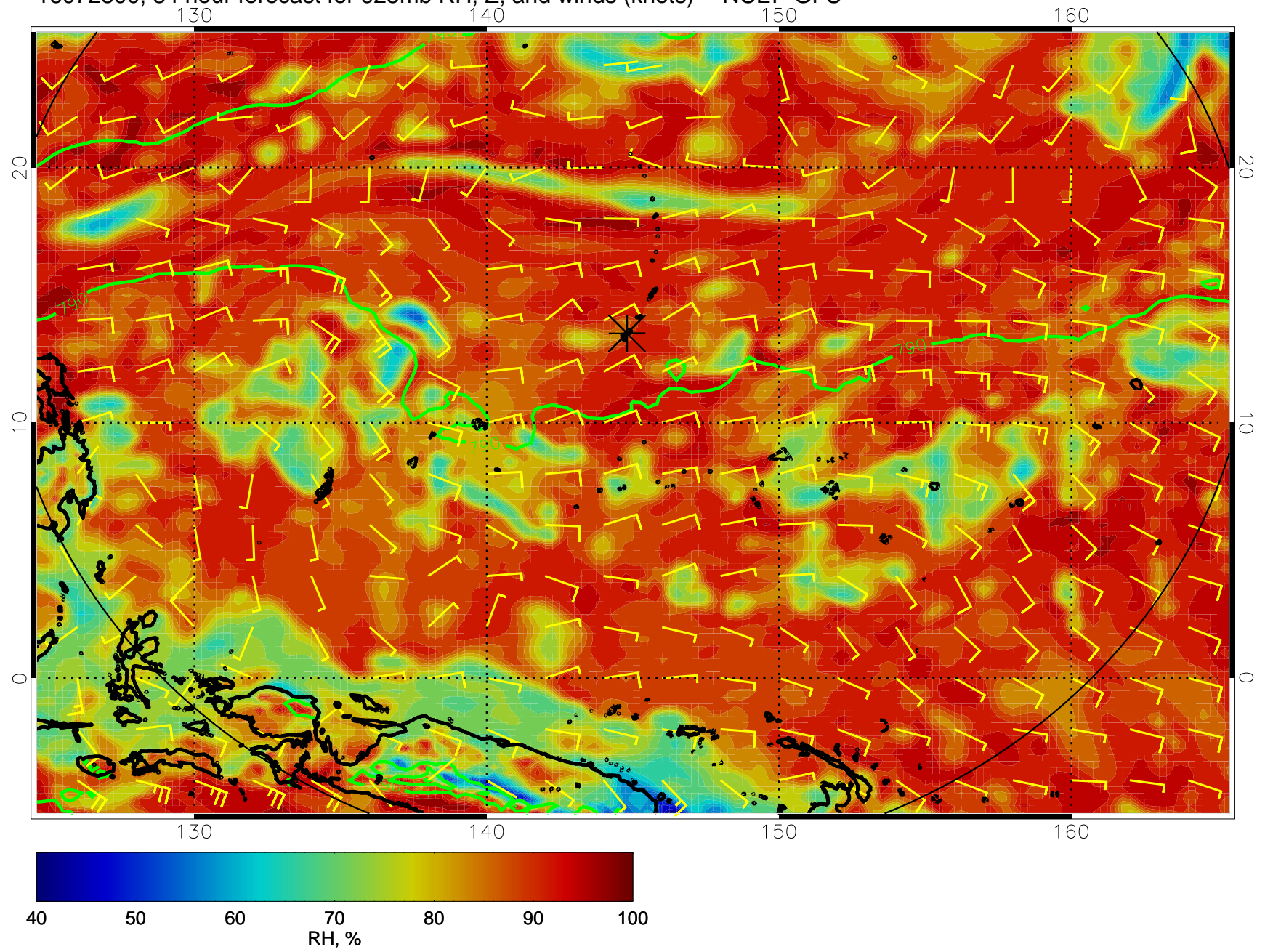
16072800, 84 hour forecast for 925mb RH, Z, and winds (knots) -- NCEP GFS
