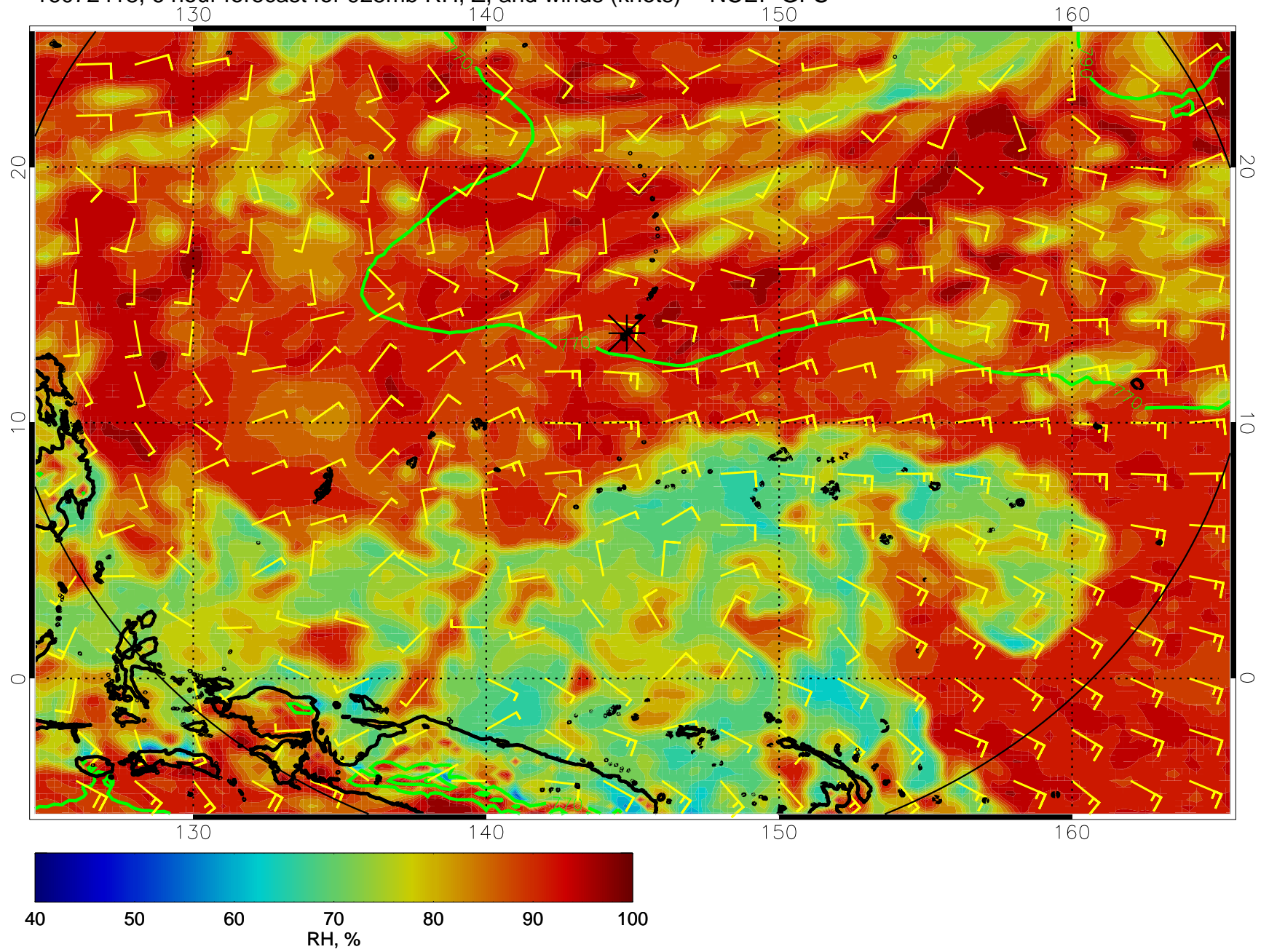
16072418, 6 hour forecast for 925mb RH, Z, and winds (knots) -- NCEP GFS
