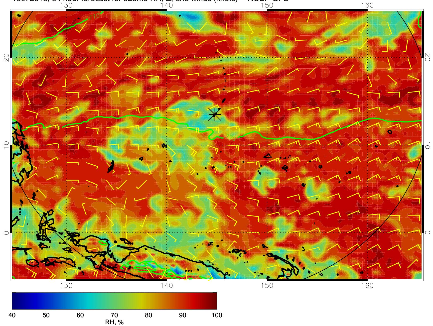
16072618, 54 hour forecast for 925mb RH, Z, and winds (knots) -- NCEP GFS
