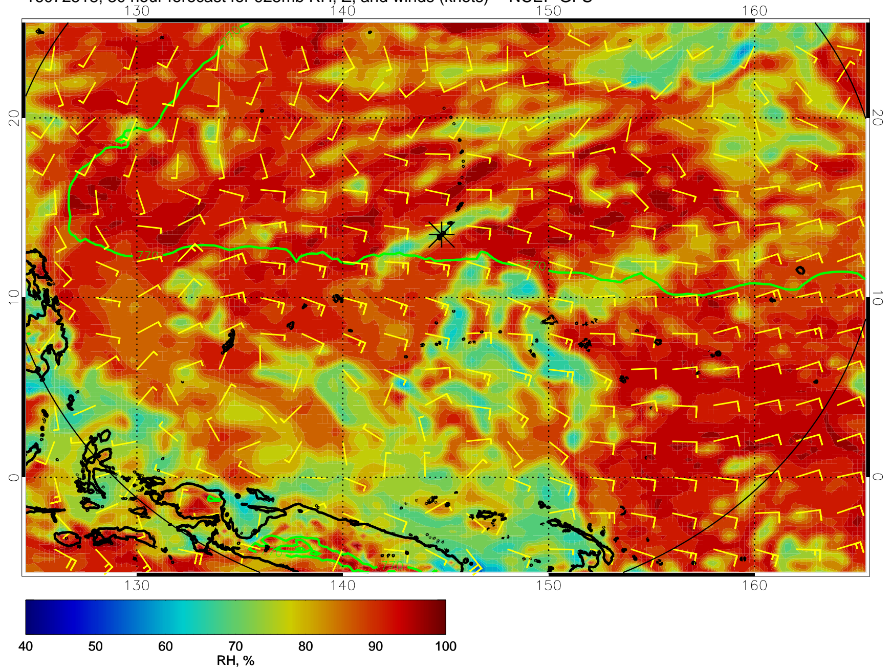
16072518, 30 hour forecast for 925mb RH, Z, and winds (knots) -- NCEP GFS
