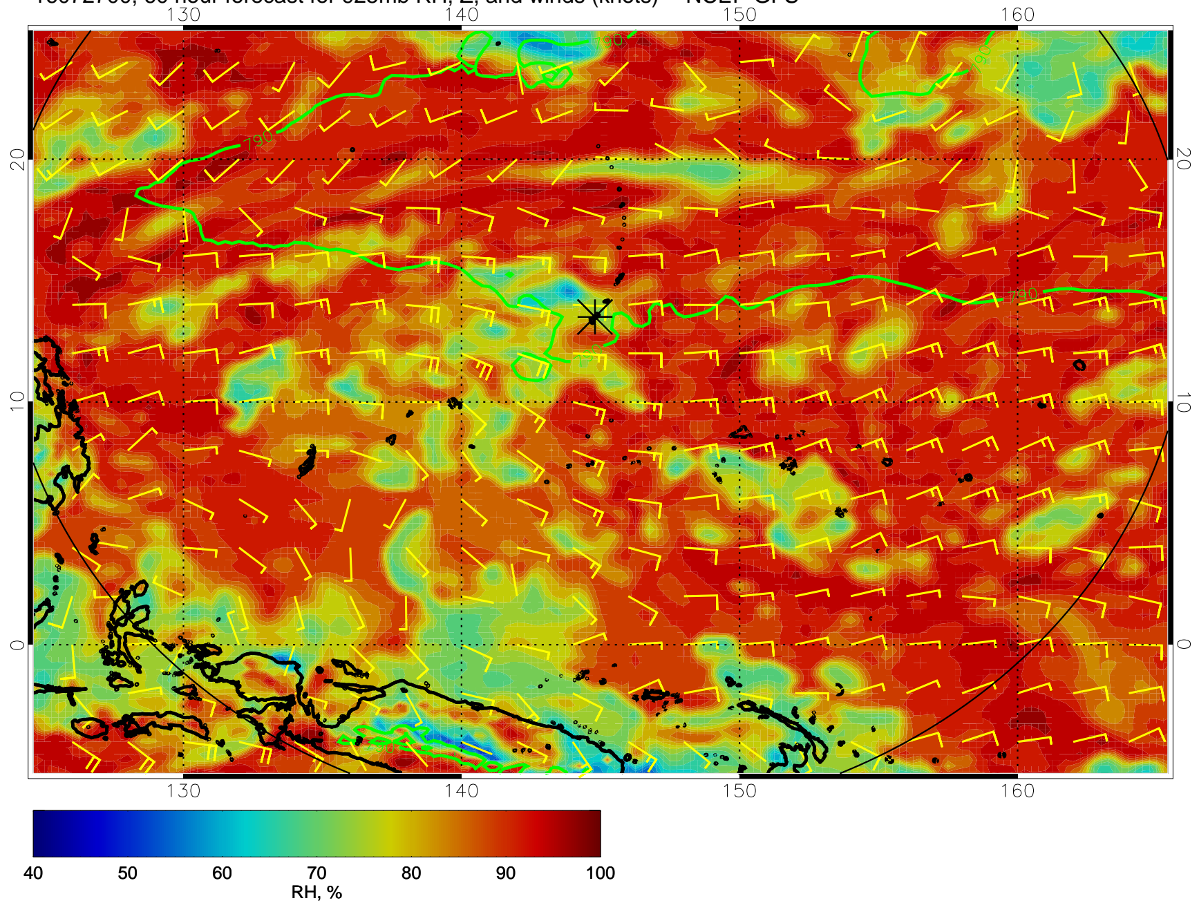
16072700, 60 hour forecast for 925mb RH, Z, and winds (knots) -- NCEP GFS
