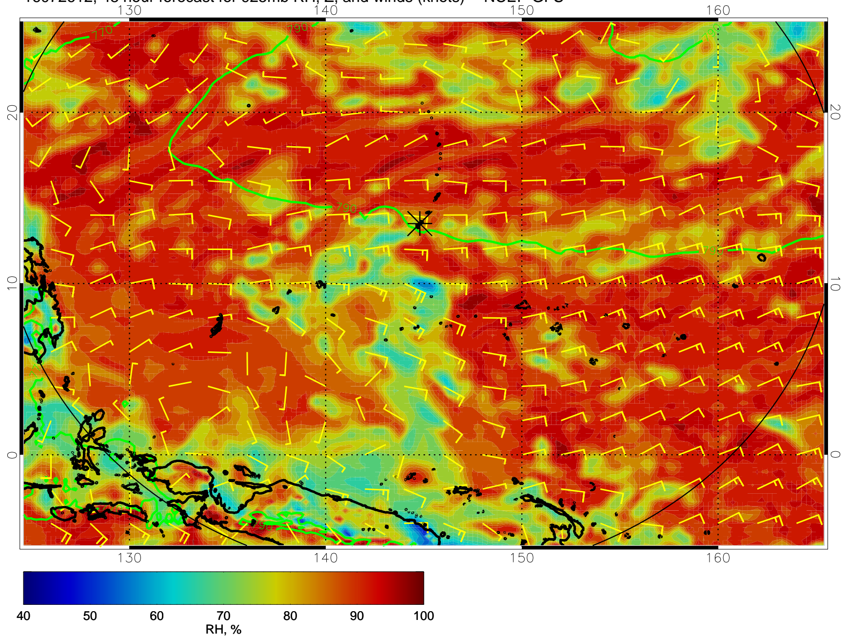
16072612, 48 hour forecast for 925mb RH, Z, and winds (knots) -- NCEP GFS
