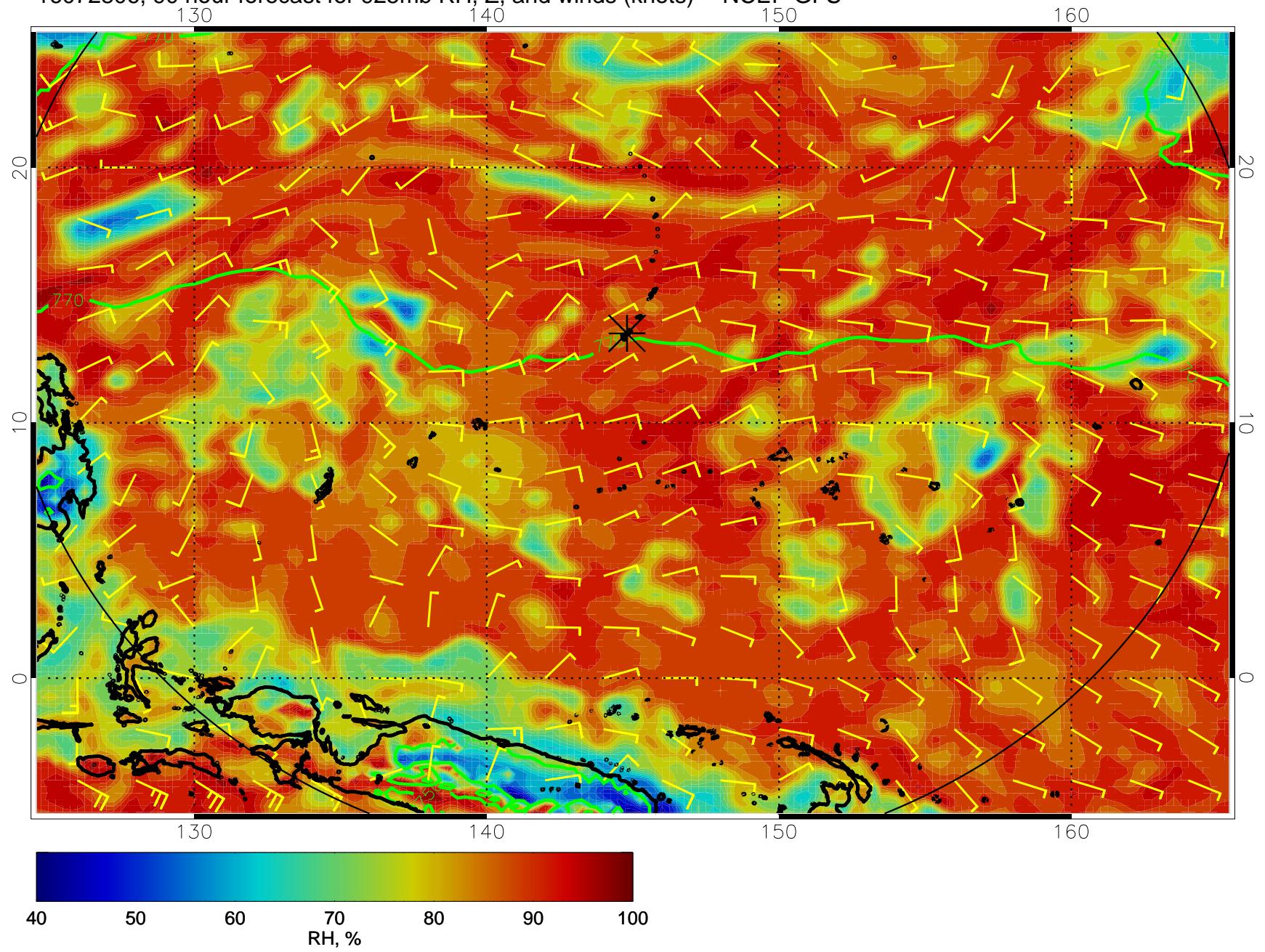
16072806, 90 hour forecast for 925mb RH, Z, and winds (knots) -- NCEP GFS
