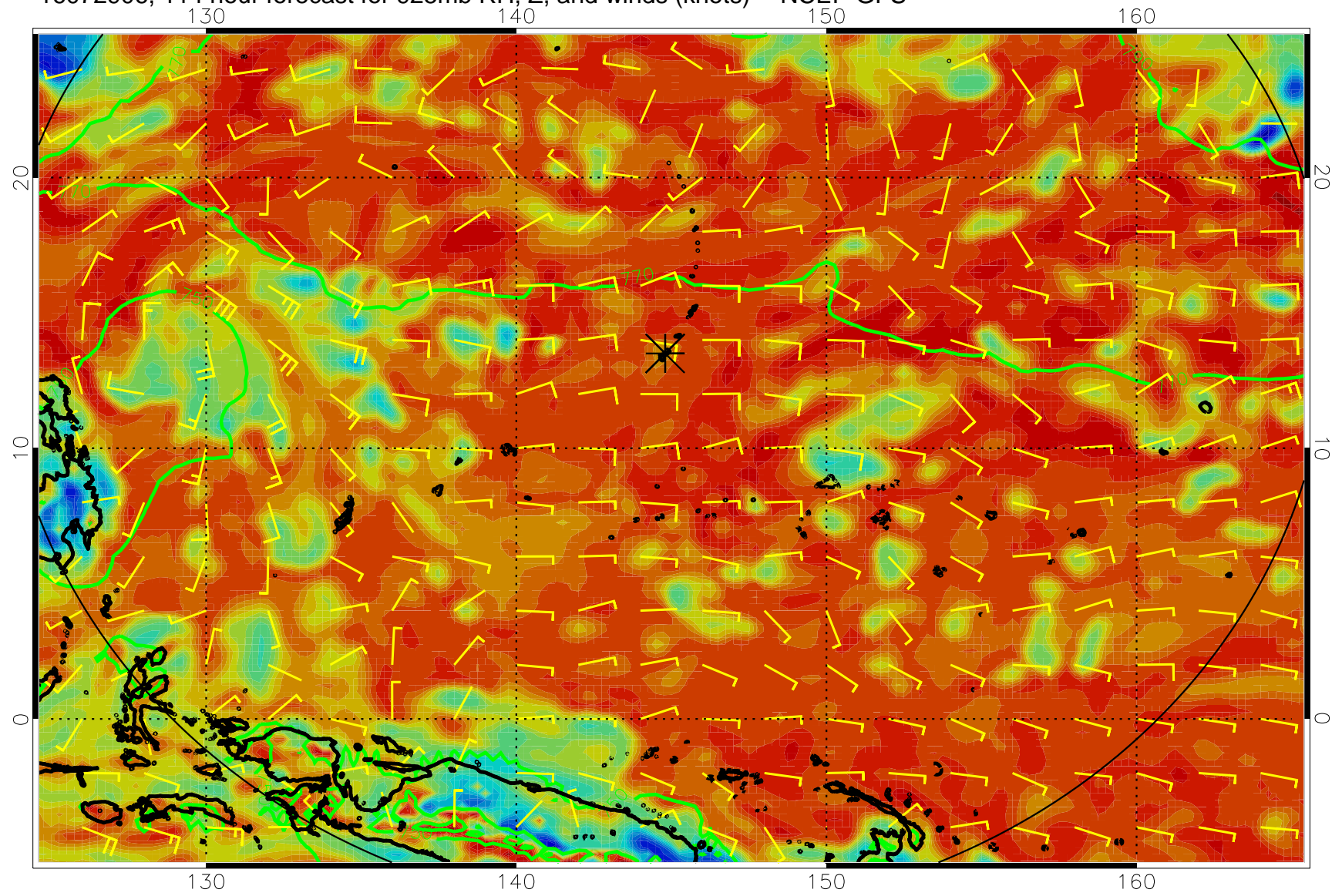
16072906, 114 hour forecast for 925mb RH, Z, and winds (knots) -- NCEP GFS
