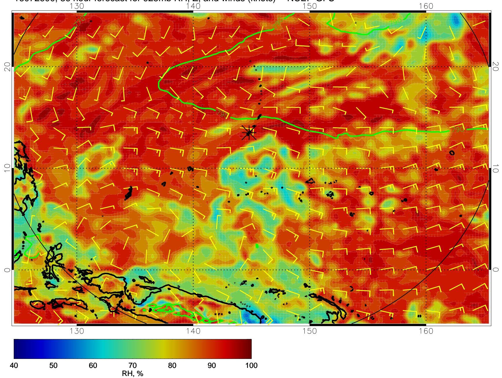
16072600, 36 hour forecast for 925mb RH, Z, and winds (knots) -- NCEP GFS
