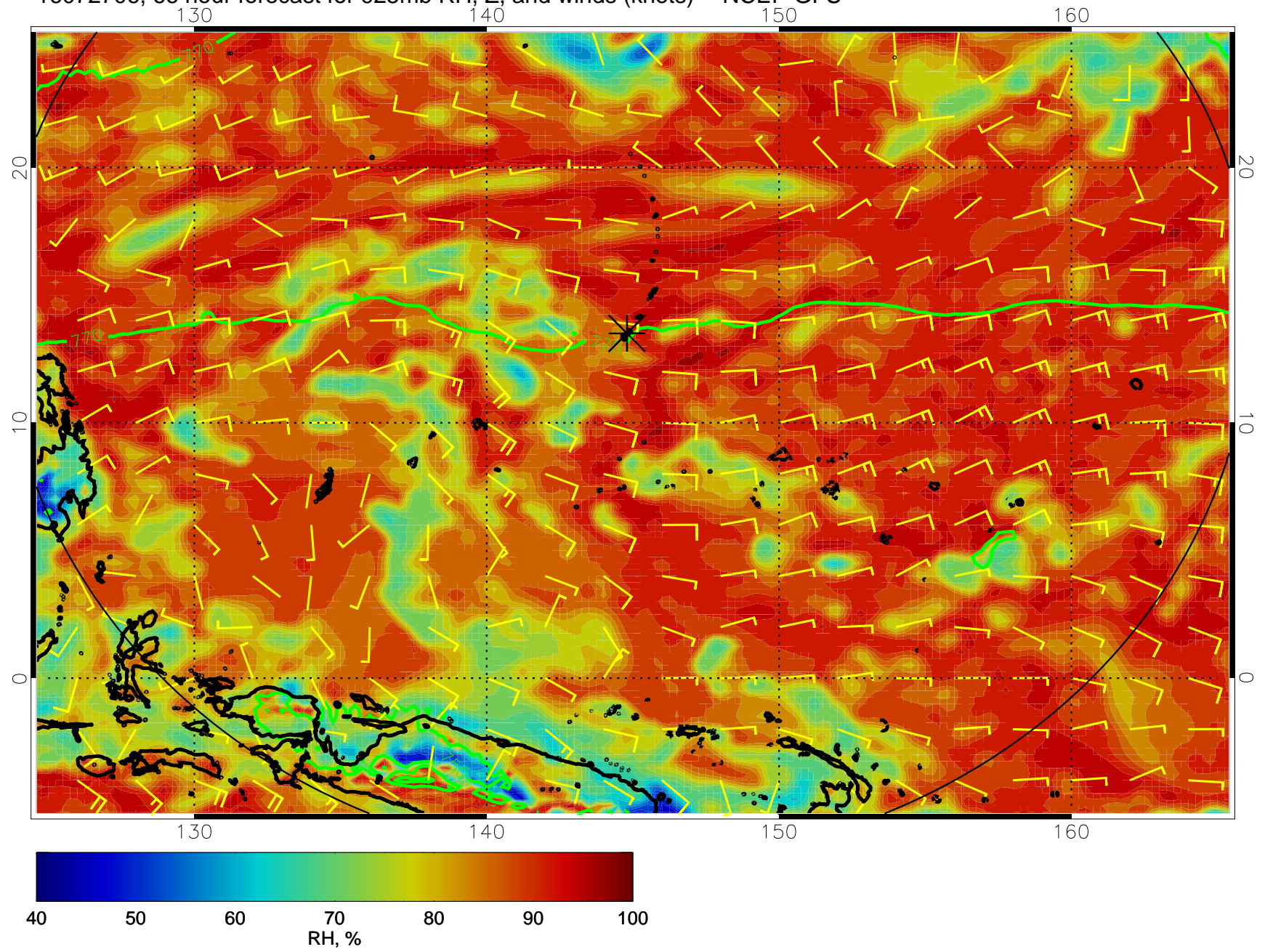
16072706, 66 hour forecast for 925mb RH, Z, and winds (knots) -- NCEP GFS
