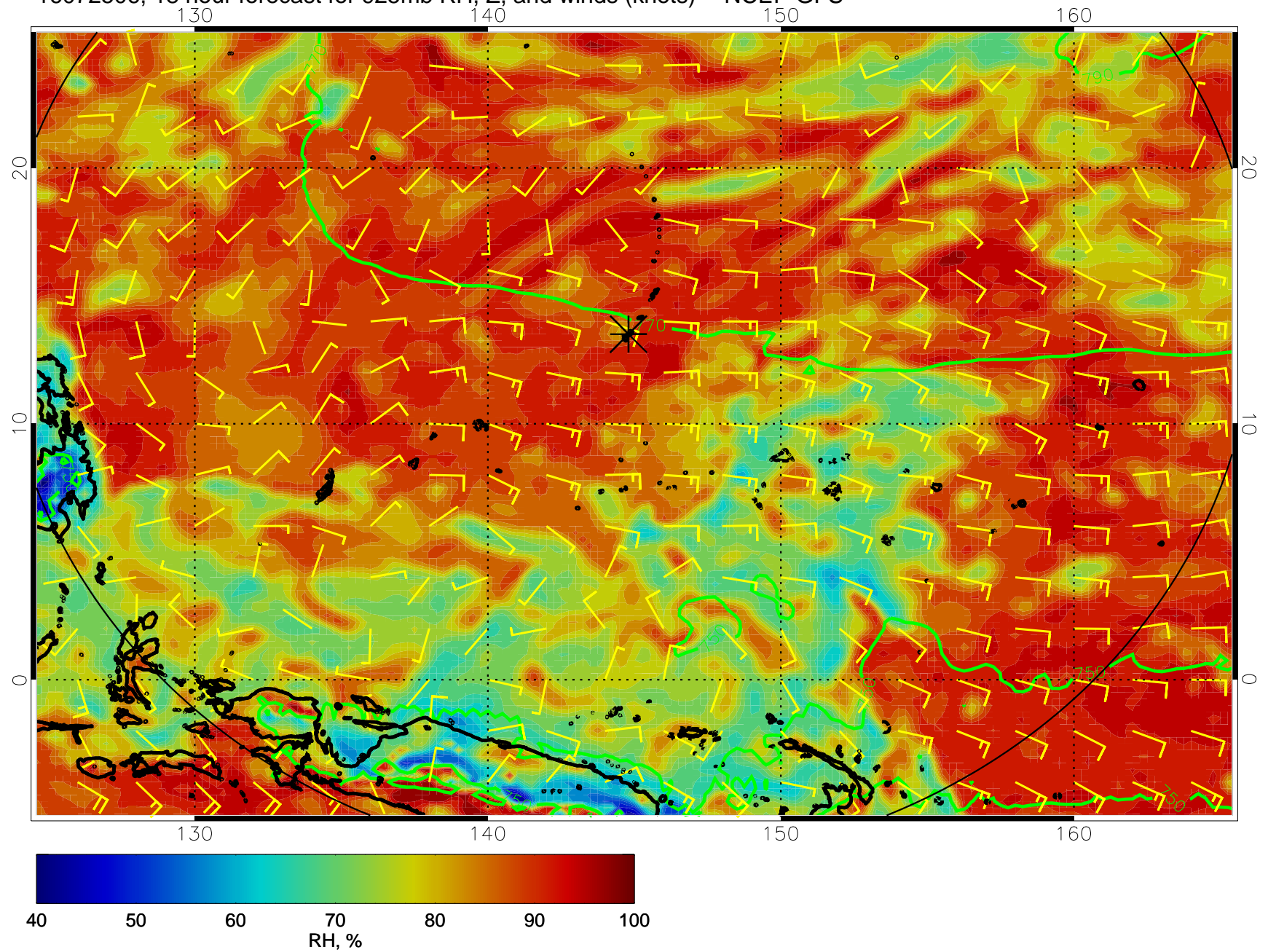
16072506, 18 hour forecast for 925mb RH, Z, and winds (knots) -- NCEP GFS
