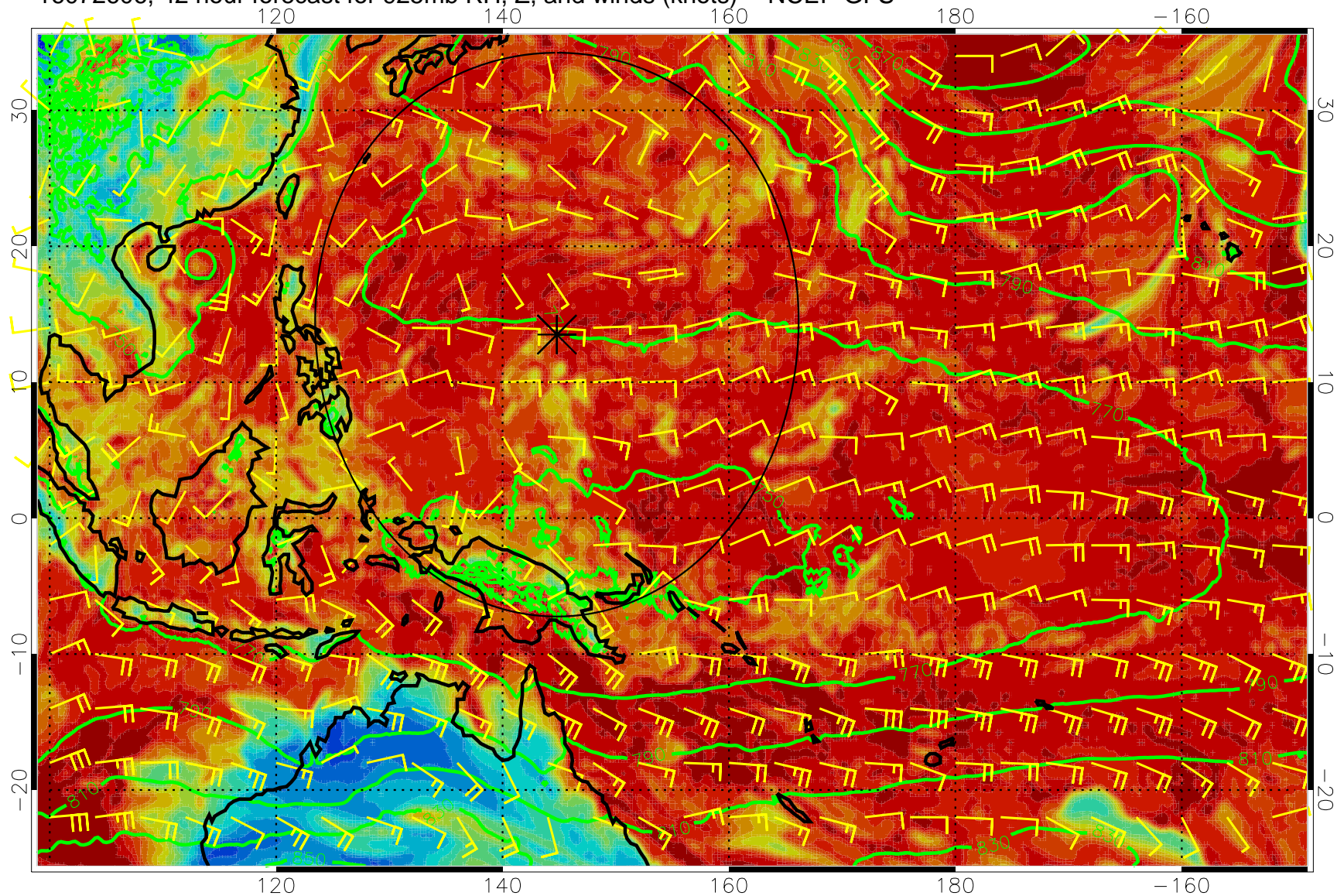
16072606, 42 hour forecast for 925mb RH, Z, and winds (knots) -- NCEP GFS
