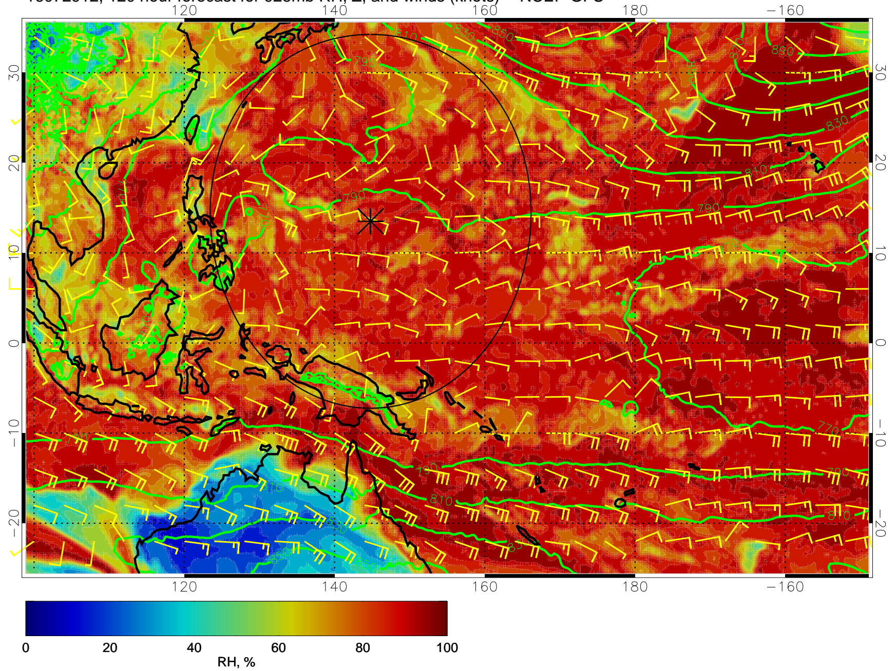
16072912, 120 hour forecast for 925mb RH, Z, and winds (knots) -- NCEP GFS
