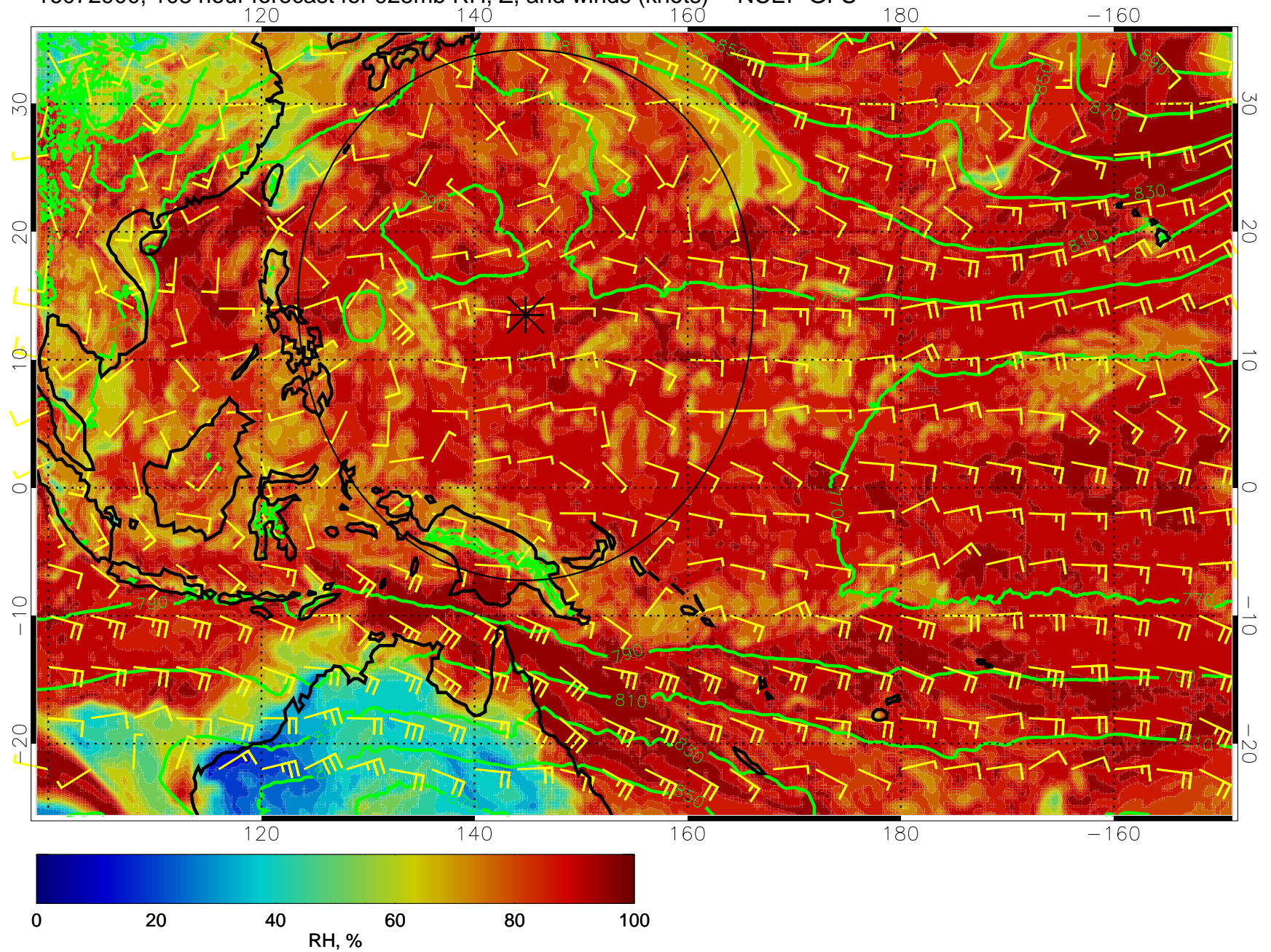
16072900, 108 hour forecast for 925mb RH, Z, and winds (knots) -- NCEP GFS
