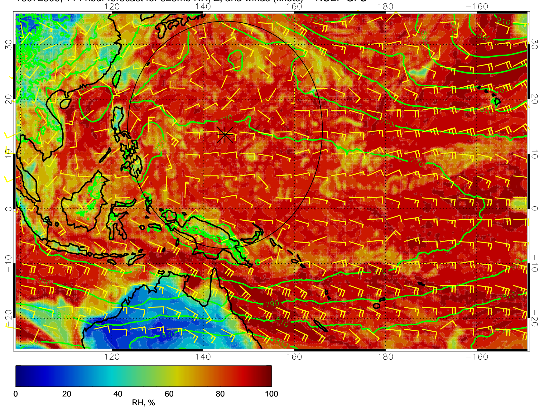
16072906, 114 hour forecast for 925mb RH, Z, and winds (knots) -- NCEP GFS
