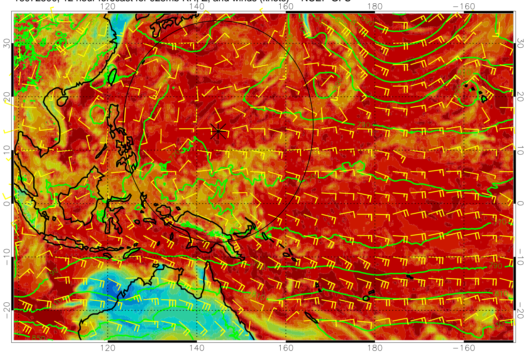
16072500, 12 hour forecast for 925mb RH, Z, and winds (knots) -- NCEP GFS
