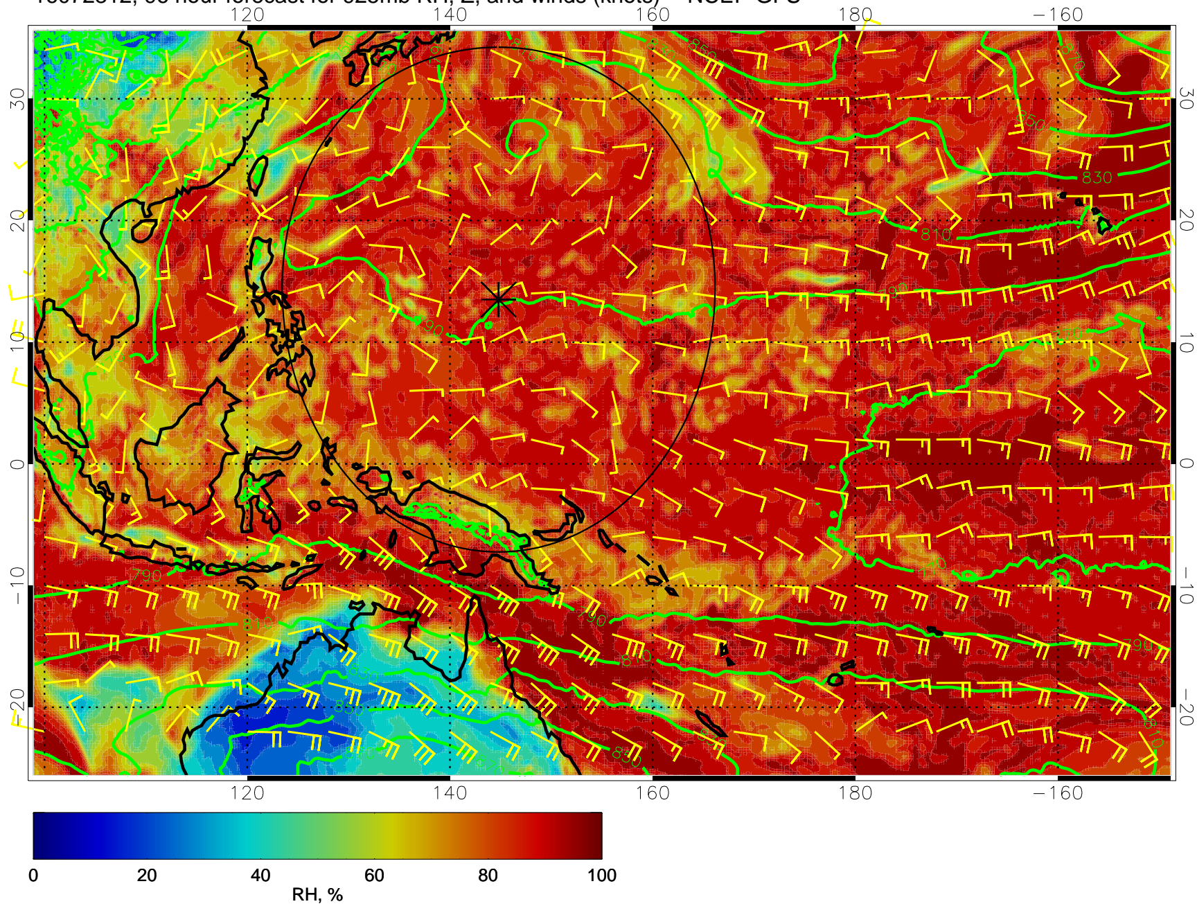
16072812, 96 hour forecast for 925mb RH, Z, and winds (knots) -- NCEP GFS
