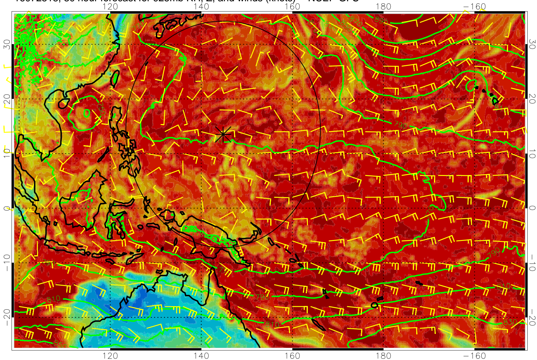
16072518, 30 hour forecast for 925mb RH, Z, and winds (knots) -- NCEP GFS
