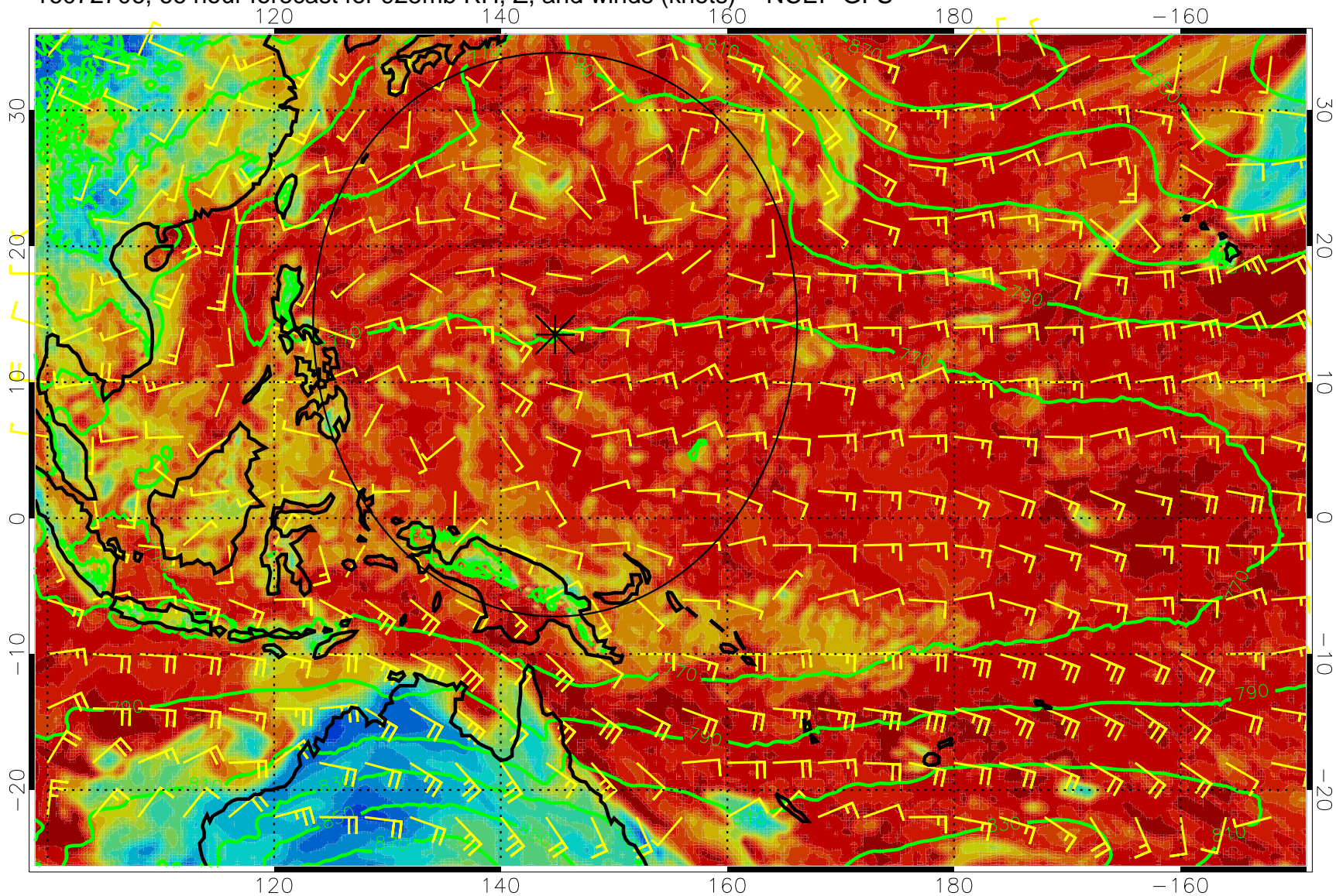
16072706, 66 hour forecast for 925mb RH, Z, and winds (knots) -- NCEP GFS
