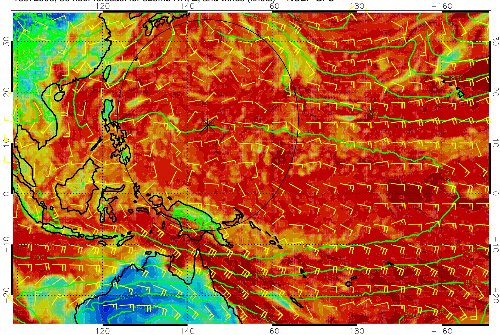
16072806, 90 hour forecast for 925mb RH, Z, and winds (knots) -- NCEP GFS
