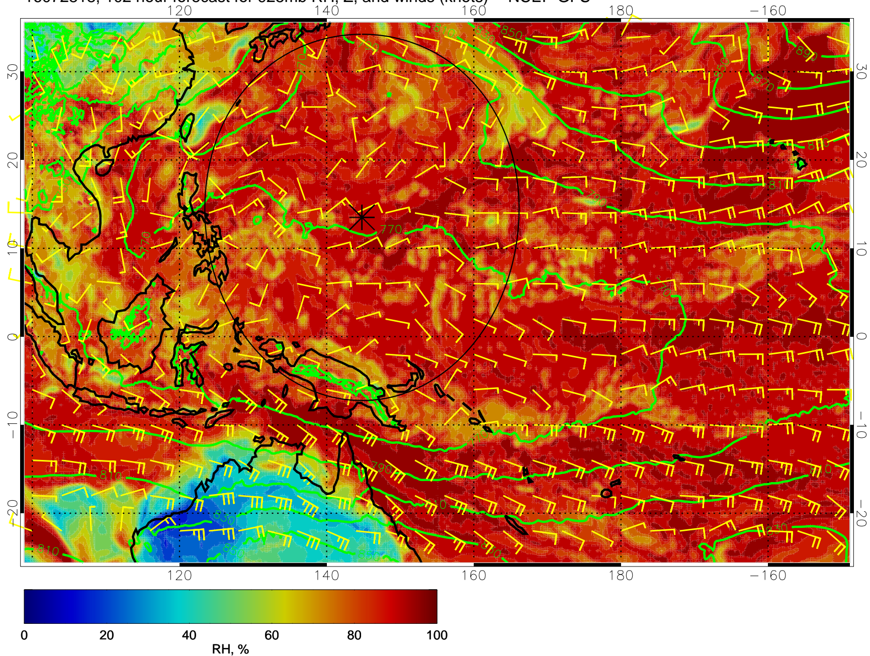
16072818, 102 hour forecast for 925mb RH, Z, and winds (knots) -- NCEP GFS
