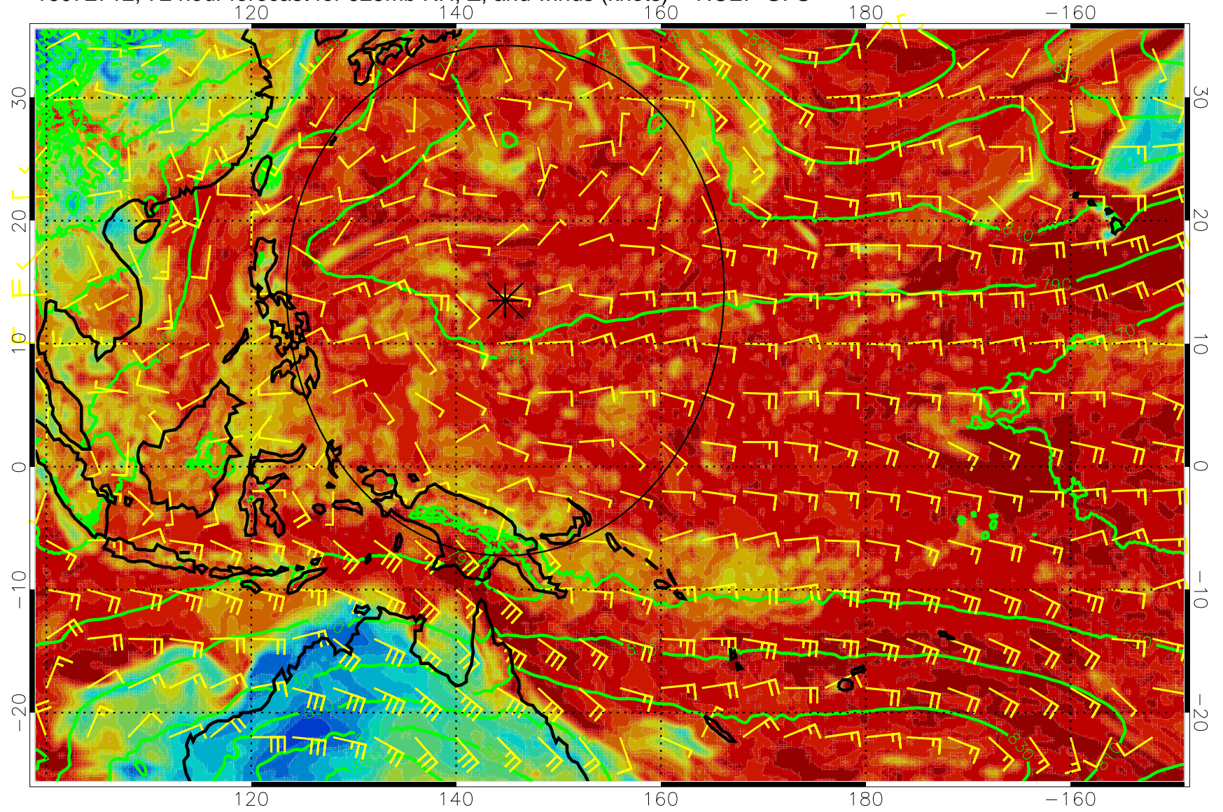
16072712, 72 hour forecast for 925mb RH, Z, and winds (knots) -- NCEP GFS
