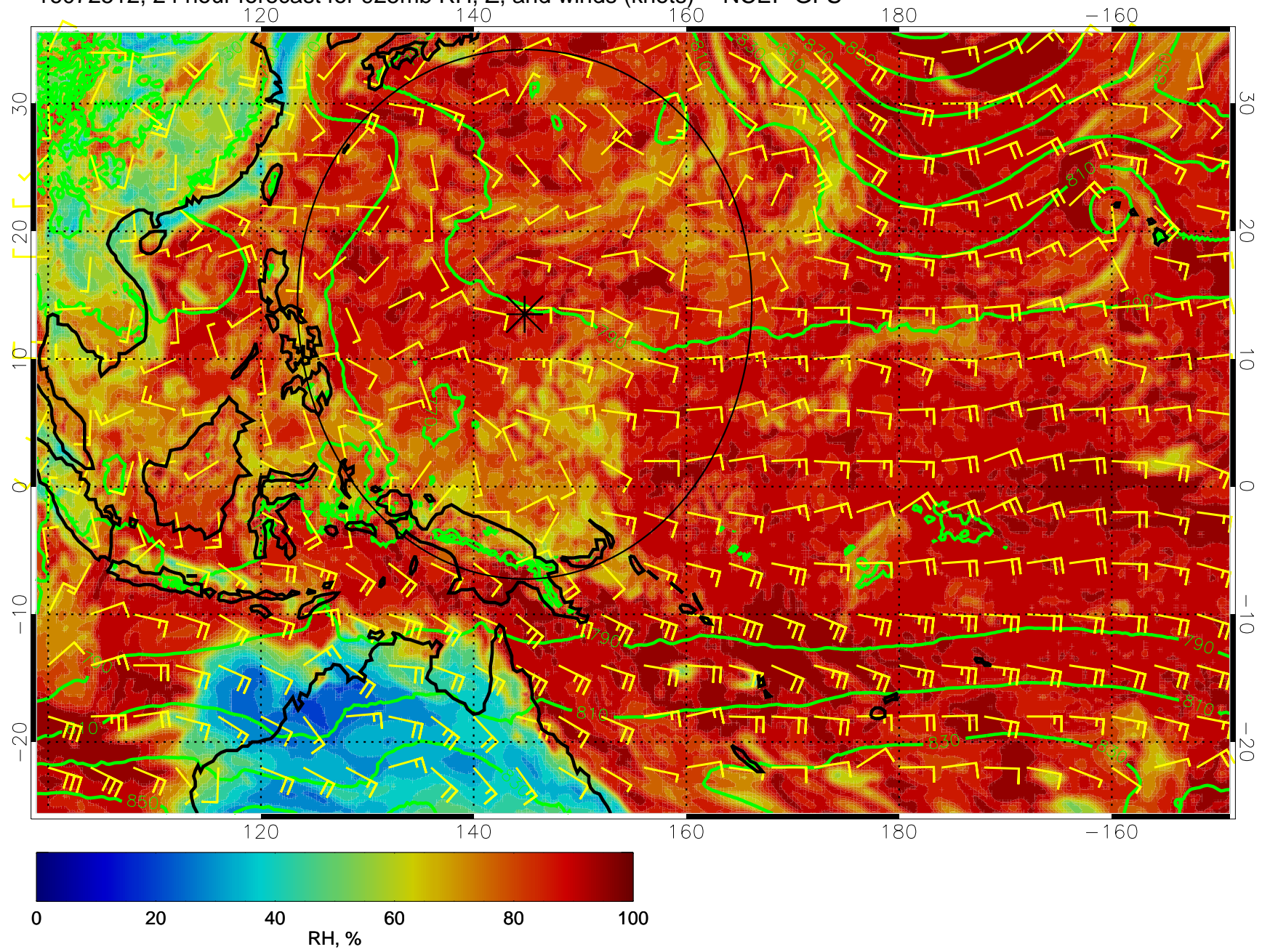
16072512, 24 hour forecast for 925mb RH, Z, and winds (knots) -- NCEP GFS
