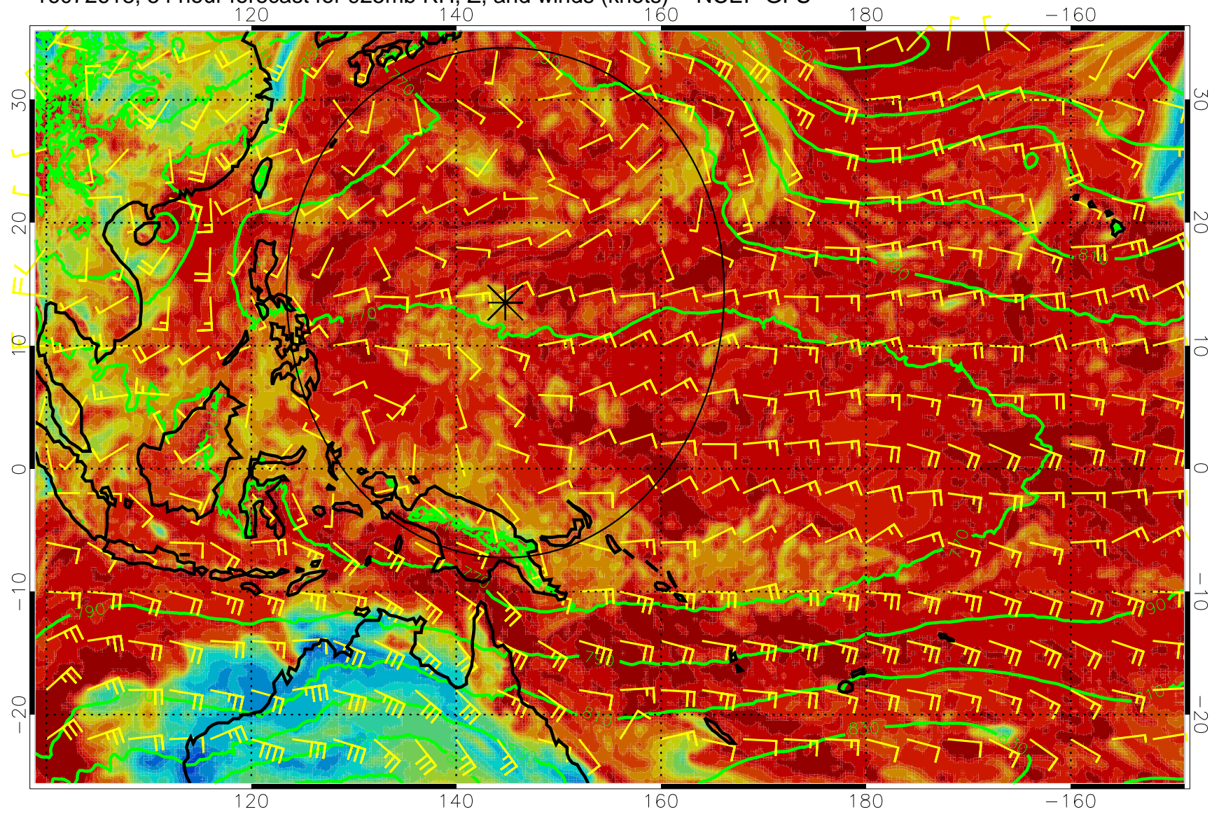
16072618, 54 hour forecast for 925mb RH, Z, and winds (knots) -- NCEP GFS
