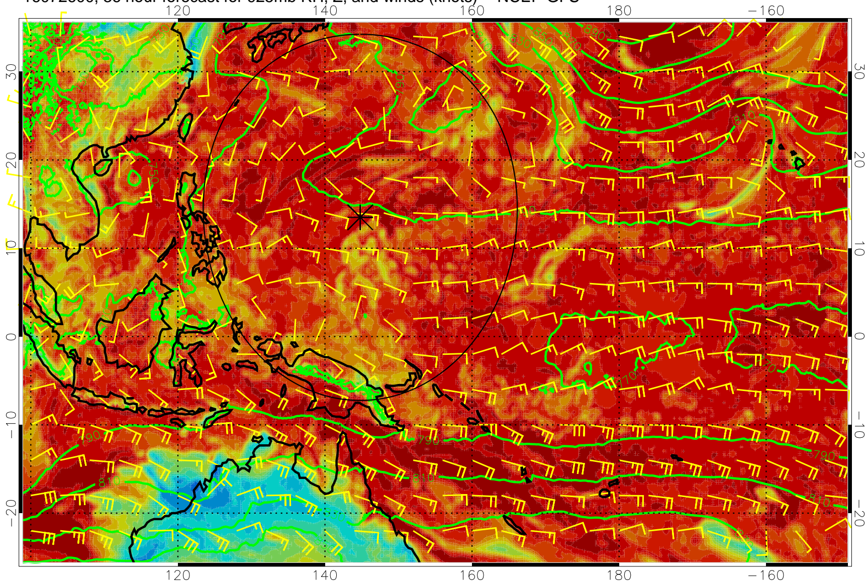
16072600, 36 hour forecast for 925mb RH, Z, and winds (knots) -- NCEP GFS
