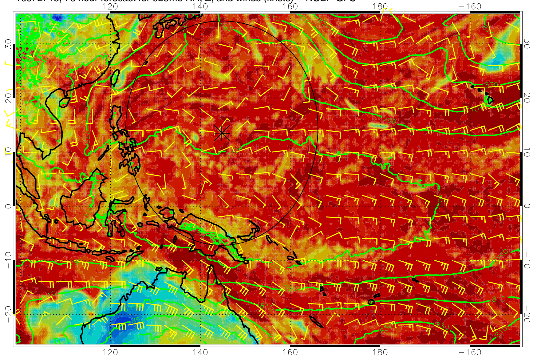
16072718, 78 hour forecast for 925mb RH, Z, and winds (knots) -- NCEP GFS
