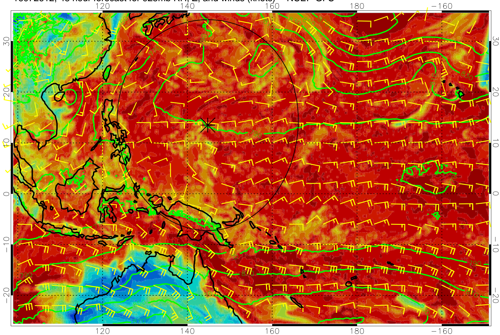
16072612, 48 hour forecast for 925mb RH, Z, and winds (knots) -- NCEP GFS
