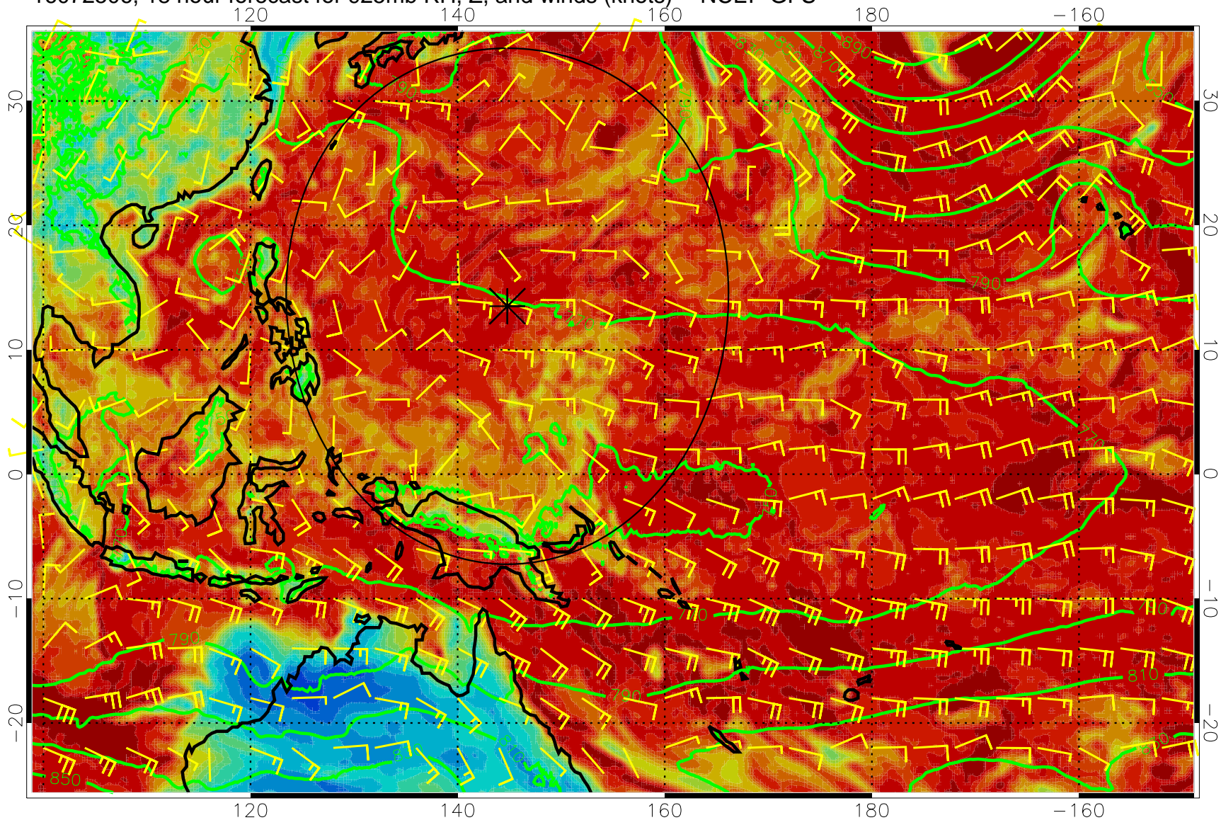
16072506, 18 hour forecast for 925mb RH, Z, and winds (knots) -- NCEP GFS
