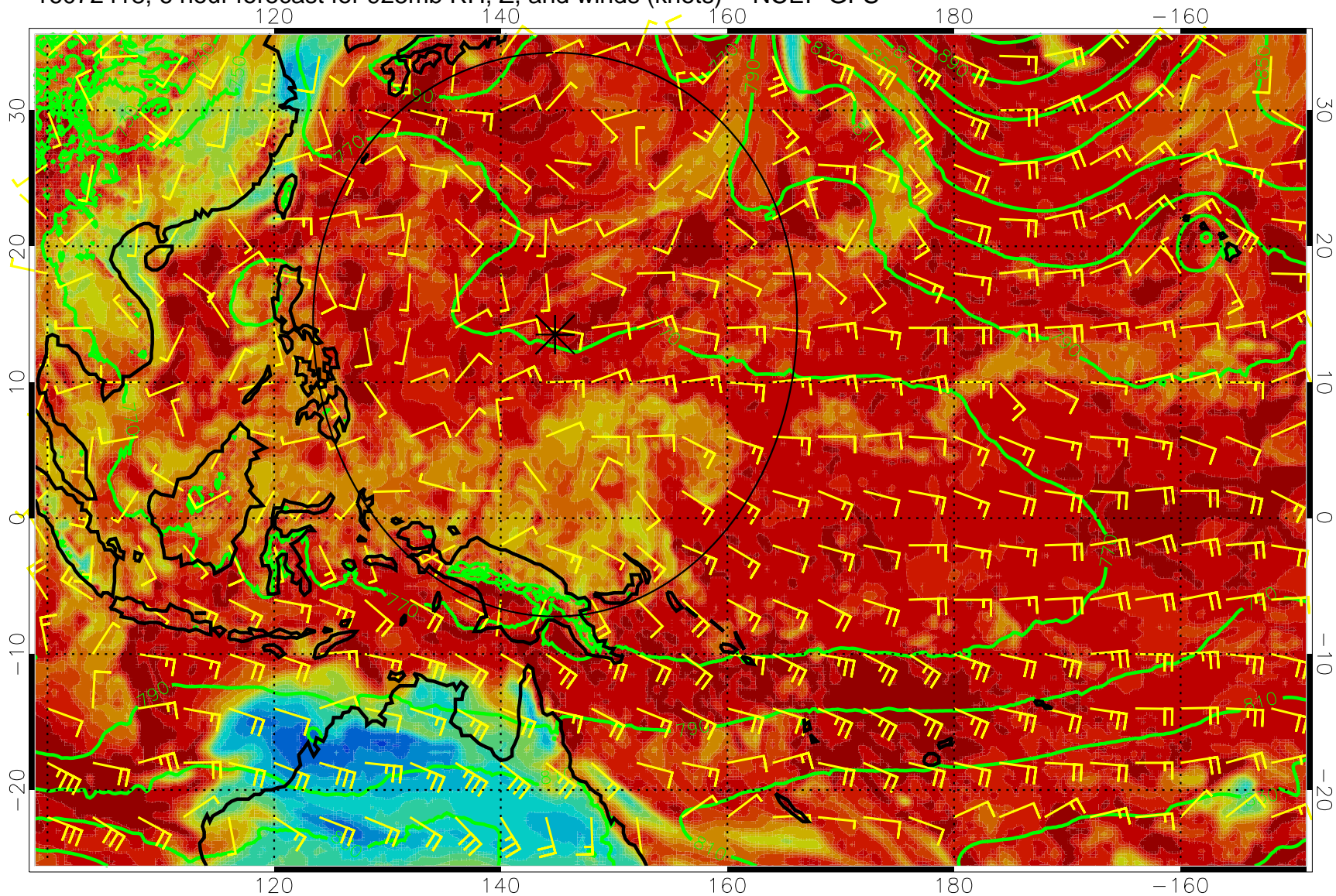
16072418, 6 hour forecast for 925mb RH, Z, and winds (knots) -- NCEP GFS
