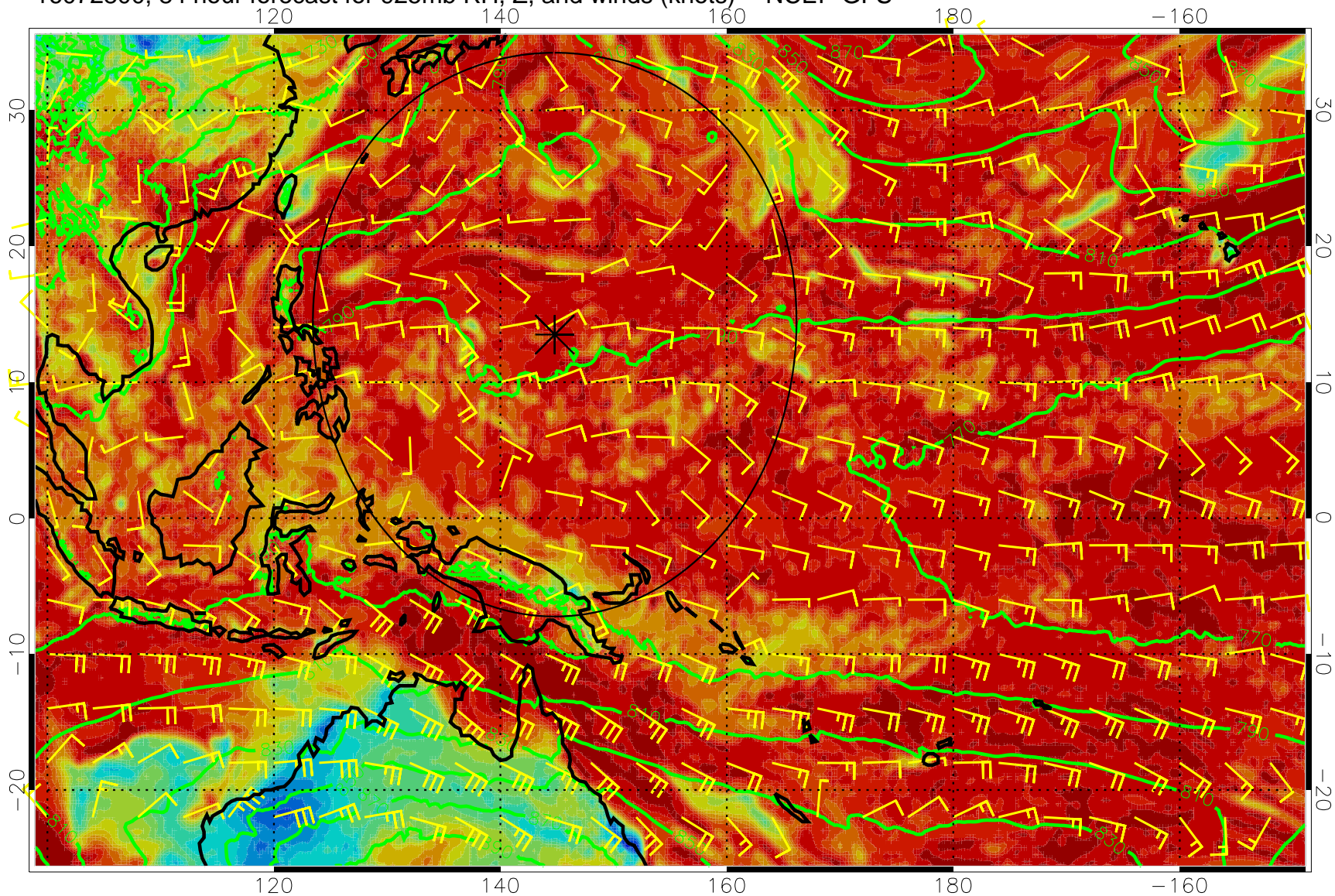
16072800, 84 hour forecast for 925mb RH, Z, and winds (knots) -- NCEP GFS
