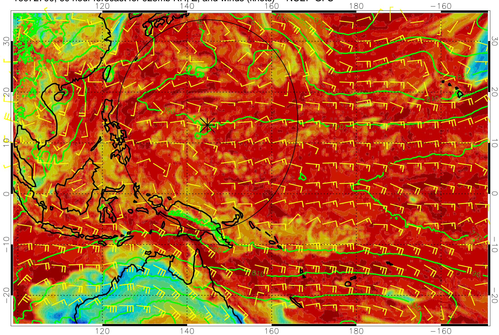
16072700, 60 hour forecast for 925mb RH, Z, and winds (knots) -- NCEP GFS
