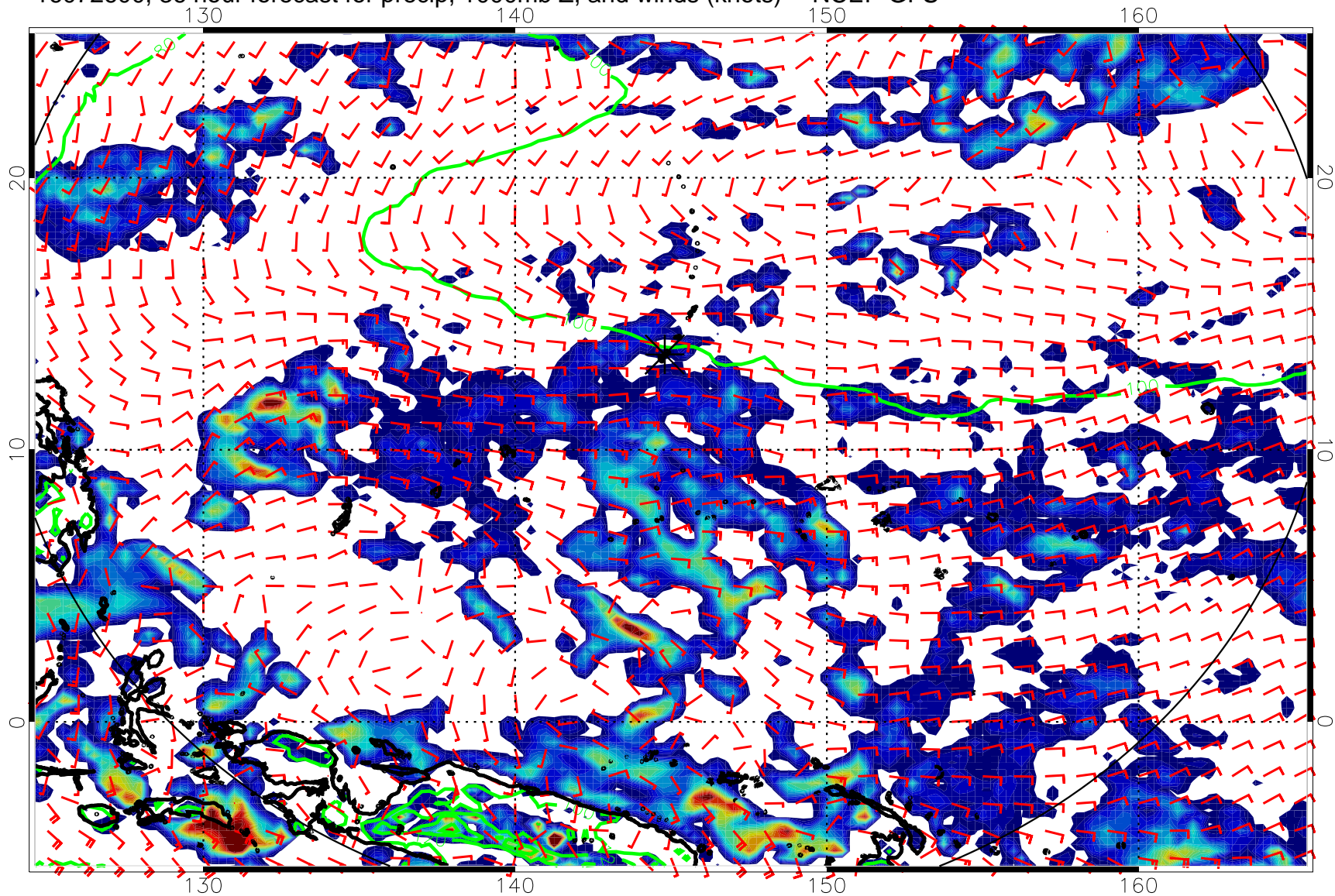
16072600, 36 hour forecast for precip, 1000mb Z, and winds (knots) -- NCEP GFS
