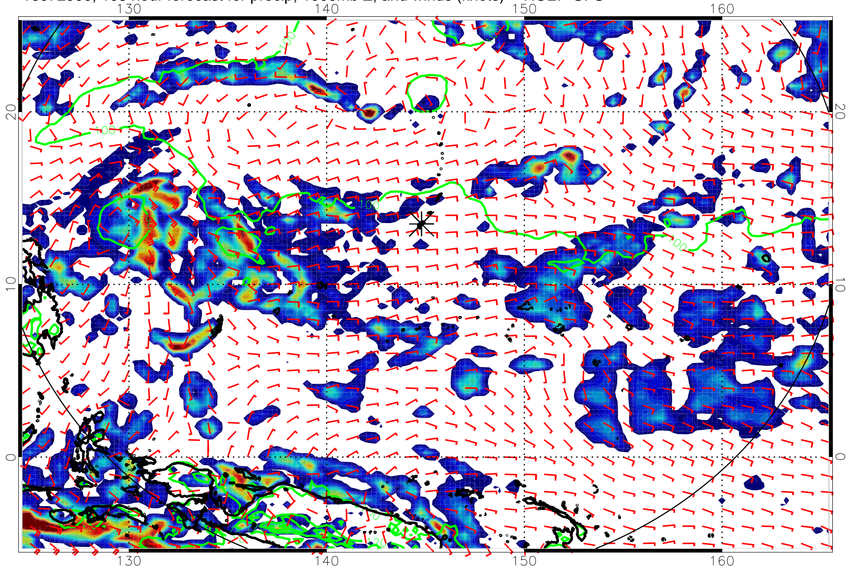
16072900, 108 hour forecast for precip, 1000mb Z, and winds (knots) -- NCEP GFS
