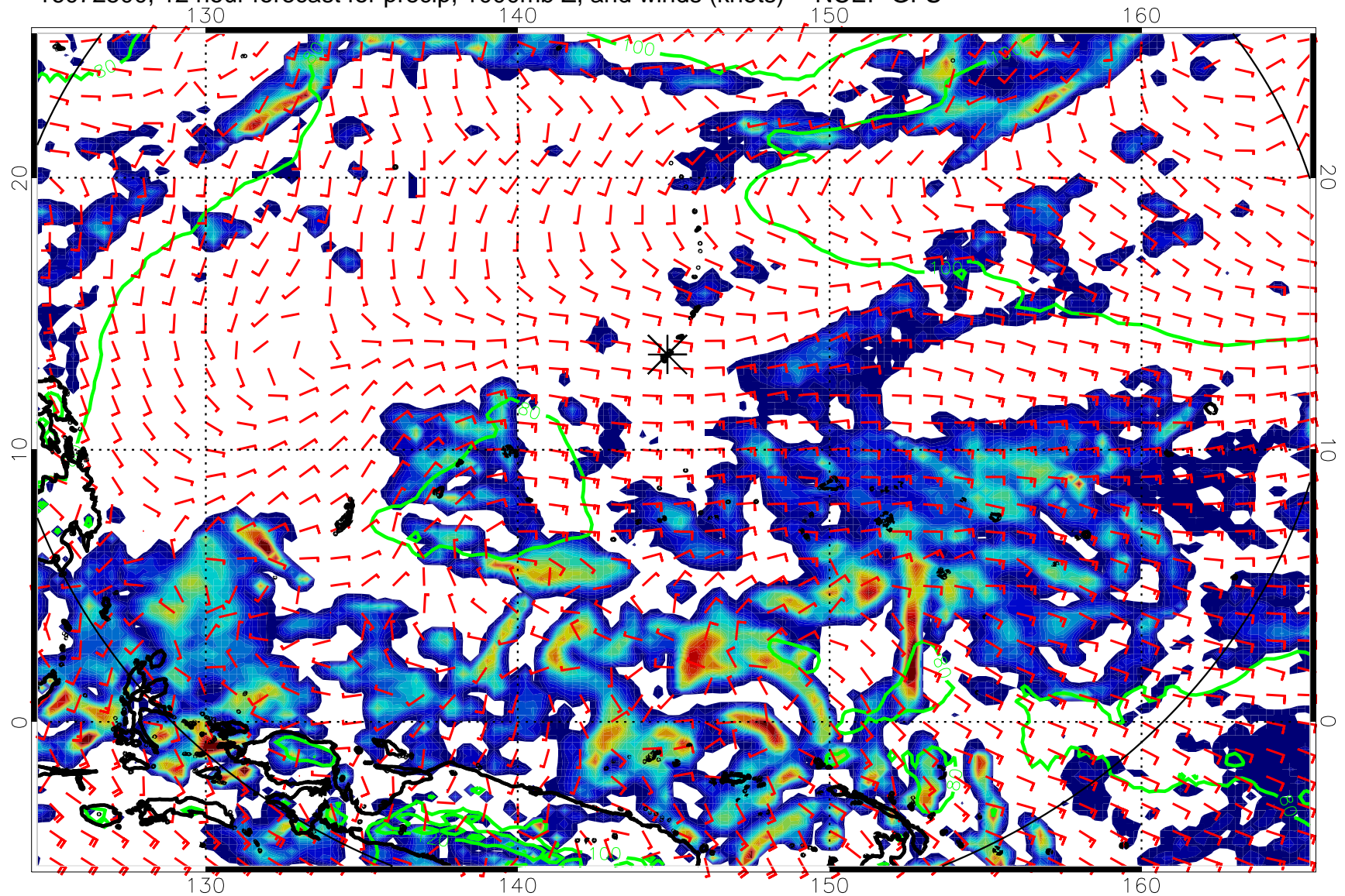
16072500, 12 hour forecast for precip, 1000mb Z, and winds (knots) -- NCEP GFS
