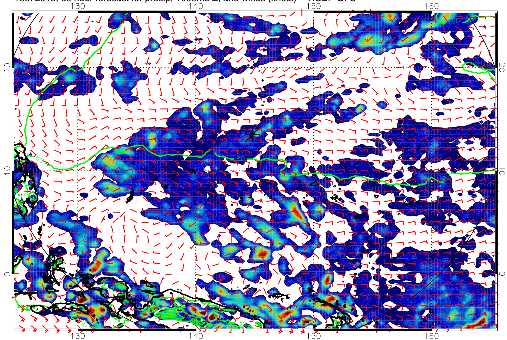
16072518, 30 hour forecast for precip, 1000mb Z, and winds (knots) -- NCEP GFS
