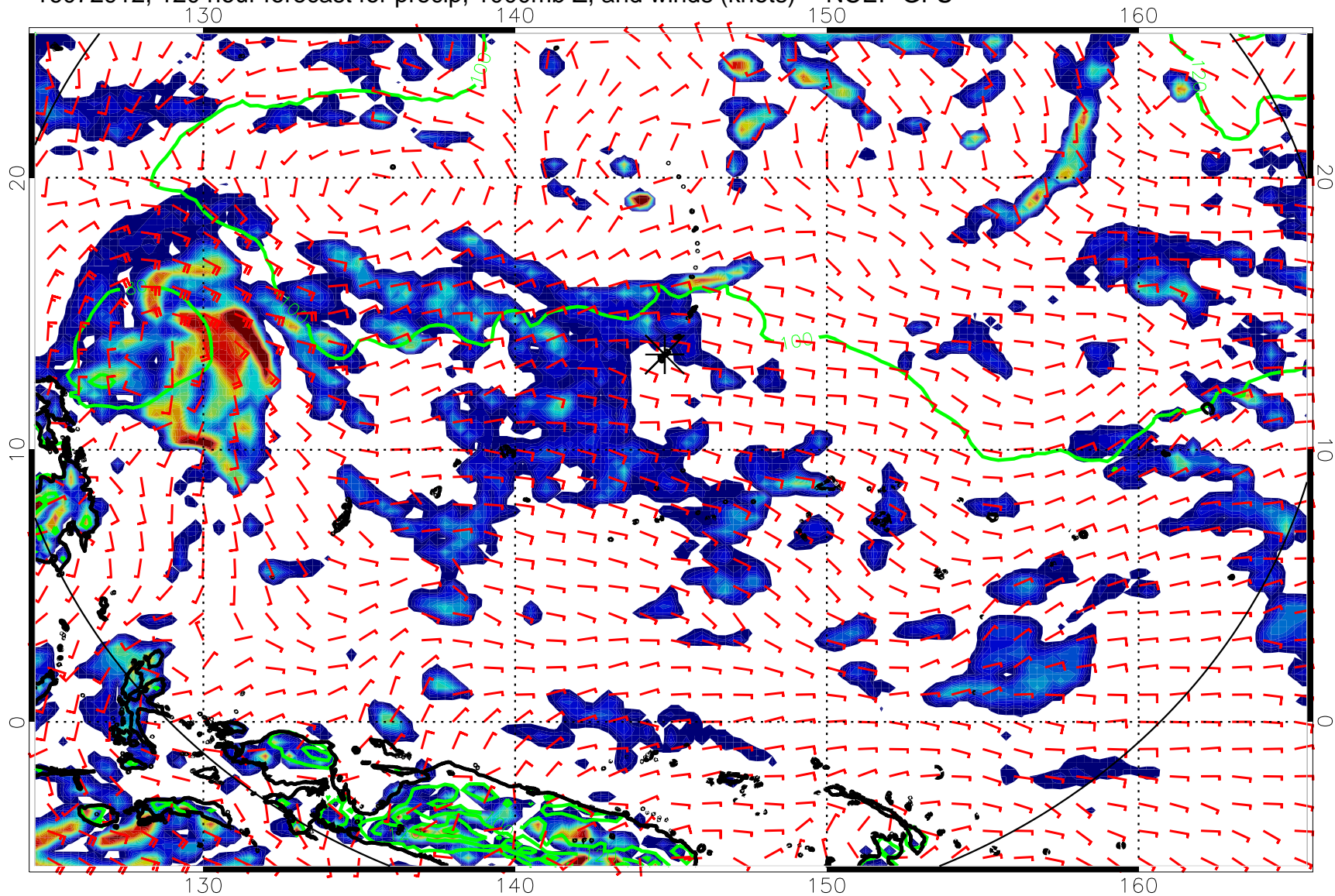
16072912, 120 hour forecast for precip, 1000mb Z, and winds (knots) -- NCEP GFS
