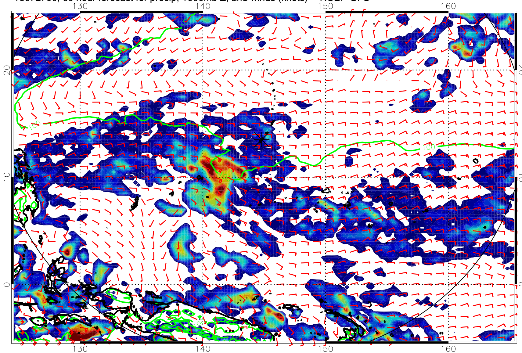
16072700, 60 hour forecast for precip, 1000mb Z, and winds (knots) -- NCEP GFS
