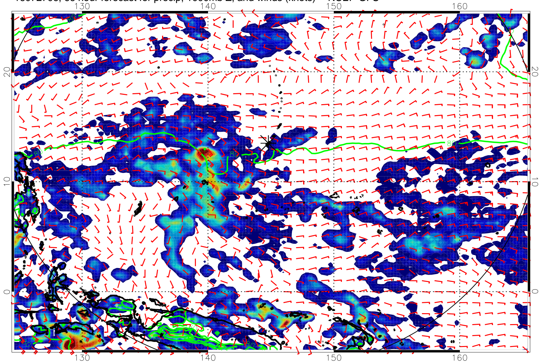
16072706, 66 hour forecast for precip, 1000mb Z, and winds (knots) -- NCEP GFS
