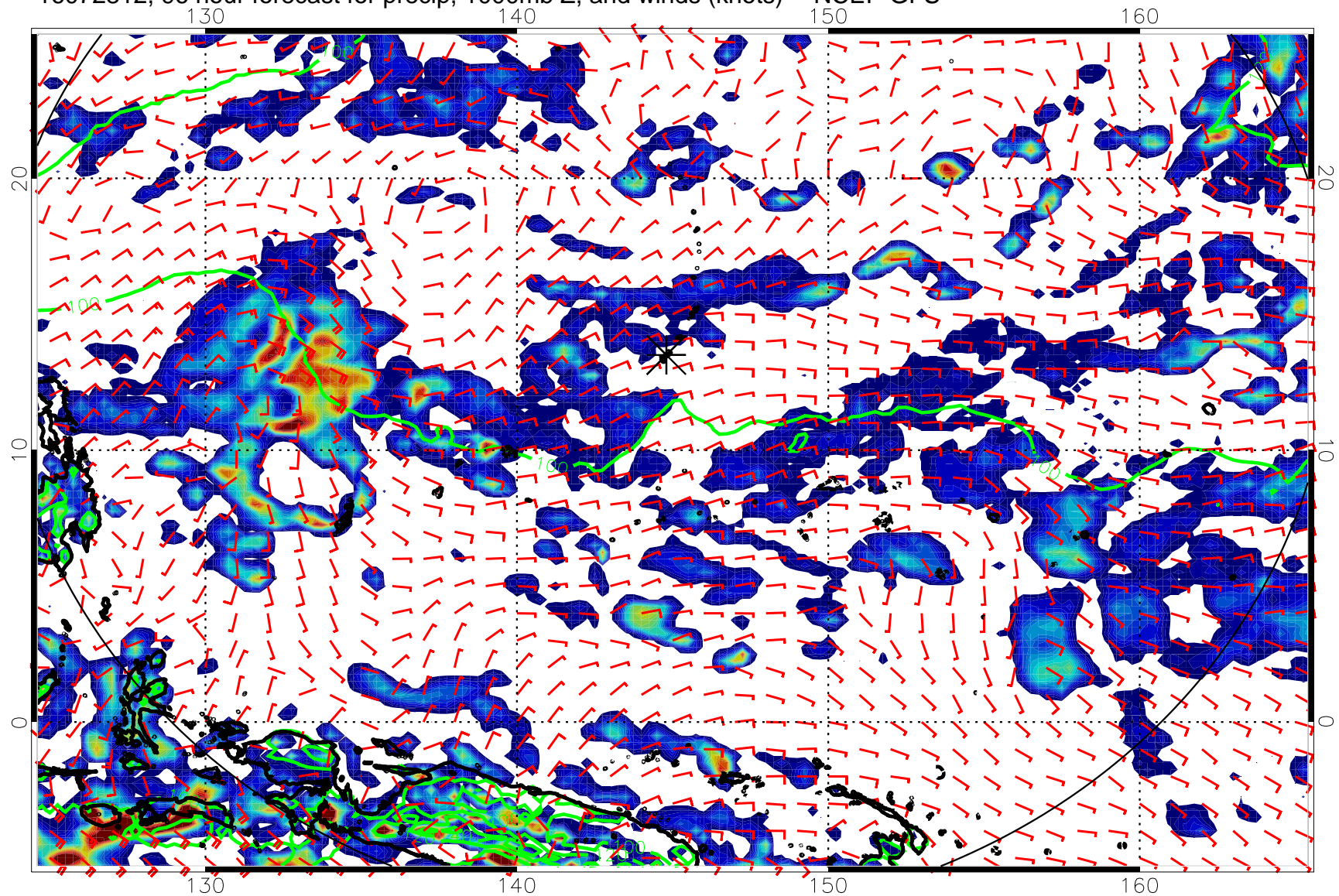
16072812, 96 hour forecast for precip, 1000mb Z, and winds (knots) -- NCEP GFS
