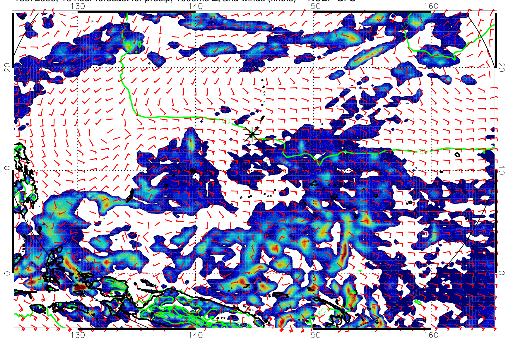
16072506, 18 hour forecast for precip, 1000mb Z, and winds (knots) -- NCEP GFS
