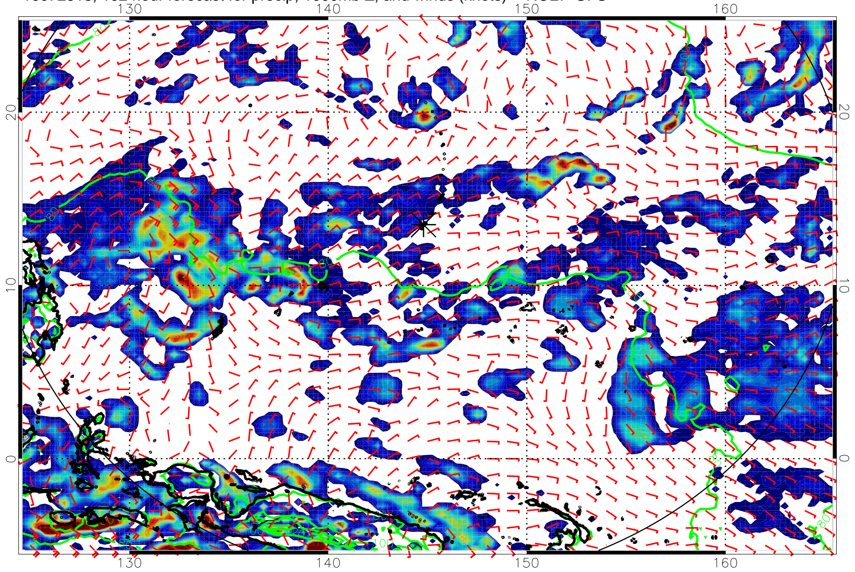
16072818, 102 hour forecast for precip, 1000mb Z, and winds (knots) -- NCEP GFS
