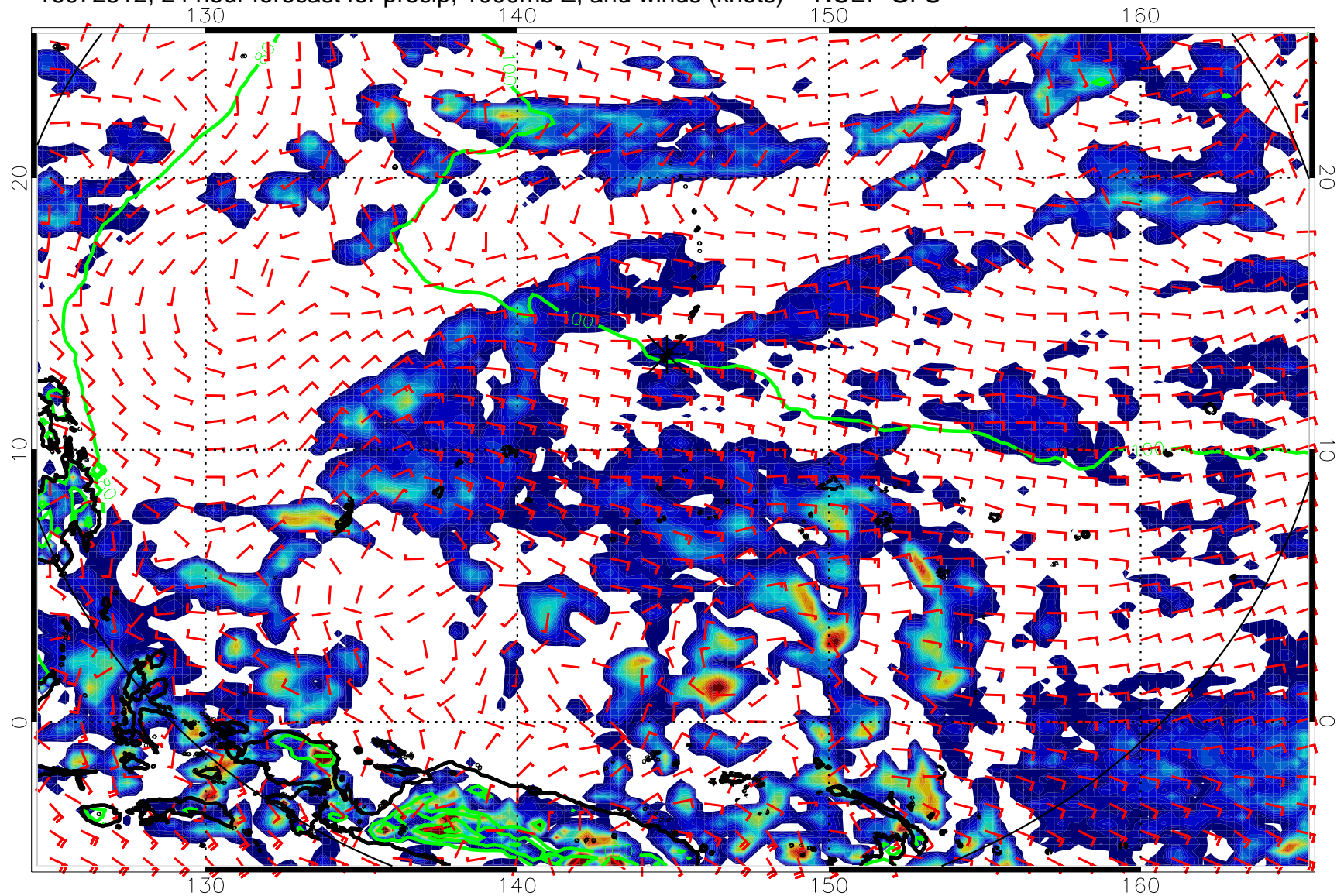
16072512, 24 hour forecast for precip, 1000mb Z, and winds (knots) -- NCEP GFS
