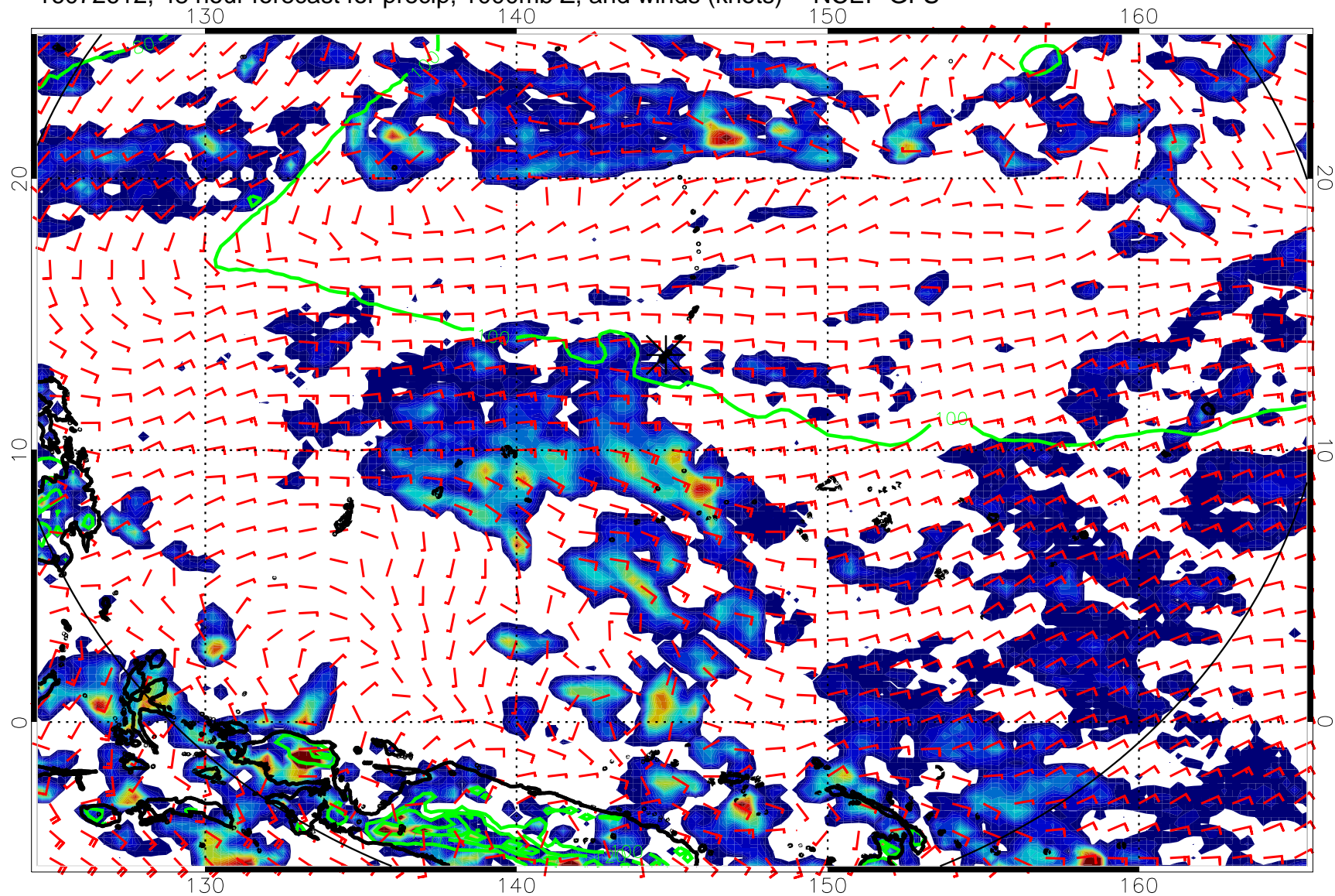
16072612, 48 hour forecast for precip, 1000mb Z, and winds (knots) -- NCEP GFS
