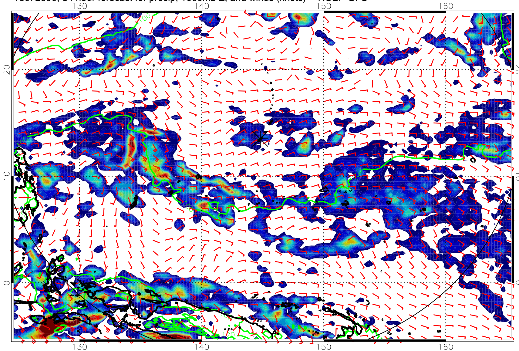
16072800, 84 hour forecast for precip, 1000mb Z, and winds (knots) -- NCEP GFS
