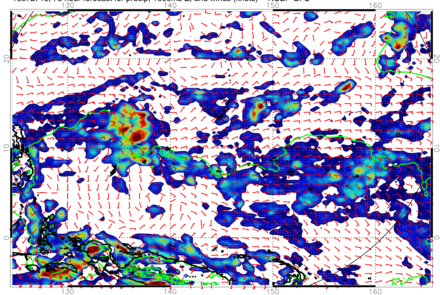
16072718, 78 hour forecast for precip, 1000mb Z, and winds (knots) -- NCEP GFS
