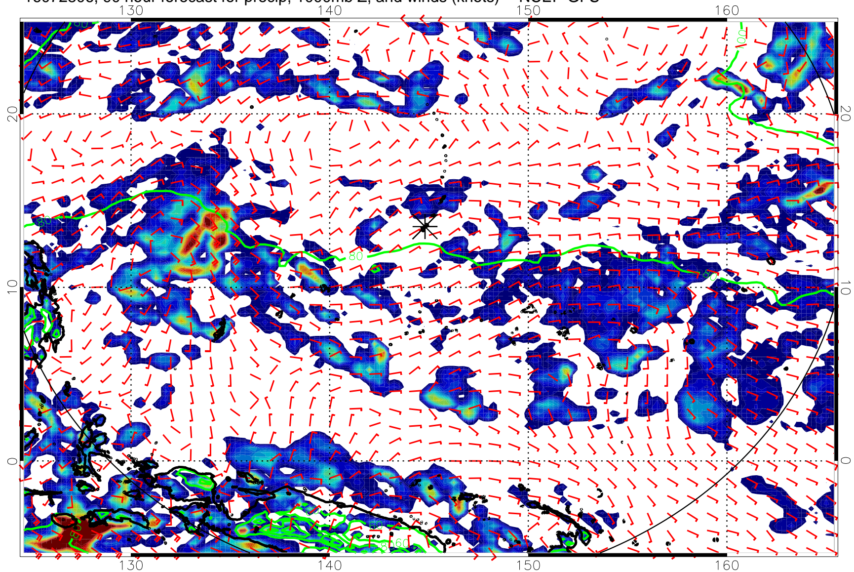
16072806, 90 hour forecast for precip, 1000mb Z, and winds (knots) -- NCEP GFS
