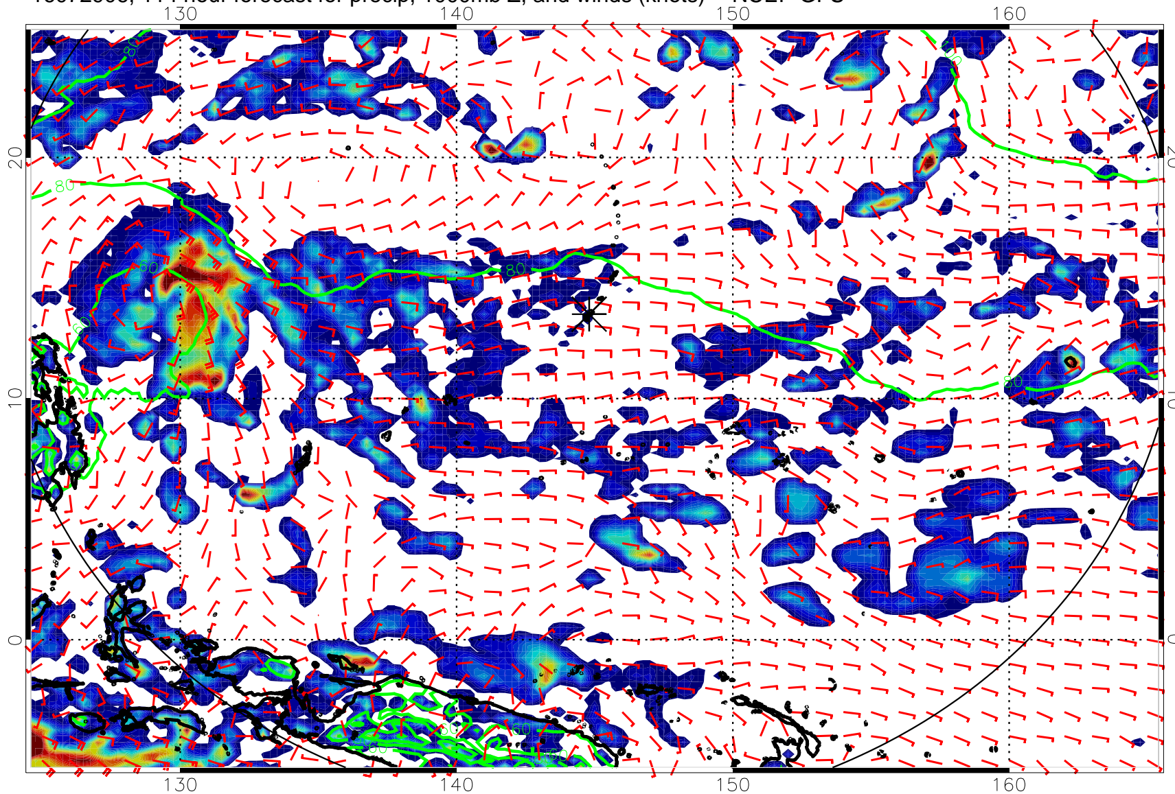
16072906, 114 hour forecast for precip, 1000mb Z, and winds (knots) -- NCEP GFS
