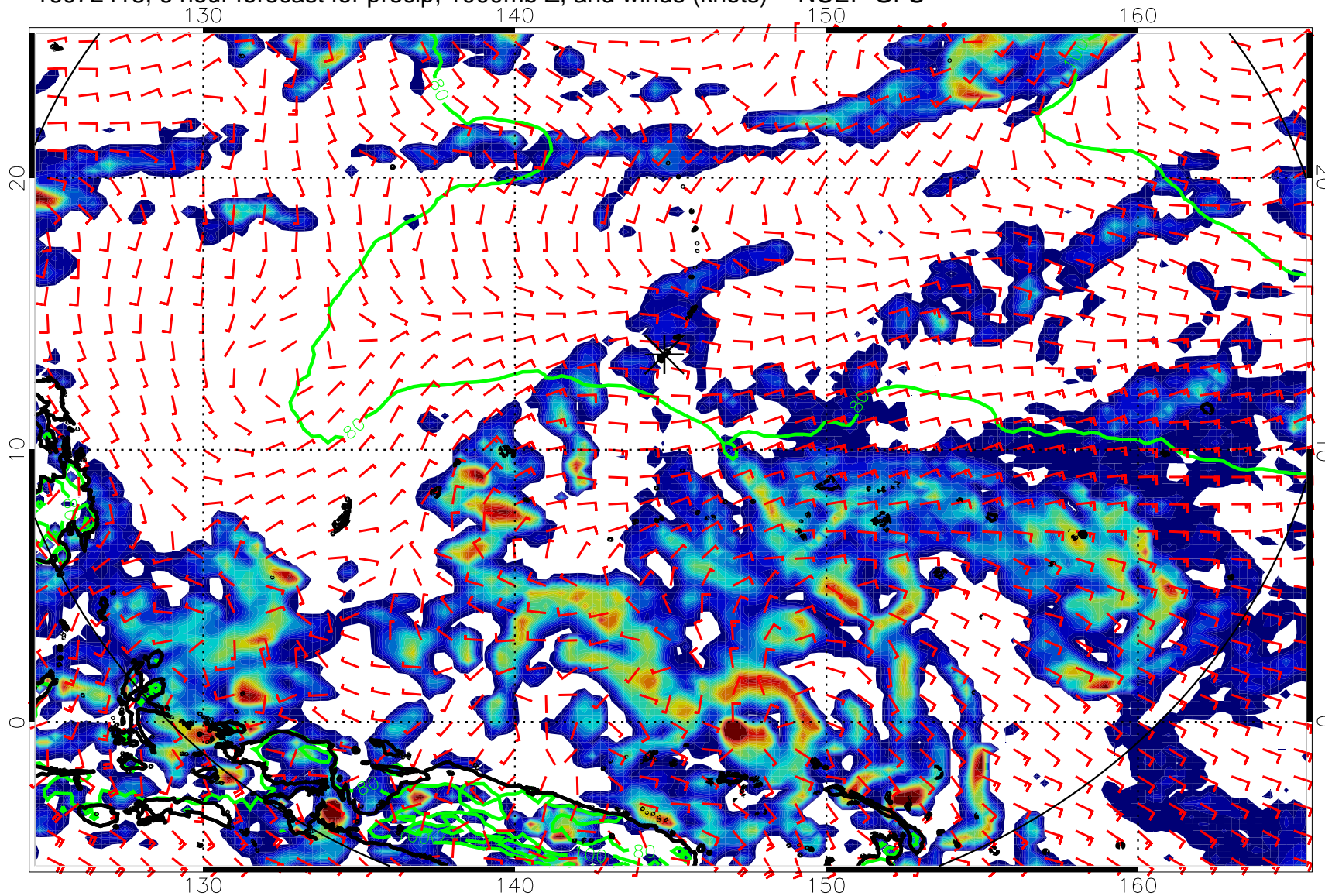
16072418, 6 hour forecast for precip, 1000mb Z, and winds (knots) -- NCEP GFS
