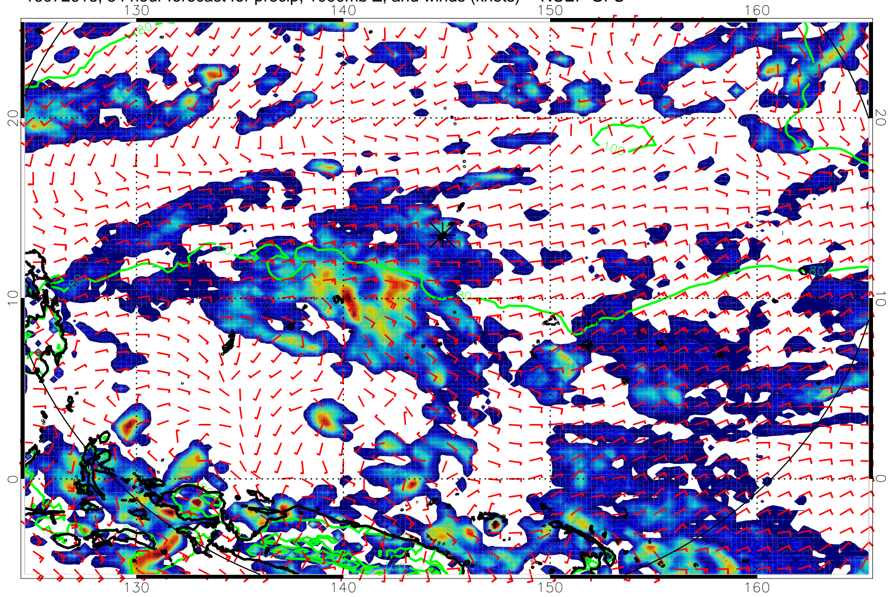
16072618, 54 hour forecast for precip, 1000mb Z, and winds (knots) -- NCEP GFS
