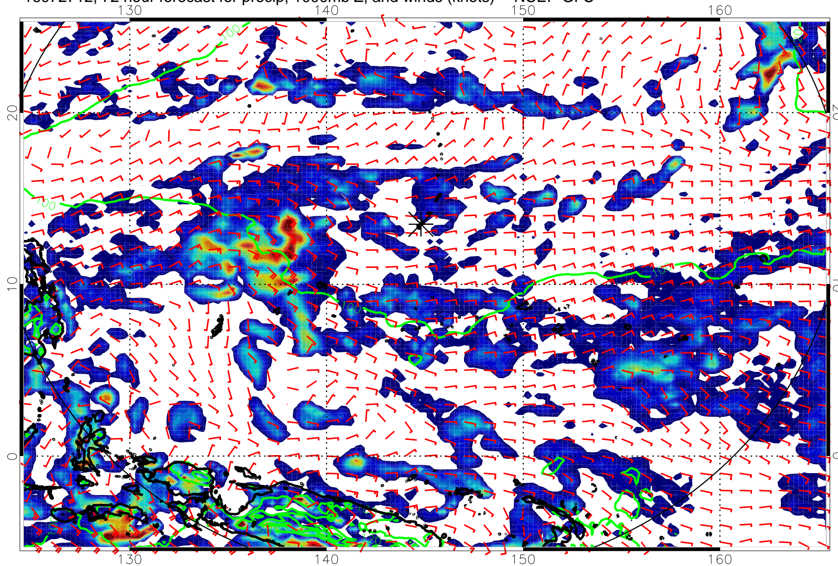
16072712, 72 hour forecast for precip, 1000mb Z, and winds (knots) -- NCEP GFS
