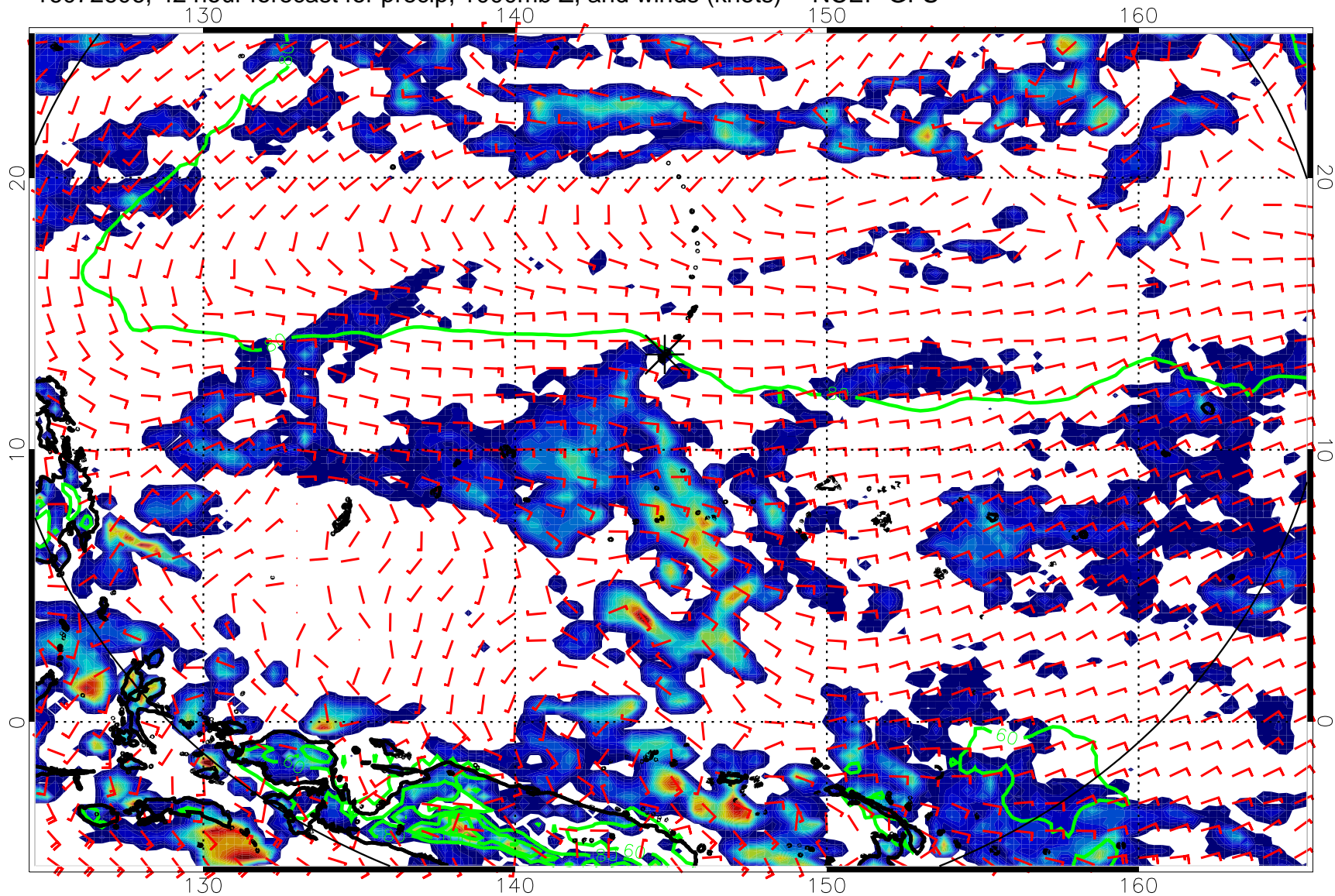
16072606, 42 hour forecast for precip, 1000mb Z, and winds (knots) -- NCEP GFS
