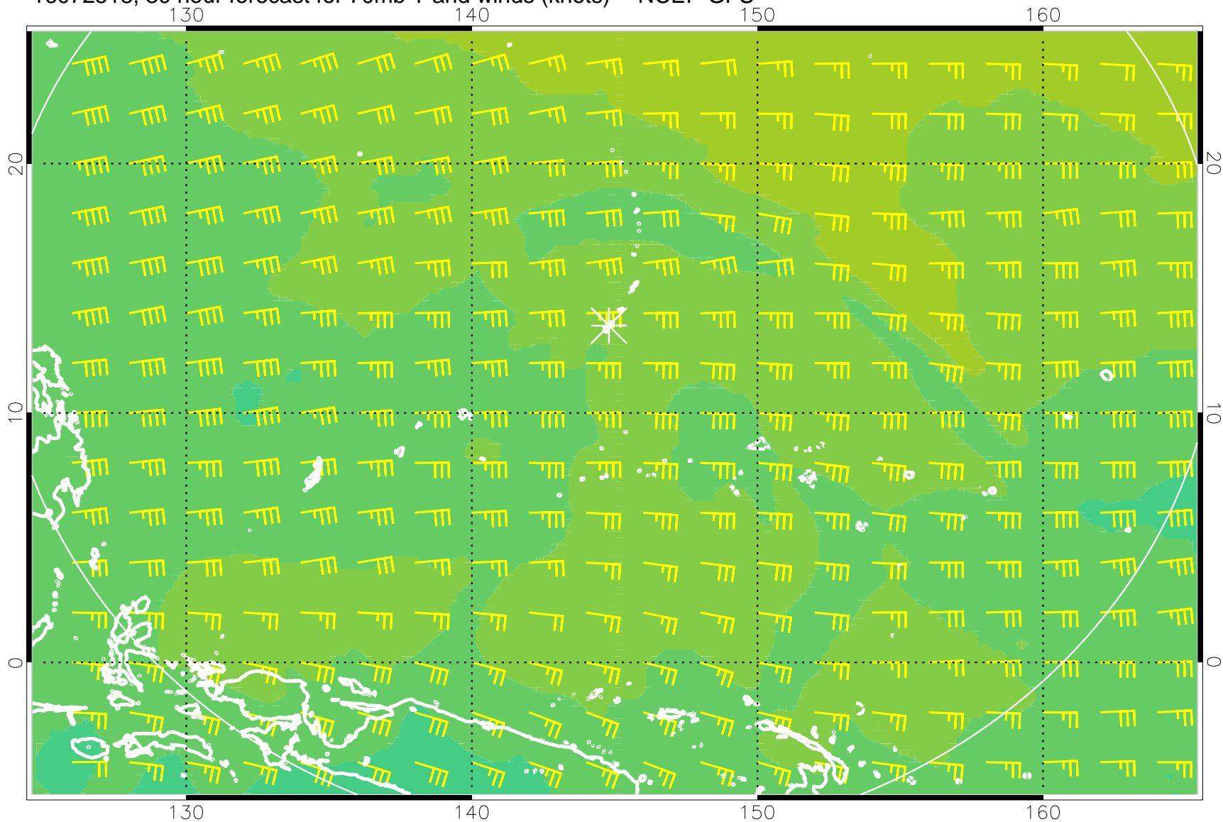
16072518, 30 hour forecast for 70mb T and winds (knots) -- NCEP GFS
