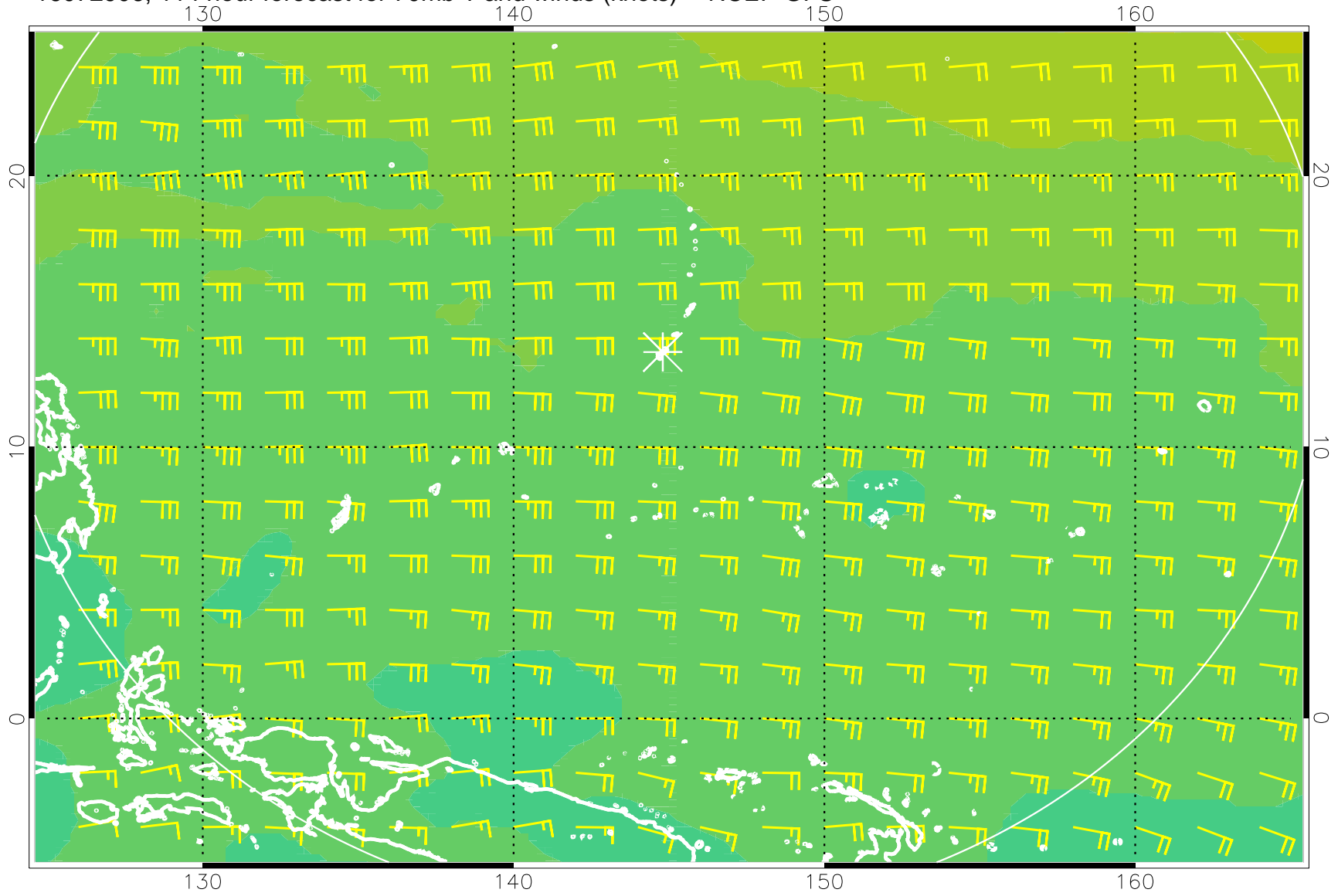
16072906, 114 hour forecast for 70mb T and winds (knots) -- NCEP GFS
