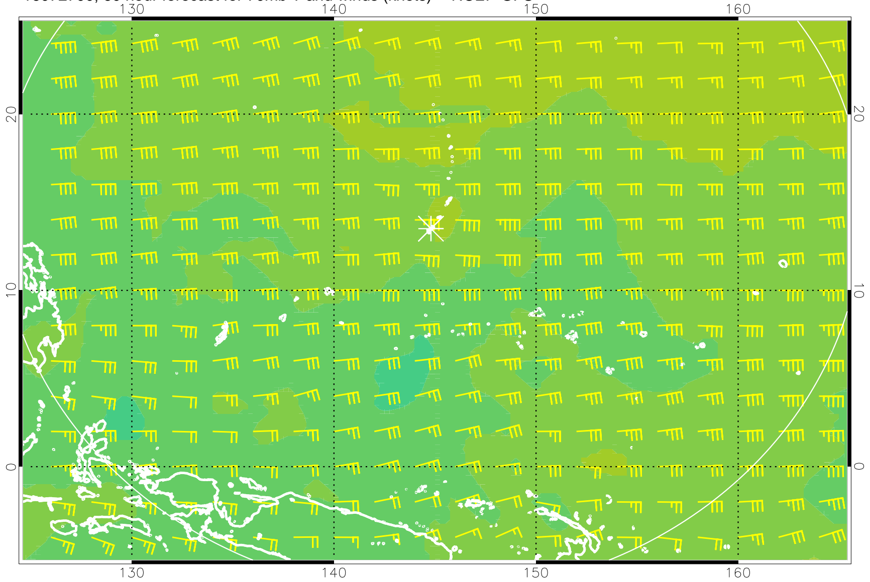
16072700, 60 hour forecast for 70mb T and winds (knots) -- NCEP GFS
