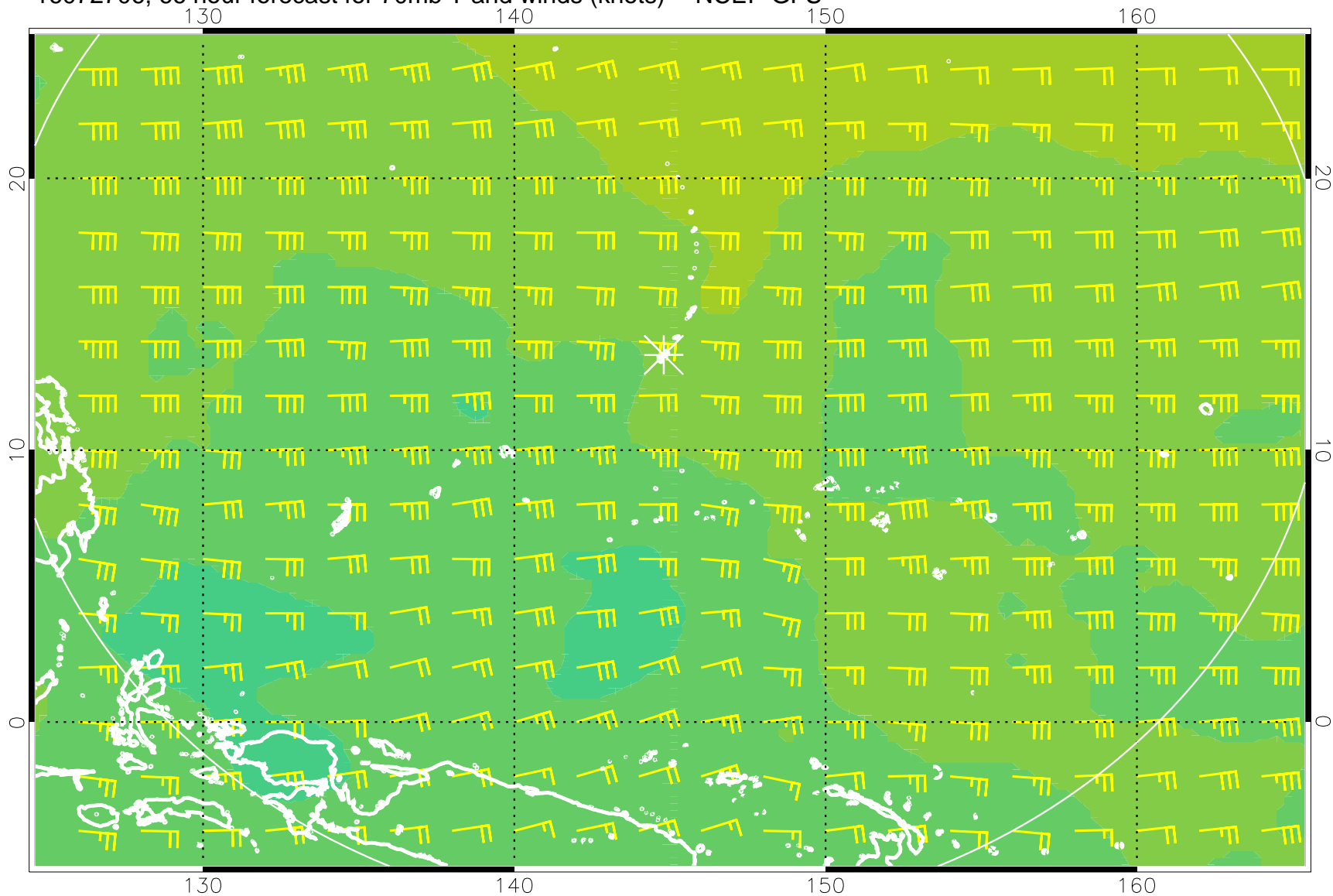
16072706, 66 hour forecast for 70mb T and winds (knots) -- NCEP GFS
