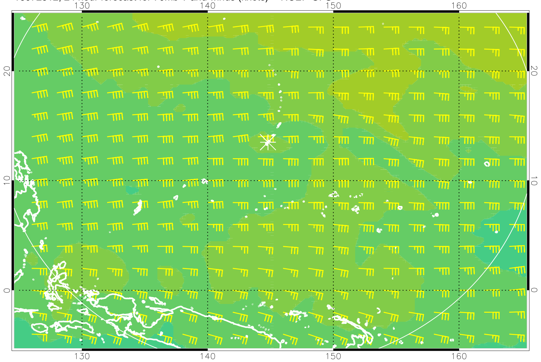
16072512, 24 hour forecast for 70mb T and winds (knots) -- NCEP GFS
