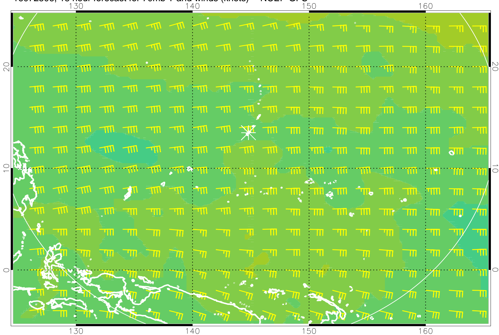
16072506, 18 hour forecast for 70mb T and winds (knots) -- NCEP GFS
