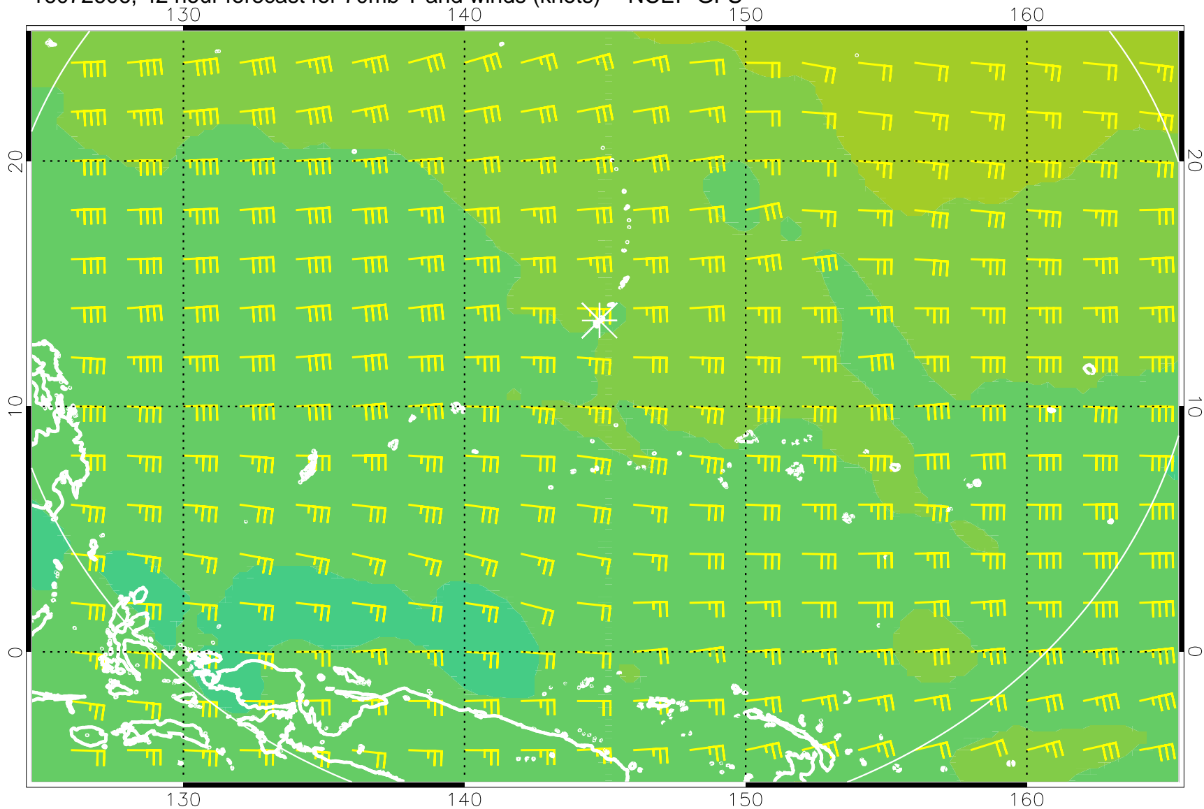
16072606, 42 hour forecast for 70mb T and winds (knots) -- NCEP GFS
