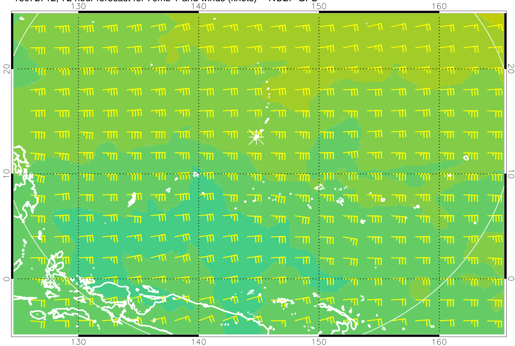
16072712, 72 hour forecast for 70mb T and winds (knots) -- NCEP GFS
