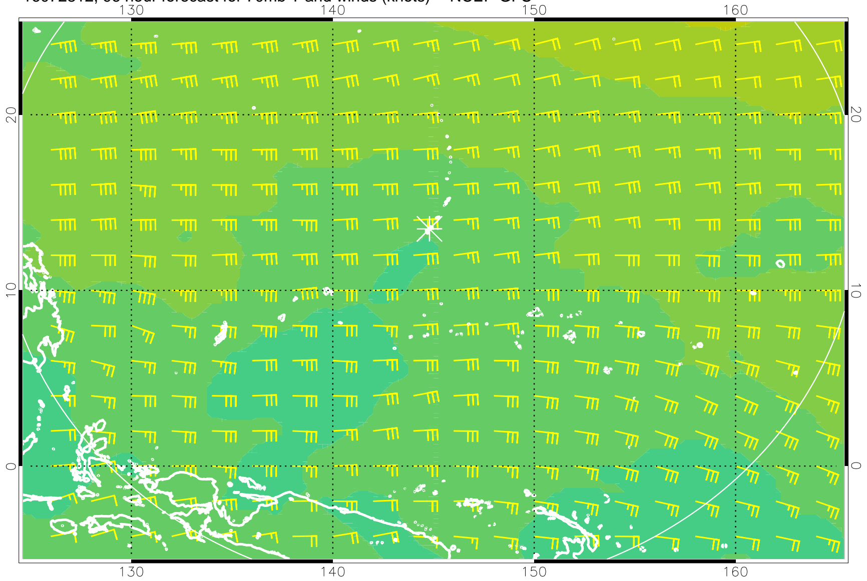
16072812, 96 hour forecast for 70mb T and winds (knots) -- NCEP GFS
