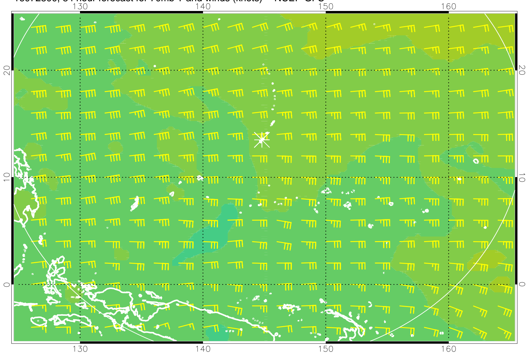
16072800, 84 hour forecast for 70mb T and winds (knots) -- NCEP GFS
