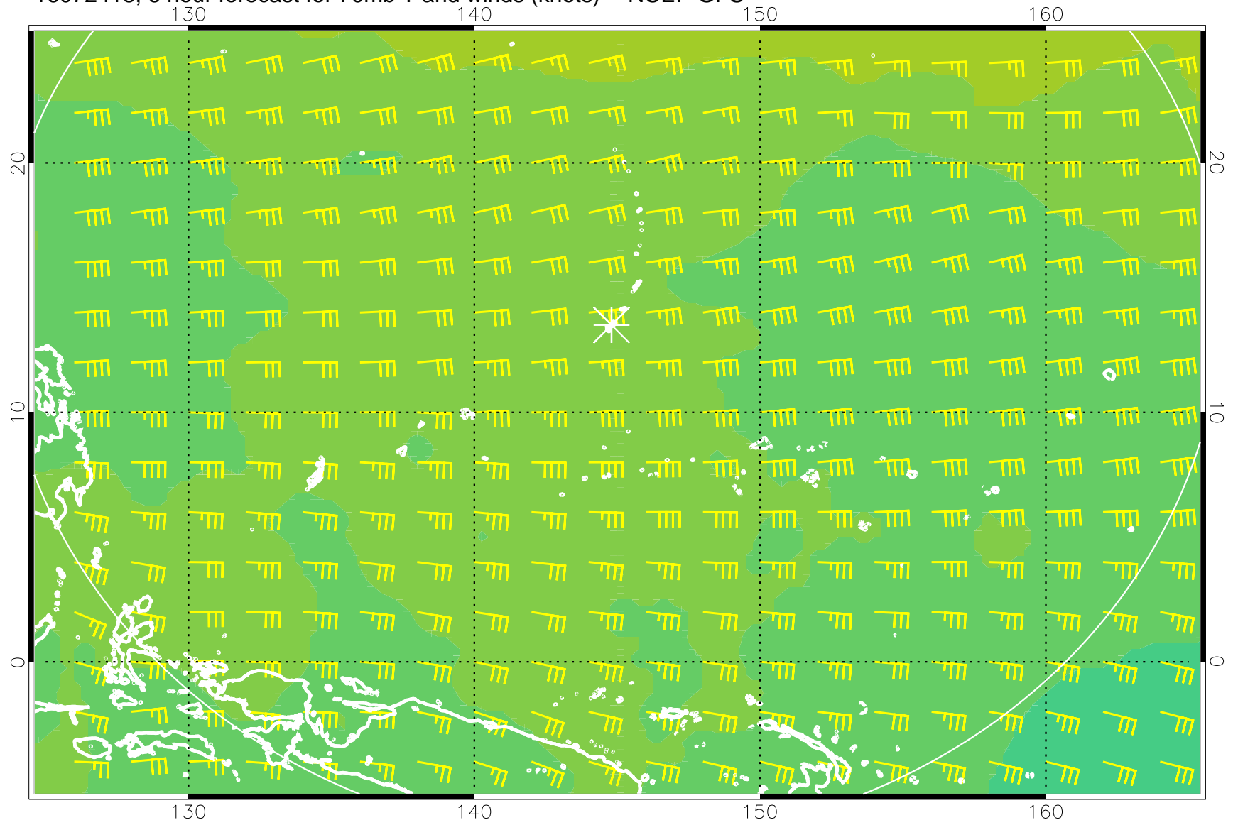
16072418, 6 hour forecast for 70mb T and winds (knots) -- NCEP GFS
