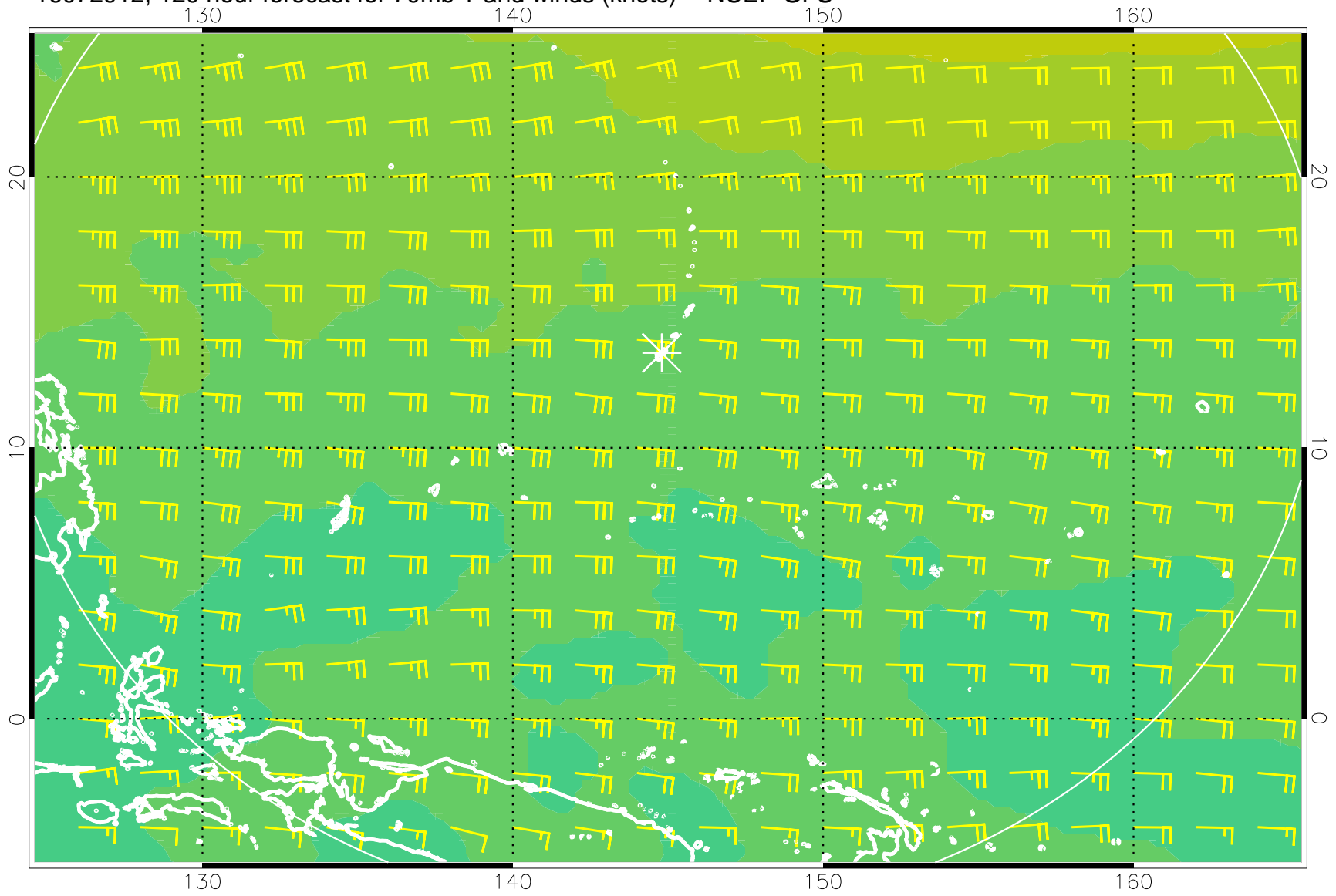
16072912, 120 hour forecast for 70mb T and winds (knots) -- NCEP GFS
