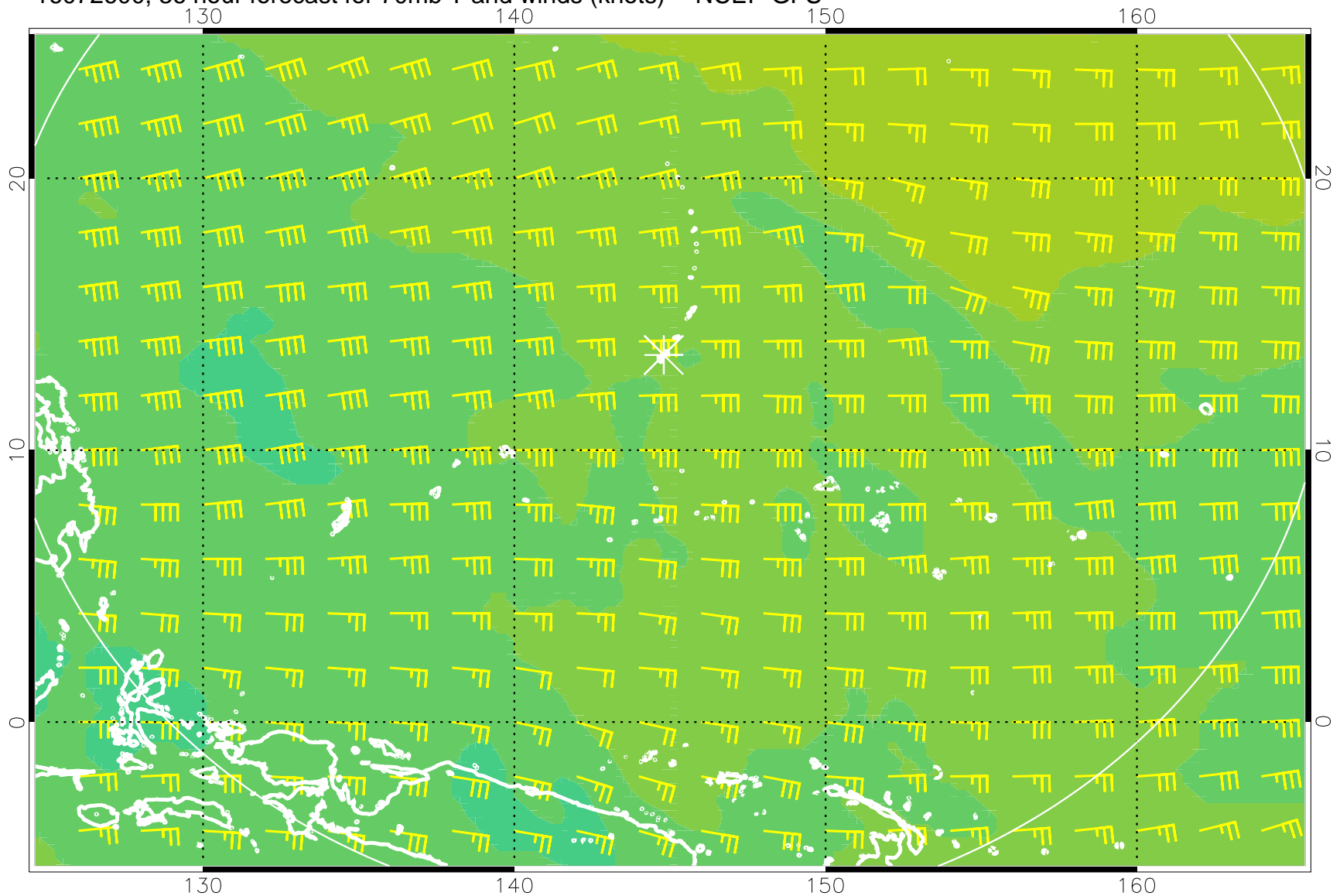
16072600, 36 hour forecast for 70mb T and winds (knots) -- NCEP GFS
