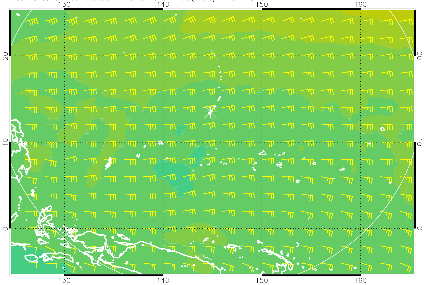
16072818, 102 hour forecast for 70mb T and winds (knots) -- NCEP GFS
