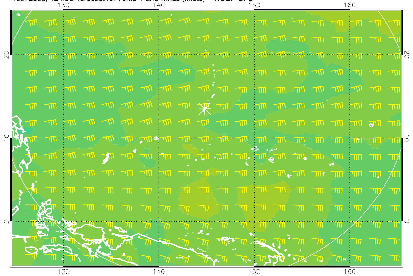
16072500, 12 hour forecast for 70mb T and winds (knots) -- NCEP GFS
