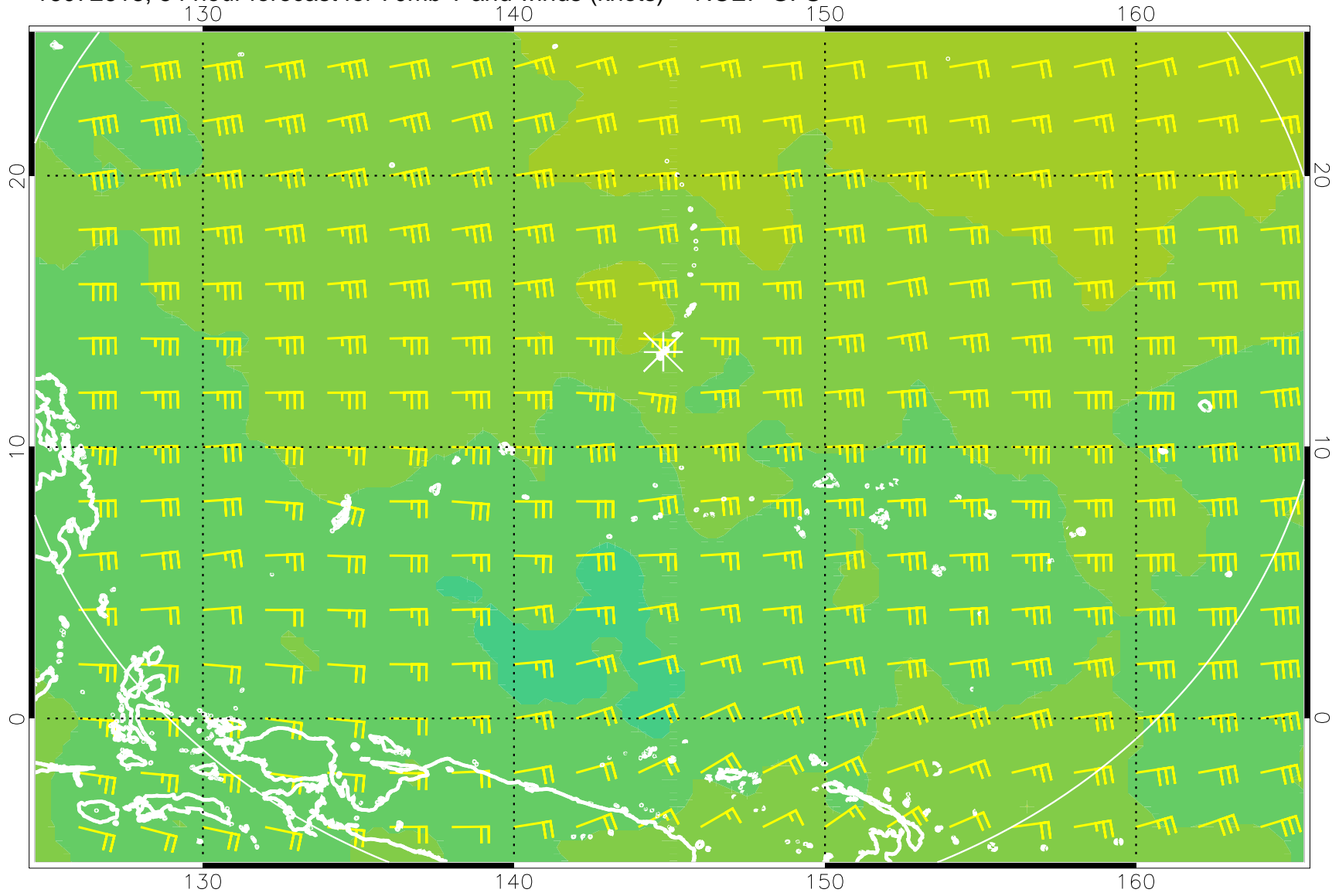
16072618, 54 hour forecast for 70mb T and winds (knots) -- NCEP GFS
