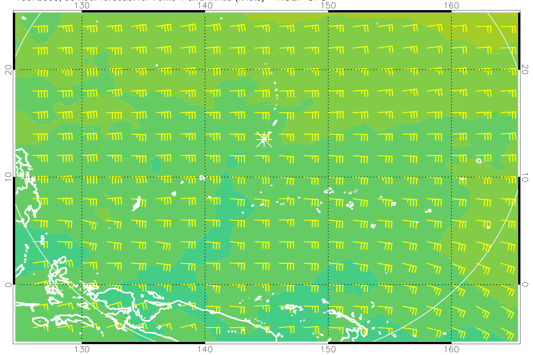
16072806, 90 hour forecast for 70mb T and winds (knots) -- NCEP GFS
