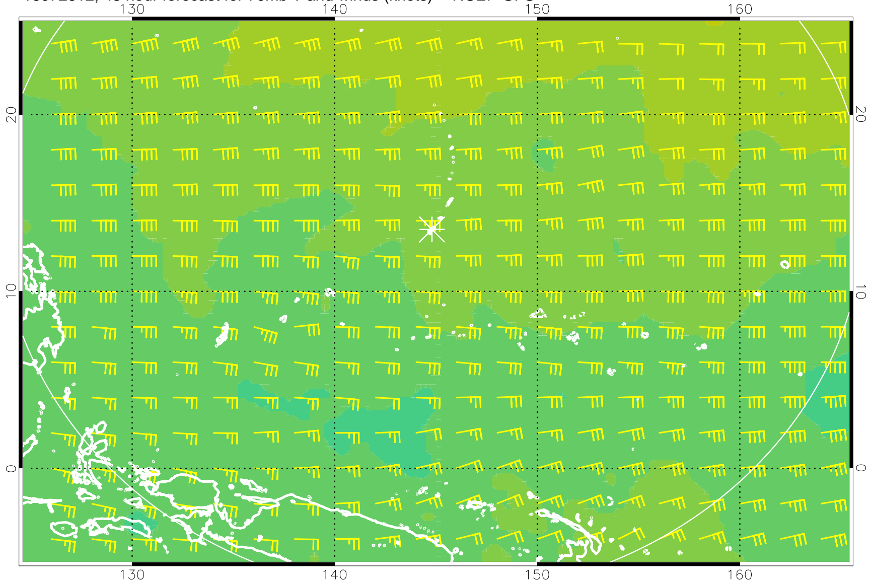
16072612, 48 hour forecast for 70mb T and winds (knots) -- NCEP GFS
