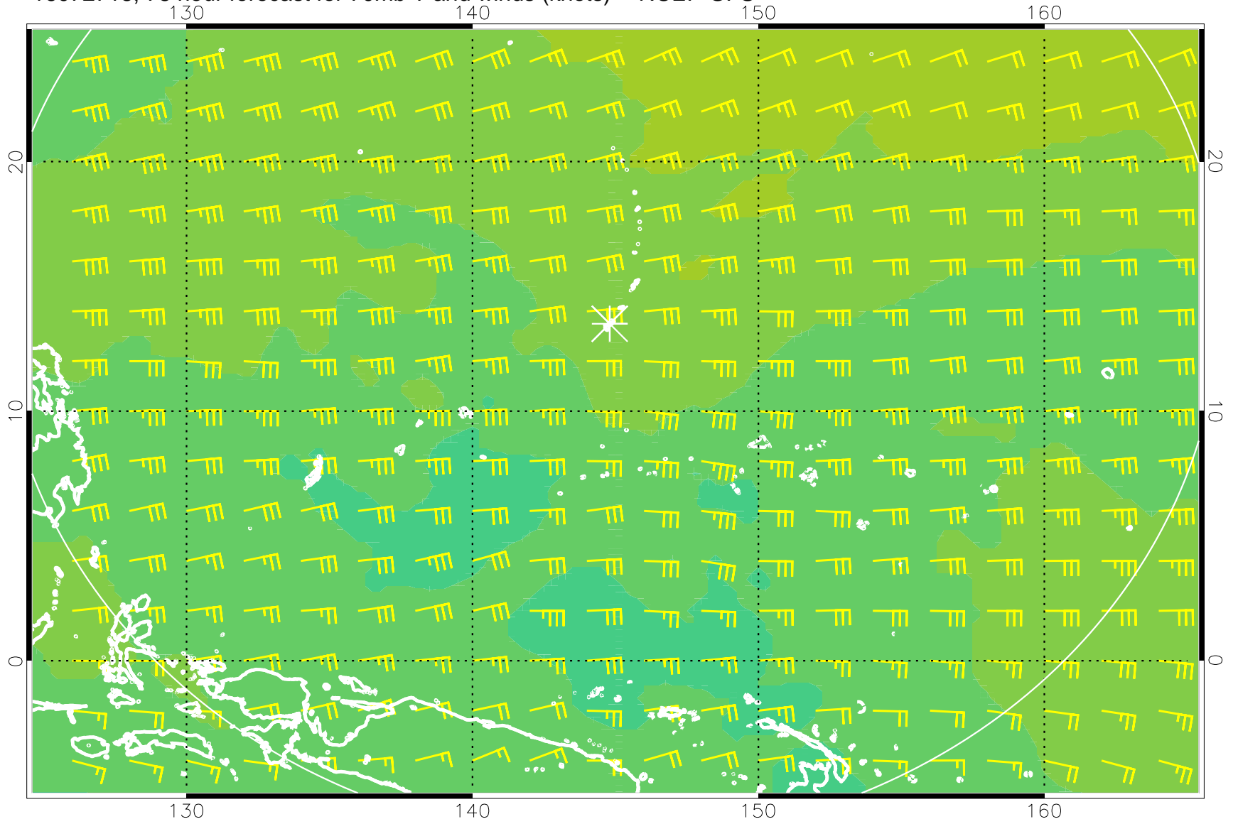
16072718, 78 hour forecast for 70mb T and winds (knots) -- NCEP GFS
