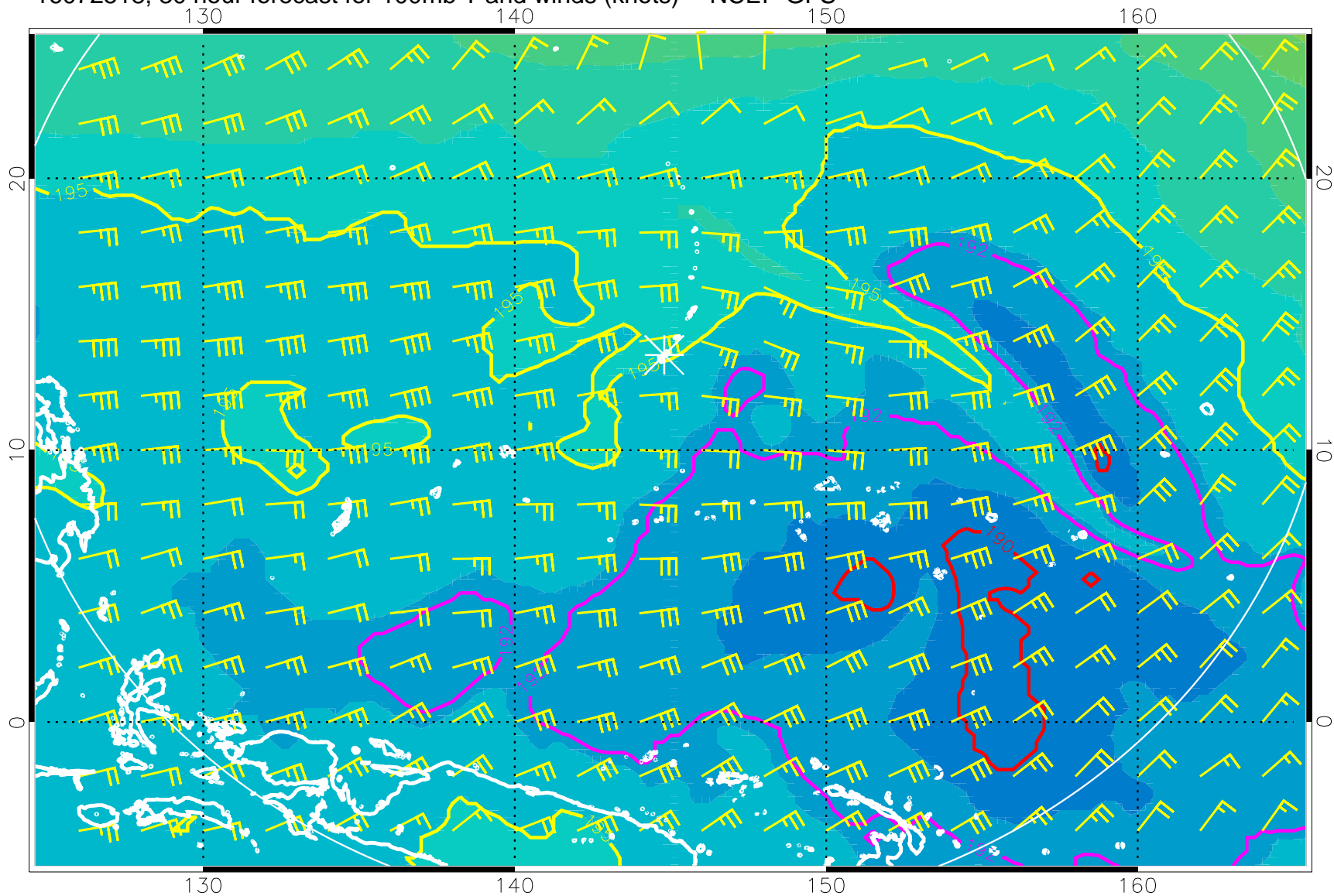
16072518, 30 hour forecast for 100mb T and winds (knots) -- NCEP GFS
