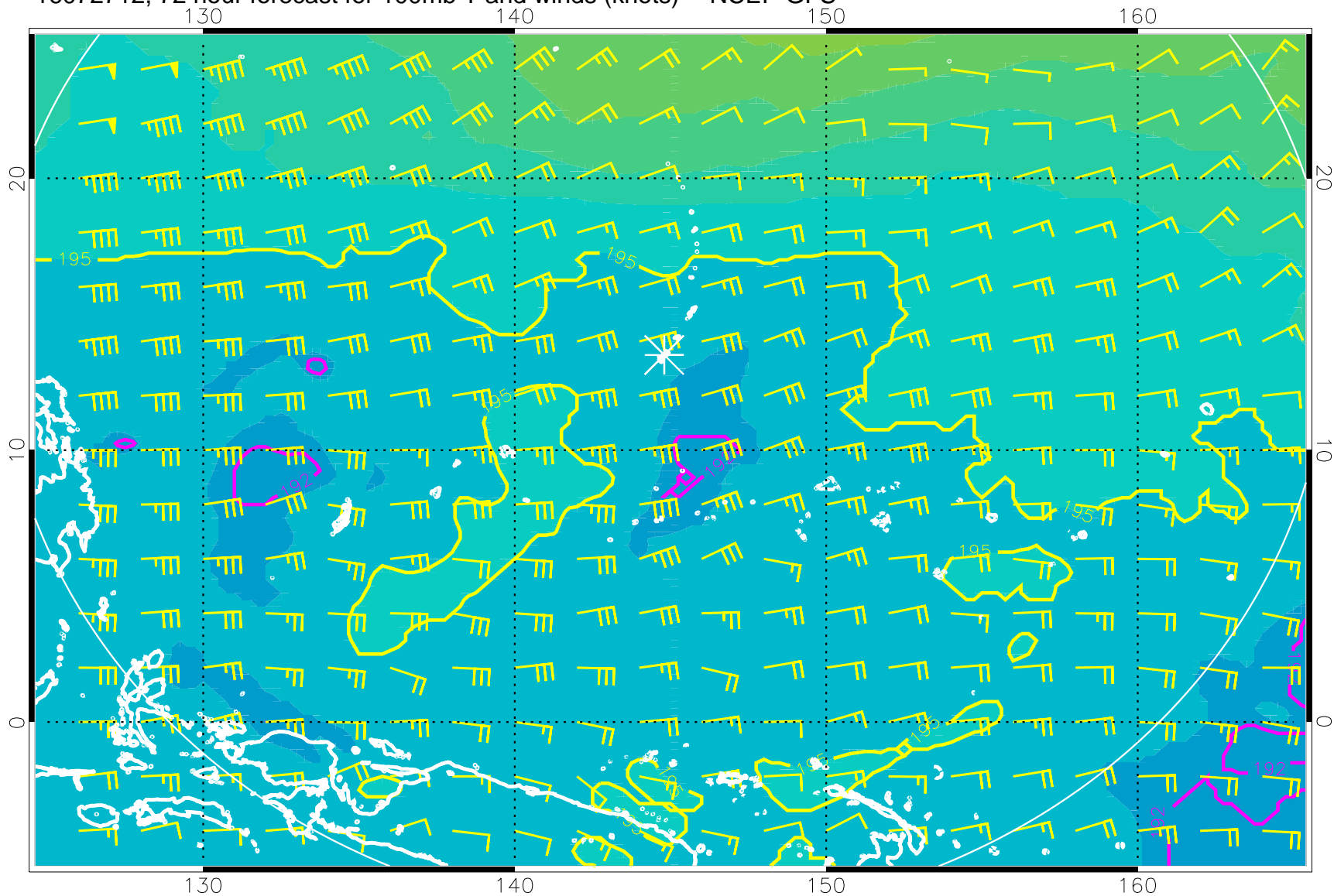
16072712, 72 hour forecast for 100mb T and winds (knots) -- NCEP GFS
