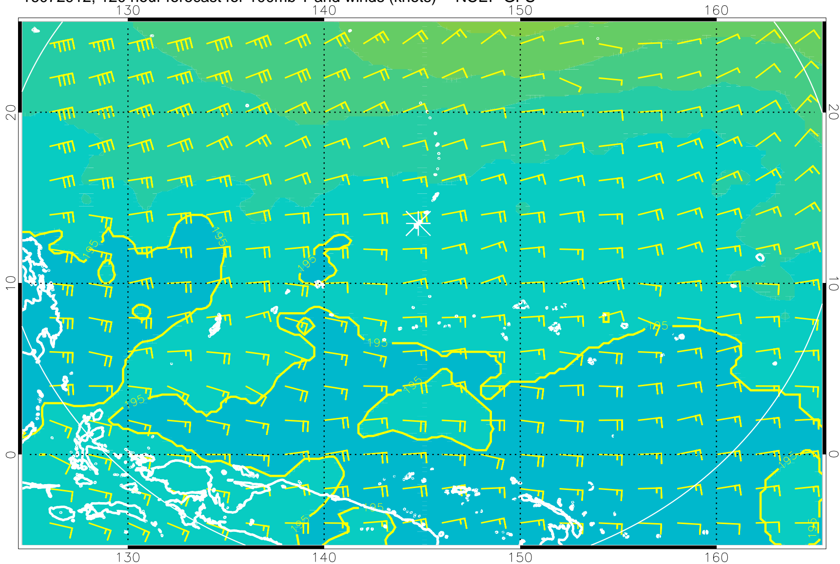
16072912, 120 hour forecast for 100mb T and winds (knots) -- NCEP GFS
