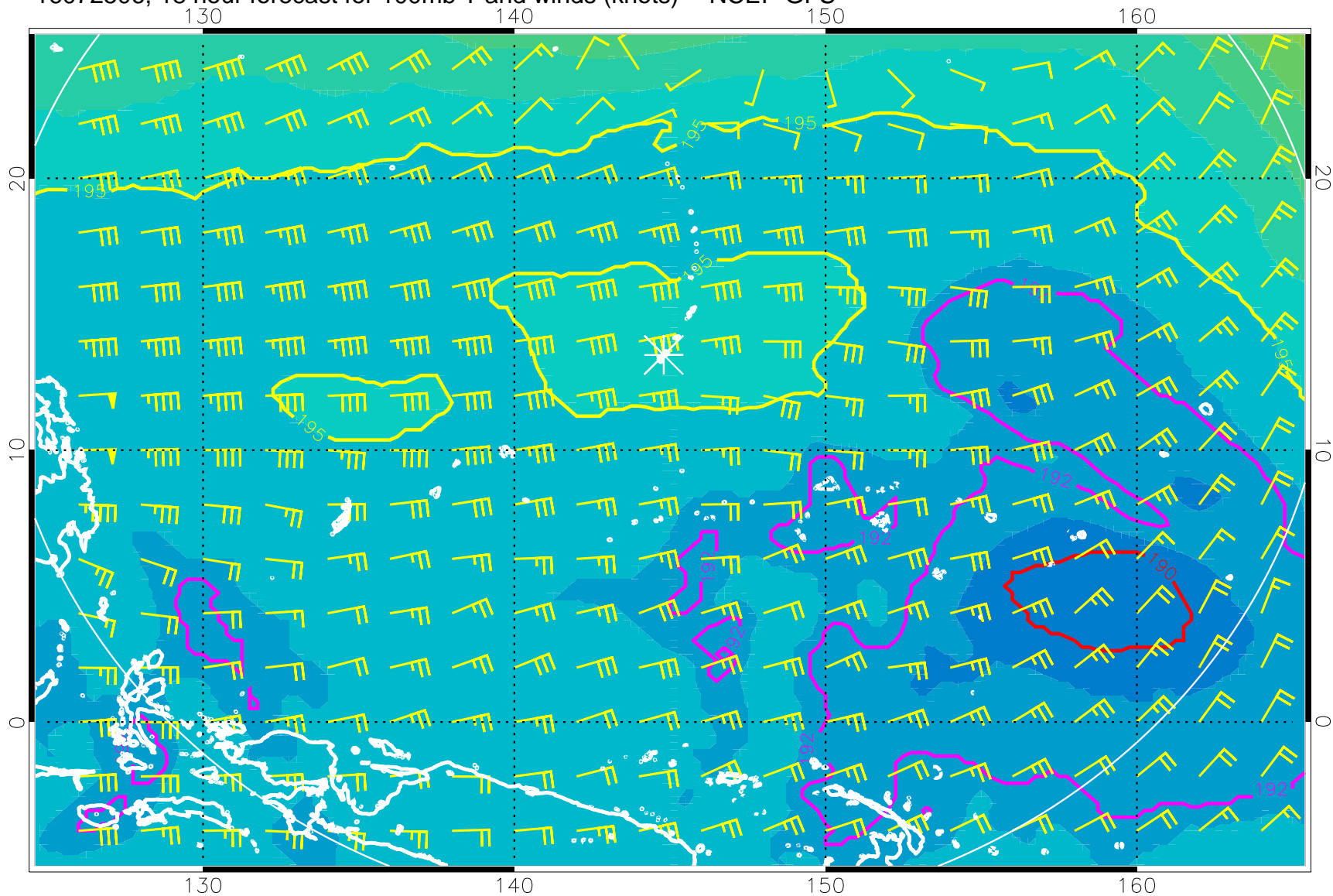
16072506, 18 hour forecast for 100mb T and winds (knots) -- NCEP GFS
