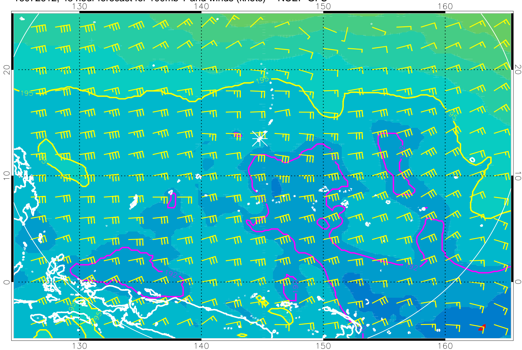
16072612, 48 hour forecast for 100mb T and winds (knots) -- NCEP GFS
