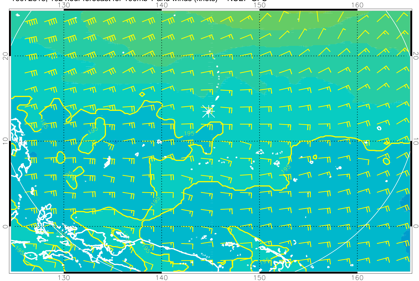
16072818, 102 hour forecast for 100mb T and winds (knots) -- NCEP GFS
