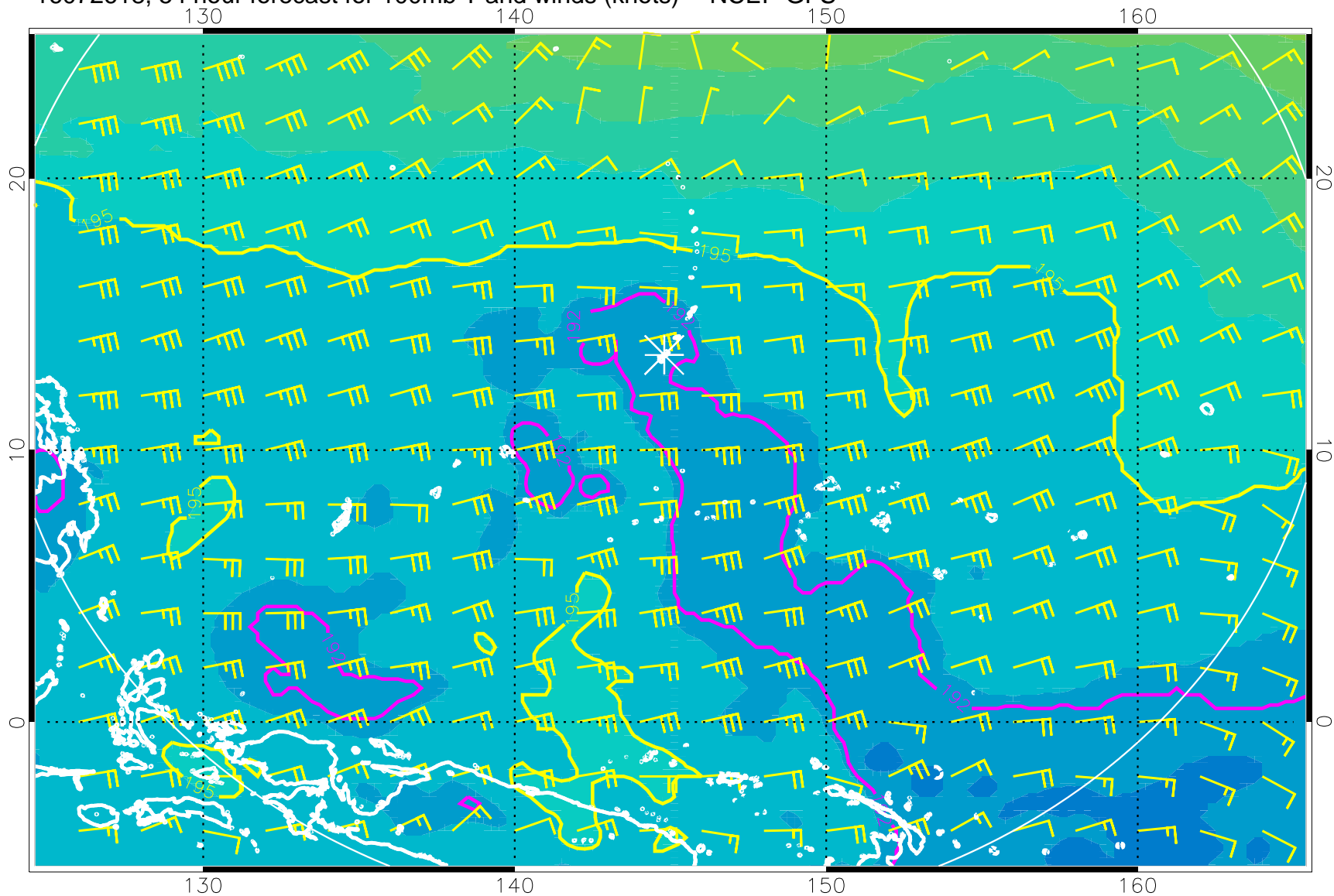
16072618, 54 hour forecast for 100mb T and winds (knots) -- NCEP GFS
