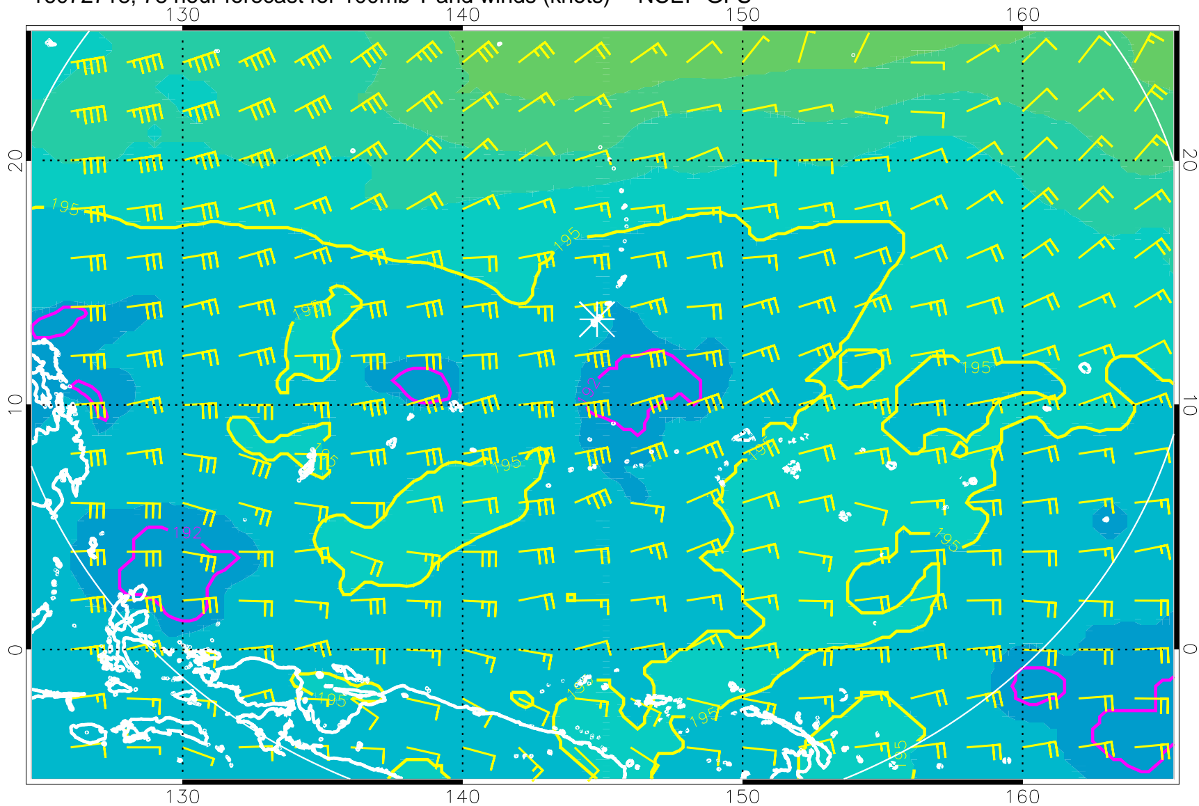
16072718, 78 hour forecast for 100mb T and winds (knots) -- NCEP GFS
