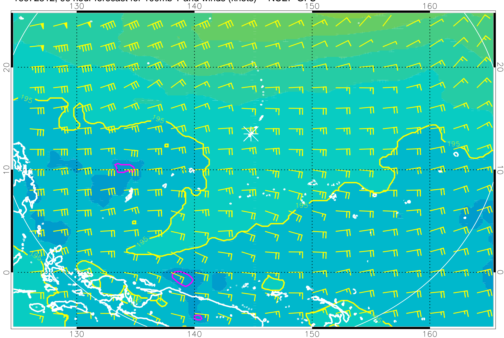
16072812, 96 hour forecast for 100mb T and winds (knots) -- NCEP GFS
