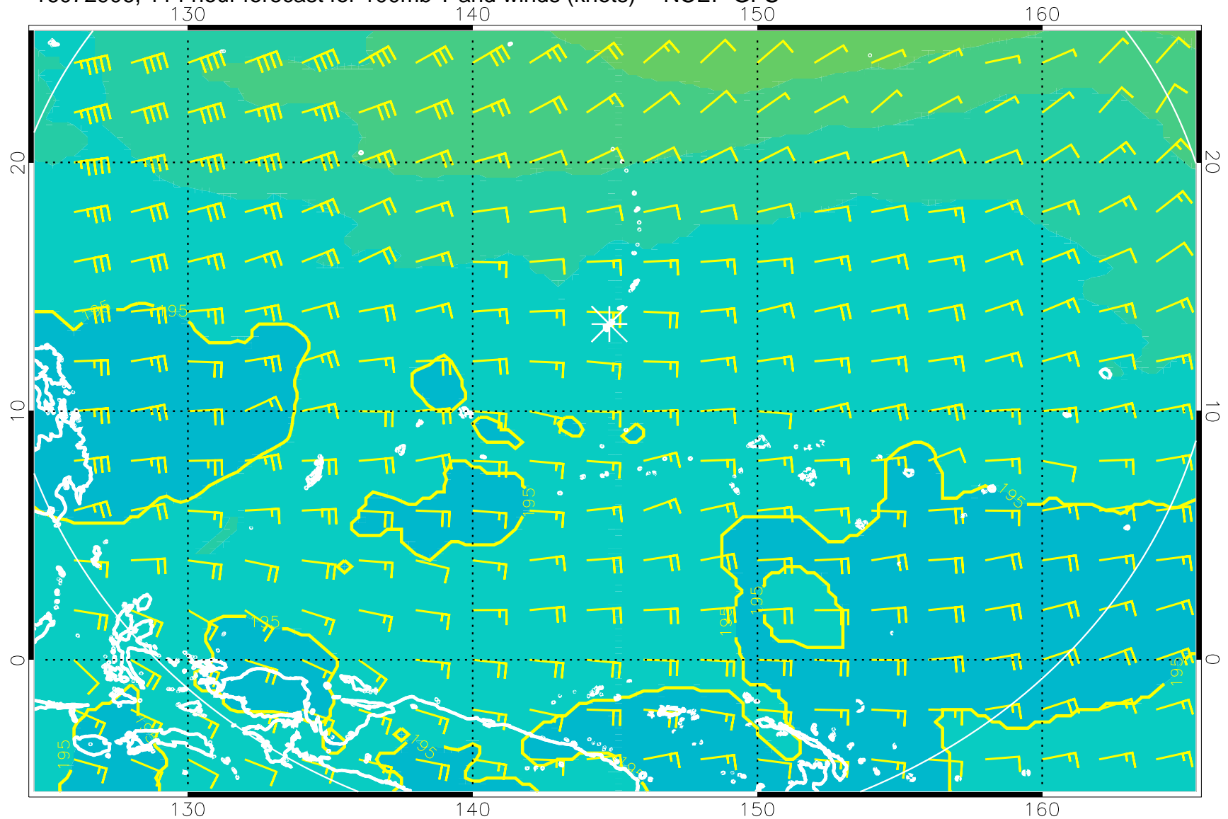
16072906, 114 hour forecast for 100mb T and winds (knots) -- NCEP GFS
