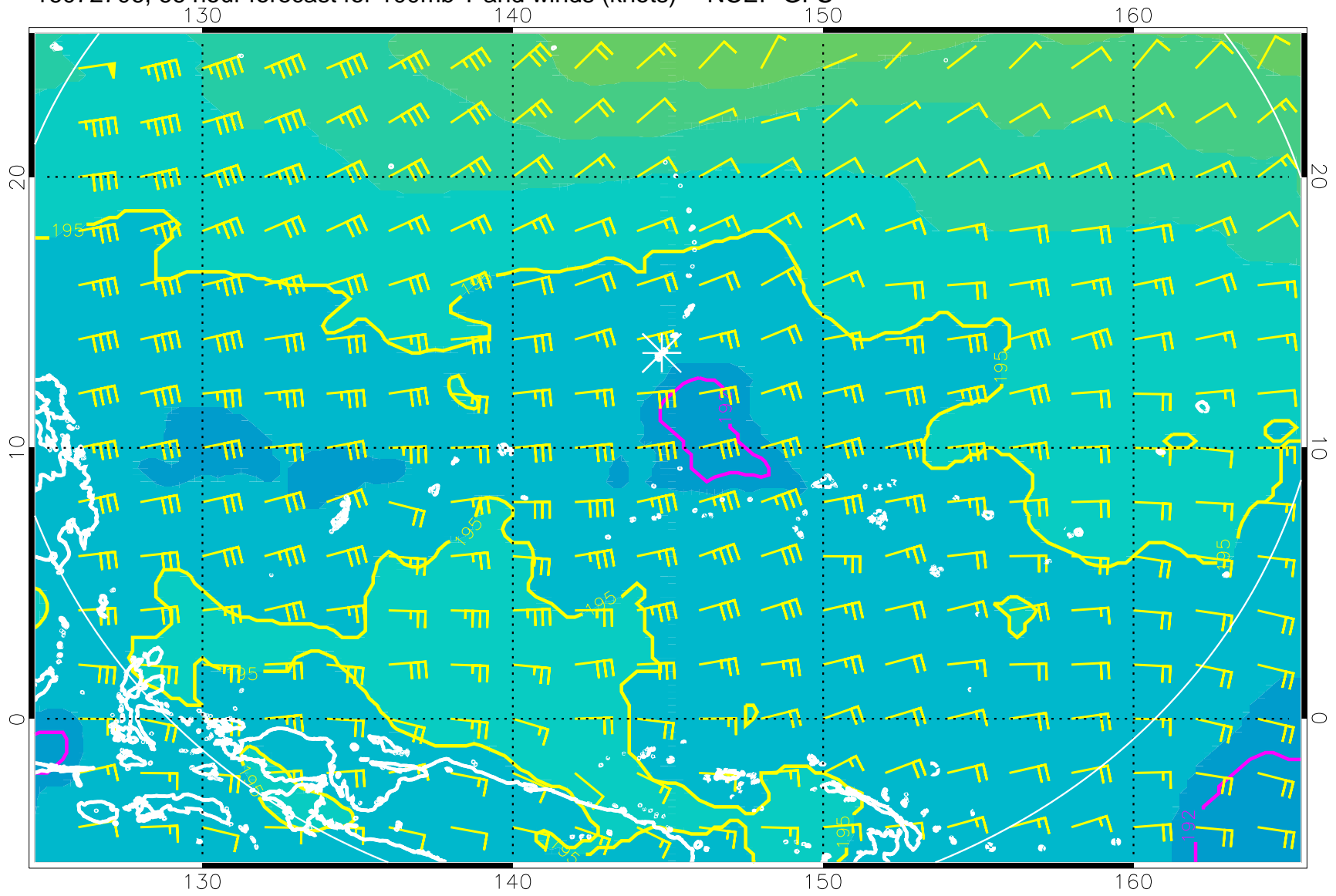
16072706, 66 hour forecast for 100mb T and winds (knots) -- NCEP GFS
