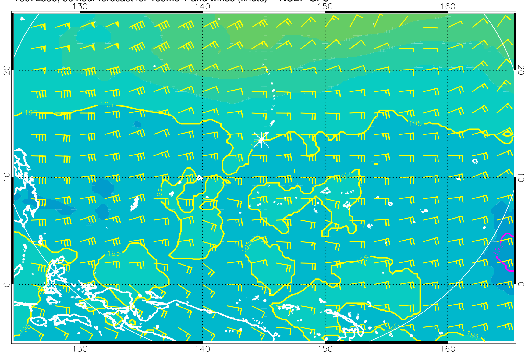
16072806, 90 hour forecast for 100mb T and winds (knots) -- NCEP GFS
