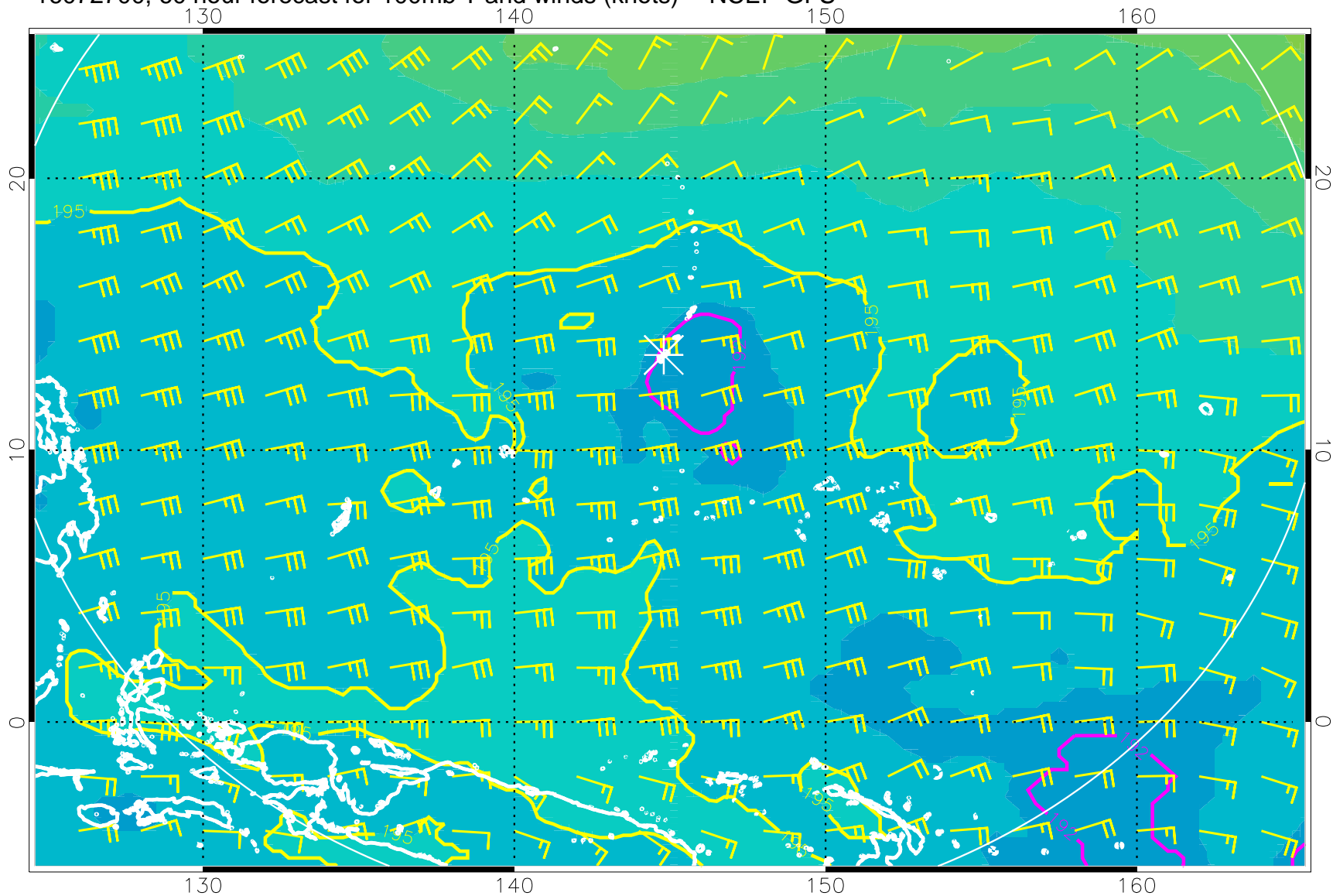
16072700, 60 hour forecast for 100mb T and winds (knots) -- NCEP GFS
