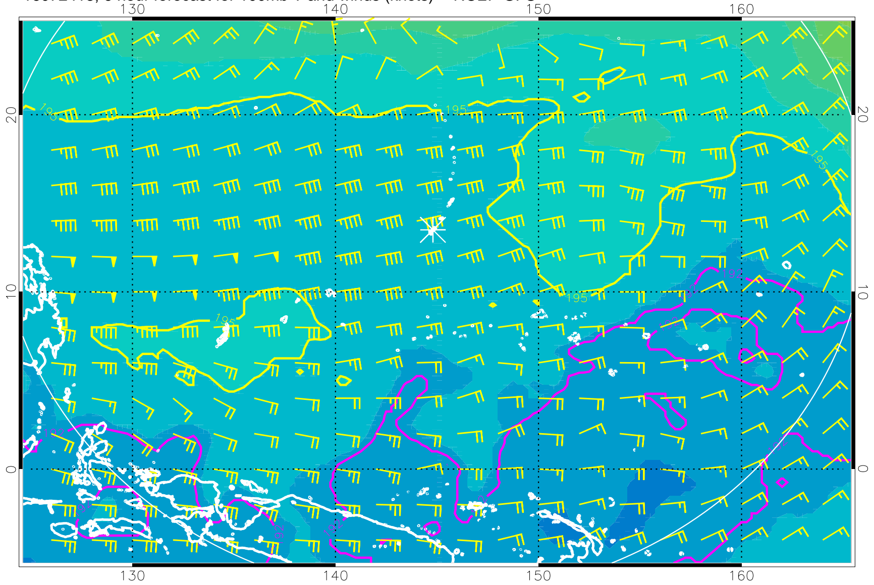
16072418, 6 hour forecast for 100mb T and winds (knots) -- NCEP GFS
