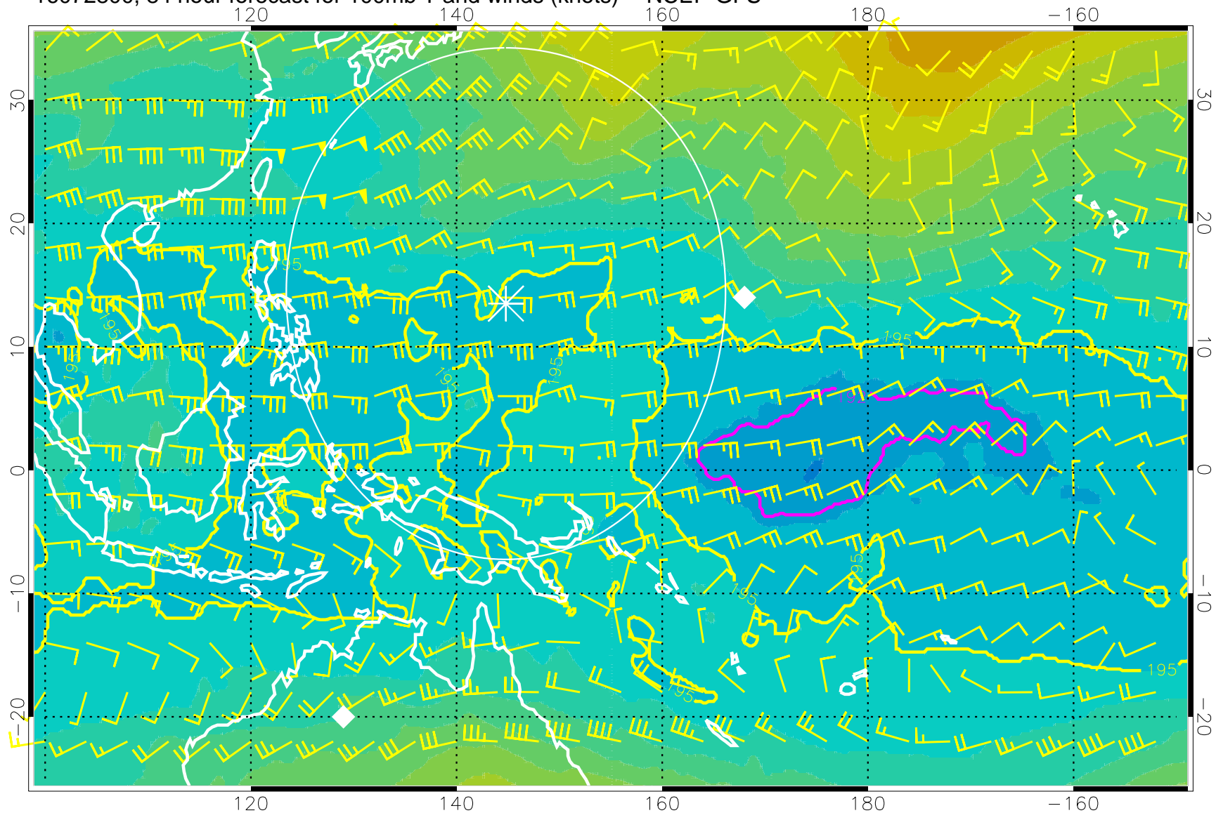
16072800, 84 hour forecast for 100mb T and winds (knots) -- NCEP GFS
