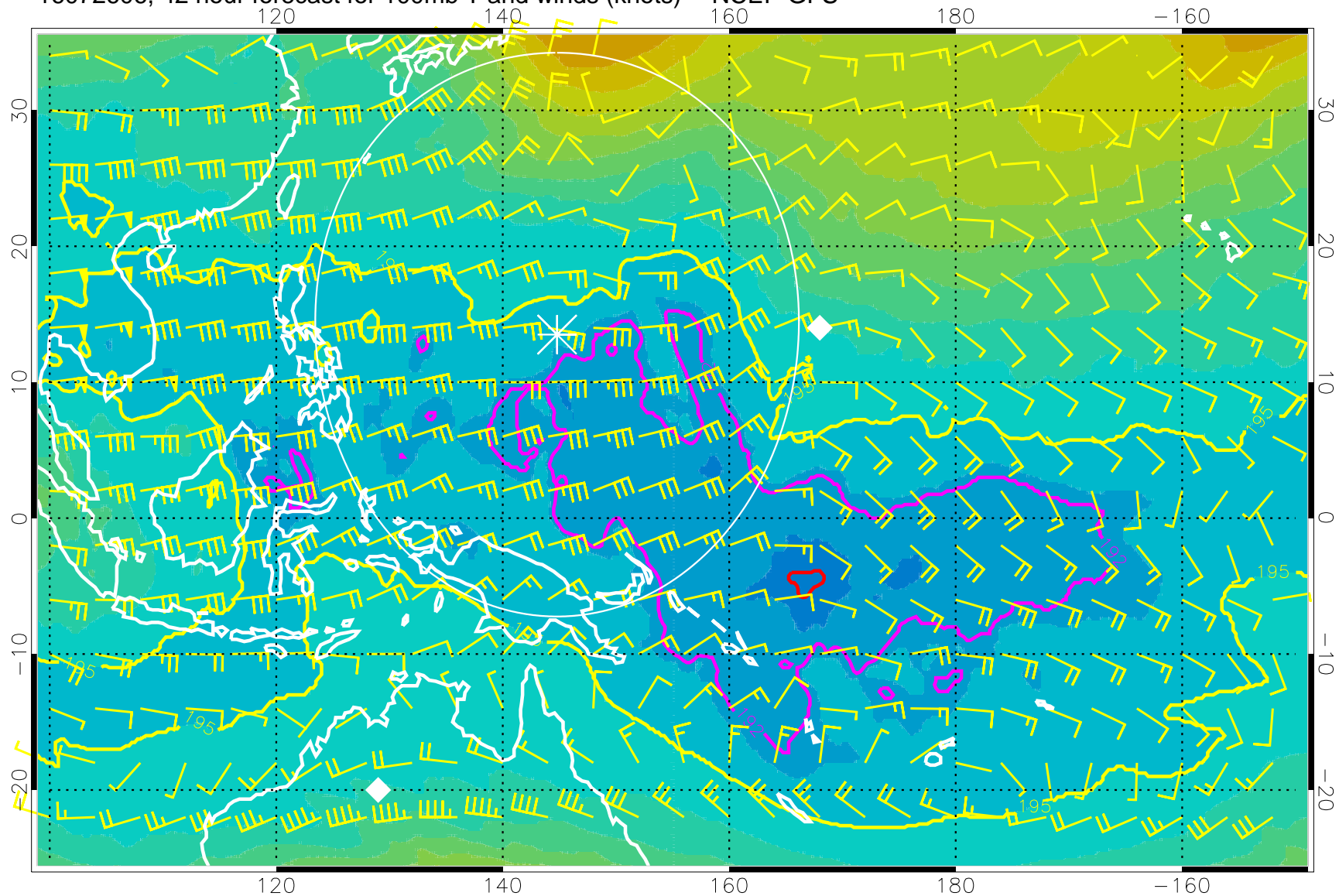
16072606, 42 hour forecast for 100mb T and winds (knots) -- NCEP GFS
