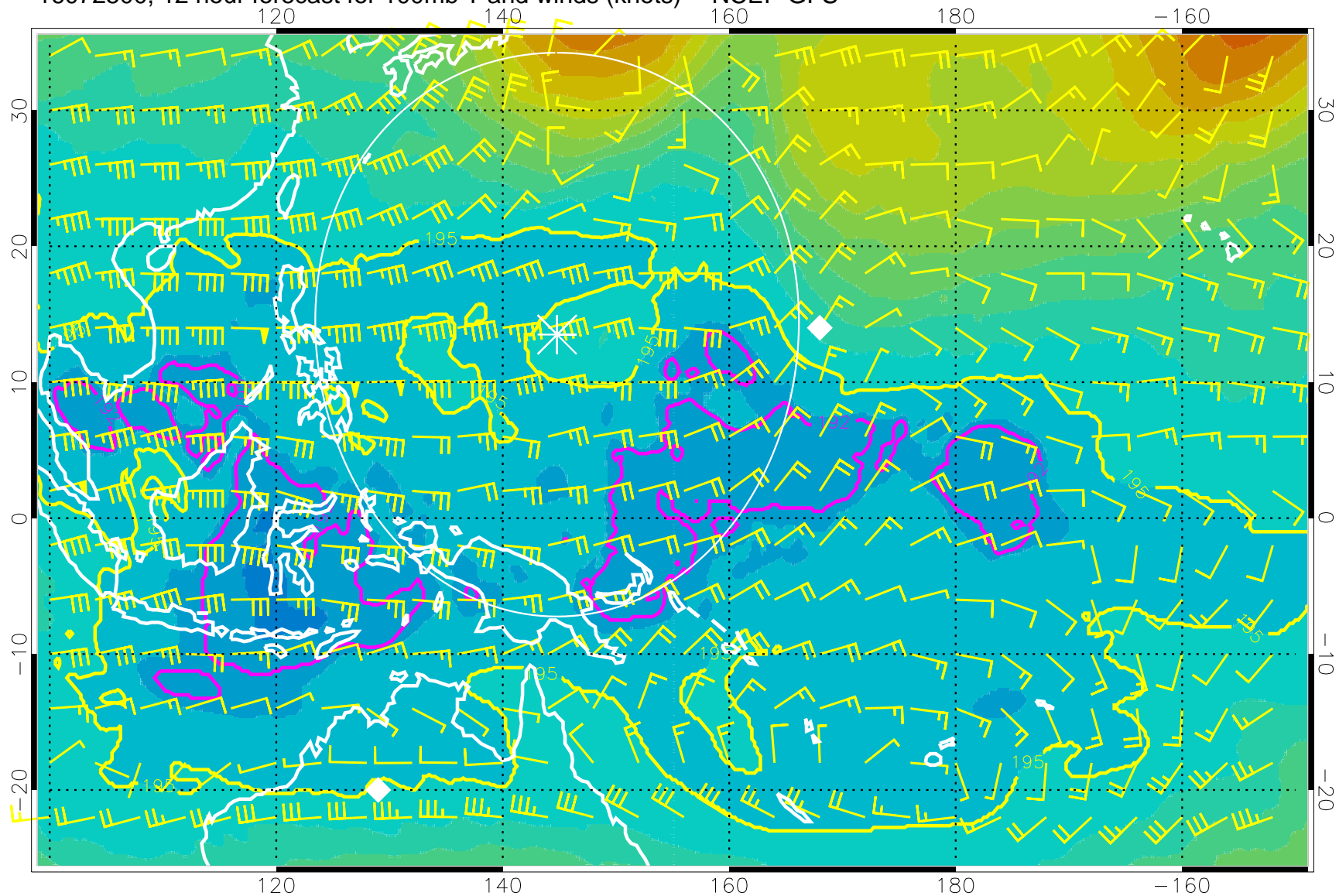
16072500, 12 hour forecast for 100mb T and winds (knots) -- NCEP GFS
