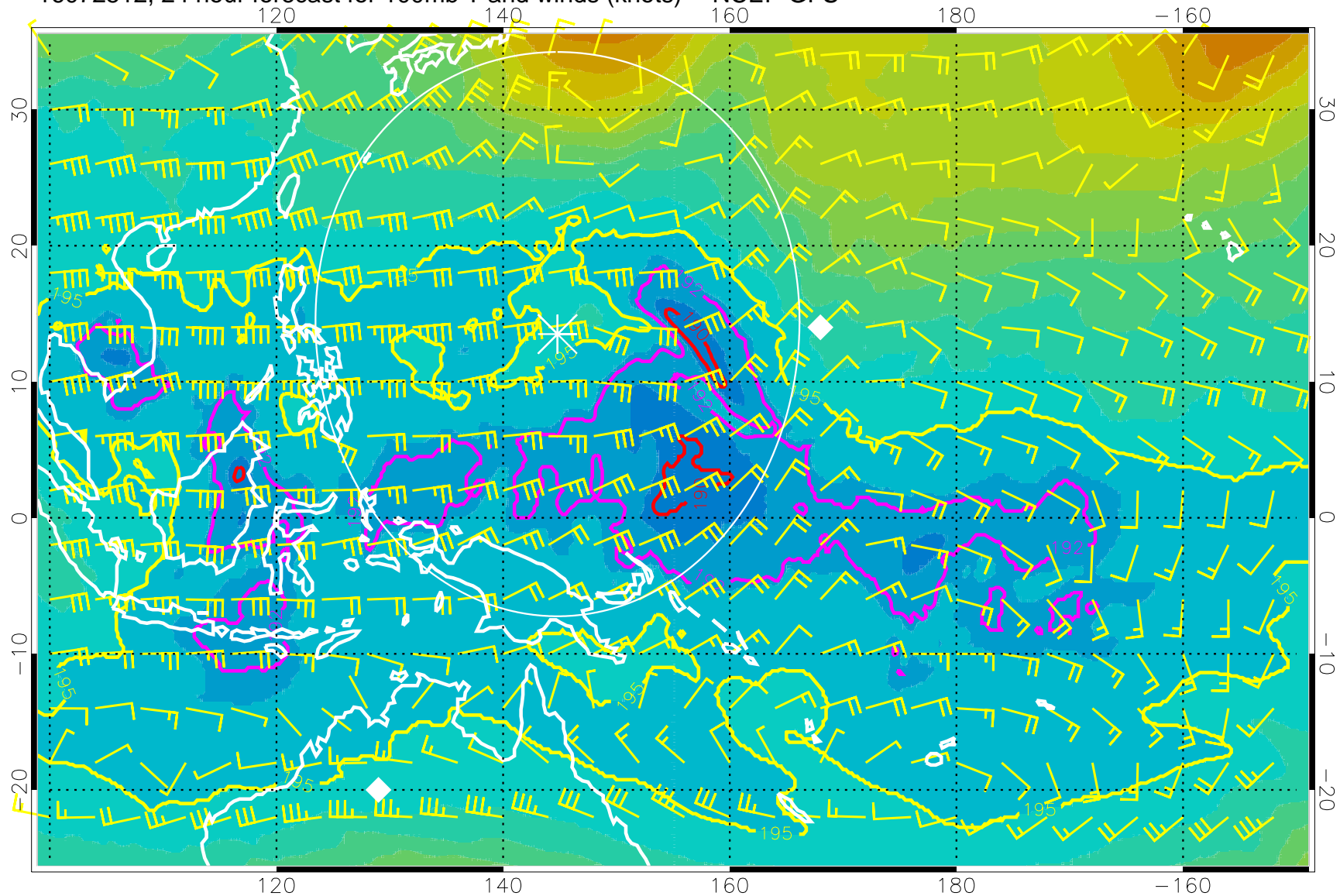
16072512, 24 hour forecast for 100mb T and winds (knots) -- NCEP GFS
