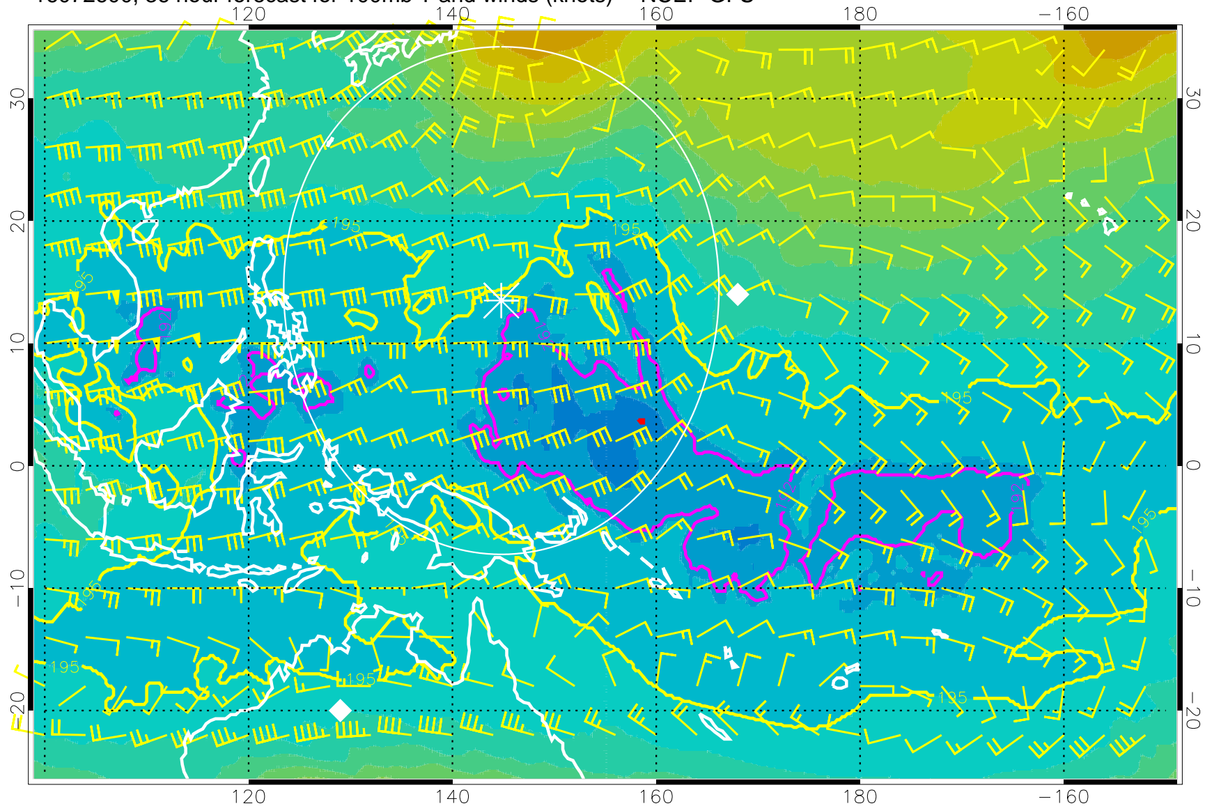
16072600, 36 hour forecast for 100mb T and winds (knots) -- NCEP GFS
