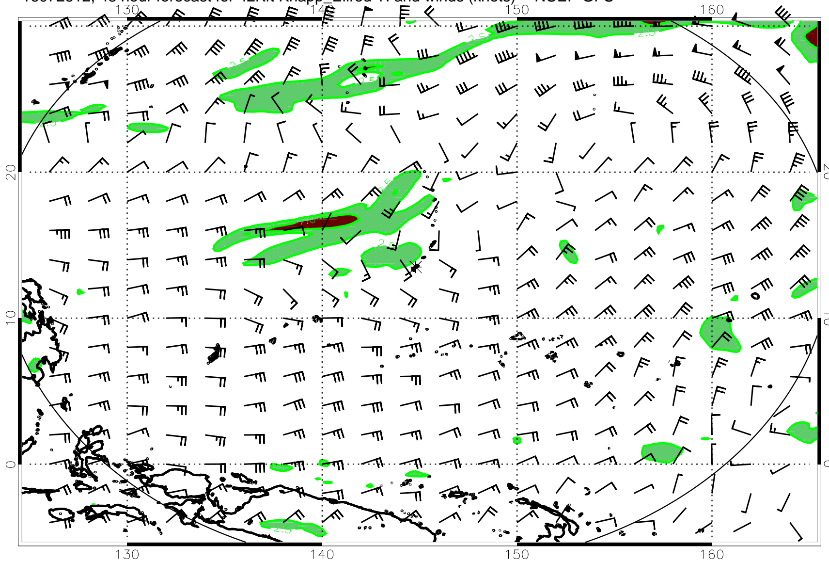
16072612, 48 hour forecast for 42Kft Knapp_Ellrod TI and winds (knots) -- NCEP GFS
