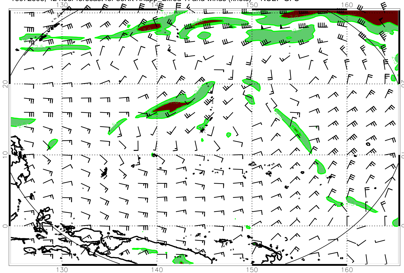
16072606, 42 hour forecast for 36Kft Knapp_Ellrod TI and winds (knots) -- NCEP GFS
