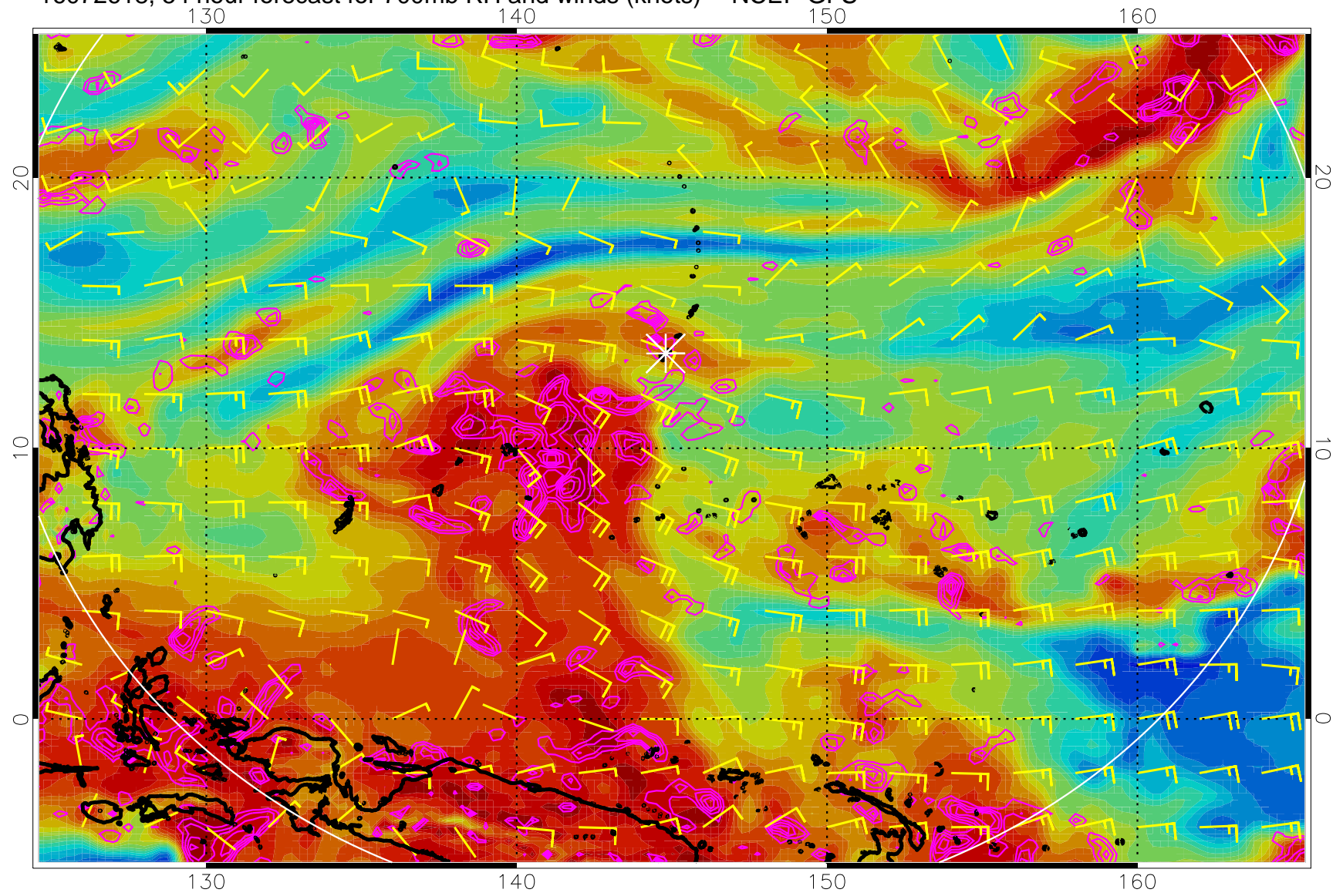
16072618, 54 hour forecast for 700mb RH and winds (knots) -- NCEP GFS
