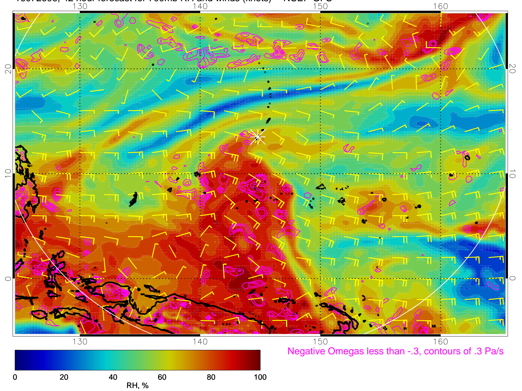
16072606, 42 hour forecast for 700mb RH and winds (knots) -- NCEP GFS
