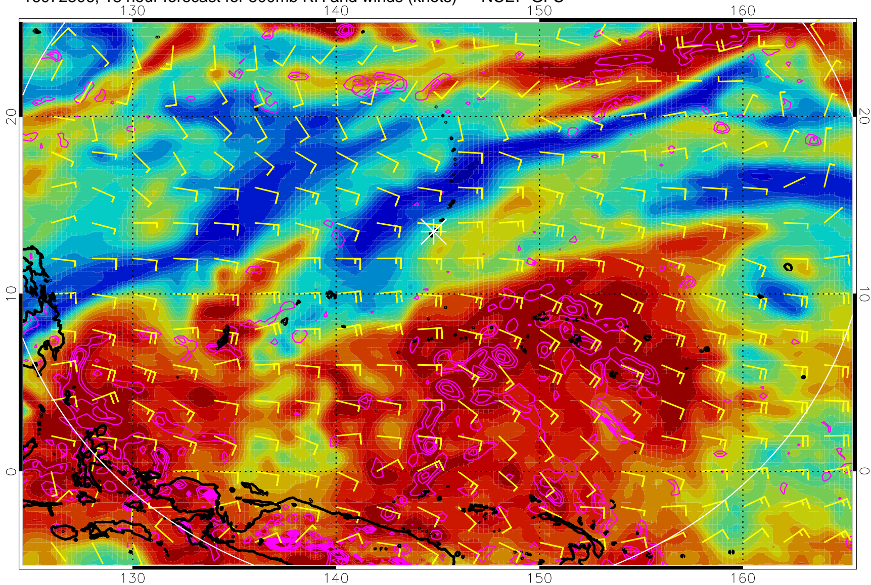
16072506, 18 hour forecast for 500mb RH and winds (knots) -- NCEP GFS
