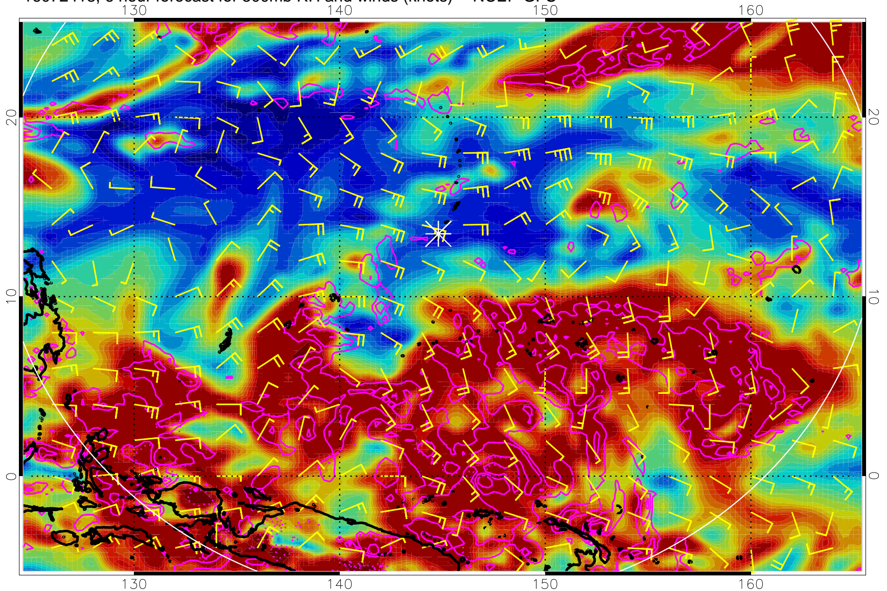
16072418, 6 hour forecast for 300mb RH and winds (knots) -- NCEP GFS
