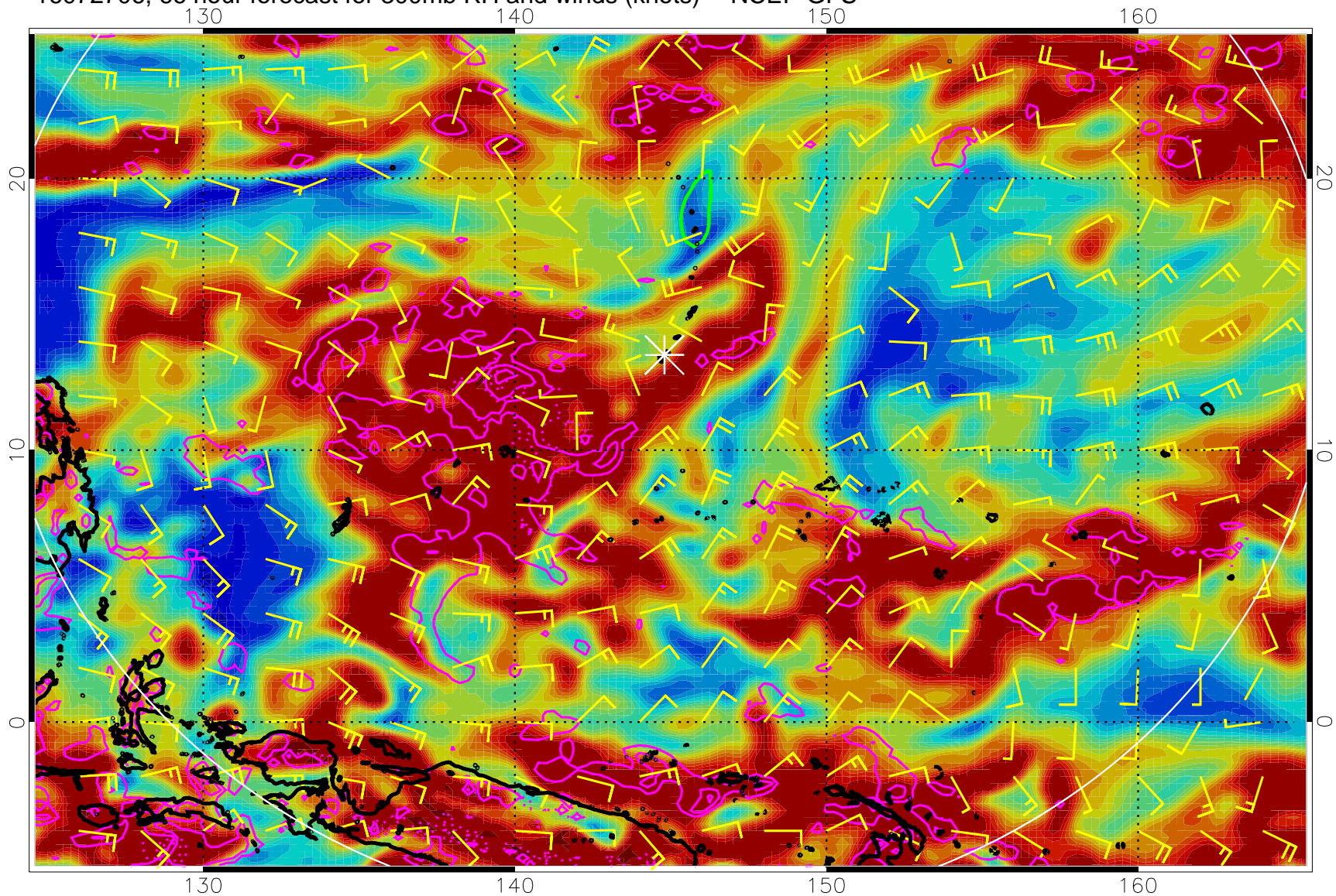
16072706, 66 hour forecast for 300mb RH and winds (knots) -- NCEP GFS
