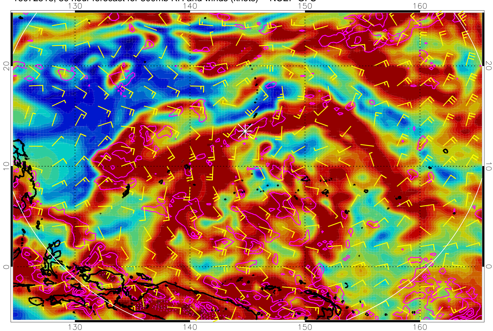
16072518, 30 hour forecast for 300mb RH and winds (knots) -- NCEP GFS
