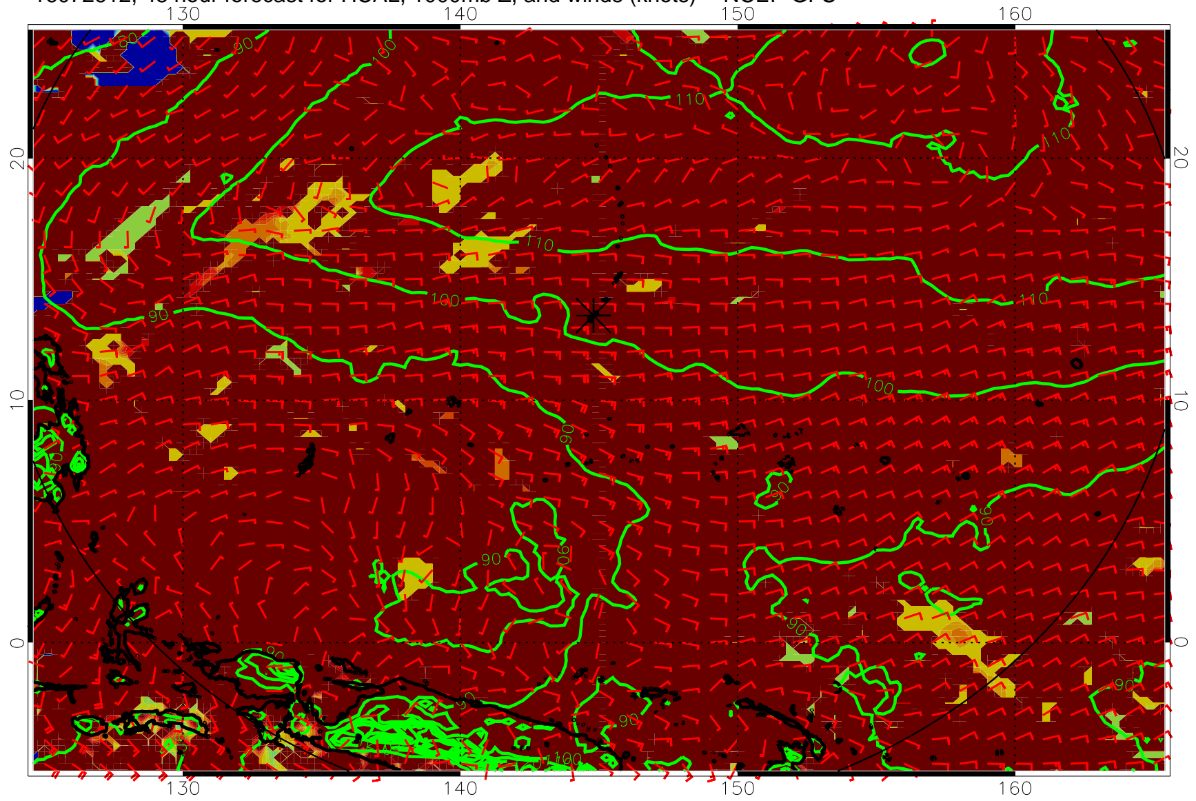
16072612, 48 hour forecast for HCAL, 1000mb Z, and winds (knots) -- NCEP GFS
