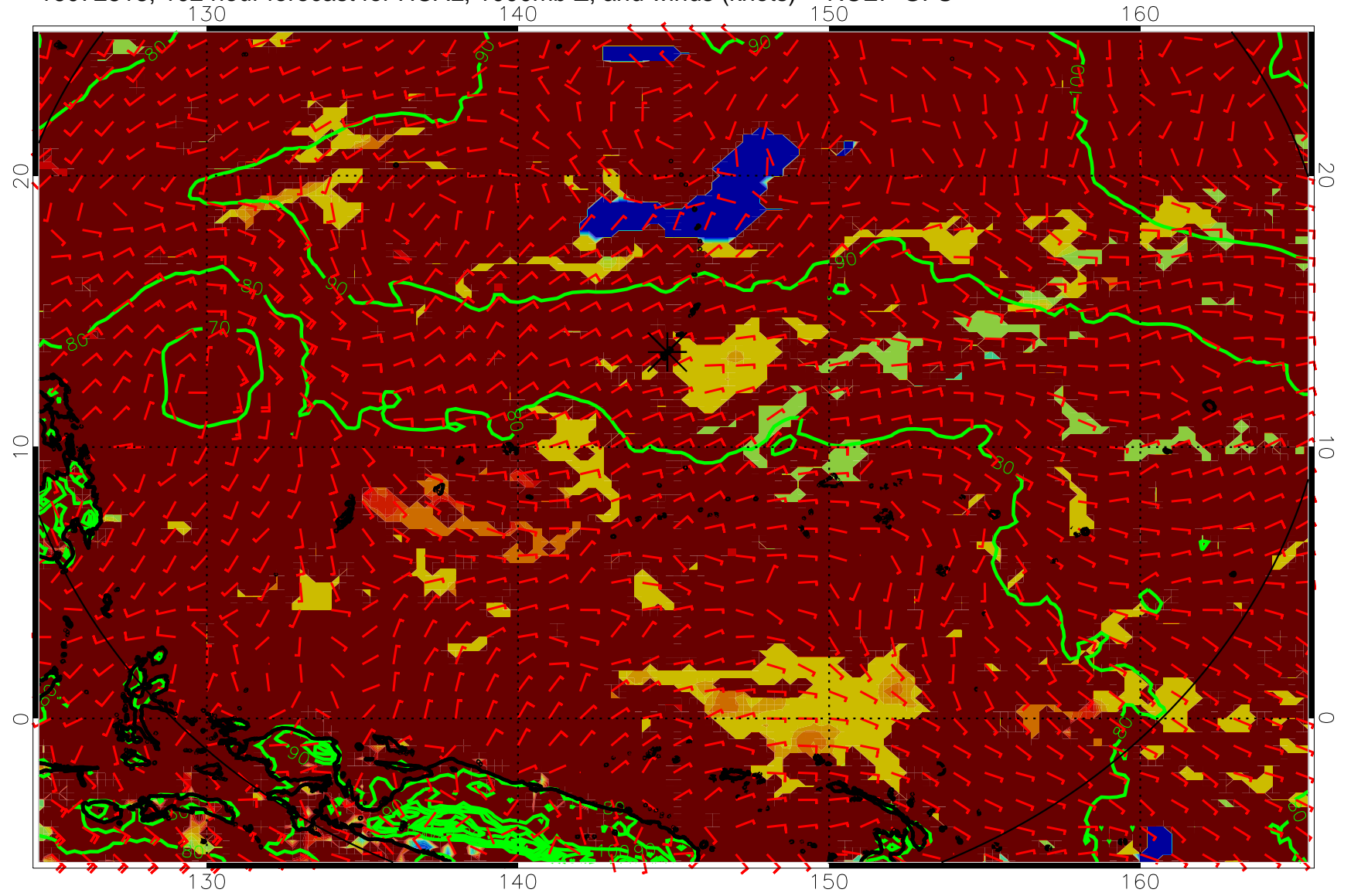
16072818, 102 hour forecast for HCAL, 1000mb Z, and winds (knots) -- NCEP GFS
