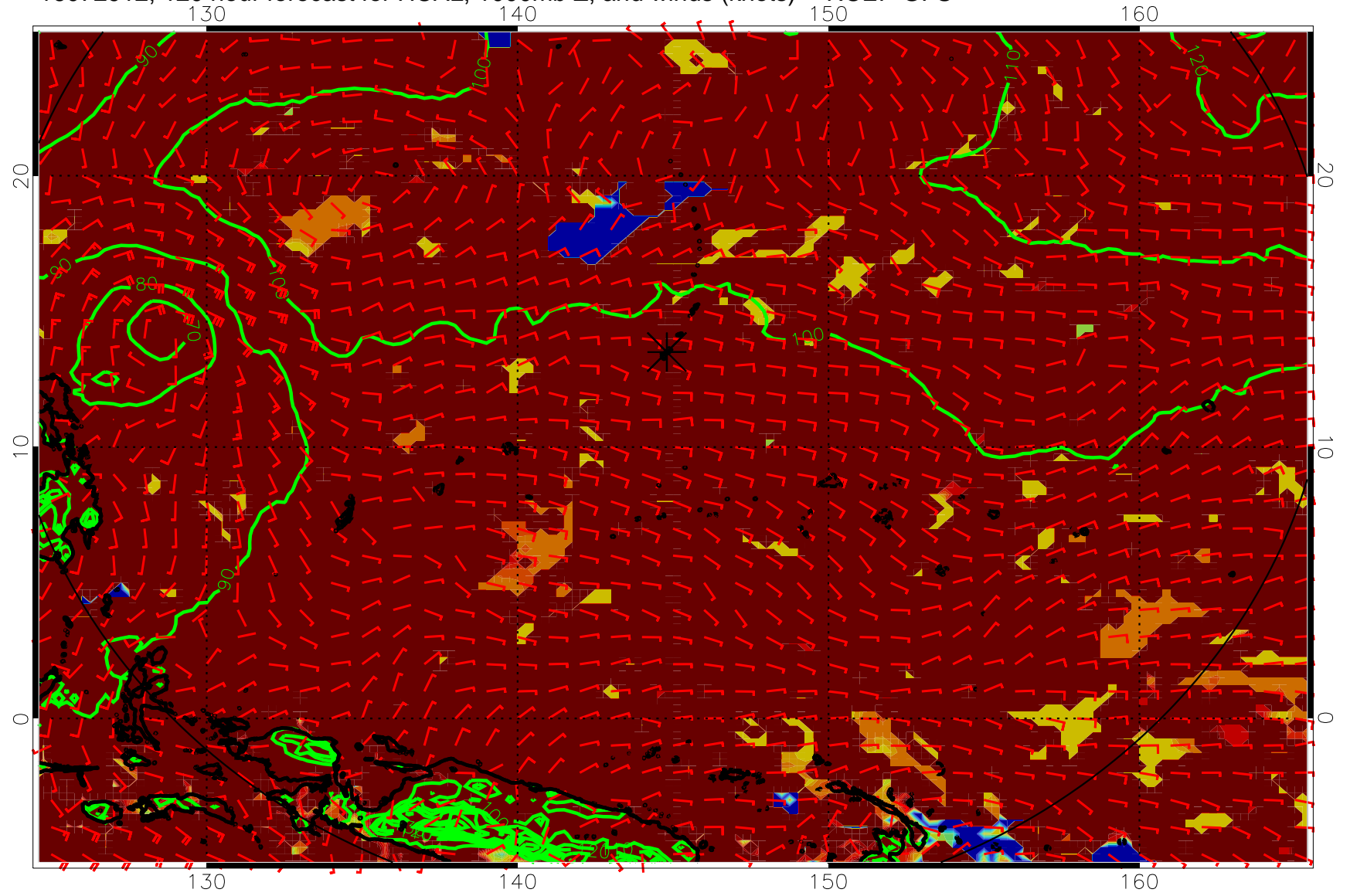
16072912, 120 hour forecast for HCAL, 1000mb Z, and winds (knots) -- NCEP GFS
