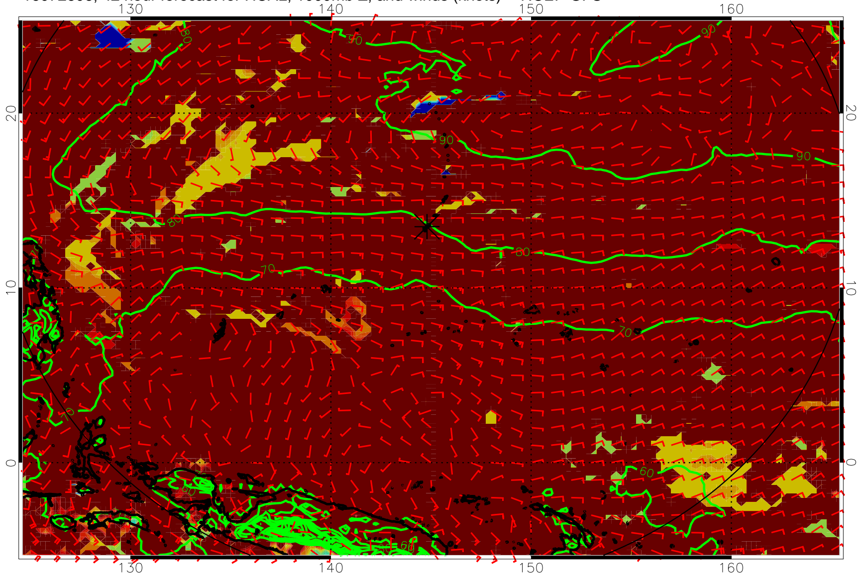
16072606, 42 hour forecast for HCAL, 1000mb Z, and winds (knots) -- NCEP GFS
