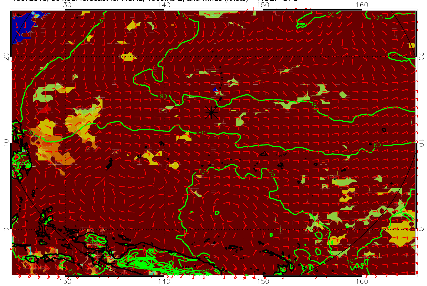
16072518, 30 hour forecast for HCAL, 1000mb Z, and winds (knots) -- NCEP GFS
