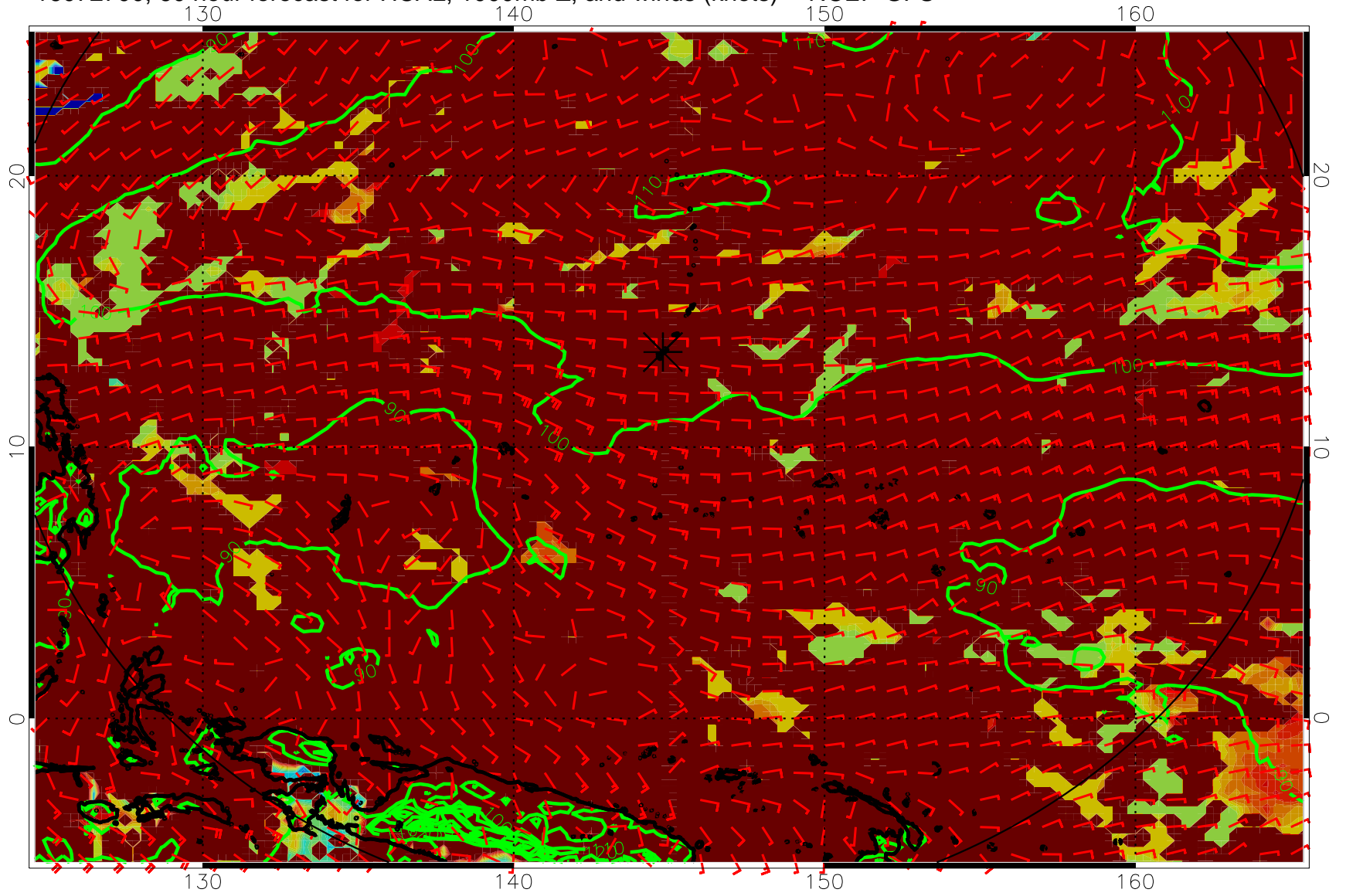
16072700, 60 hour forecast for HCAL, 1000mb Z, and winds (knots) -- NCEP GFS
