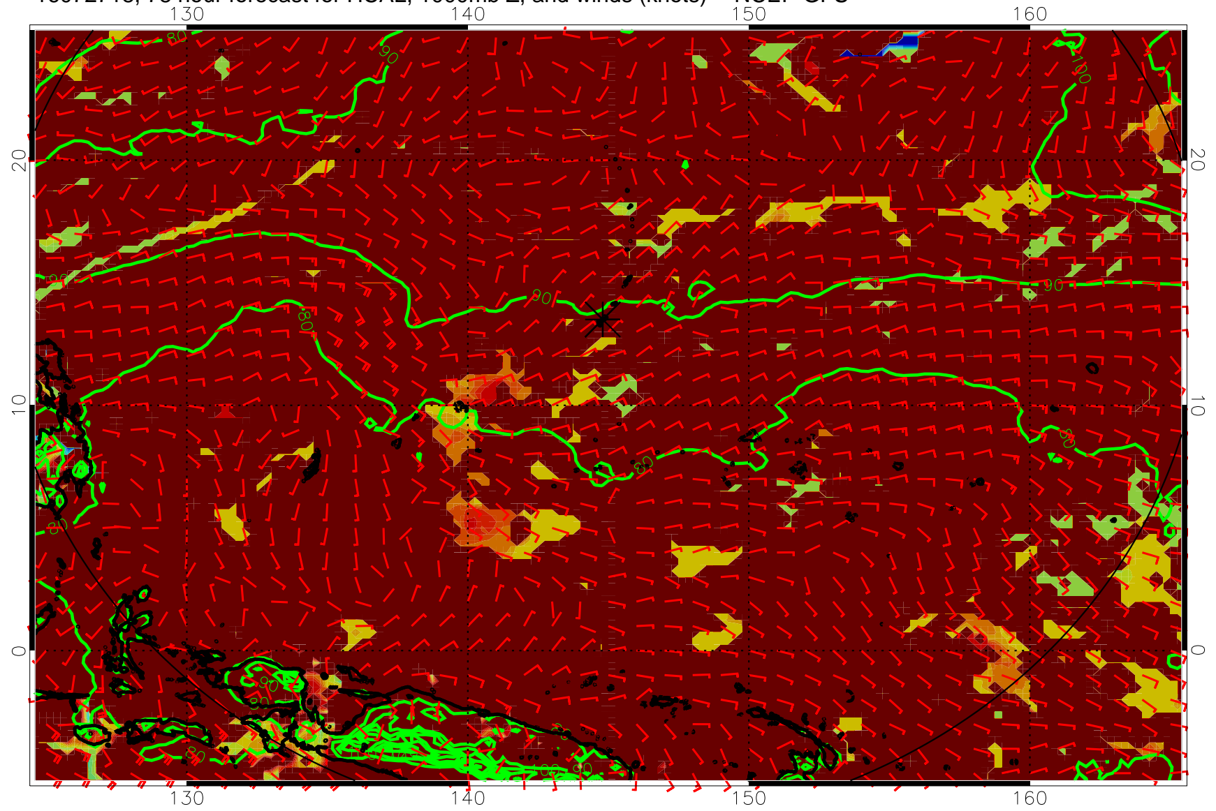
16072718, 78 hour forecast for HCAL, 1000mb Z, and winds (knots) -- NCEP GFS
