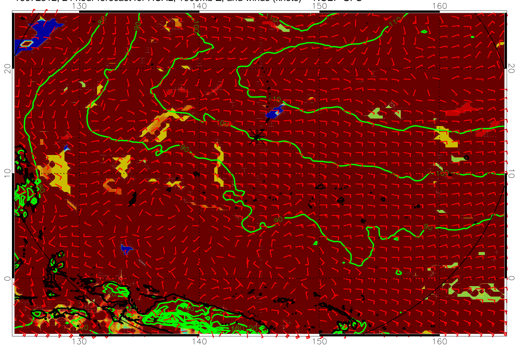
16072512, 24 hour forecast for HCAL, 1000mb Z, and winds (knots) -- NCEP GFS
