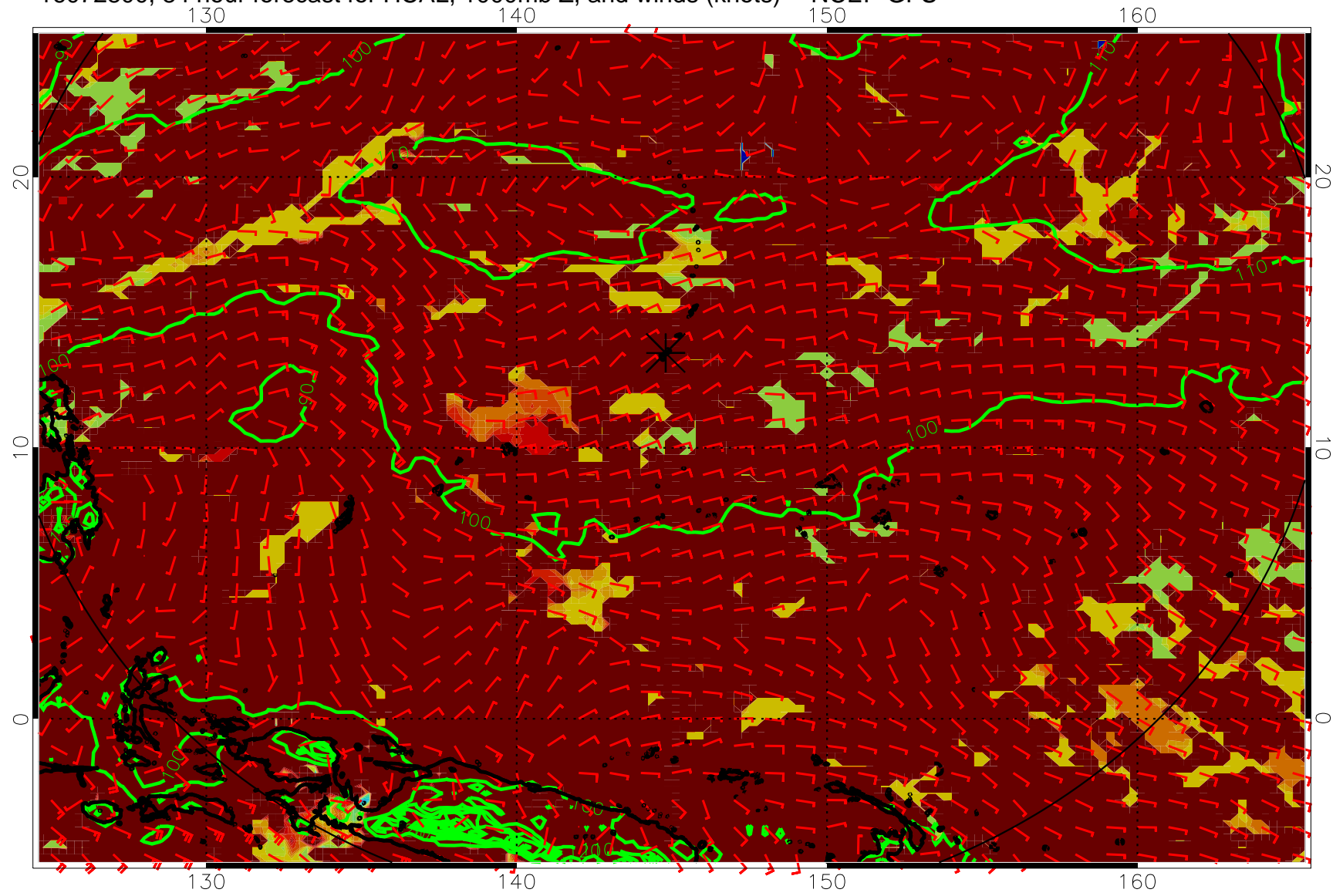
16072800, 84 hour forecast for HCAL, 1000mb Z, and winds (knots) -- NCEP GFS
