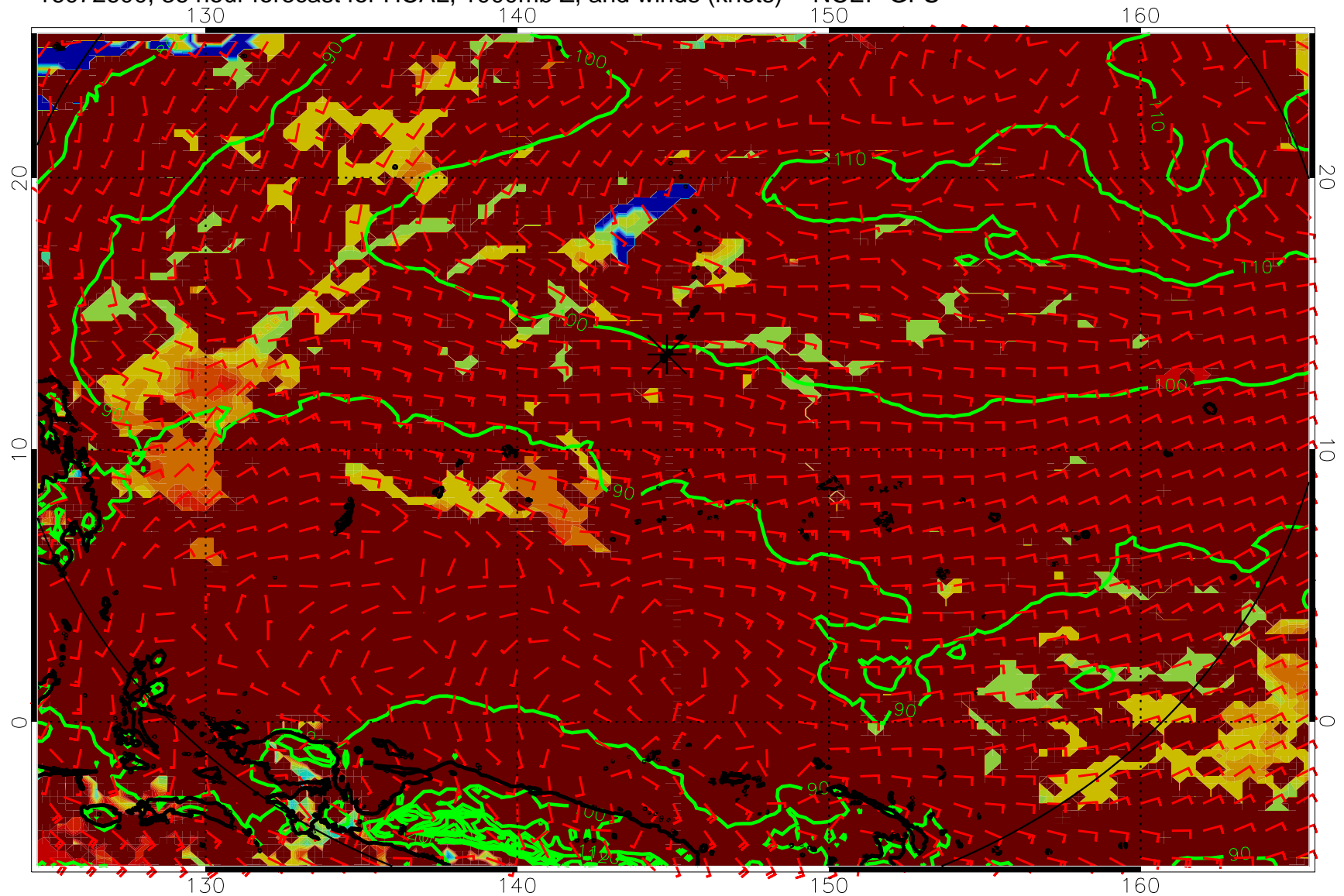
16072600, 36 hour forecast for HCAL, 1000mb Z, and winds (knots) -- NCEP GFS
