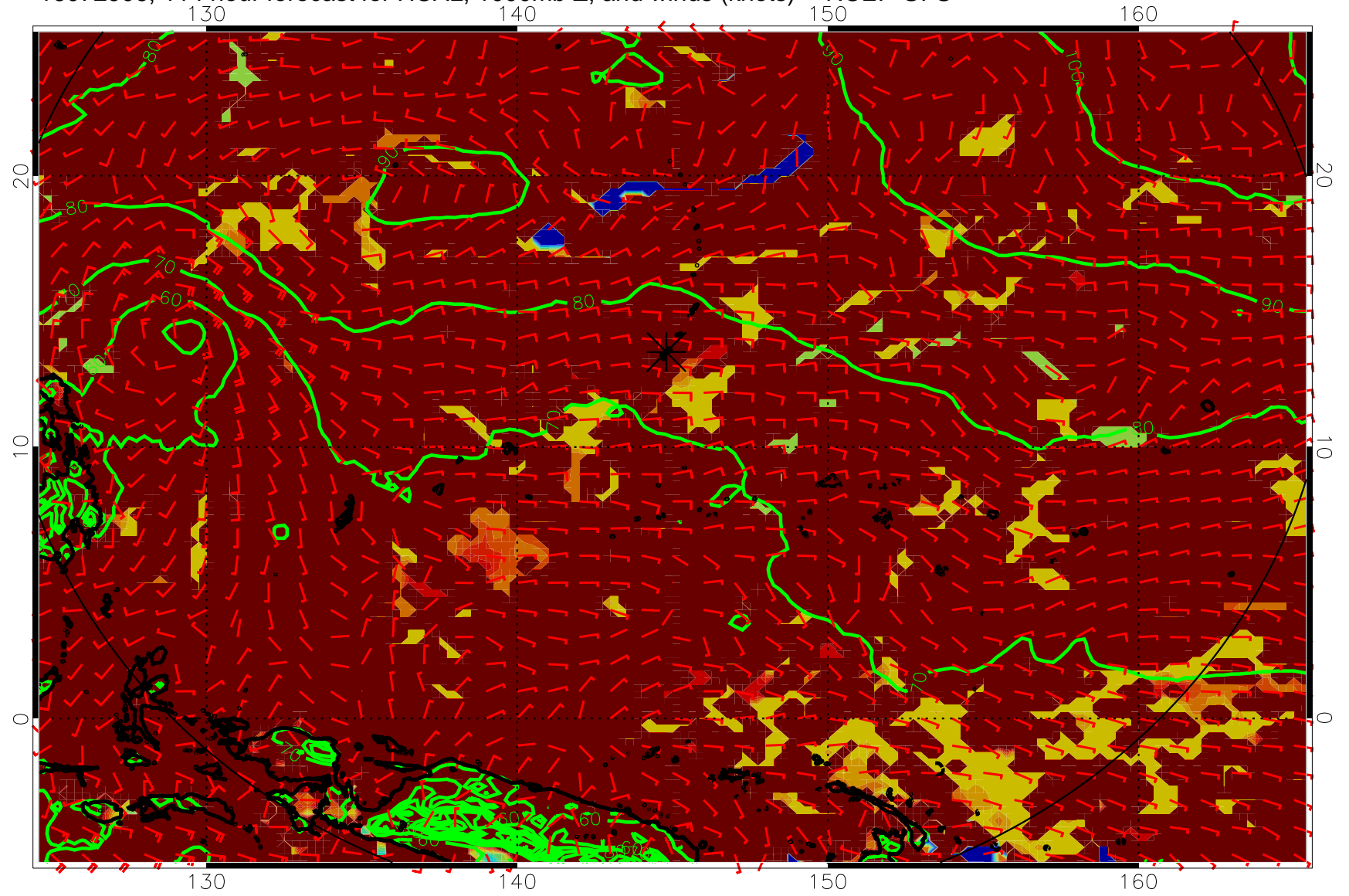
16072906, 114 hour forecast for HCAL, 1000mb Z, and winds (knots) -- NCEP GFS
