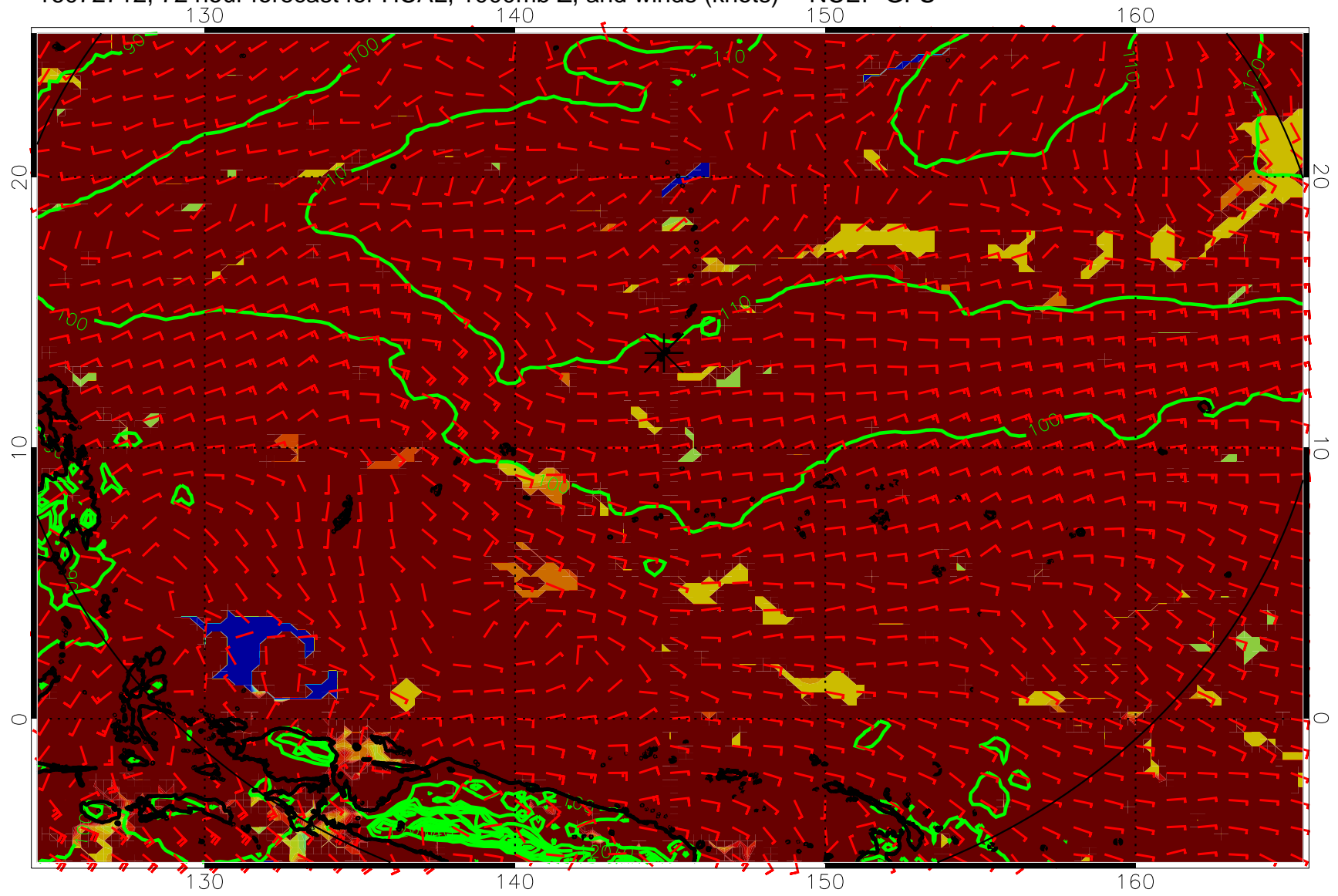
16072712, 72 hour forecast for HCAL, 1000mb Z, and winds (knots) -- NCEP GFS
