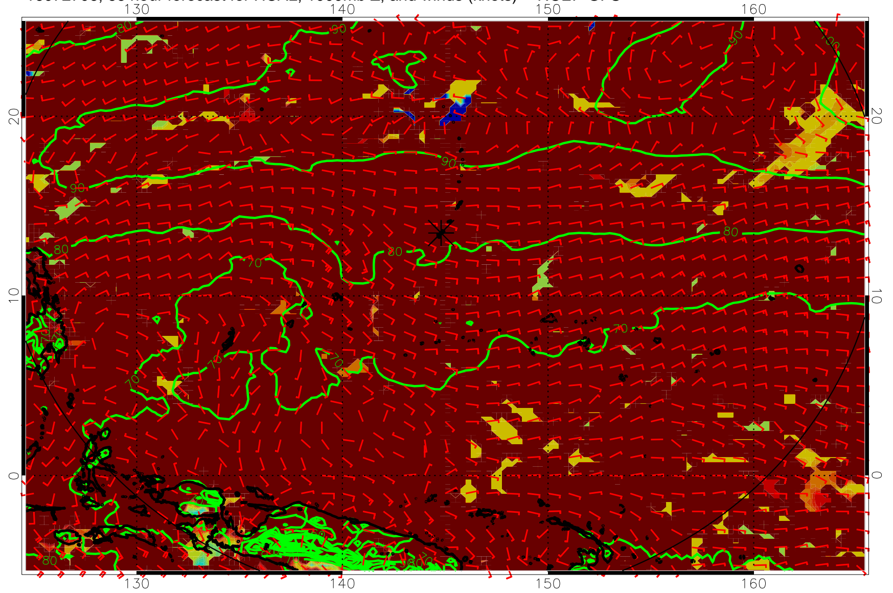
16072706, 66 hour forecast for HCAL, 1000mb Z, and winds (knots) -- NCEP GFS
