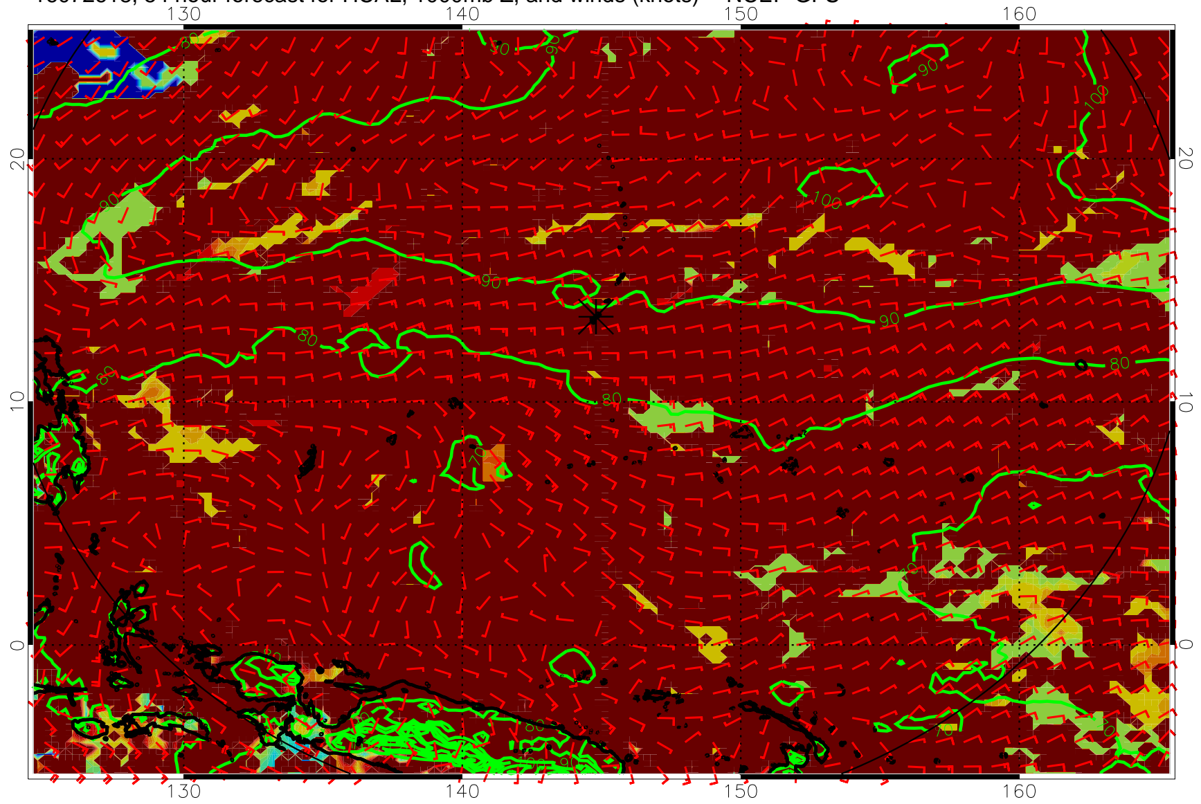
16072618, 54 hour forecast for HCAL, 1000mb Z, and winds (knots) -- NCEP GFS
