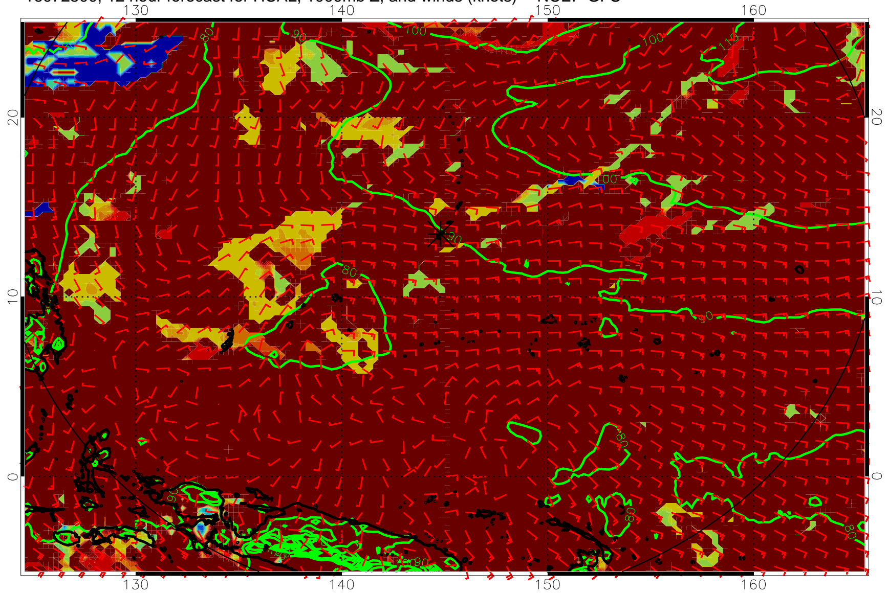
16072500, 12 hour forecast for HCAL, 1000mb Z, and winds (knots) -- NCEP GFS
