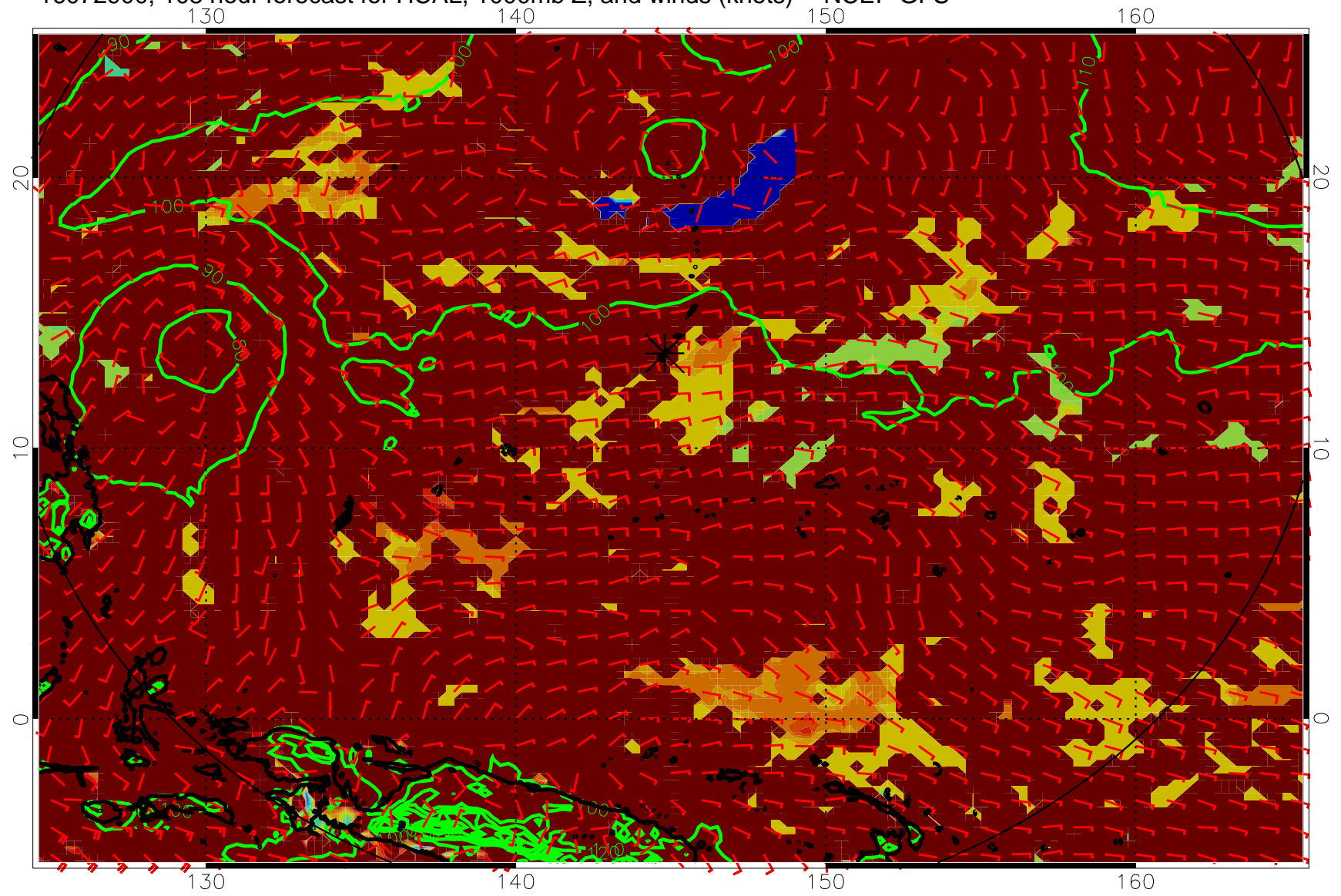
16072900, 108 hour forecast for HCAL, 1000mb Z, and winds (knots) -- NCEP GFS
