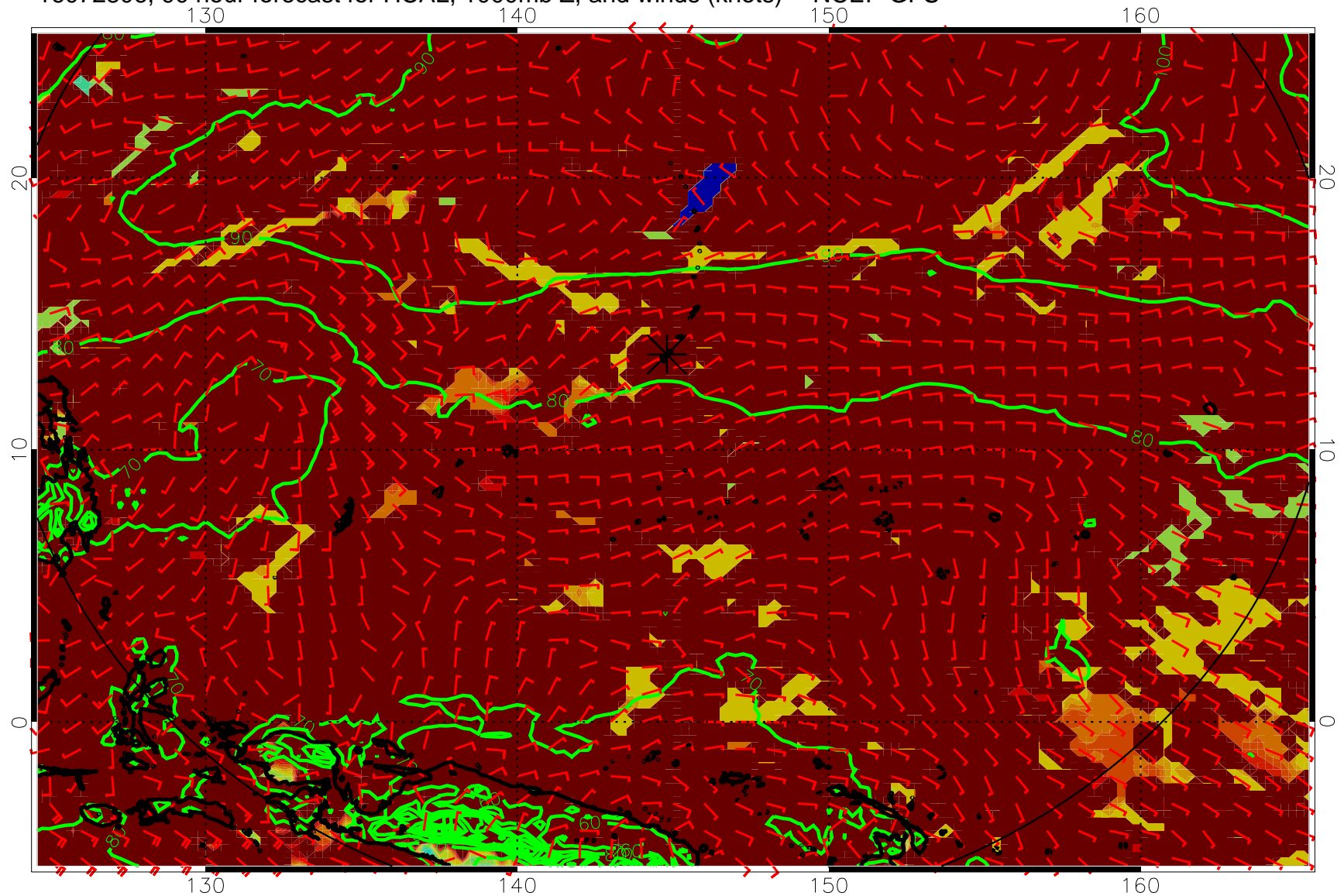
16072806, 90 hour forecast for HCAL, 1000mb Z, and winds (knots) -- NCEP GFS
