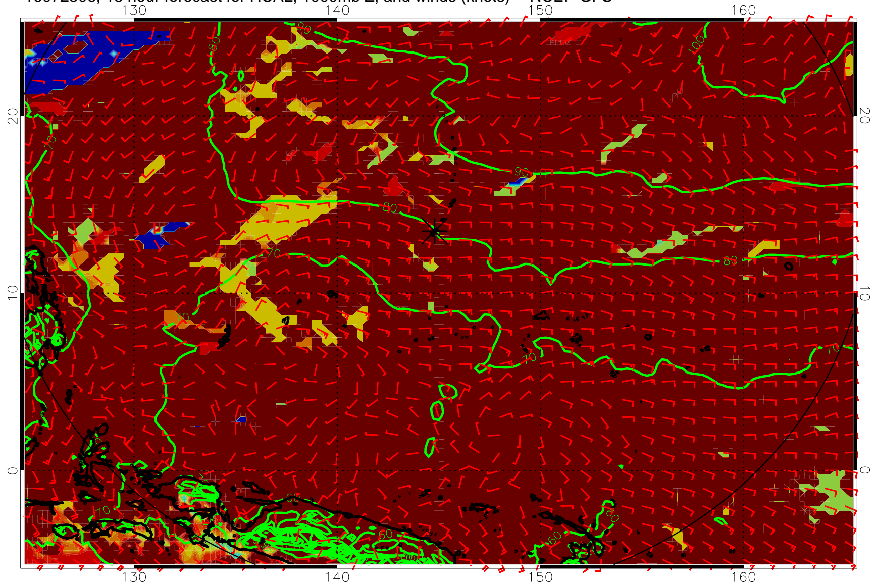
16072506, 18 hour forecast for HCAL, 1000mb Z, and winds (knots) -- NCEP GFS
