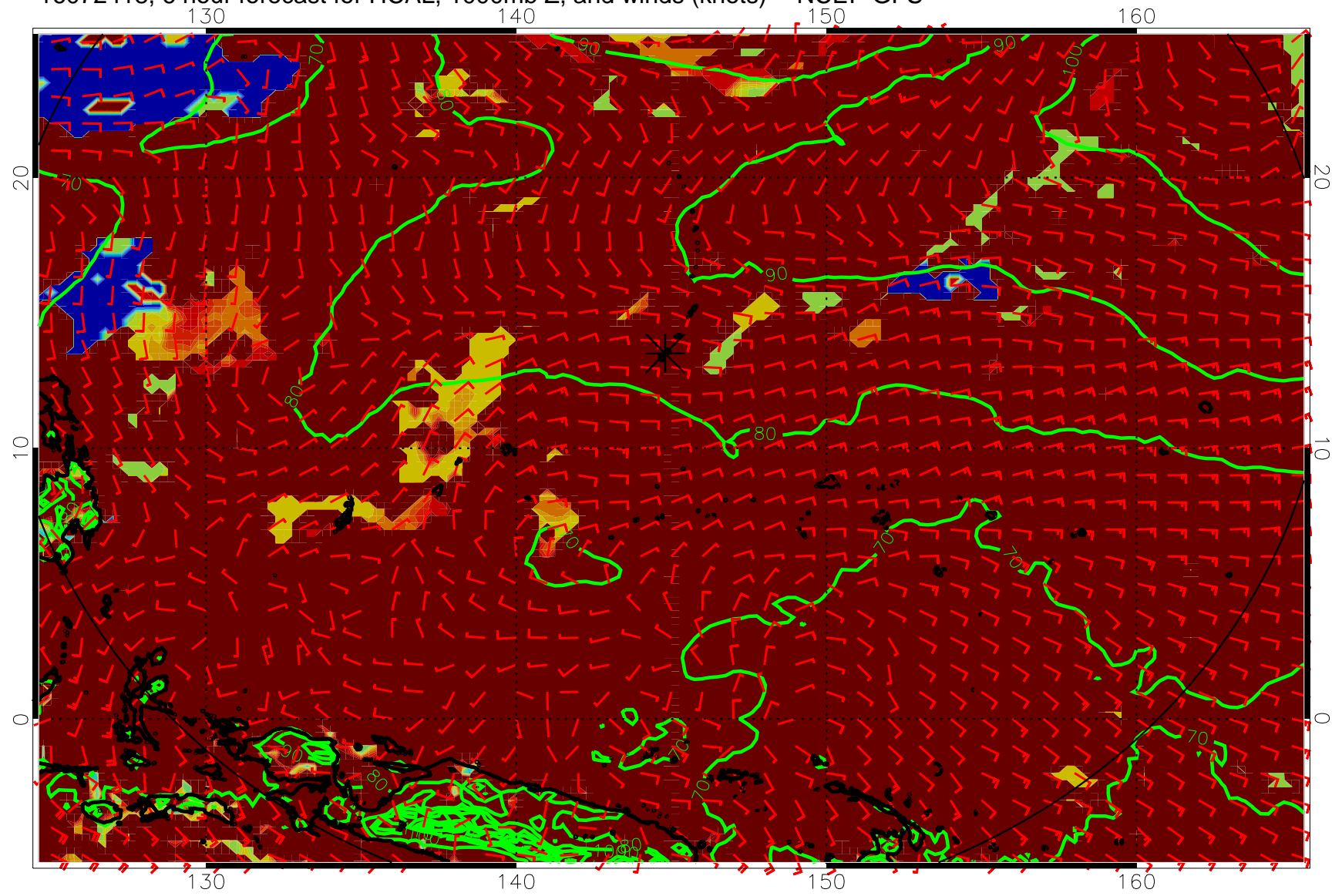
16072418, 6 hour forecast for HCAL, 1000mb Z, and winds (knots) -- NCEP GFS
