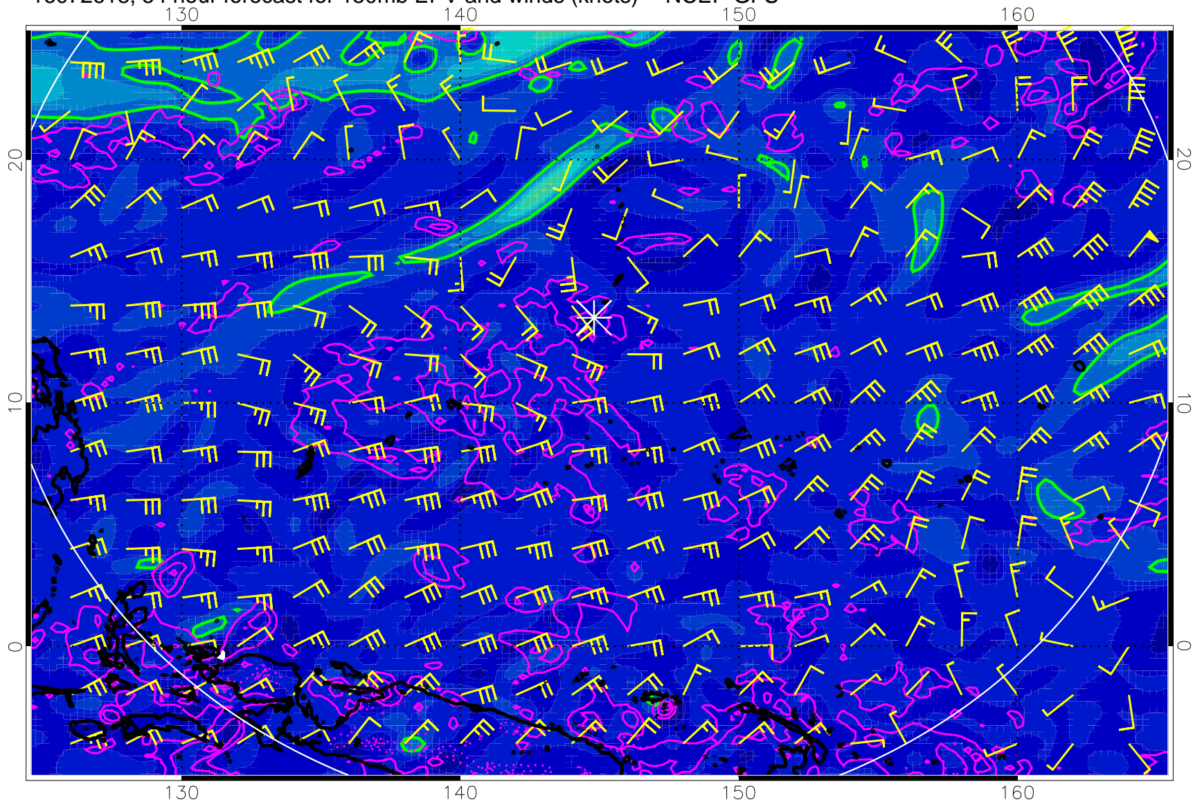
16072618, 54 hour forecast for 150mb EPV and winds (knots) -- NCEP GFS
