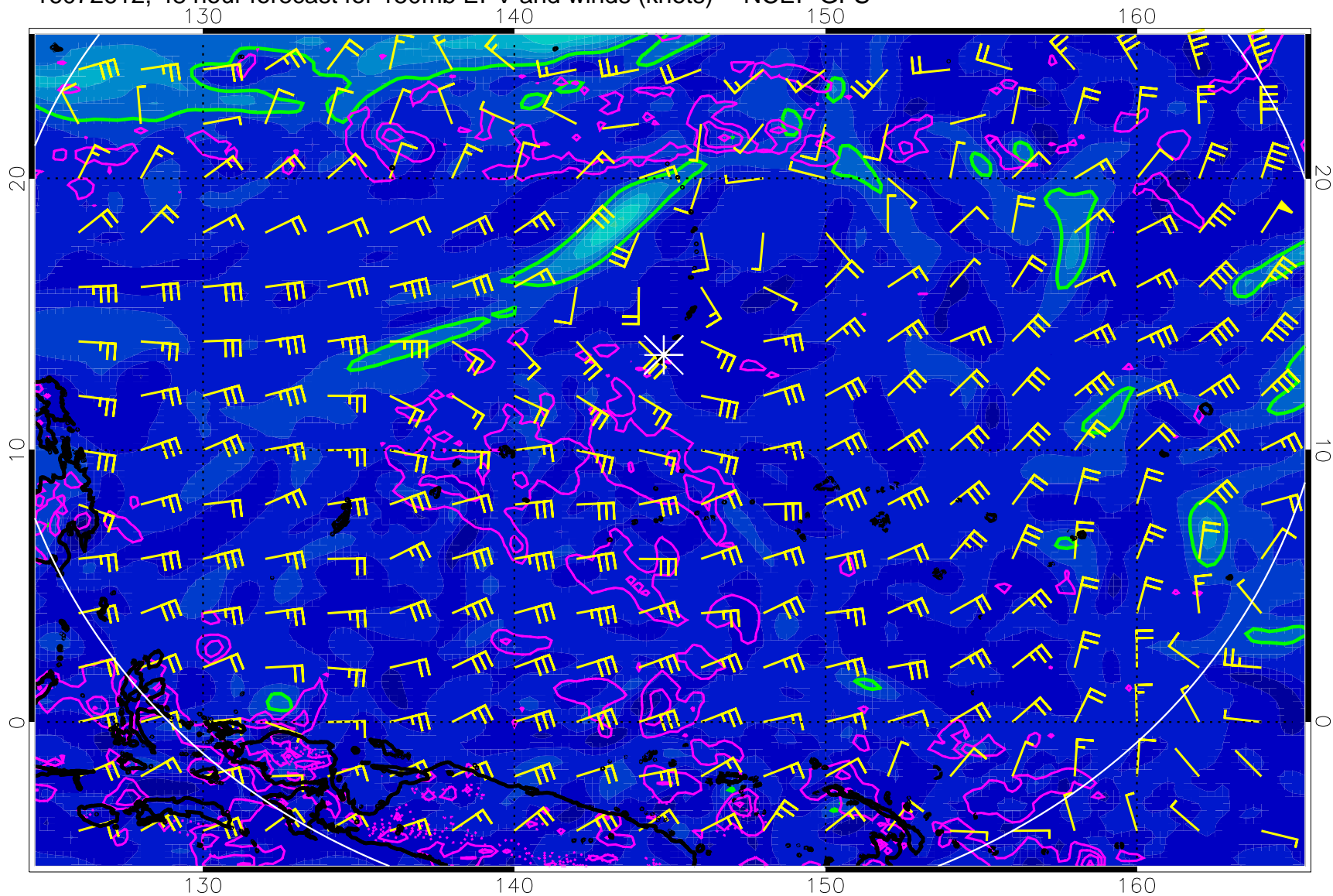
16072612, 48 hour forecast for 150mb EPV and winds (knots) -- NCEP GFS
