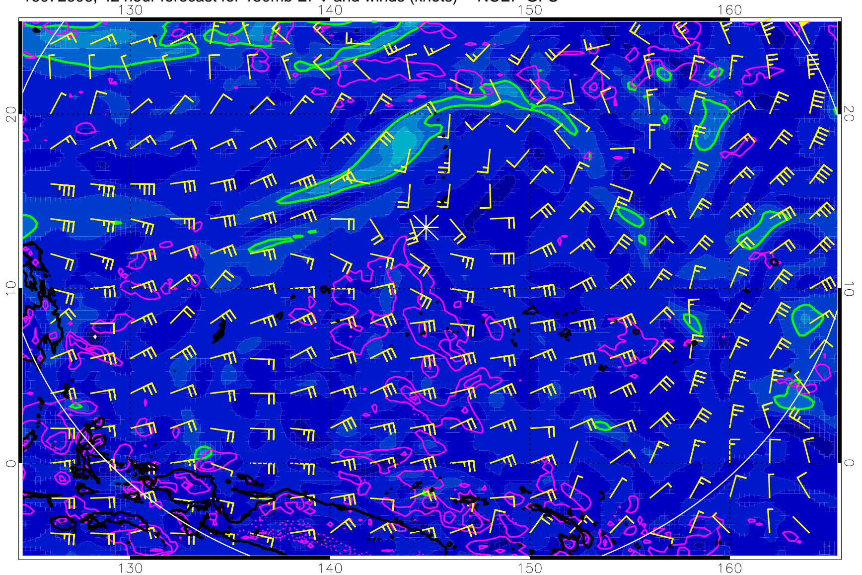
16072606, 42 hour forecast for 150mb EPV and winds (knots) -- NCEP GFS
