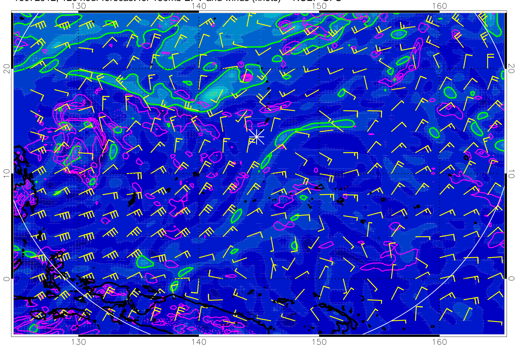
16072912, 120 hour forecast for 150mb EPV and winds (knots) -- NCEP GFS
