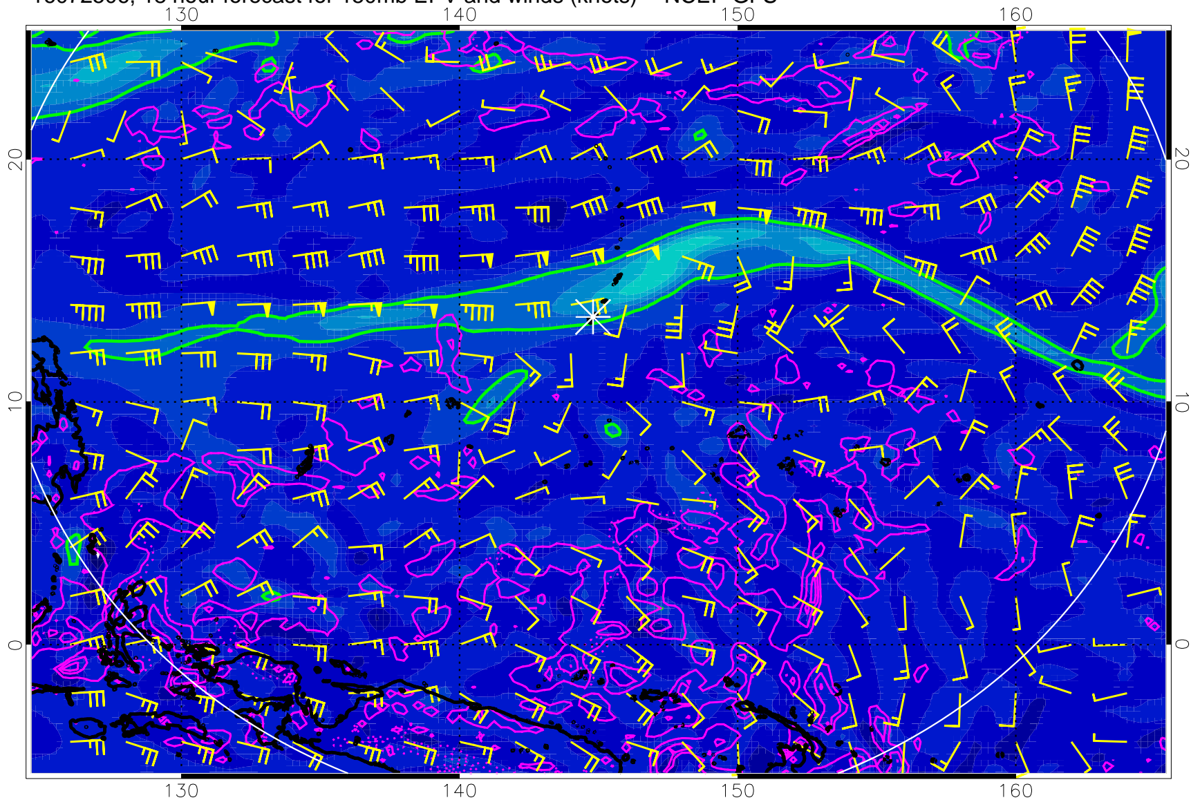
16072506, 18 hour forecast for 150mb EPV and winds (knots) -- NCEP GFS
