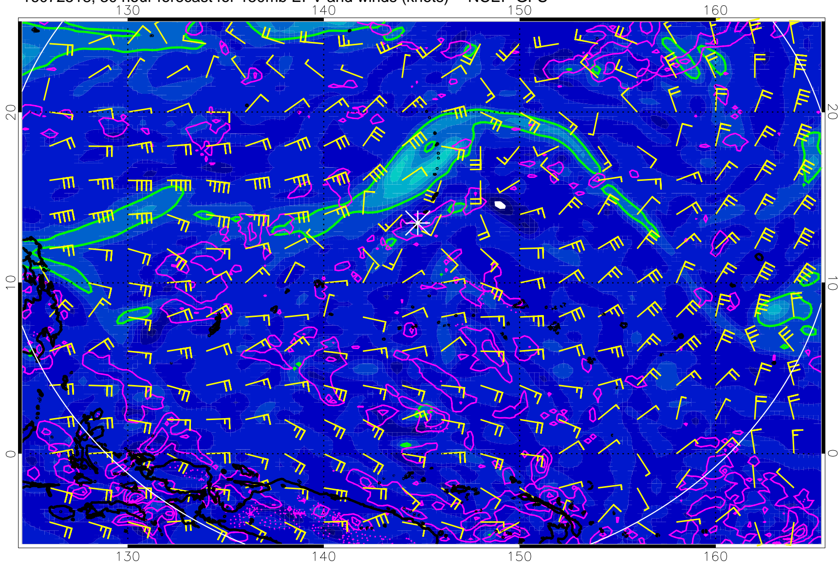
16072518, 30 hour forecast for 150mb EPV and winds (knots) -- NCEP GFS
