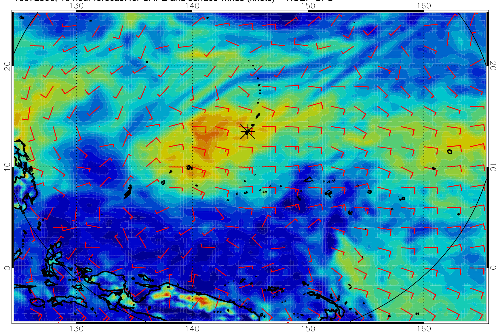
16072506, 18 hour forecast for CAPE and surface winds (knots) -- NCEP GFS
