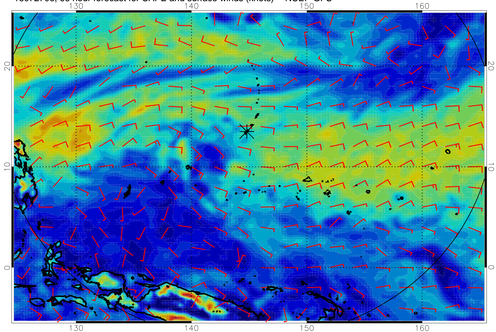
16072706, 66 hour forecast for CAPE and surface winds (knots) -- NCEP GFS
