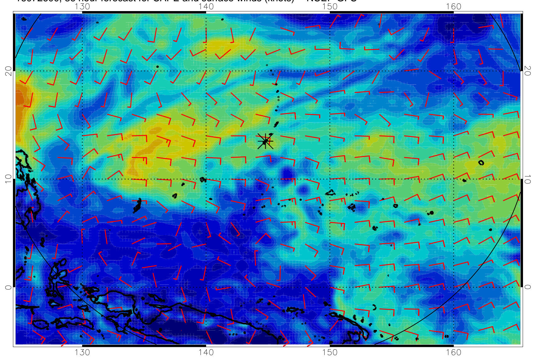
16072600, 36 hour forecast for CAPE and surface winds (knots) -- NCEP GFS
