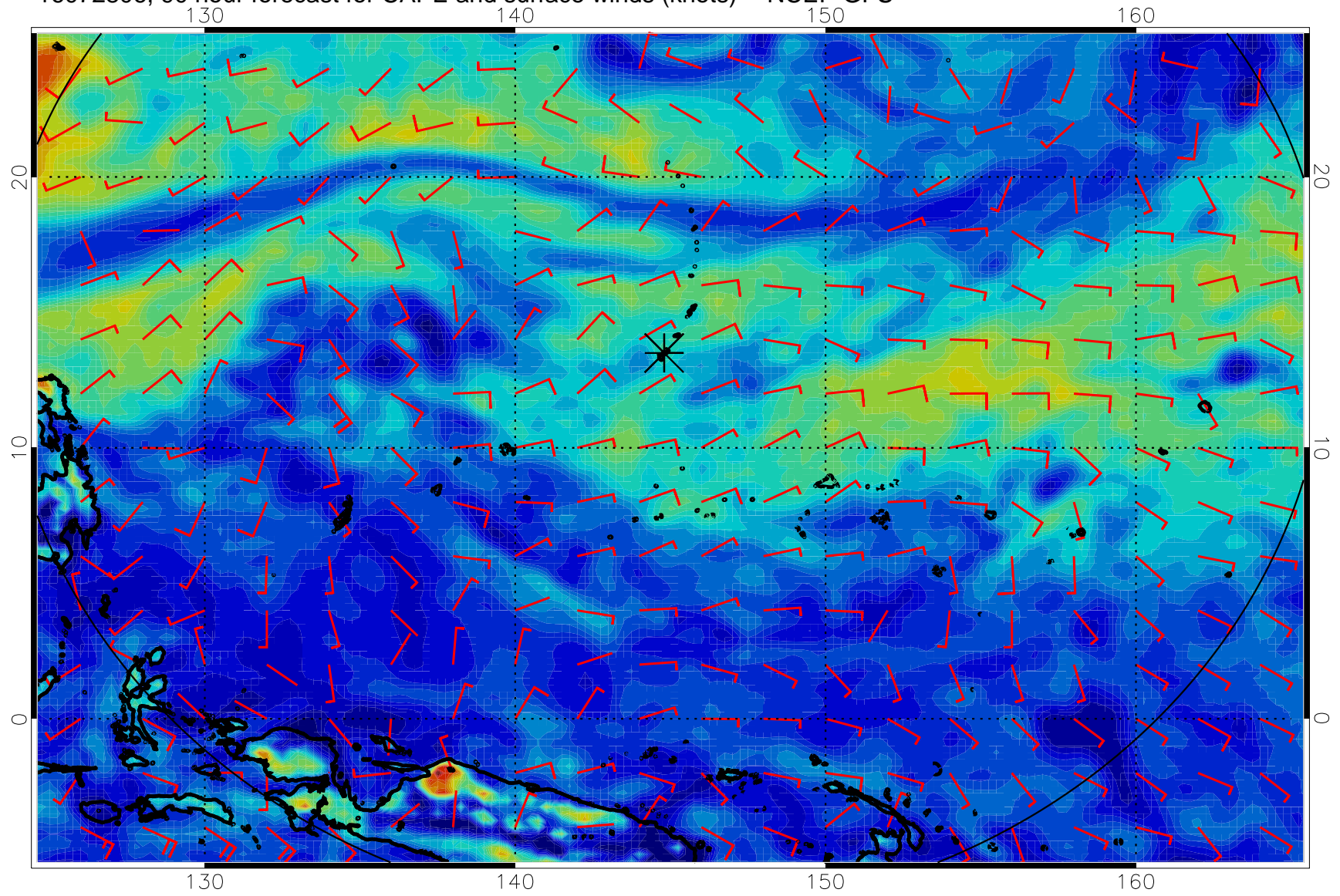
16072806, 90 hour forecast for CAPE and surface winds (knots) -- NCEP GFS
