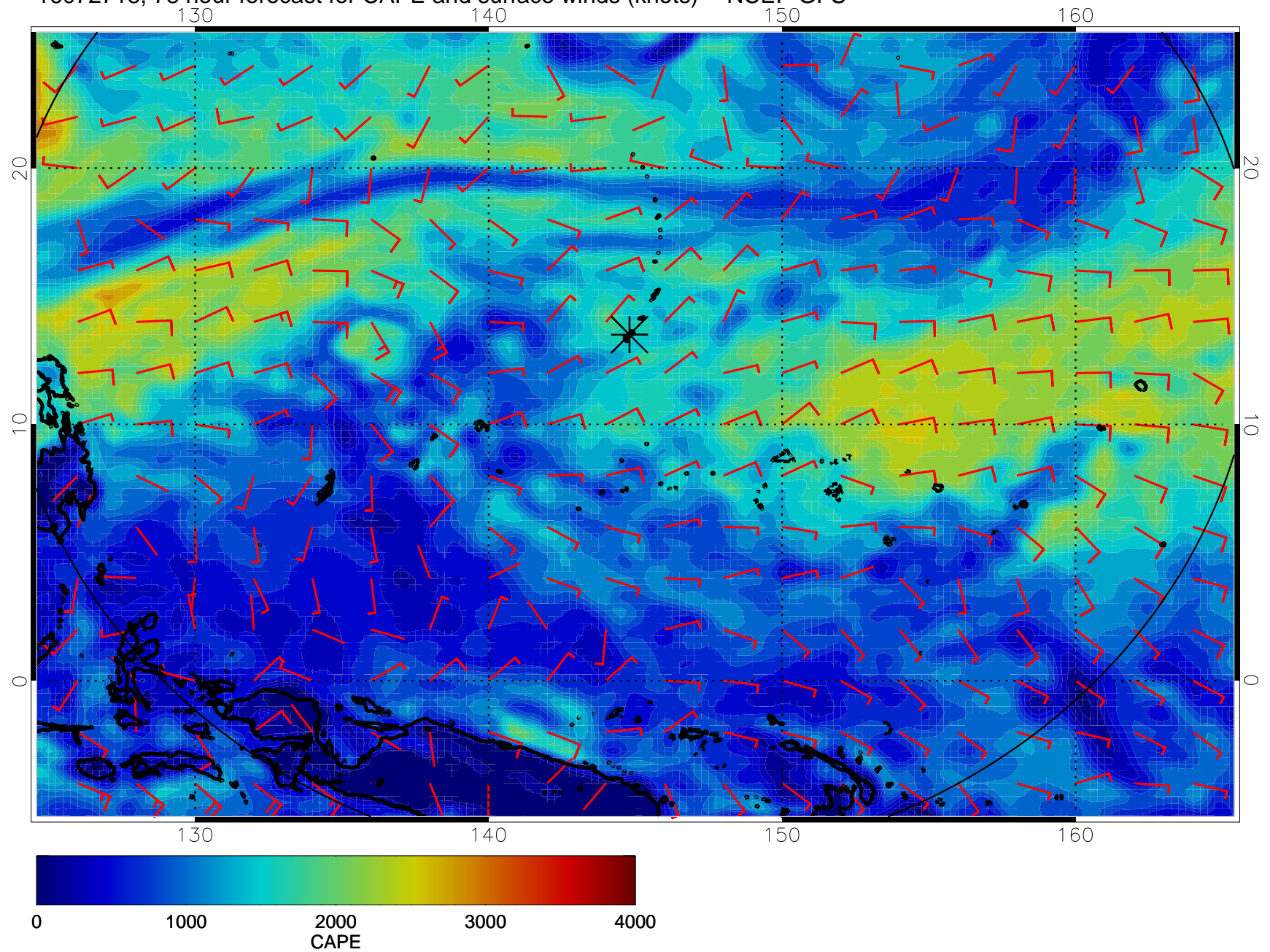
16072718, 78 hour forecast for CAPE and surface winds (knots) -- NCEP GFS
