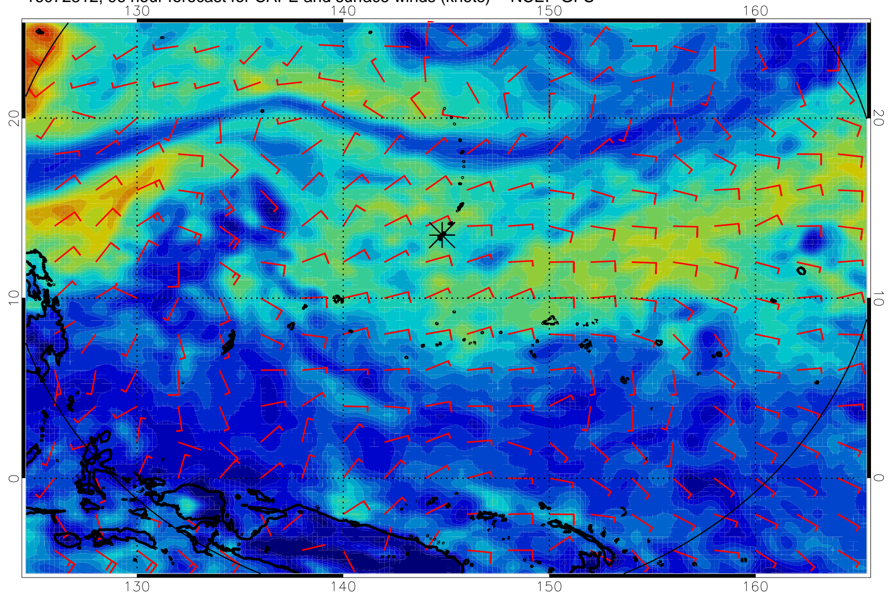
16072812, 96 hour forecast for CAPE and surface winds (knots) -- NCEP GFS
