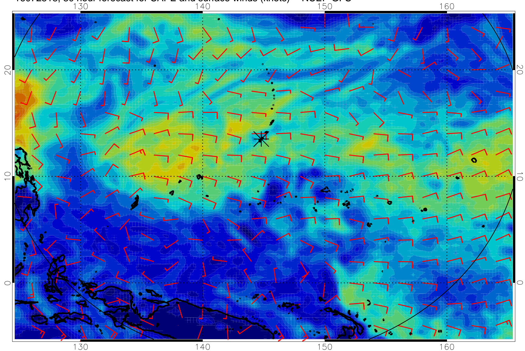
16072518, 30 hour forecast for CAPE and surface winds (knots) -- NCEP GFS
