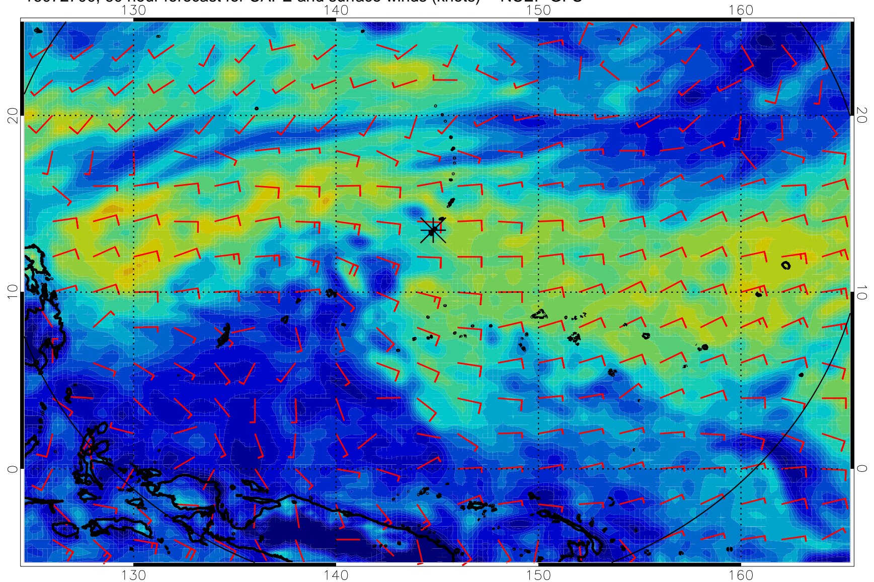
16072700, 60 hour forecast for CAPE and surface winds (knots) -- NCEP GFS
