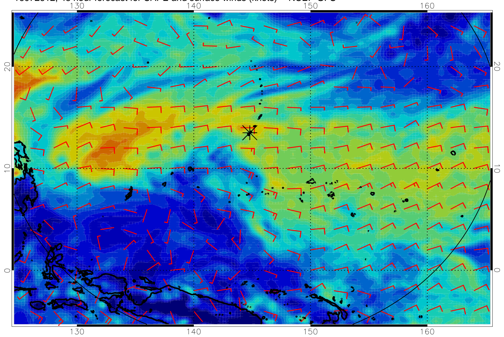
16072612, 48 hour forecast for CAPE and surface winds (knots) -- NCEP GFS
