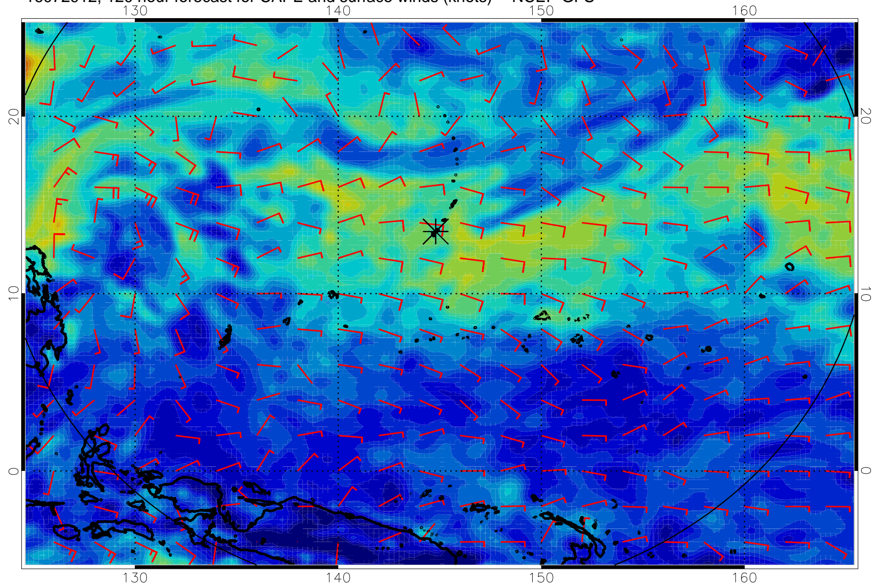
16072912, 120 hour forecast for CAPE and surface winds (knots) -- NCEP GFS
