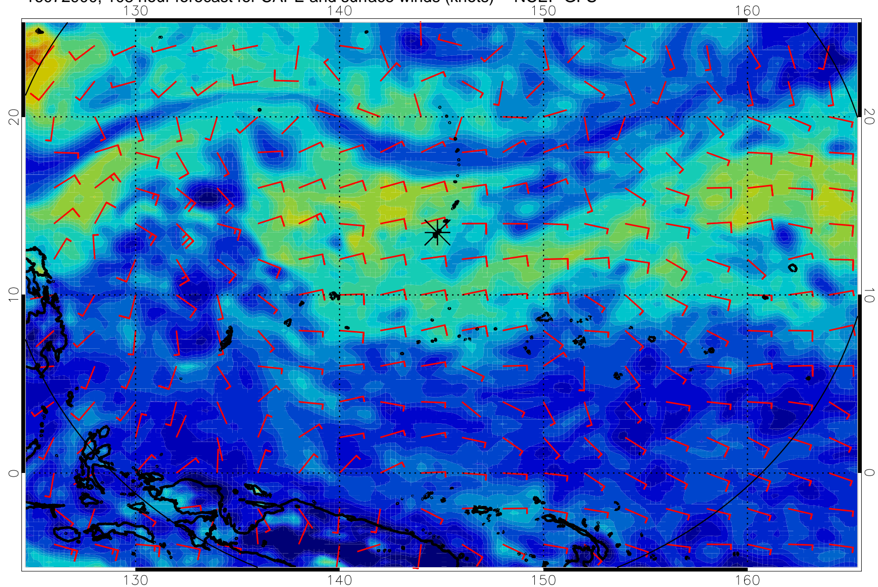
16072900, 108 hour forecast for CAPE and surface winds (knots) -- NCEP GFS
