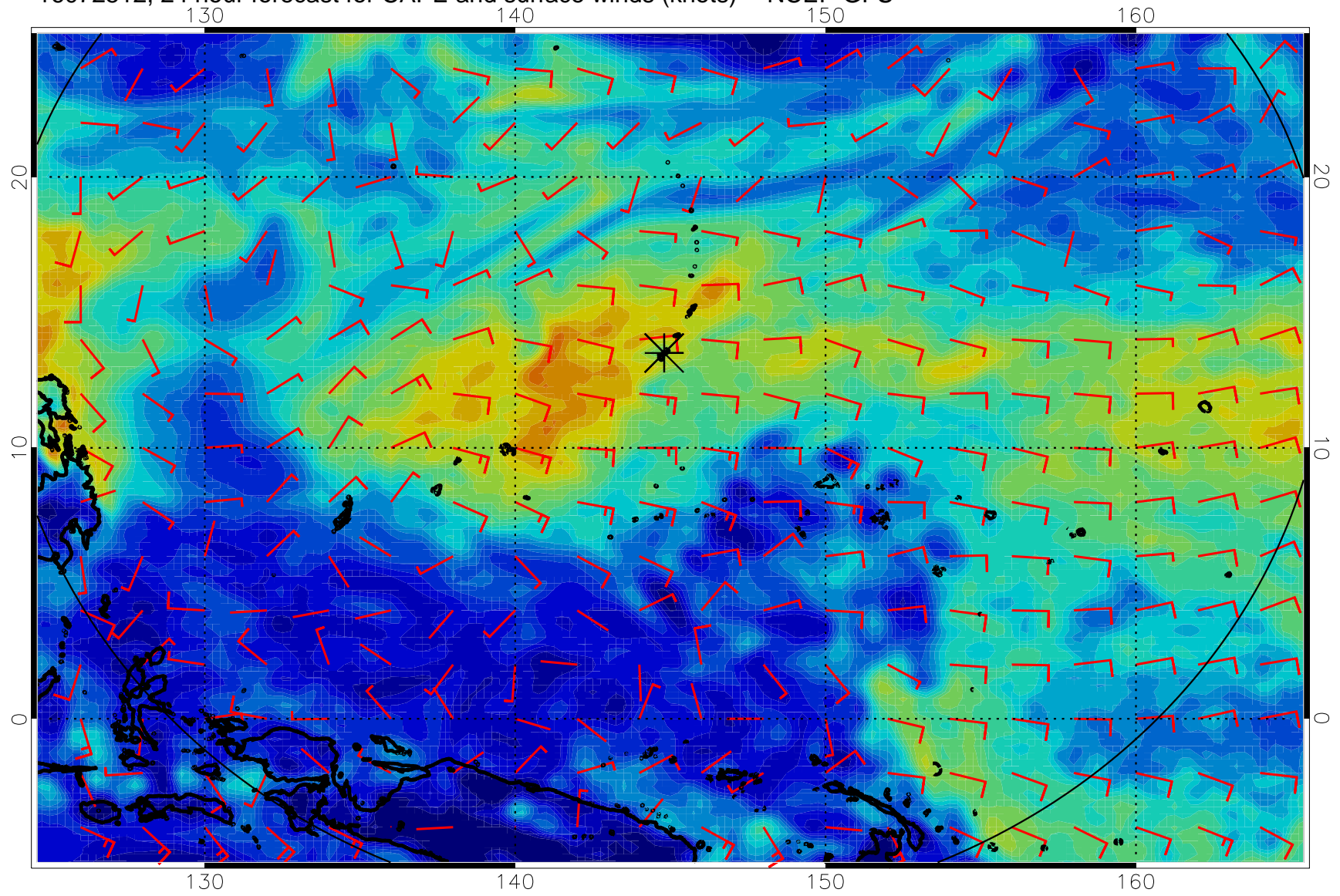
16072512, 24 hour forecast for CAPE and surface winds (knots) -- NCEP GFS
