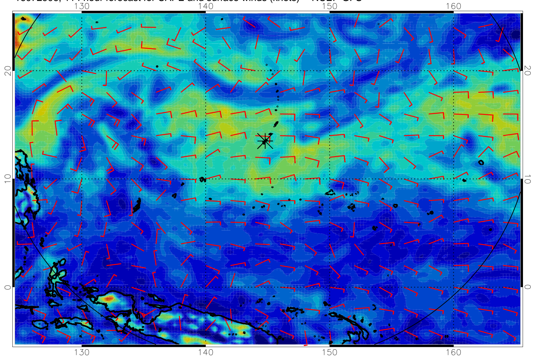
16072906, 114 hour forecast for CAPE and surface winds (knots) -- NCEP GFS
