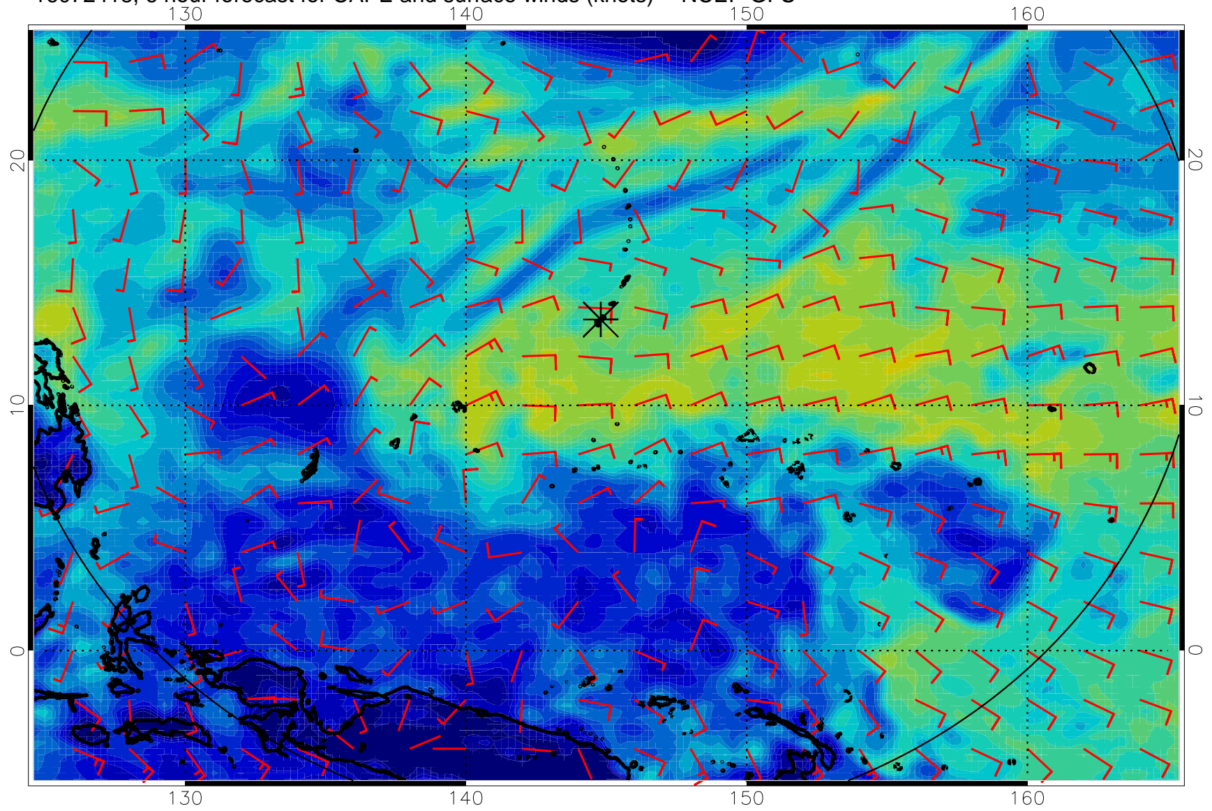
16072418, 6 hour forecast for CAPE and surface winds (knots) -- NCEP GFS
