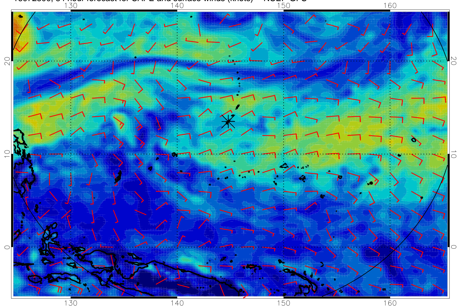
16072800, 84 hour forecast for CAPE and surface winds (knots) -- NCEP GFS
