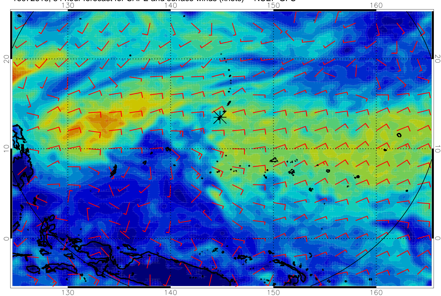
16072618, 54 hour forecast for CAPE and surface winds (knots) -- NCEP GFS
