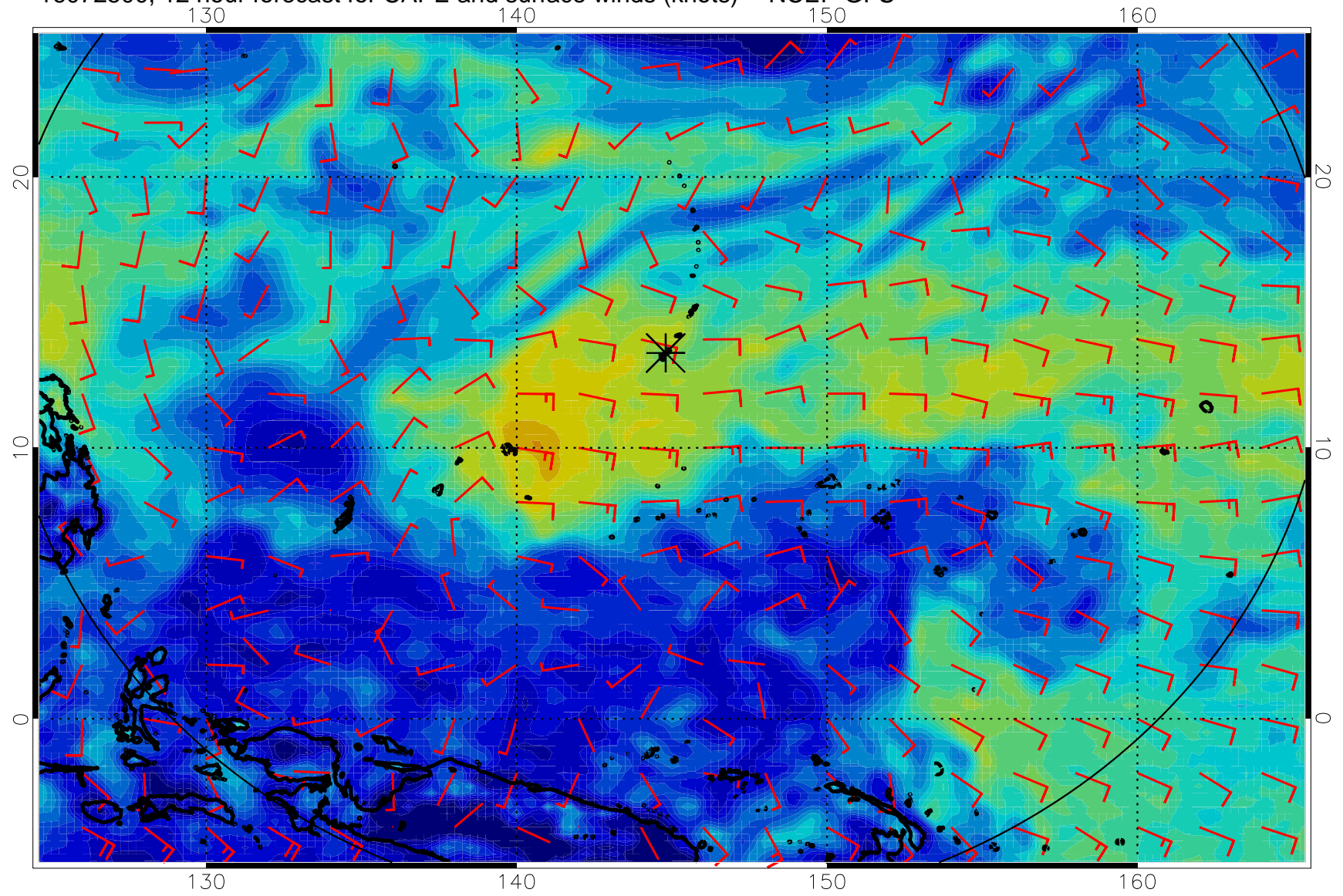
16072500, 12 hour forecast for CAPE and surface winds (knots) -- NCEP GFS
