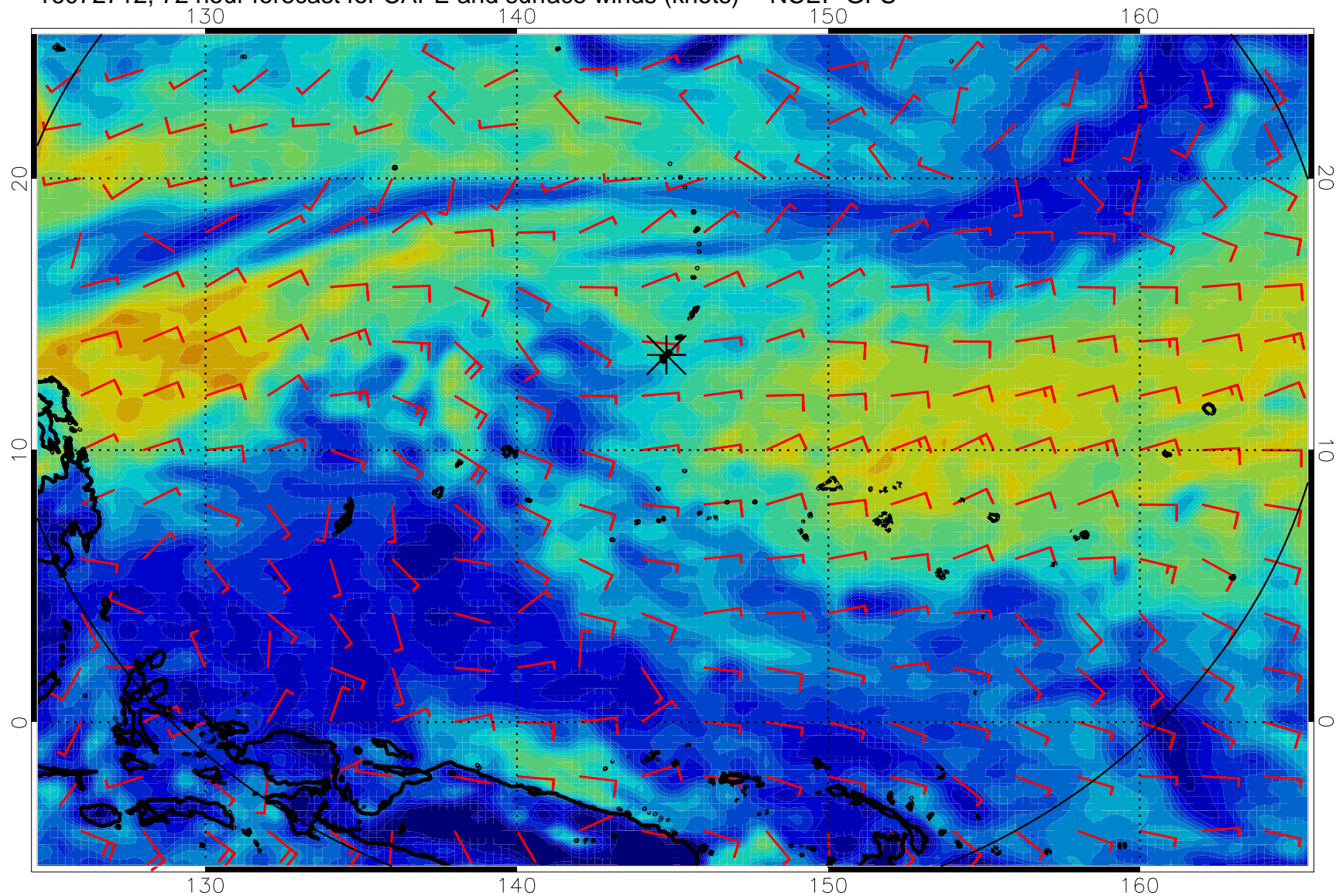
16072712, 72 hour forecast for CAPE and surface winds (knots) -- NCEP GFS
