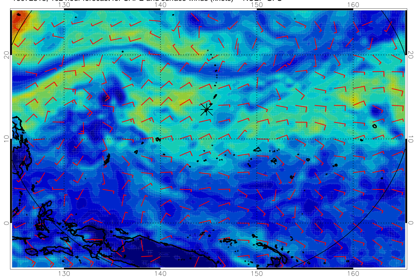
16072818, 102 hour forecast for CAPE and surface winds (knots) -- NCEP GFS
