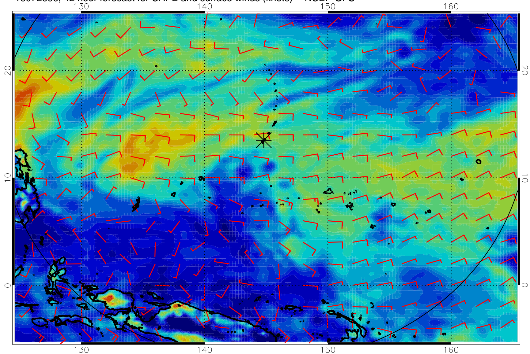
16072606, 42 hour forecast for CAPE and surface winds (knots) -- NCEP GFS
