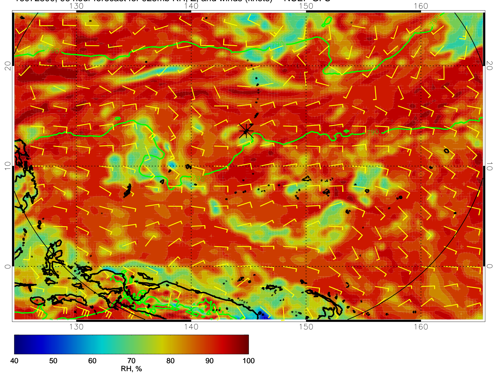
16072800, 96 hour forecast for 925mb RH, Z, and winds (knots) -- NCEP GFS
