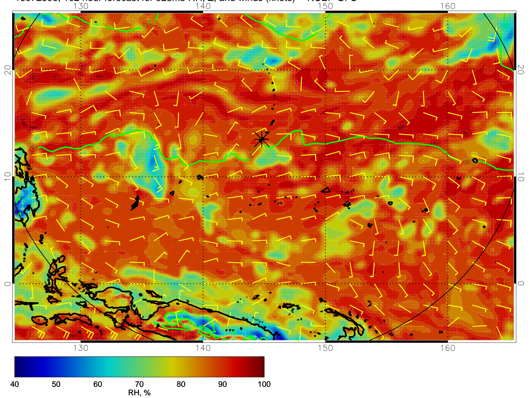
16072806, 102 hour forecast for 925mb RH, Z, and winds (knots) -- NCEP GFS
