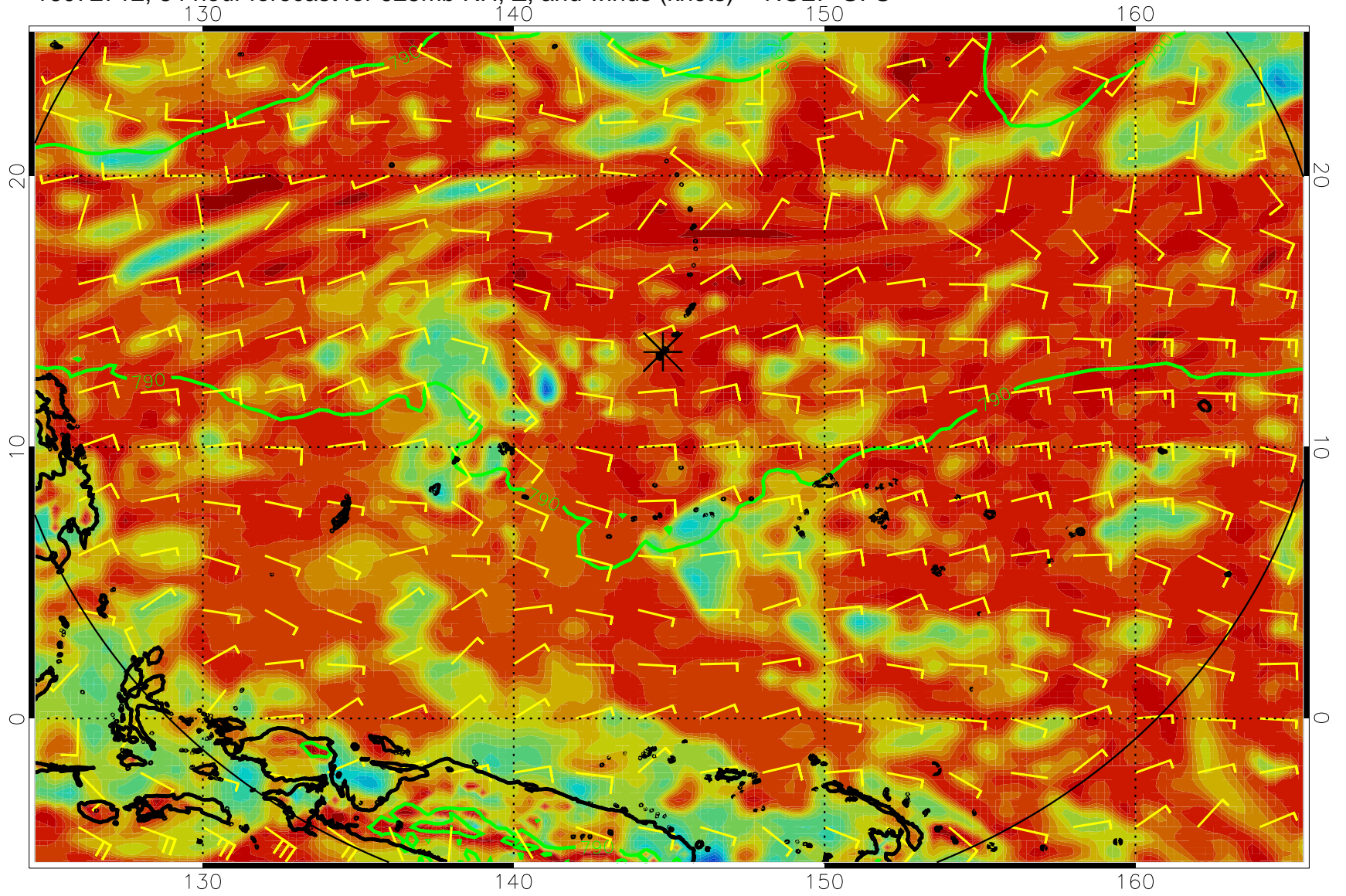
16072712, 84 hour forecast for 925mb RH, Z, and winds (knots) -- NCEP GFS
