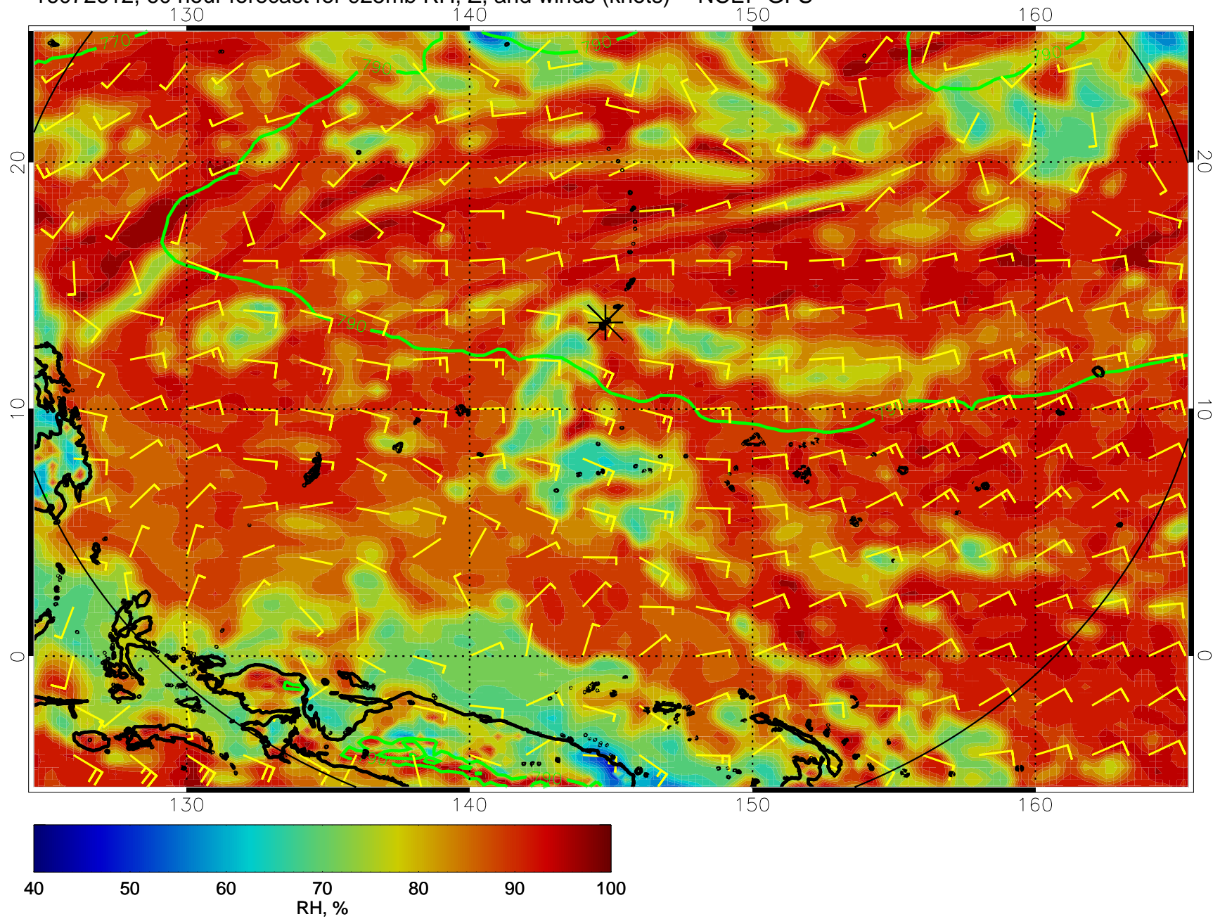
16072612, 60 hour forecast for 925mb RH, Z, and winds (knots) -- NCEP GFS
