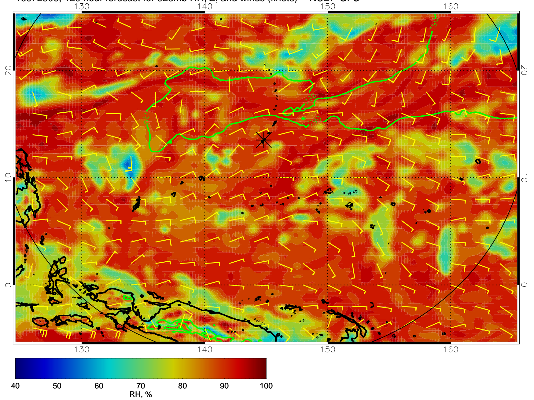
16072900, 120 hour forecast for 925mb RH, Z, and winds (knots) -- NCEP GFS
