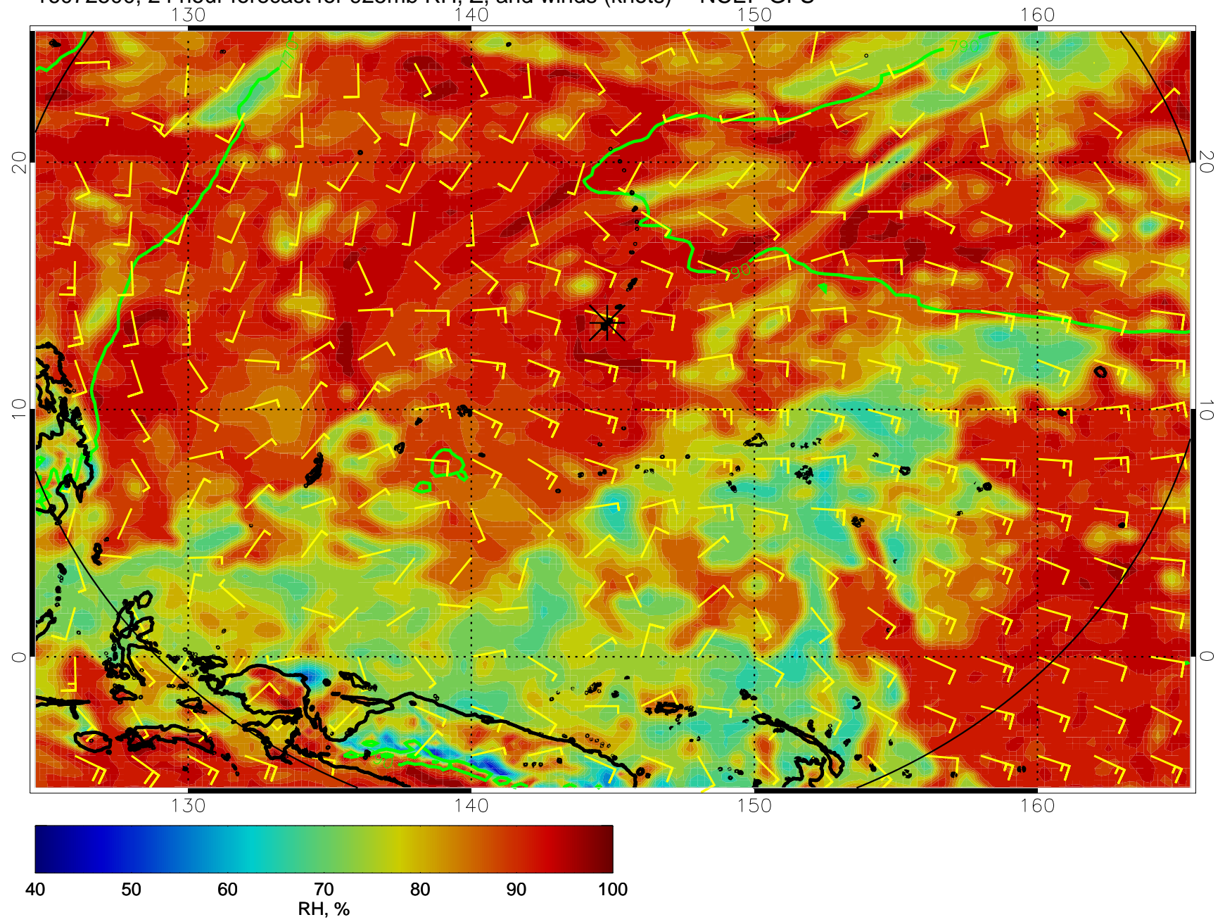
16072500, 24 hour forecast for 925mb RH, Z, and winds (knots) -- NCEP GFS
