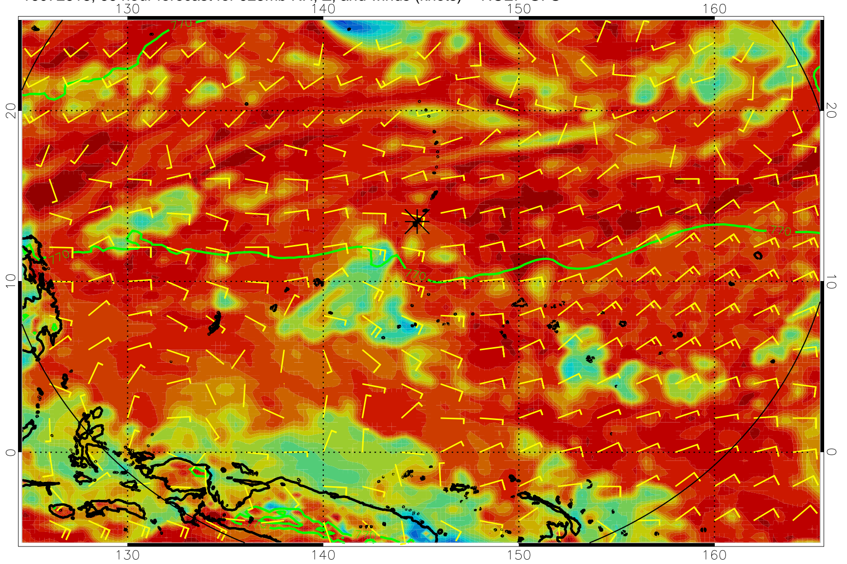
16072618, 66 hour forecast for 925mb RH, Z, and winds (knots) -- NCEP GFS
