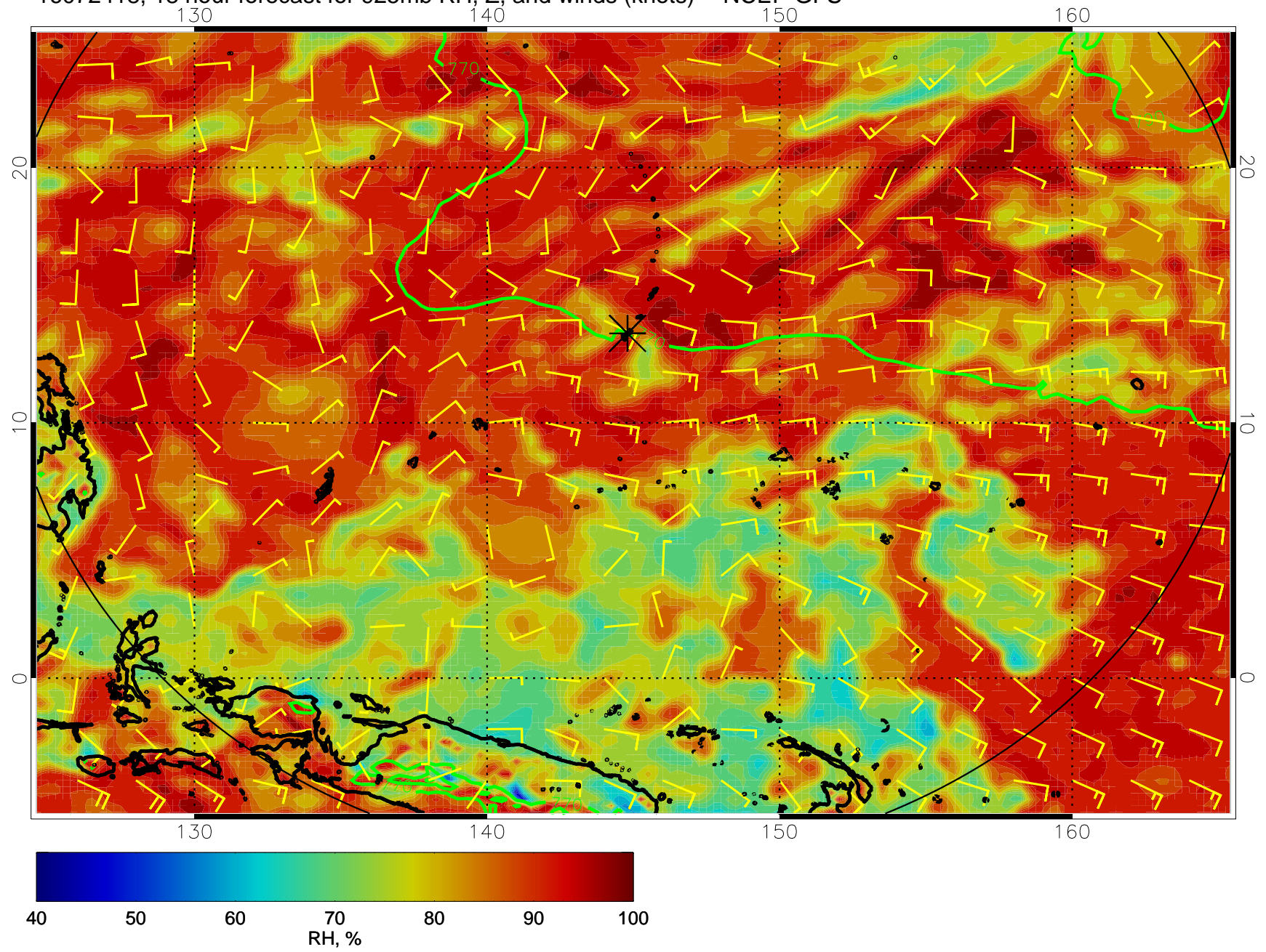
16072418, 18 hour forecast for 925mb RH, Z, and winds (knots) -- NCEP GFS
