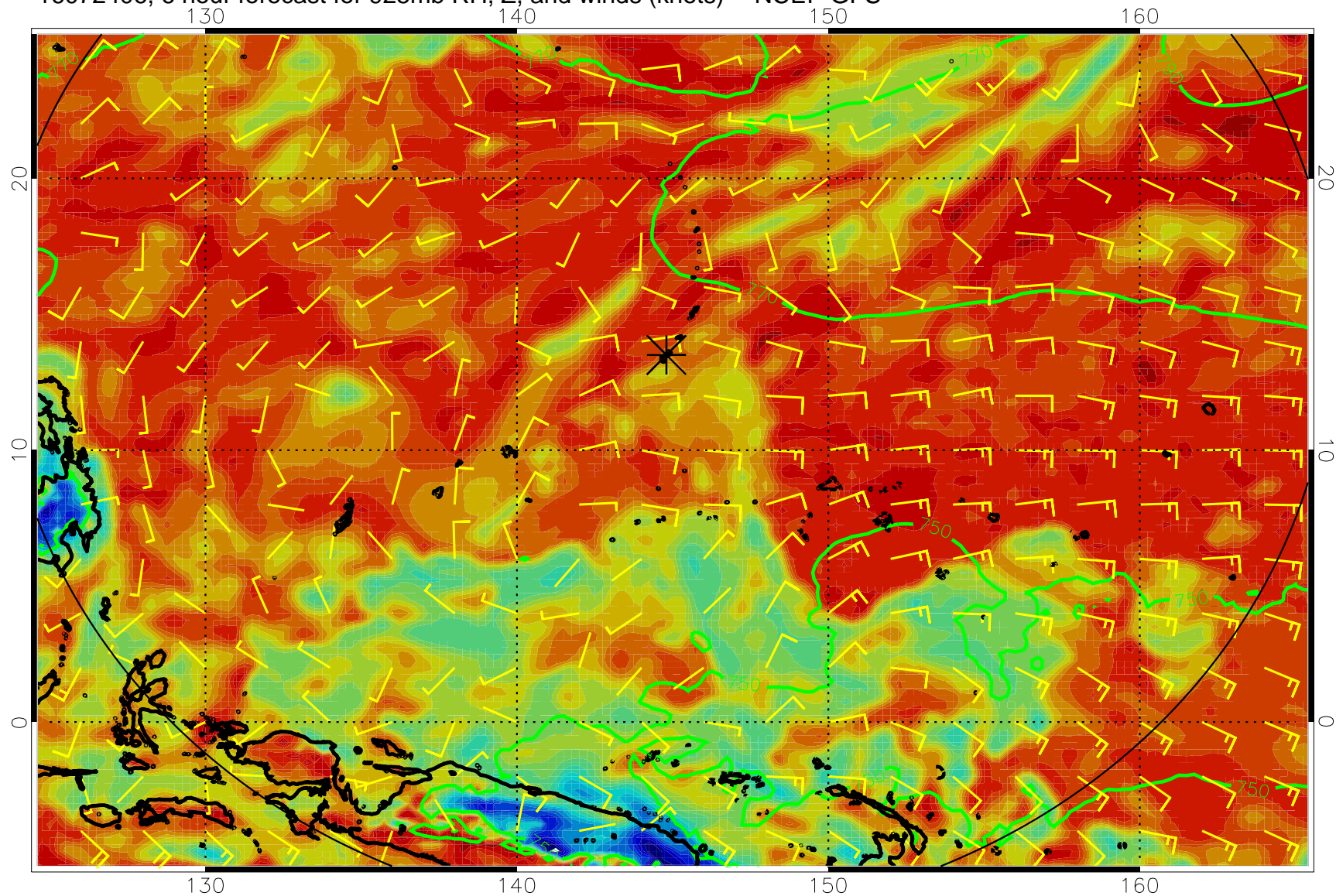
16072406, 6 hour forecast for 925mb RH, Z, and winds (knots) -- NCEP GFS
