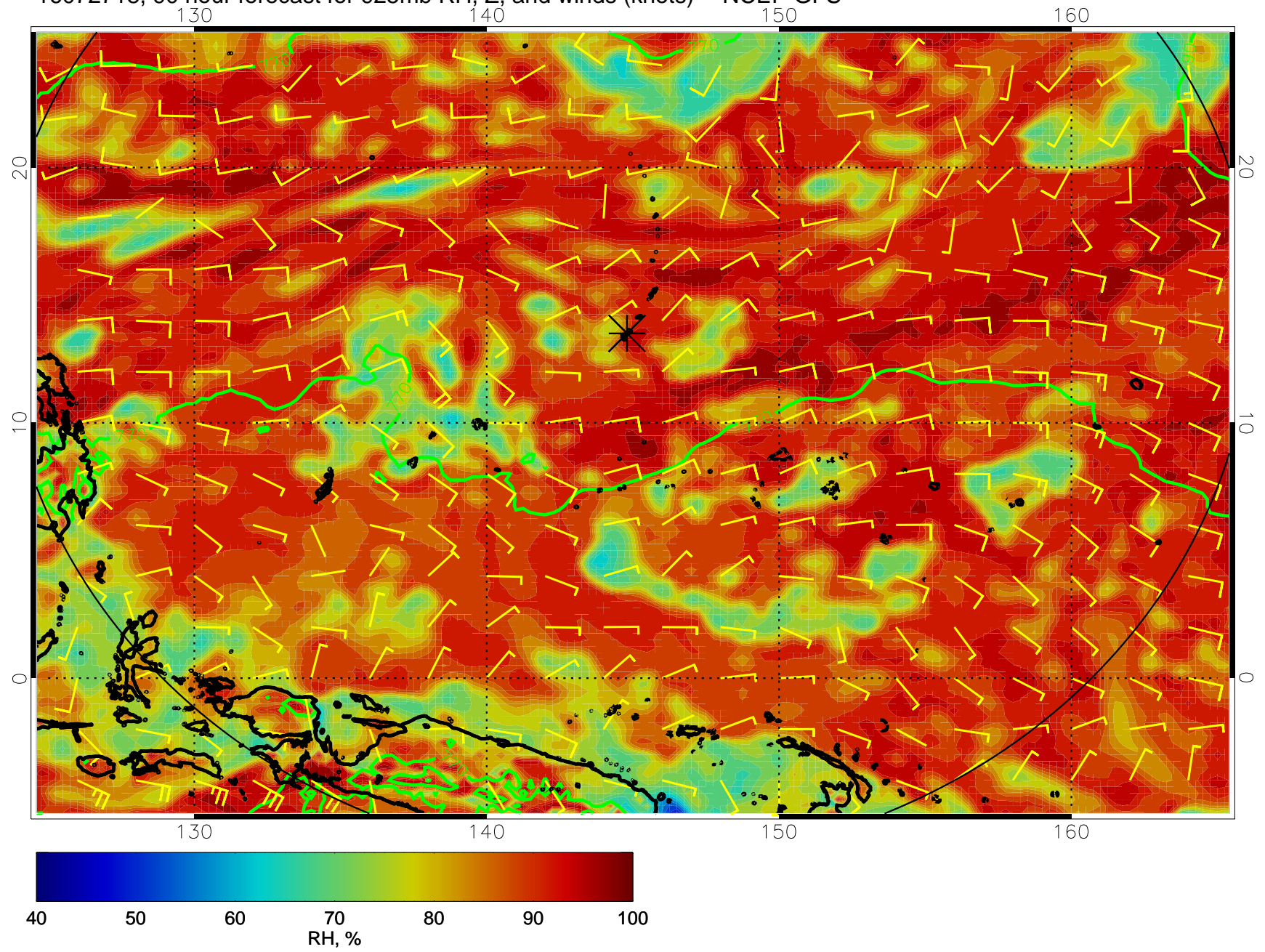
16072718, 90 hour forecast for 925mb RH, Z, and winds (knots) -- NCEP GFS
