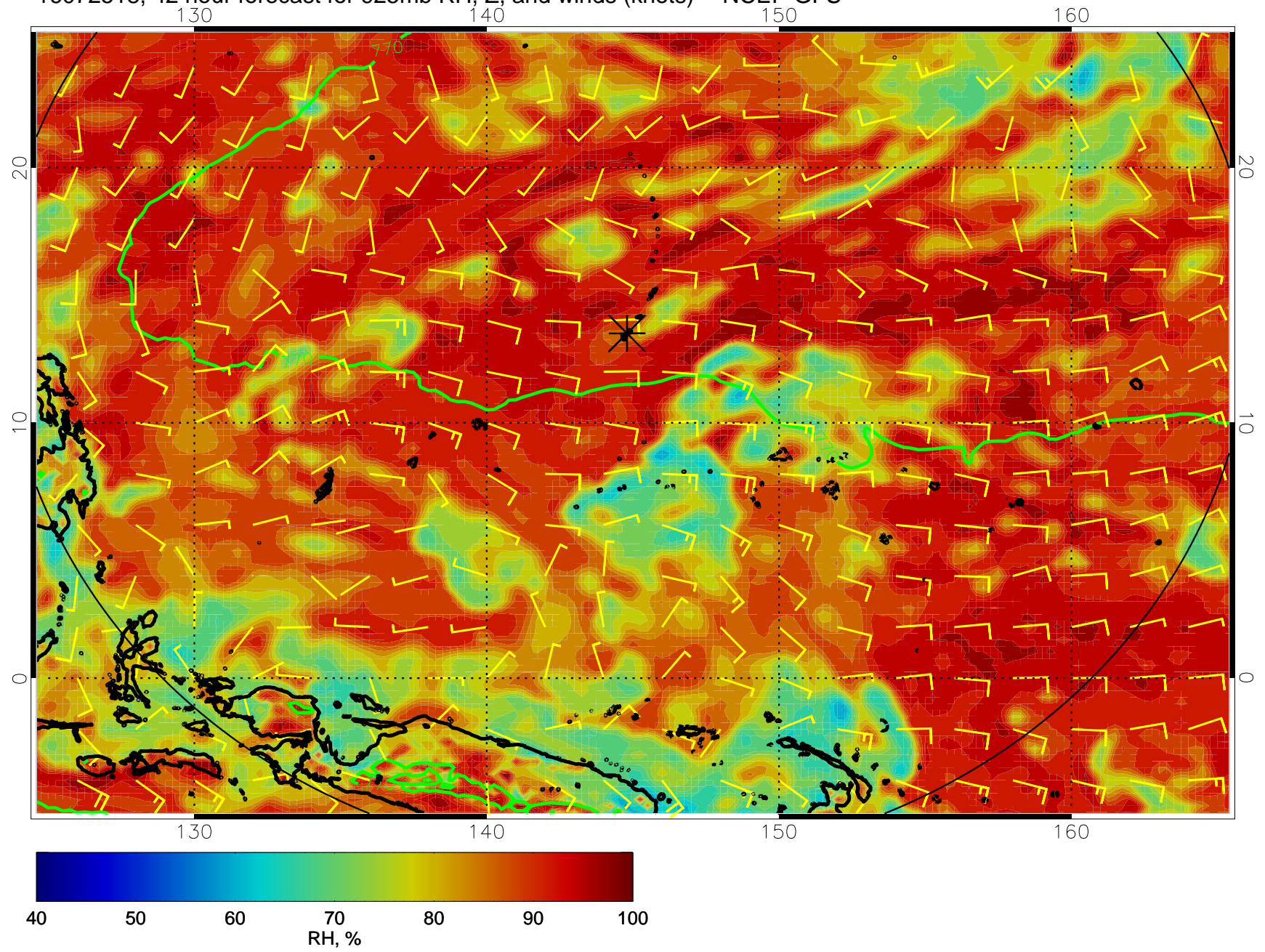
16072518, 42 hour forecast for 925mb RH, Z, and winds (knots) -- NCEP GFS
