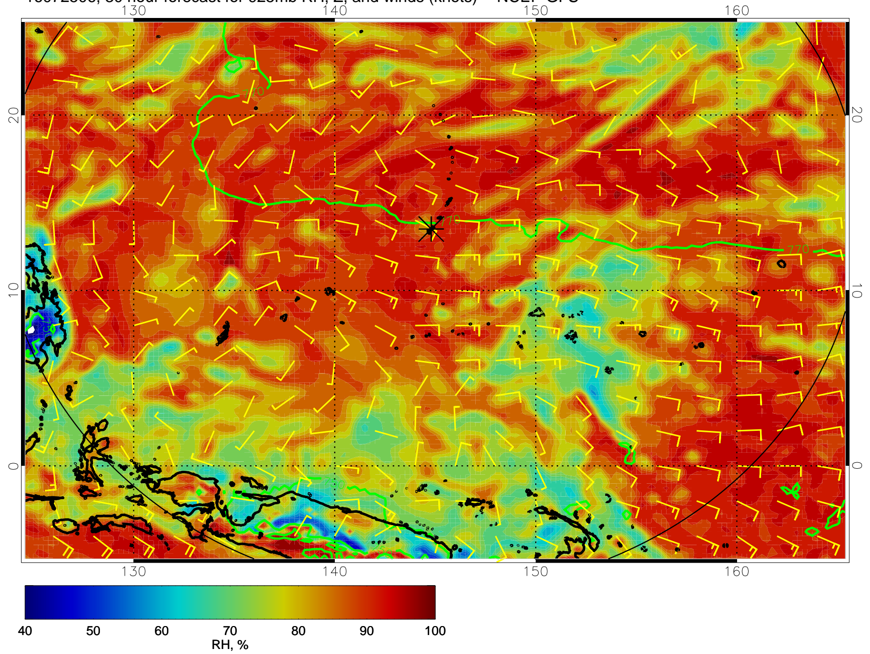
16072506, 30 hour forecast for 925mb RH, Z, and winds (knots) -- NCEP GFS
