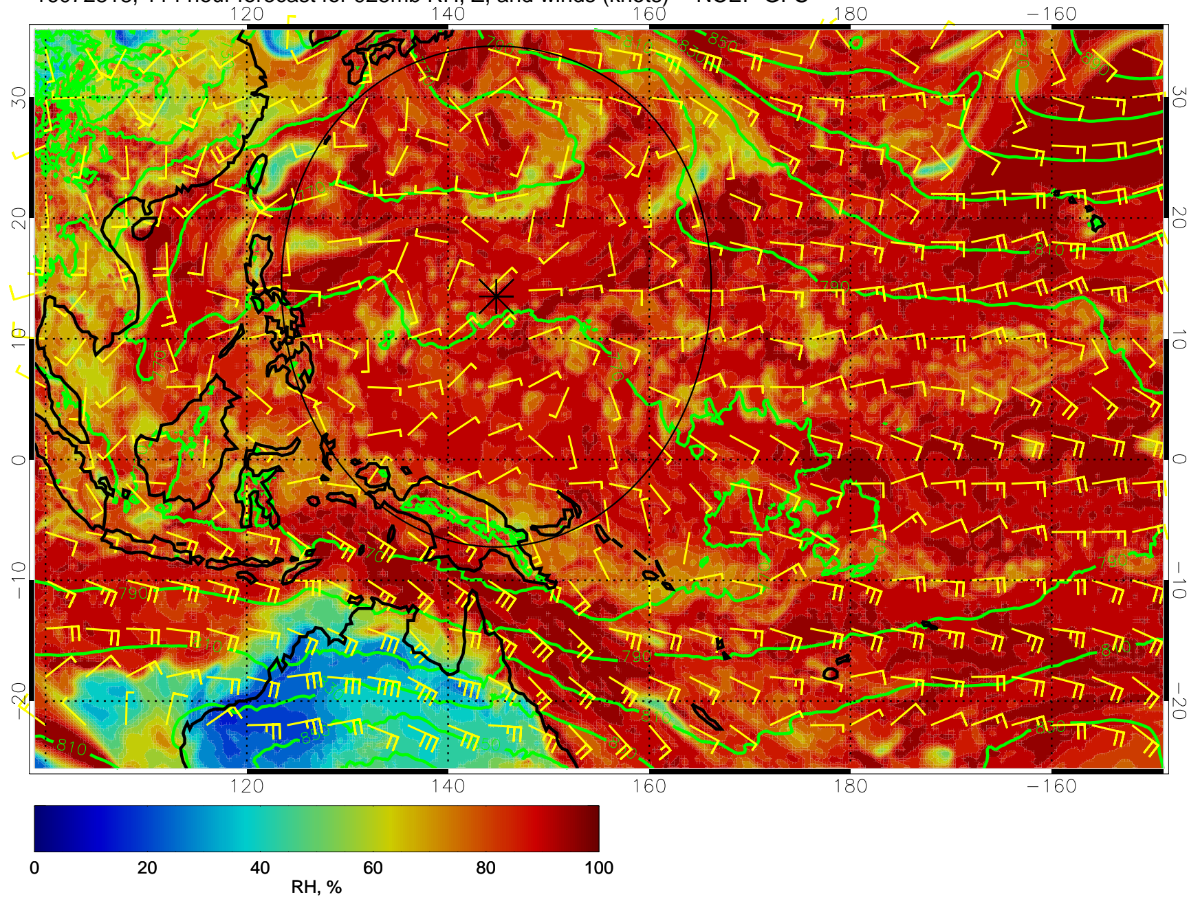
16072818, 114 hour forecast for 925mb RH, Z, and winds (knots) -- NCEP GFS
