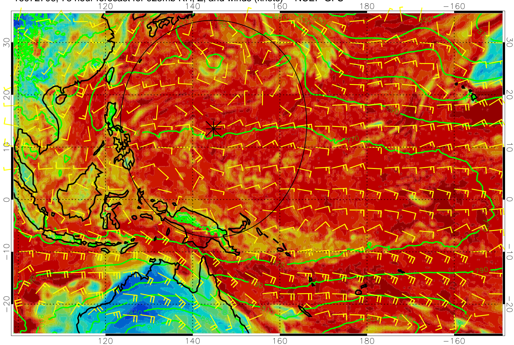
16072706, 78 hour forecast for 925mb RH, Z, and winds (knots) -- NCEP GFS
