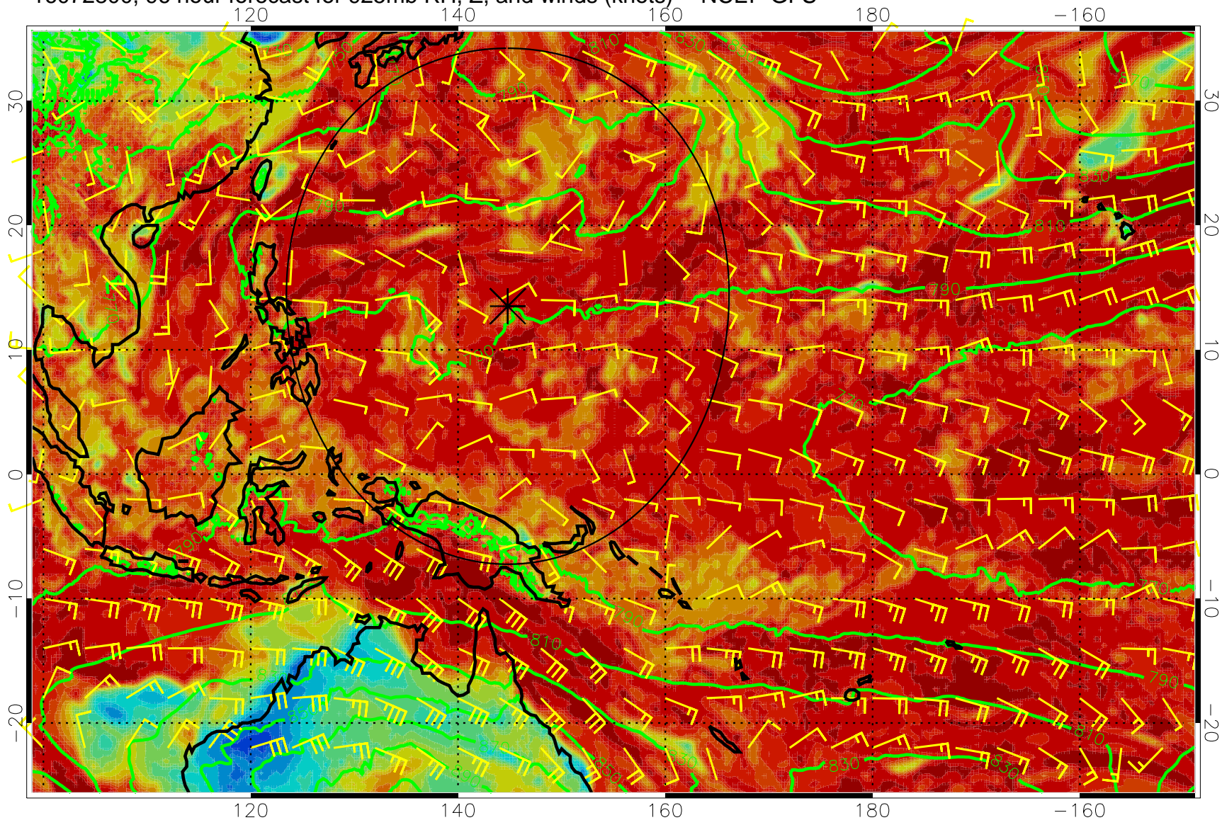
16072800, 96 hour forecast for 925mb RH, Z, and winds (knots) -- NCEP GFS
