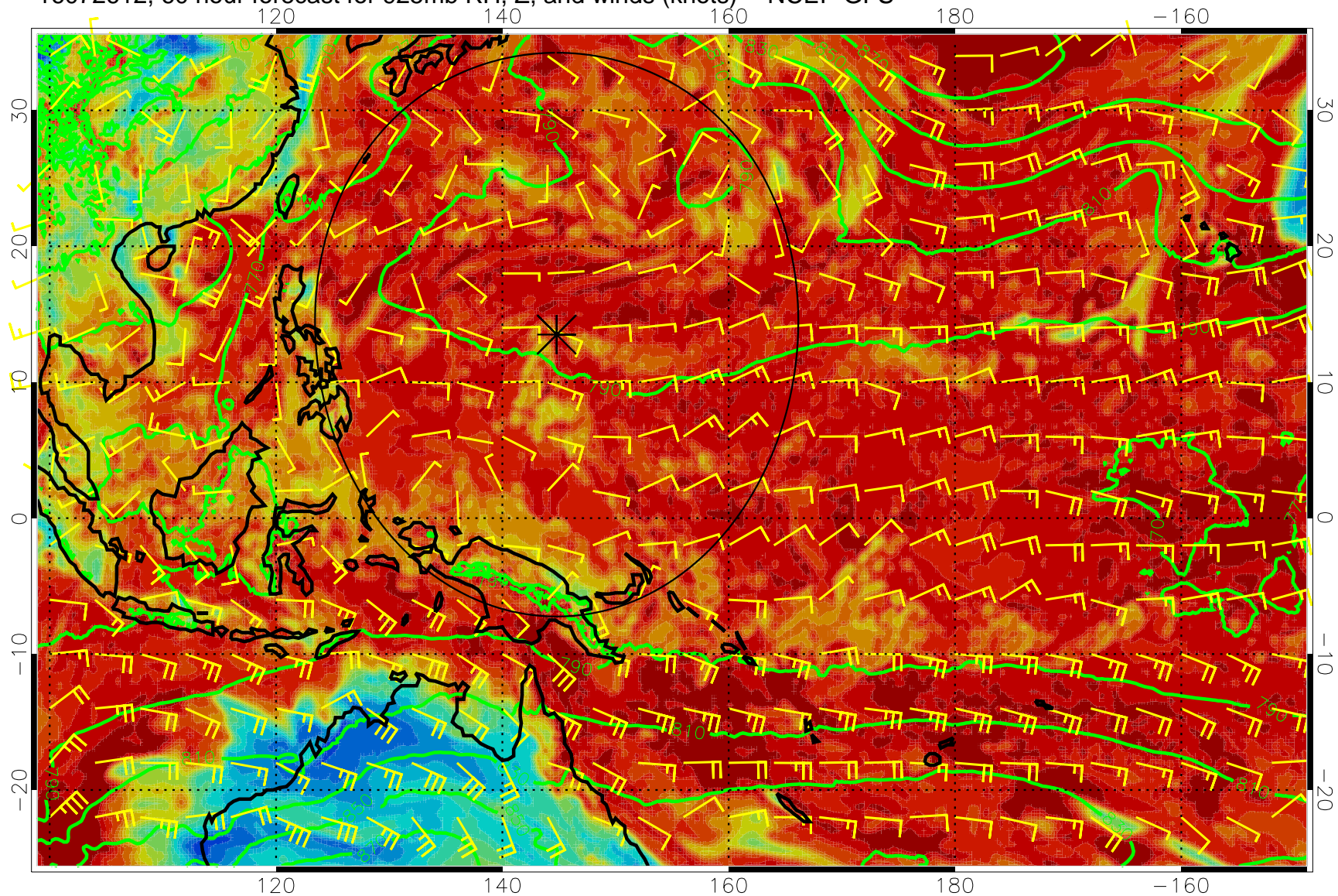
16072612, 60 hour forecast for 925mb RH, Z, and winds (knots) -- NCEP GFS
