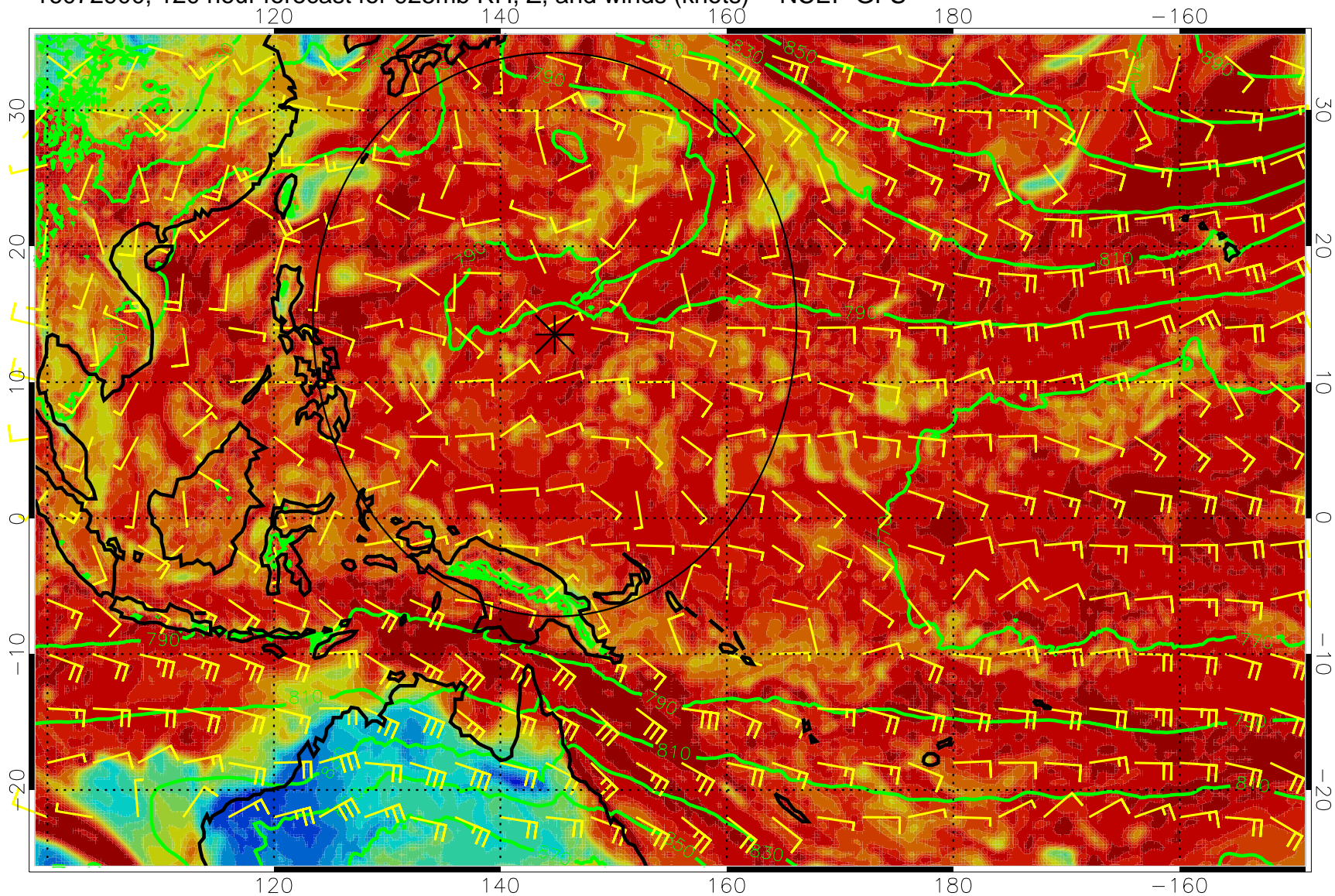
16072900, 120 hour forecast for 925mb RH, Z, and winds (knots) -- NCEP GFS
