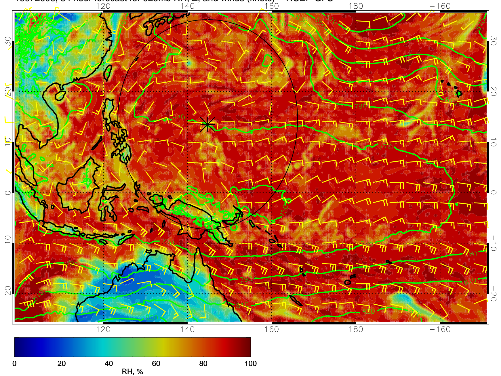
16072606, 54 hour forecast for 925mb RH, Z, and winds (knots) -- NCEP GFS
