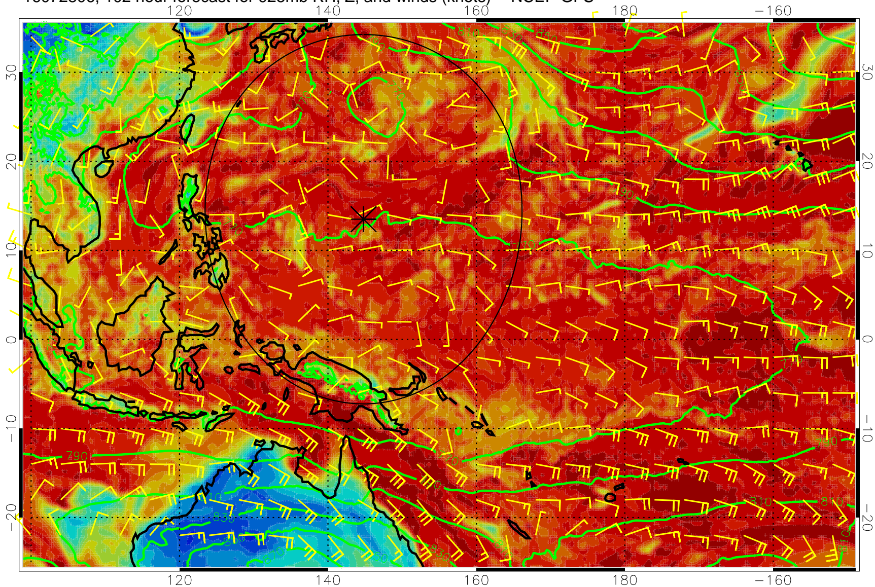
16072806, 102 hour forecast for 925mb RH, Z, and winds (knots) -- NCEP GFS
