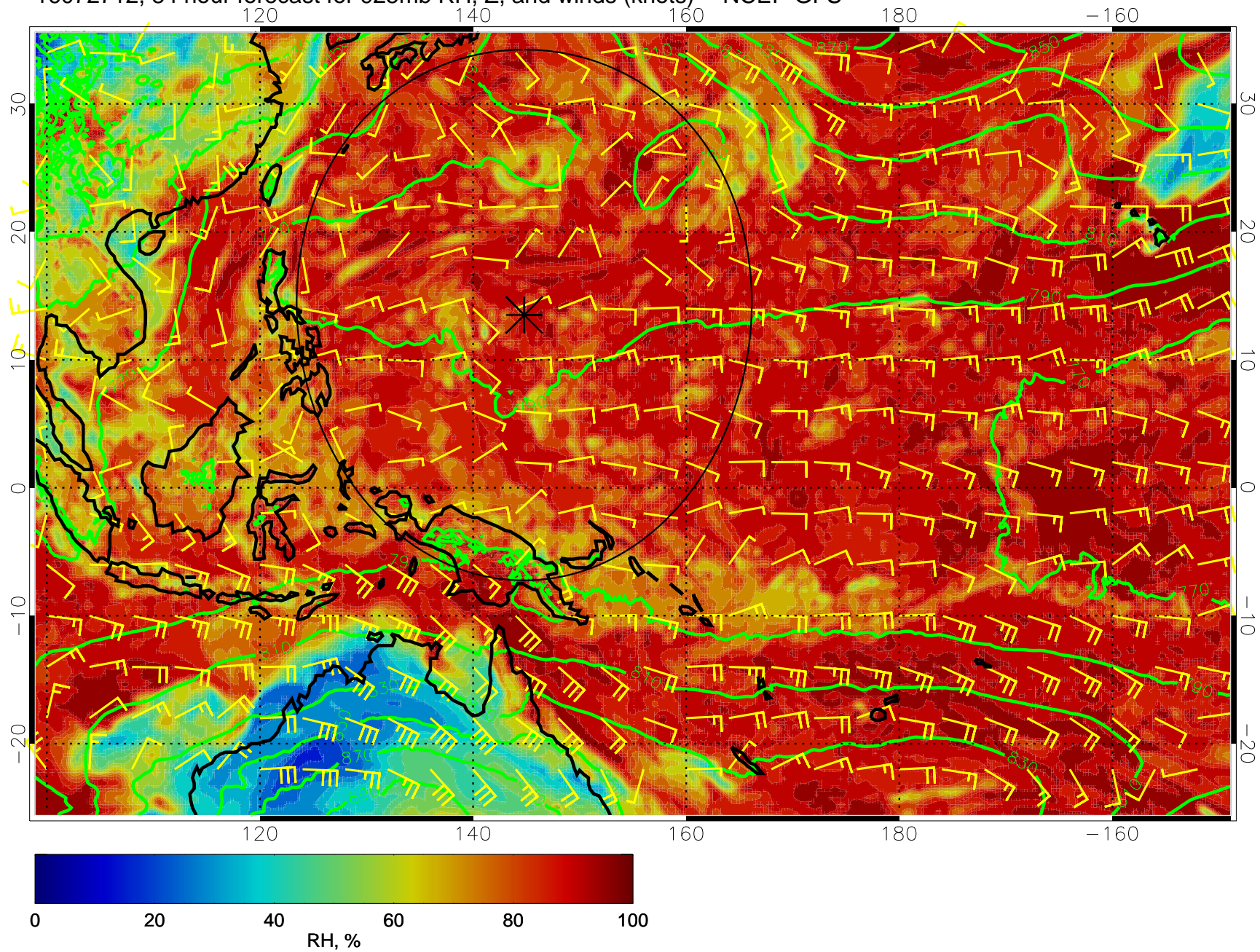
16072712, 84 hour forecast for 925mb RH, Z, and winds (knots) -- NCEP GFS
