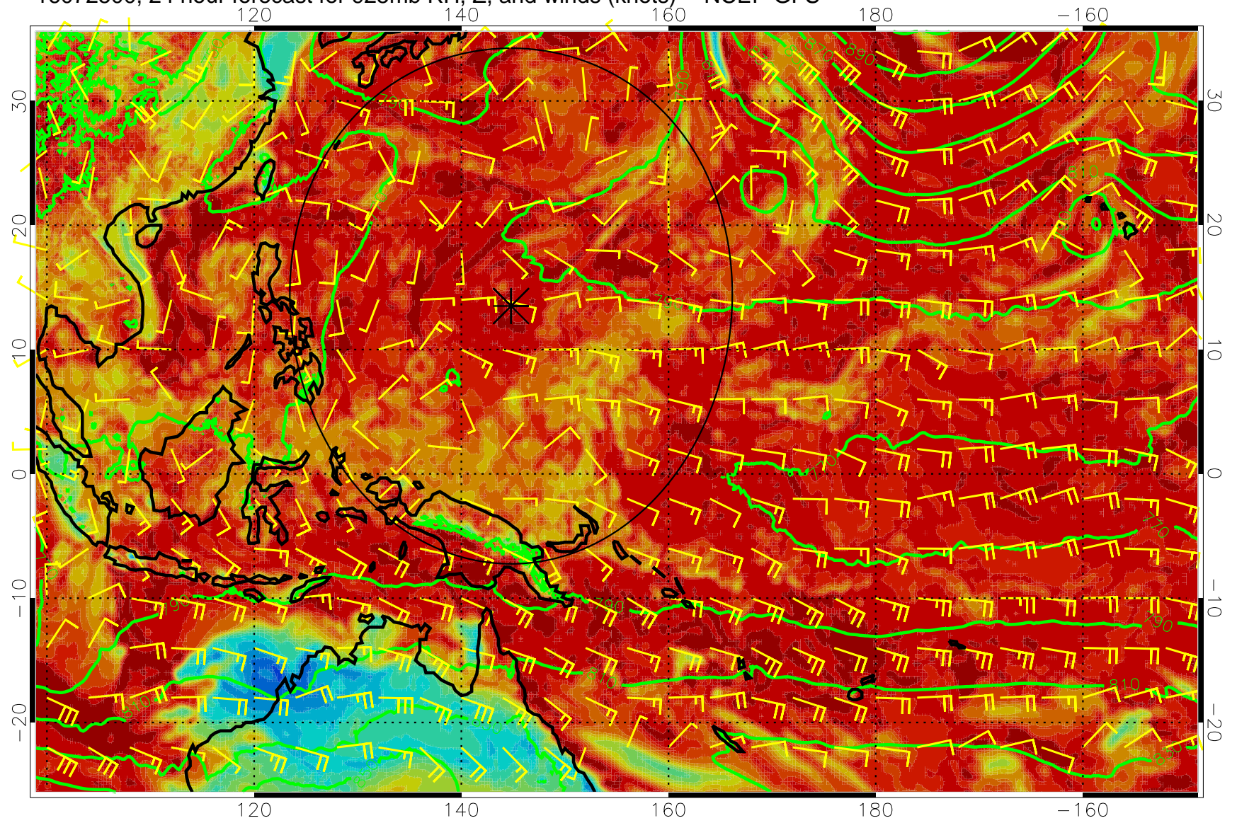
16072500, 24 hour forecast for 925mb RH, Z, and winds (knots) -- NCEP GFS
