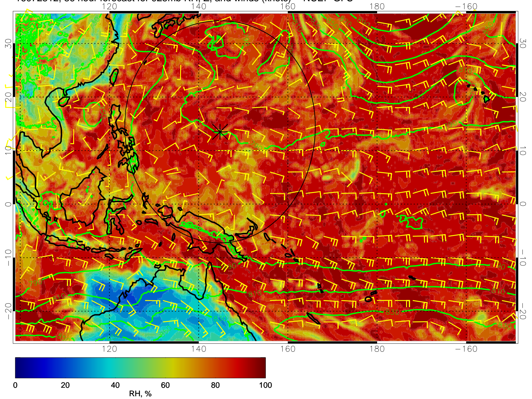
16072512, 36 hour forecast for 925mb RH, Z, and winds (knots) -- NCEP GFS
