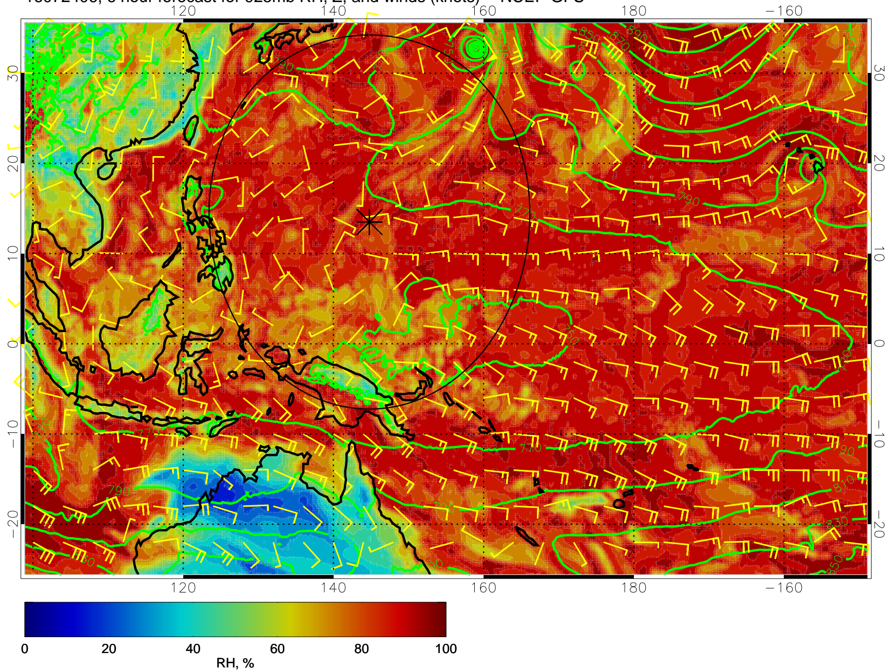
16072406, 6 hour forecast for 925mb RH, Z, and winds (knots) -- NCEP GFS
