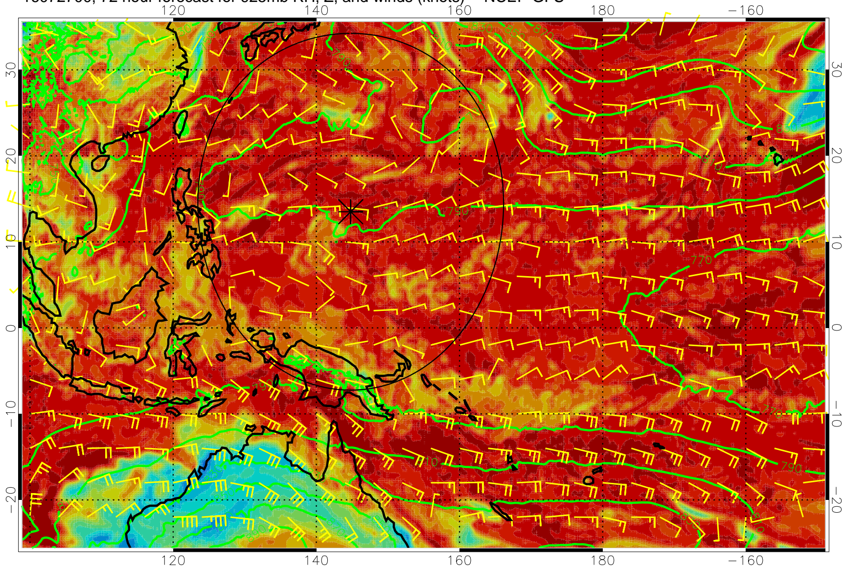
16072700, 72 hour forecast for 925mb RH, Z, and winds (knots) -- NCEP GFS
