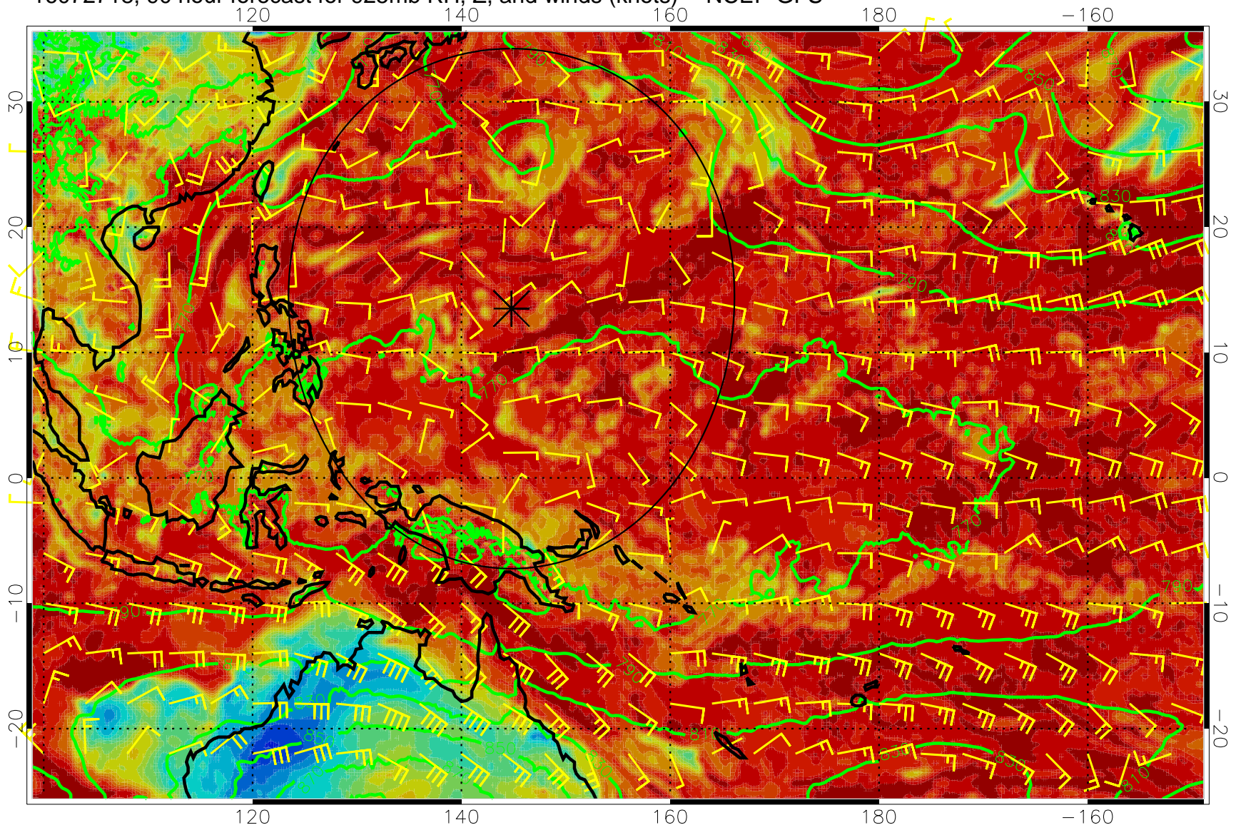
16072718, 90 hour forecast for 925mb RH, Z, and winds (knots) -- NCEP GFS
