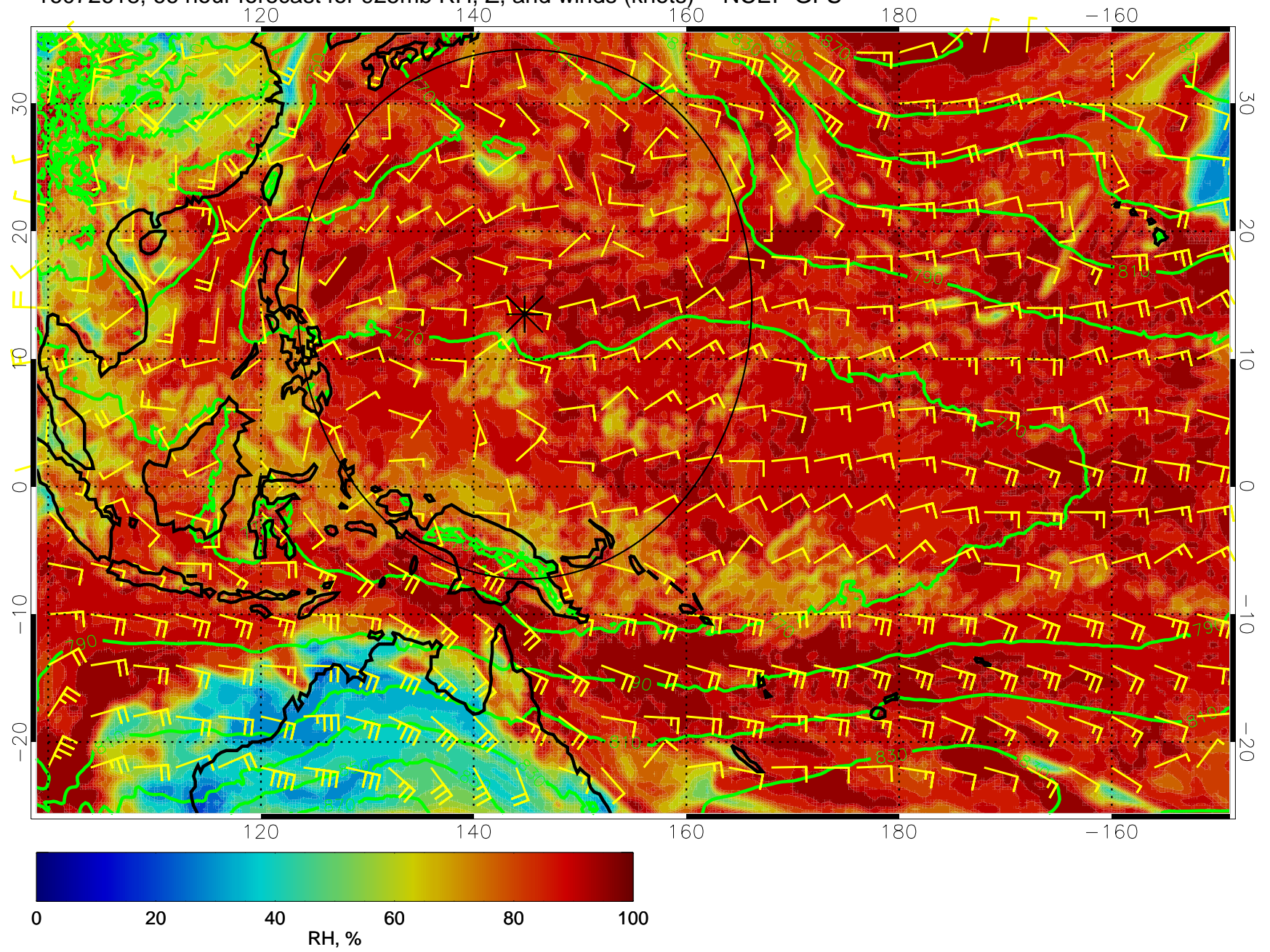
16072618, 66 hour forecast for 925mb RH, Z, and winds (knots) -- NCEP GFS
