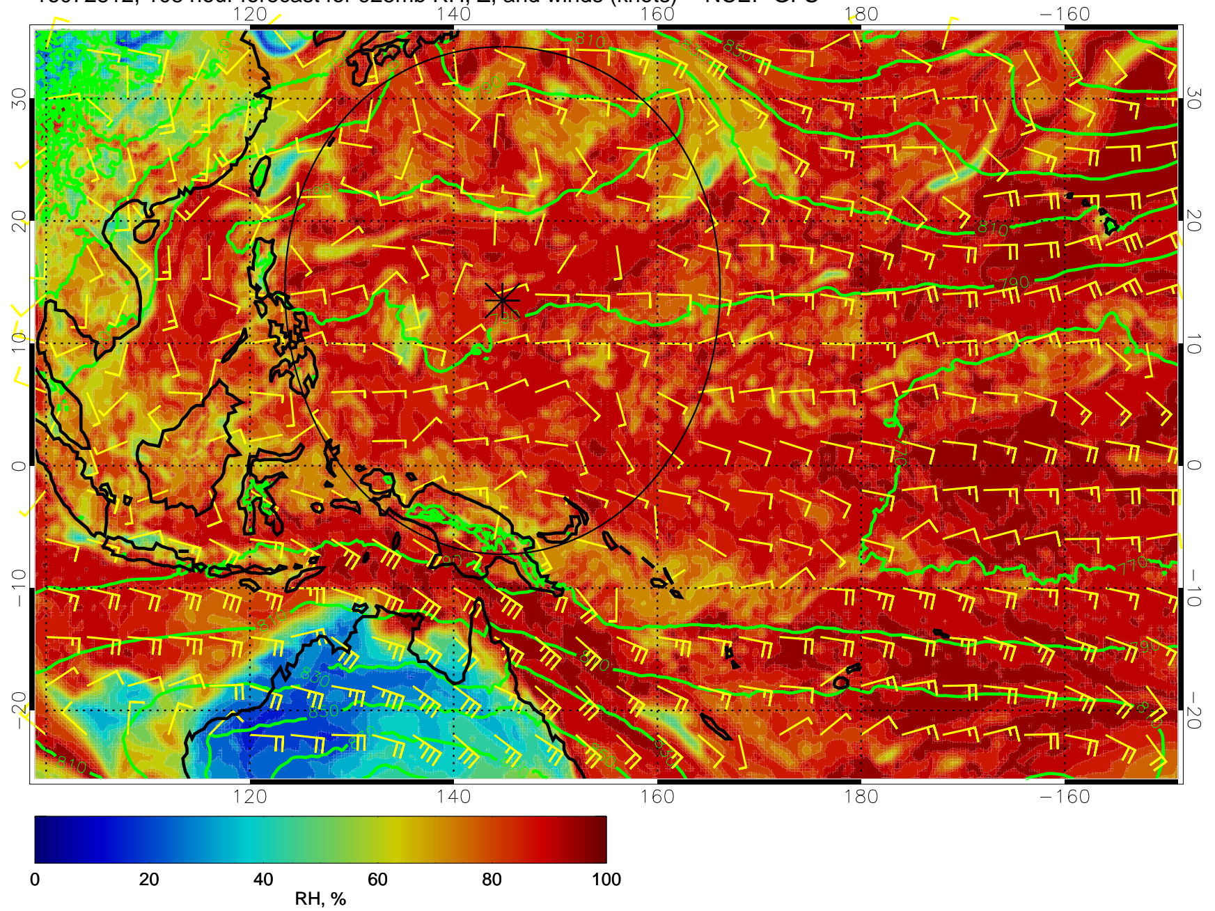
16072812, 108 hour forecast for 925mb RH, Z, and winds (knots) -- NCEP GFS
