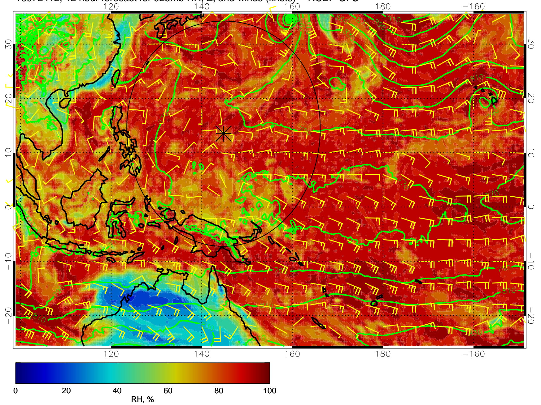
16072412, 12 hour forecast for 925mb RH, Z, and winds (knots) -- NCEP GFS
