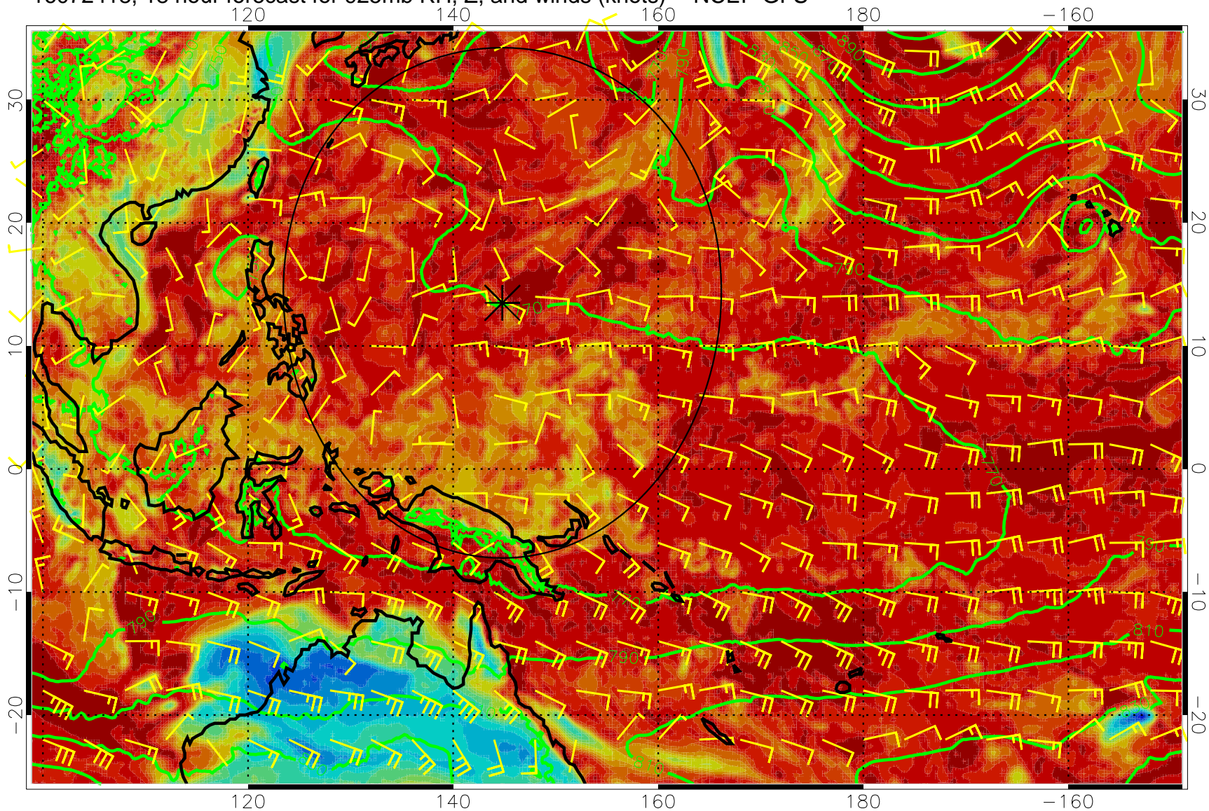
16072418, 18 hour forecast for 925mb RH, Z, and winds (knots) -- NCEP GFS
