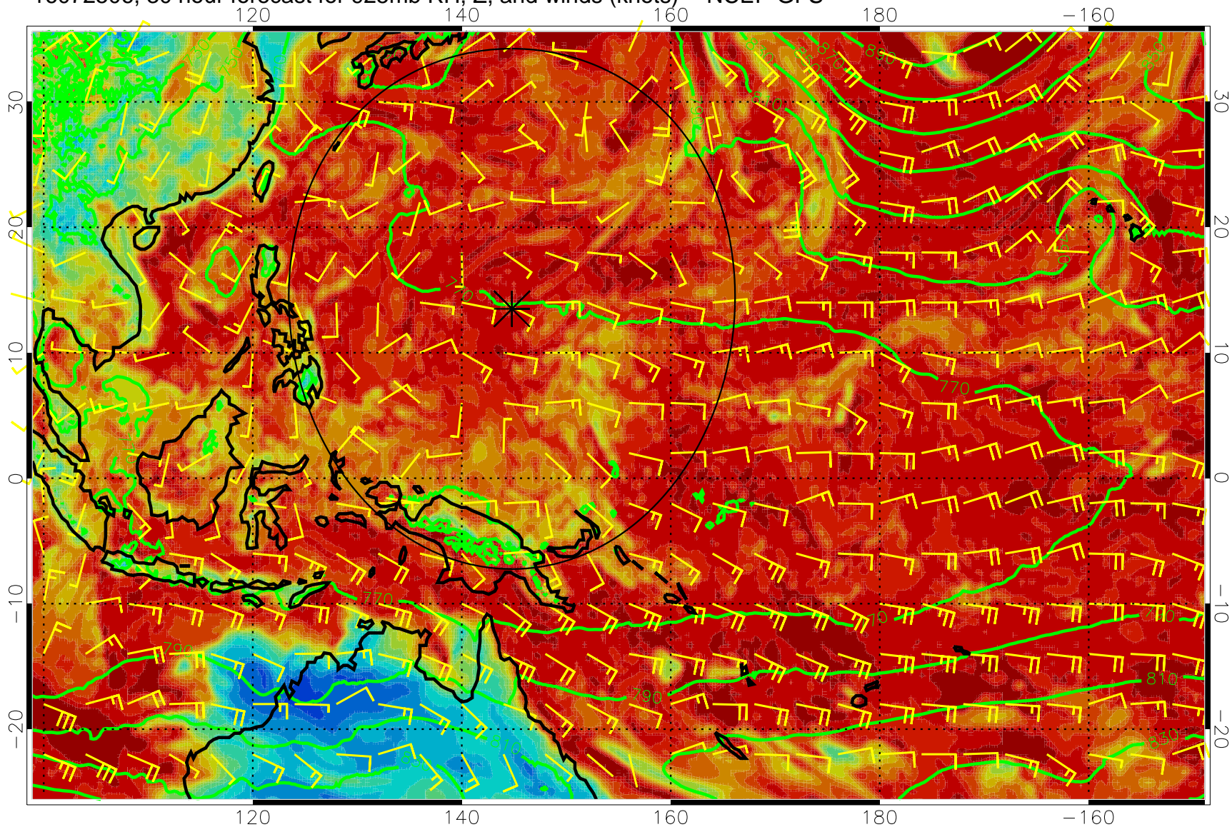
16072506, 30 hour forecast for 925mb RH, Z, and winds (knots) -- NCEP GFS
