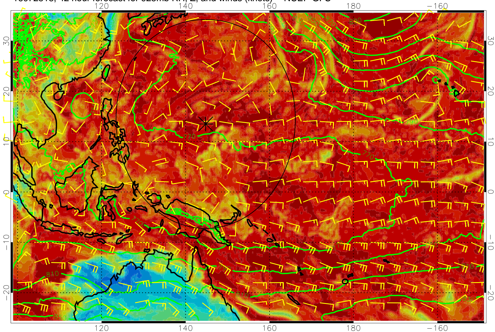
16072518, 42 hour forecast for 925mb RH, Z, and winds (knots) -- NCEP GFS
