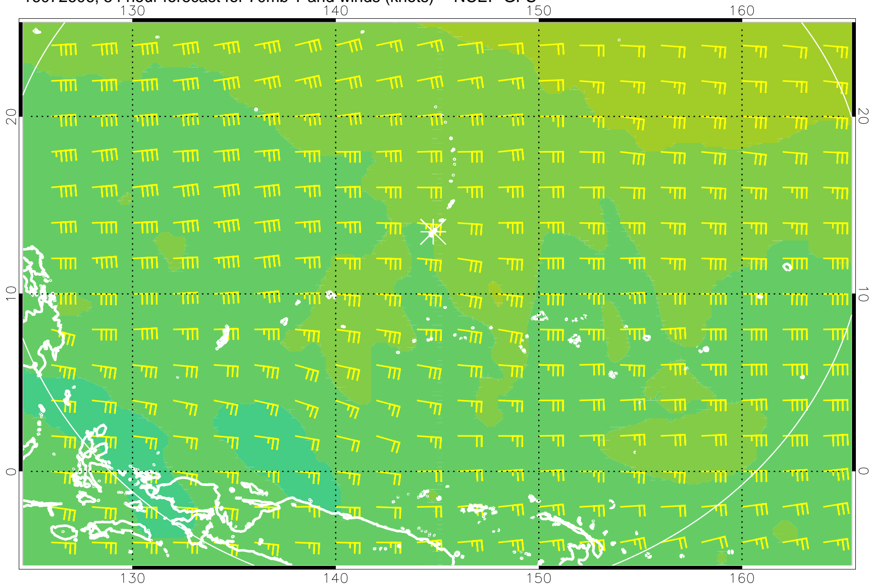
16072606, 54 hour forecast for 70mb T and winds (knots) -- NCEP GFS
