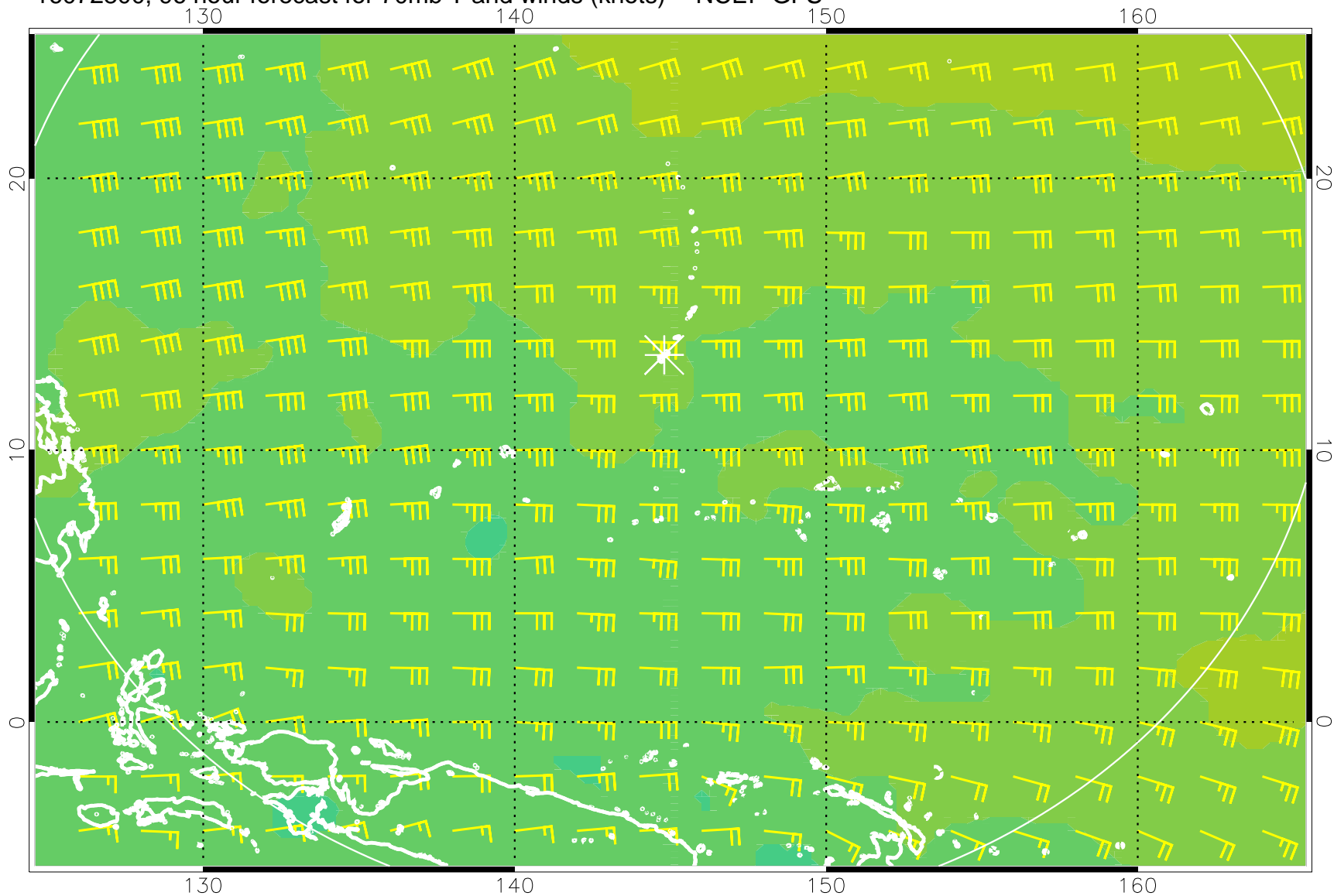
16072800, 96 hour forecast for 70mb T and winds (knots) -- NCEP GFS
