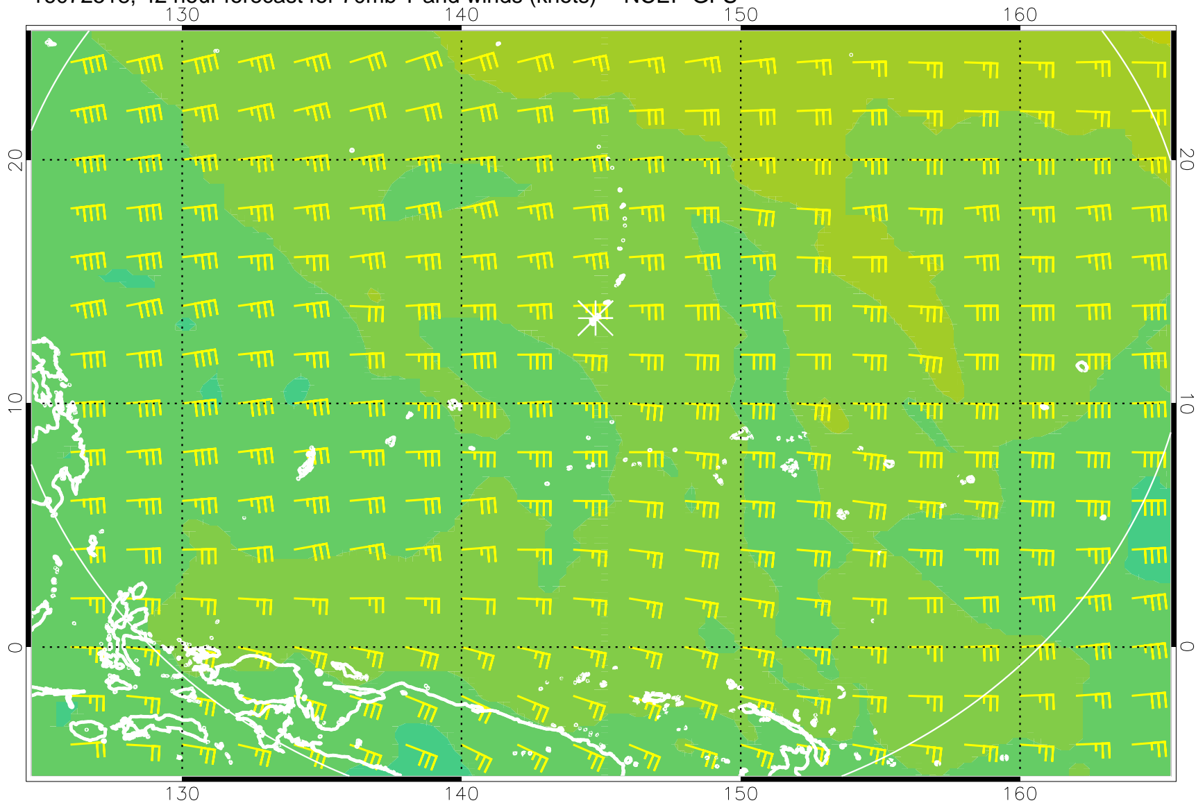
16072518, 42 hour forecast for 70mb T and winds (knots) -- NCEP GFS
