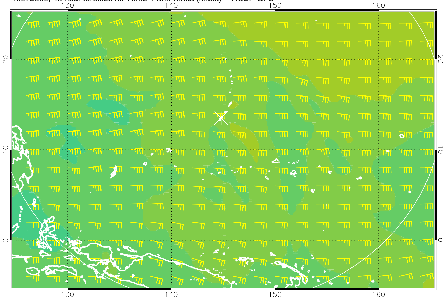
16072600, 48 hour forecast for 70mb T and winds (knots) -- NCEP GFS
