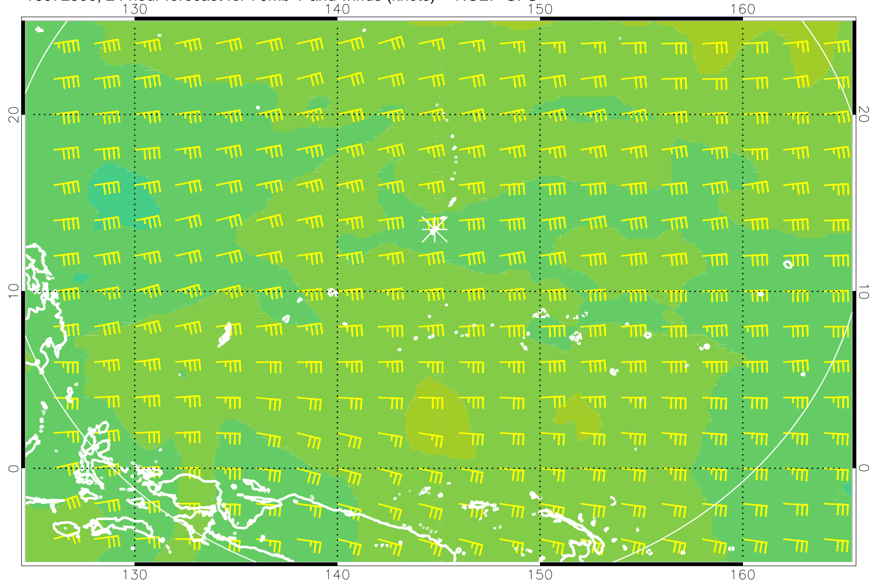
16072500, 24 hour forecast for 70mb T and winds (knots) -- NCEP GFS
