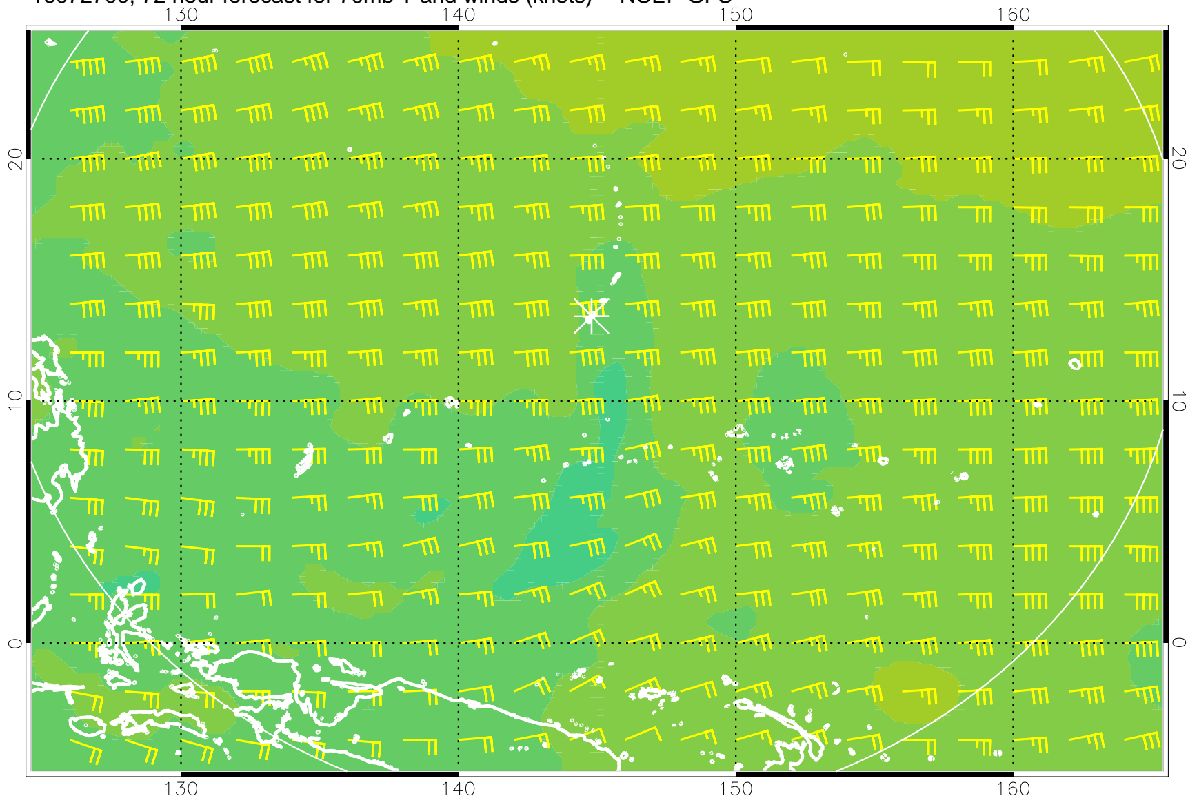
16072700, 72 hour forecast for 70mb T and winds (knots) -- NCEP GFS
