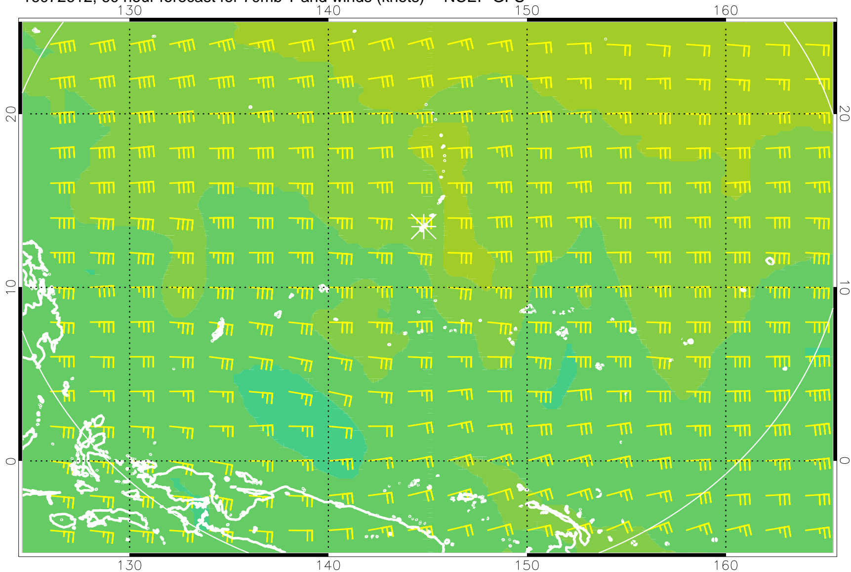
16072612, 60 hour forecast for 70mb T and winds (knots) -- NCEP GFS
