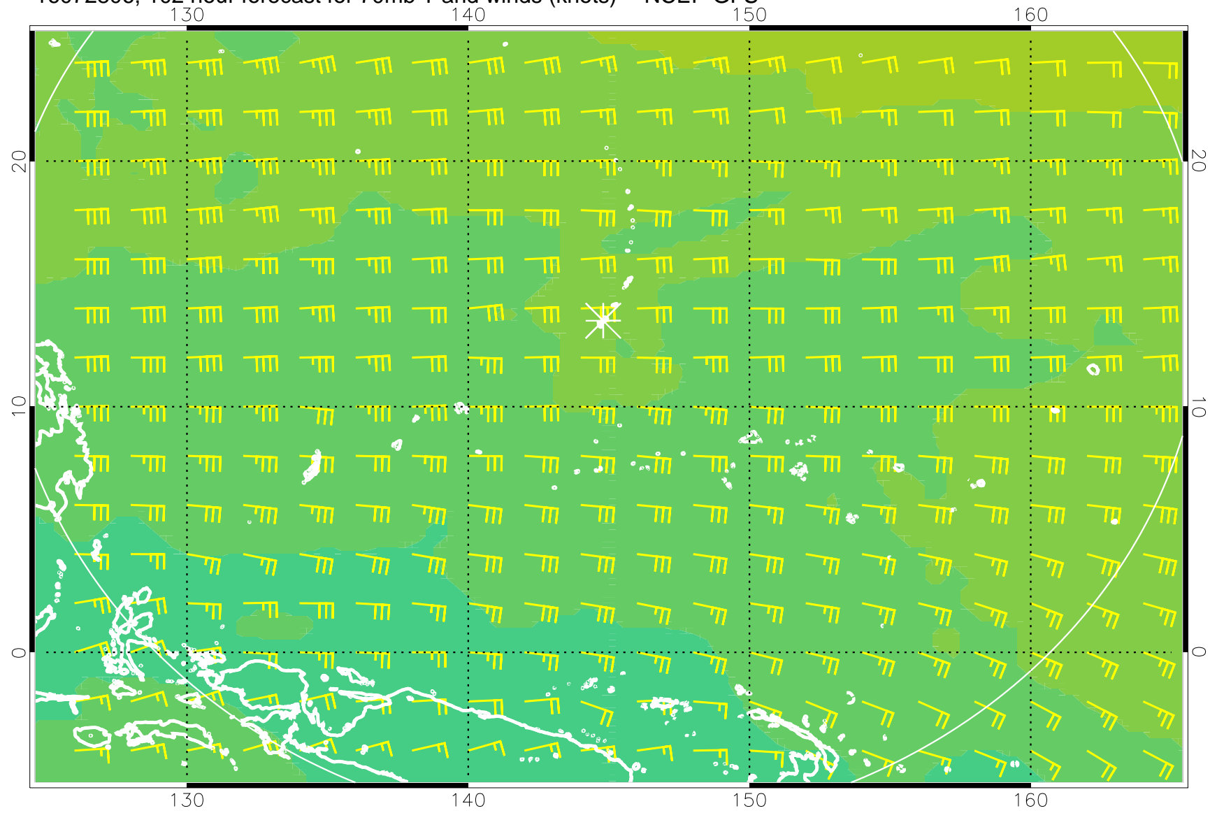
16072806, 102 hour forecast for 70mb T and winds (knots) -- NCEP GFS
