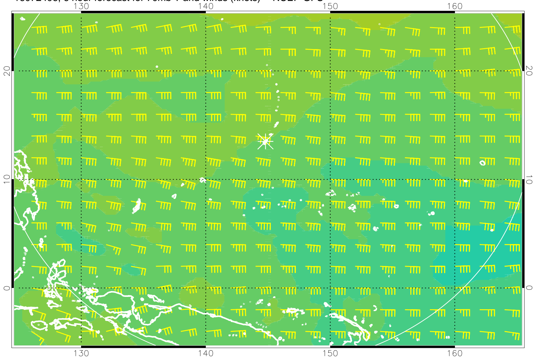
16072406, 6 hour forecast for 70mb T and winds (knots) -- NCEP GFS
