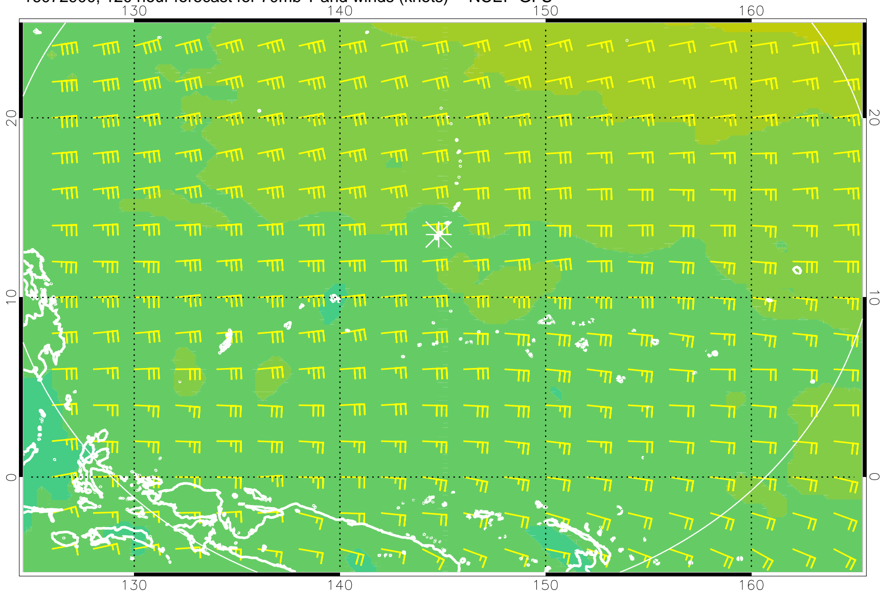
16072900, 120 hour forecast for 70mb T and winds (knots) -- NCEP GFS
