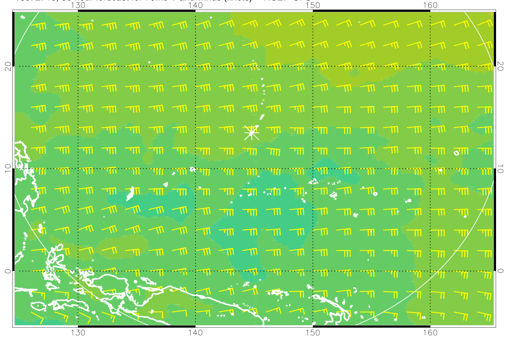
16072718, 90 hour forecast for 70mb T and winds (knots) -- NCEP GFS
