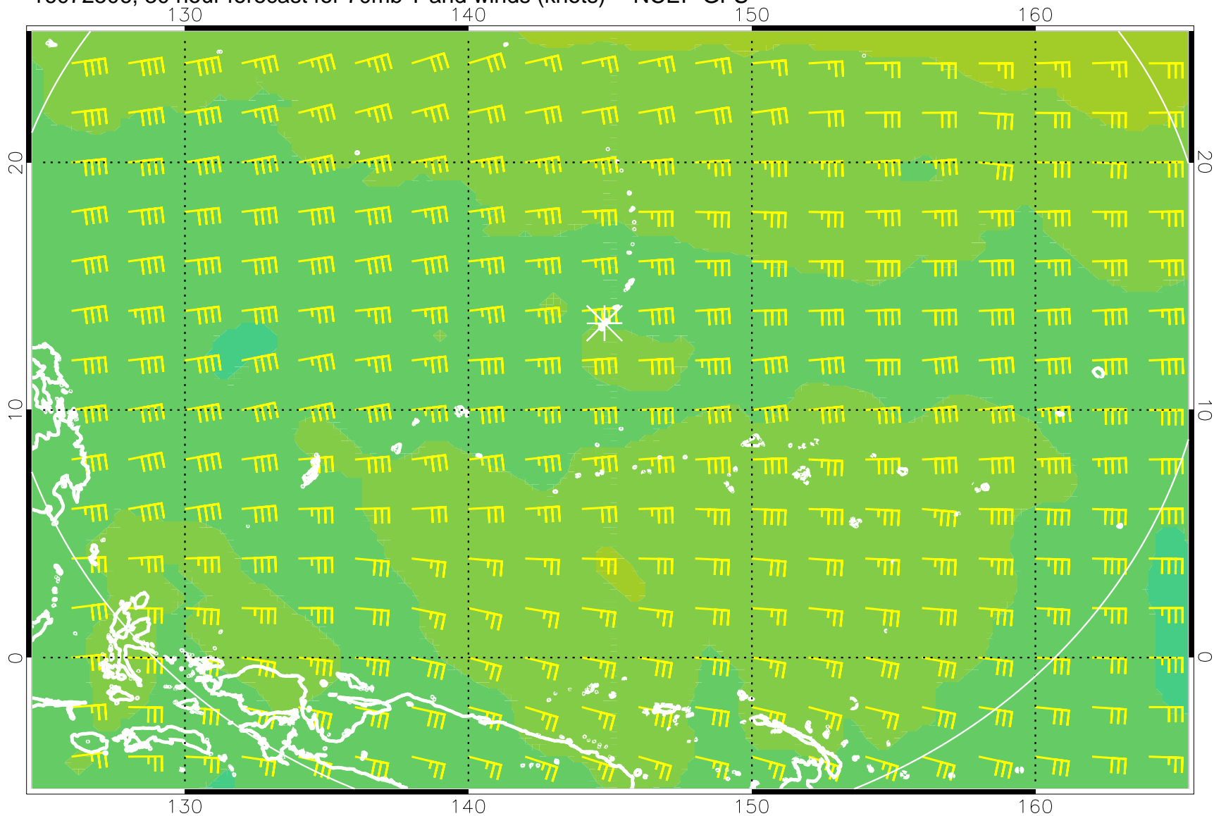
16072506, 30 hour forecast for 70mb T and winds (knots) -- NCEP GFS
