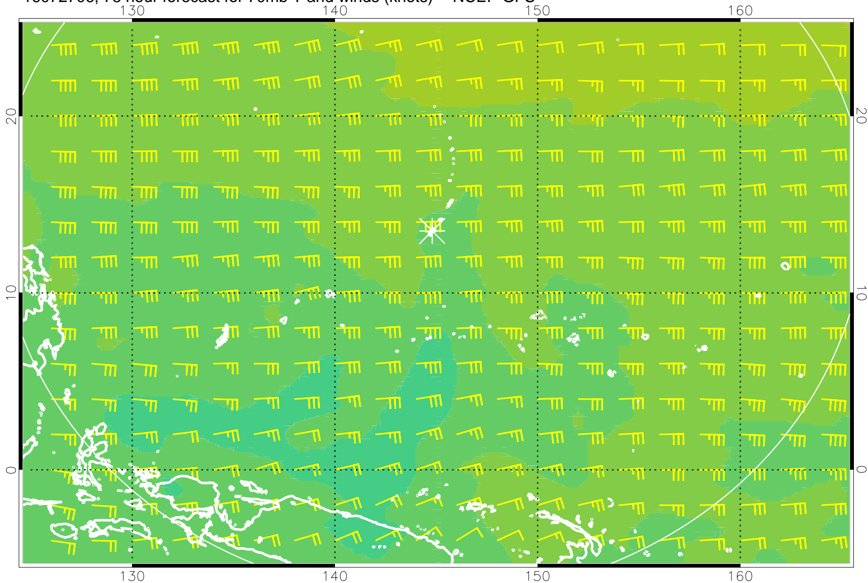
16072706, 78 hour forecast for 70mb T and winds (knots) -- NCEP GFS
