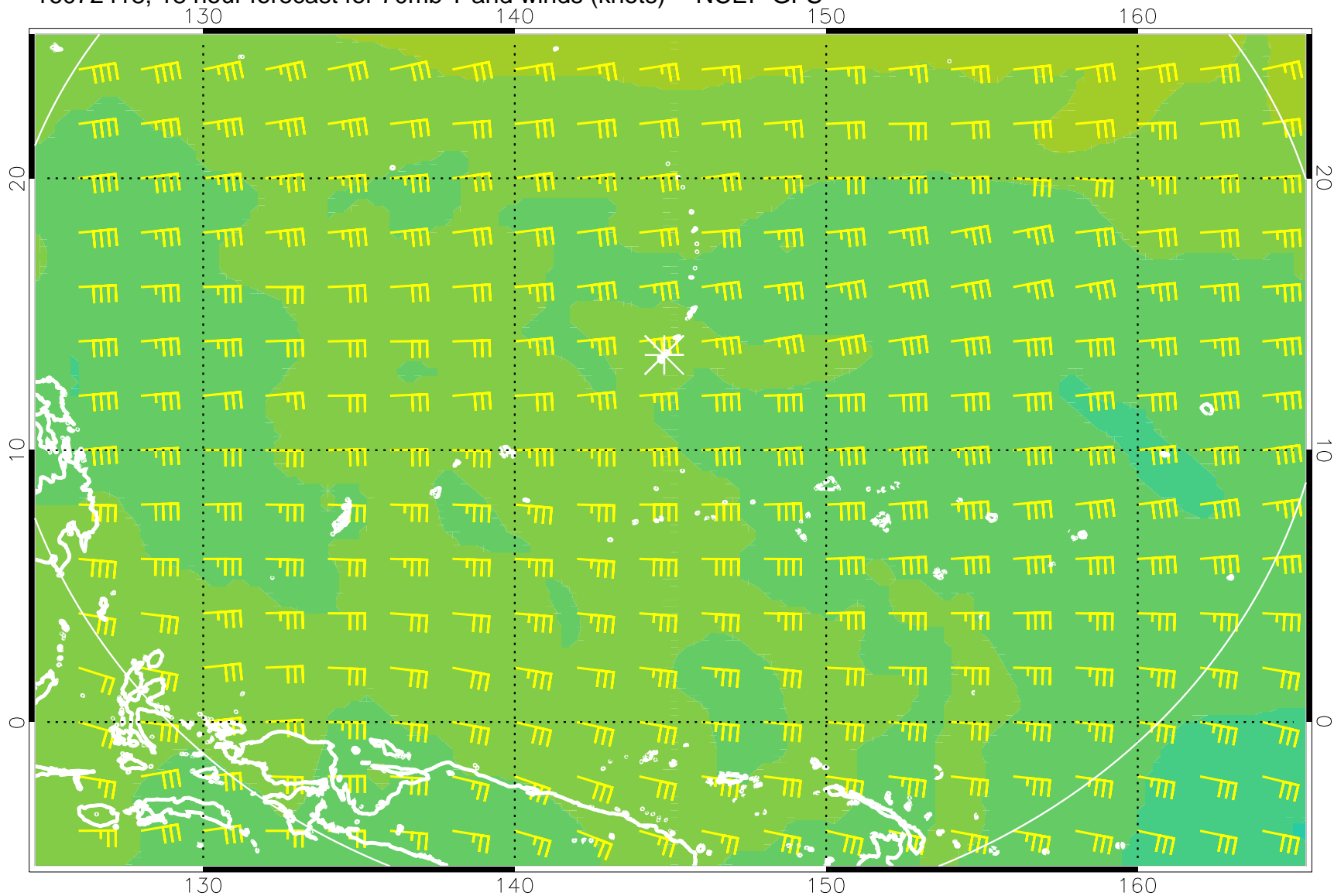
16072418, 18 hour forecast for 70mb T and winds (knots) -- NCEP GFS
