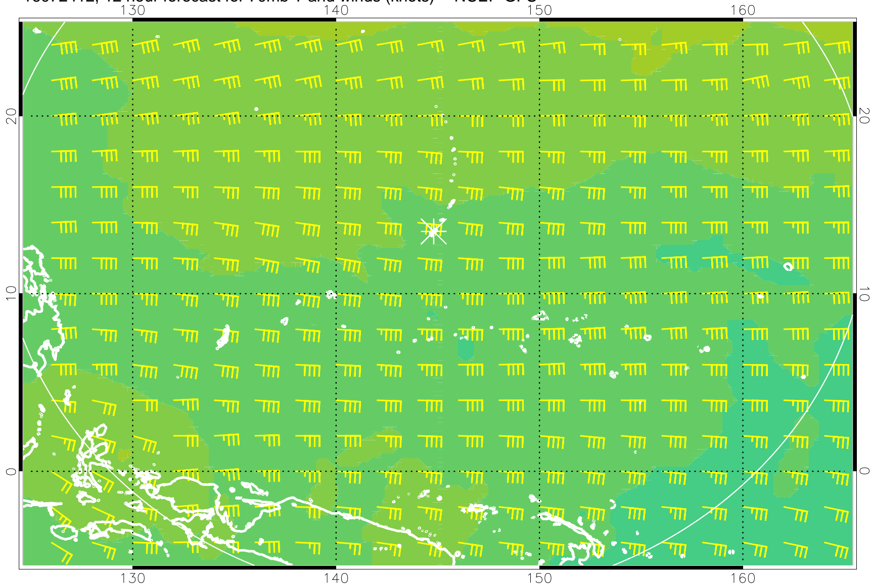
16072412, 12 hour forecast for 70mb T and winds (knots) -- NCEP GFS
