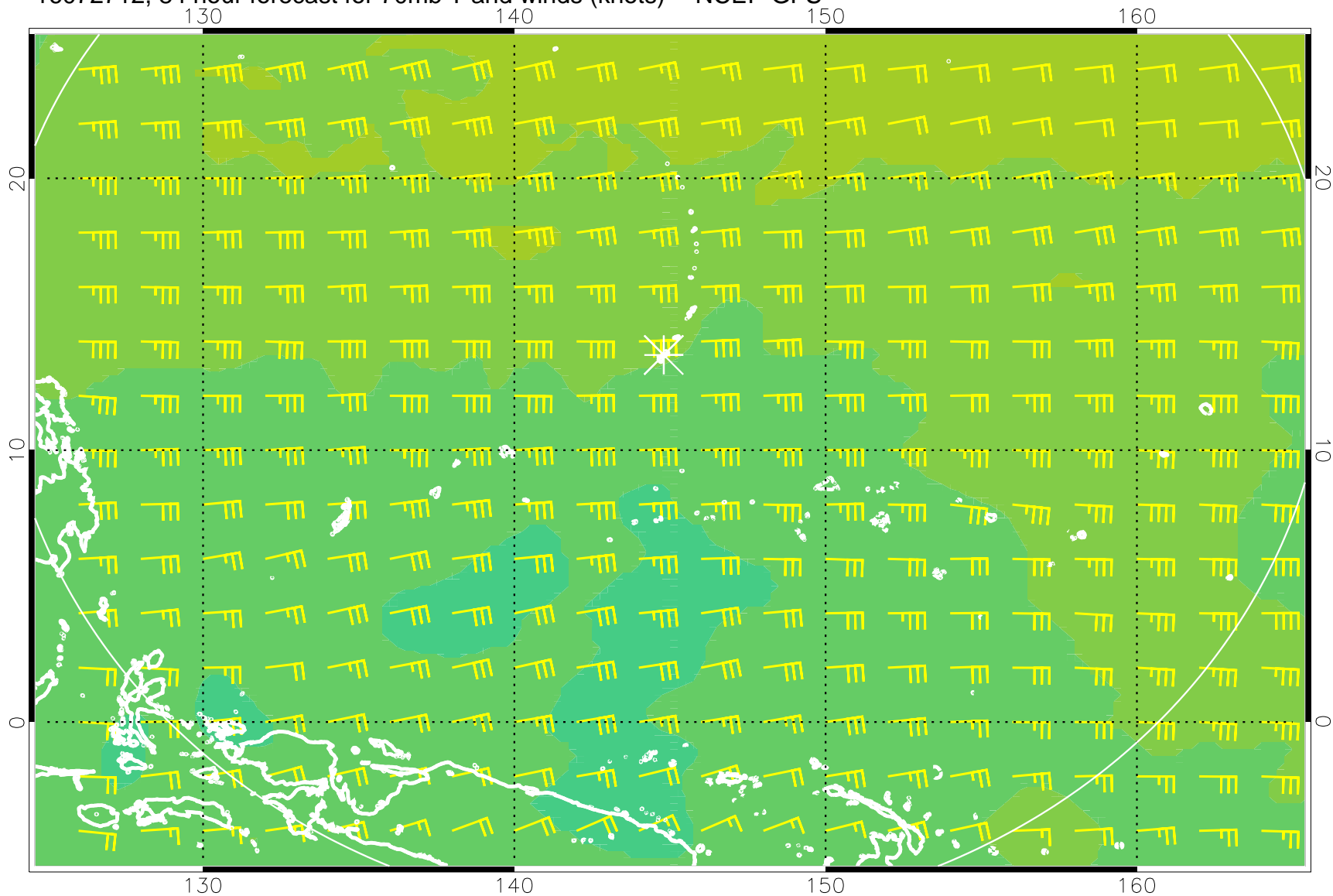
16072712, 84 hour forecast for 70mb T and winds (knots) -- NCEP GFS
