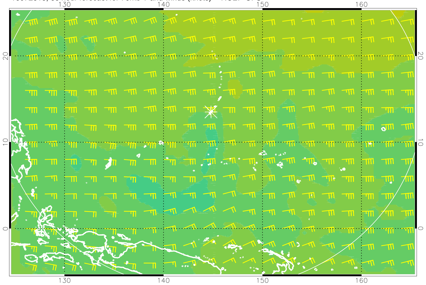
16072618, 66 hour forecast for 70mb T and winds (knots) -- NCEP GFS
