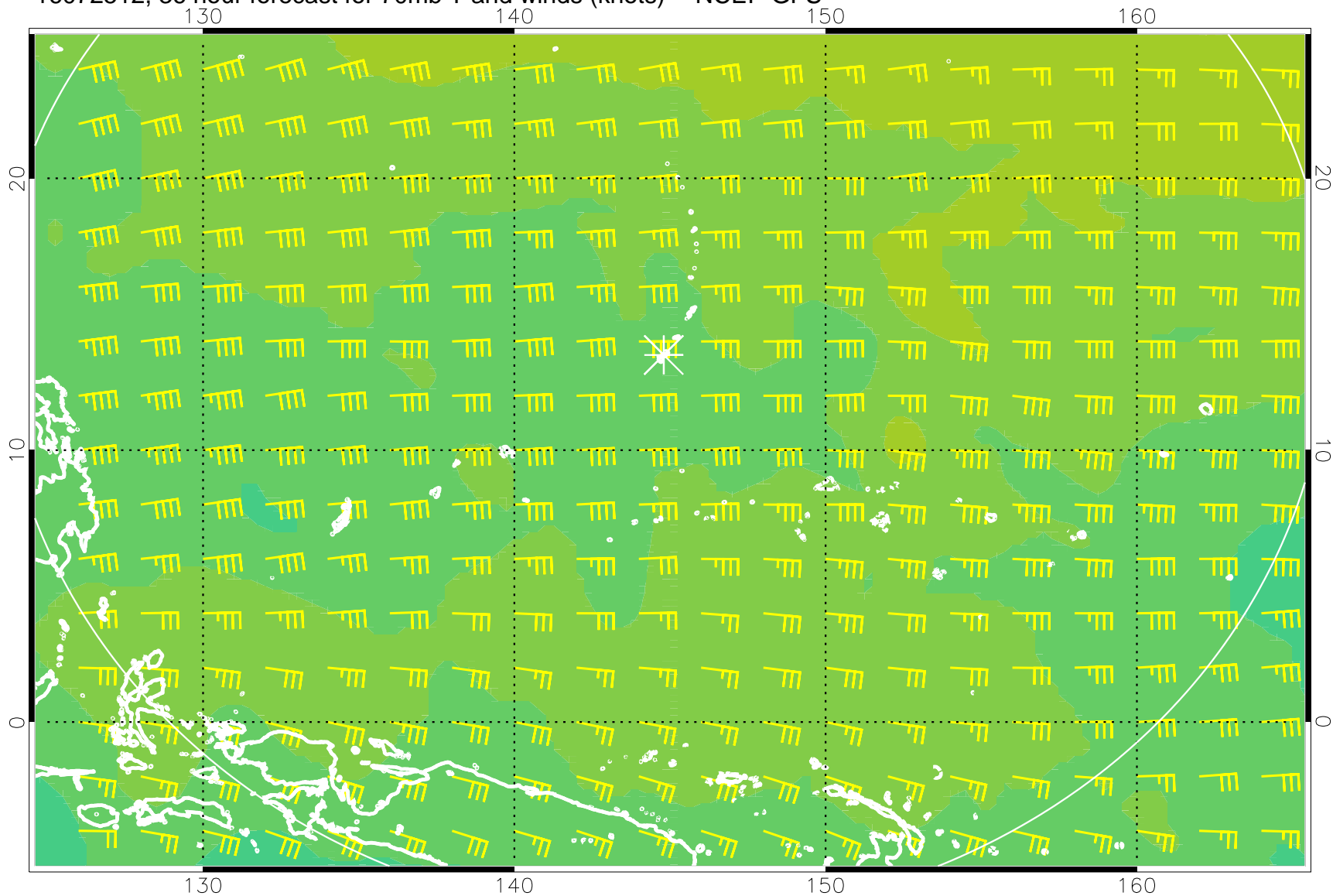
16072512, 36 hour forecast for 70mb T and winds (knots) -- NCEP GFS
