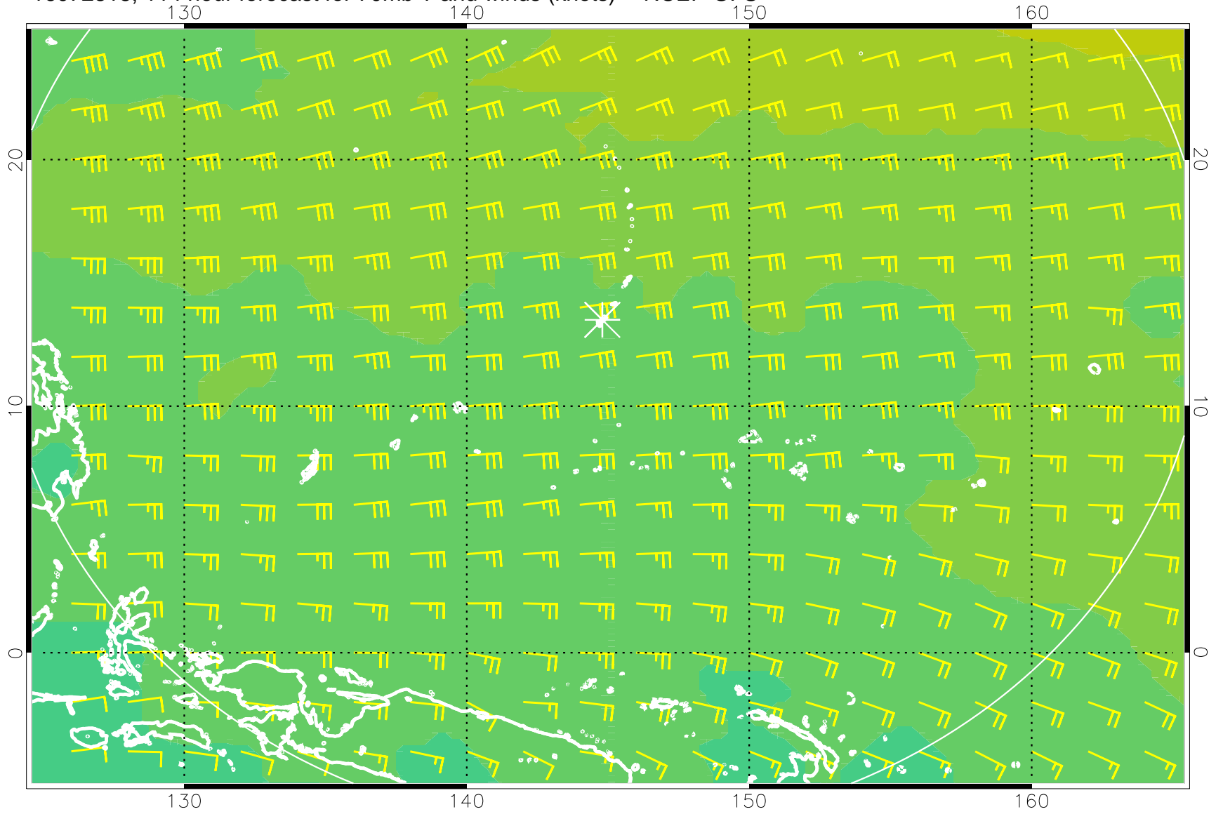
16072818, 114 hour forecast for 70mb T and winds (knots) -- NCEP GFS
