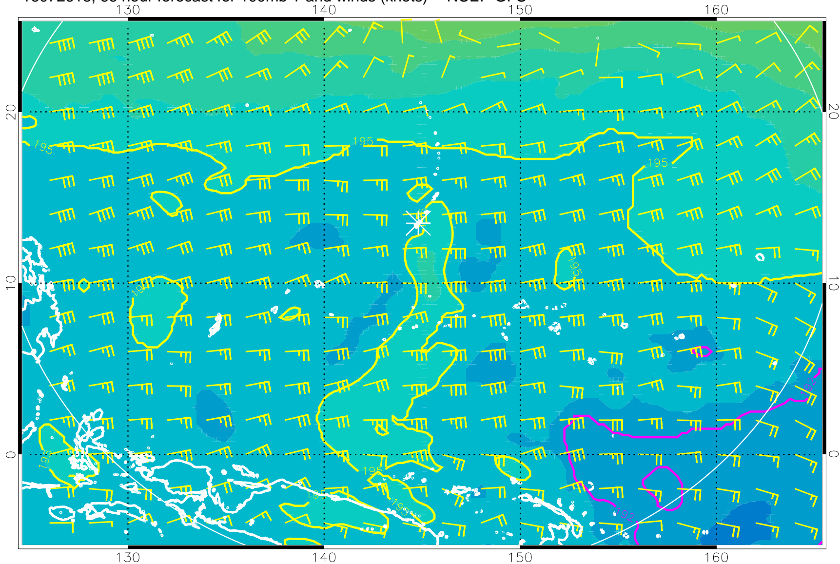
16072618, 66 hour forecast for 100mb T and winds (knots) -- NCEP GFS
