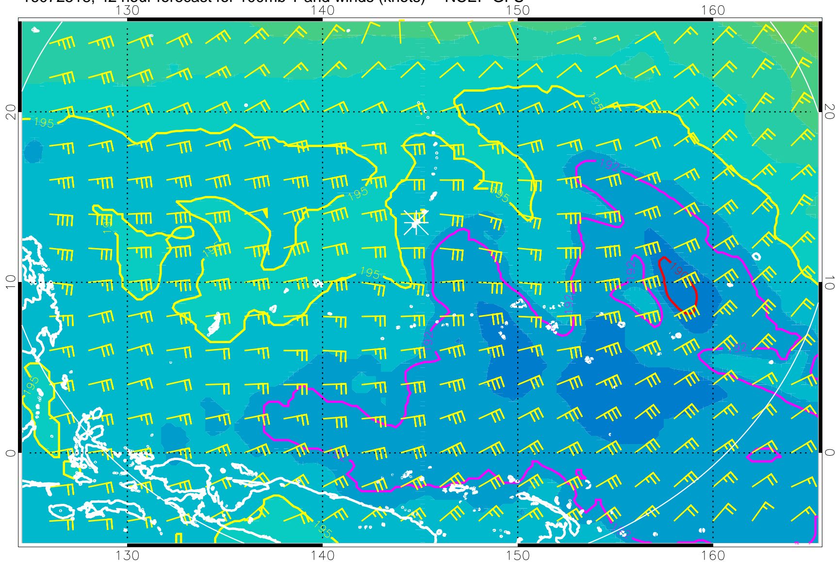
16072518, 42 hour forecast for 100mb T and winds (knots) -- NCEP GFS
