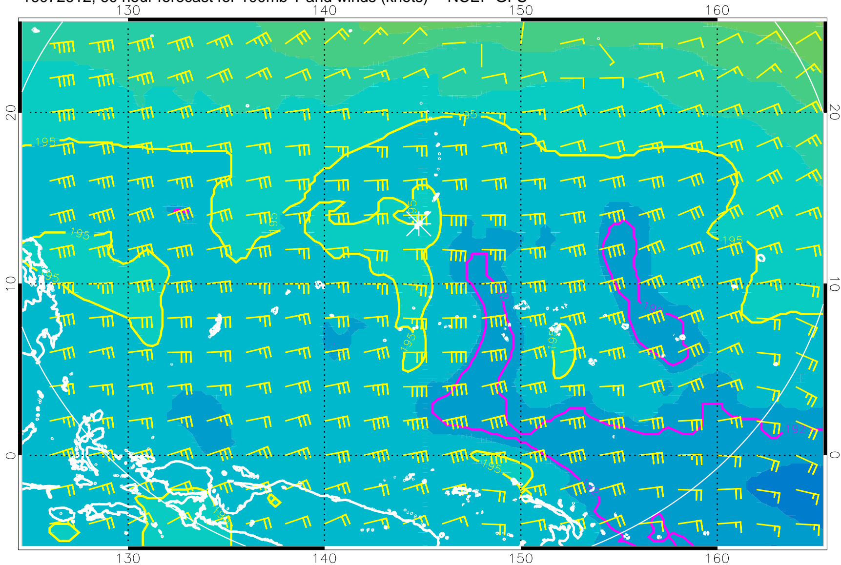
16072612, 60 hour forecast for 100mb T and winds (knots) -- NCEP GFS
