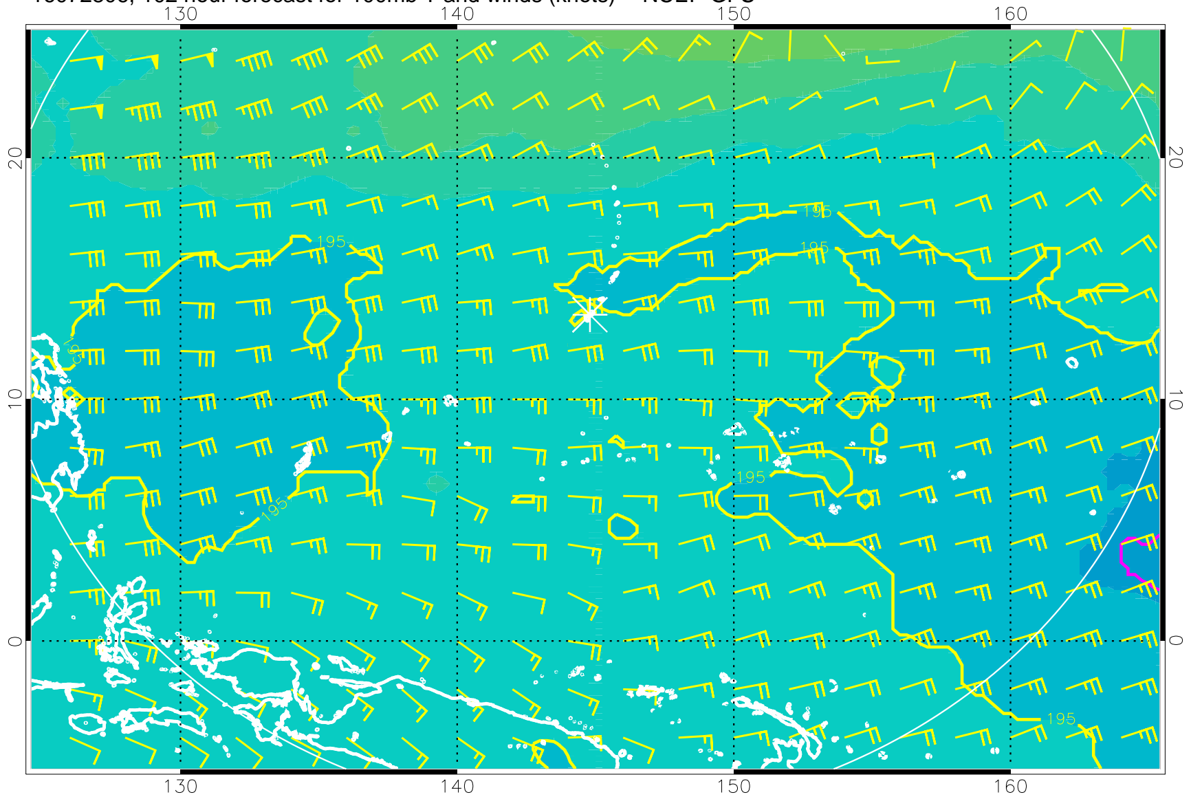
16072806, 102 hour forecast for 100mb T and winds (knots) -- NCEP GFS
