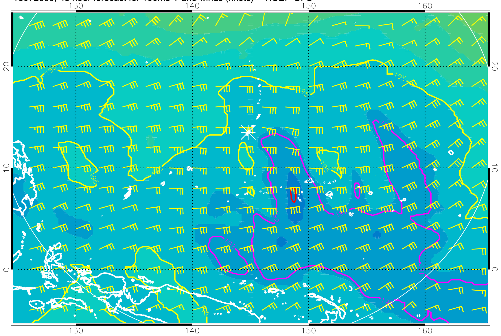
16072600, 48 hour forecast for 100mb T and winds (knots) -- NCEP GFS
