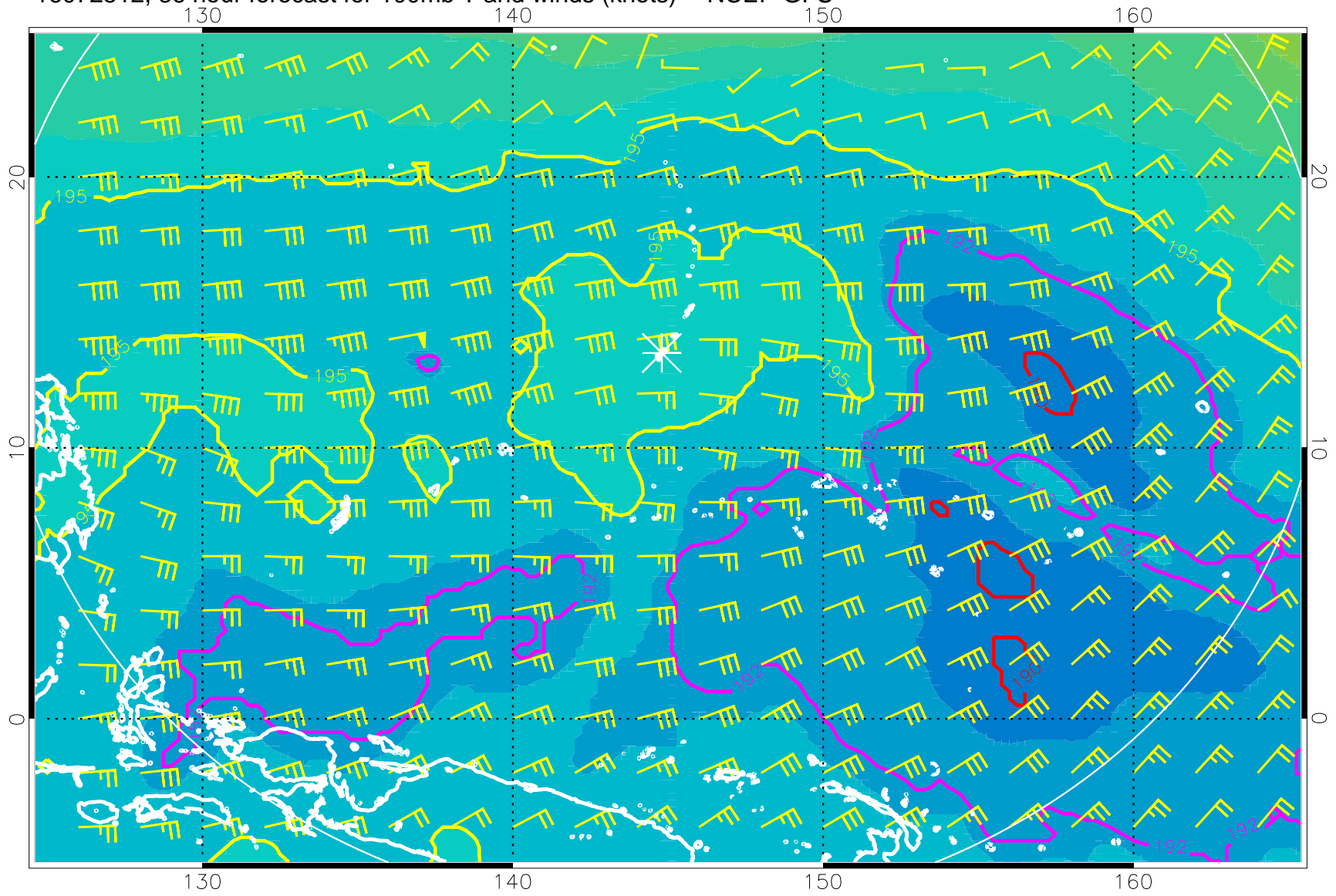
16072512, 36 hour forecast for 100mb T and winds (knots) -- NCEP GFS
