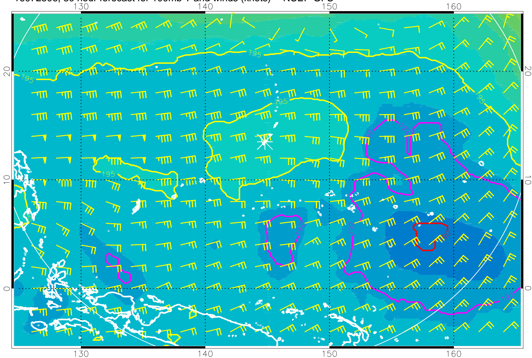
16072506, 30 hour forecast for 100mb T and winds (knots) -- NCEP GFS
