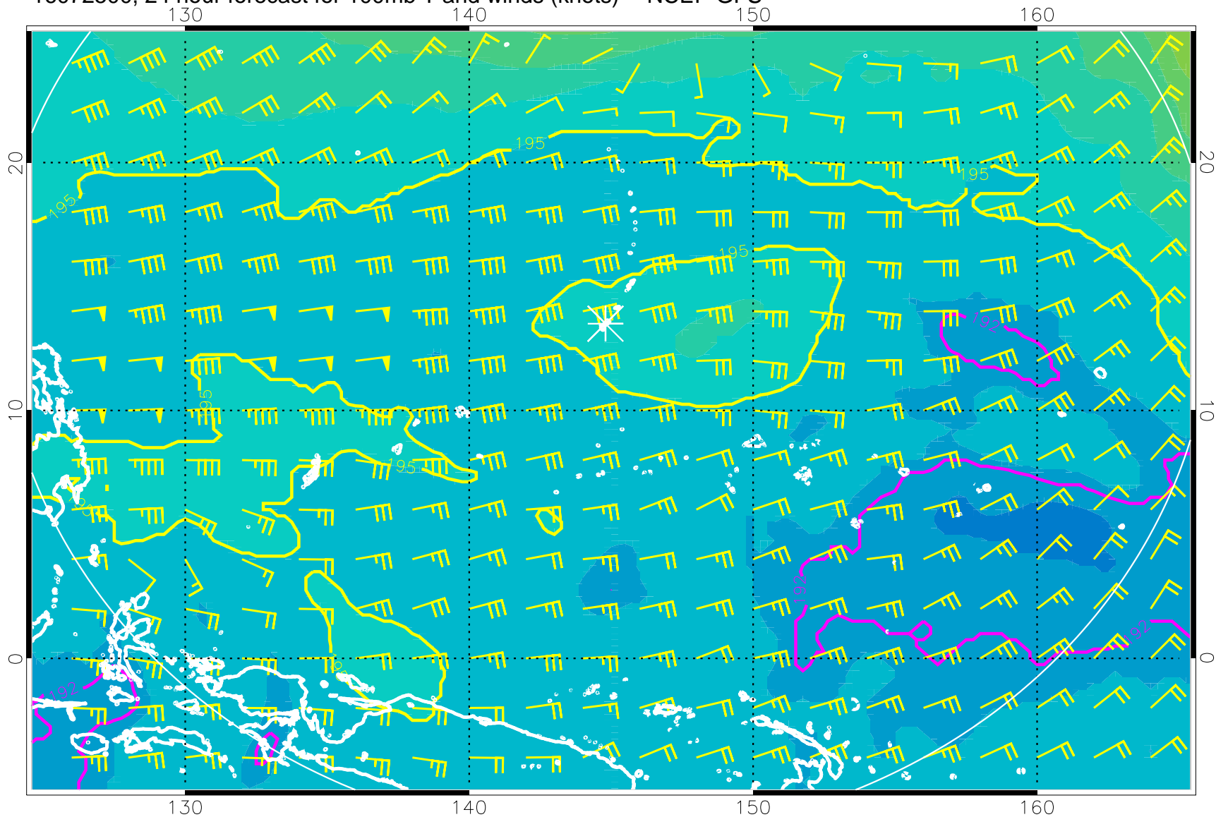
16072500, 24 hour forecast for 100mb T and winds (knots) -- NCEP GFS
