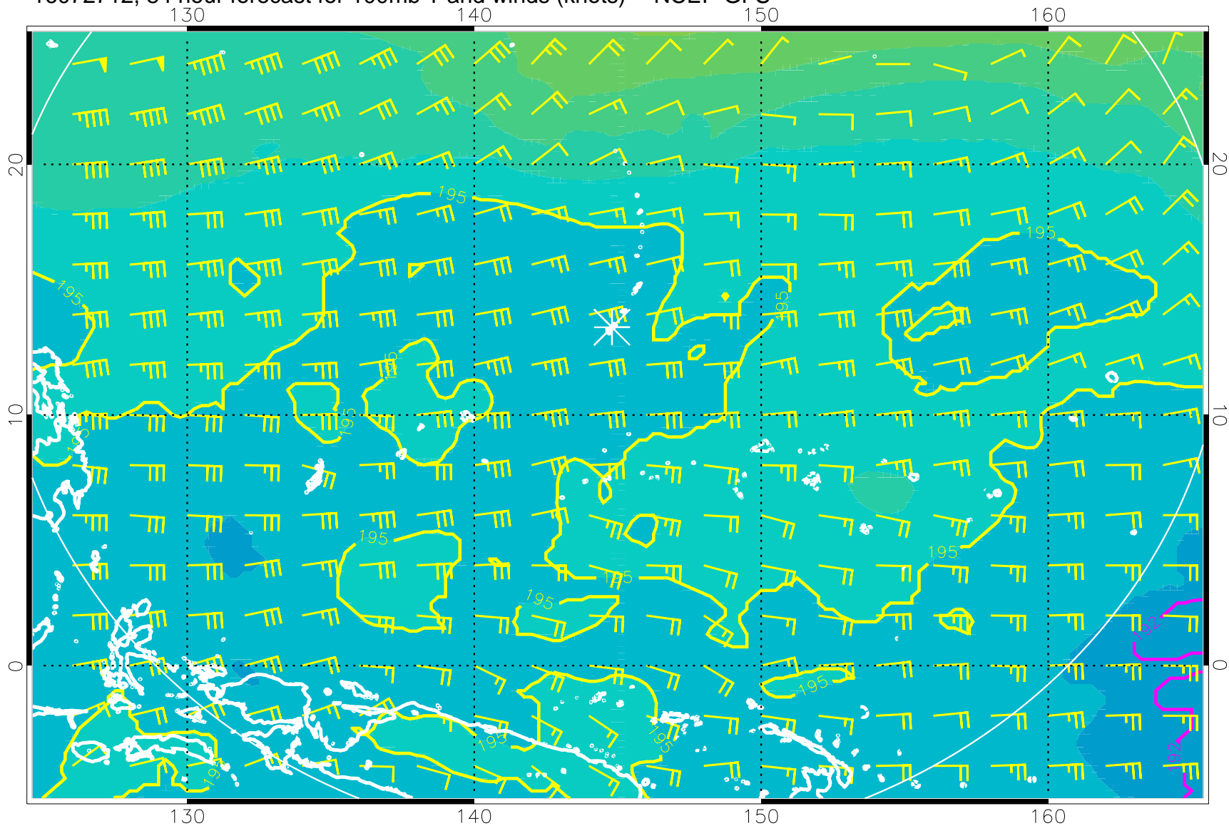
16072712, 84 hour forecast for 100mb T and winds (knots) -- NCEP GFS
