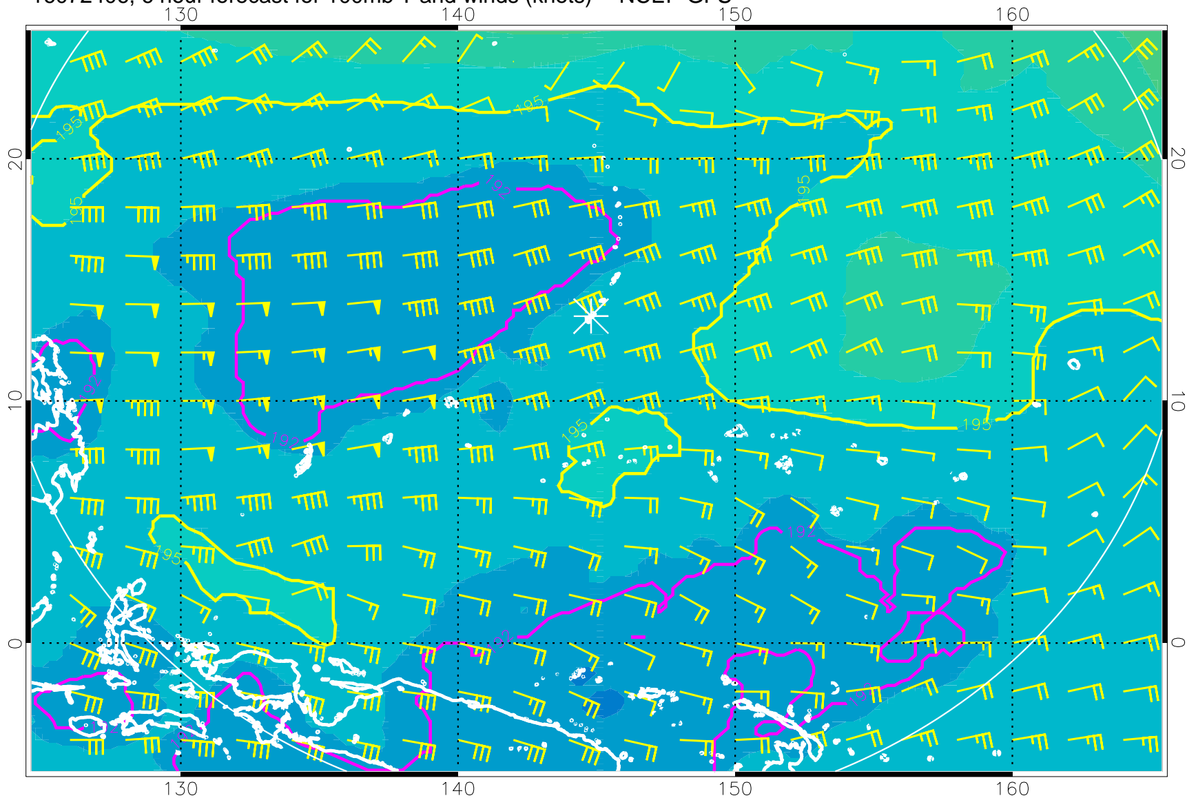
16072406, 6 hour forecast for 100mb T and winds (knots) -- NCEP GFS
