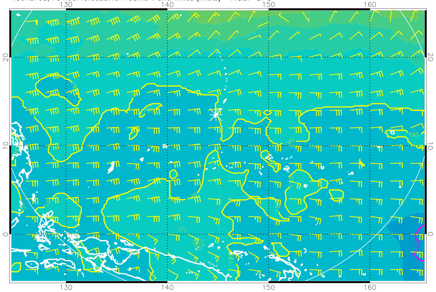
16072706, 78 hour forecast for 100mb T and winds (knots) -- NCEP GFS
