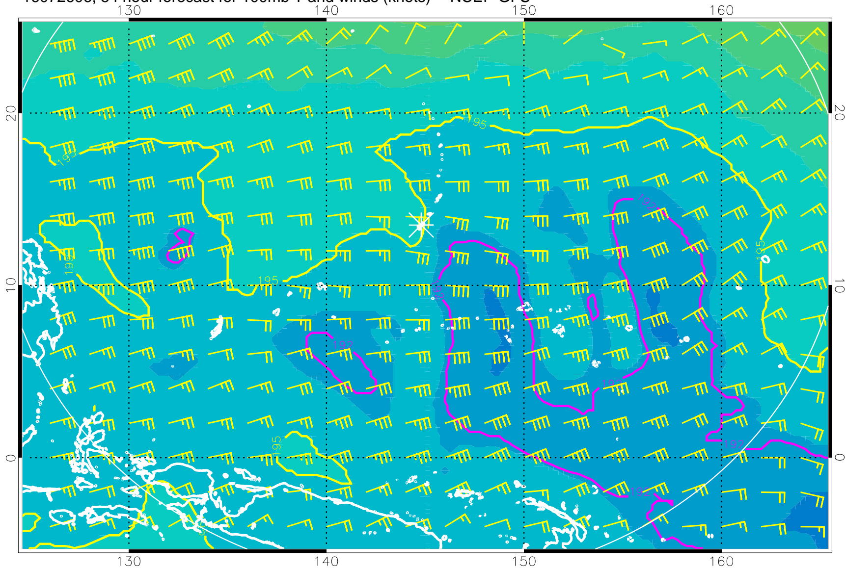
16072606, 54 hour forecast for 100mb T and winds (knots) -- NCEP GFS
