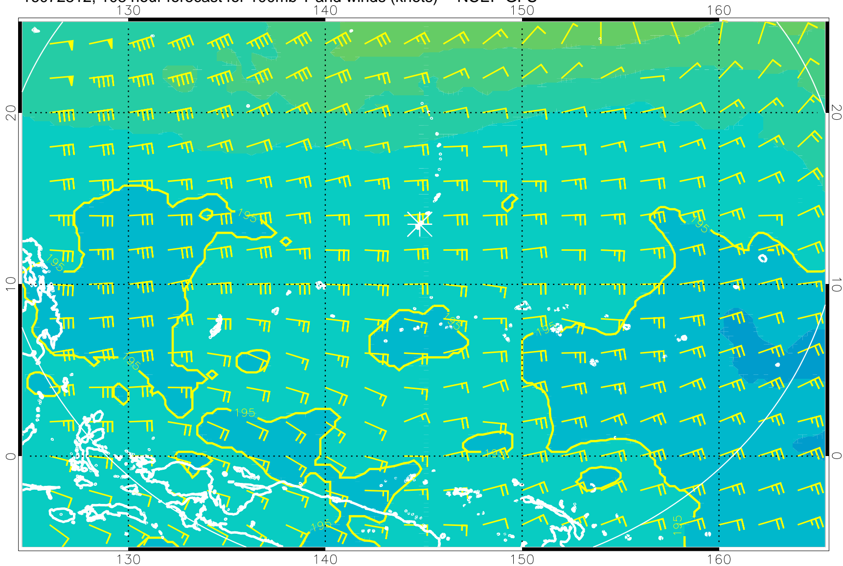
16072812, 108 hour forecast for 100mb T and winds (knots) -- NCEP GFS
