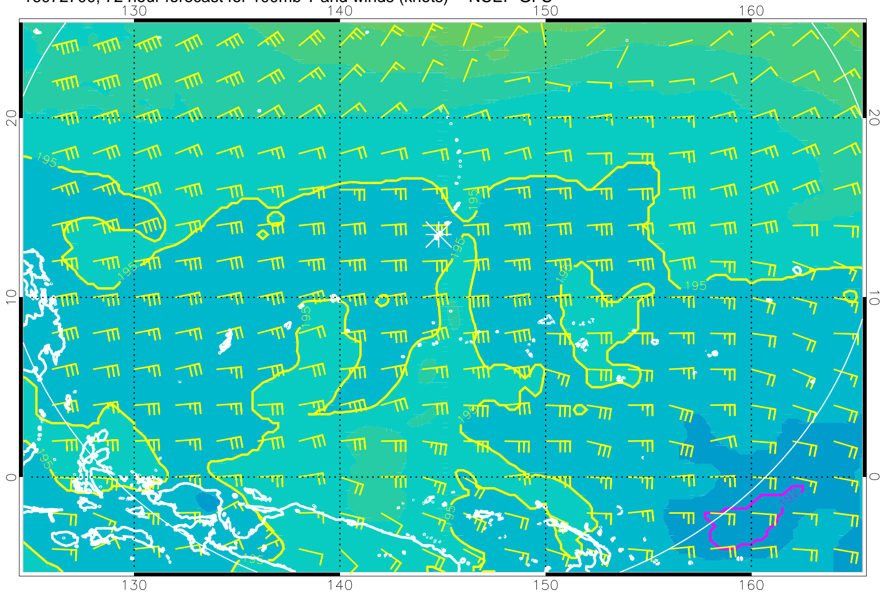
16072700, 72 hour forecast for 100mb T and winds (knots) -- NCEP GFS
