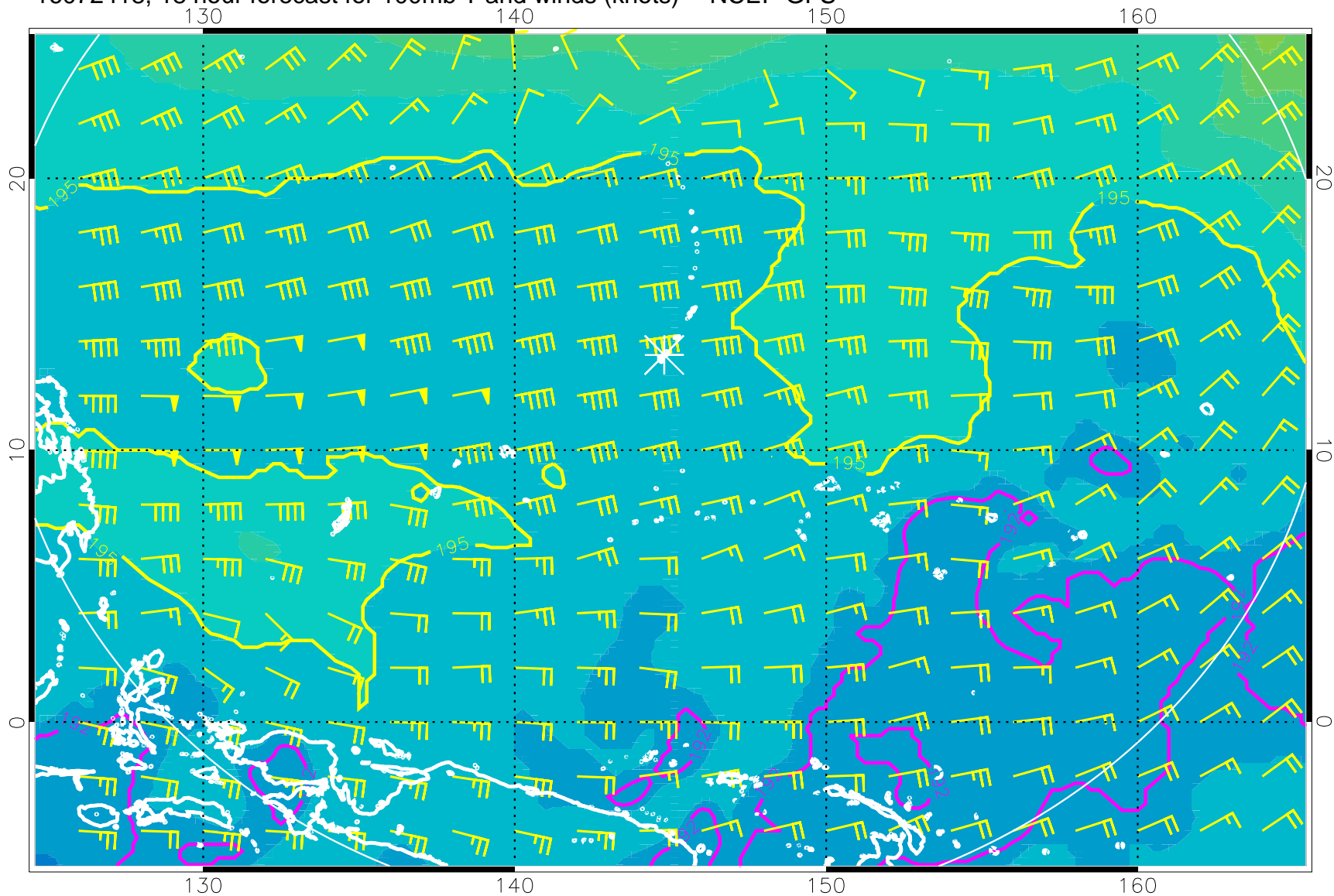
16072418, 18 hour forecast for 100mb T and winds (knots) -- NCEP GFS
