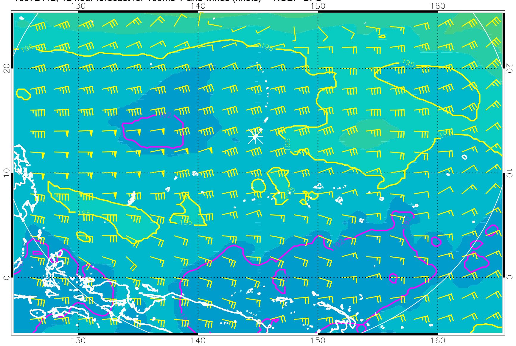
16072412, 12 hour forecast for 100mb T and winds (knots) -- NCEP GFS
