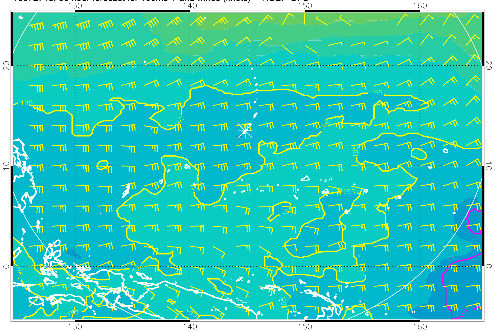
16072718, 90 hour forecast for 100mb T and winds (knots) -- NCEP GFS
