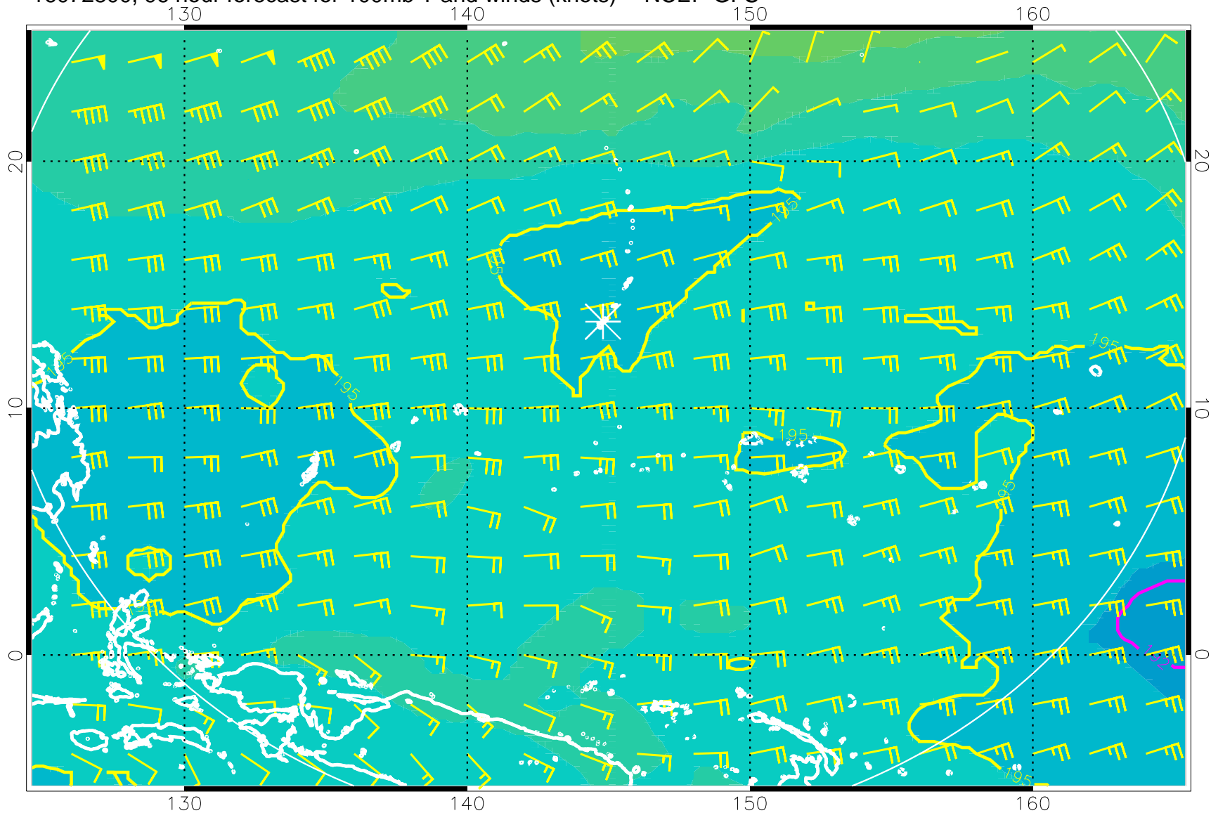
16072800, 96 hour forecast for 100mb T and winds (knots) -- NCEP GFS
