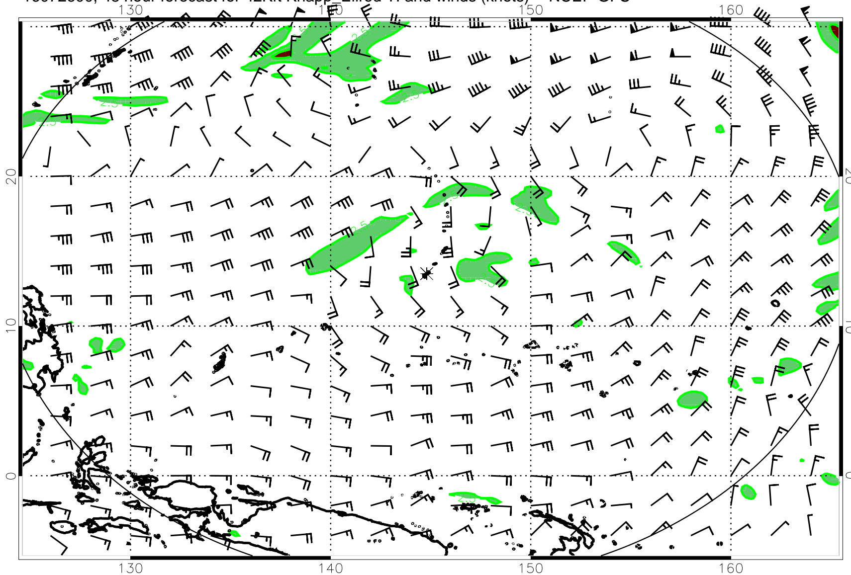
16072600, 48 hour forecast for 42Kft Knapp_Ellrod TI and winds (knots) -- NCEP GFS
