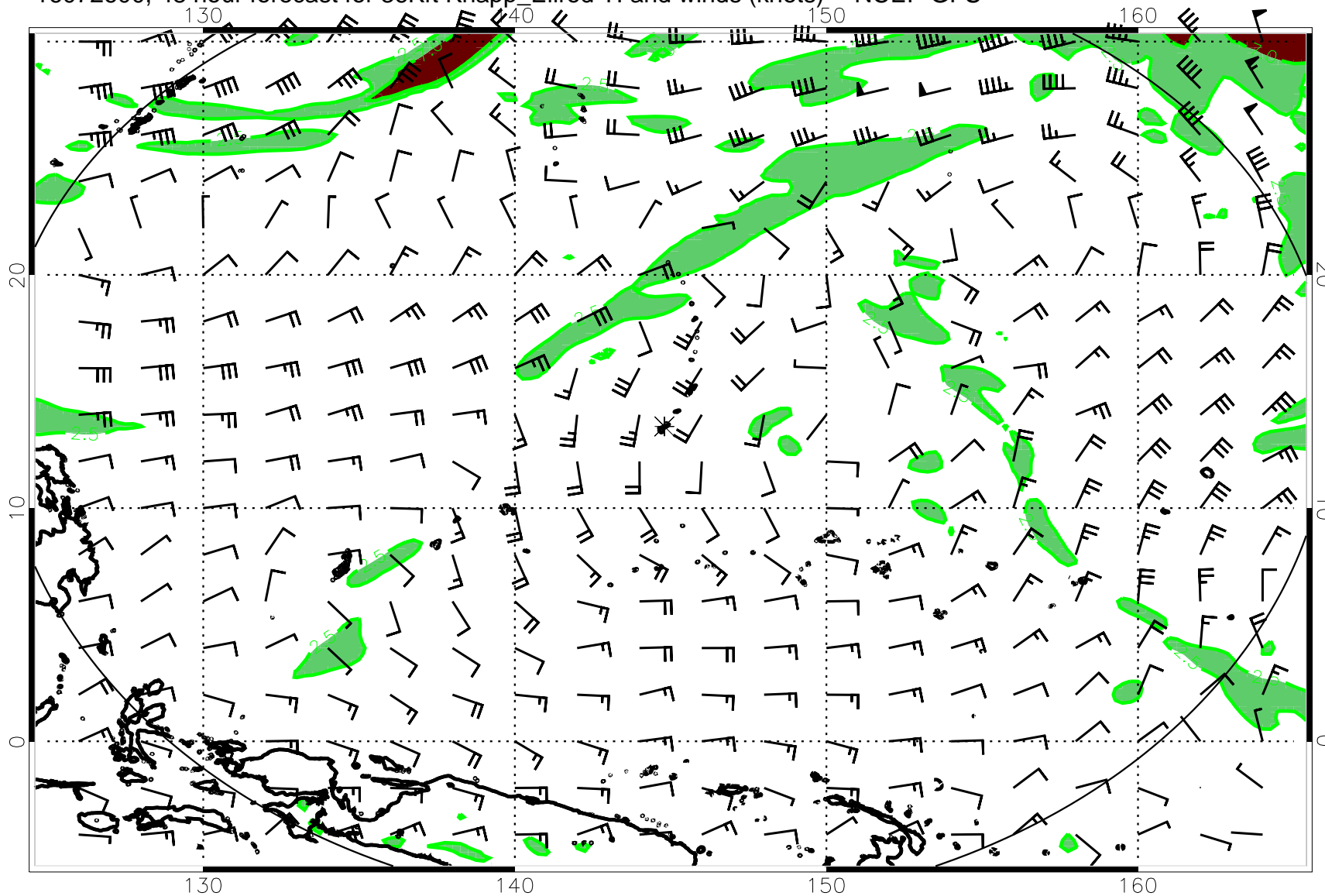
16072600, 48 hour forecast for 36Kft Knapp_Ellrod TI and winds (knots) -- NCEP GFS
