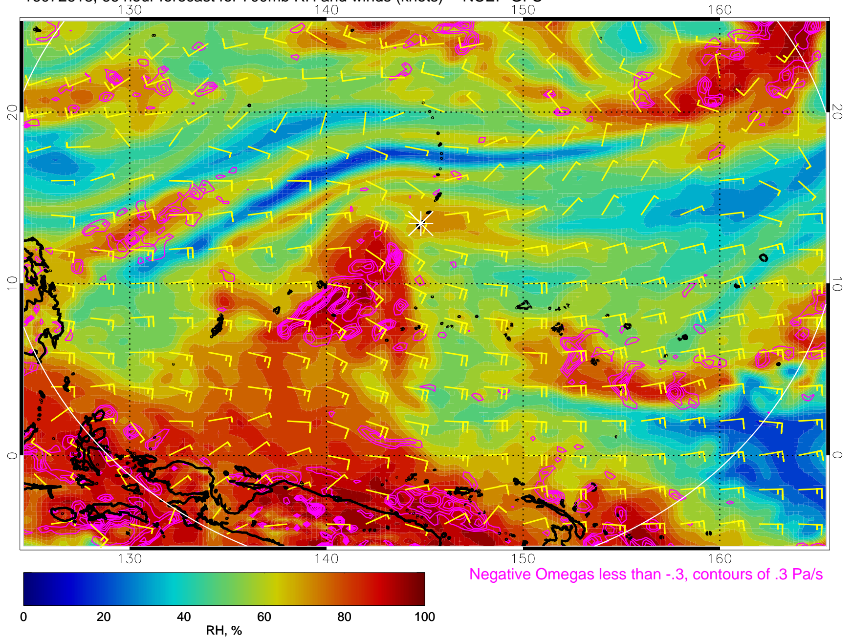
16072618, 66 hour forecast for 700mb RH and winds (knots) -- NCEP GFS
