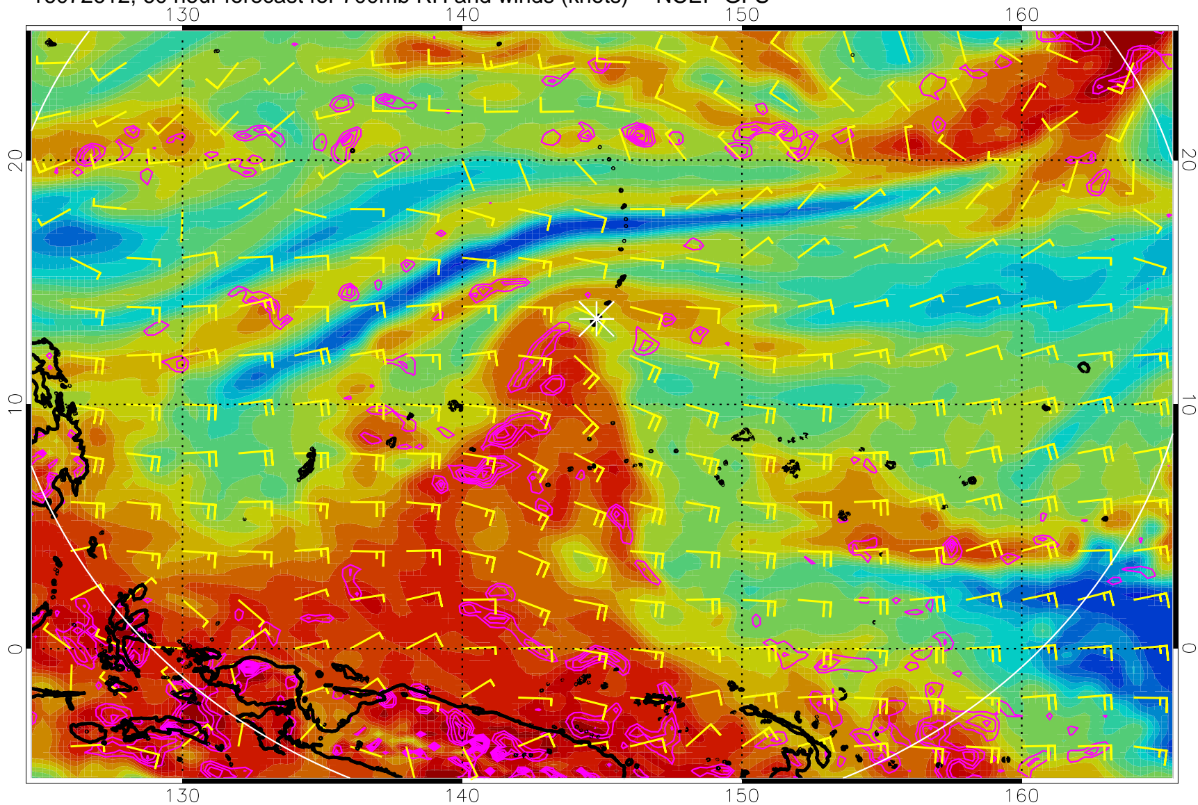
16072612, 60 hour forecast for 700mb RH and winds (knots) -- NCEP GFS
