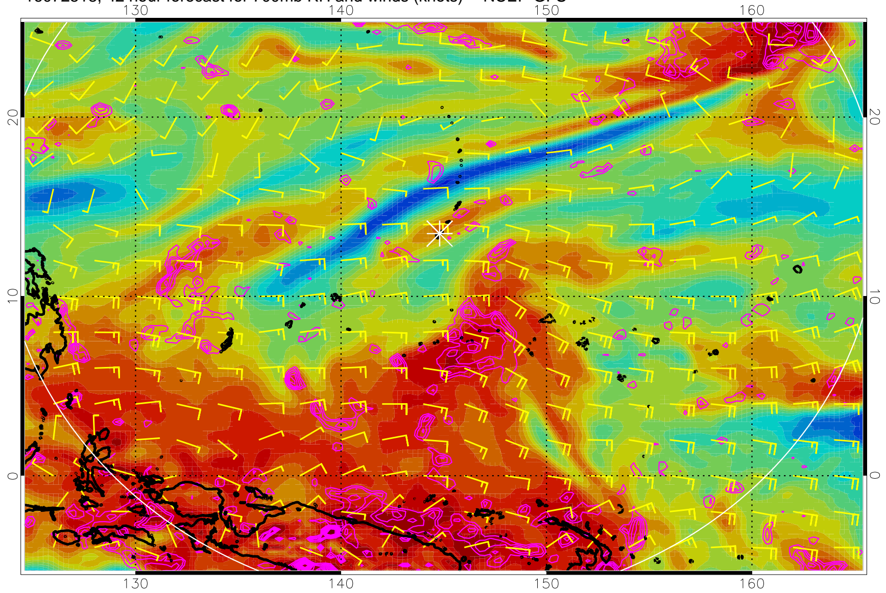
16072518, 42 hour forecast for 700mb RH and winds (knots) -- NCEP GFS
