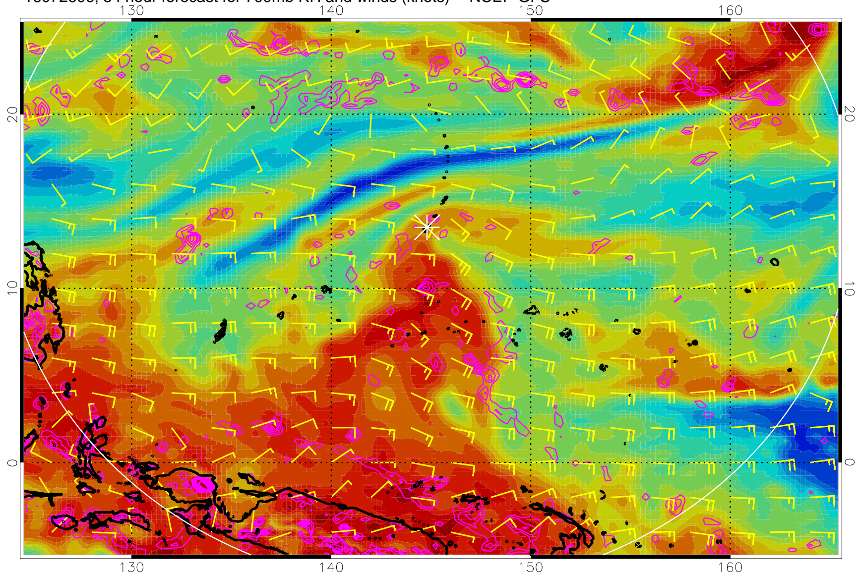
16072606, 54 hour forecast for 700mb RH and winds (knots) -- NCEP GFS
