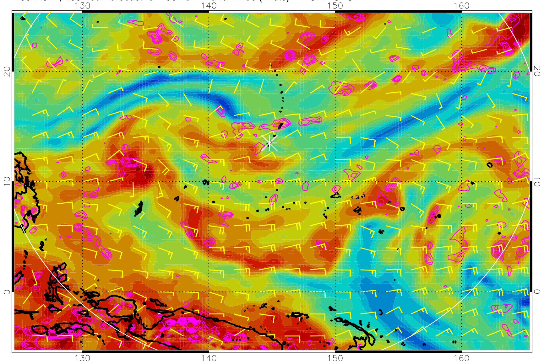
16072812, 108 hour forecast for 700mb RH and winds (knots) -- NCEP GFS
