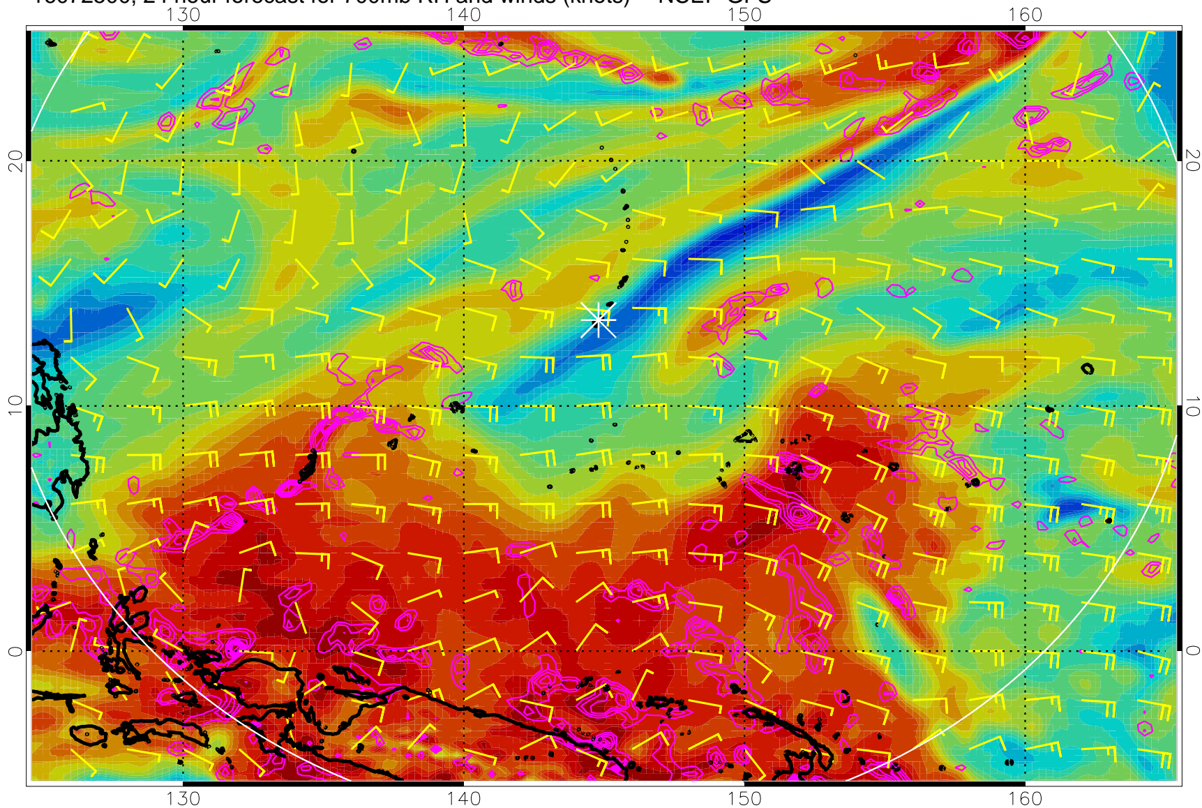
16072500, 24 hour forecast for 700mb RH and winds (knots) -- NCEP GFS
