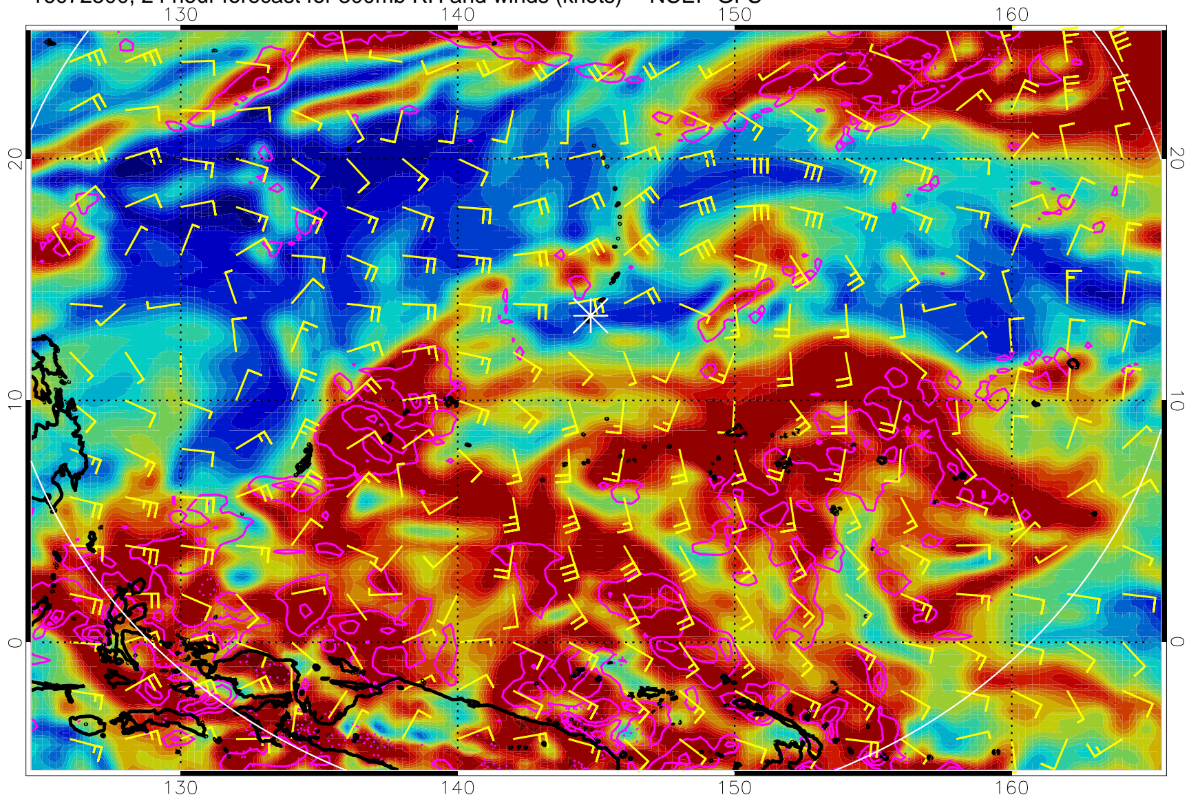
16072500, 24 hour forecast for 300mb RH and winds (knots) -- NCEP GFS
