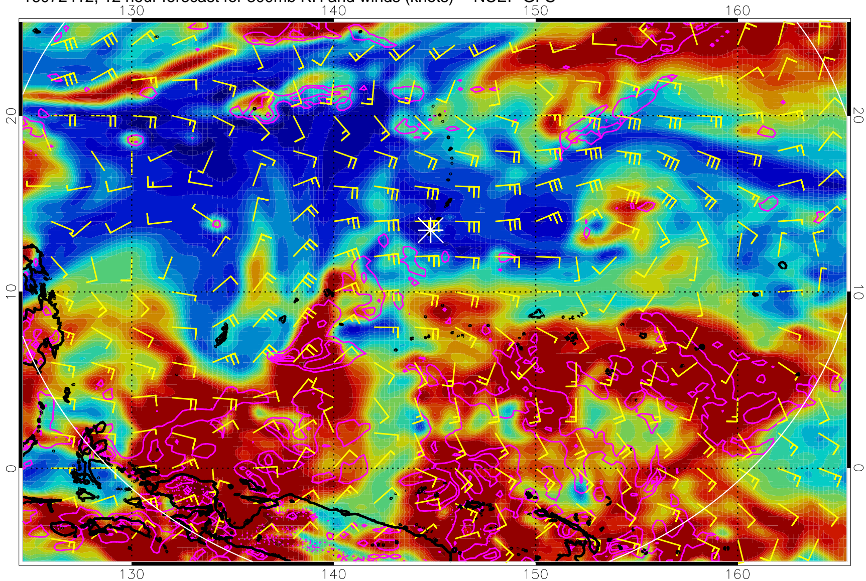
16072412, 12 hour forecast for 300mb RH and winds (knots) -- NCEP GFS
