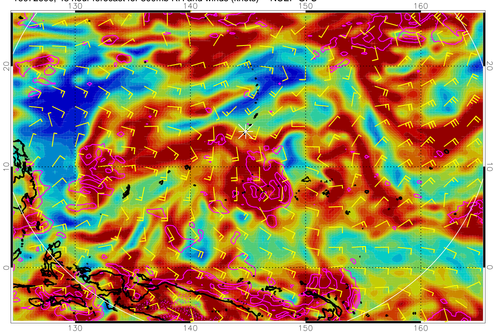
16072600, 48 hour forecast for 300mb RH and winds (knots) -- NCEP GFS
