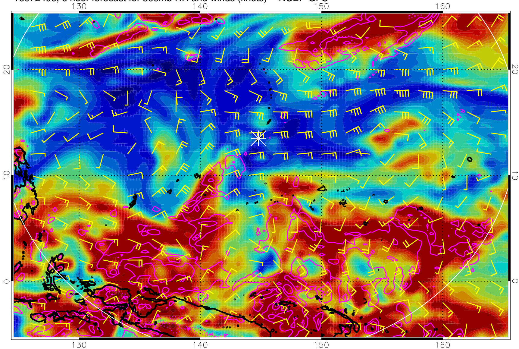
16072406, 6 hour forecast for 300mb RH and winds (knots) -- NCEP GFS
