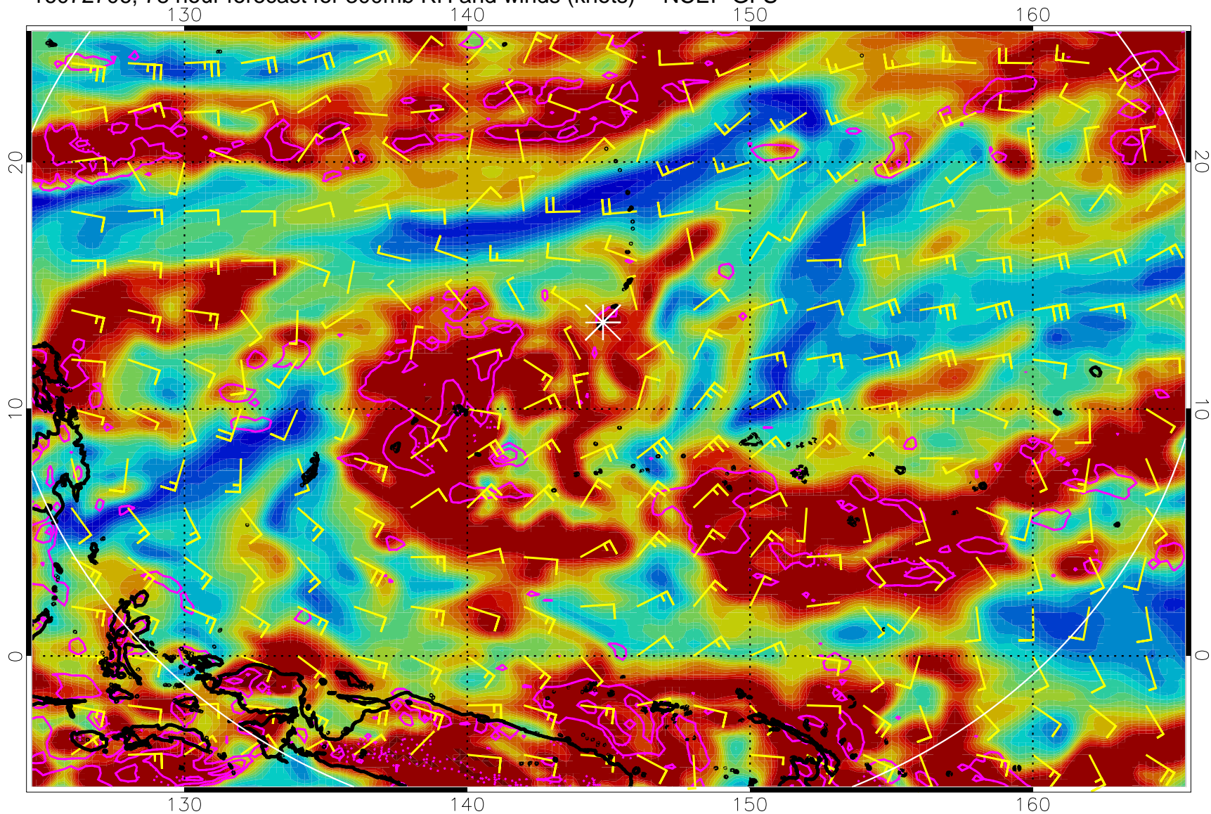
16072706, 78 hour forecast for 300mb RH and winds (knots) -- NCEP GFS
