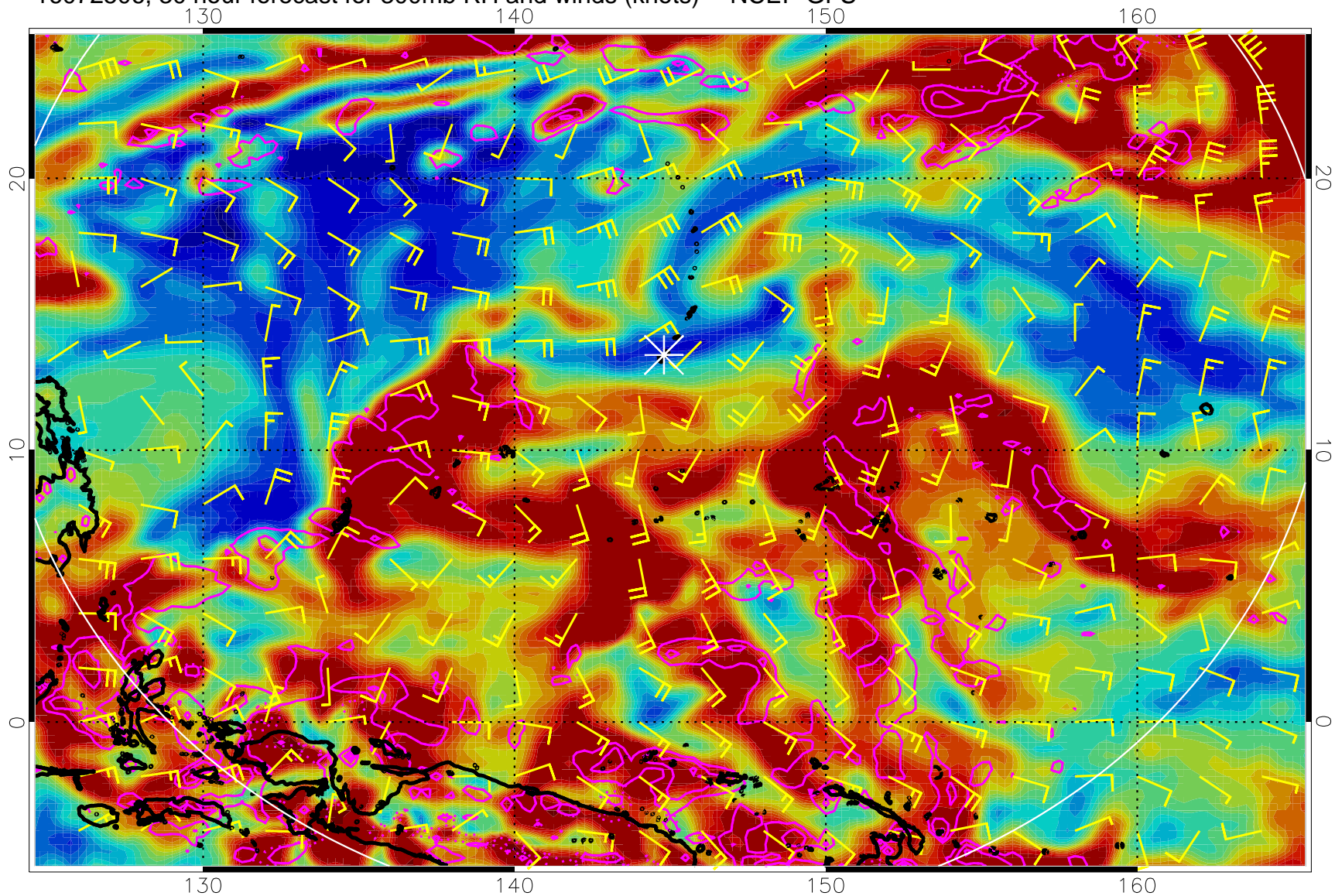
16072506, 30 hour forecast for 300mb RH and winds (knots) -- NCEP GFS
