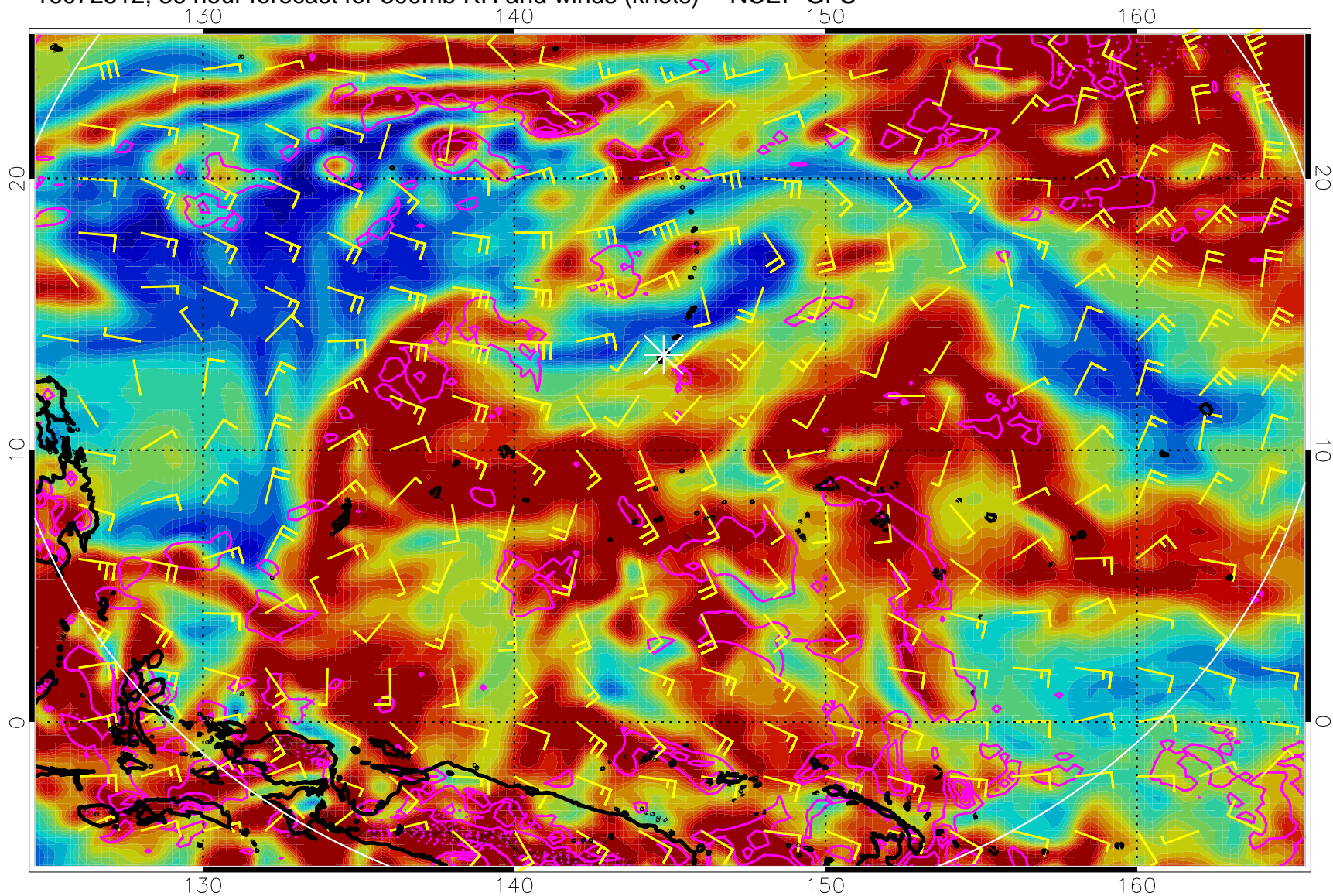
16072512, 36 hour forecast for 300mb RH and winds (knots) -- NCEP GFS
