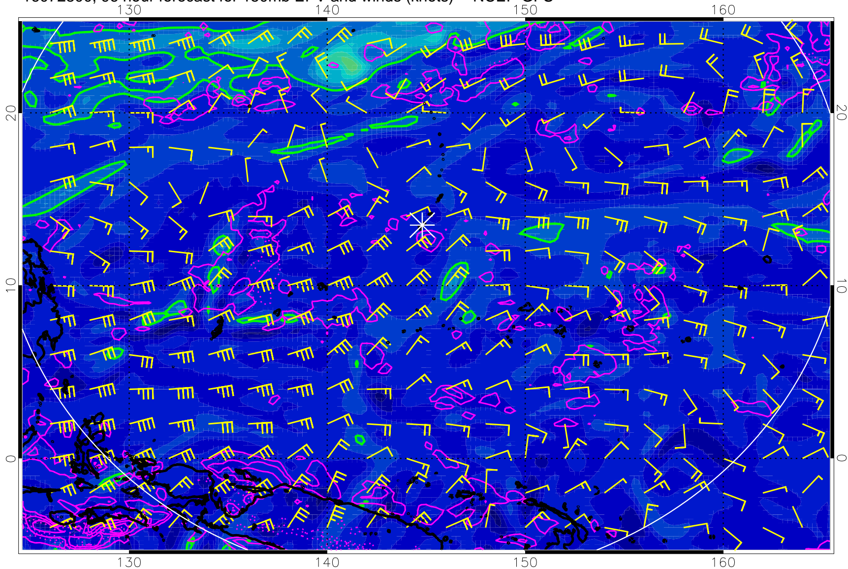
16072800, 96 hour forecast for 150mb EPV and winds (knots) -- NCEP GFS
