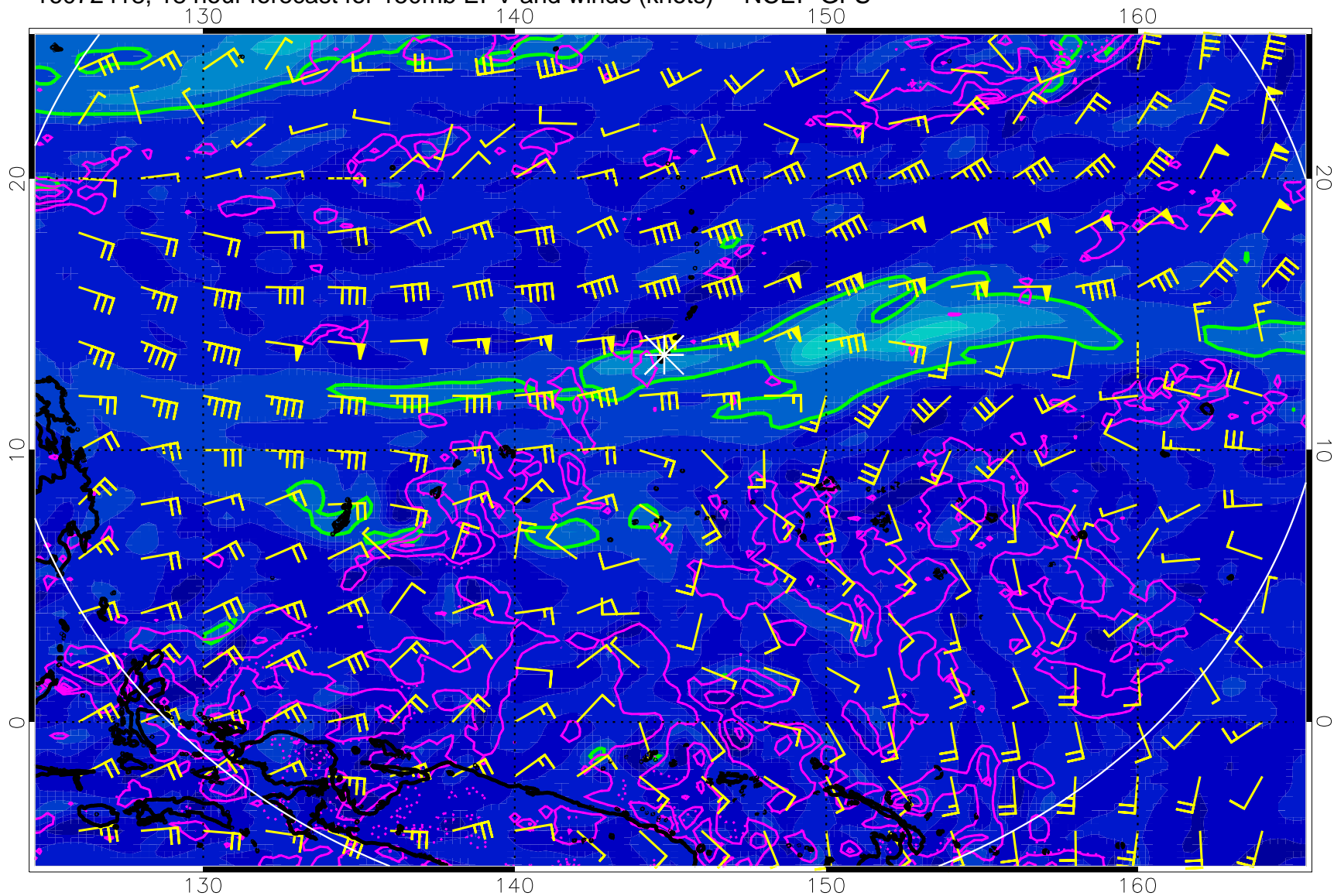
16072418, 18 hour forecast for 150mb EPV and winds (knots) -- NCEP GFS
