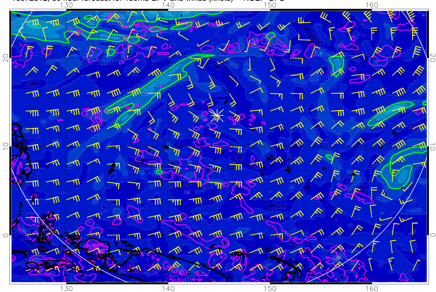
16072612, 60 hour forecast for 150mb EPV and winds (knots) -- NCEP GFS
