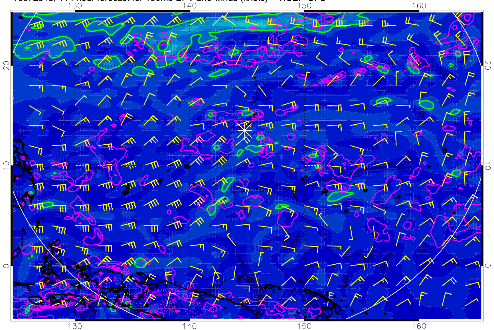
16072818, 114 hour forecast for 150mb EPV and winds (knots) -- NCEP GFS
