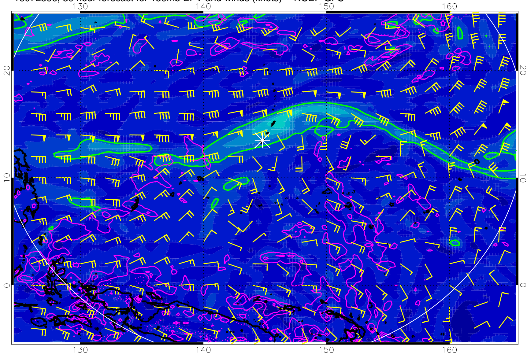
16072506, 30 hour forecast for 150mb EPV and winds (knots) -- NCEP GFS
