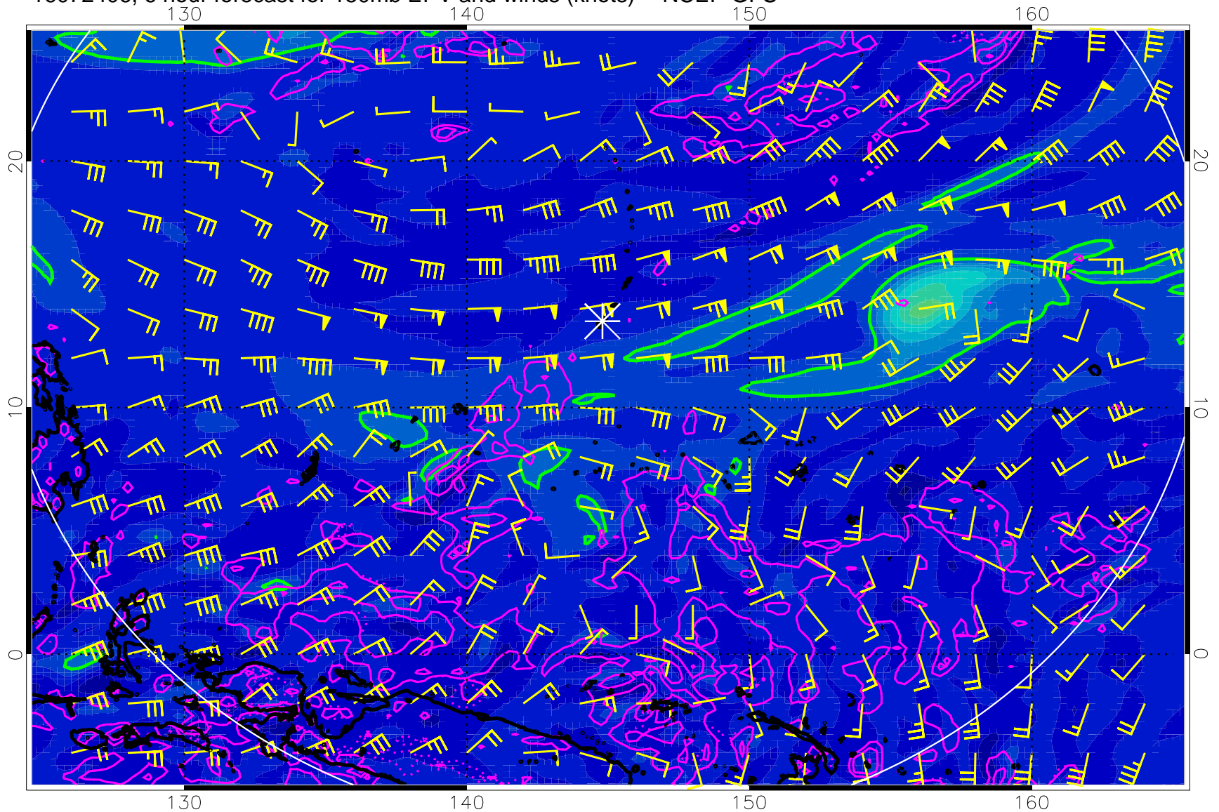
16072406, 6 hour forecast for 150mb EPV and winds (knots) -- NCEP GFS
