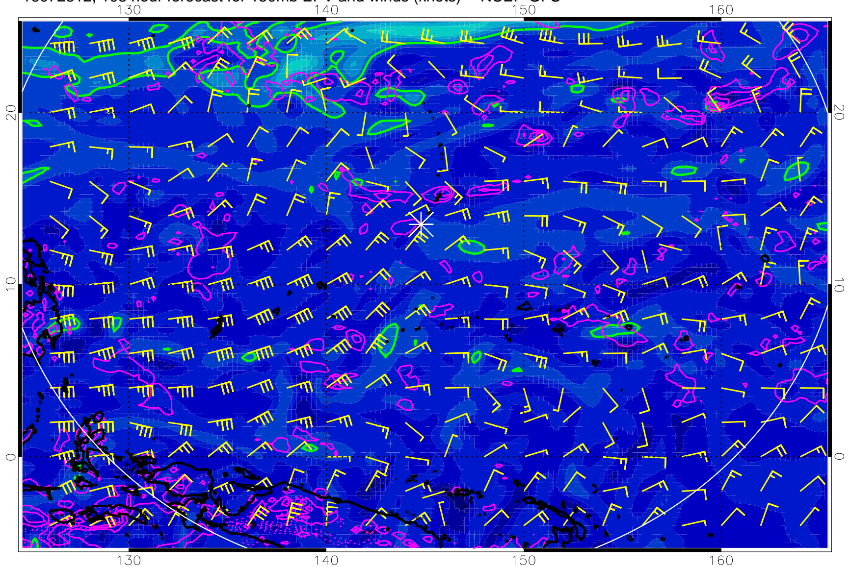
16072812, 108 hour forecast for 150mb EPV and winds (knots) -- NCEP GFS
