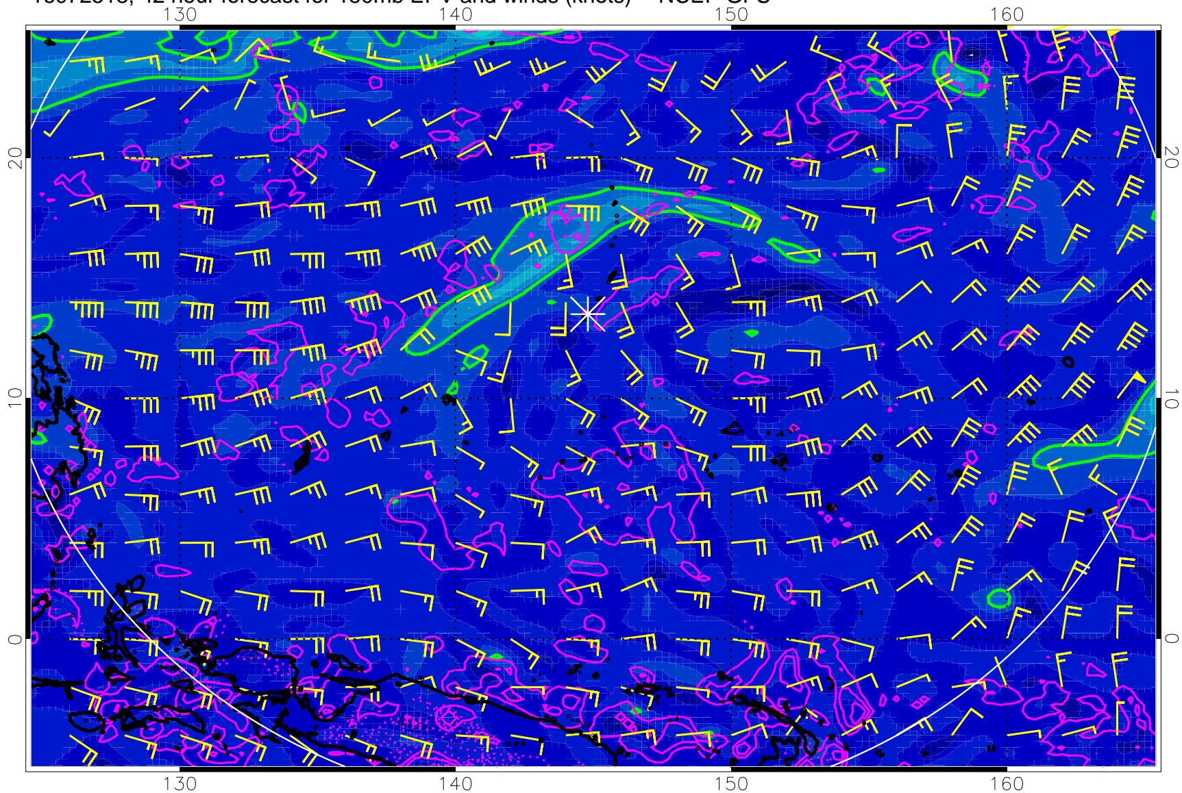
16072518, 42 hour forecast for 150mb EPV and winds (knots) -- NCEP GFS
