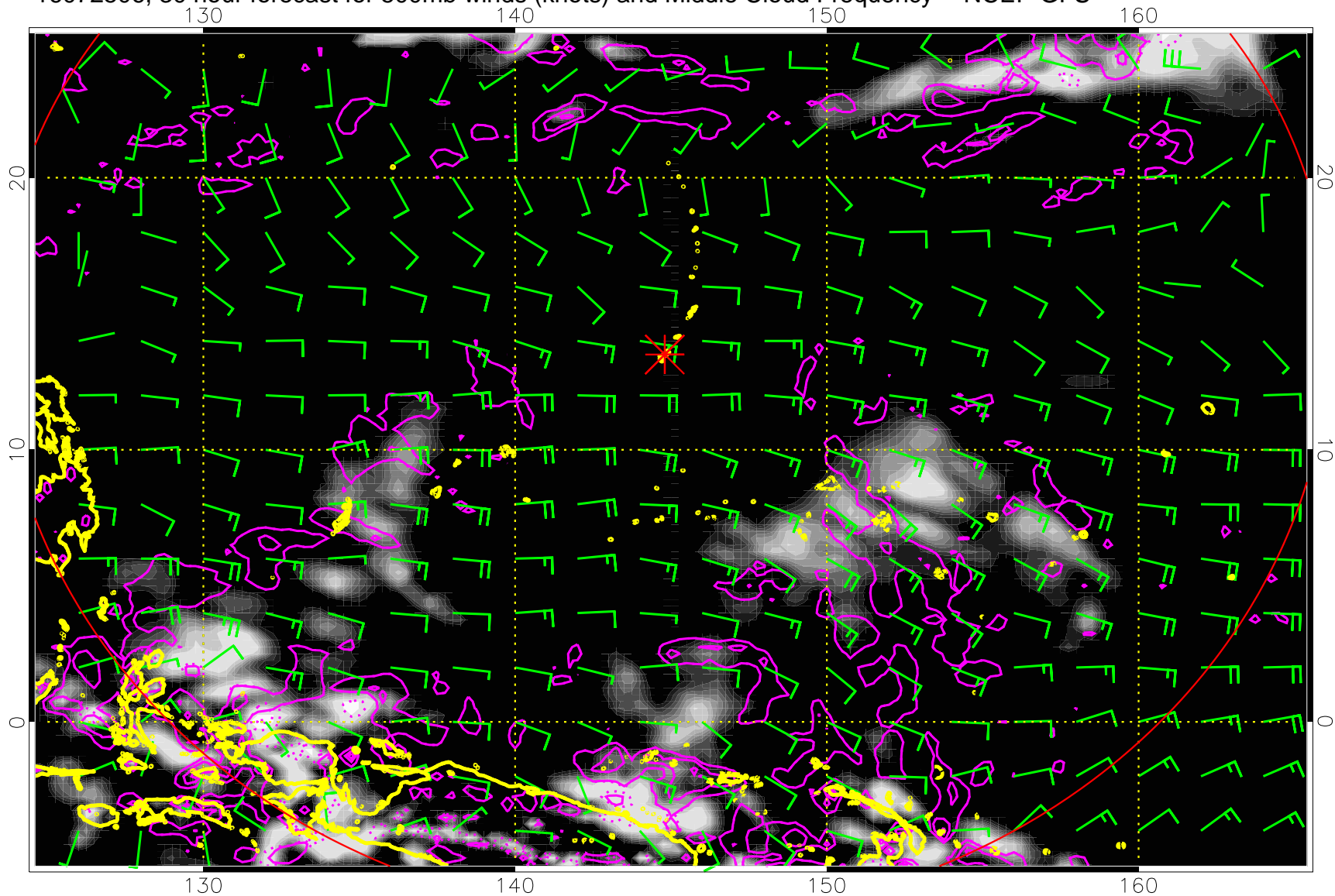
16072506, 30 hour forecast for 500mb winds (knots) and Middle Cloud Frequency -- NCEP GFS
