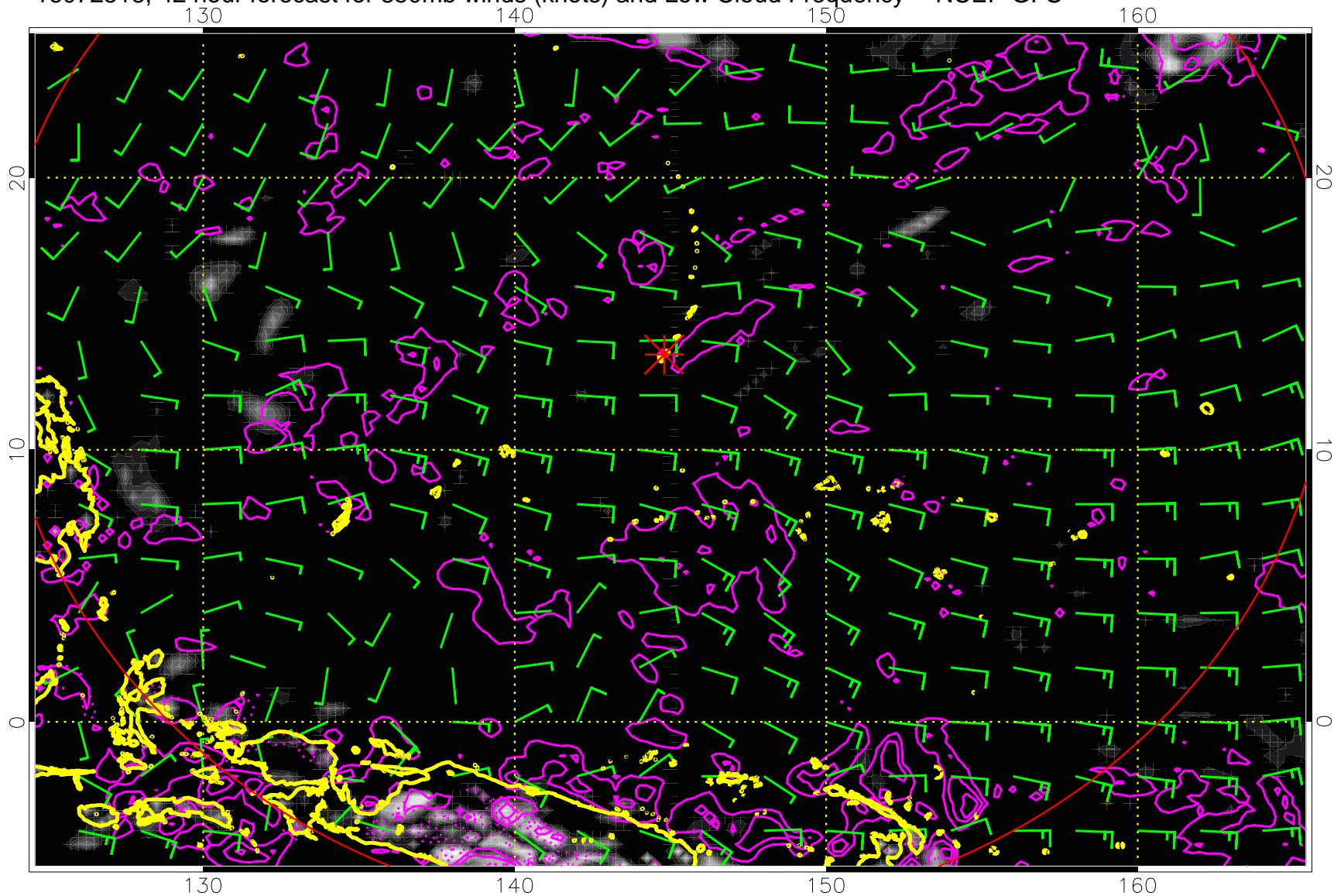
16072518, 42 hour forecast for 850mb winds (knots) and Low Cloud Frequency -- NCEP GFS
