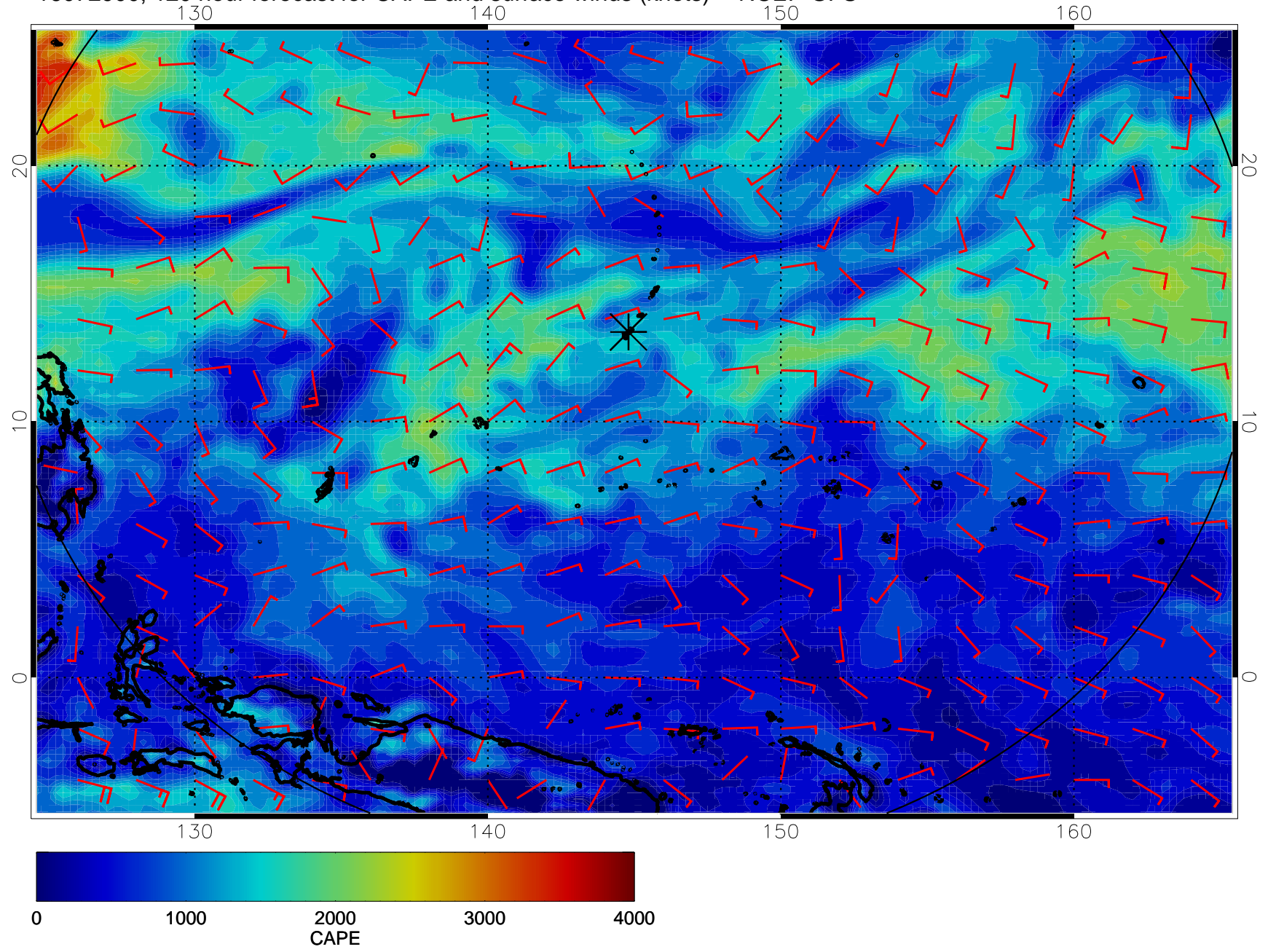
16072900, 120 hour forecast for CAPE and surface winds (knots) -- NCEP GFS
