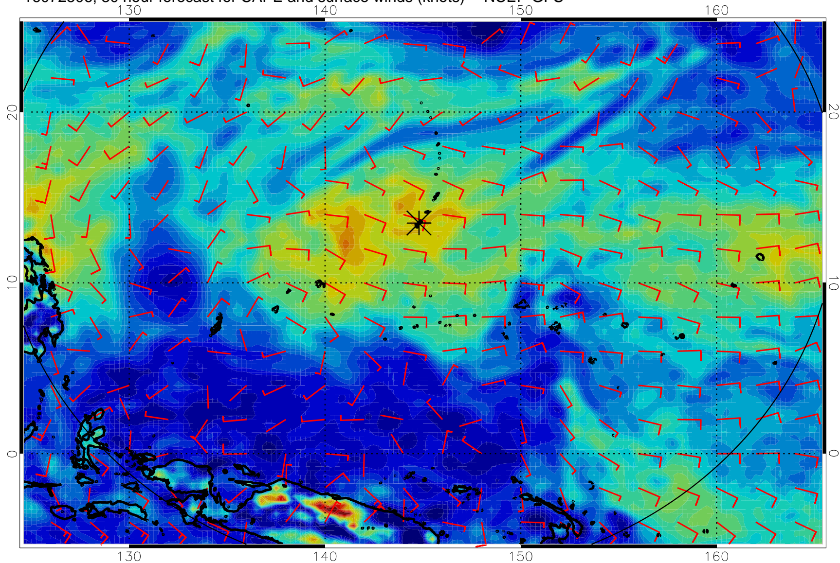
16072506, 30 hour forecast for CAPE and surface winds (knots) -- NCEP GFS
