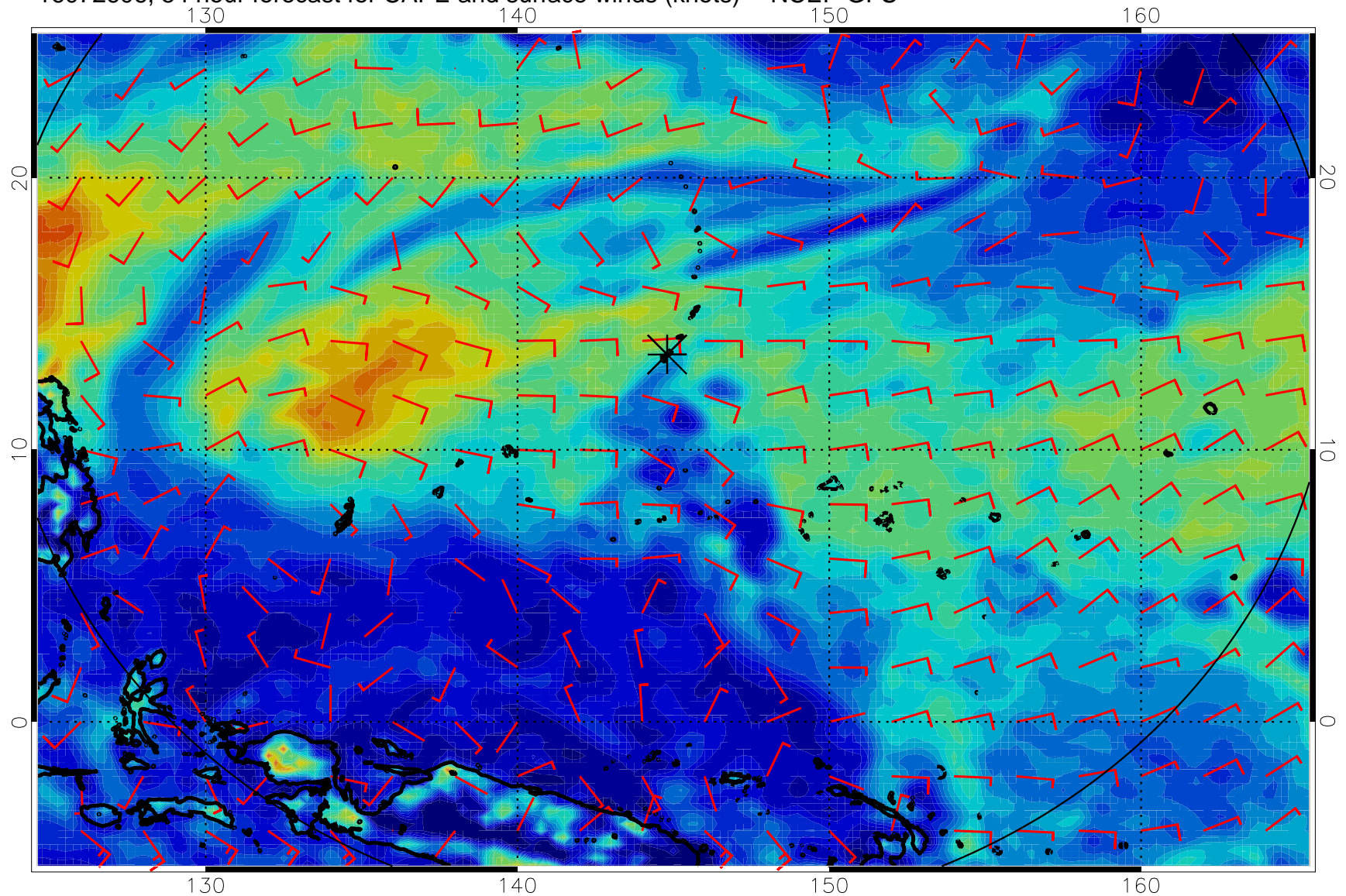
16072606, 54 hour forecast for CAPE and surface winds (knots) -- NCEP GFS
