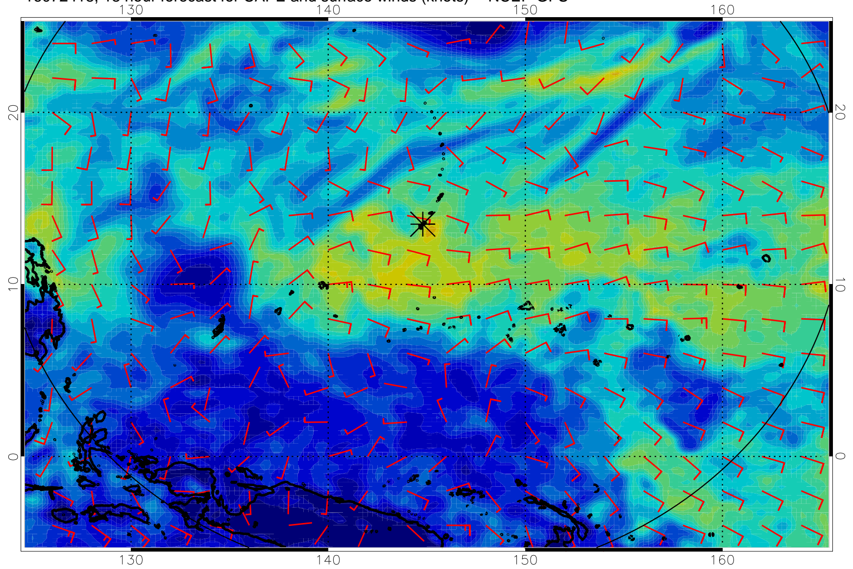
16072418, 18 hour forecast for CAPE and surface winds (knots) -- NCEP GFS
