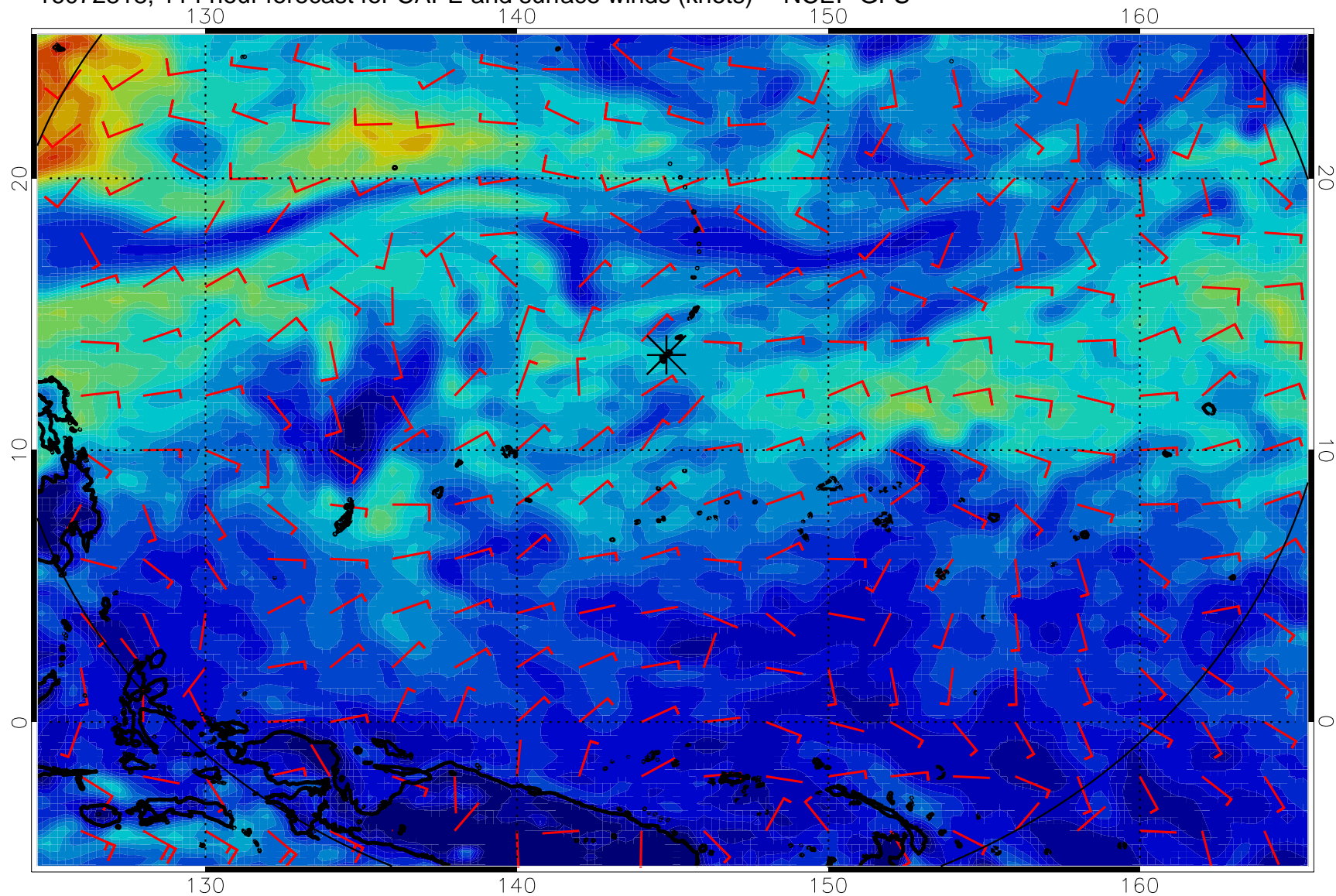
16072818, 114 hour forecast for CAPE and surface winds (knots) -- NCEP GFS
