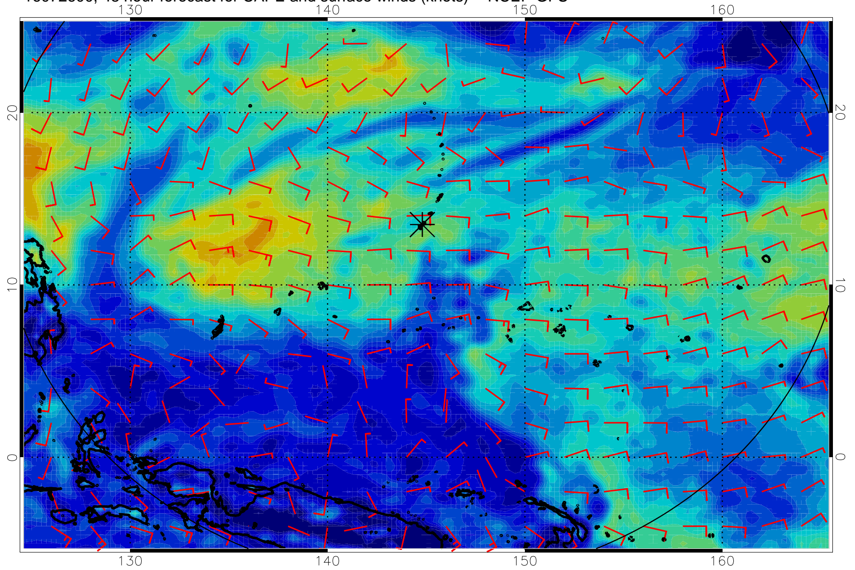
16072600, 48 hour forecast for CAPE and surface winds (knots) -- NCEP GFS
