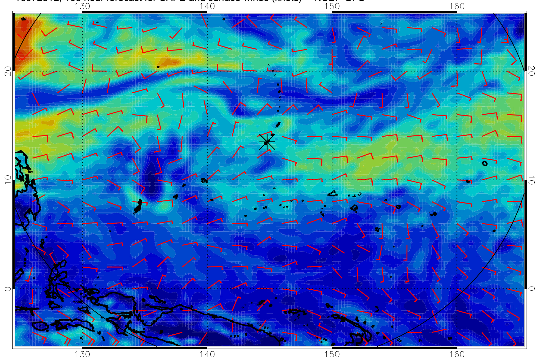
16072812, 108 hour forecast for CAPE and surface winds (knots) -- NCEP GFS
