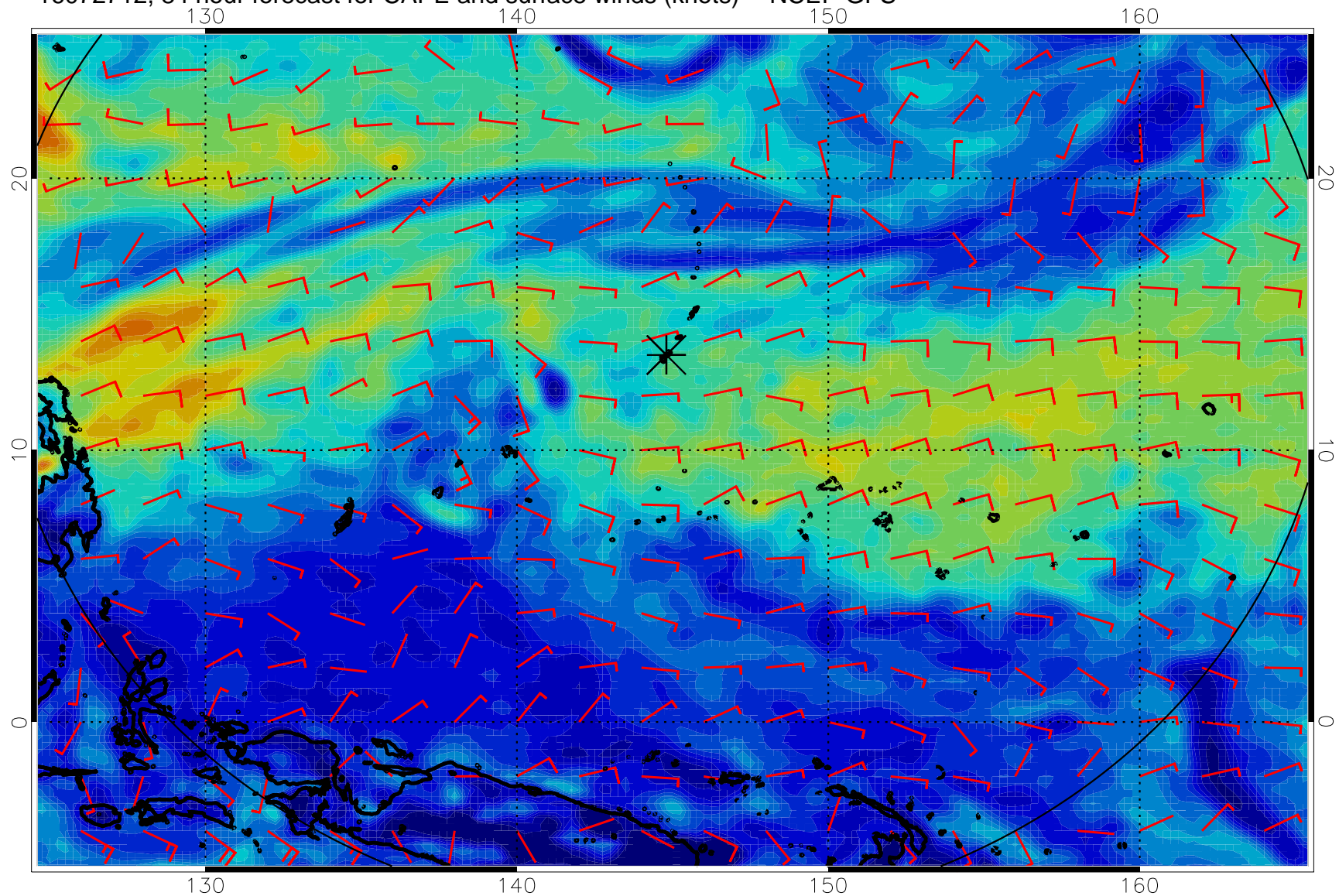
16072712, 84 hour forecast for CAPE and surface winds (knots) -- NCEP GFS
