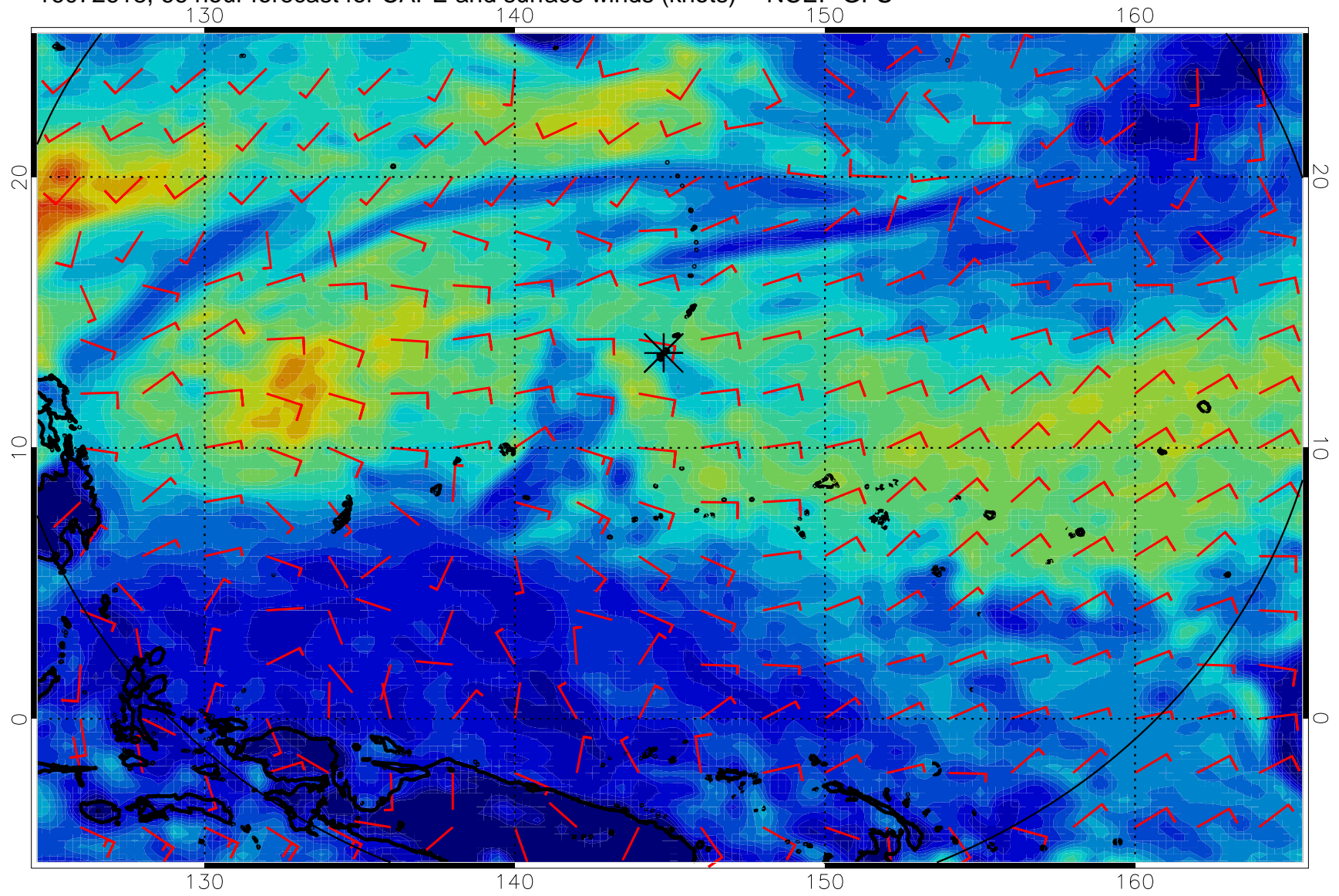
16072618, 66 hour forecast for CAPE and surface winds (knots) -- NCEP GFS
