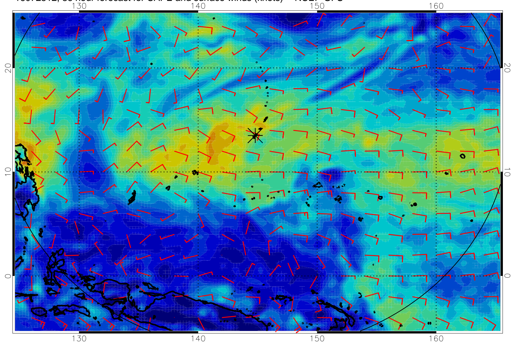
16072512, 36 hour forecast for CAPE and surface winds (knots) -- NCEP GFS
