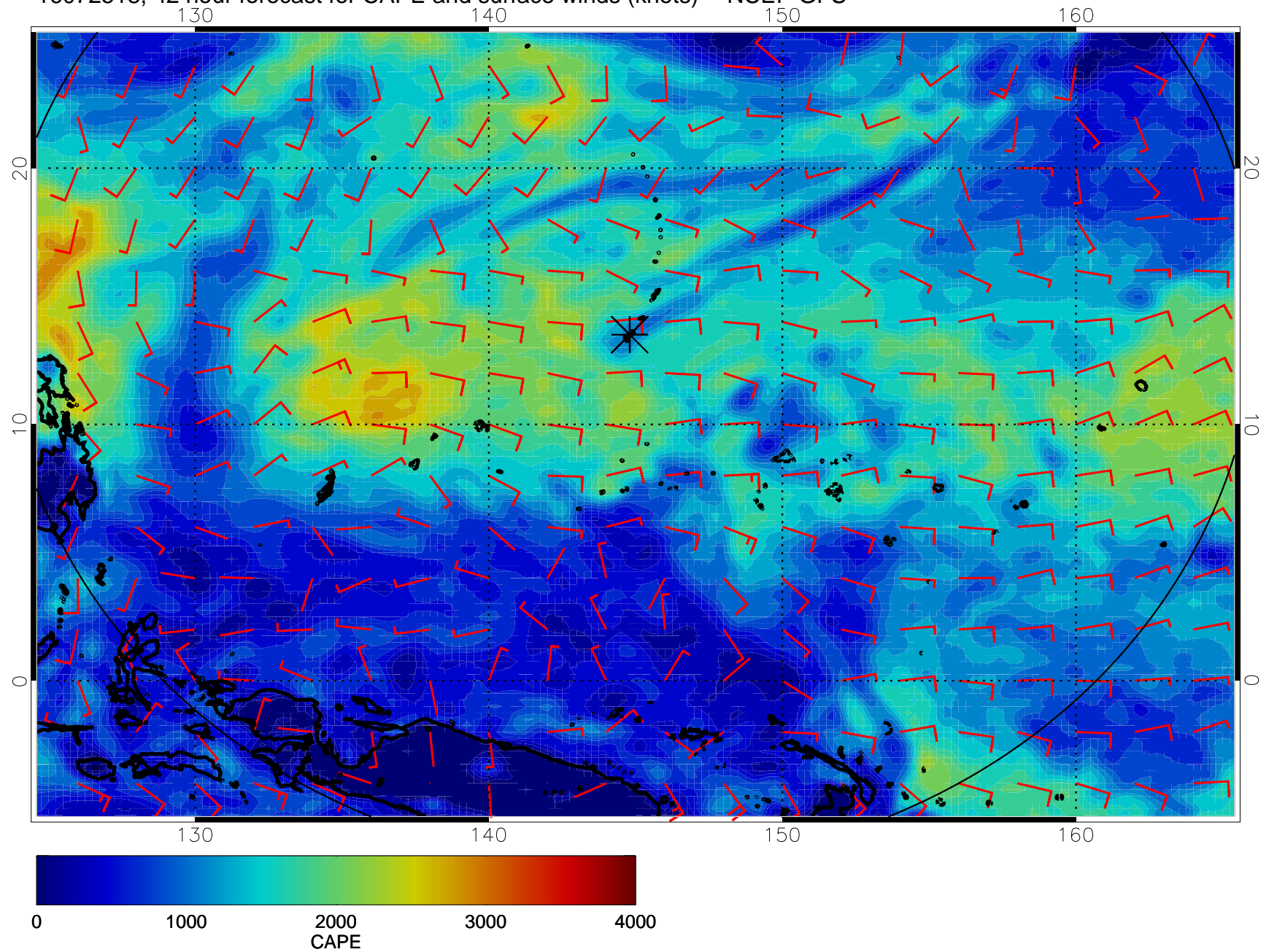
16072518, 42 hour forecast for CAPE and surface winds (knots) -- NCEP GFS
