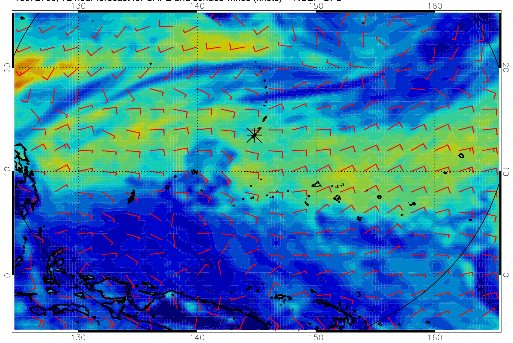
16072700, 72 hour forecast for CAPE and surface winds (knots) -- NCEP GFS
