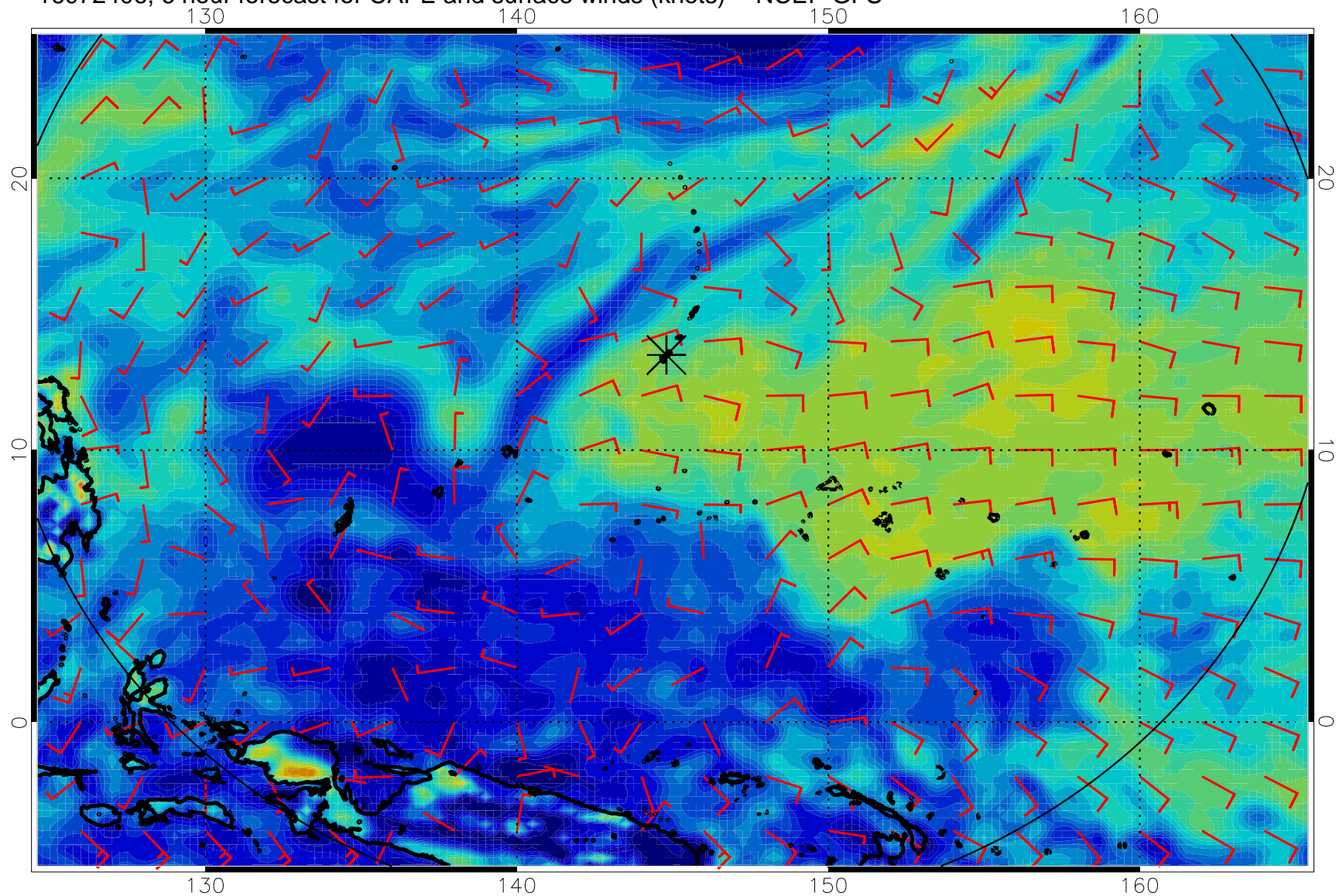
16072406, 6 hour forecast for CAPE and surface winds (knots) -- NCEP GFS
