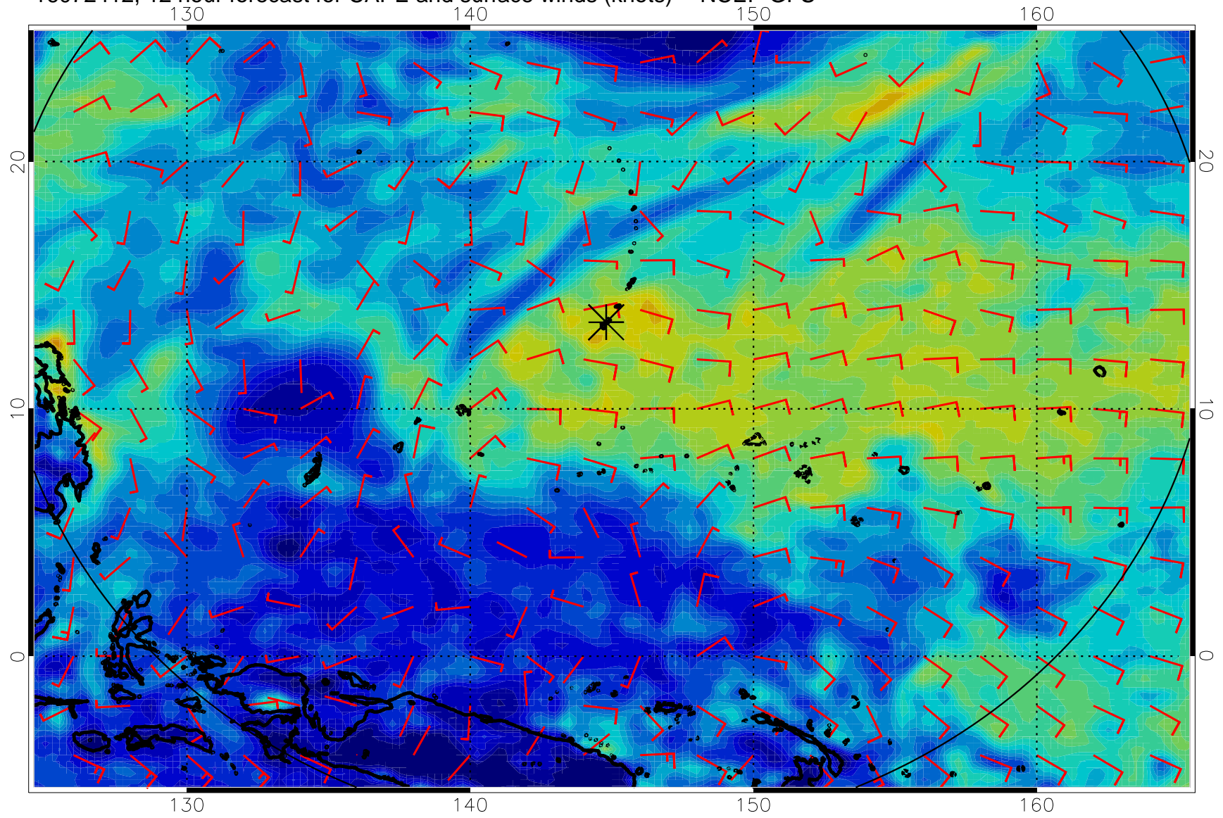
16072412, 12 hour forecast for CAPE and surface winds (knots) -- NCEP GFS
