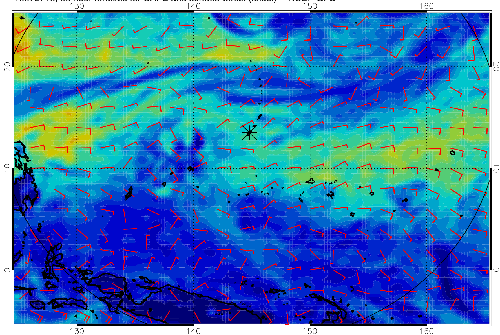
16072718, 90 hour forecast for CAPE and surface winds (knots) -- NCEP GFS
