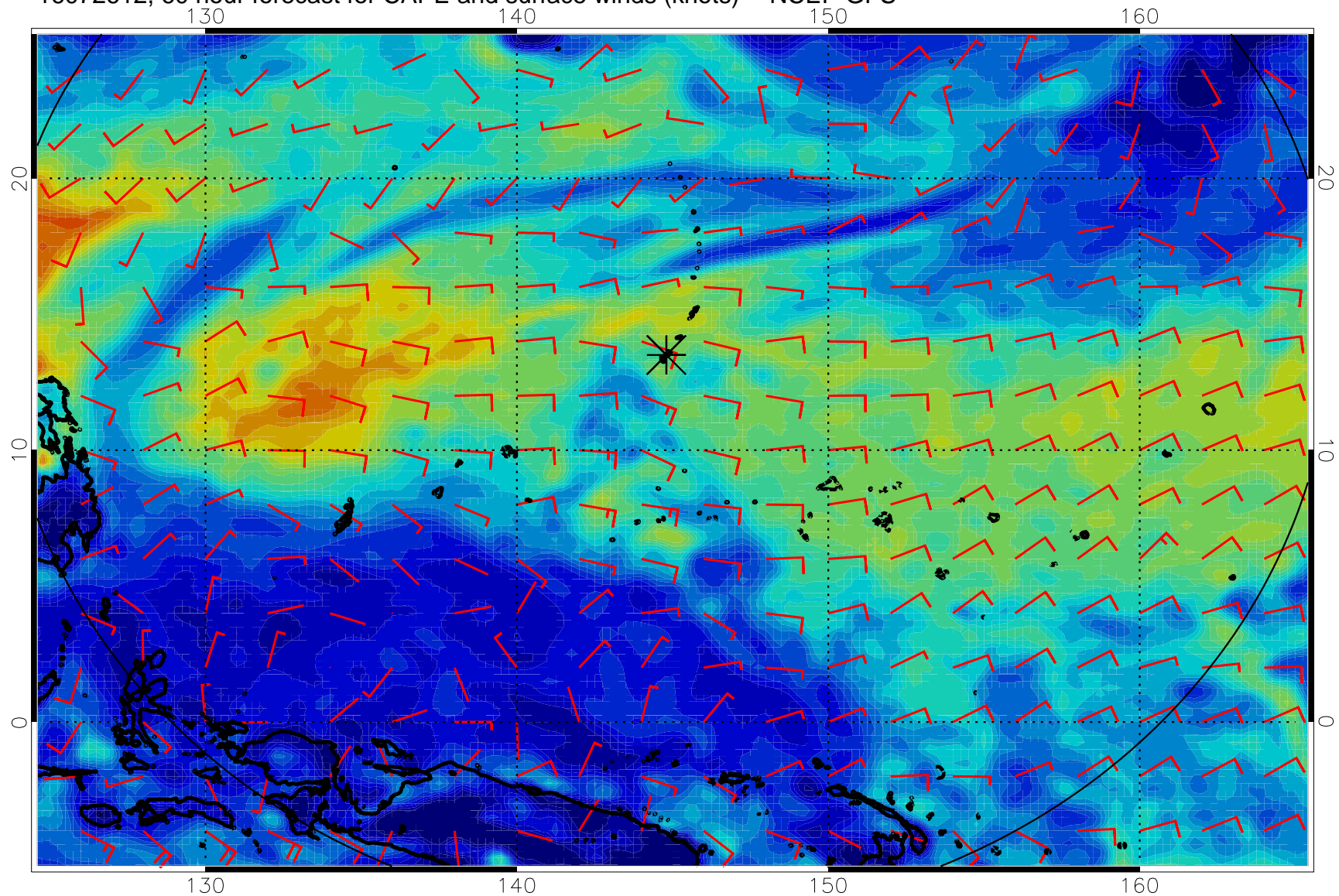
16072612, 60 hour forecast for CAPE and surface winds (knots) -- NCEP GFS
