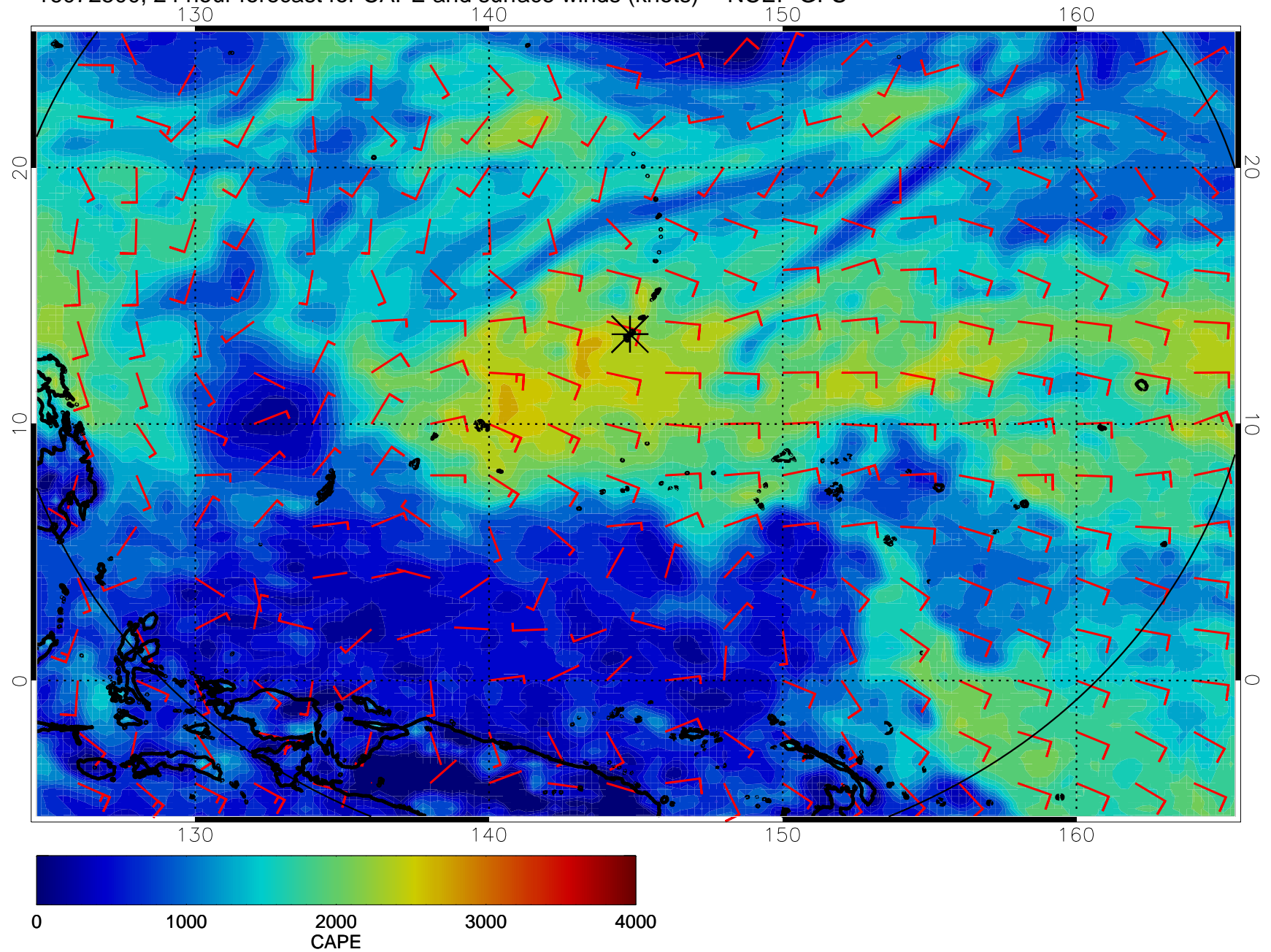
16072500, 24 hour forecast for CAPE and surface winds (knots) -- NCEP GFS
