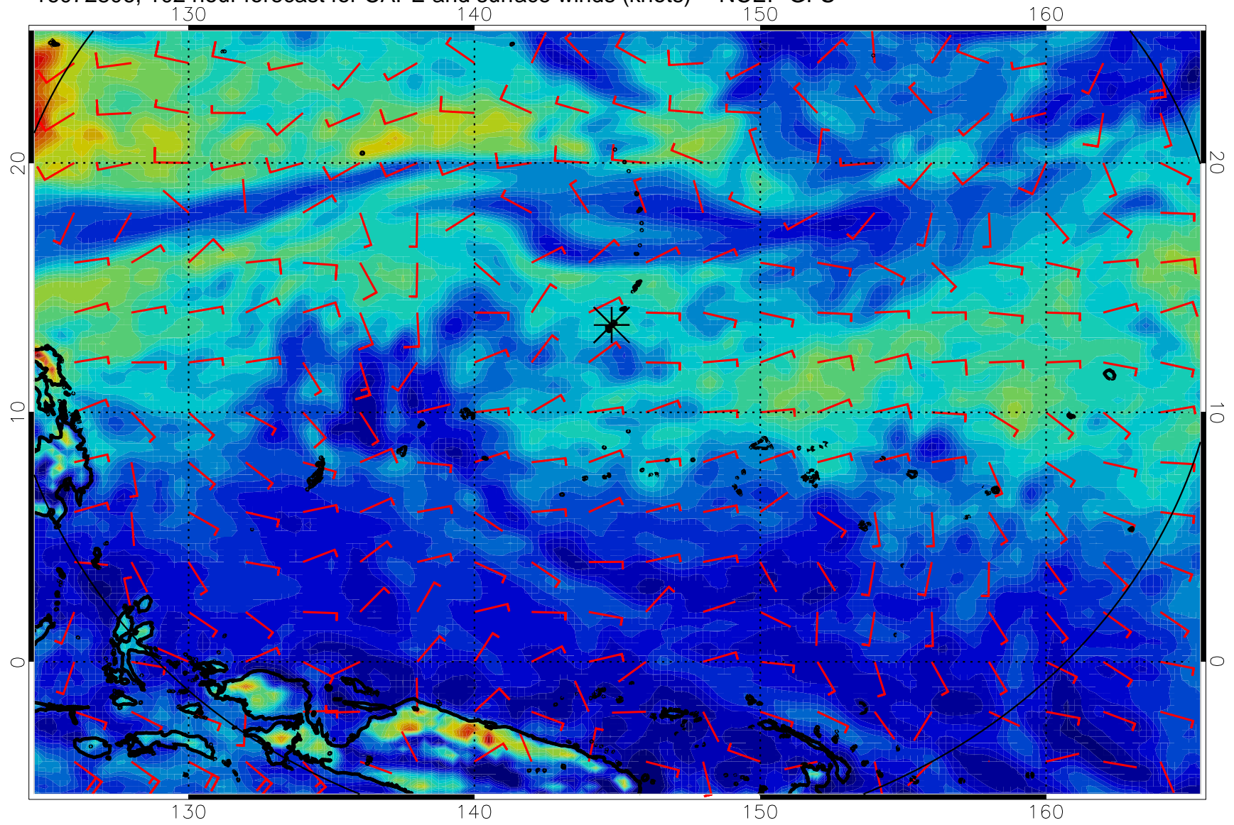
16072806, 102 hour forecast for CAPE and surface winds (knots) -- NCEP GFS
