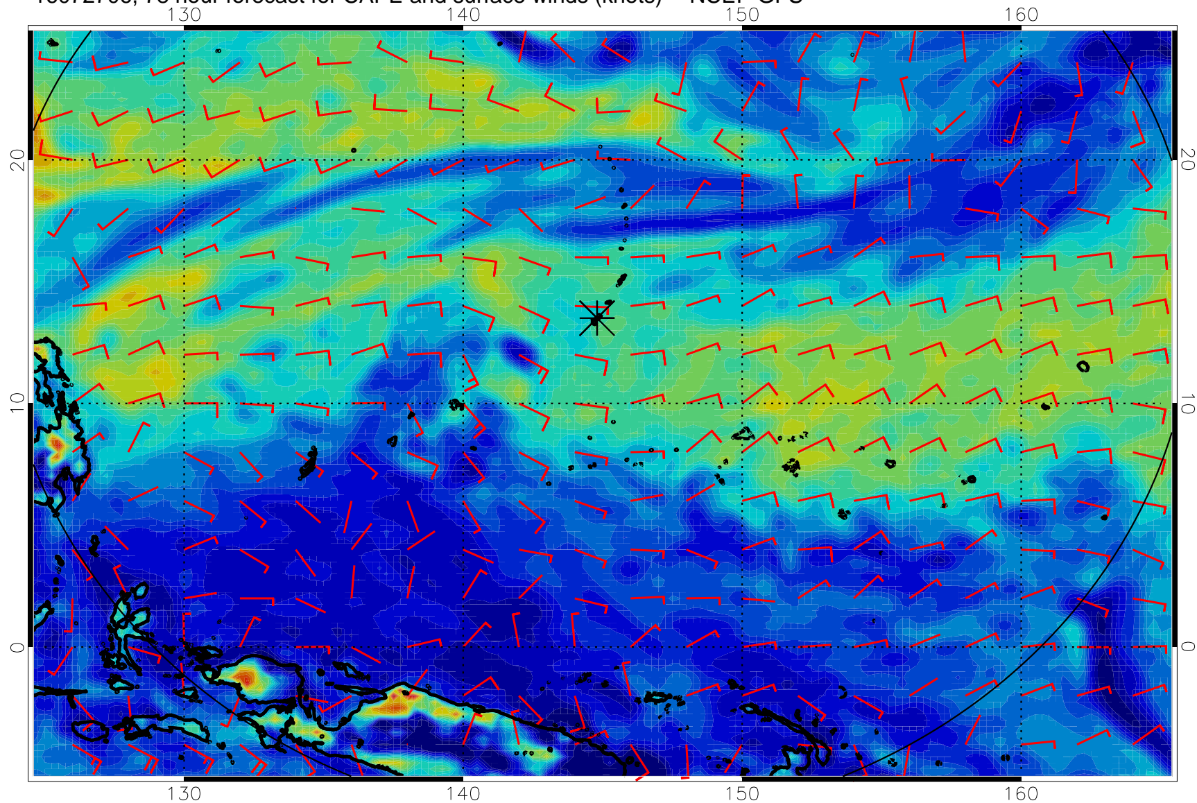
16072706, 78 hour forecast for CAPE and surface winds (knots) -- NCEP GFS
