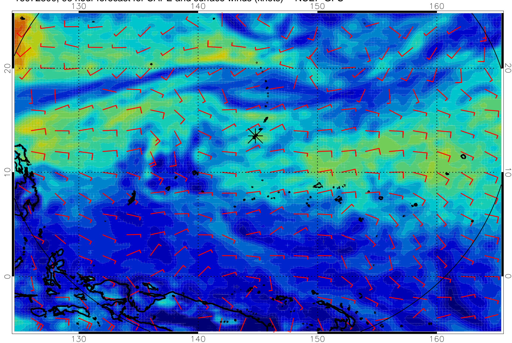
16072800, 96 hour forecast for CAPE and surface winds (knots) -- NCEP GFS
