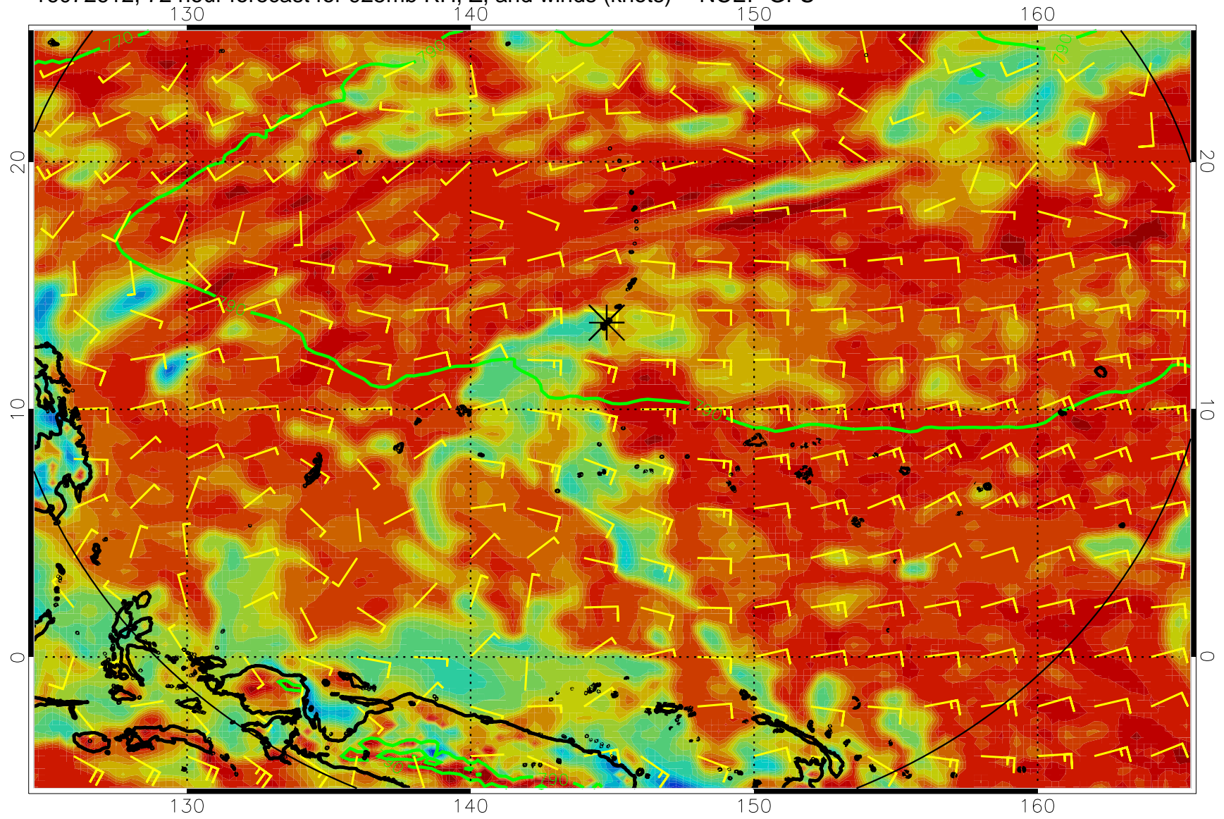
16072612, 72 hour forecast for 925mb RH, Z, and winds (knots) -- NCEP GFS
