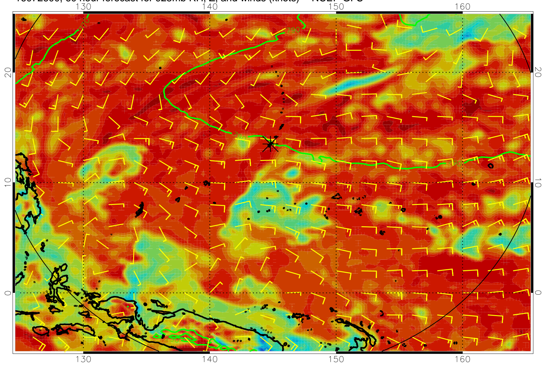
16072600, 60 hour forecast for 925mb RH, Z, and winds (knots) -- NCEP GFS
