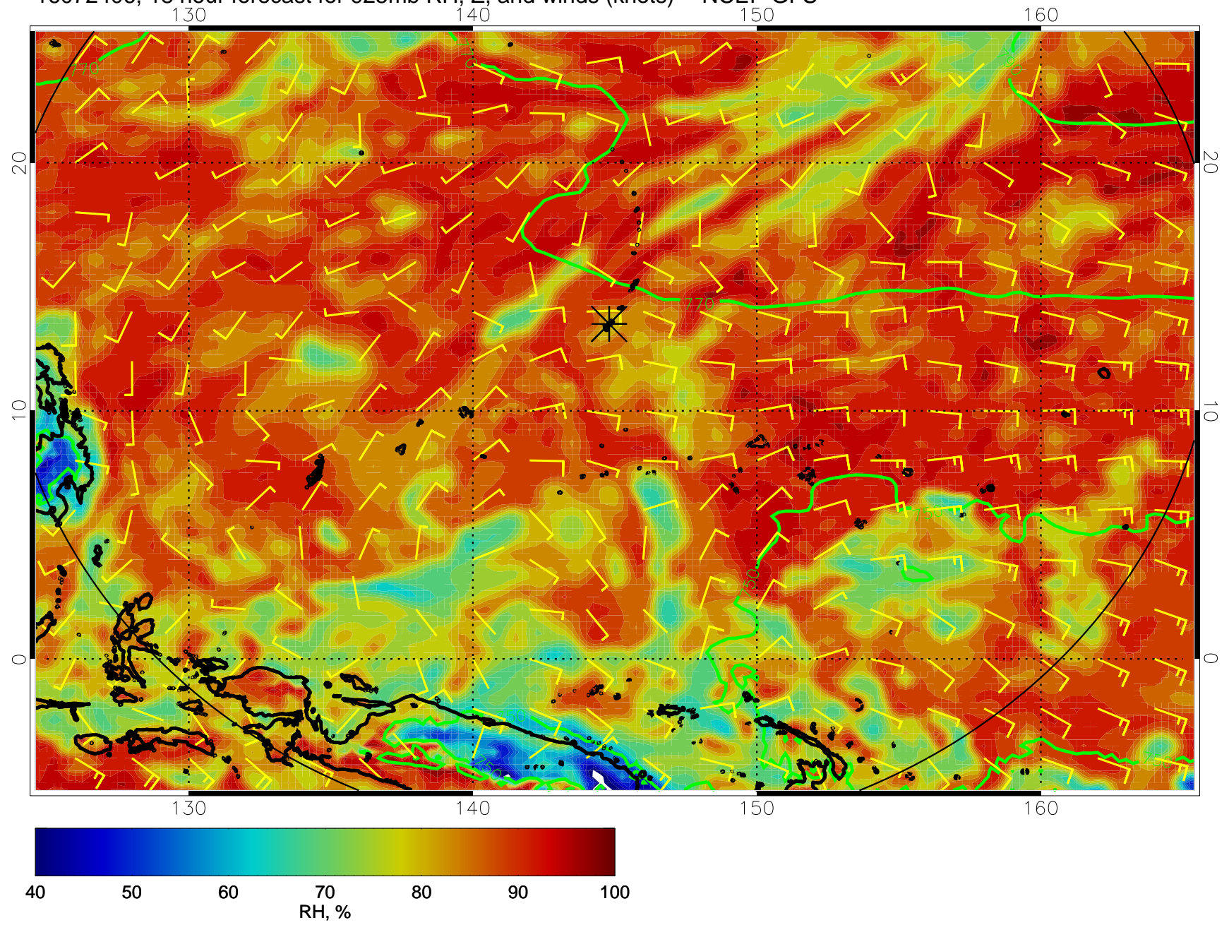
16072406, 18 hour forecast for 925mb RH, Z, and winds (knots) -- NCEP GFS
