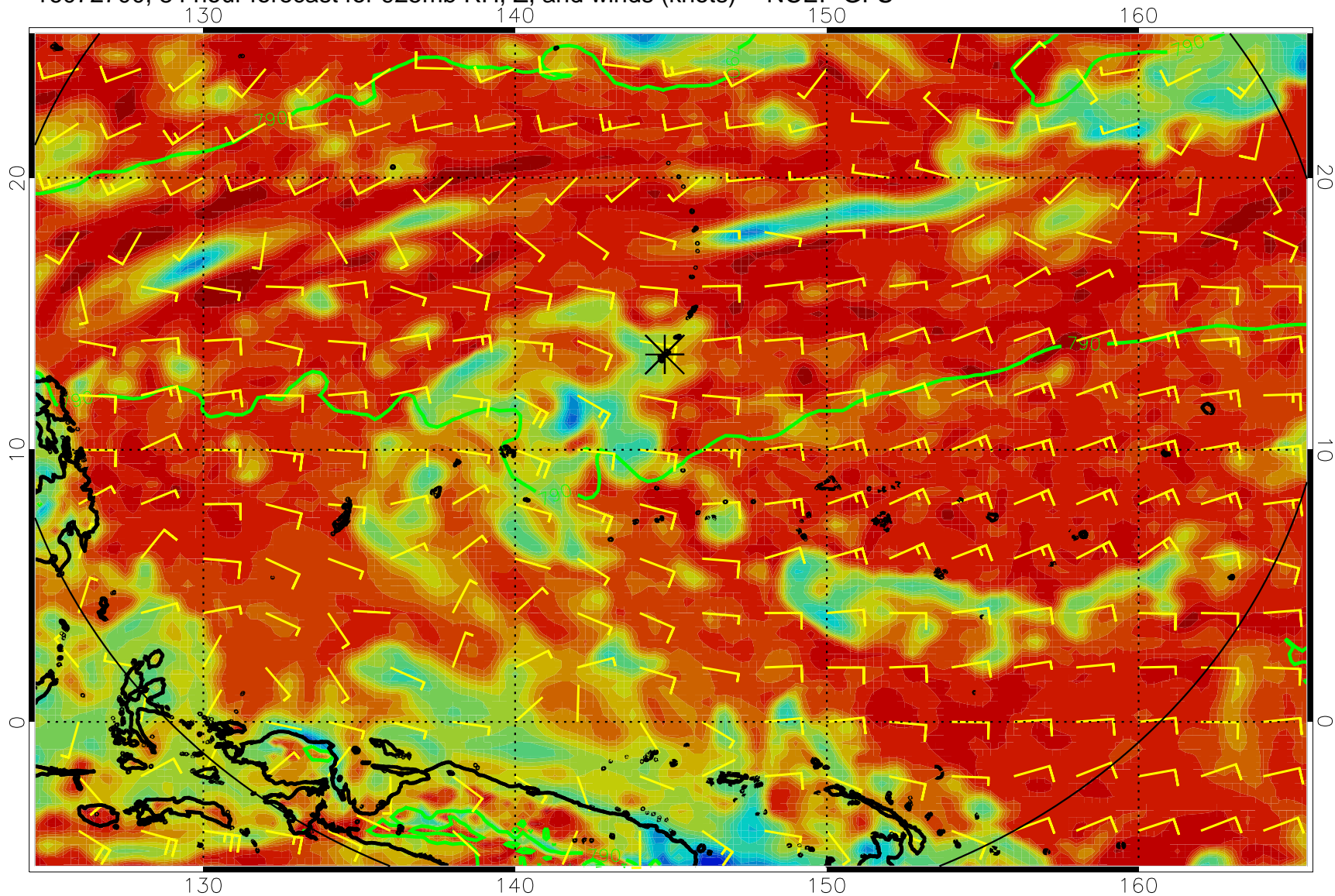
16072700, 84 hour forecast for 925mb RH, Z, and winds (knots) -- NCEP GFS
