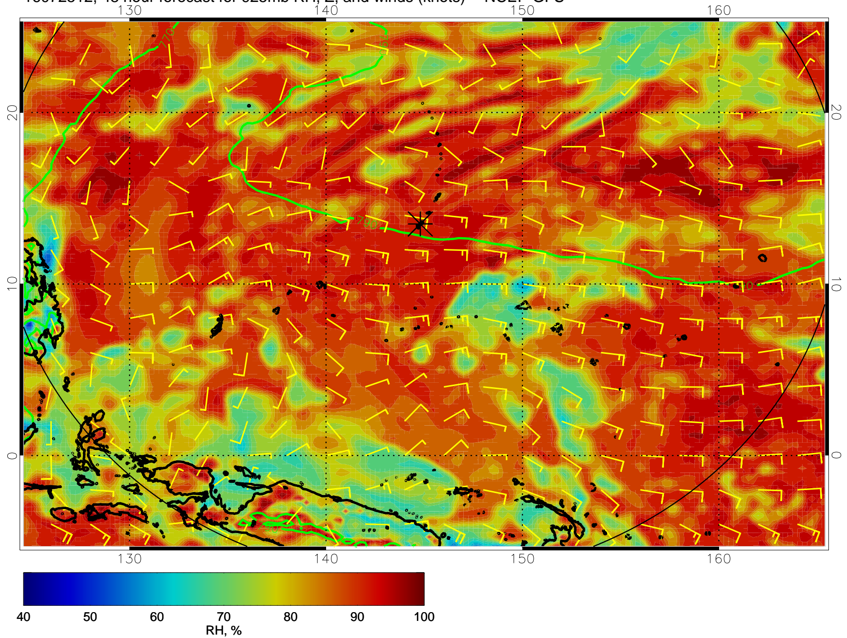
16072512, 48 hour forecast for 925mb RH, Z, and winds (knots) -- NCEP GFS
