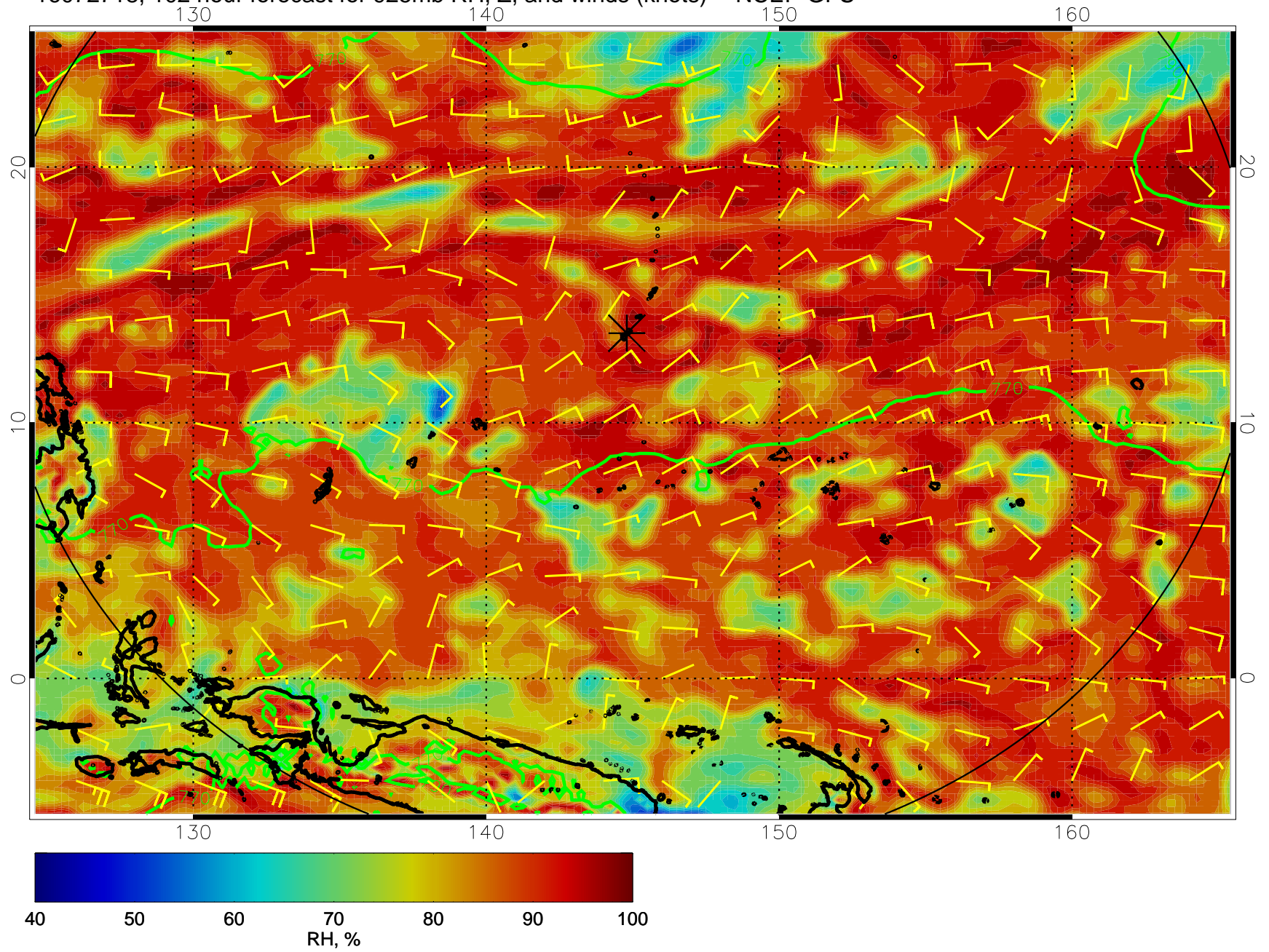
16072718, 102 hour forecast for 925mb RH, Z, and winds (knots) -- NCEP GFS
