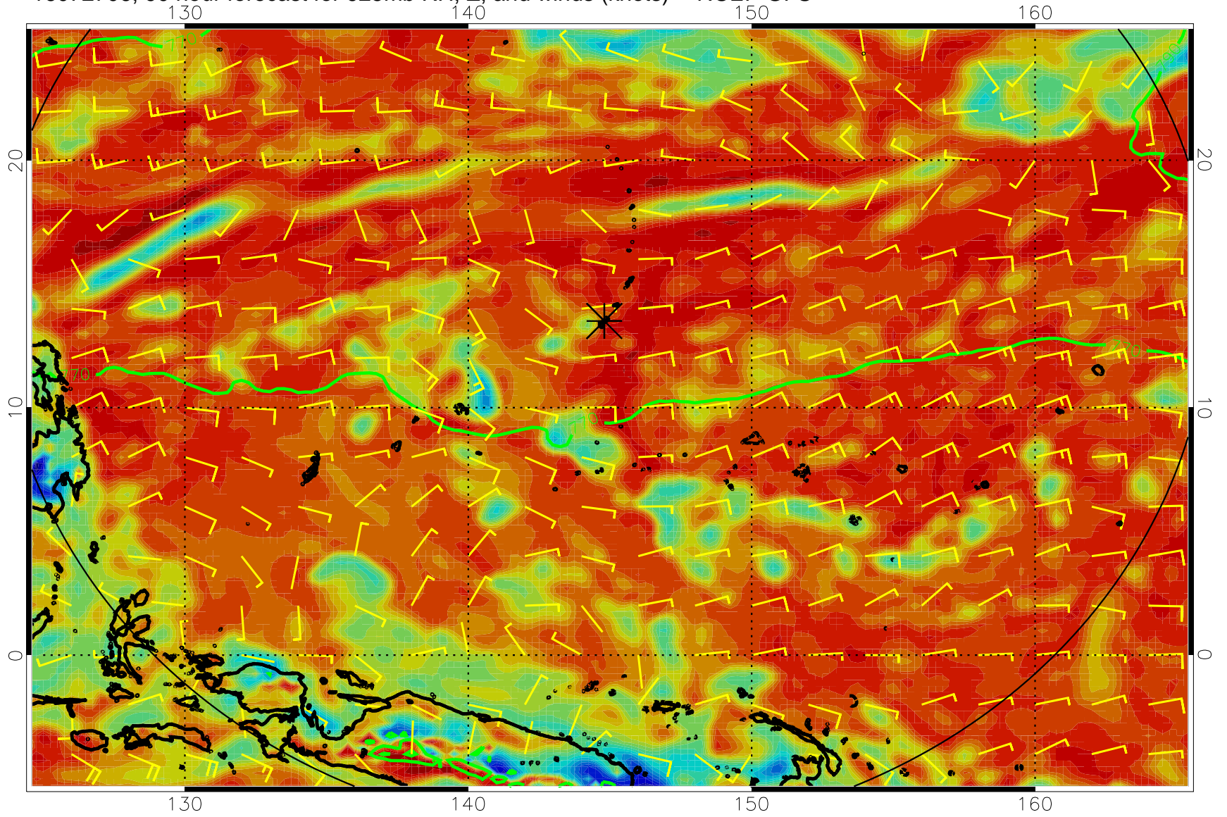
16072706, 90 hour forecast for 925mb RH, Z, and winds (knots) -- NCEP GFS
