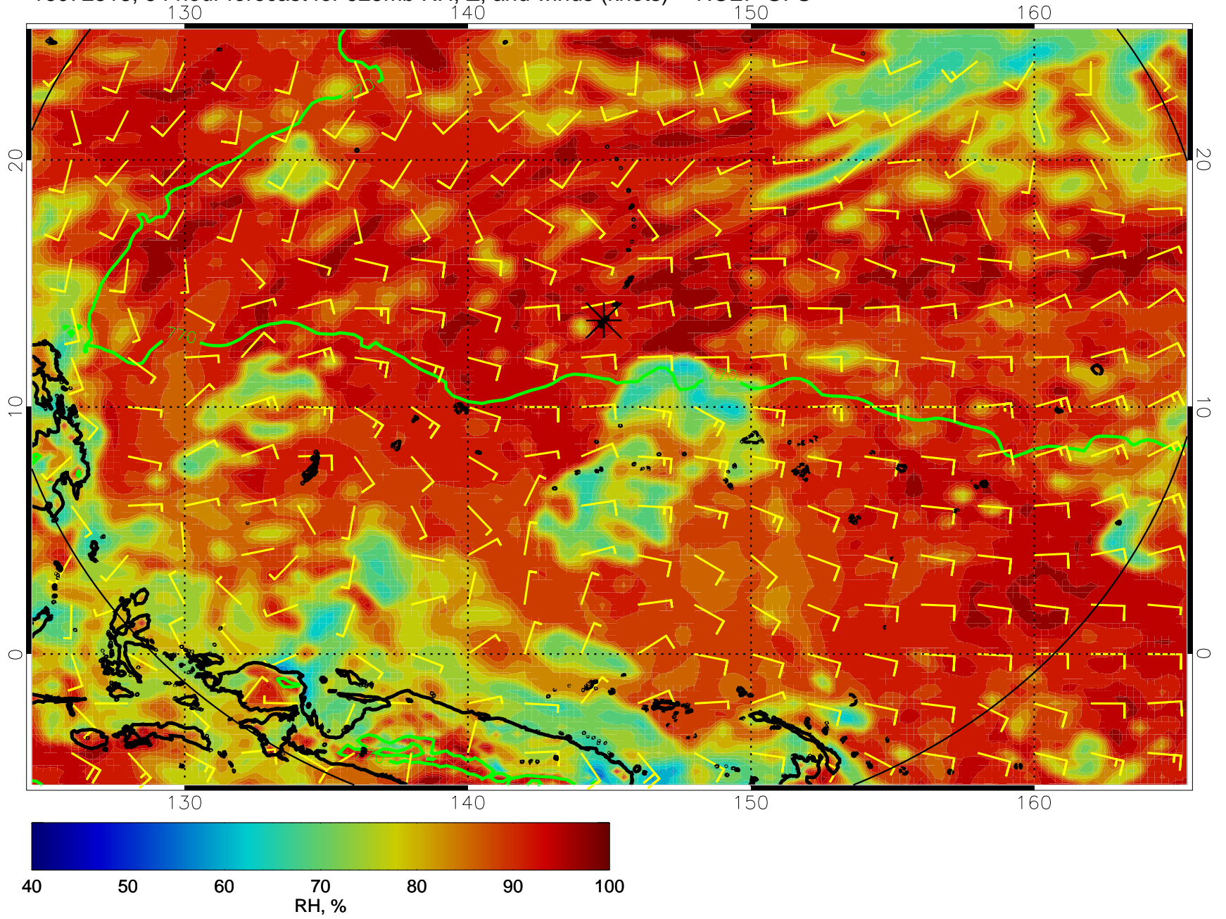
16072518, 54 hour forecast for 925mb RH, Z, and winds (knots) -- NCEP GFS
