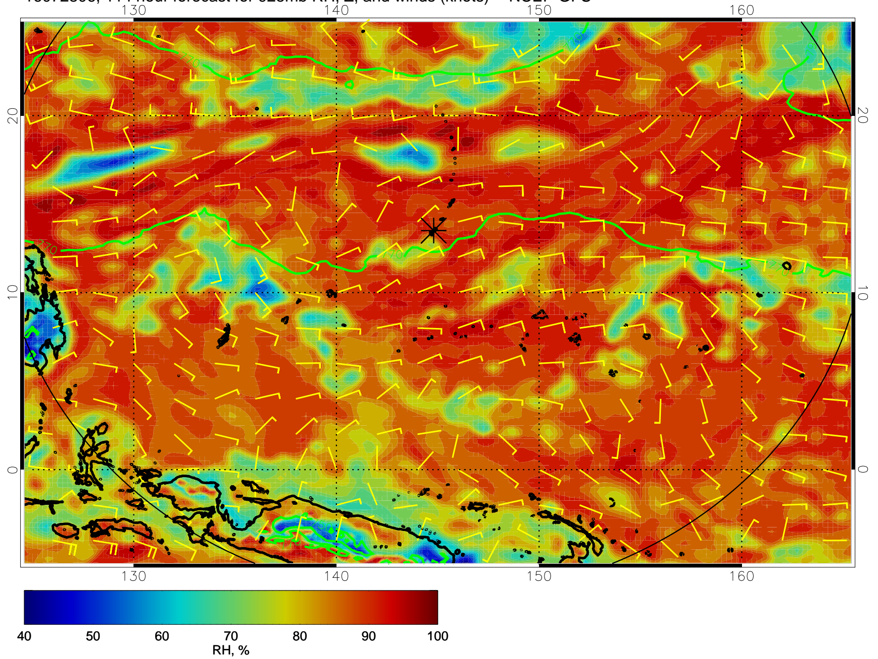
16072806, 114 hour forecast for 925mb RH, Z, and winds (knots) -- NCEP GFS
