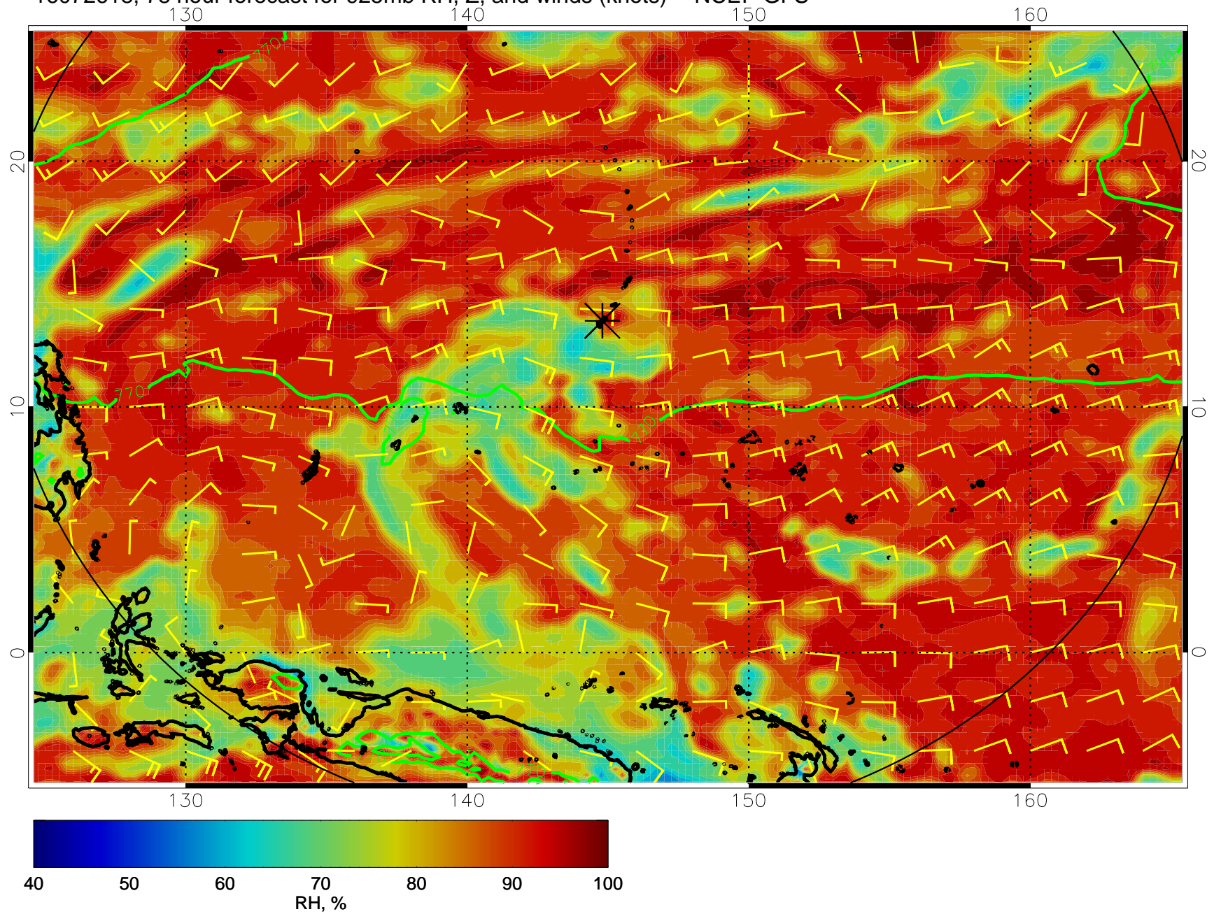
16072618, 78 hour forecast for 925mb RH, Z, and winds (knots) -- NCEP GFS
