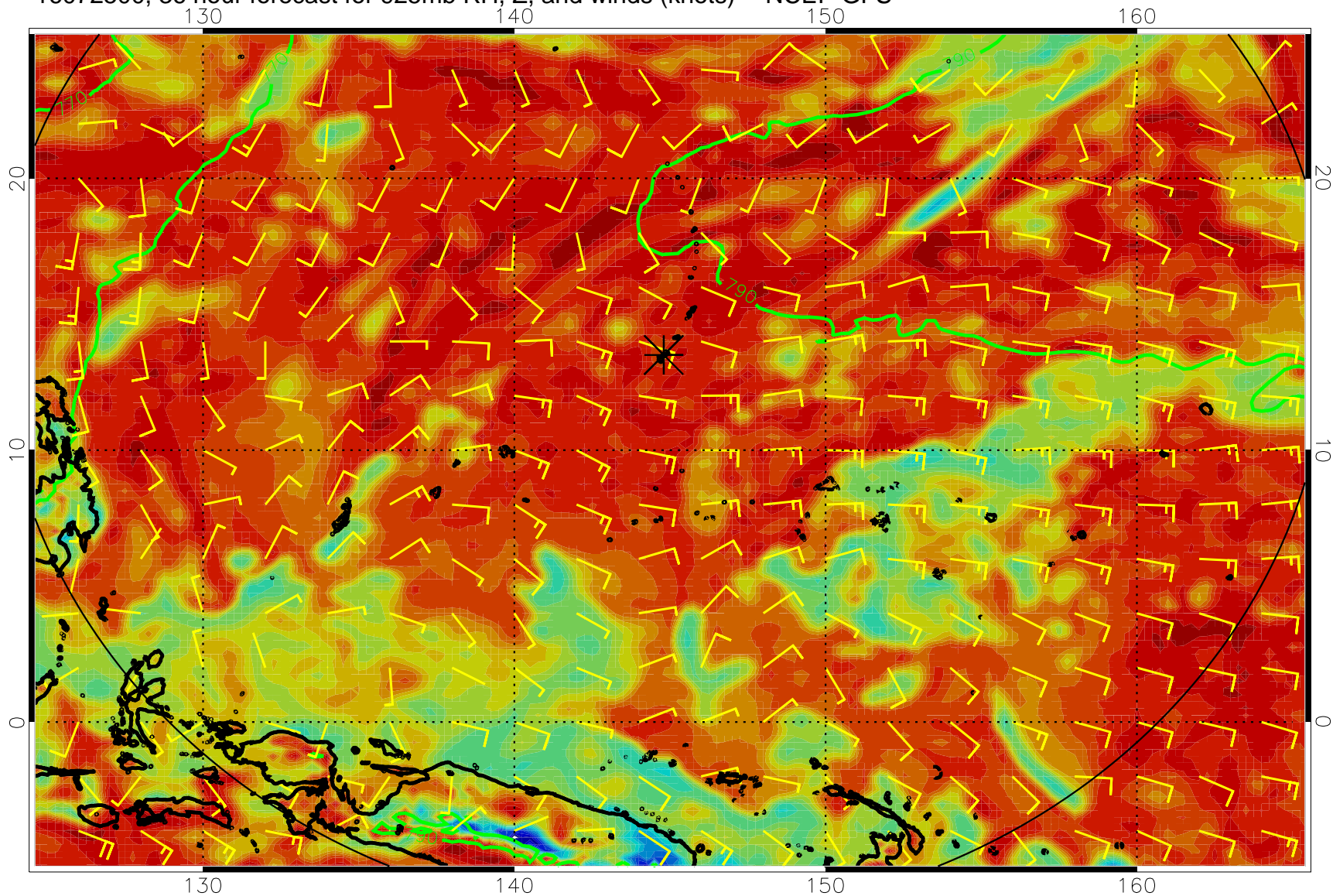
16072500, 36 hour forecast for 925mb RH, Z, and winds (knots) -- NCEP GFS
