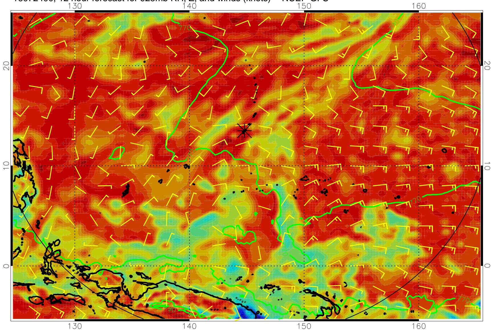
16072400, 12 hour forecast for 925mb RH, Z, and winds (knots) -- NCEP GFS
