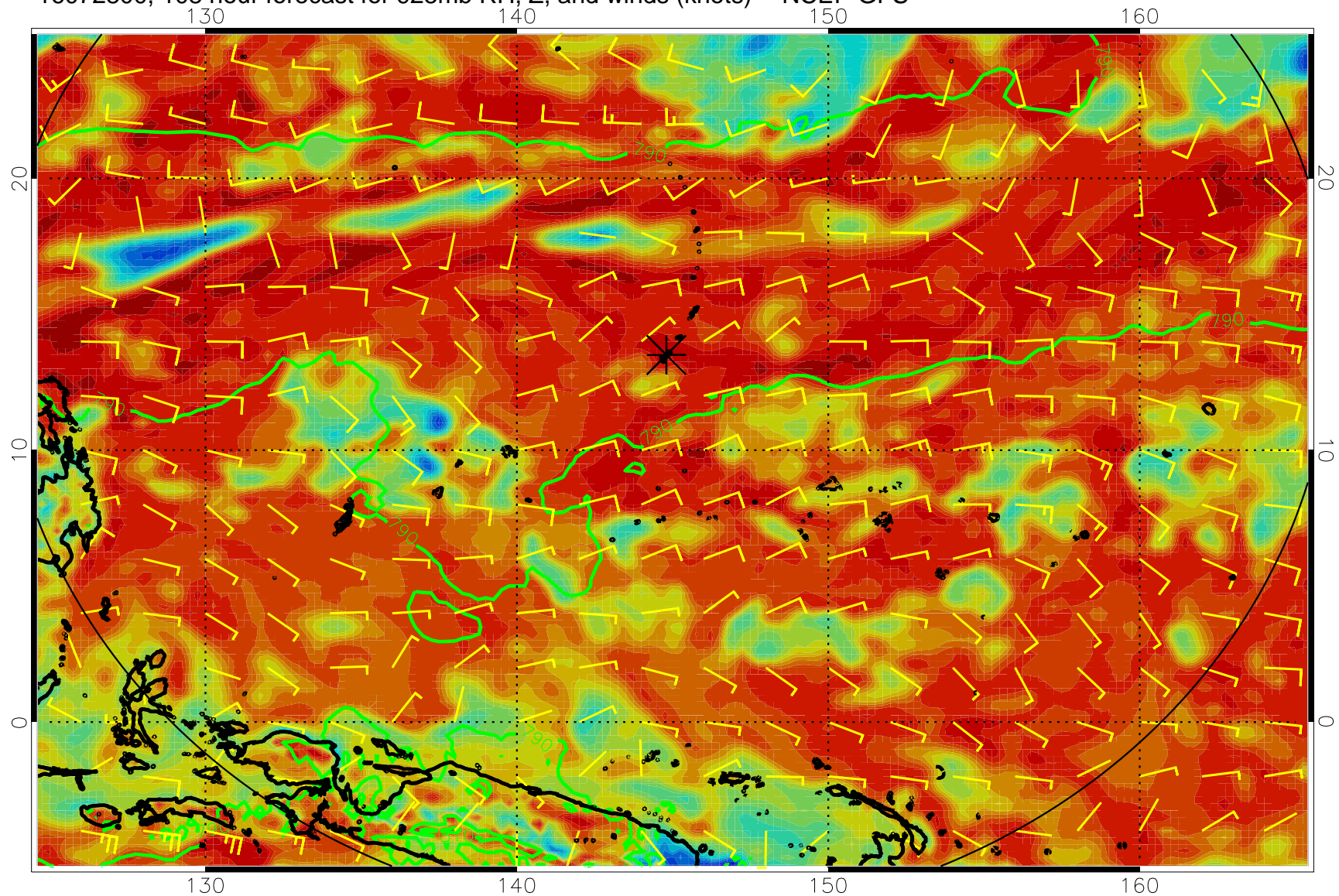
16072800, 108 hour forecast for 925mb RH, Z, and winds (knots) -- NCEP GFS
