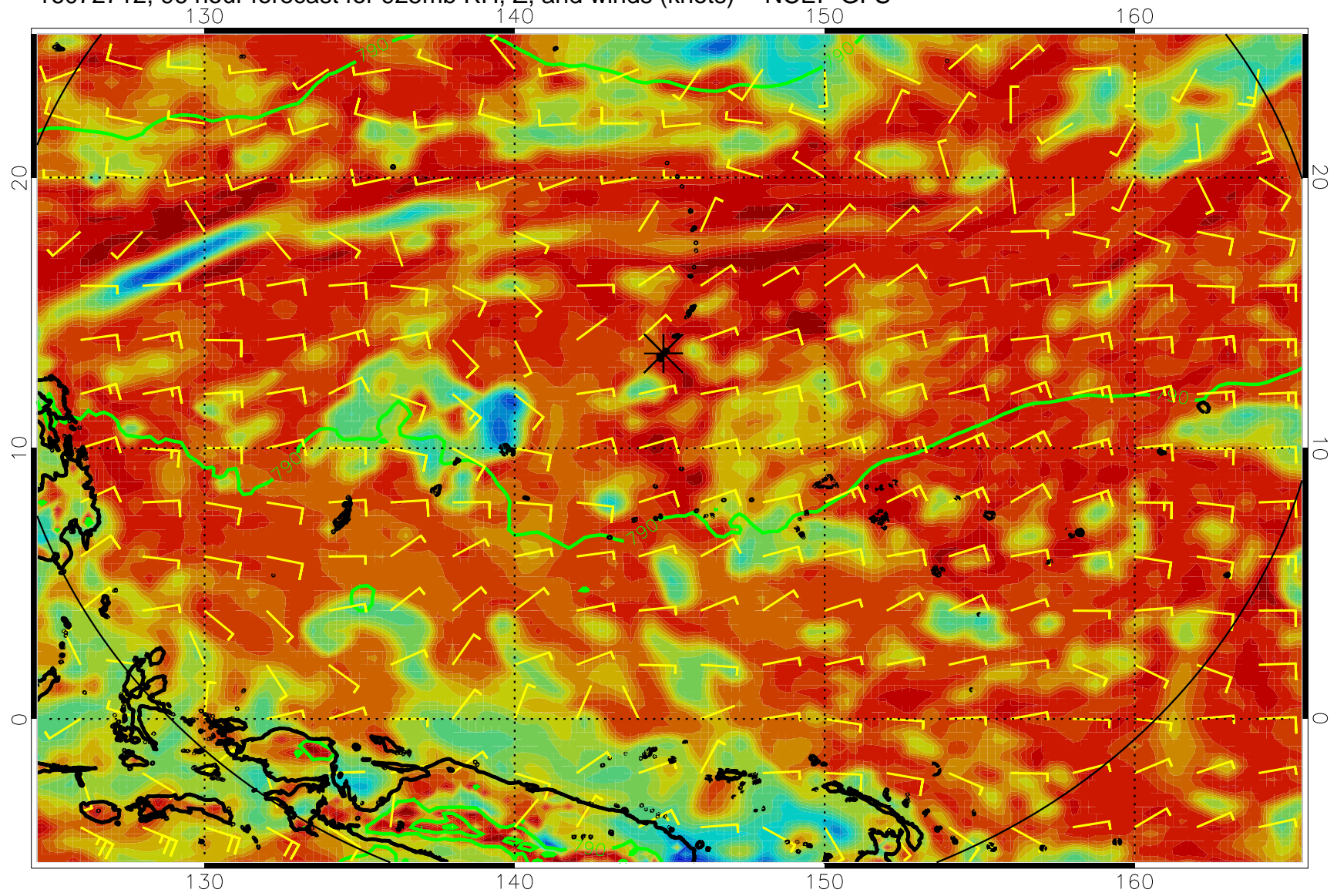
16072712, 96 hour forecast for 925mb RH, Z, and winds (knots) -- NCEP GFS
