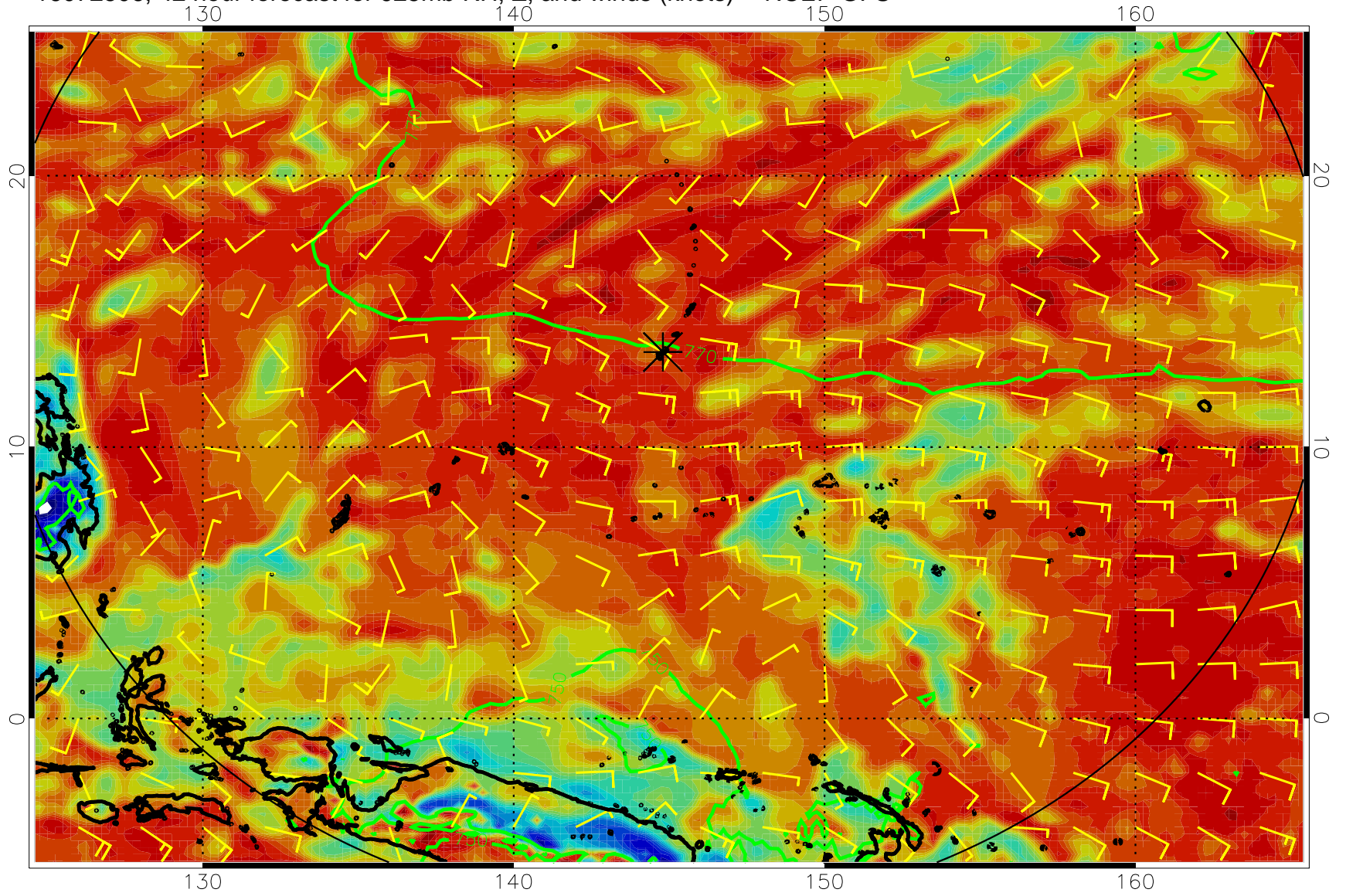
16072506, 42 hour forecast for 925mb RH, Z, and winds (knots) -- NCEP GFS
