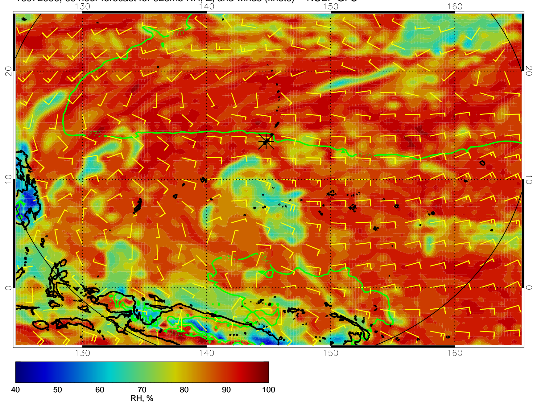
16072606, 66 hour forecast for 925mb RH, Z, and winds (knots) -- NCEP GFS
