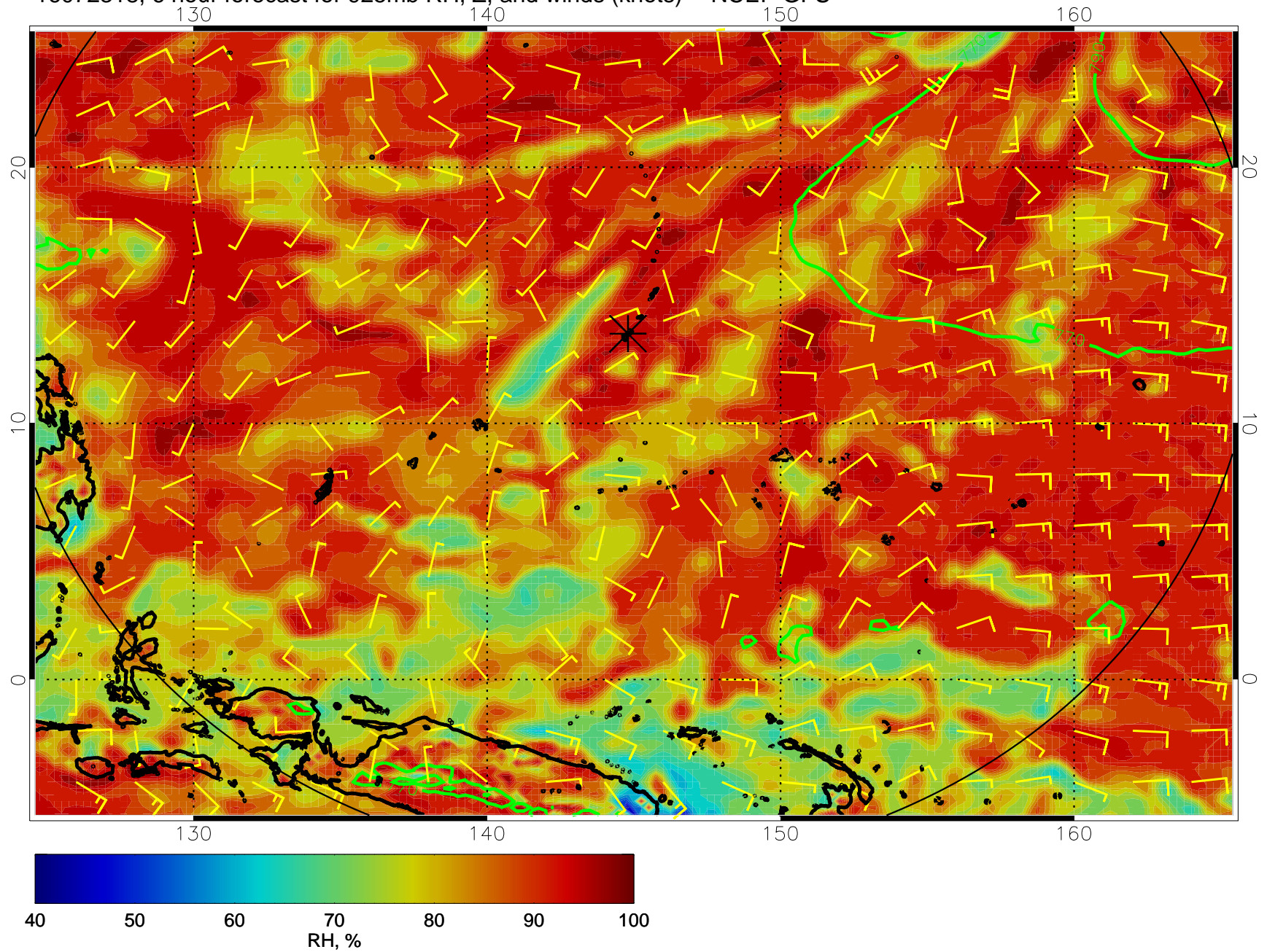
16072318, 6 hour forecast for 925mb RH, Z, and winds (knots) -- NCEP GFS
