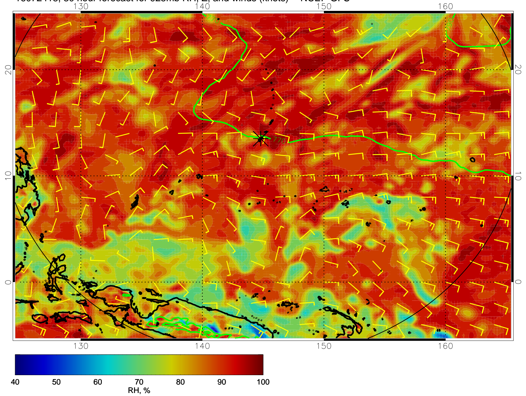
16072418, 30 hour forecast for 925mb RH, Z, and winds (knots) -- NCEP GFS
