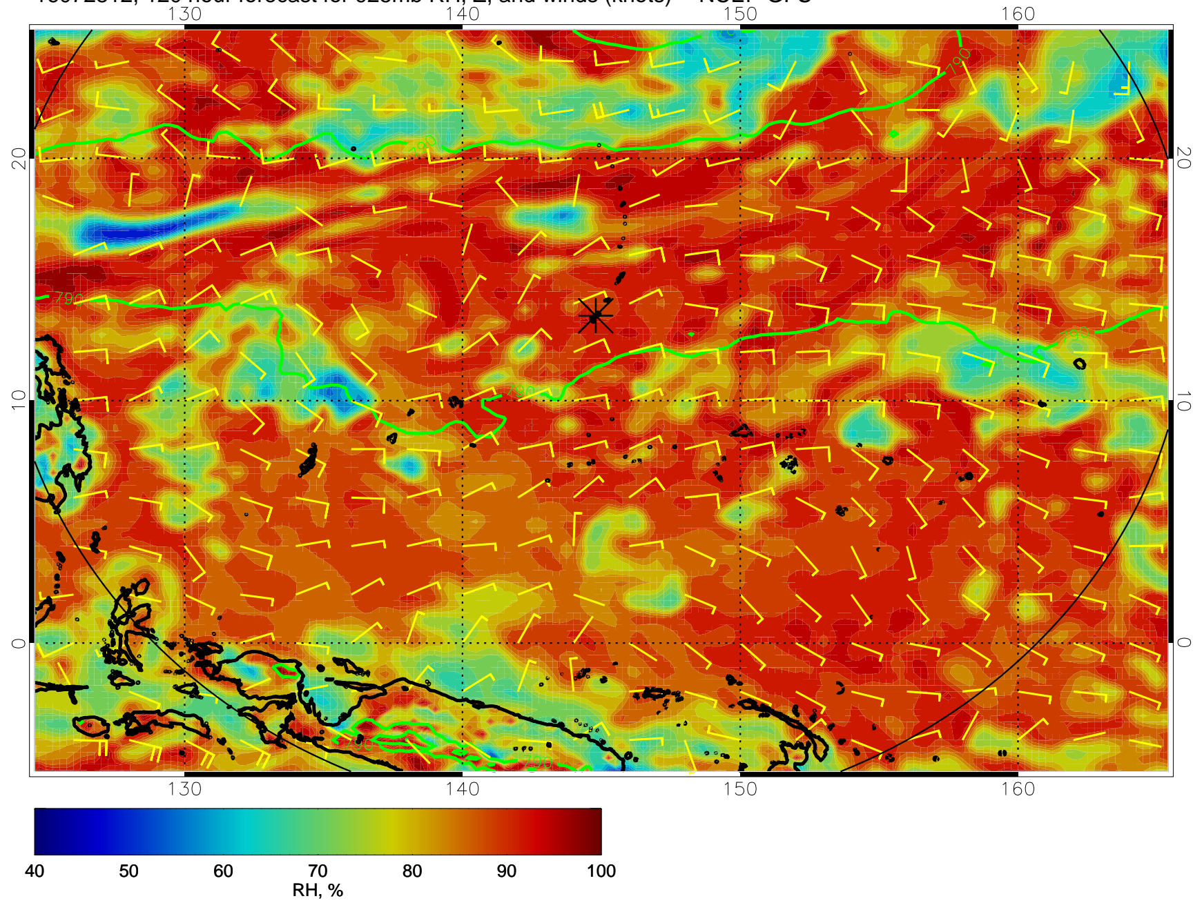
16072812, 120 hour forecast for 925mb RH, Z, and winds (knots) -- NCEP GFS
