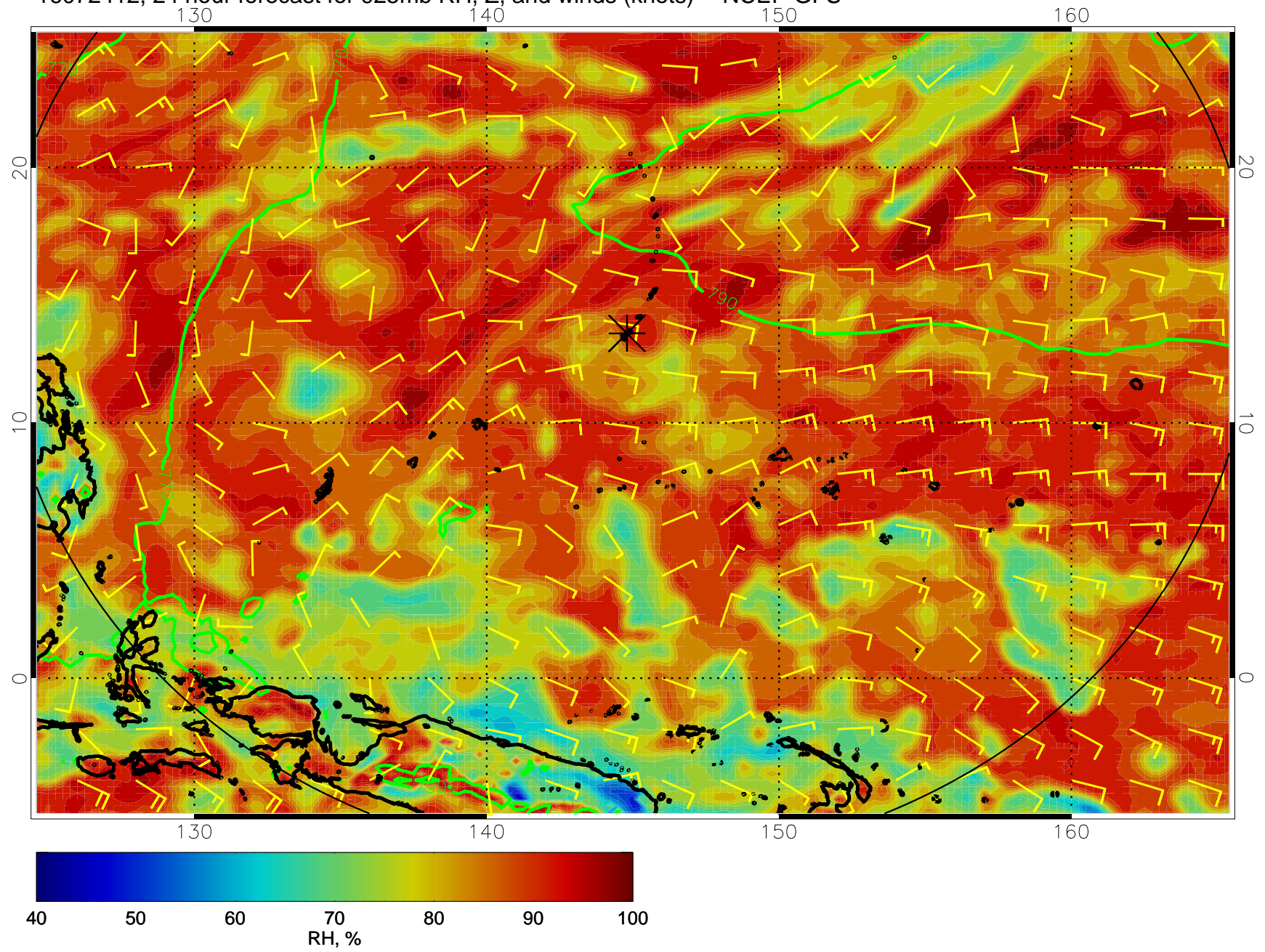
16072412, 24 hour forecast for 925mb RH, Z, and winds (knots) -- NCEP GFS
