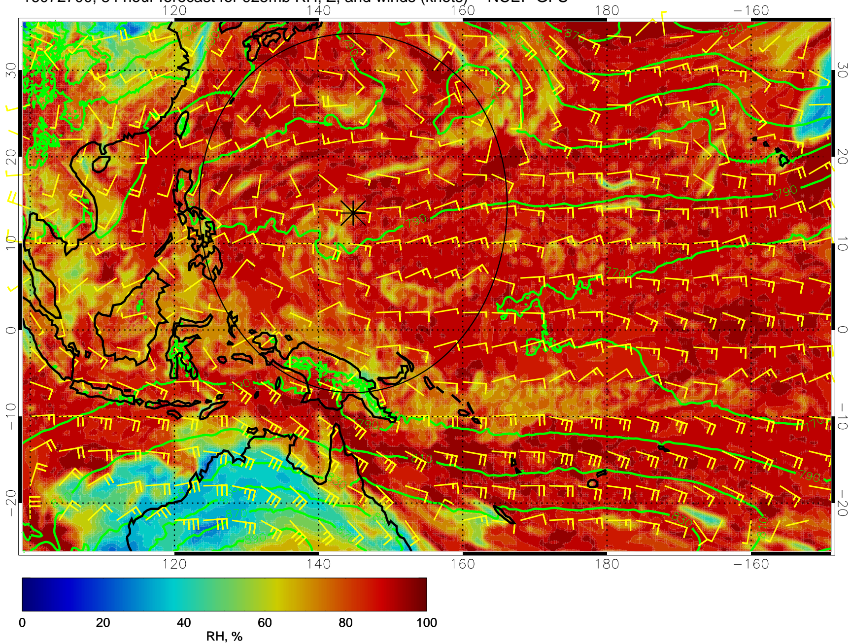
16072700, 84 hour forecast for 925mb RH, Z, and winds (knots) -- NCEP GFS
