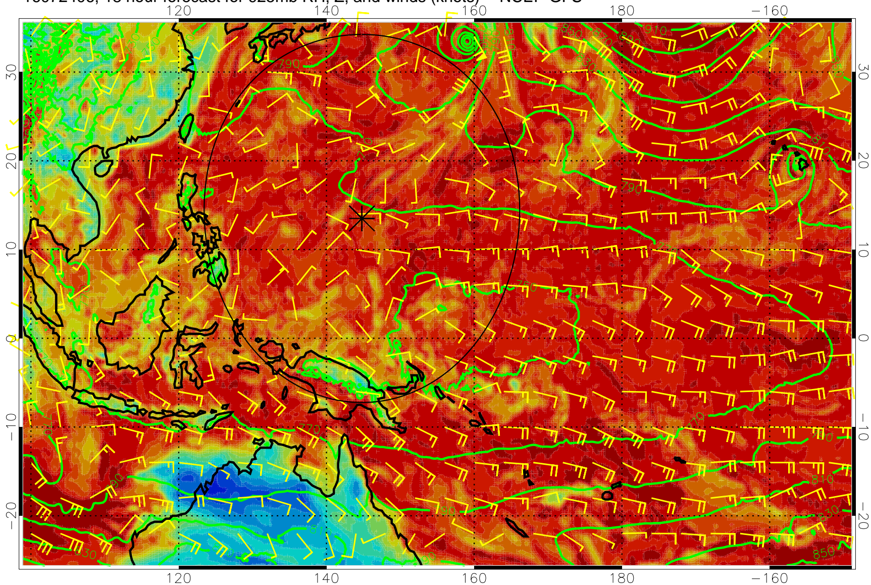
16072406, 18 hour forecast for 925mb RH, Z, and winds (knots) -- NCEP GFS
