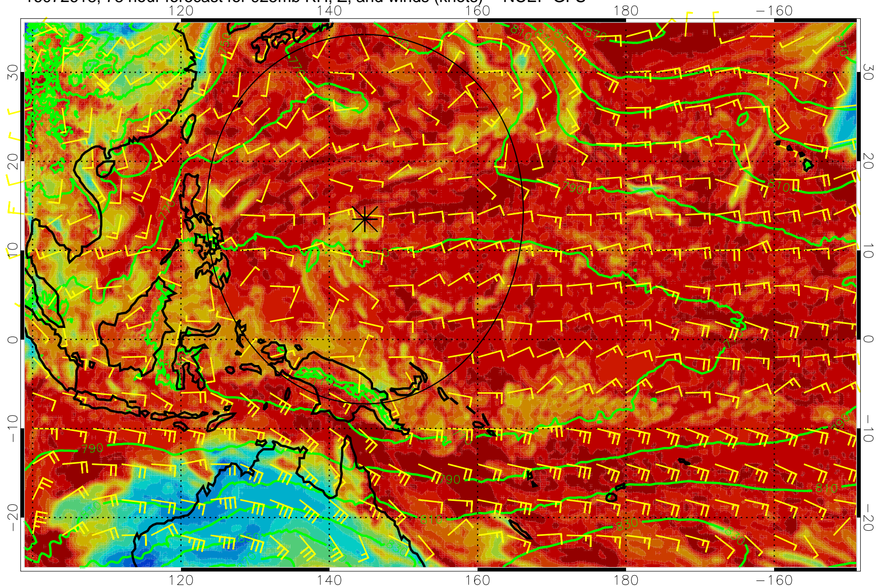
16072618, 78 hour forecast for 925mb RH, Z, and winds (knots) -- NCEP GFS
