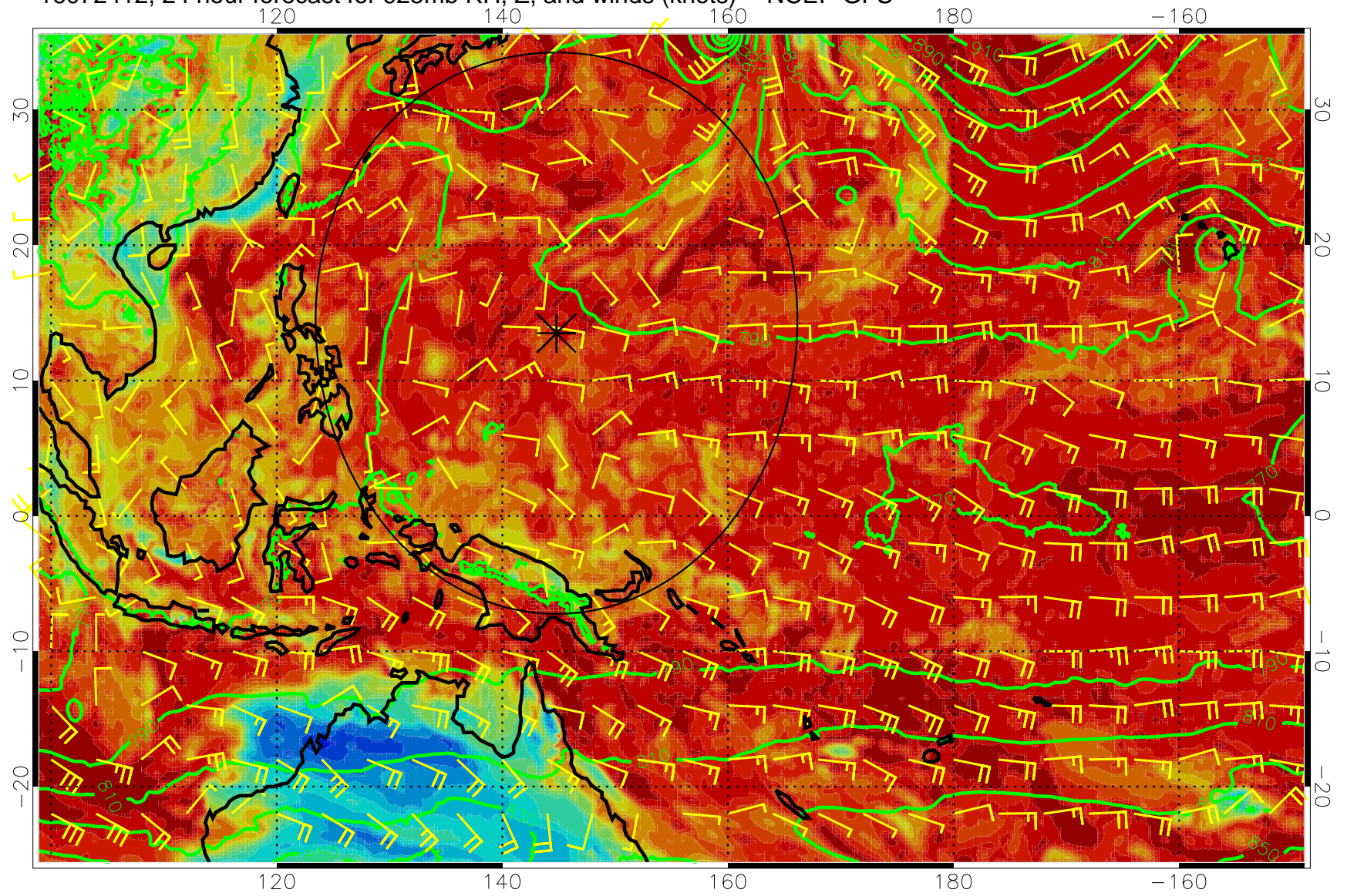
16072412, 24 hour forecast for 925mb RH, Z, and winds (knots) -- NCEP GFS
