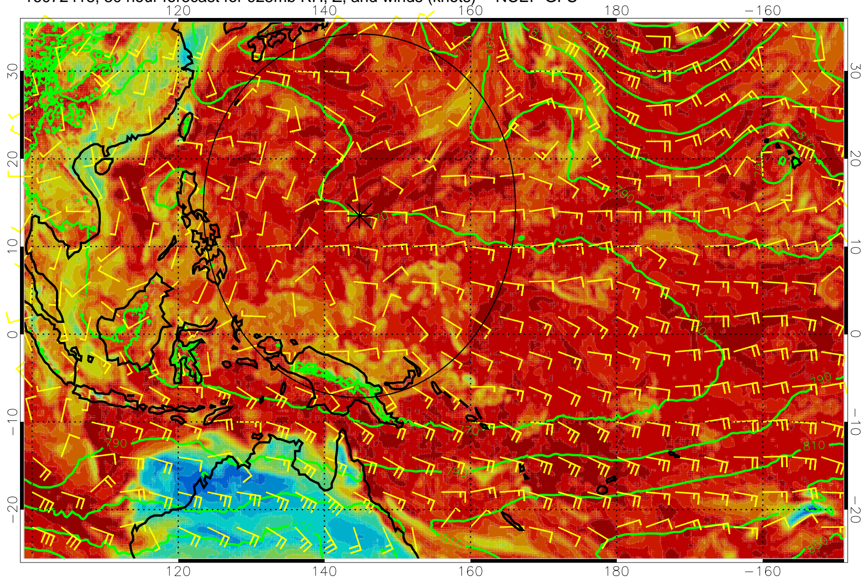
16072418, 30 hour forecast for 925mb RH, Z, and winds (knots) -- NCEP GFS
