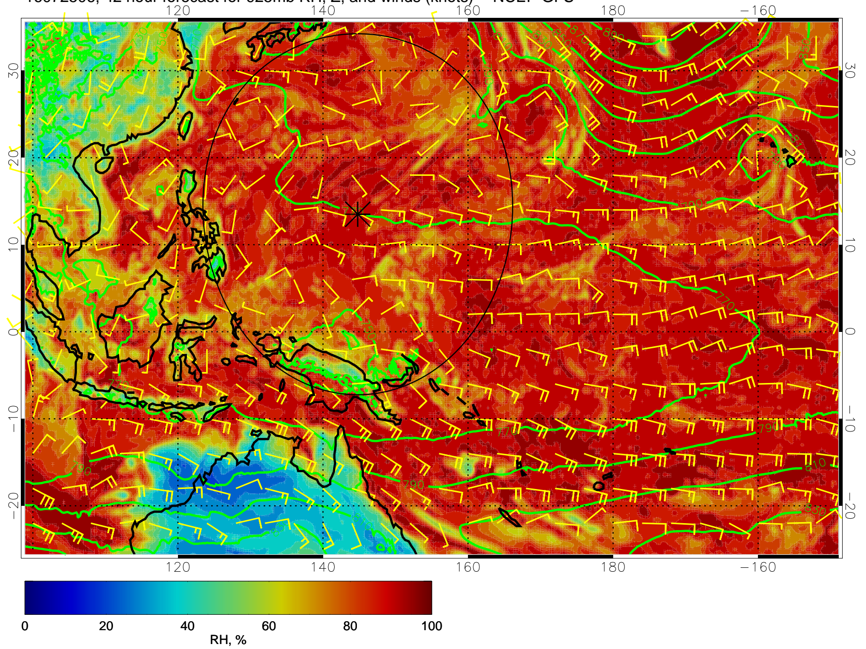
16072506, 42 hour forecast for 925mb RH, Z, and winds (knots) -- NCEP GFS
