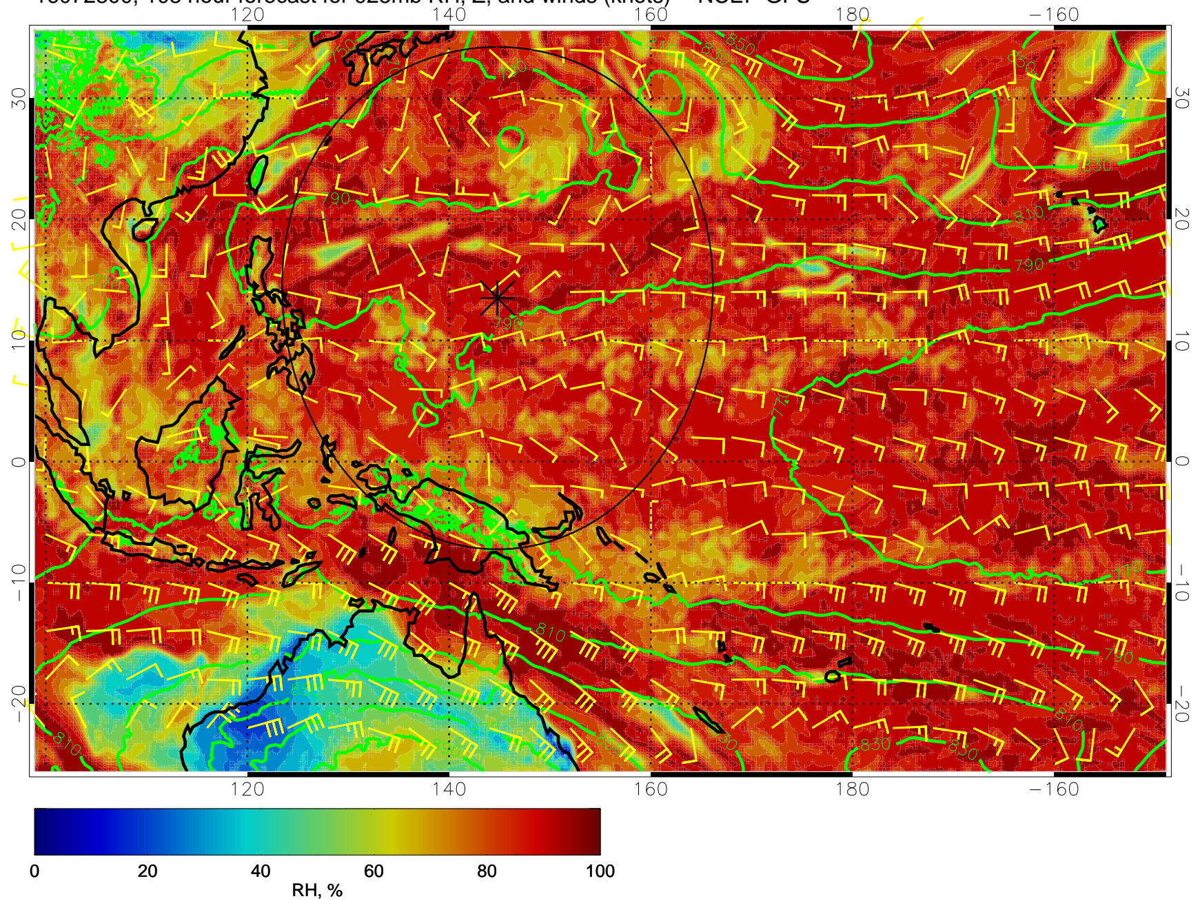
16072800, 108 hour forecast for 925mb RH, Z, and winds (knots) -- NCEP GFS
