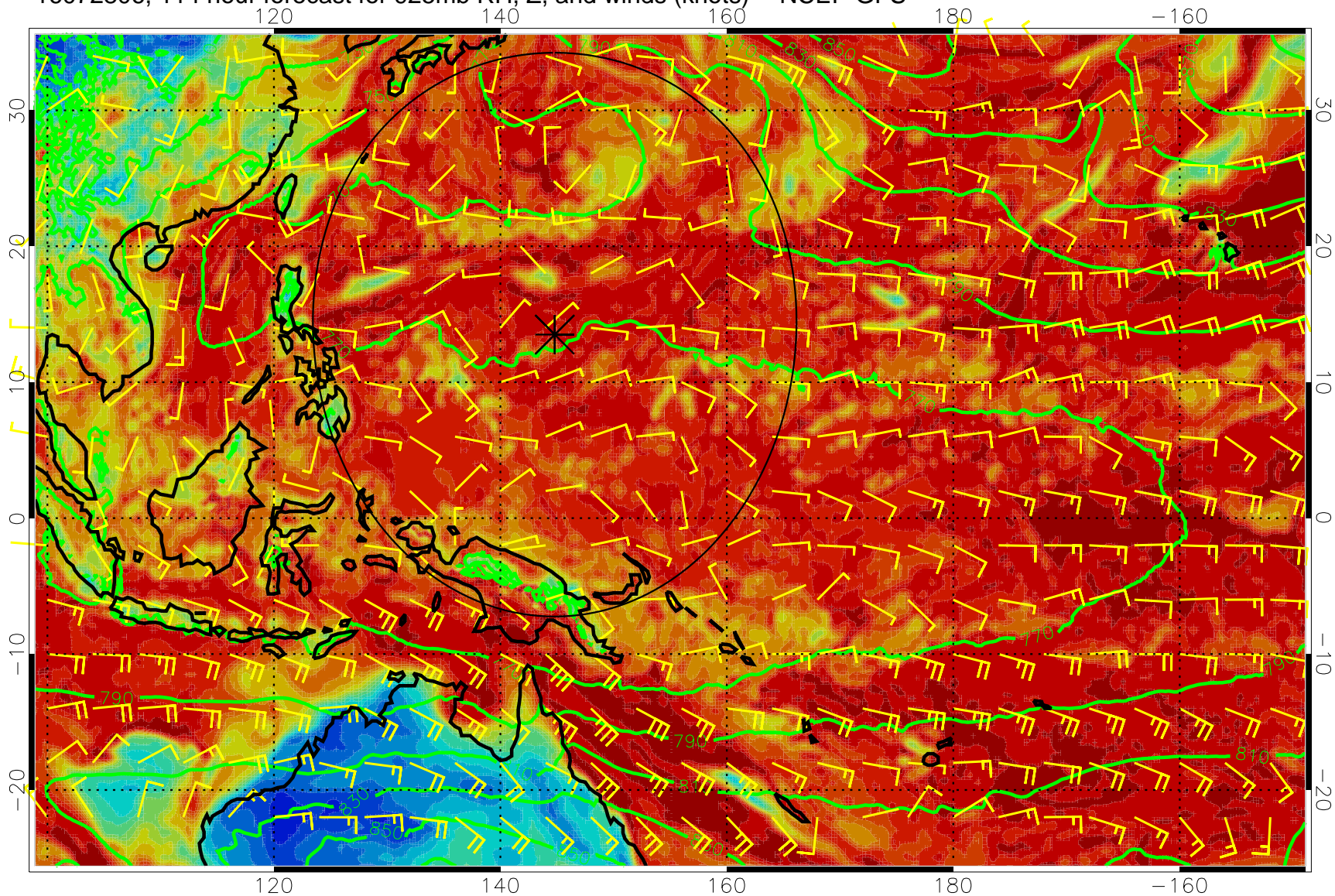
16072806, 114 hour forecast for 925mb RH, Z, and winds (knots) -- NCEP GFS
