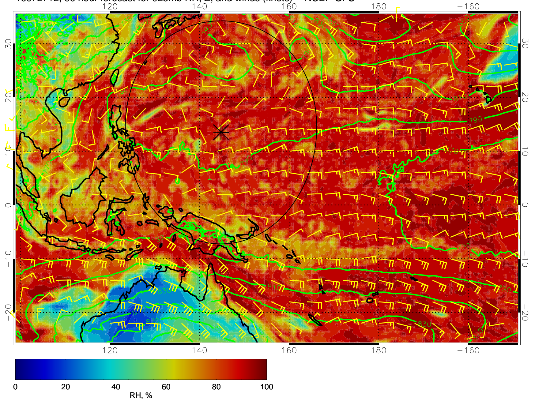
16072712, 96 hour forecast for 925mb RH, Z, and winds (knots) -- NCEP GFS
