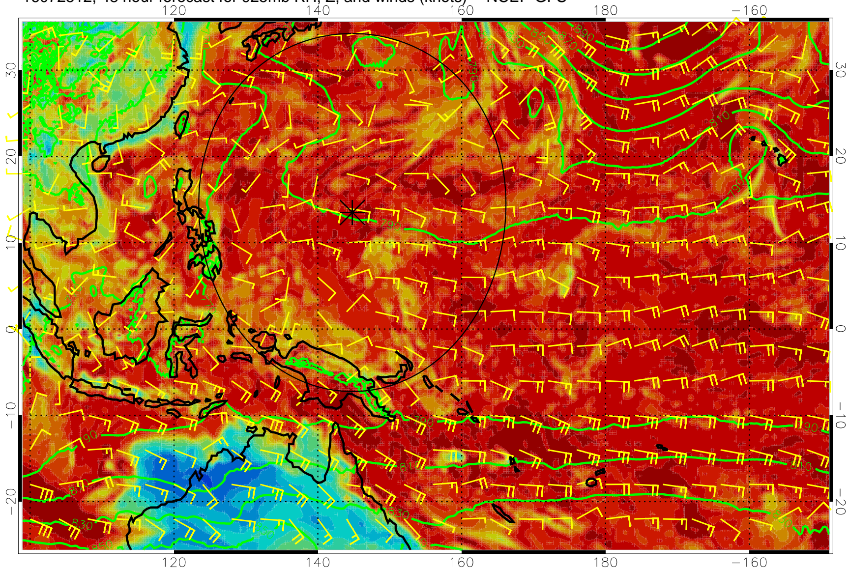
16072512, 48 hour forecast for 925mb RH, Z, and winds (knots) -- NCEP GFS
