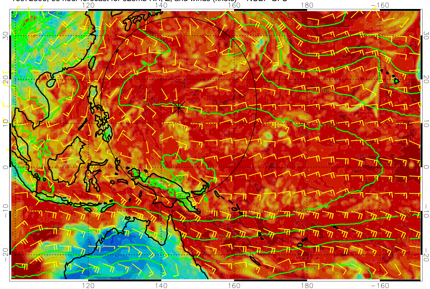
16072606, 66 hour forecast for 925mb RH, Z, and winds (knots) -- NCEP GFS
