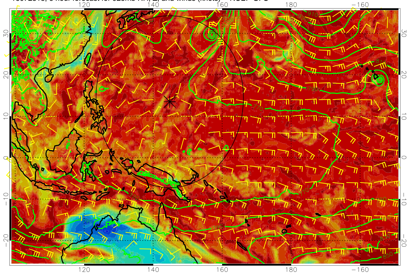
16072318, 6 hour forecast for 925mb RH, Z, and winds (knots) -- NCEP GFS
