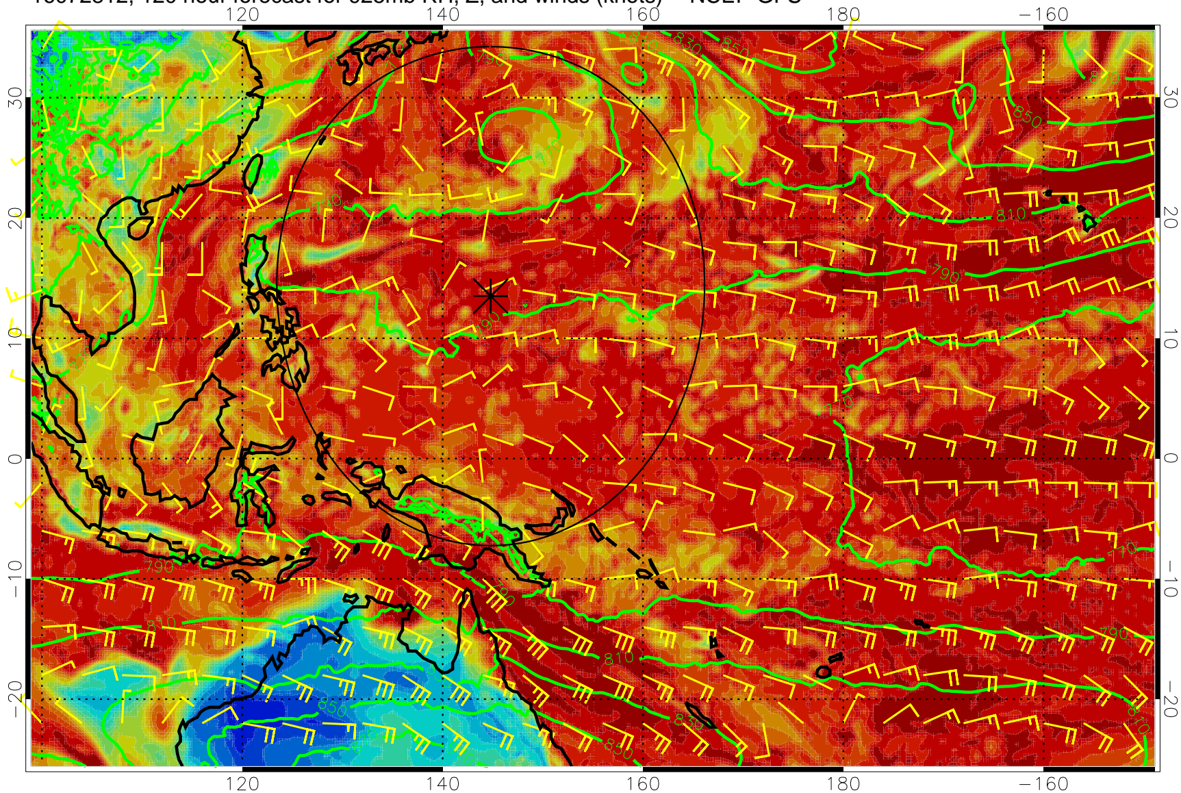
16072812, 120 hour forecast for 925mb RH, Z, and winds (knots) -- NCEP GFS
