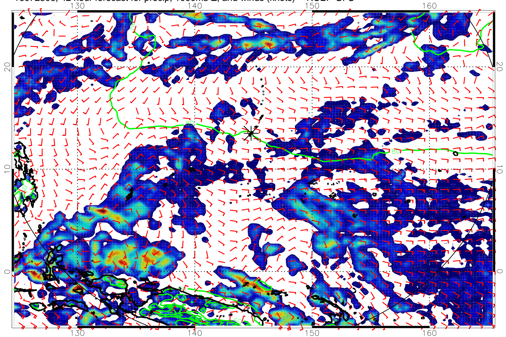
16072506, 42 hour forecast for precip, 1000mb Z, and winds (knots) -- NCEP GFS
