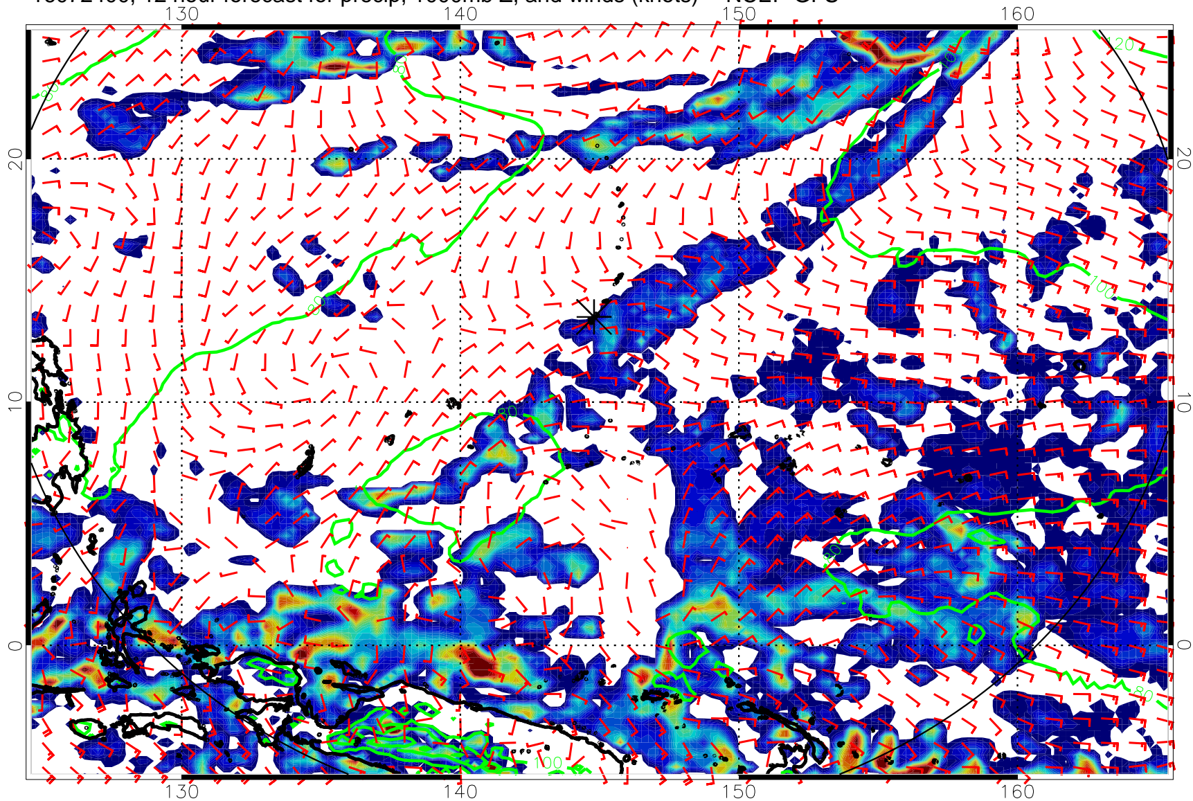
16072400, 12 hour forecast for precip, 1000mb Z, and winds (knots) -- NCEP GFS
