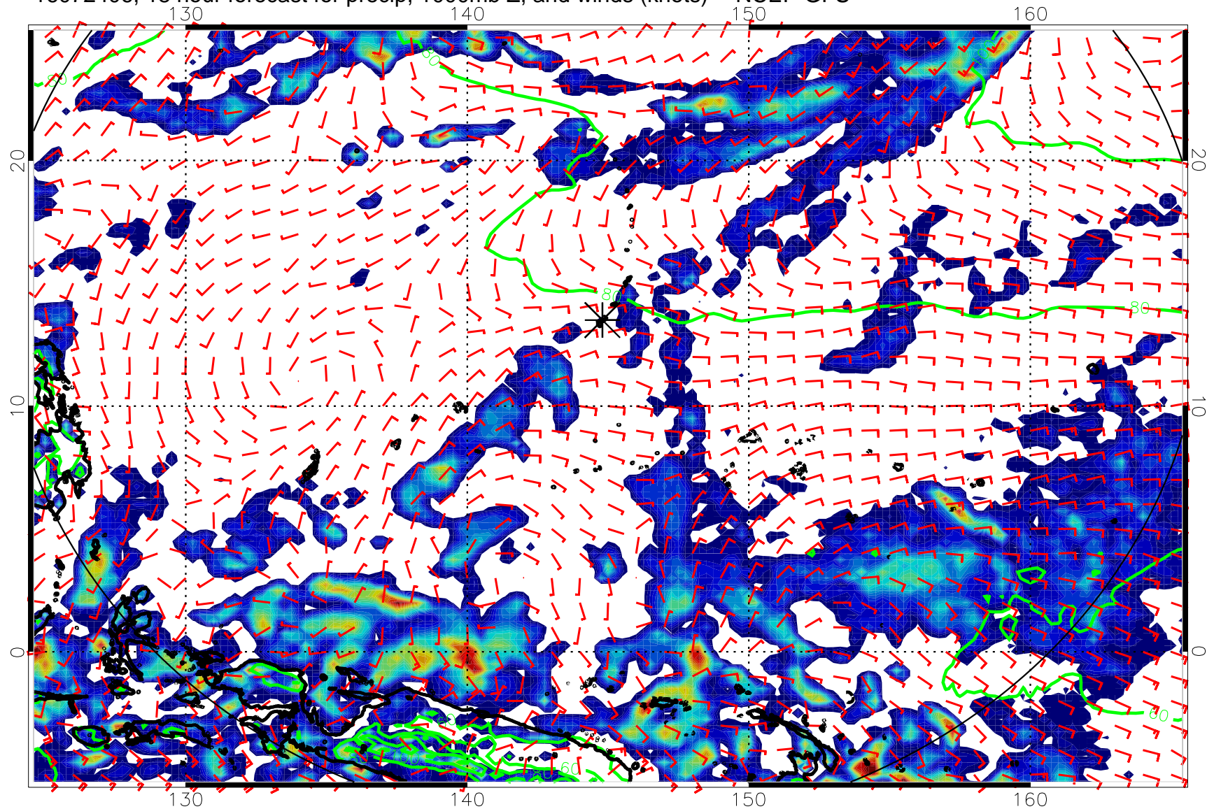
16072406, 18 hour forecast for precip, 1000mb Z, and winds (knots) -- NCEP GFS
