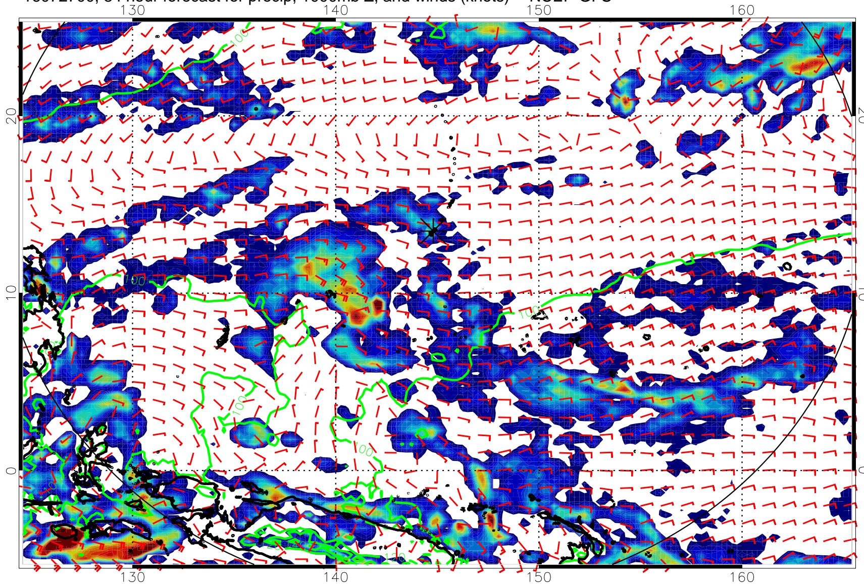
16072700, 84 hour forecast for precip, 1000mb Z, and winds (knots) -- NCEP GFS
