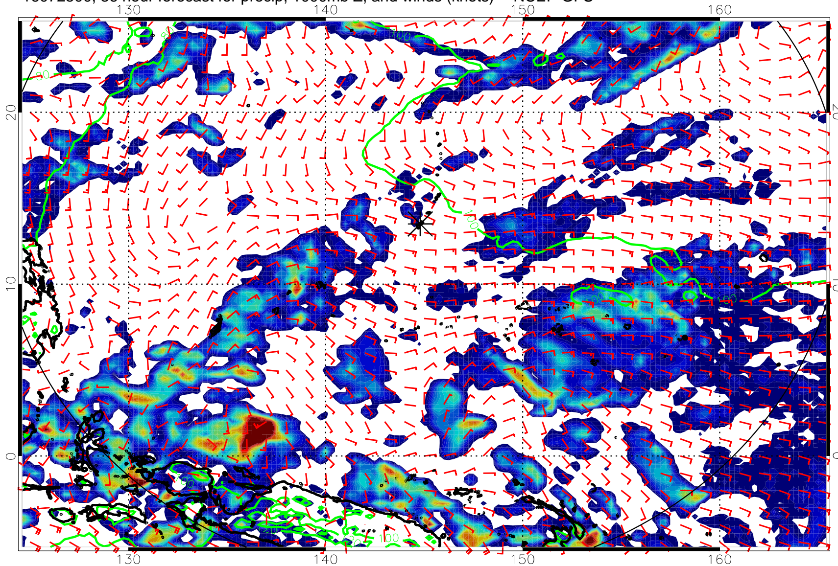
16072500, 36 hour forecast for precip, 1000mb Z, and winds (knots) -- NCEP GFS
