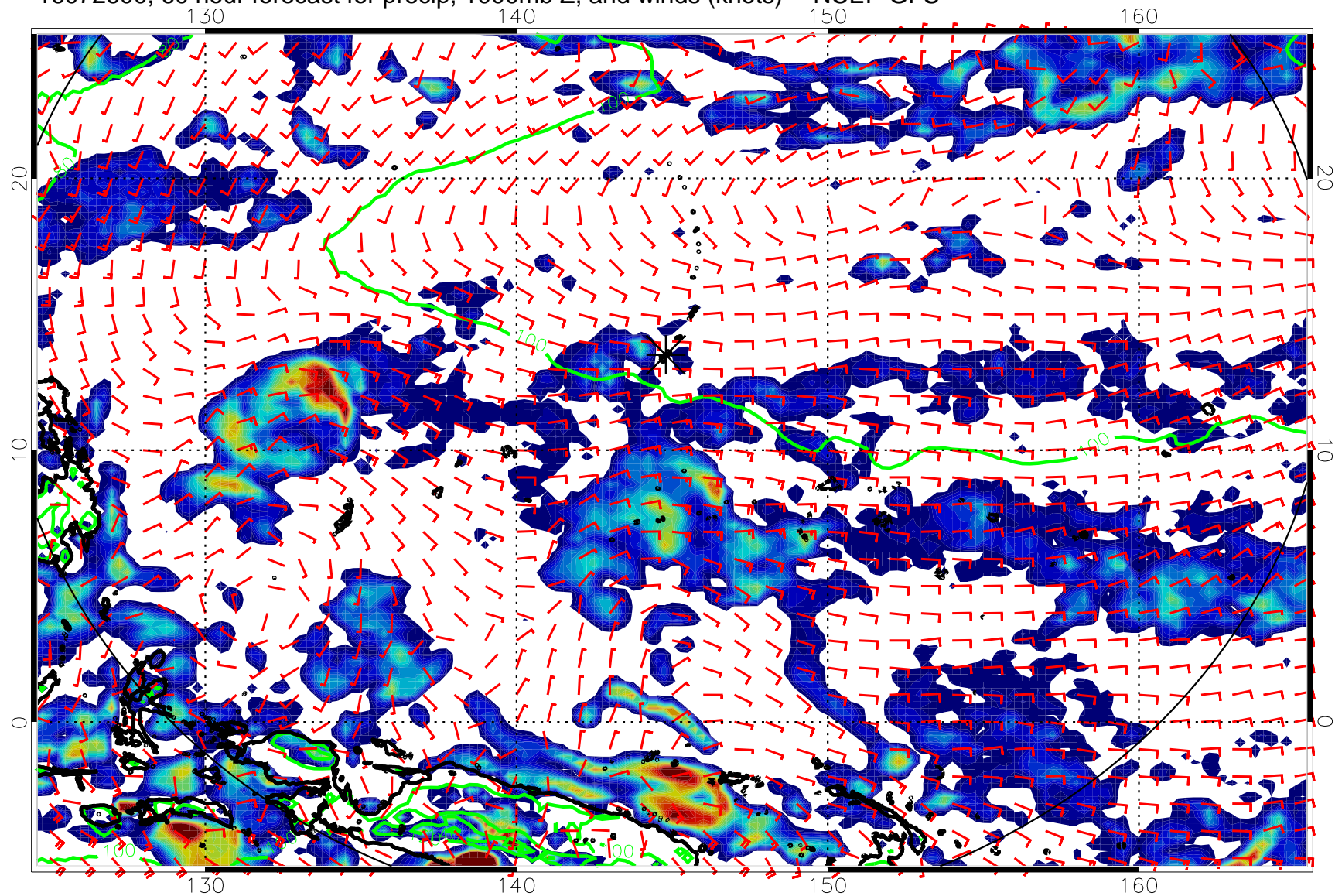
16072600, 60 hour forecast for precip, 1000mb Z, and winds (knots) -- NCEP GFS
