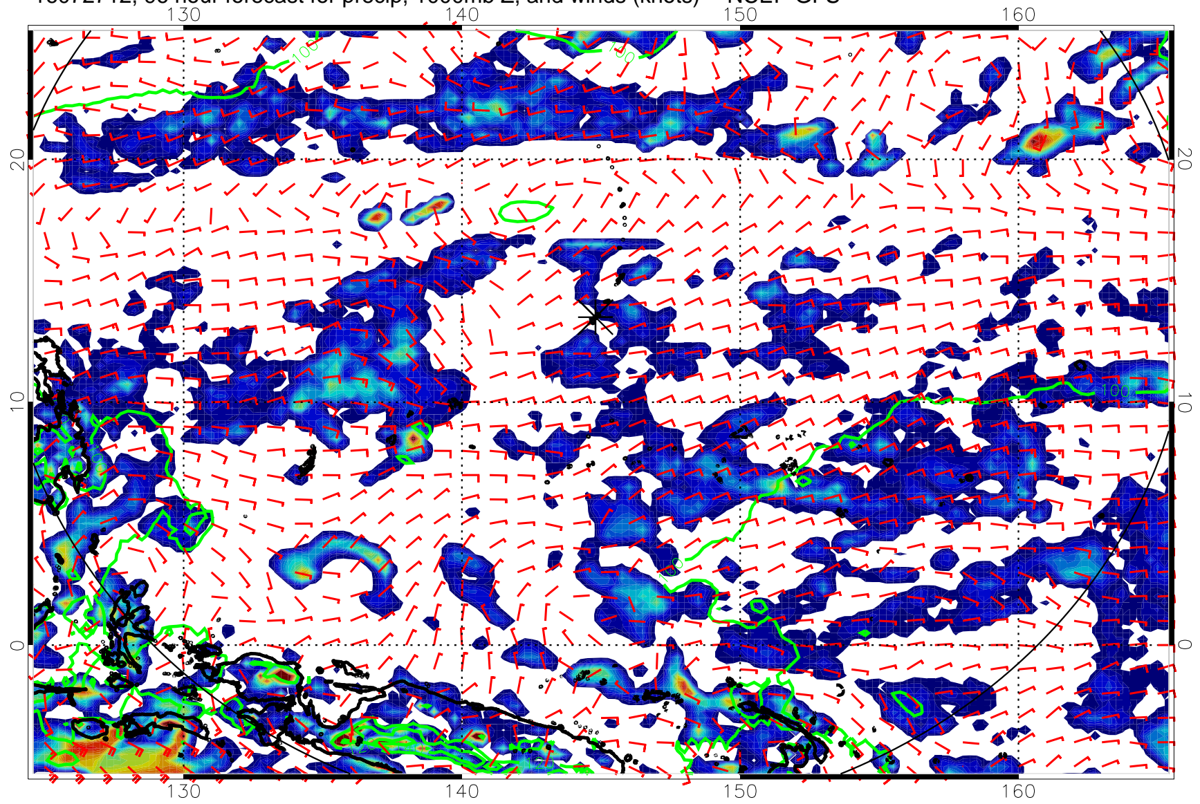
16072712, 96 hour forecast for precip, 1000mb Z, and winds (knots) -- NCEP GFS
