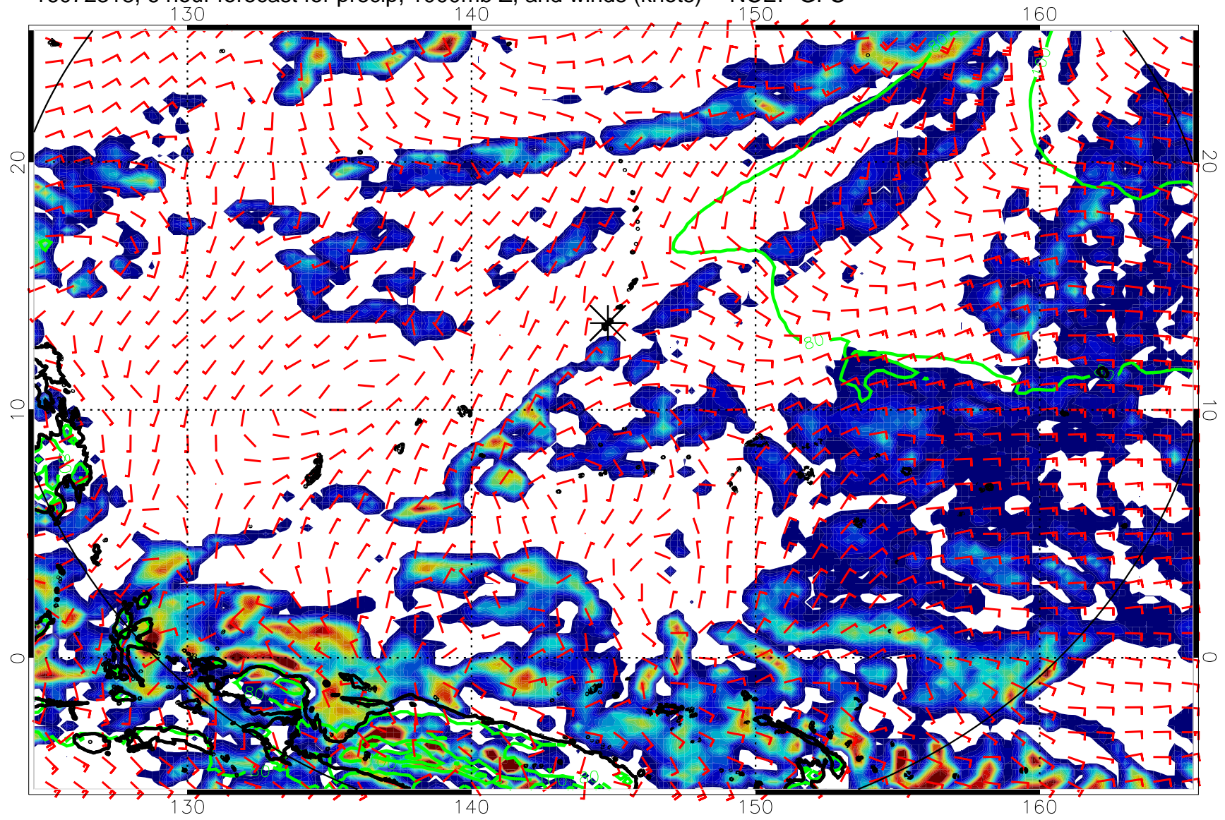
16072318, 6 hour forecast for precip, 1000mb Z, and winds (knots) -- NCEP GFS
