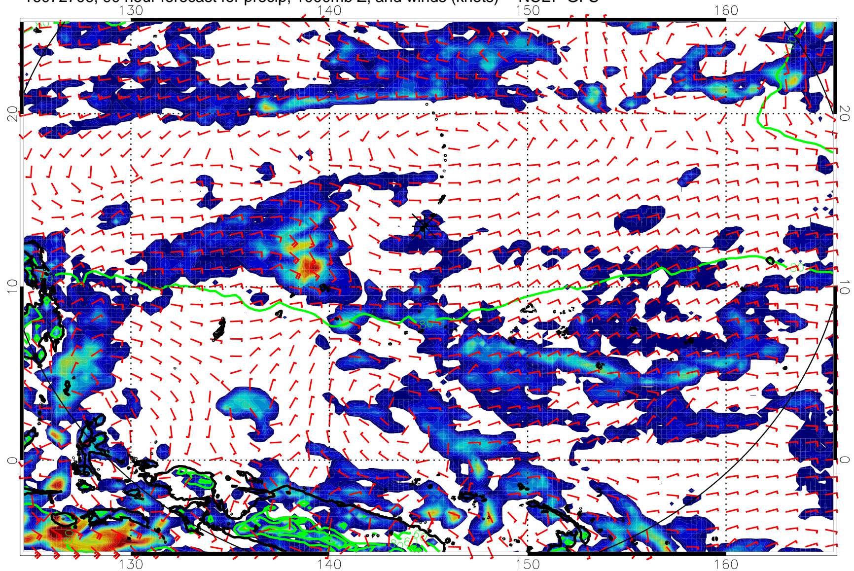
16072706, 90 hour forecast for precip, 1000mb Z, and winds (knots) -- NCEP GFS
