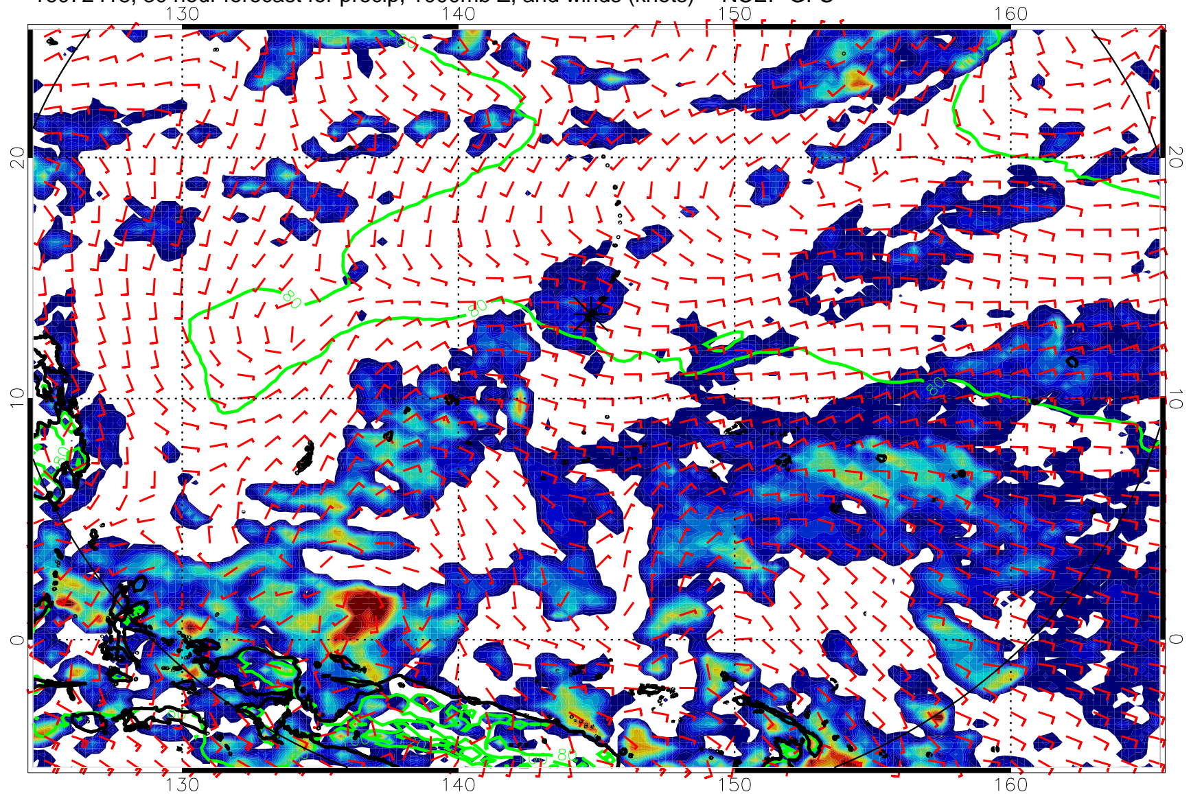
16072418, 30 hour forecast for precip, 1000mb Z, and winds (knots) -- NCEP GFS
