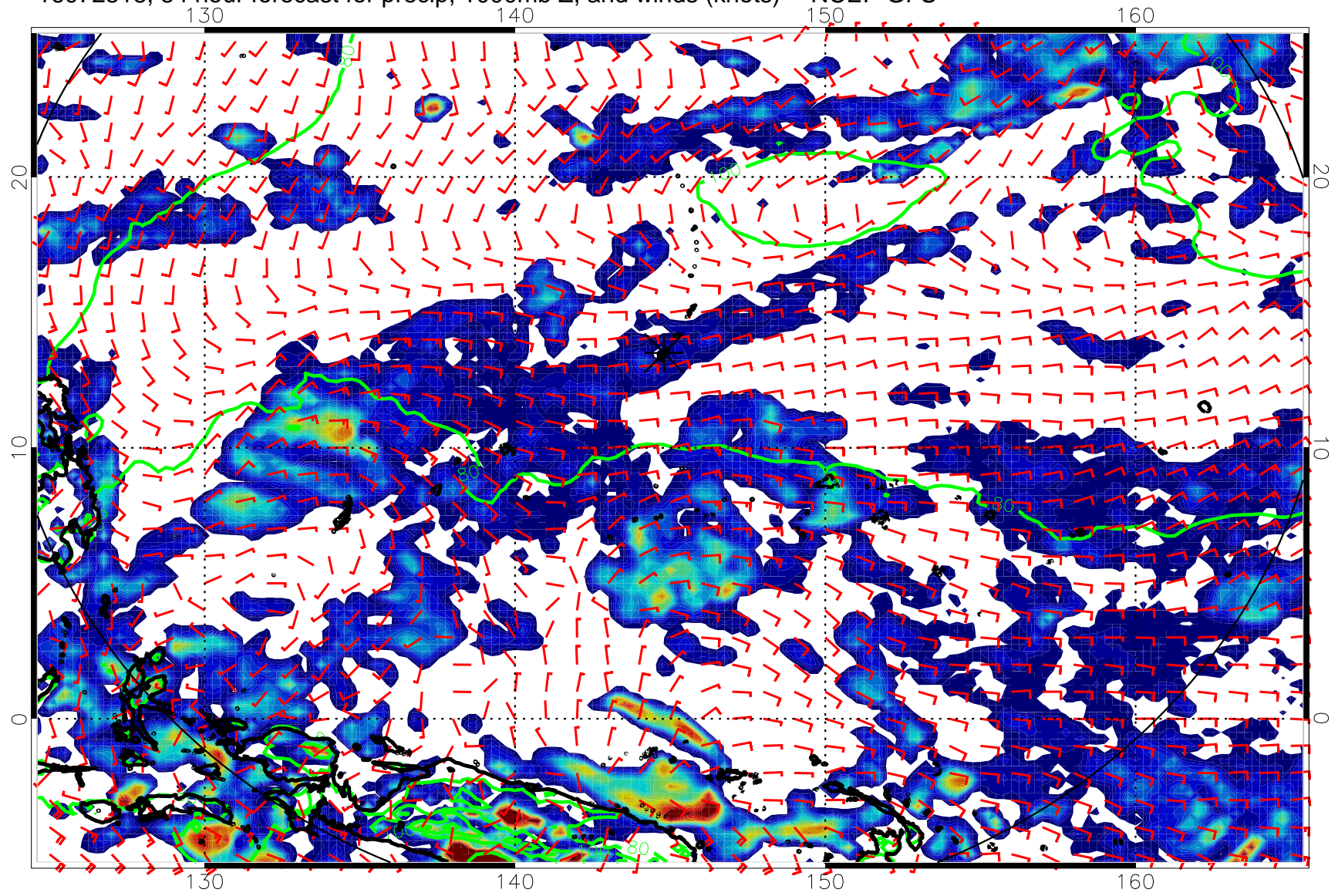
16072518, 54 hour forecast for precip, 1000mb Z, and winds (knots) -- NCEP GFS
