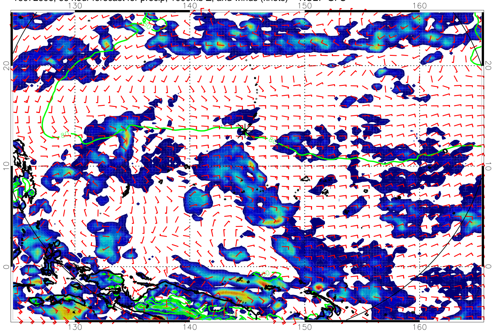
16072606, 66 hour forecast for precip, 1000mb Z, and winds (knots) -- NCEP GFS
