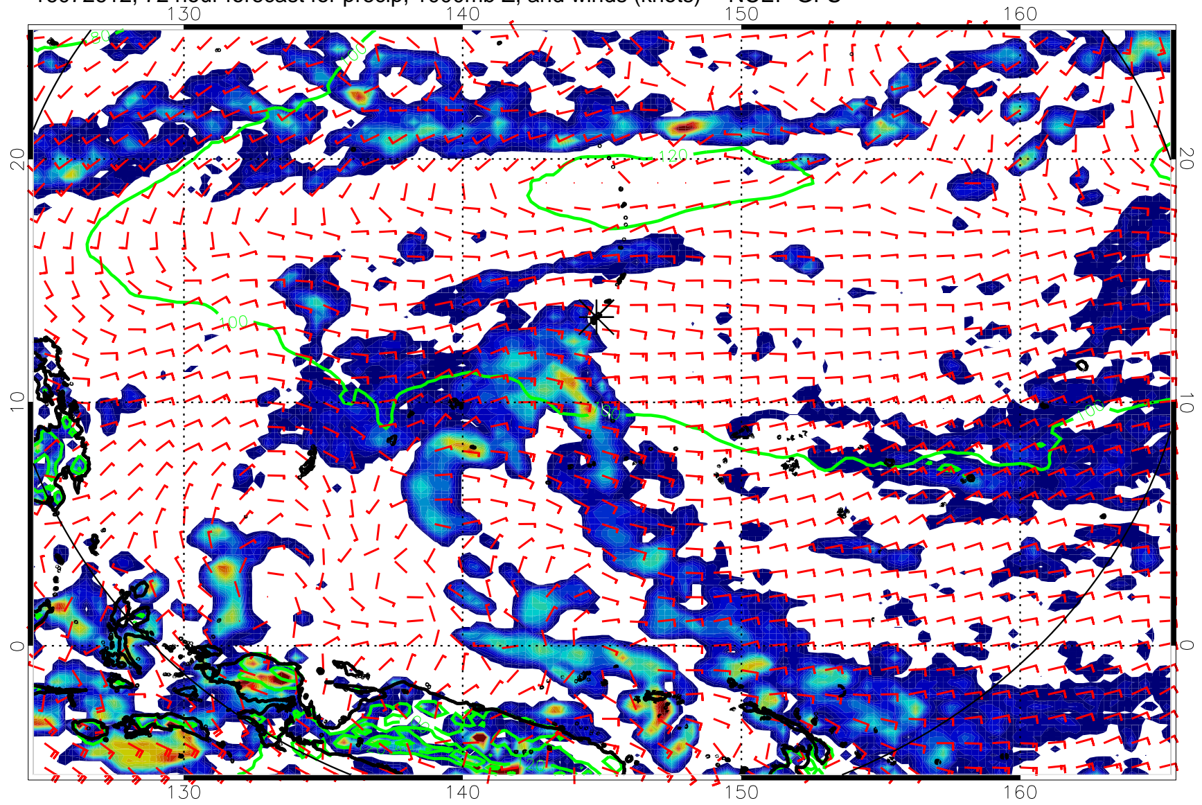
16072612, 72 hour forecast for precip, 1000mb Z, and winds (knots) -- NCEP GFS
