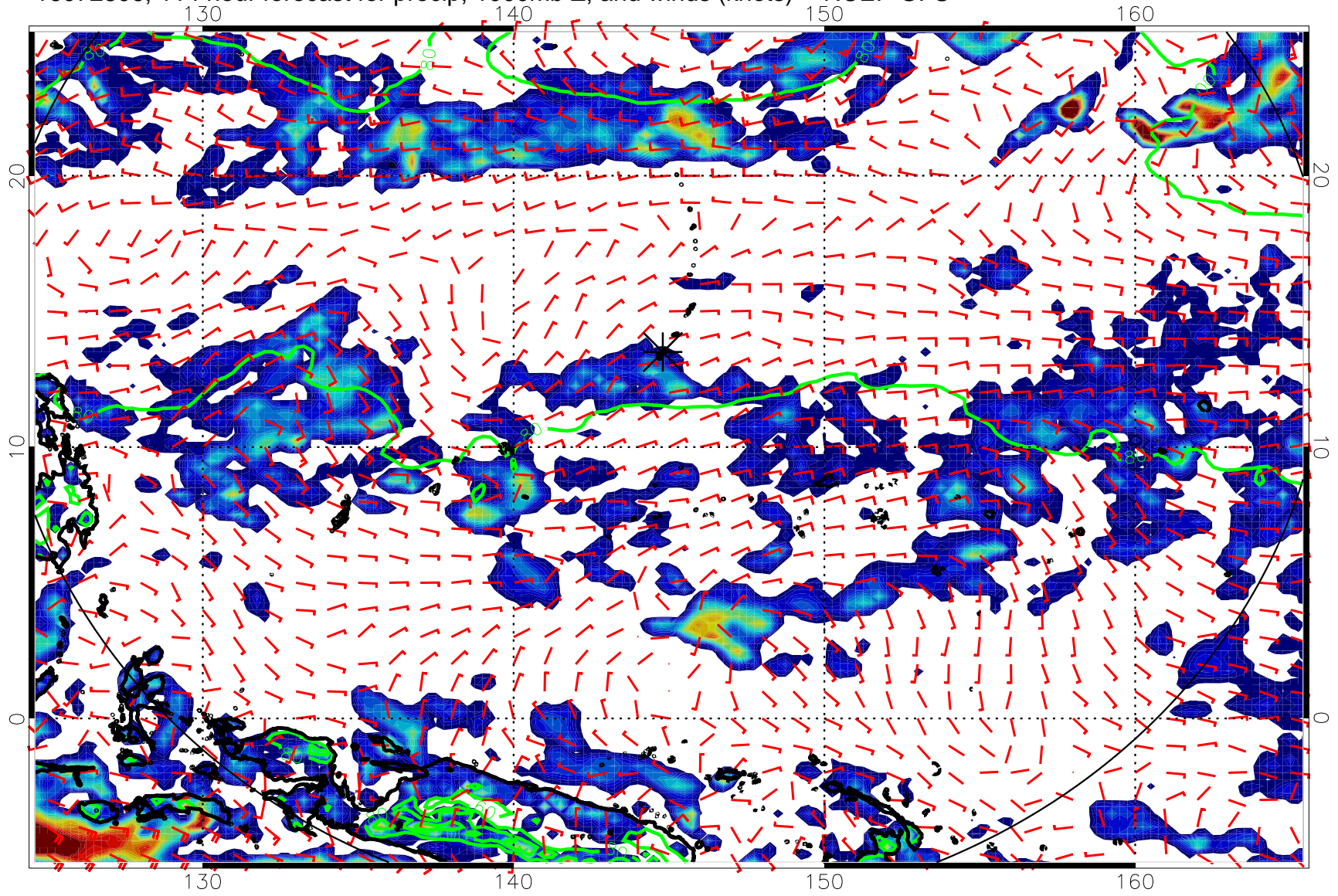
16072806, 114 hour forecast for precip, 1000mb Z, and winds (knots) -- NCEP GFS
