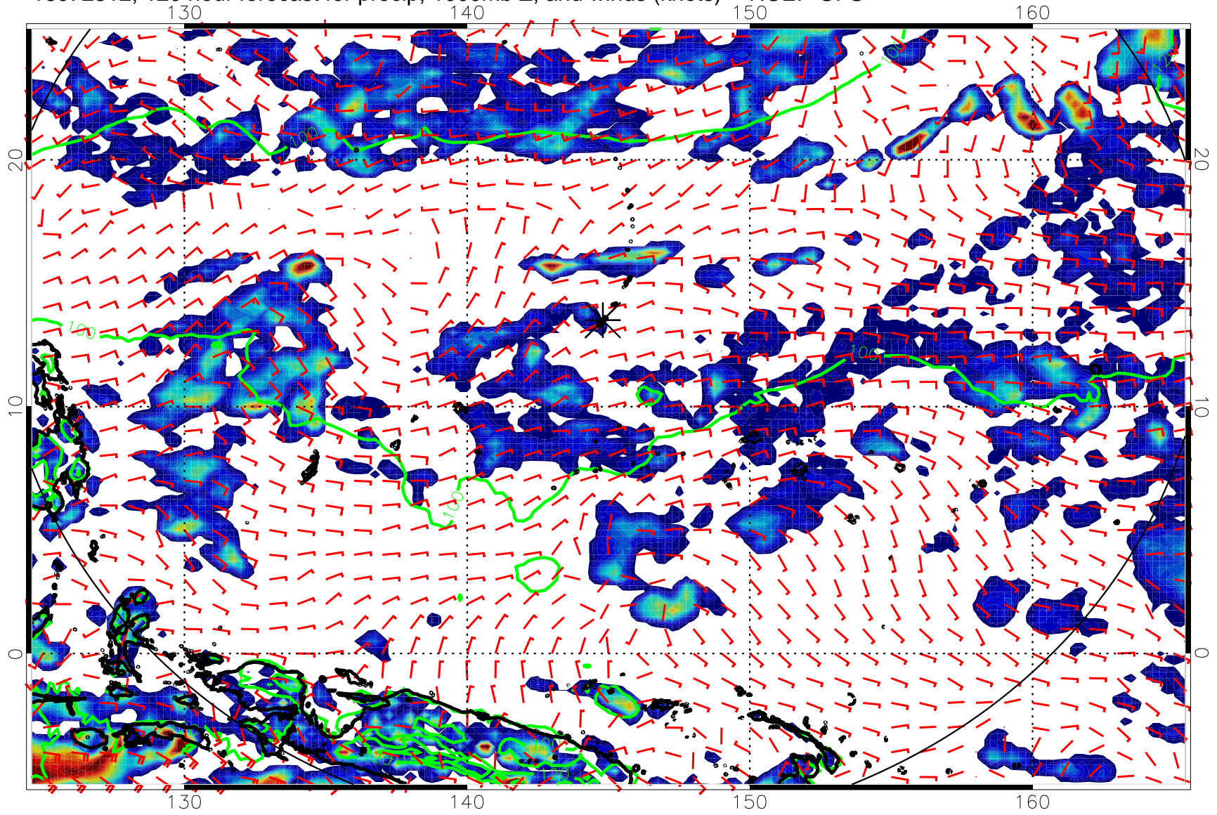
16072812, 120 hour forecast for precip, 1000mb Z, and winds (knots) -- NCEP GFS
