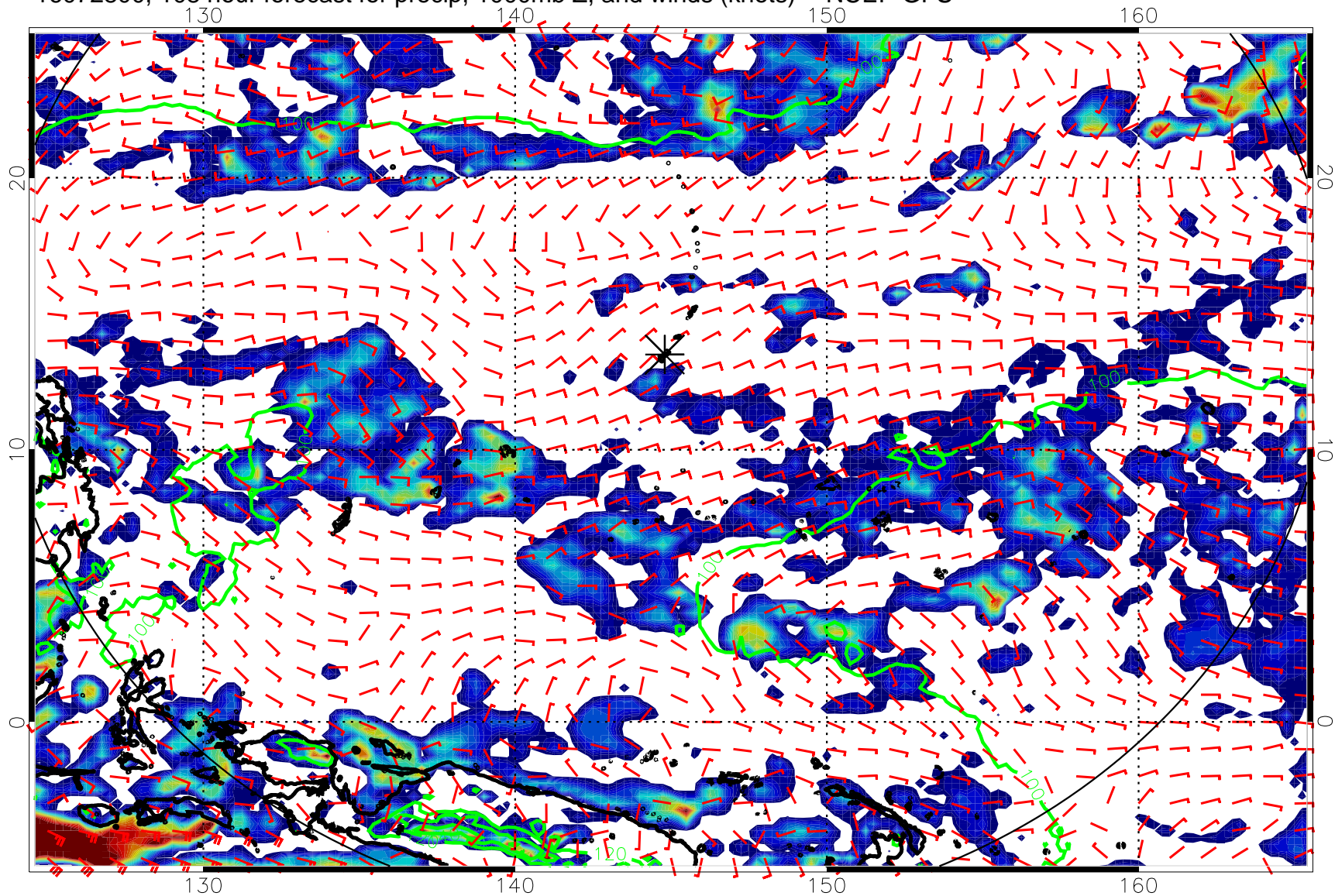
16072800, 108 hour forecast for precip, 1000mb Z, and winds (knots) -- NCEP GFS
