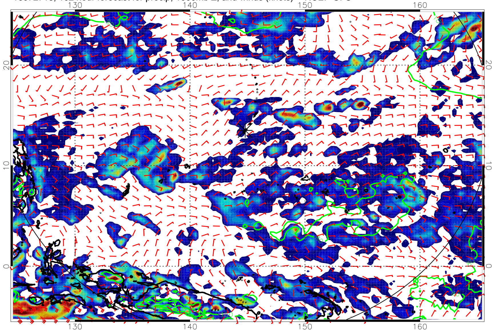
16072718, 102 hour forecast for precip, 1000mb Z, and winds (knots) -- NCEP GFS
