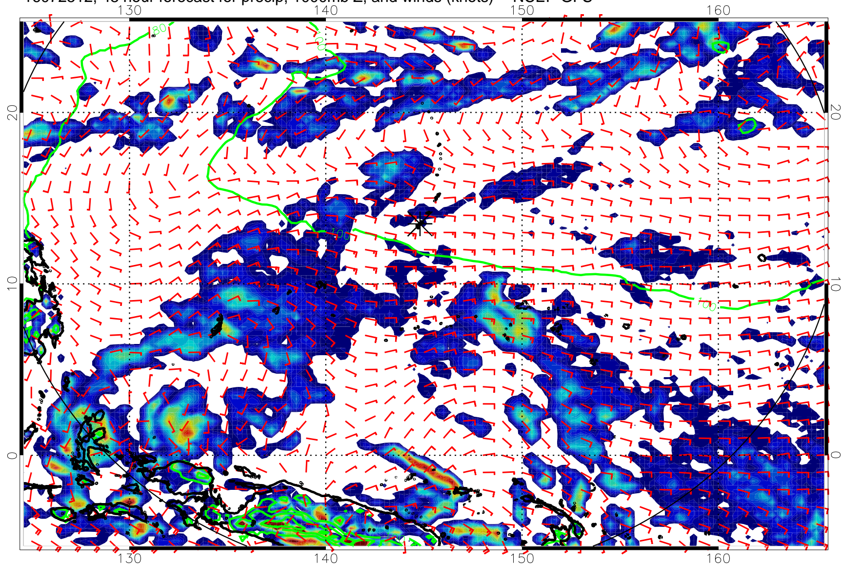
16072512, 48 hour forecast for precip, 1000mb Z, and winds (knots) -- NCEP GFS
