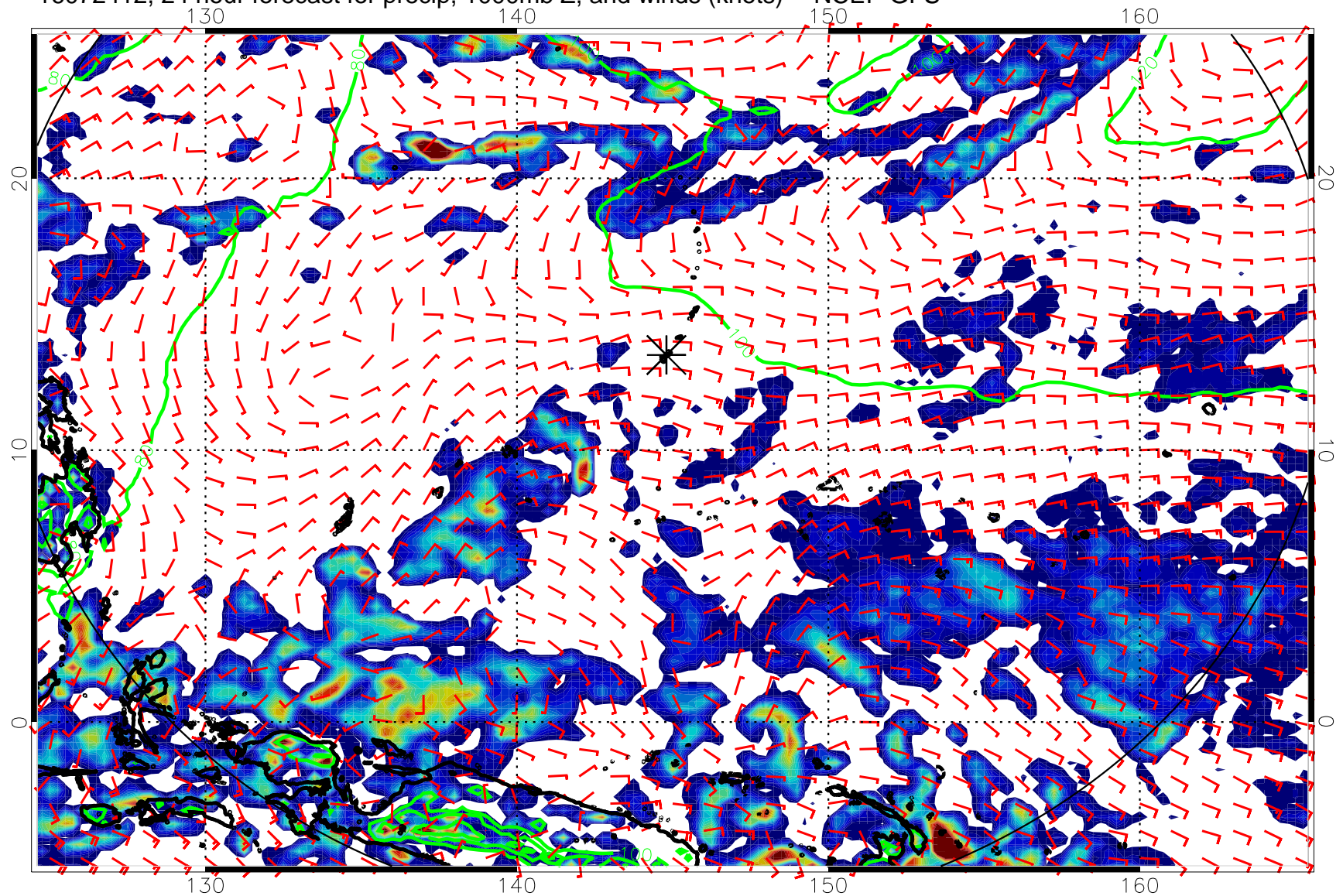
16072412, 24 hour forecast for precip, 1000mb Z, and winds (knots) -- NCEP GFS
