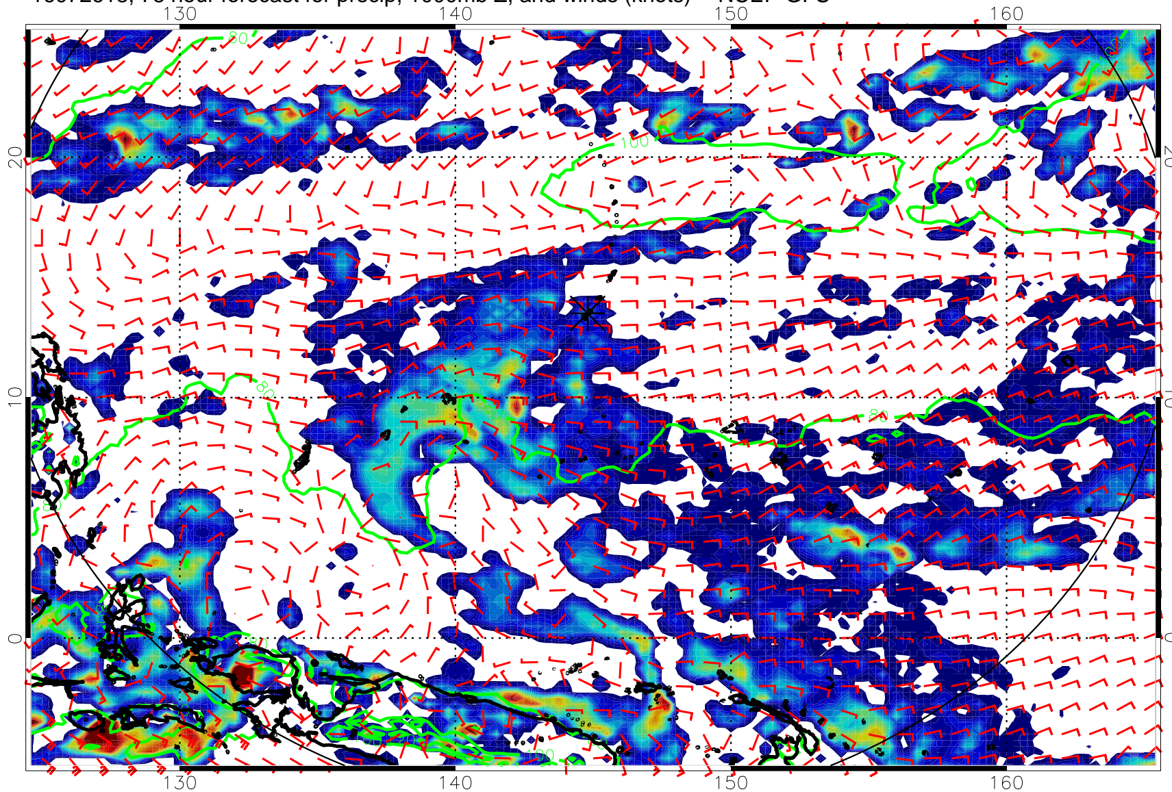
16072618, 78 hour forecast for precip, 1000mb Z, and winds (knots) -- NCEP GFS
