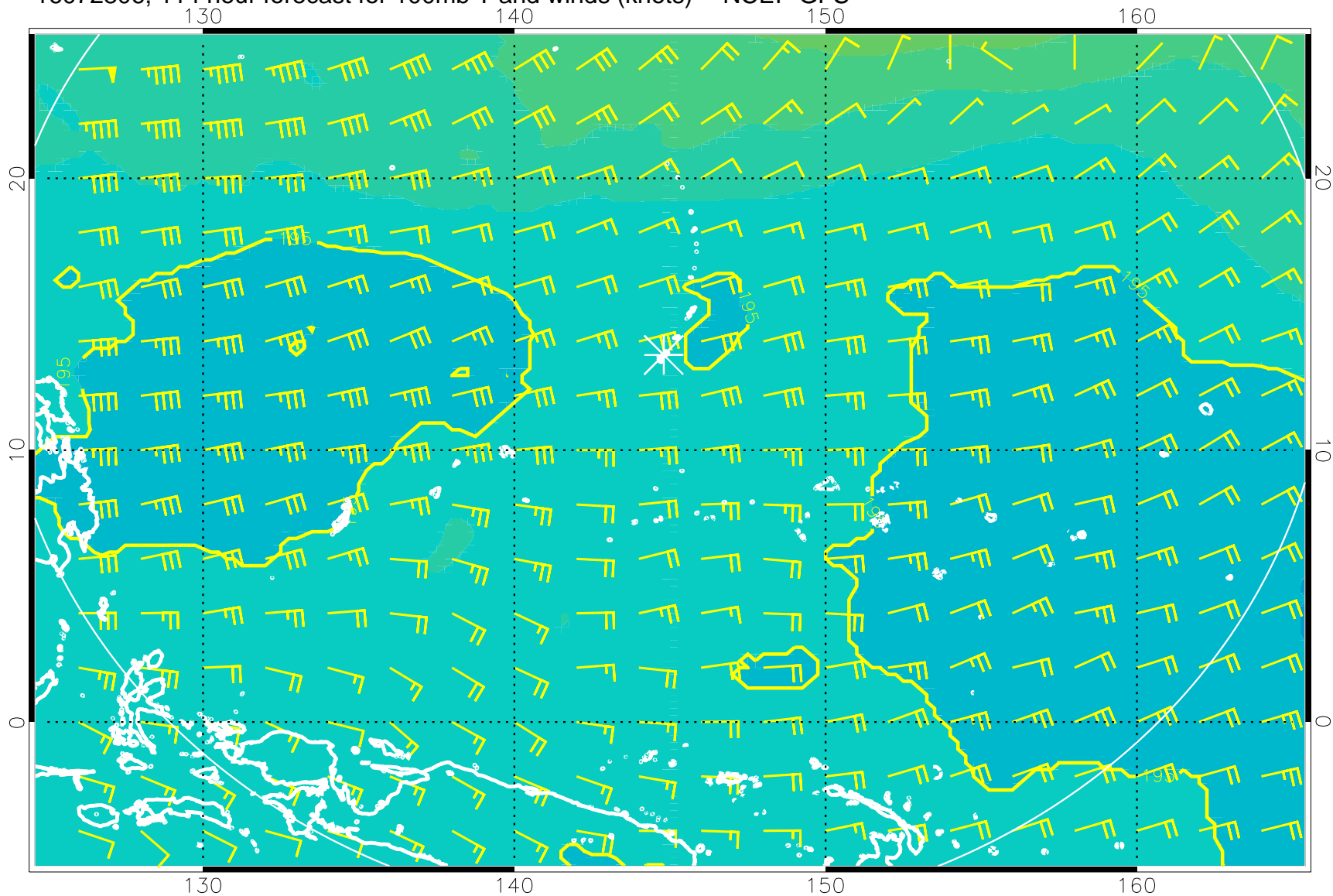
16072806, 114 hour forecast for 100mb T and winds (knots) -- NCEP GFS
