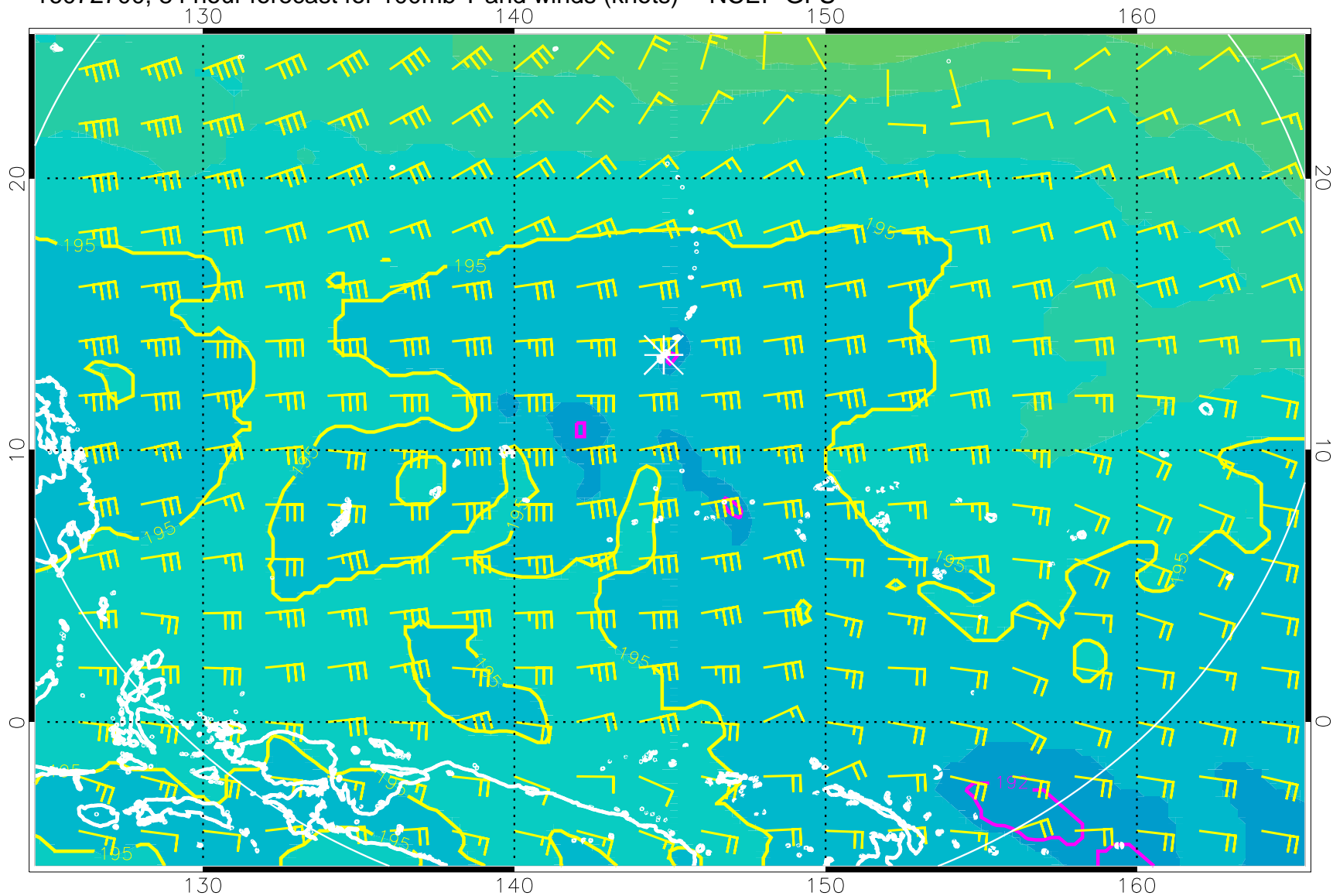
16072700, 84 hour forecast for 100mb T and winds (knots) -- NCEP GFS
