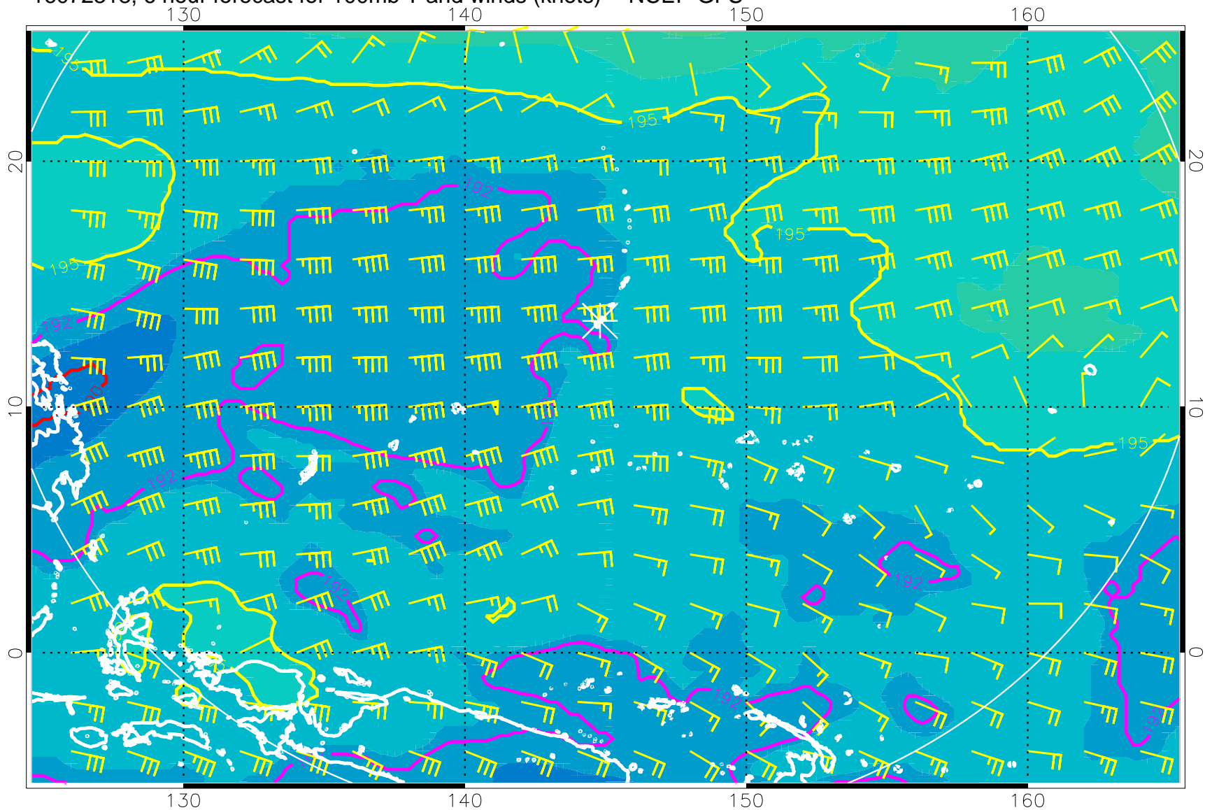
16072318, 6 hour forecast for 100mb T and winds (knots) -- NCEP GFS
