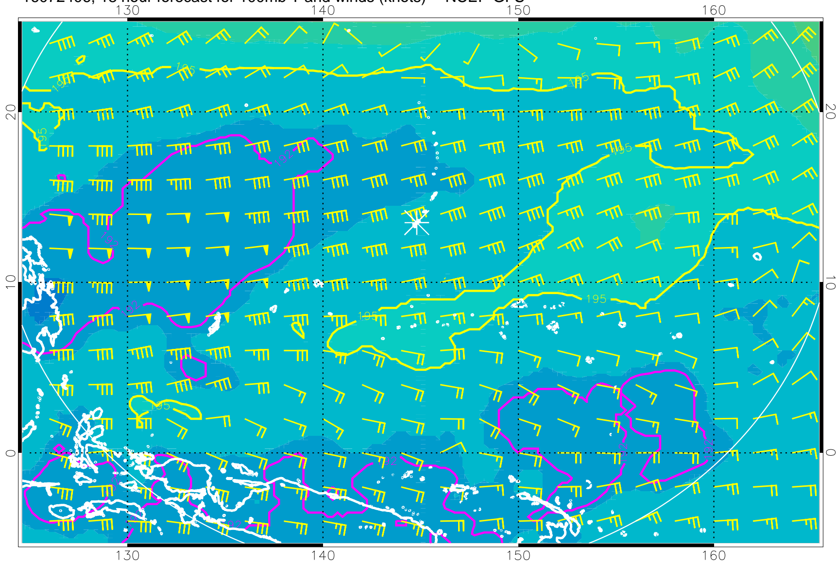
16072406, 18 hour forecast for 100mb T and winds (knots) -- NCEP GFS
