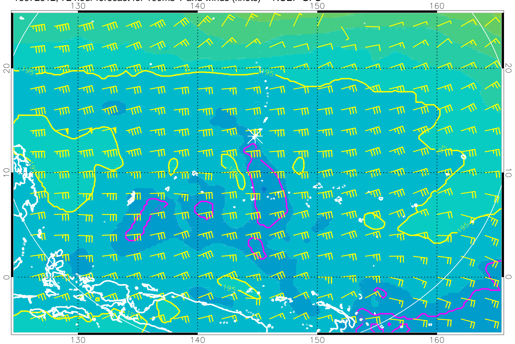
16072612, 72 hour forecast for 100mb T and winds (knots) -- NCEP GFS
