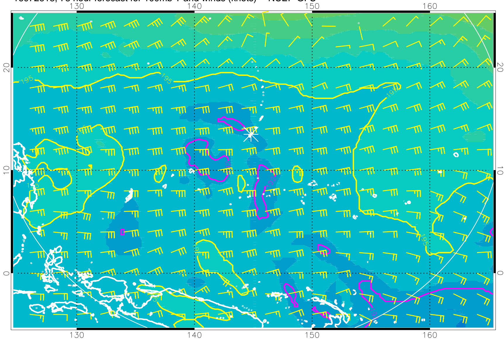
16072618, 78 hour forecast for 100mb T and winds (knots) -- NCEP GFS
