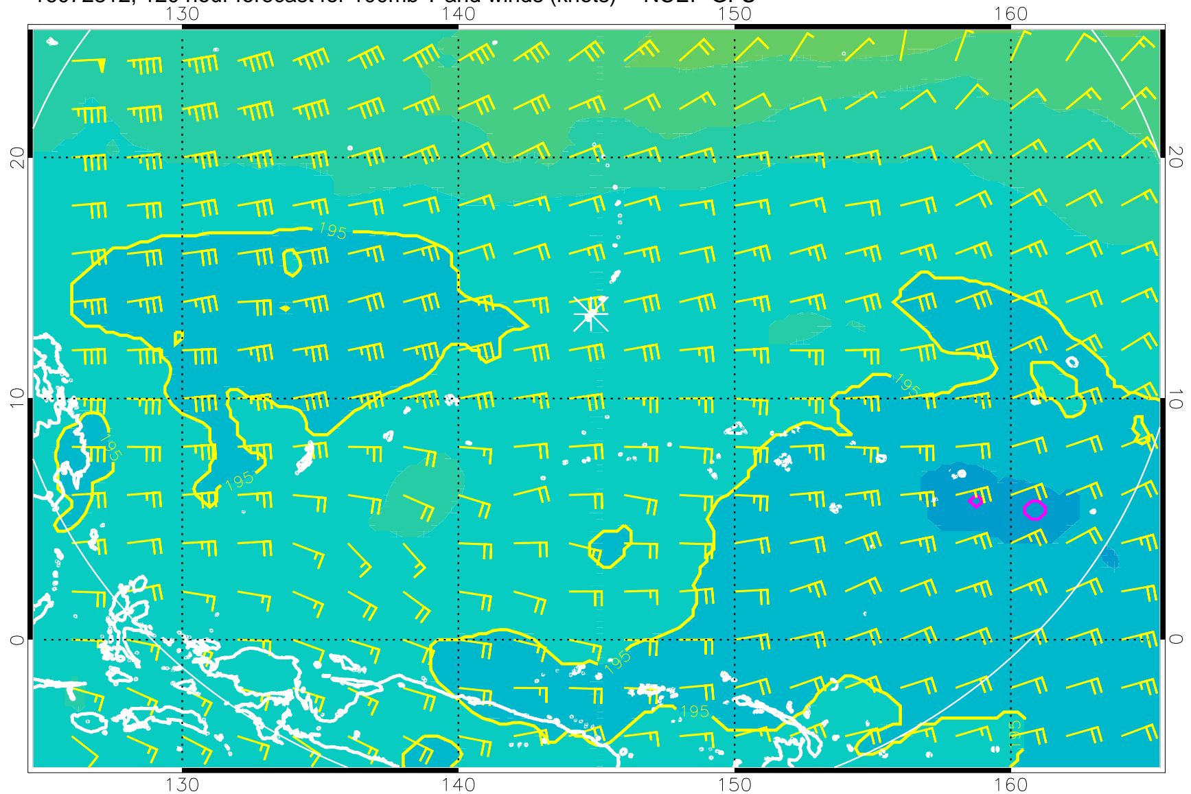
16072812, 120 hour forecast for 100mb T and winds (knots) -- NCEP GFS
