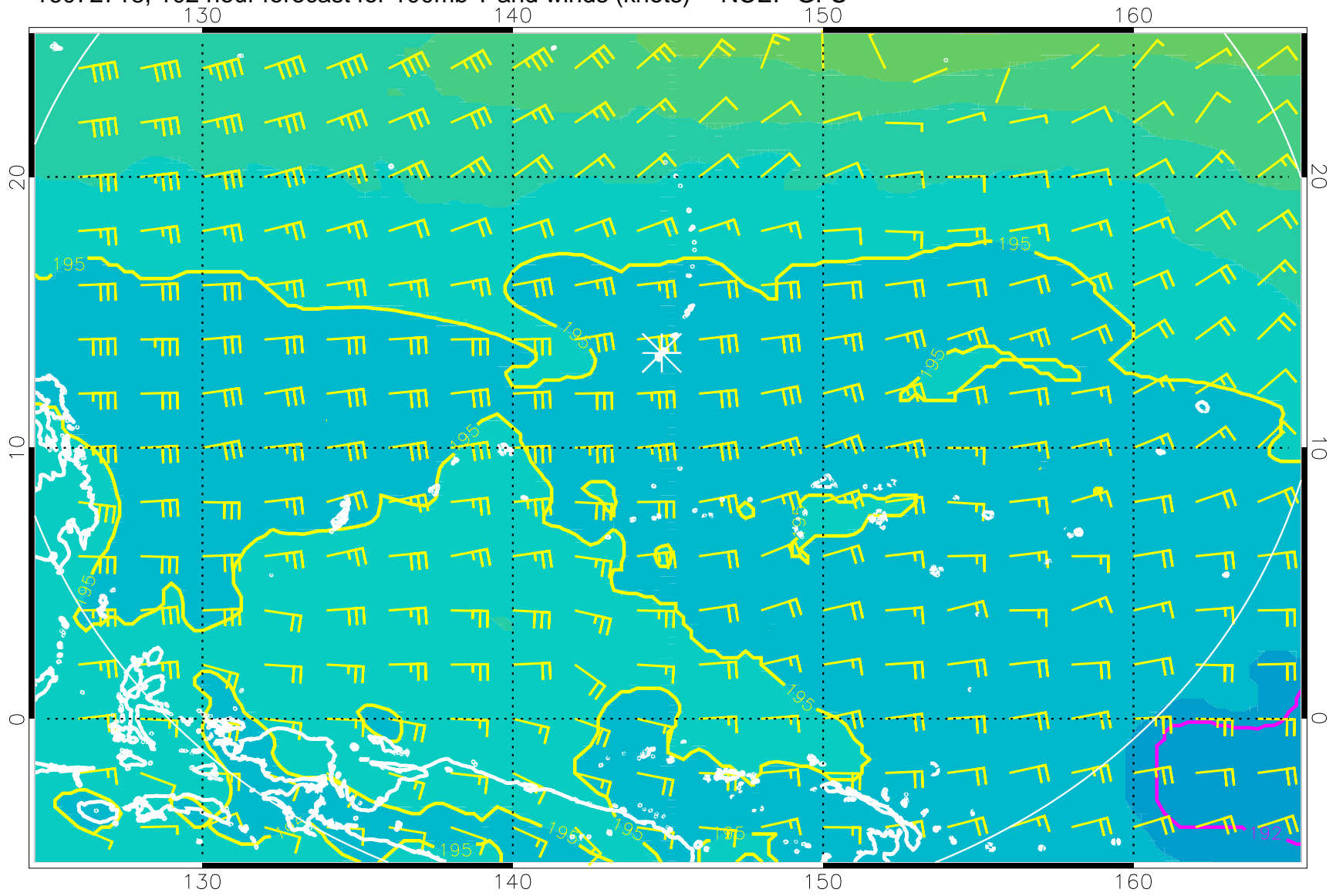
16072718, 102 hour forecast for 100mb T and winds (knots) -- NCEP GFS
