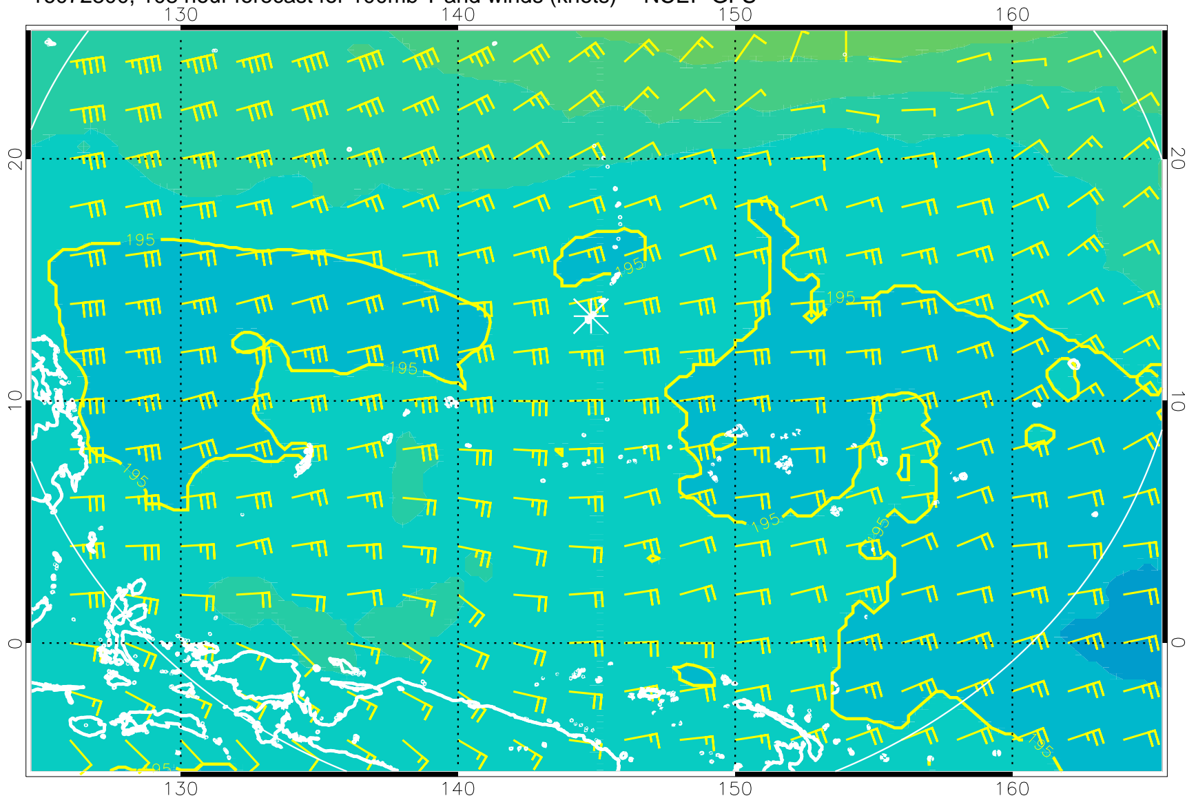
16072800, 108 hour forecast for 100mb T and winds (knots) -- NCEP GFS
