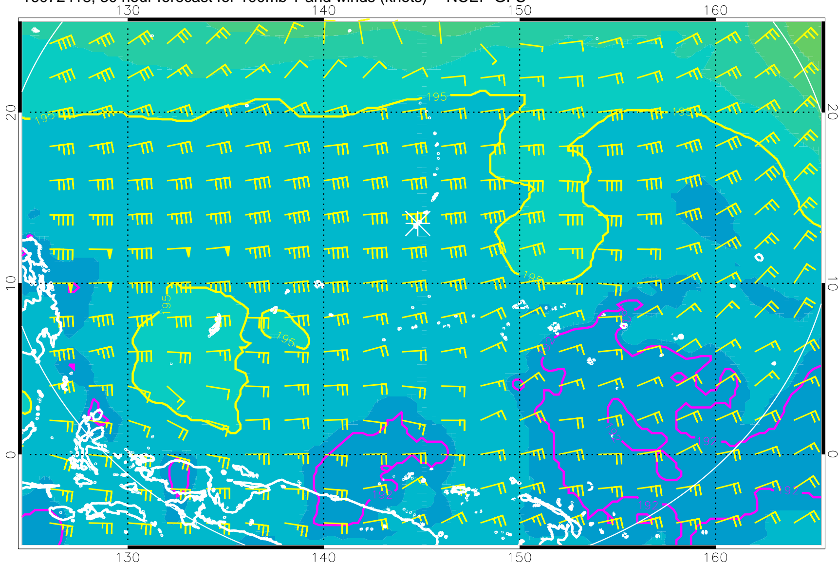
16072418, 30 hour forecast for 100mb T and winds (knots) -- NCEP GFS
