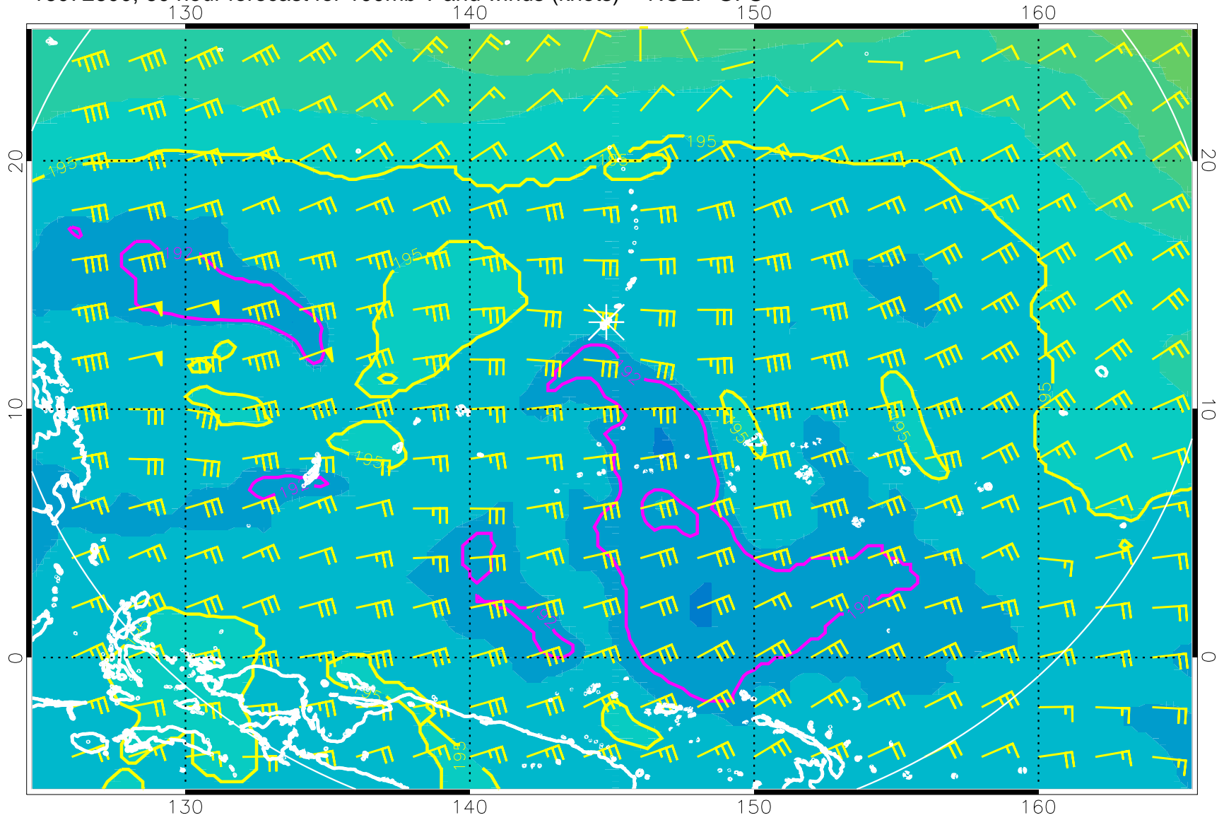
16072600, 60 hour forecast for 100mb T and winds (knots) -- NCEP GFS
