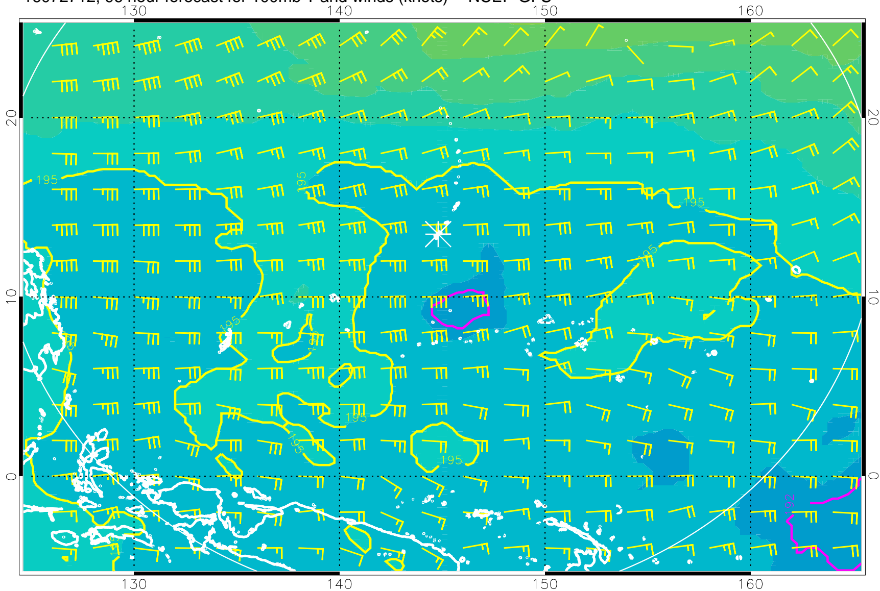
16072712, 96 hour forecast for 100mb T and winds (knots) -- NCEP GFS
