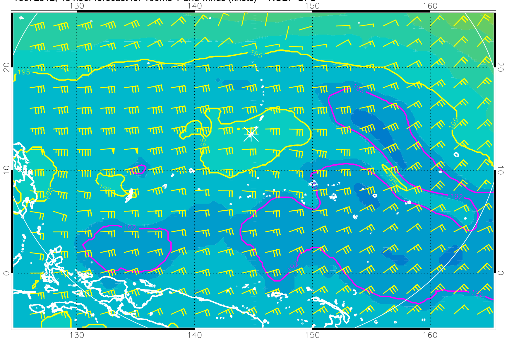
16072512, 48 hour forecast for 100mb T and winds (knots) -- NCEP GFS
