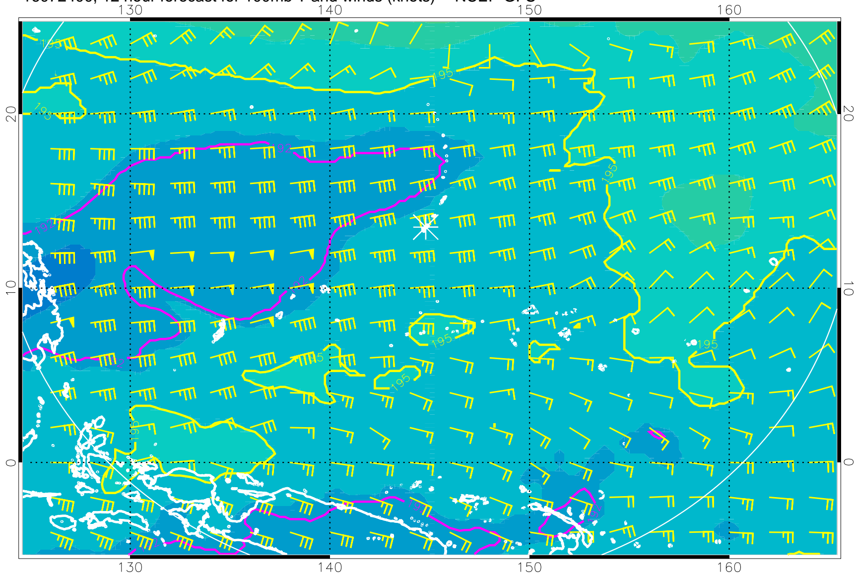
16072400, 12 hour forecast for 100mb T and winds (knots) -- NCEP GFS
