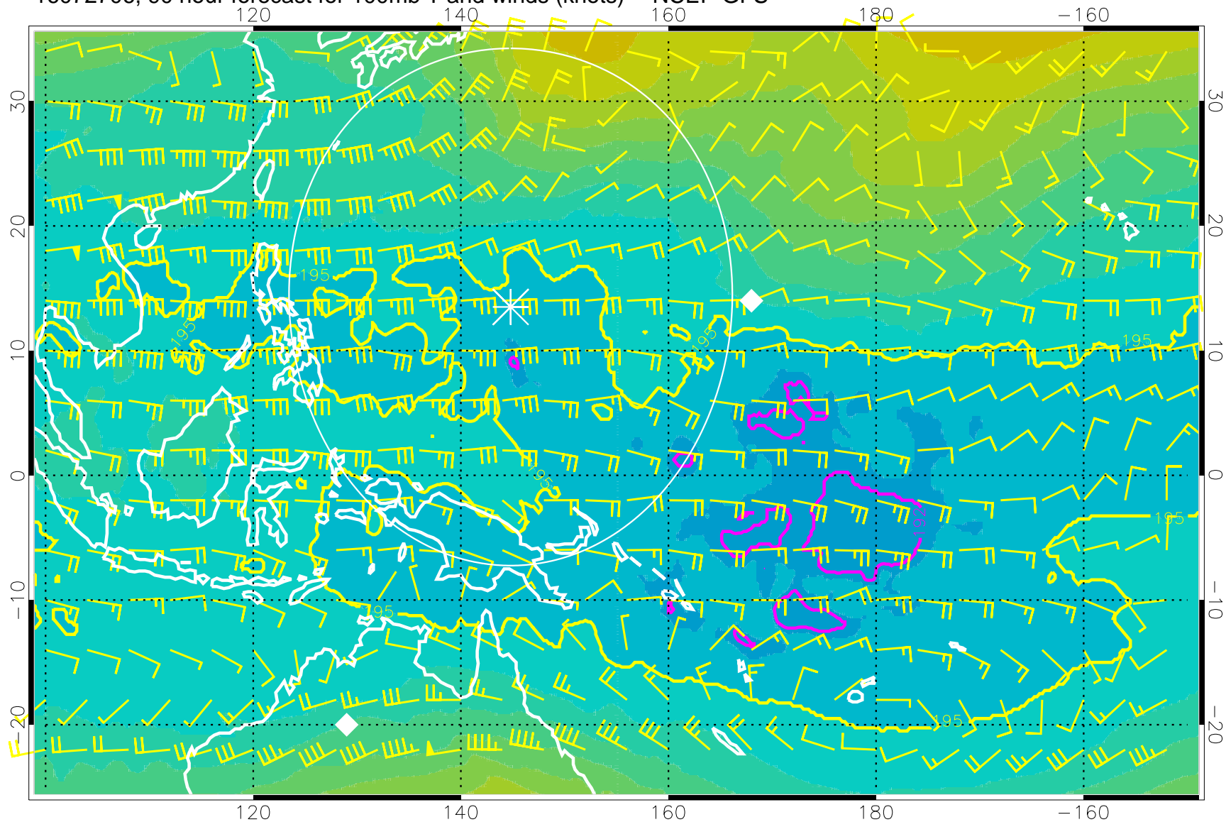
16072706, 90 hour forecast for 100mb T and winds (knots) -- NCEP GFS
