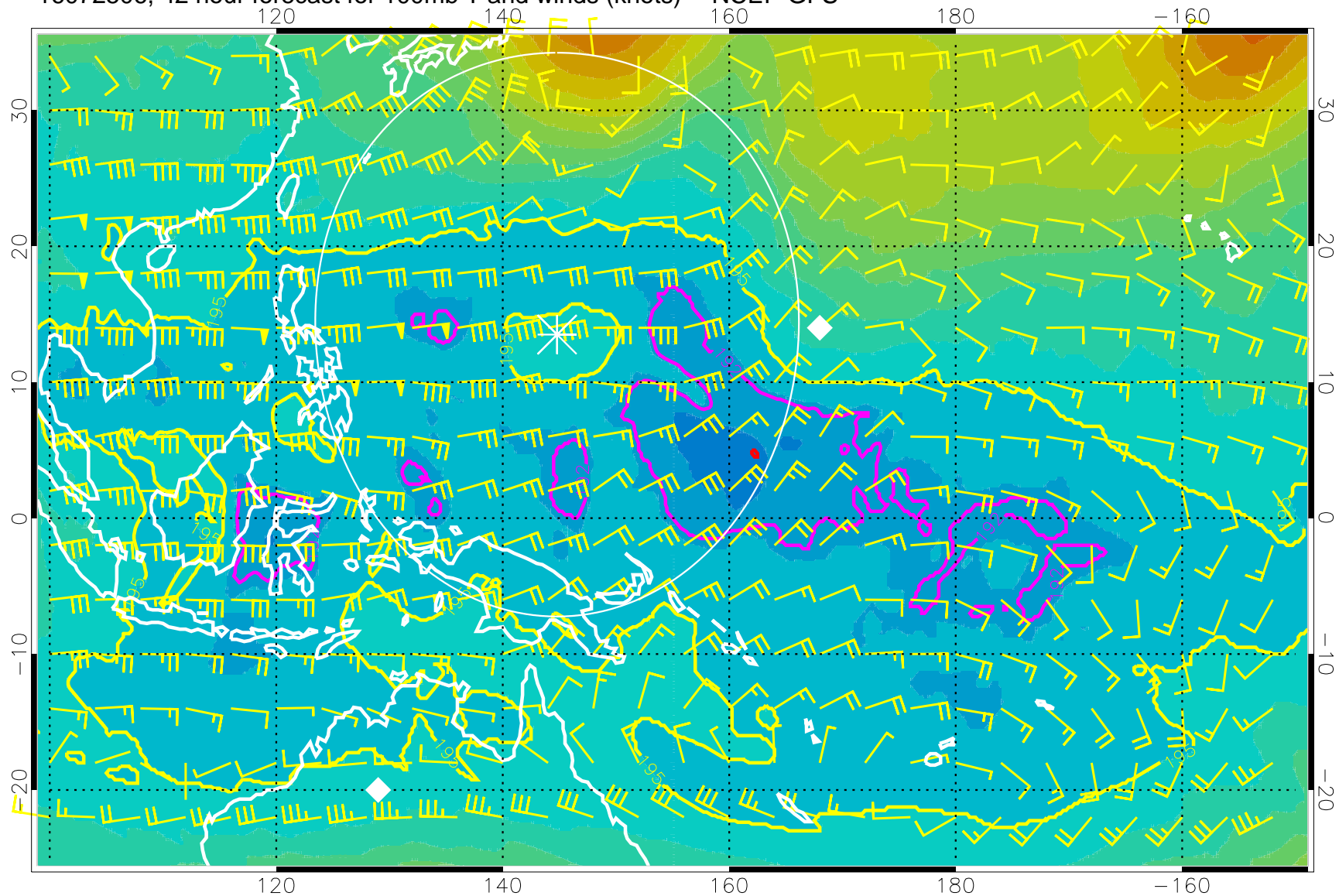
16072506, 42 hour forecast for 100mb T and winds (knots) -- NCEP GFS
