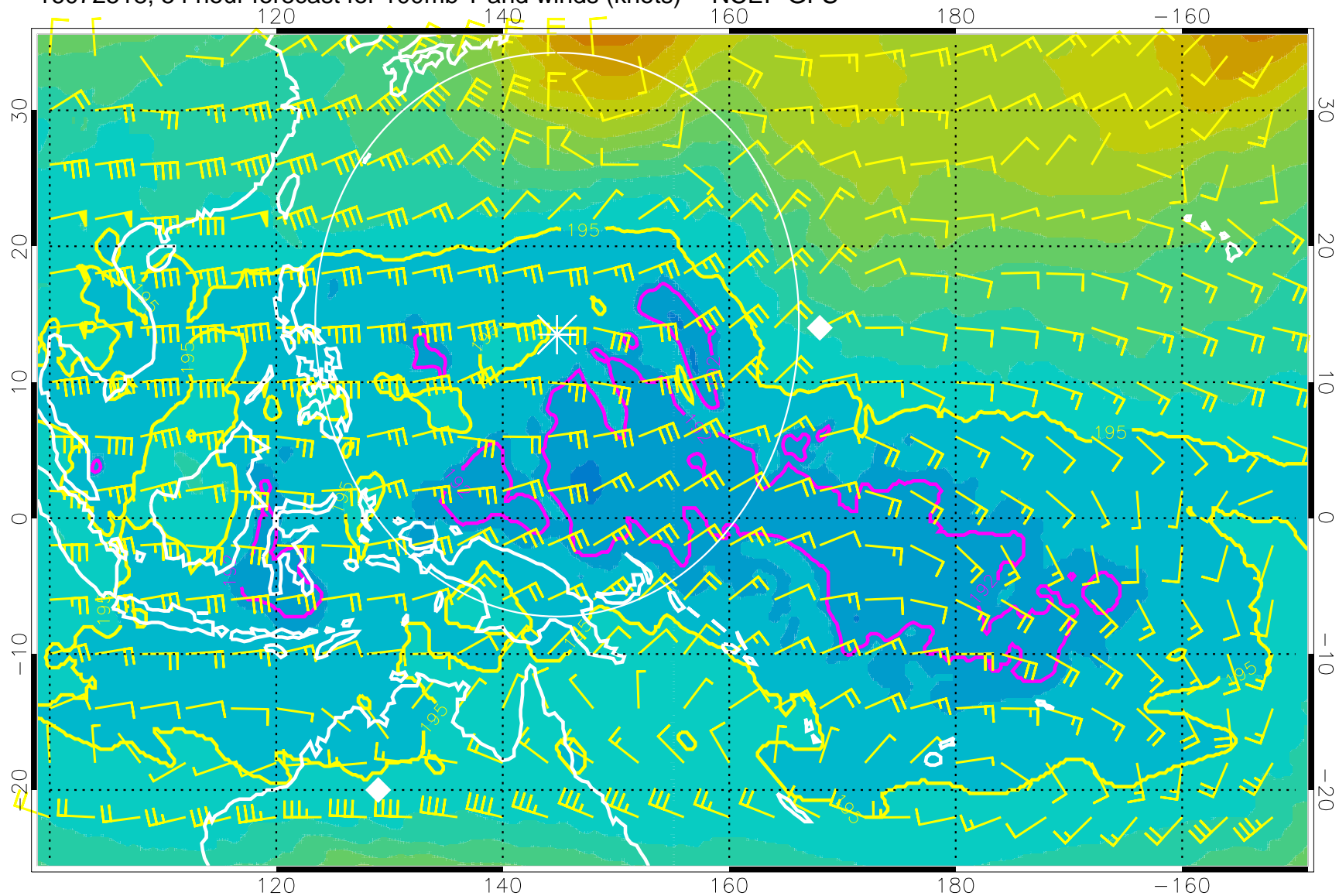
16072518, 54 hour forecast for 100mb T and winds (knots) -- NCEP GFS
