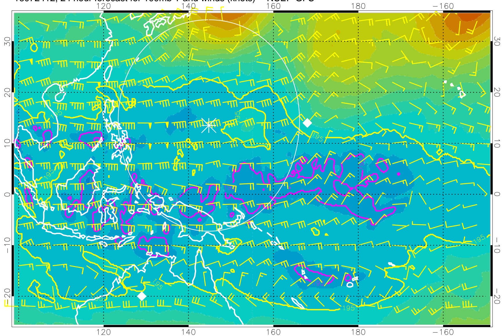
16072412, 24 hour forecast for 100mb T and winds (knots) -- NCEP GFS
