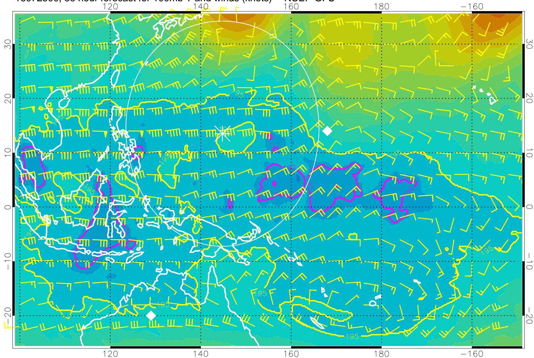
16072500, 36 hour forecast for 100mb T and winds (knots) -- NCEP GFS
