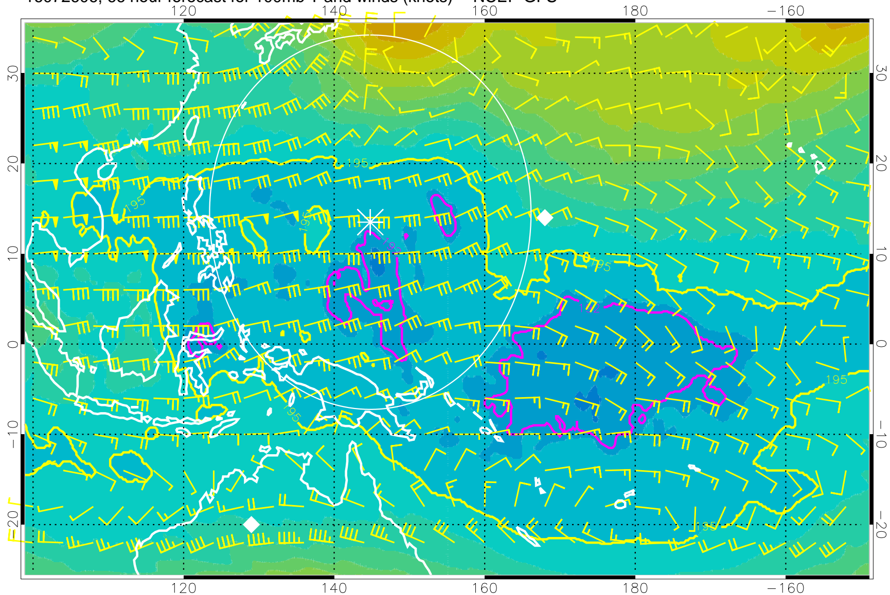
16072606, 66 hour forecast for 100mb T and winds (knots) -- NCEP GFS
