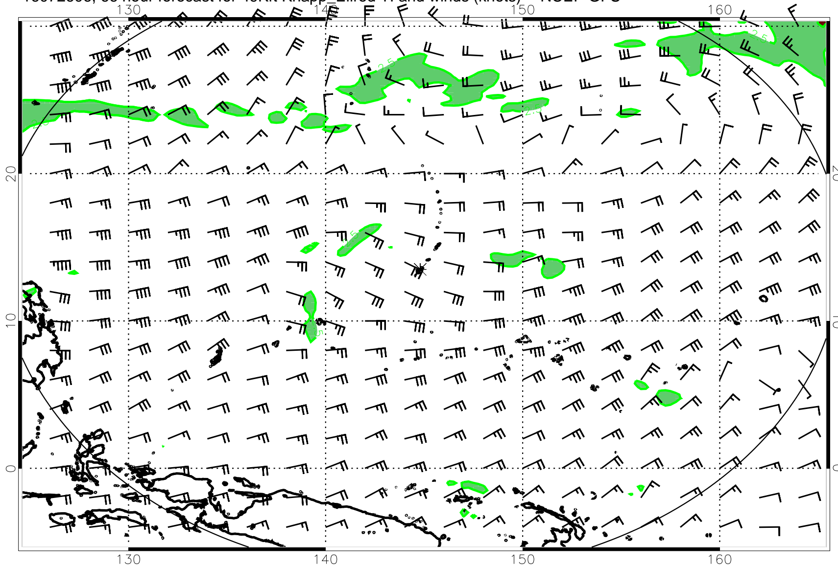
16072606, 66 hour forecast for 49Kft Knapp_Ellrod TI and winds (knots) -- NCEP GFS
