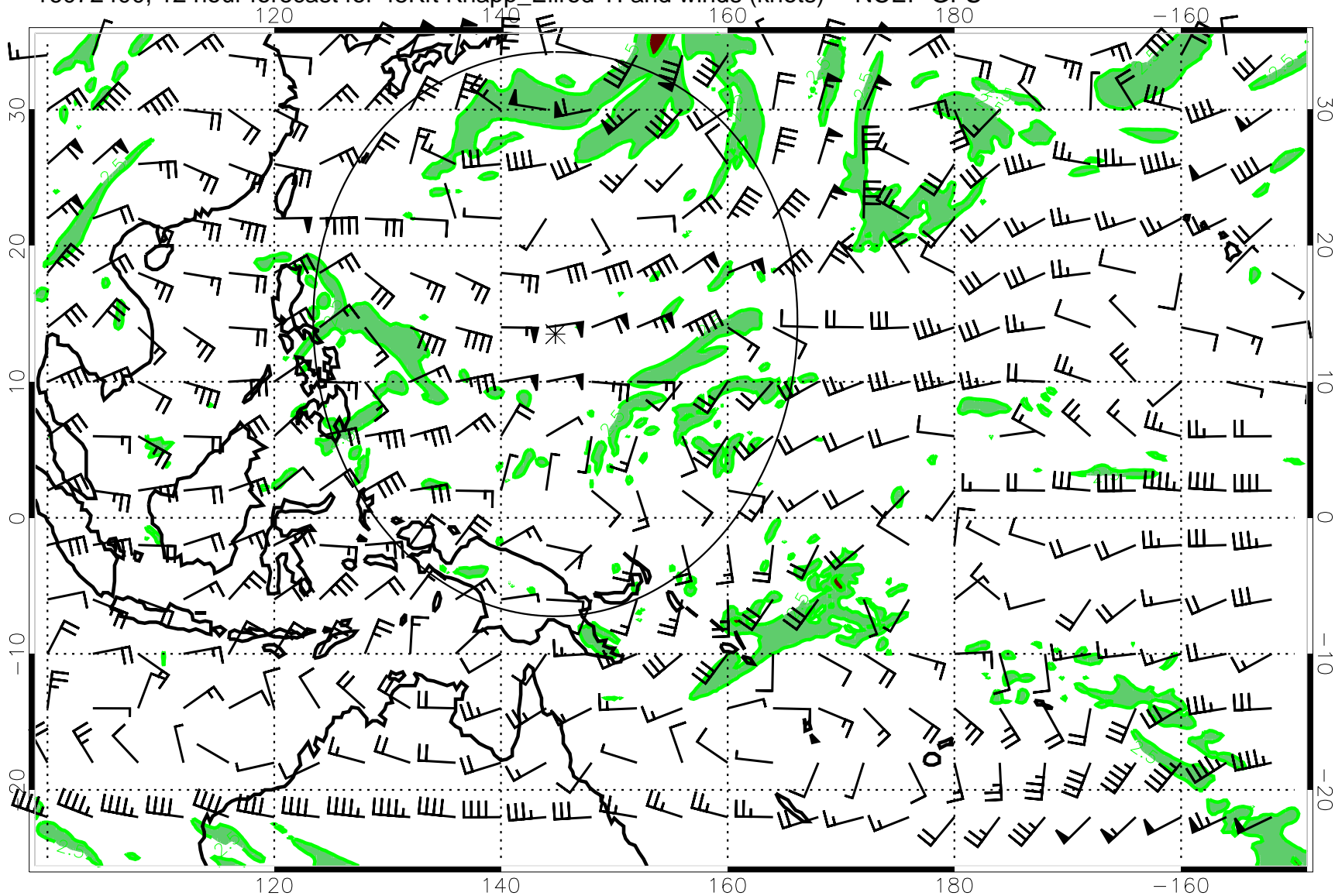
16072400, 12 hour forecast for 45Kft Knapp_Ellrod TI and winds (knots) -- NCEP GFS
