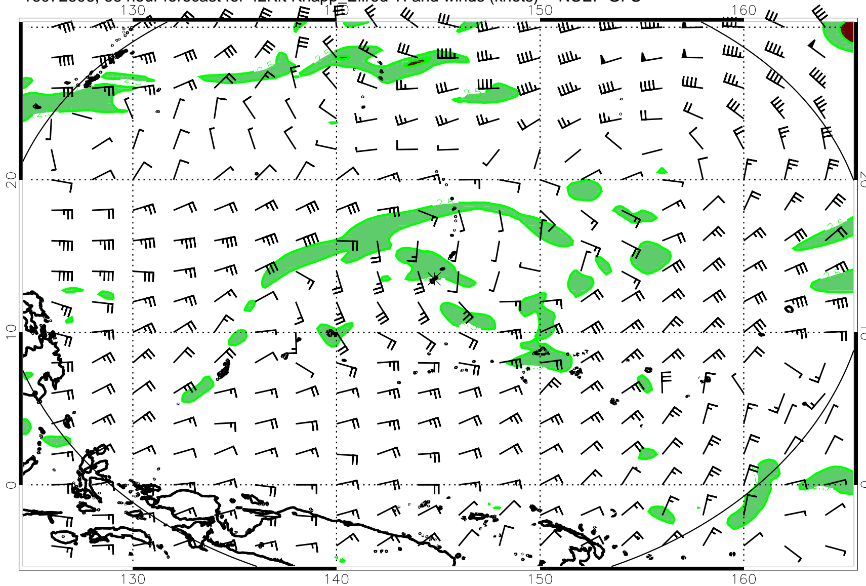
16072606, 66 hour forecast for 42Kft Knapp_Ellrod TI and winds (knots) -- NCEP GFS
