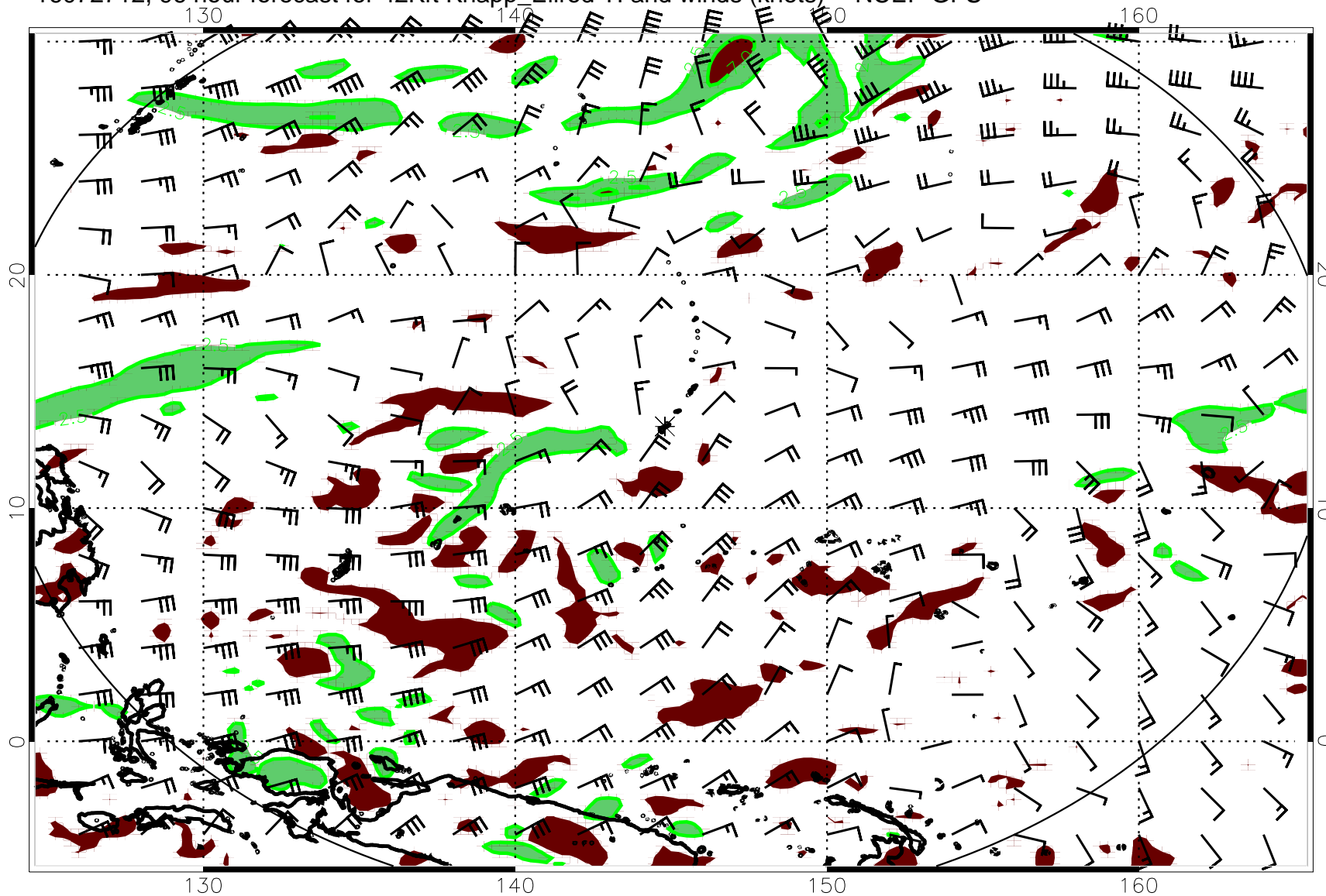
16072712, 96 hour forecast for 42Kft Knapp Ellrod TI and winds (knots) -- NCEP GFS
