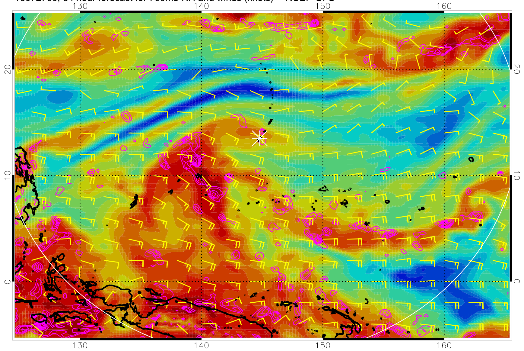
16072700, 84 hour forecast for 700mb RH and winds (knots) -- NCEP GFS
