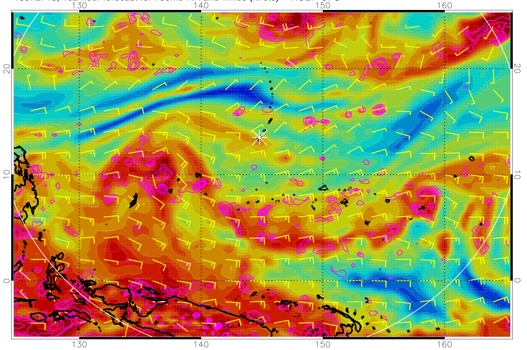
16072718, 102 hour forecast for 700mb RH and winds (knots) -- NCEP GFS
