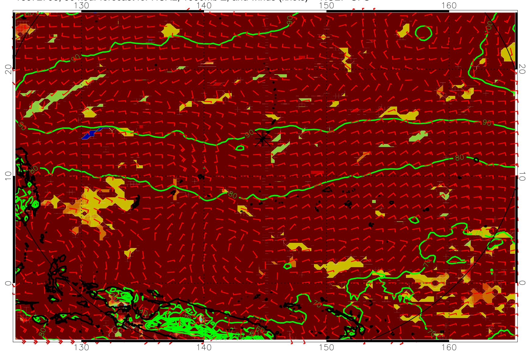
16072706, 90 hour forecast for HCAL, 1000mb Z, and winds (knots) -- NCEP GFS
