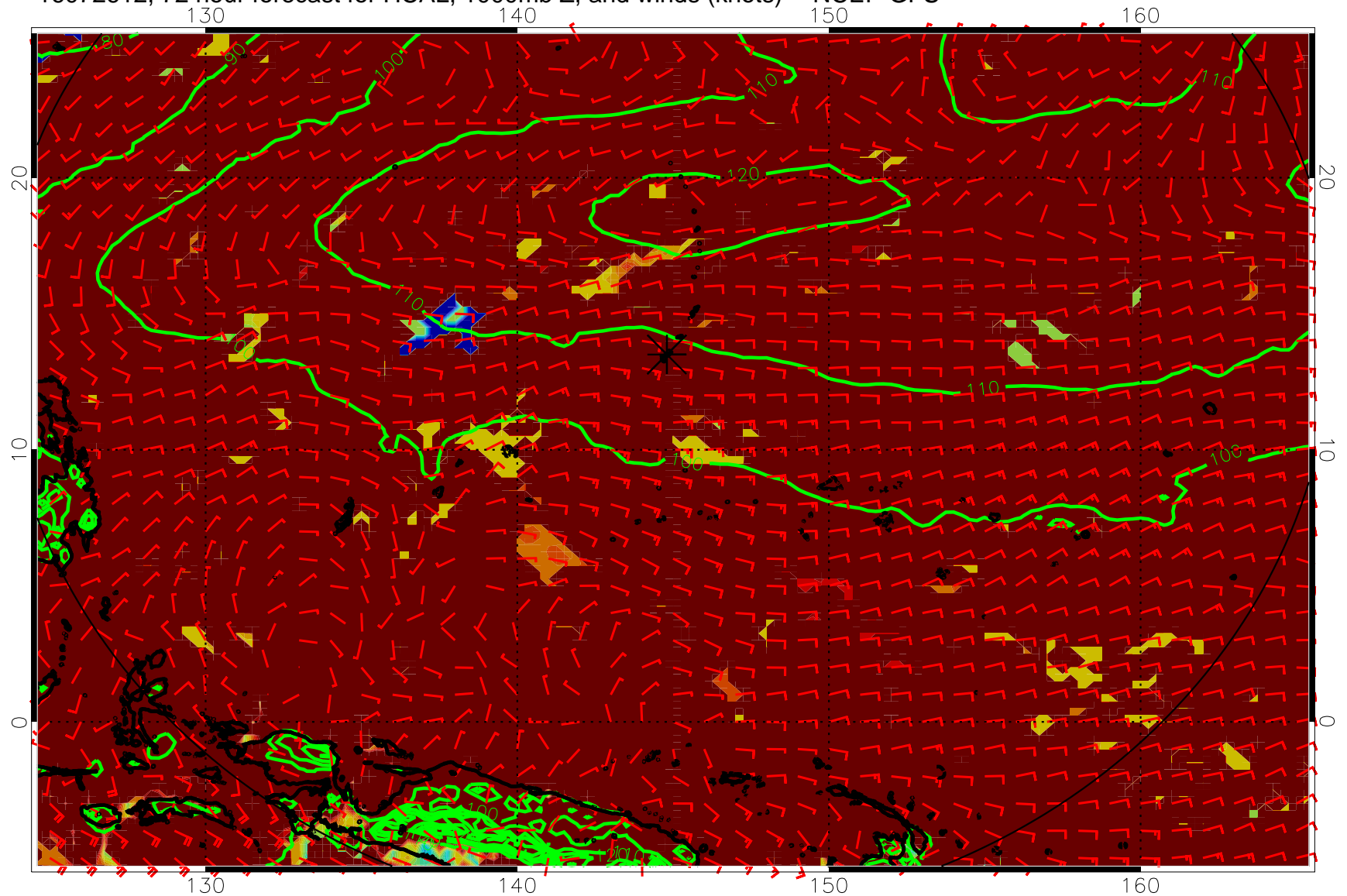
16072612, 72 hour forecast for HCAL, 1000mb Z, and winds (knots) -- NCEP GFS
