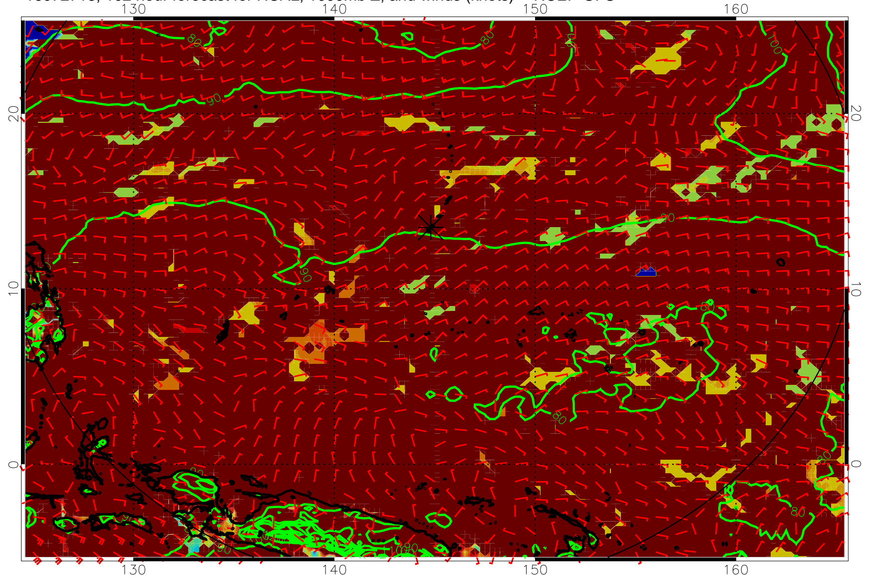
16072718, 102 hour forecast for HCAL, 1000mb Z, and winds (knots) -- NCEP GFS
