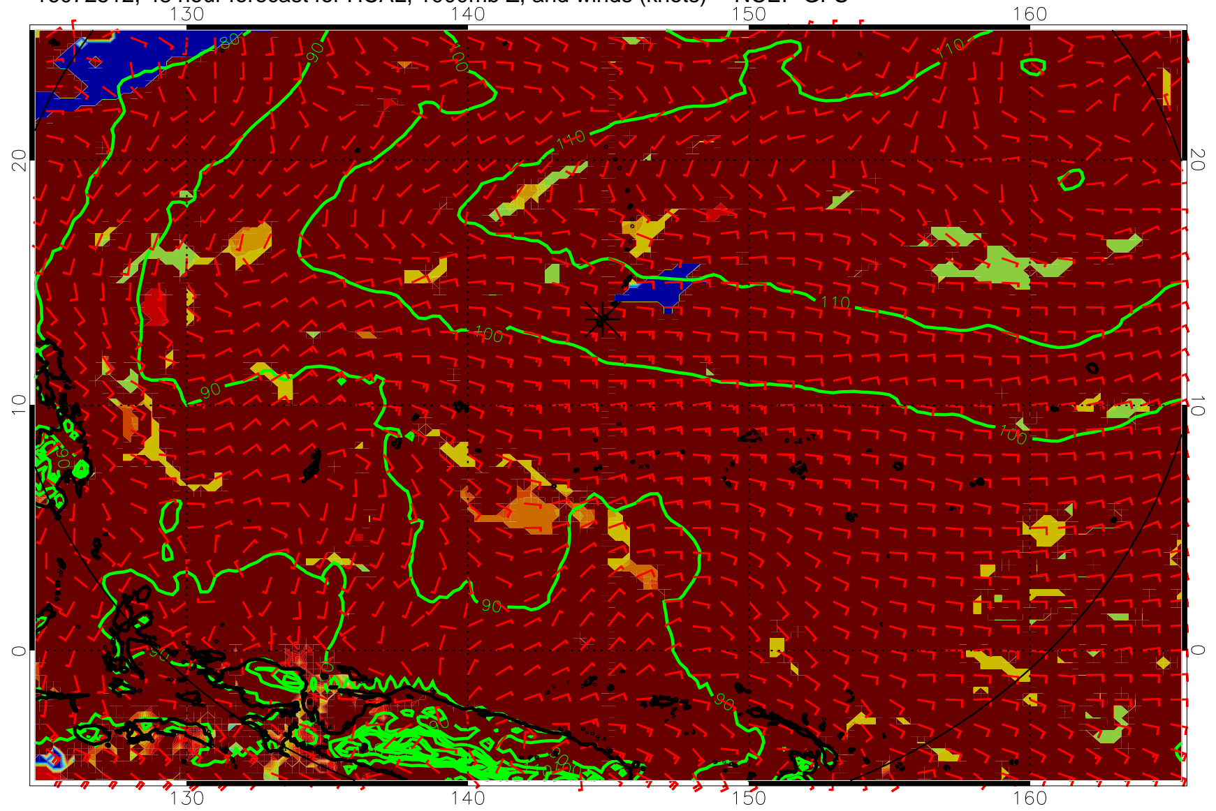
16072512, 48 hour forecast for HCAL, 1000mb Z, and winds (knots) -- NCEP GFS
