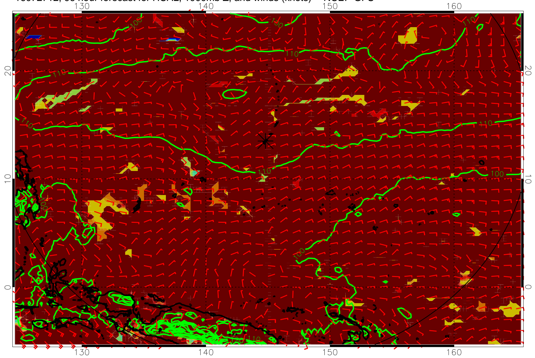
16072712, 96 hour forecast for HCAL, 1000mb Z, and winds (knots) -- NCEP GFS
