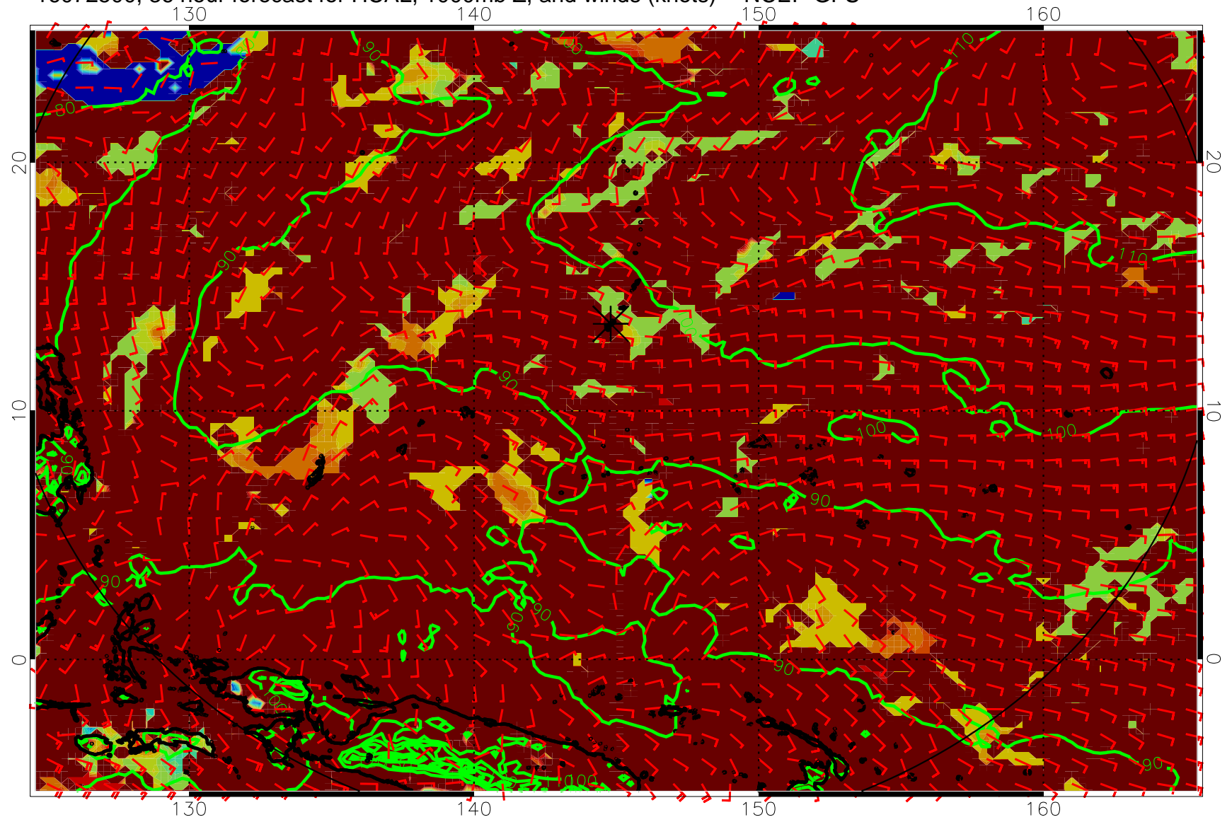
16072500, 36 hour forecast for HCAL, 1000mb Z, and winds (knots) -- NCEP GFS
