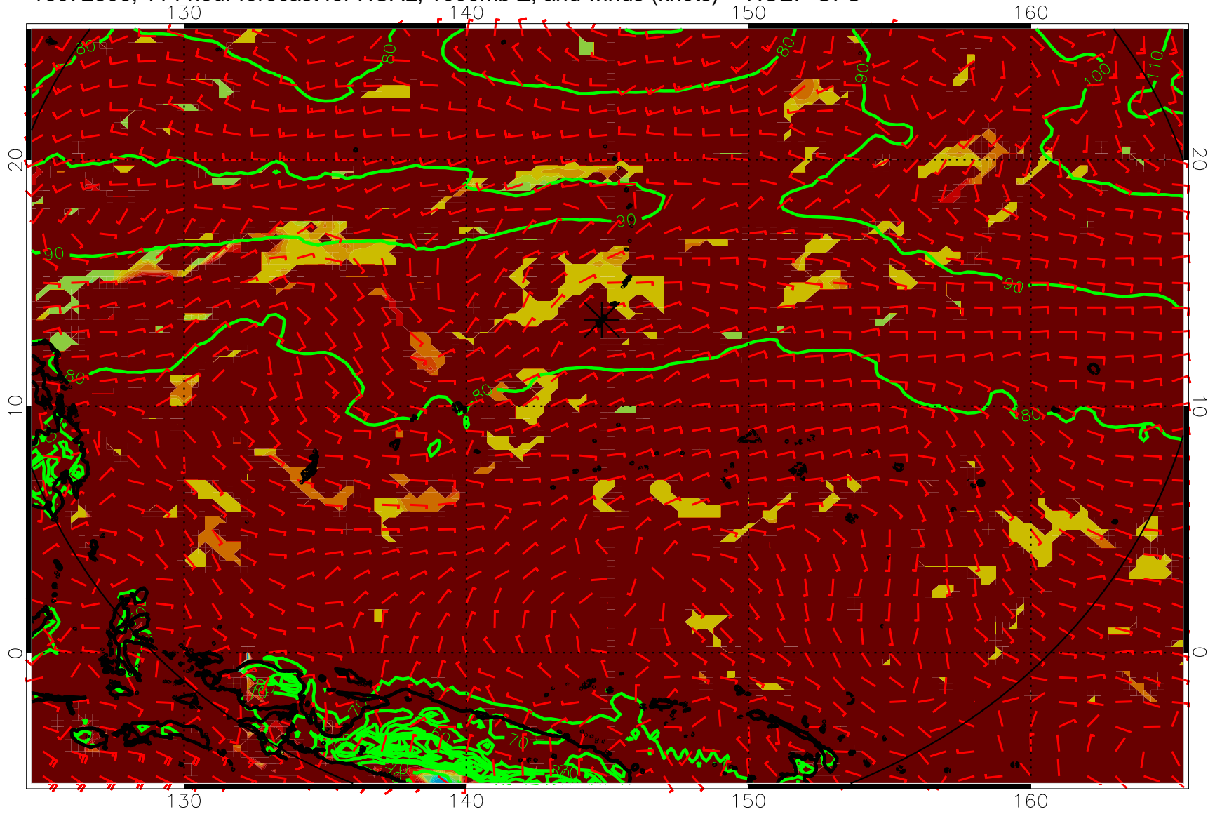
16072806, 114 hour forecast for HCAL, 1000mb Z, and winds (knots) -- NCEP GFS
