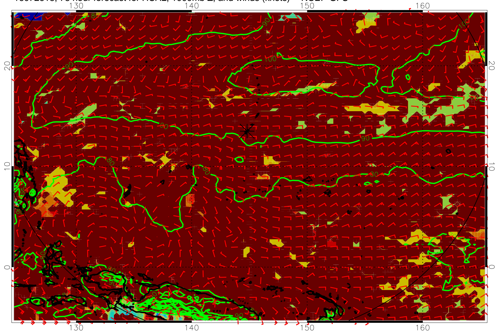
16072618, 78 hour forecast for HCAL, 1000mb Z, and winds (knots) -- NCEP GFS
