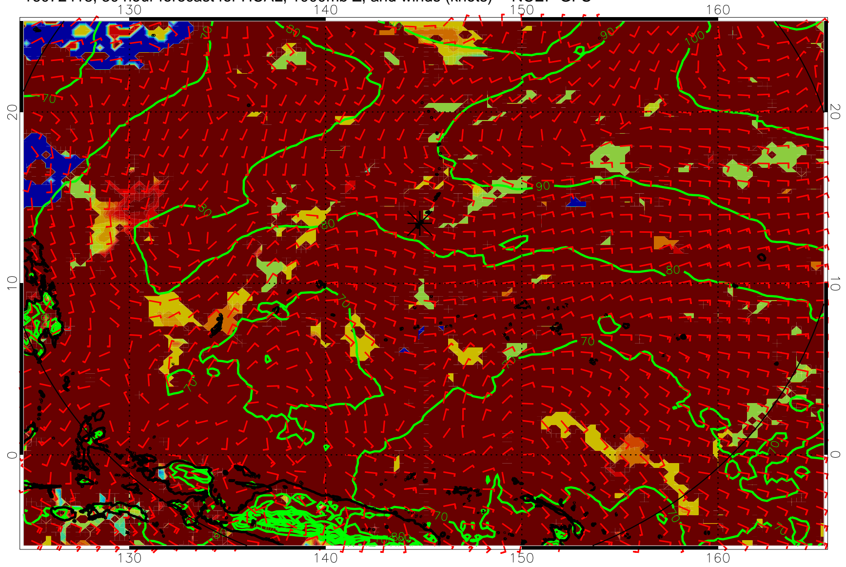
16072418, 30 hour forecast for HCAL, 1000mb Z, and winds (knots) -- NCEP GFS
