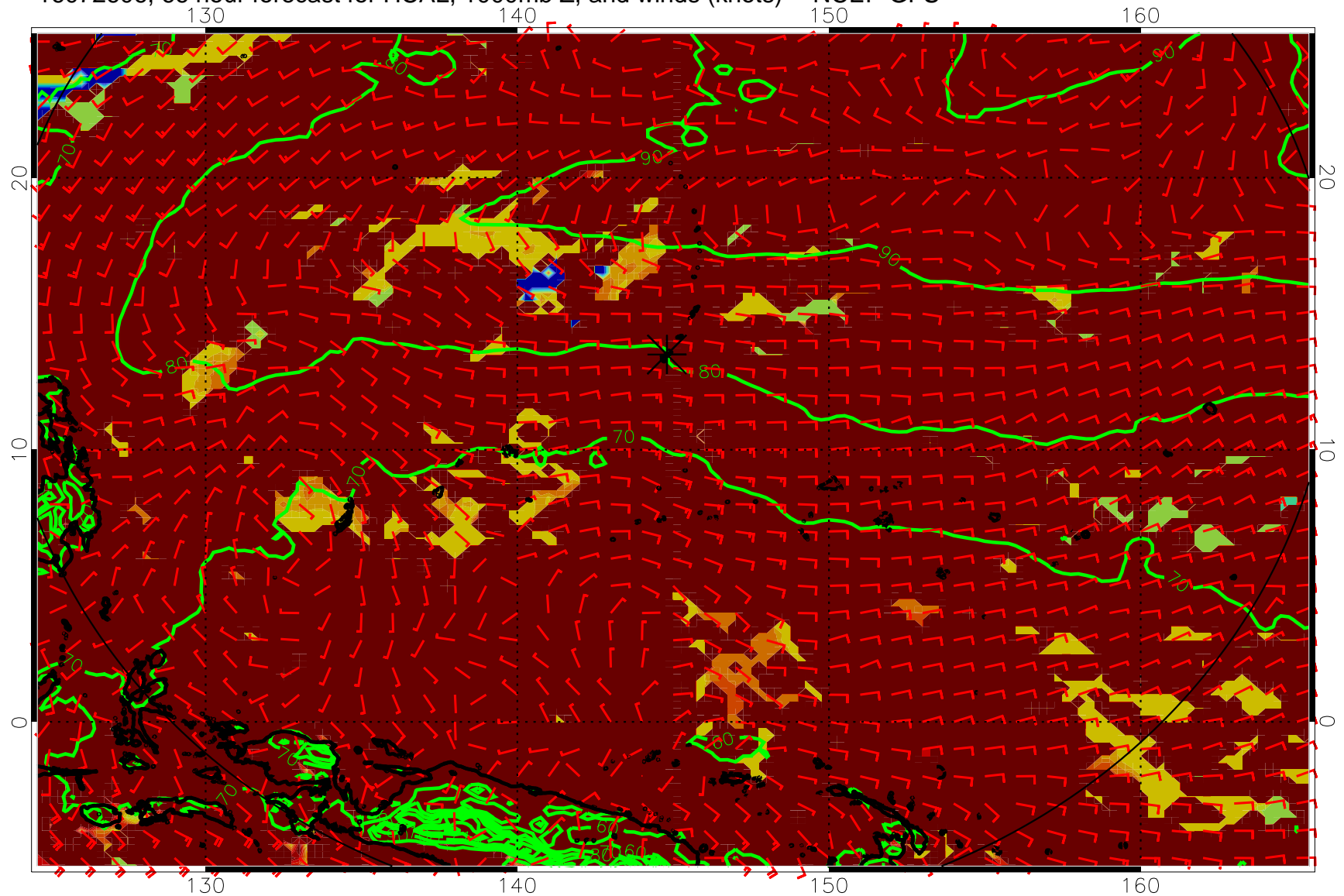
16072606, 66 hour forecast for HCAL, 1000mb Z, and winds (knots) -- NCEP GFS
