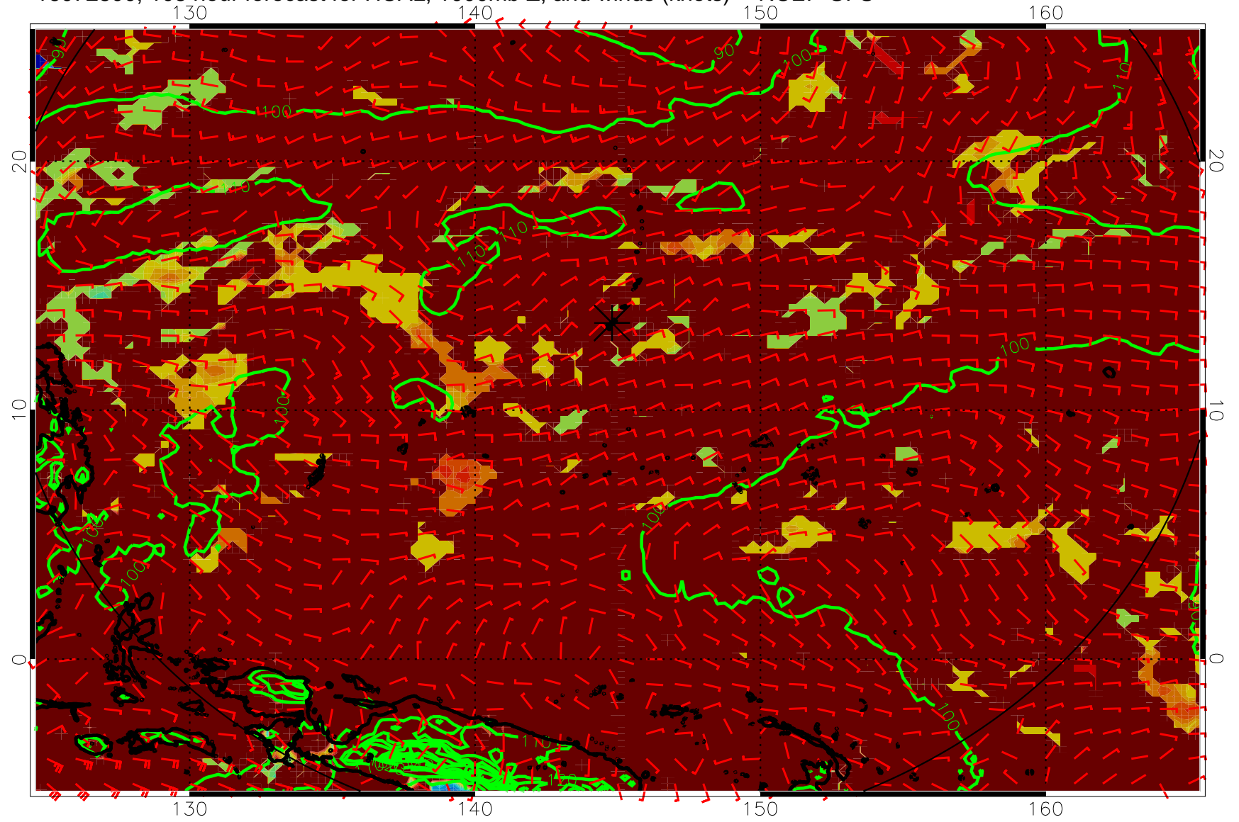
16072800, 108 hour forecast for HCAL, 1000mb Z, and winds (knots) -- NCEP GFS
