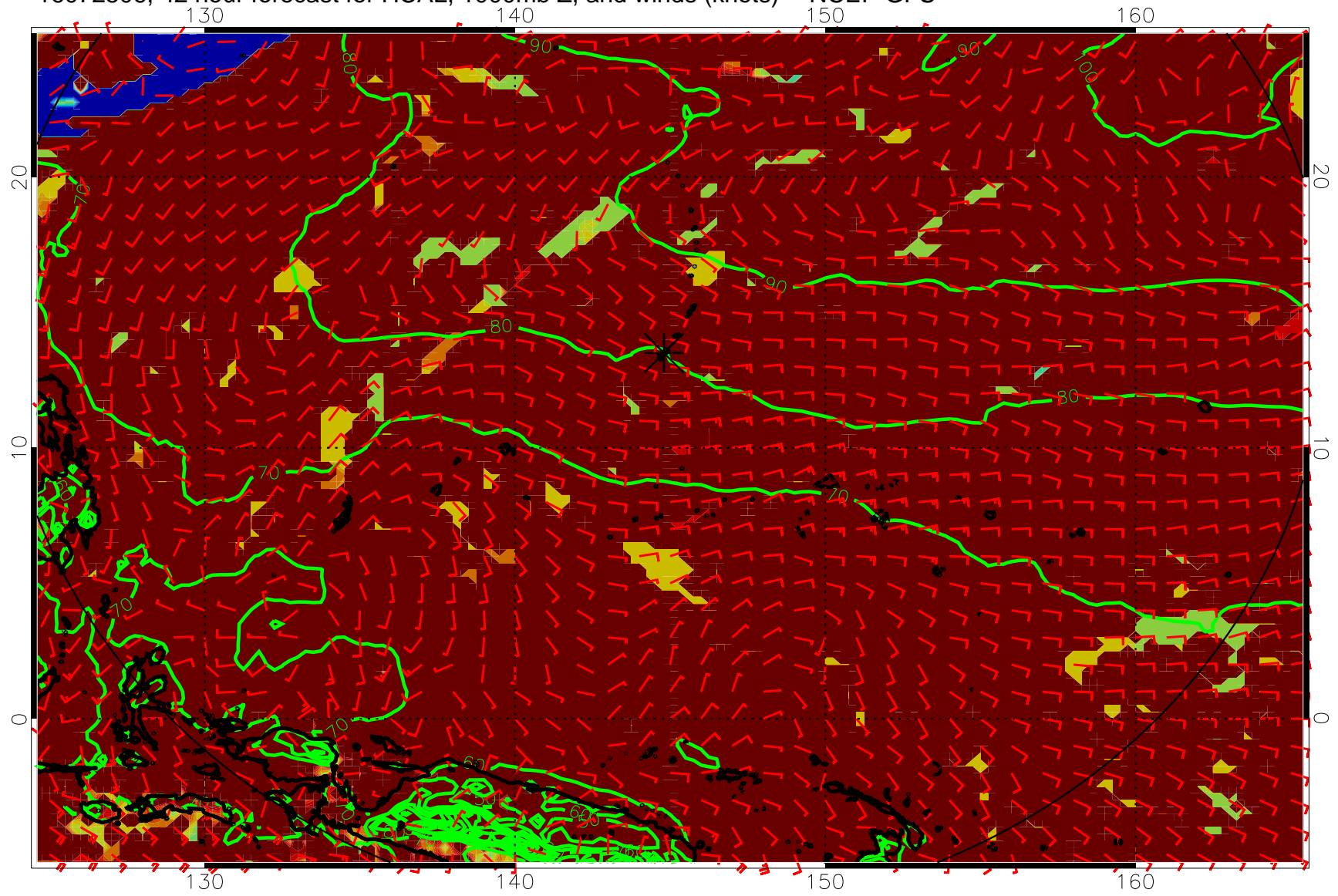
16072506, 42 hour forecast for HCAL, 1000mb Z, and winds (knots) -- NCEP GFS
