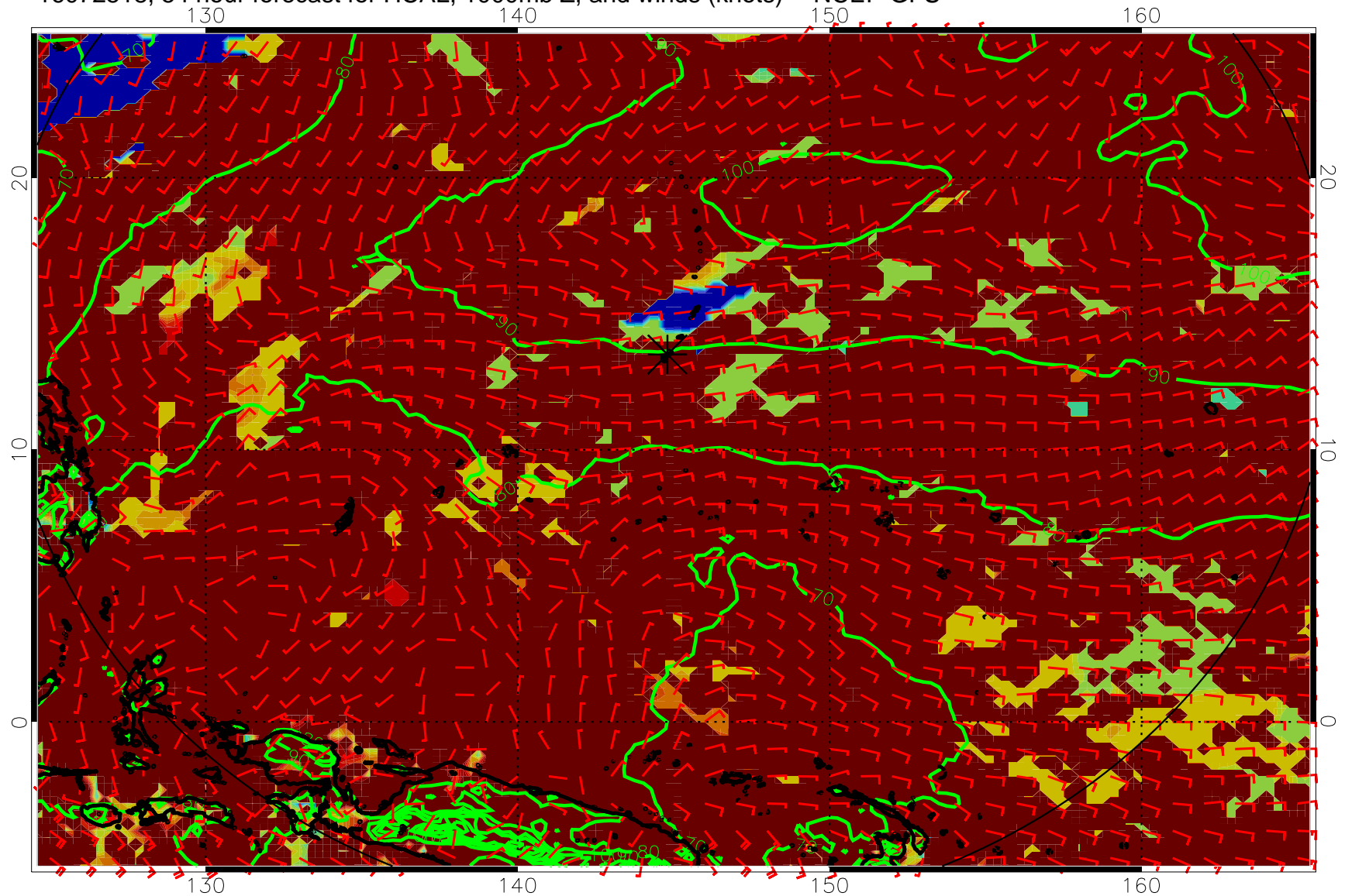
16072518, 54 hour forecast for HCAL, 1000mb Z, and winds (knots) -- NCEP GFS
