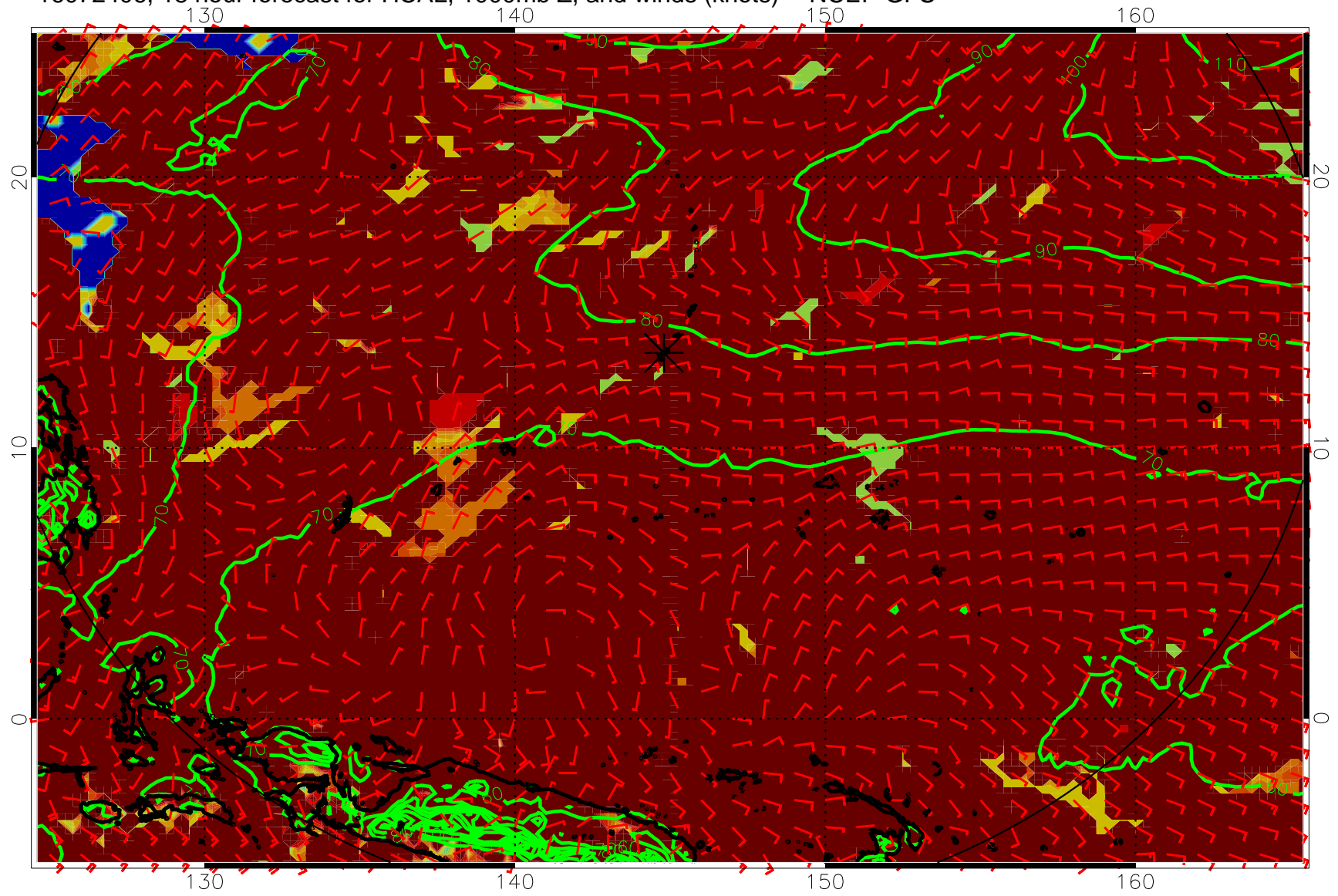
16072406, 18 hour forecast for HCAL, 1000mb Z, and winds (knots) -- NCEP GFS
