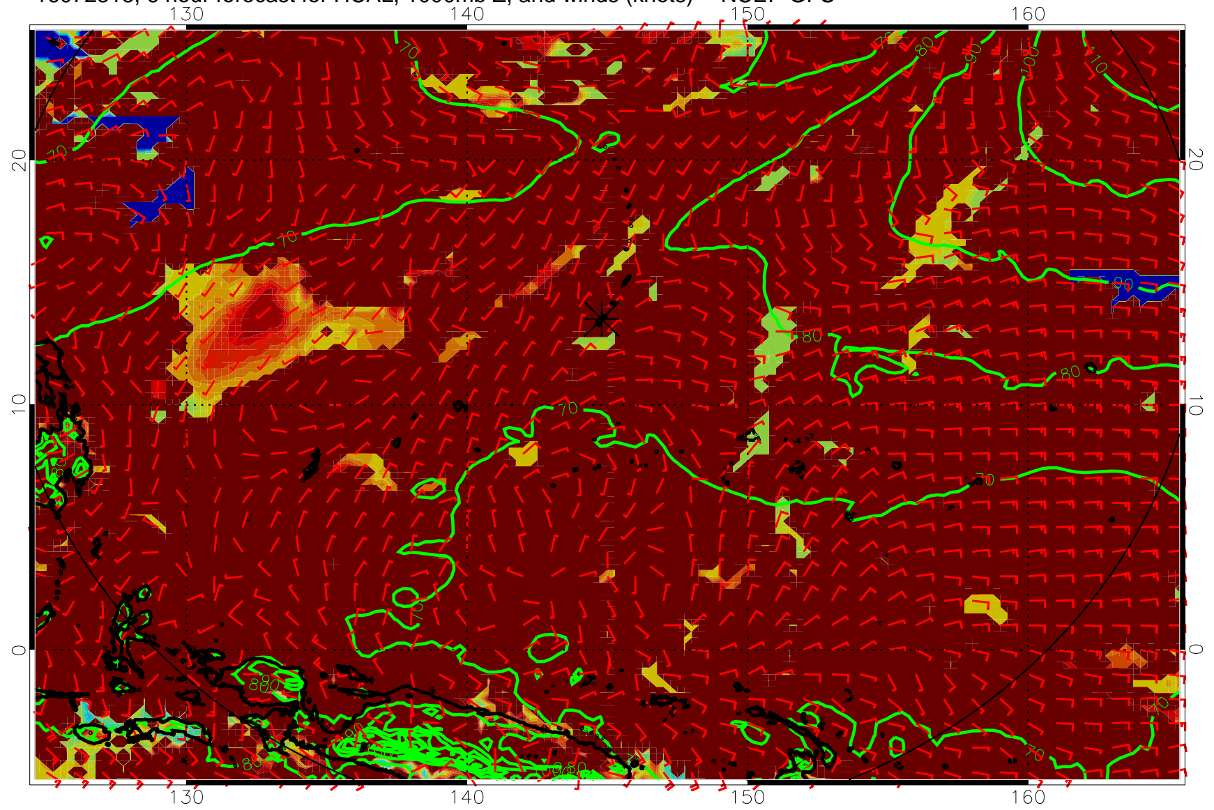
16072318, 6 hour forecast for HCAL, 1000mb Z, and winds (knots) -- NCEP GFS
