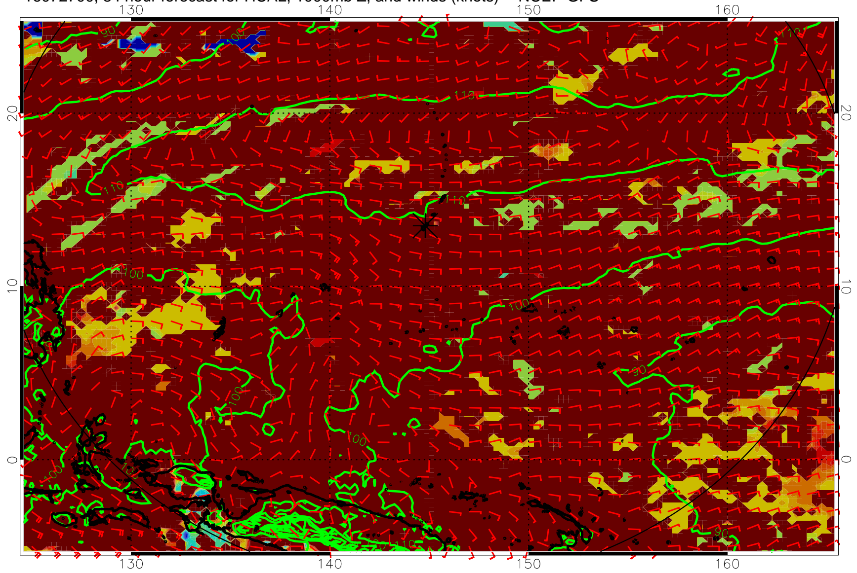
16072700, 84 hour forecast for HCAL, 1000mb Z, and winds (knots) -- NCEP GFS
