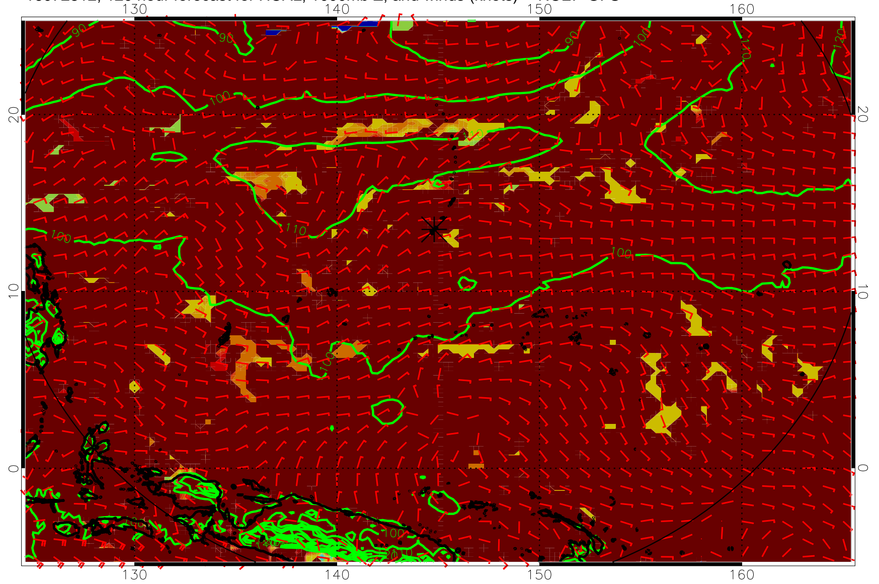
16072812, 120 hour forecast for HCAL, 1000mb Z, and winds (knots) -- NCEP GFS
