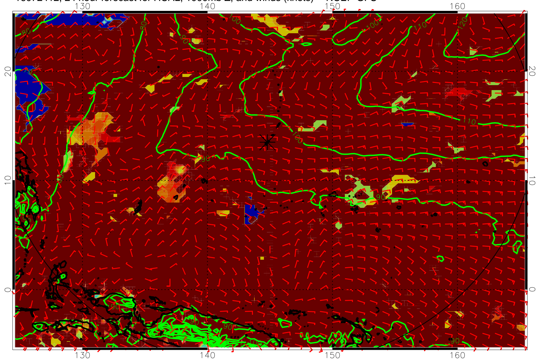
16072412, 24 hour forecast for HCAL, 1000mb Z, and winds (knots) -- NCEP GFS
