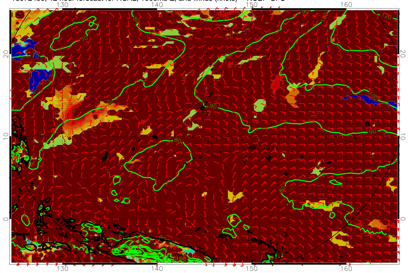
16072400, 12 hour forecast for HCAL, 1000mb Z, and winds (knots) -- NCEP GFS
