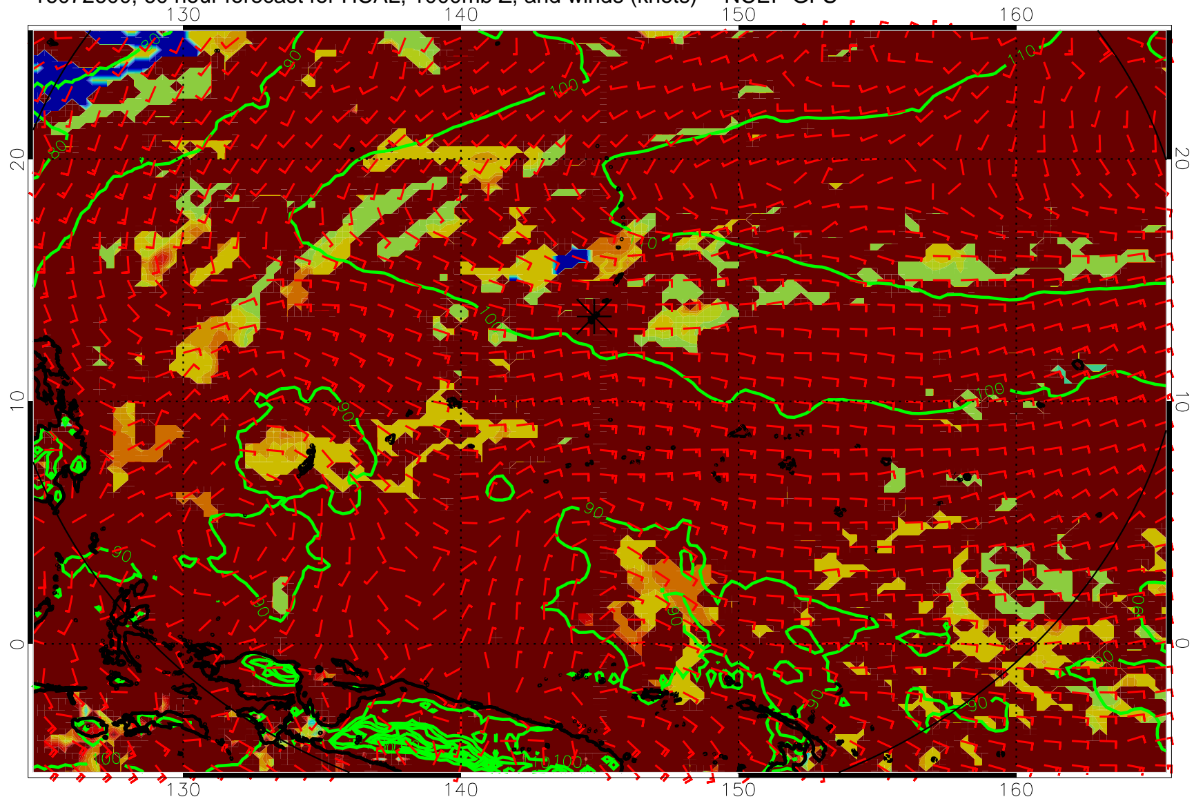
16072600, 60 hour forecast for HCAL, 1000mb Z, and winds (knots) -- NCEP GFS
