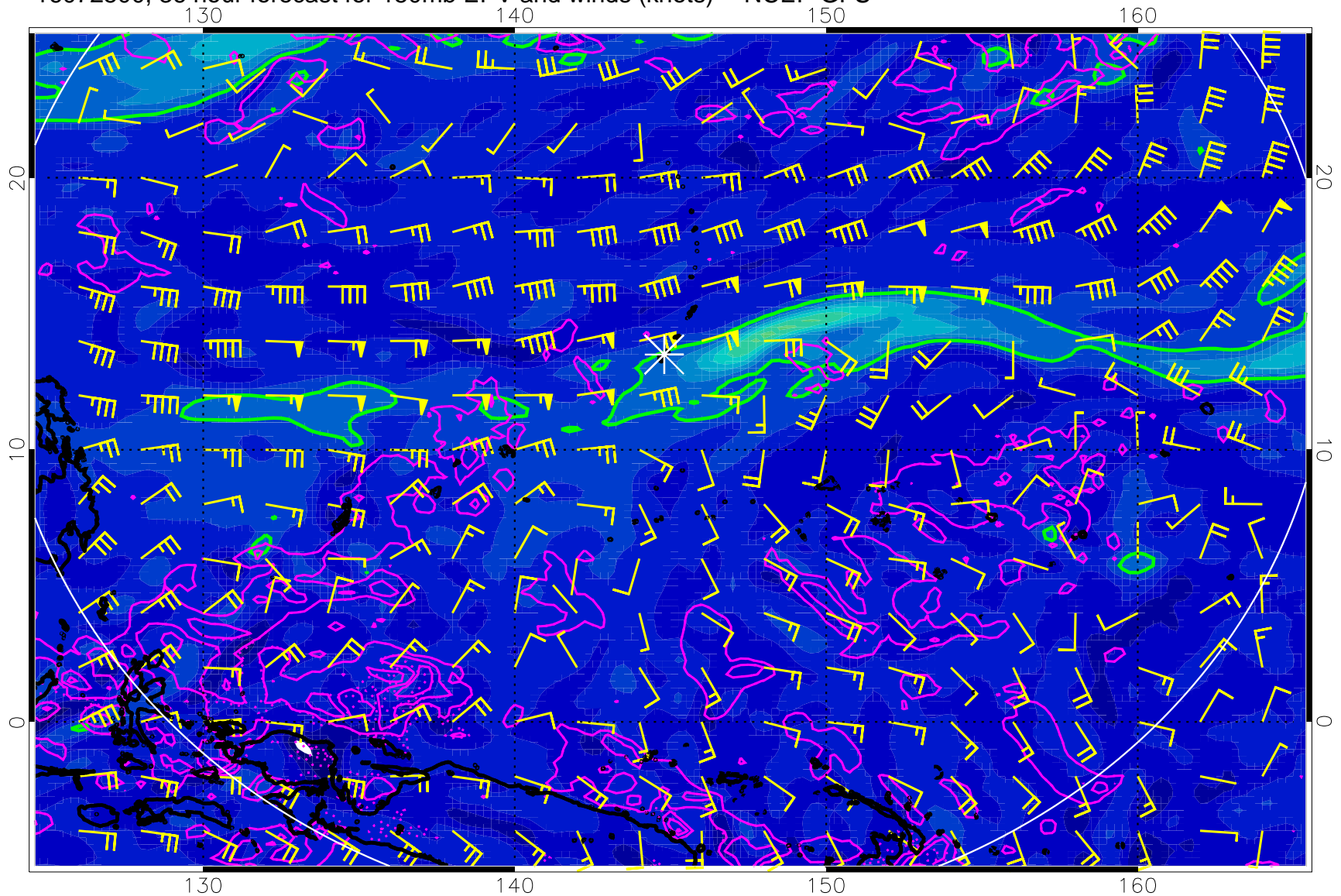
16072500, 36 hour forecast for 150mb EPV and winds (knots) -- NCEP GFS
