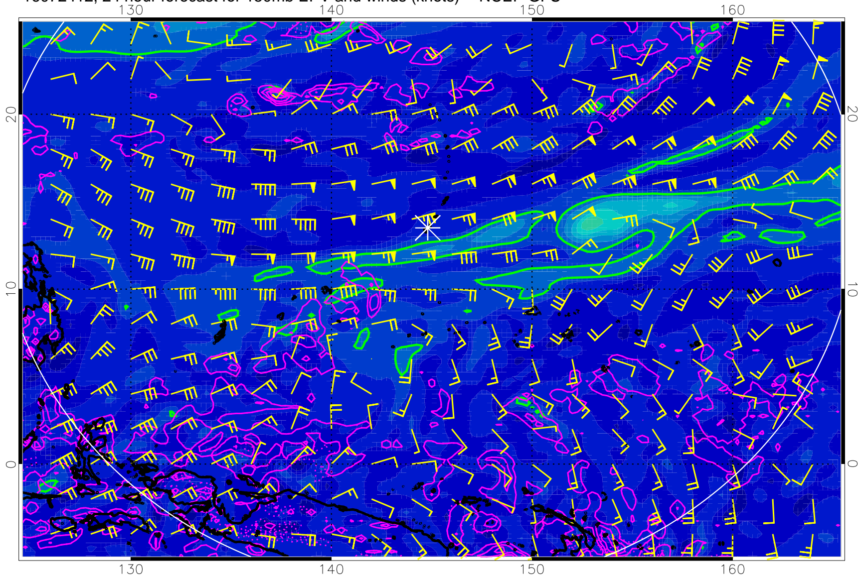
16072412, 24 hour forecast for 150mb EPV and winds (knots) -- NCEP GFS
