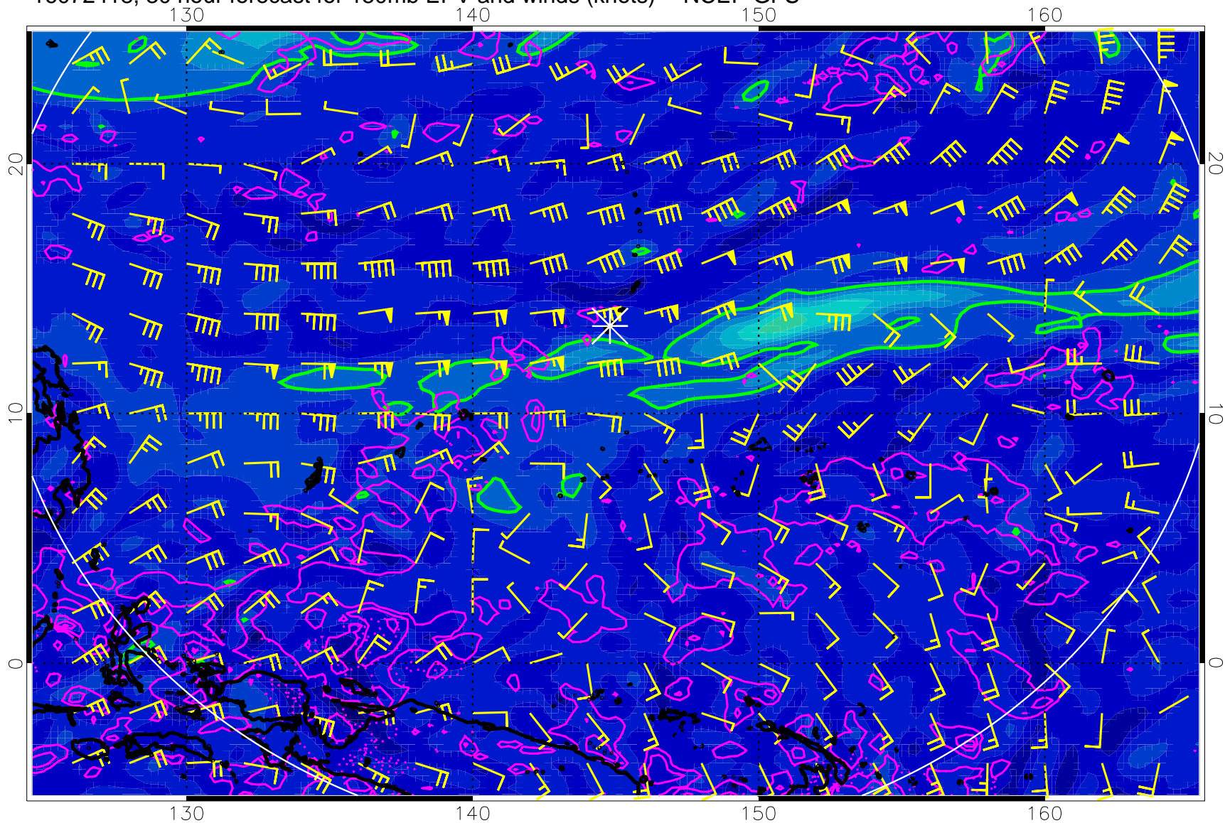
16072418, 30 hour forecast for 150mb EPV and winds (knots) -- NCEP GFS
