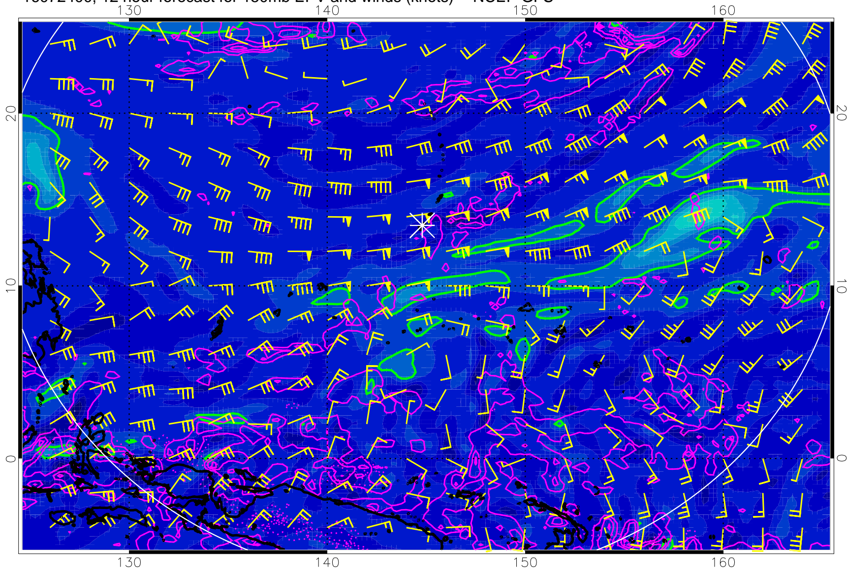
16072400, 12 hour forecast for 150mb EPV and winds (knots) -- NCEP GFS
