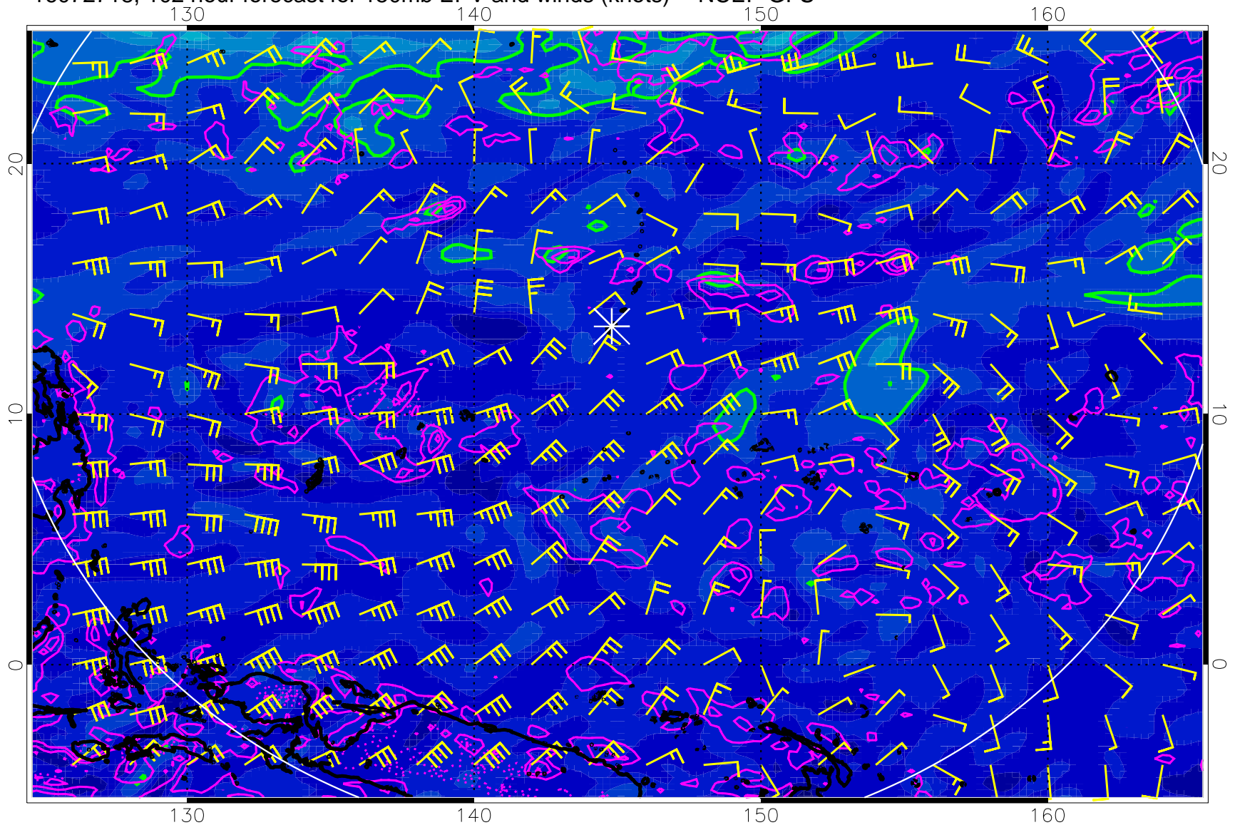
16072718, 102 hour forecast for 150mb EPV and winds (knots) -- NCEP GFS
