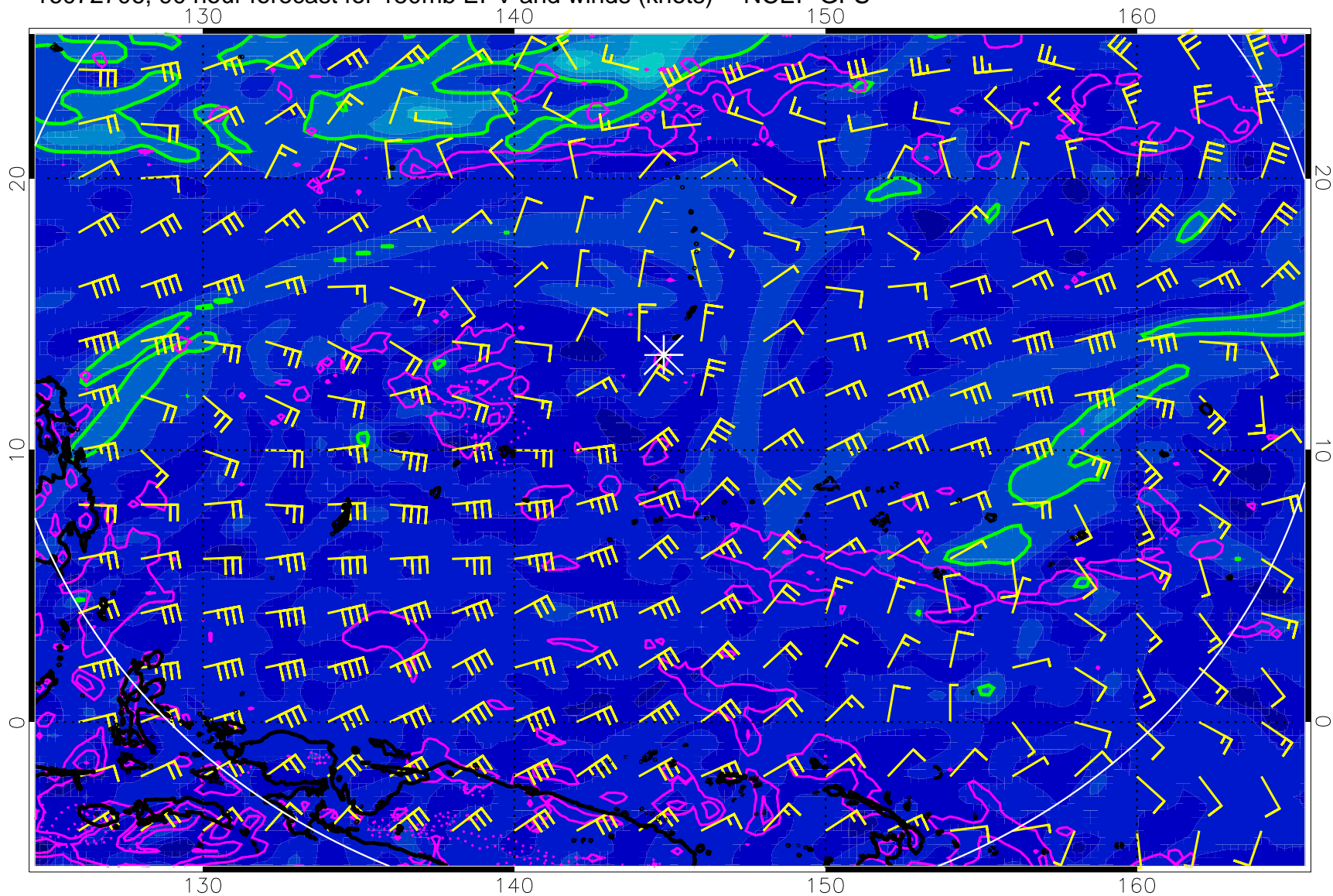
16072706, 90 hour forecast for 150mb EPV and winds (knots) -- NCEP GFS
