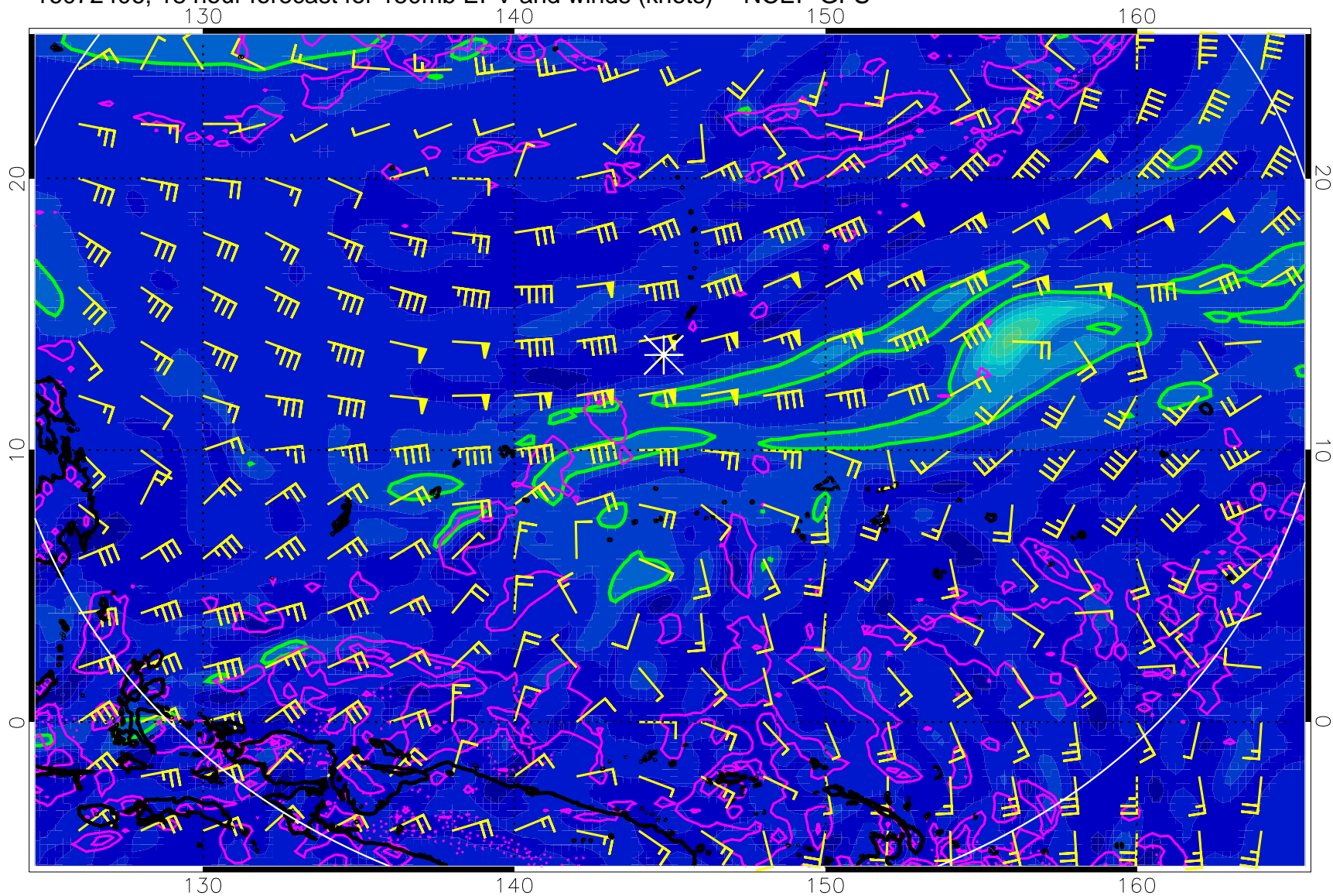
16072406, 18 hour forecast for 150mb EPV and winds (knots) -- NCEP GFS
