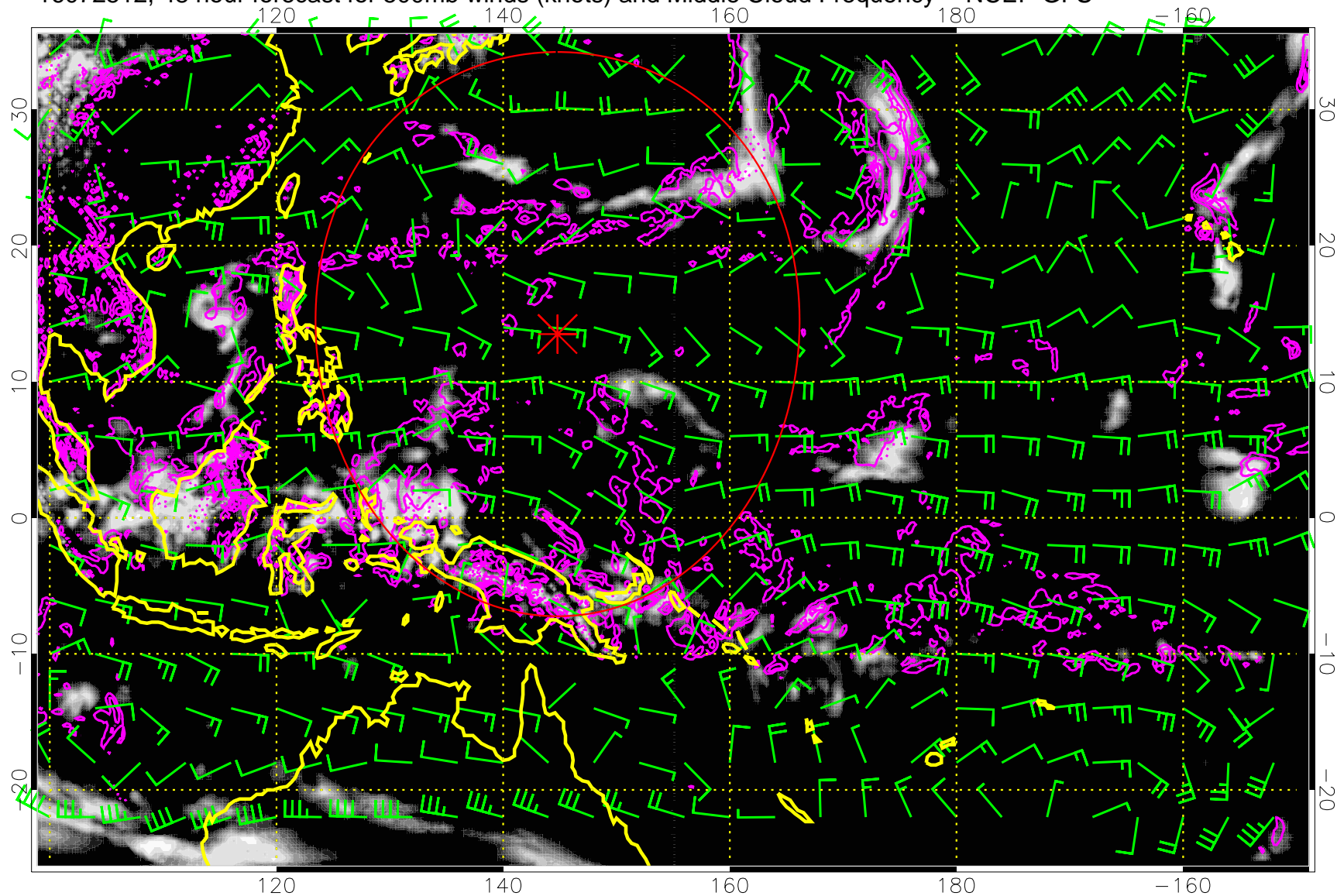
16072512, 48 hour forecast for 500mb winds (knots) and Middle Cloud Frequency -- NCEP GFS
