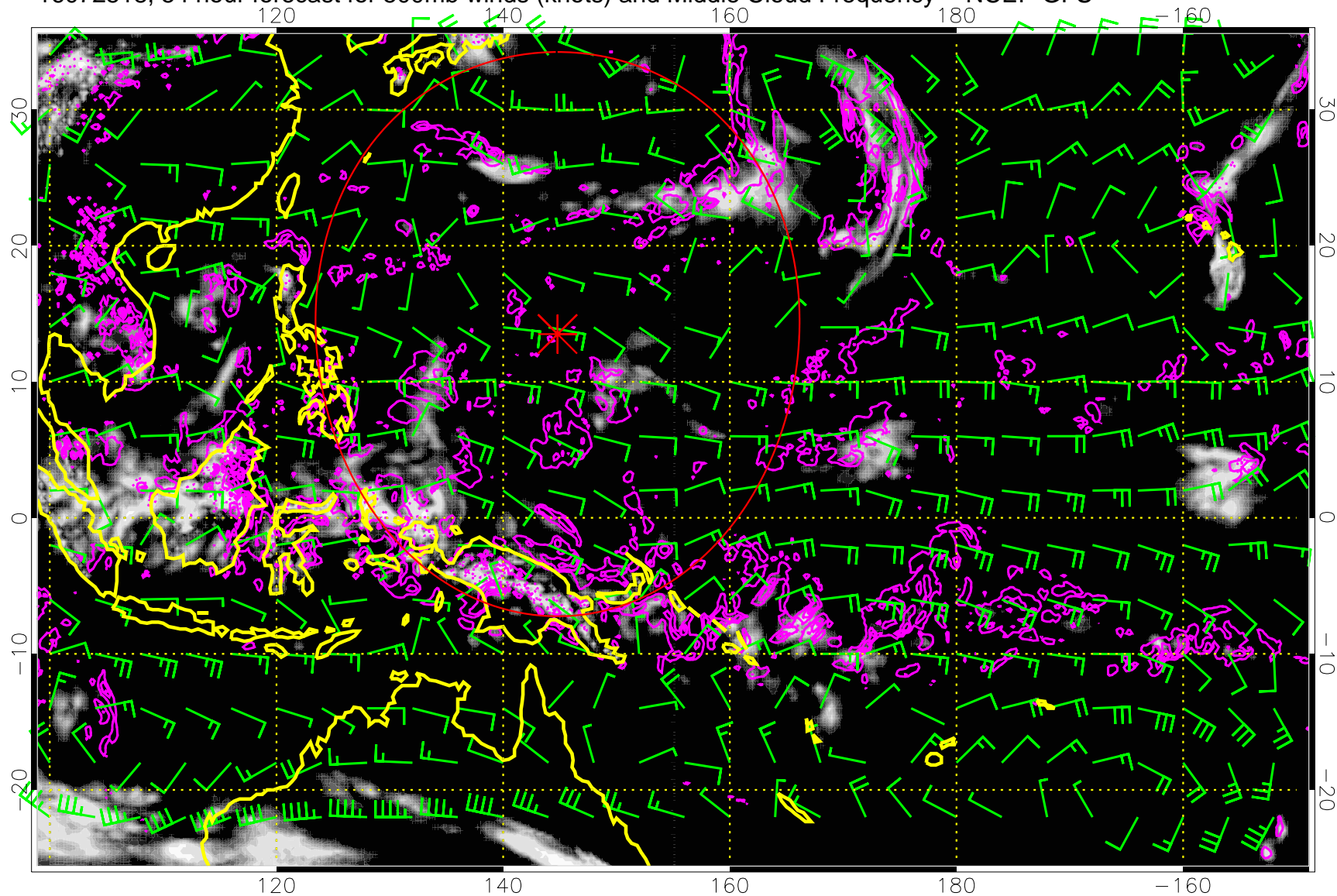
16072518, 54 hour forecast for 500mb winds (knots) and Middle Cloud Frequency -- NCEP GFS
