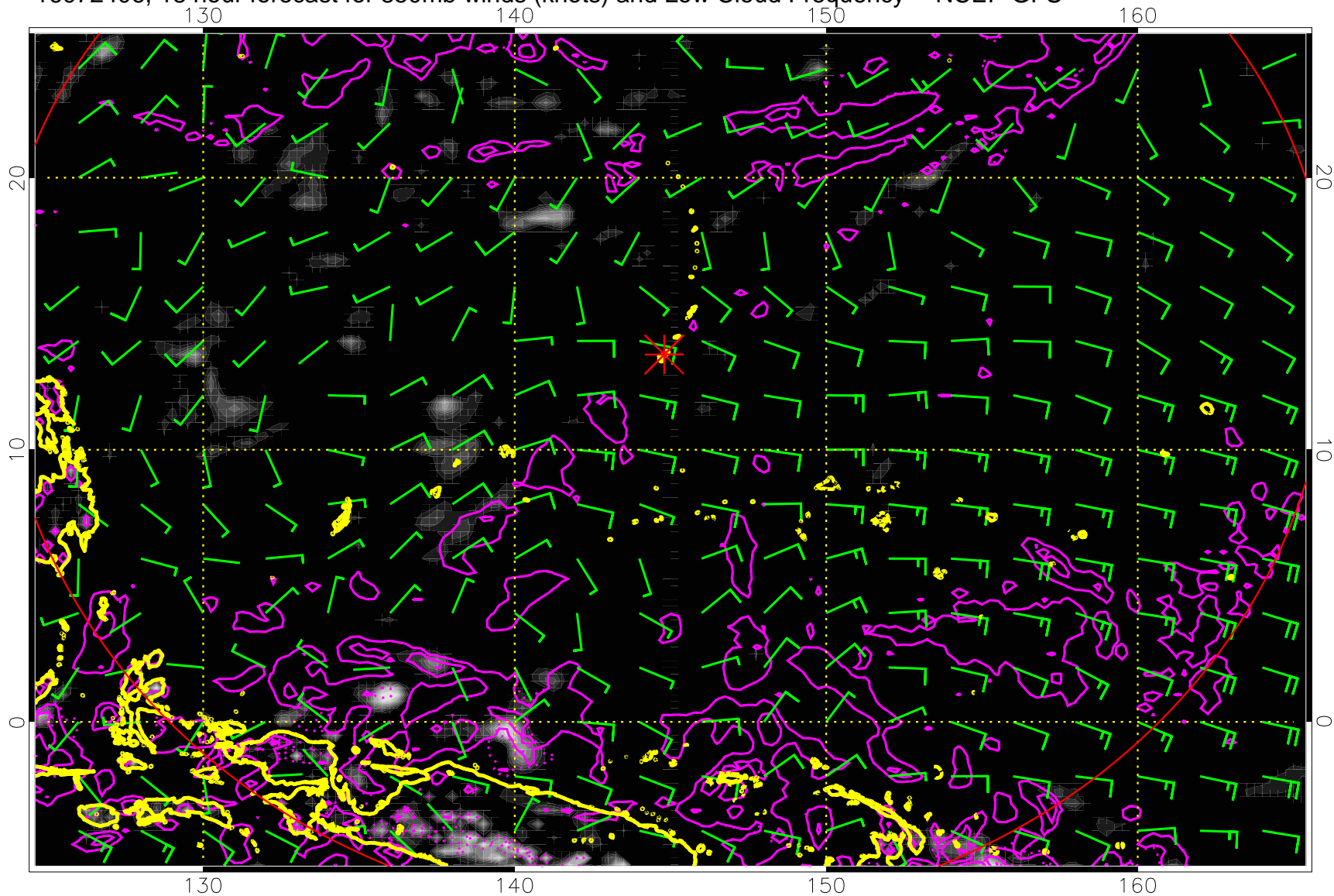
16072406, 18 hour forecast for 850mb winds (knots) and Low Cloud Frequency -- NCEP GFS
