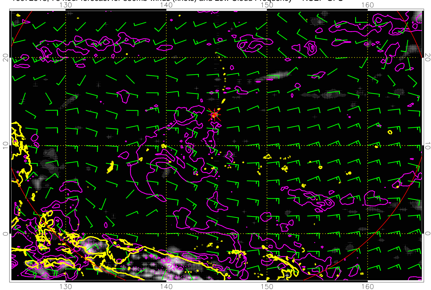
16072618, 78 hour forecast for 850mb winds (knots) and Low Cloud Frequency -- NCEP GFS
