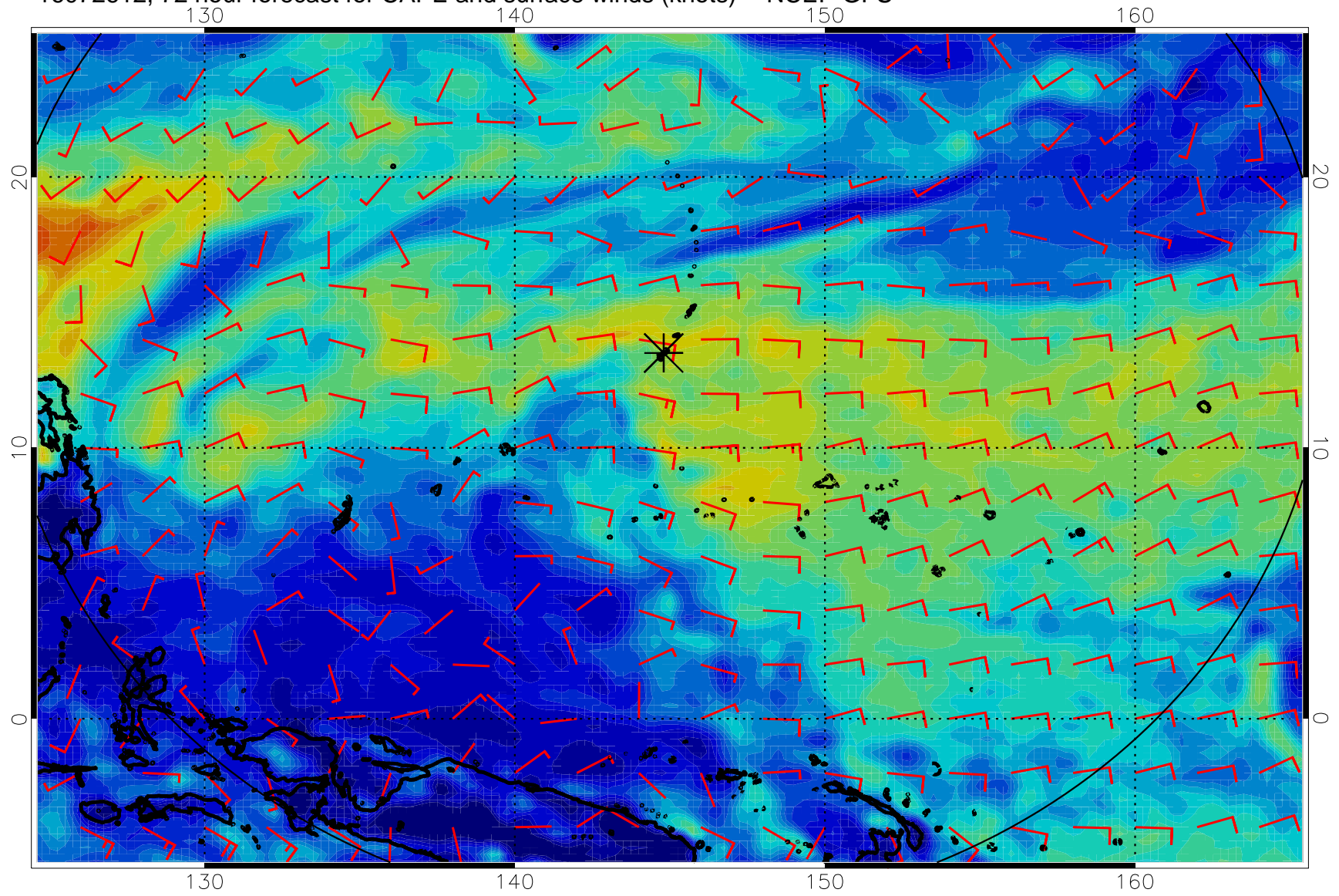
16072612, 72 hour forecast for CAPE and surface winds (knots) -- NCEP GFS
