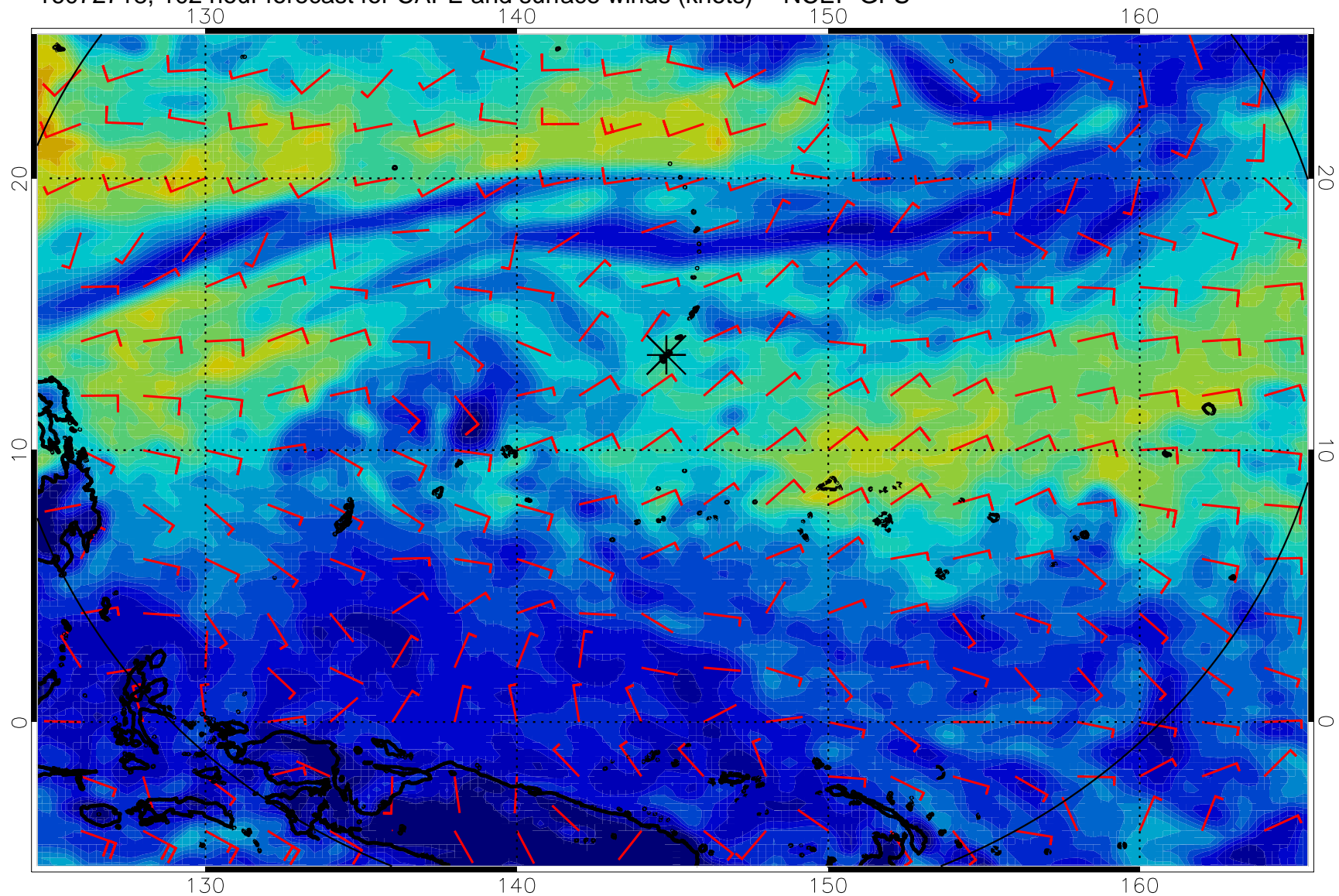
16072718, 102 hour forecast for CAPE and surface winds (knots) -- NCEP GFS
