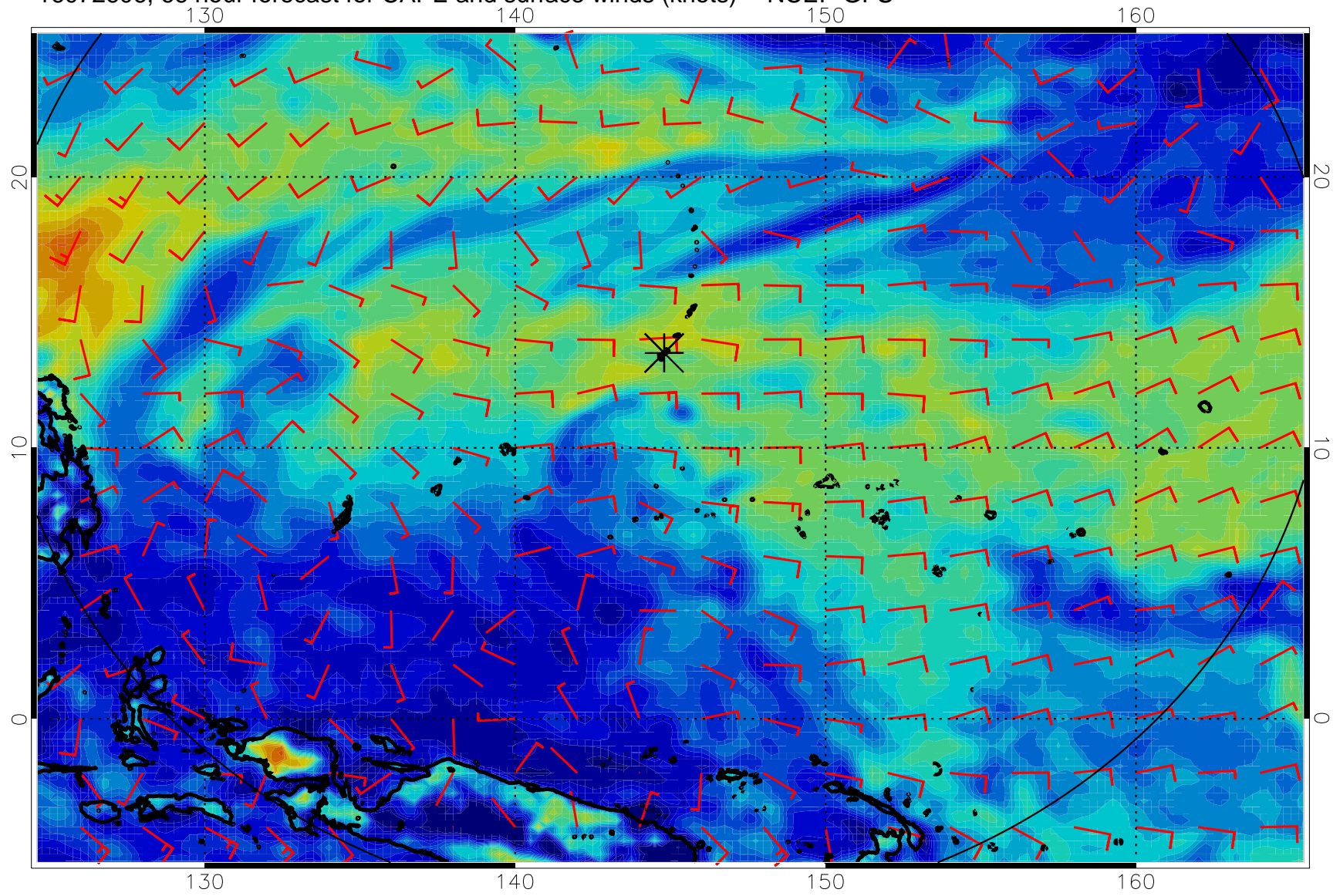
16072606, 66 hour forecast for CAPE and surface winds (knots) -- NCEP GFS
