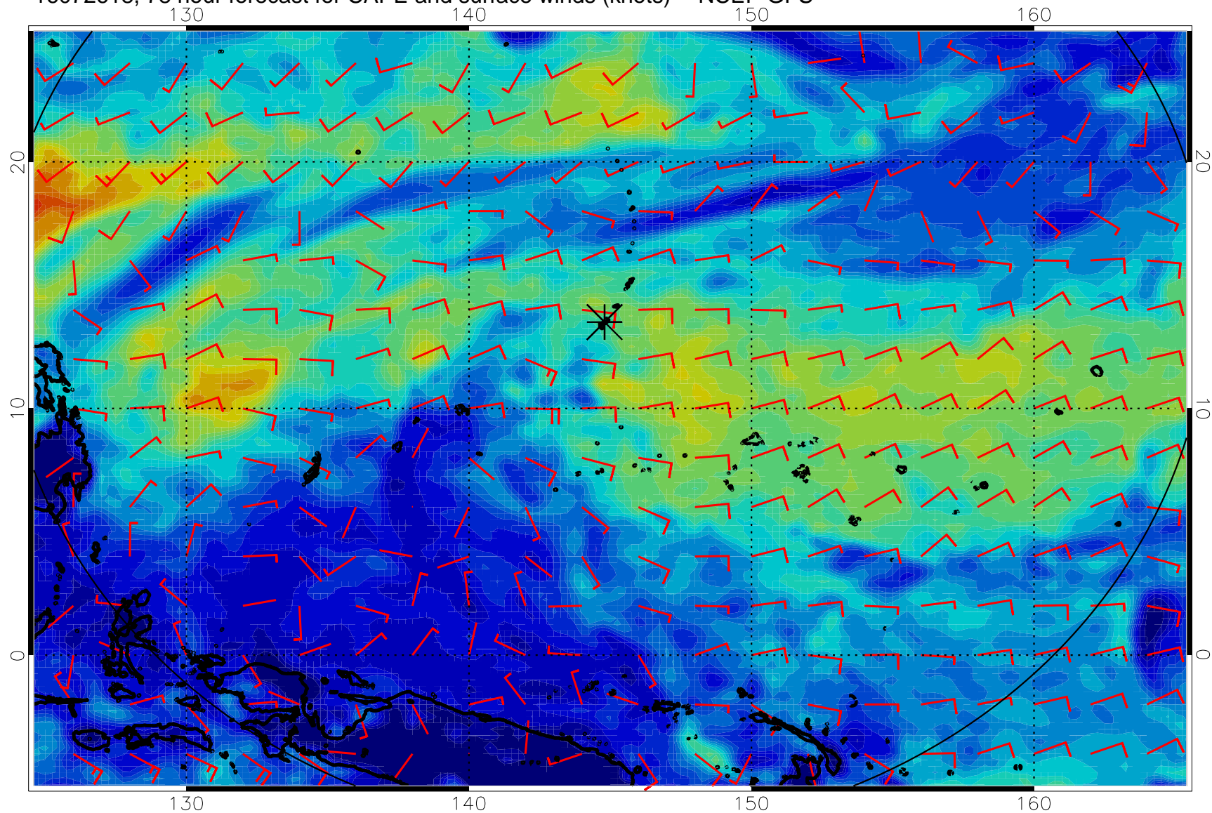
16072618, 78 hour forecast for CAPE and surface winds (knots) -- NCEP GFS
