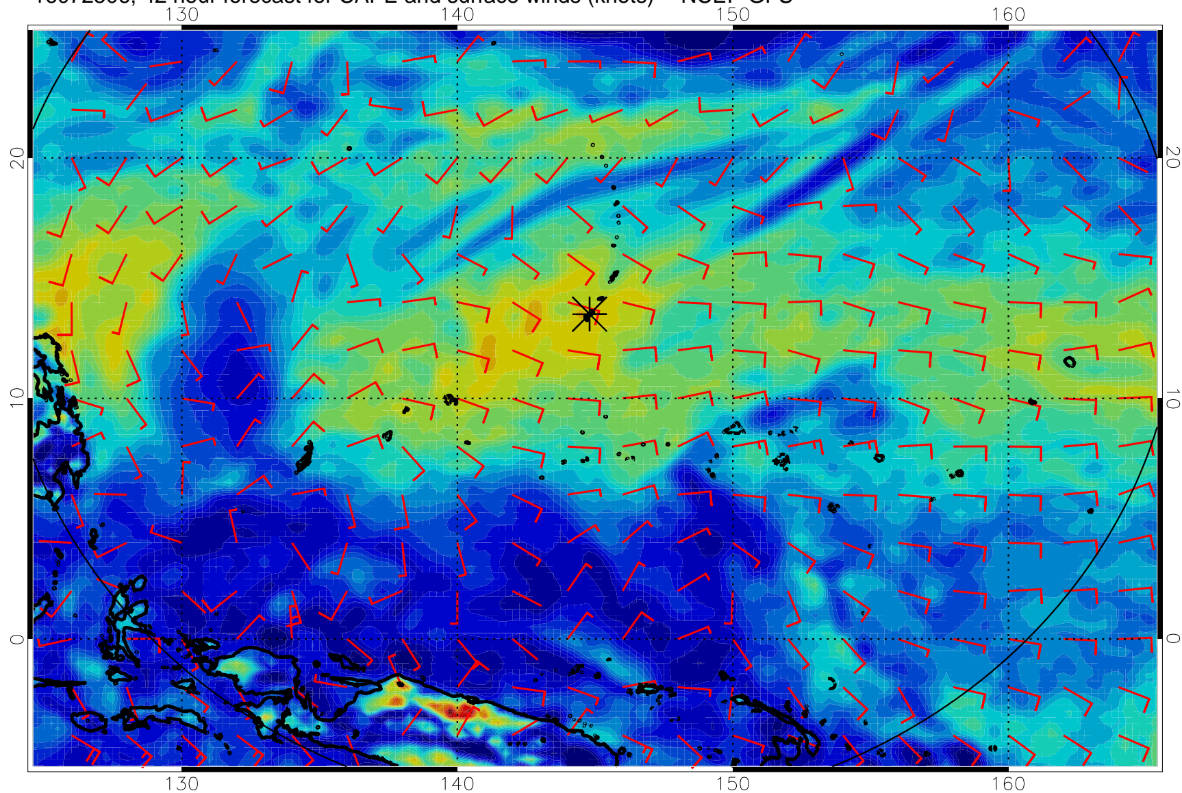
16072506, 42 hour forecast for CAPE and surface winds (knots) -- NCEP GFS
