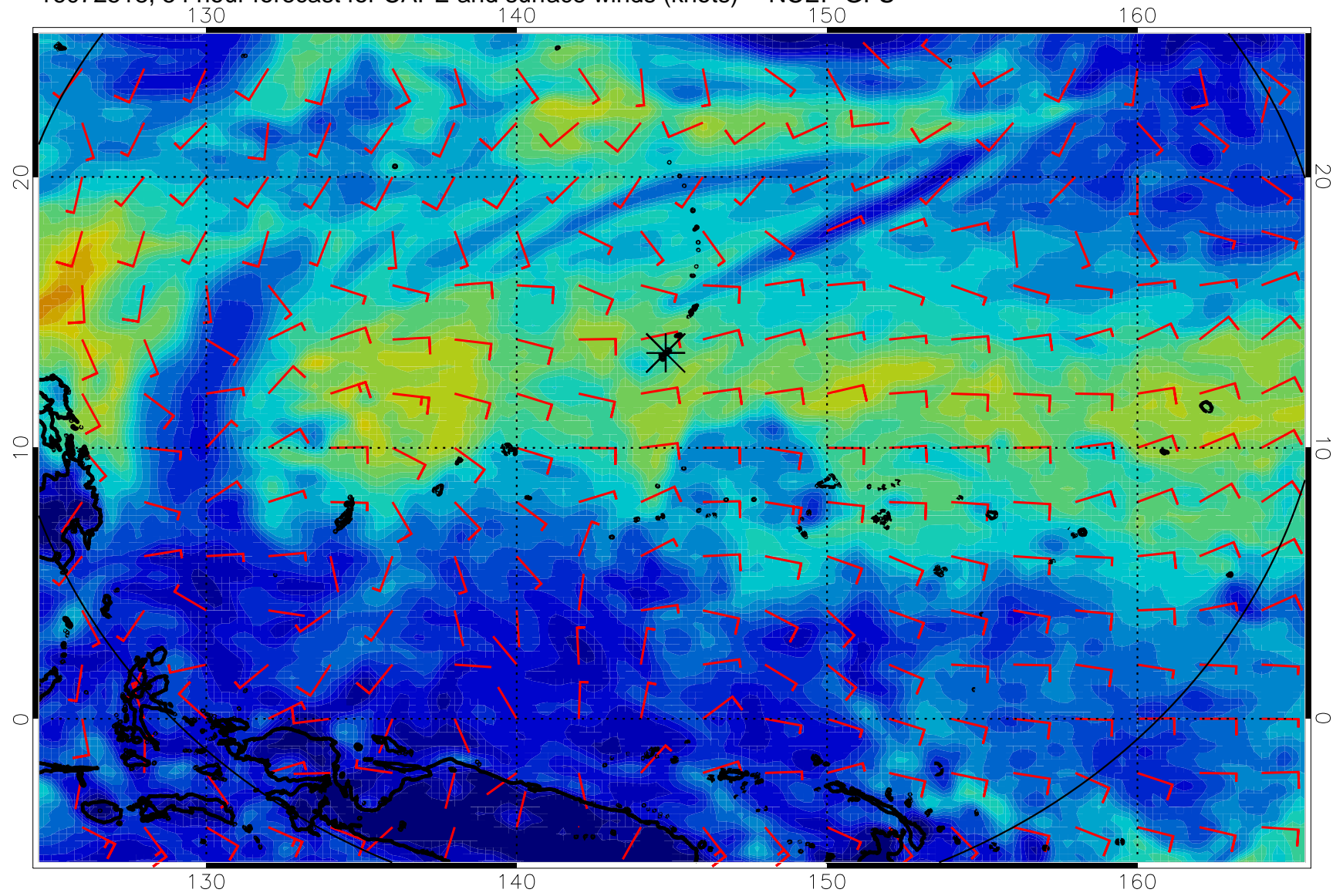
16072518, 54 hour forecast for CAPE and surface winds (knots) -- NCEP GFS
