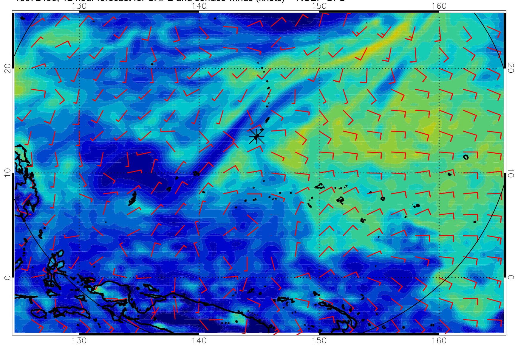
16072400, 12 hour forecast for CAPE and surface winds (knots) -- NCEP GFS
