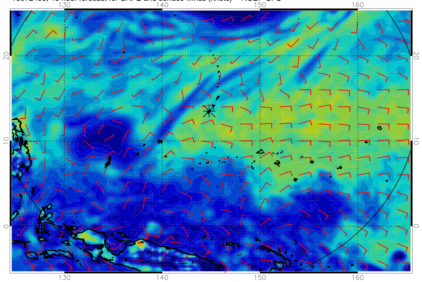
16072406, 18 hour forecast for CAPE and surface winds (knots) -- NCEP GFS
