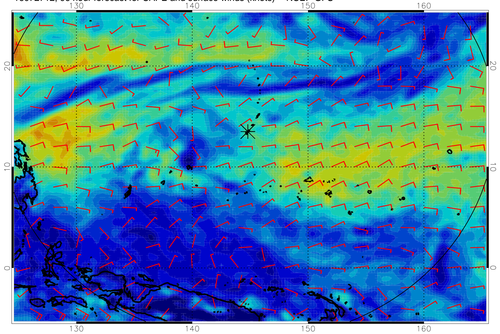
16072712, 96 hour forecast for CAPE and surface winds (knots) -- NCEP GFS
