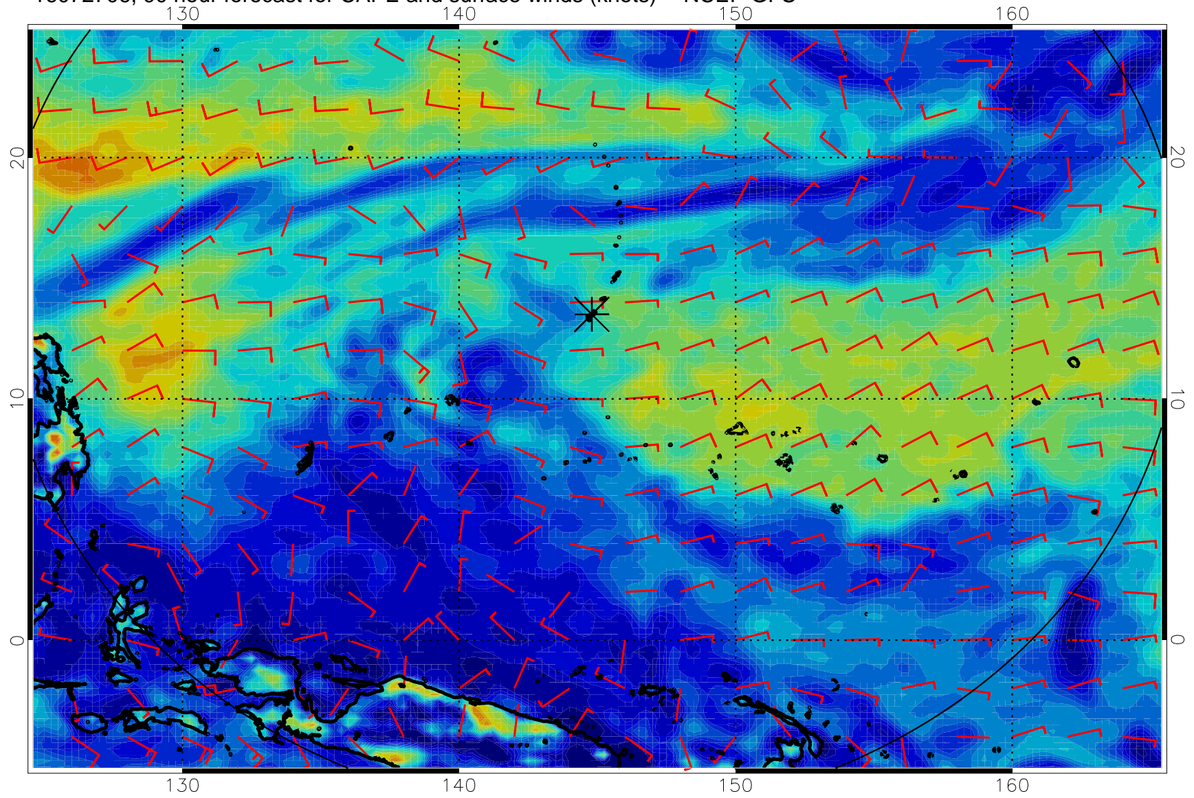
16072706, 90 hour forecast for CAPE and surface winds (knots) -- NCEP GFS
