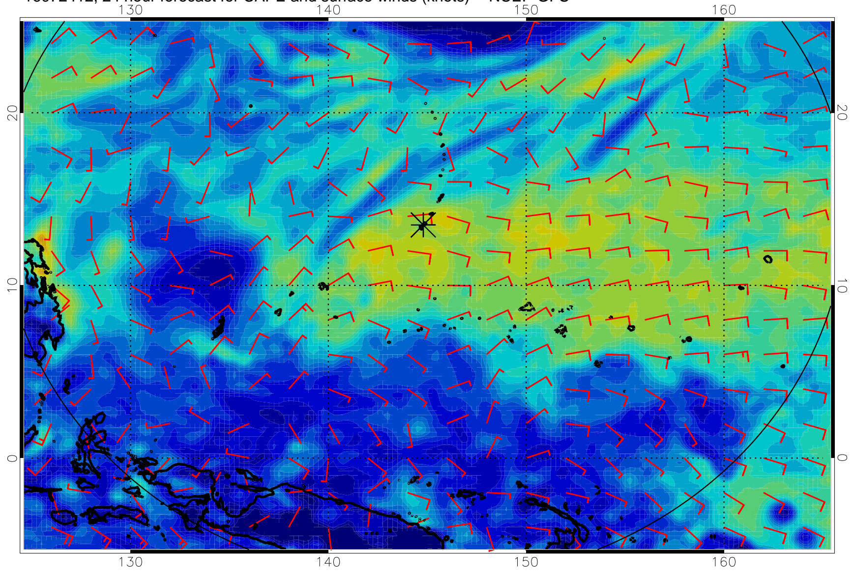
16072412, 24 hour forecast for CAPE and surface winds (knots) -- NCEP GFS
