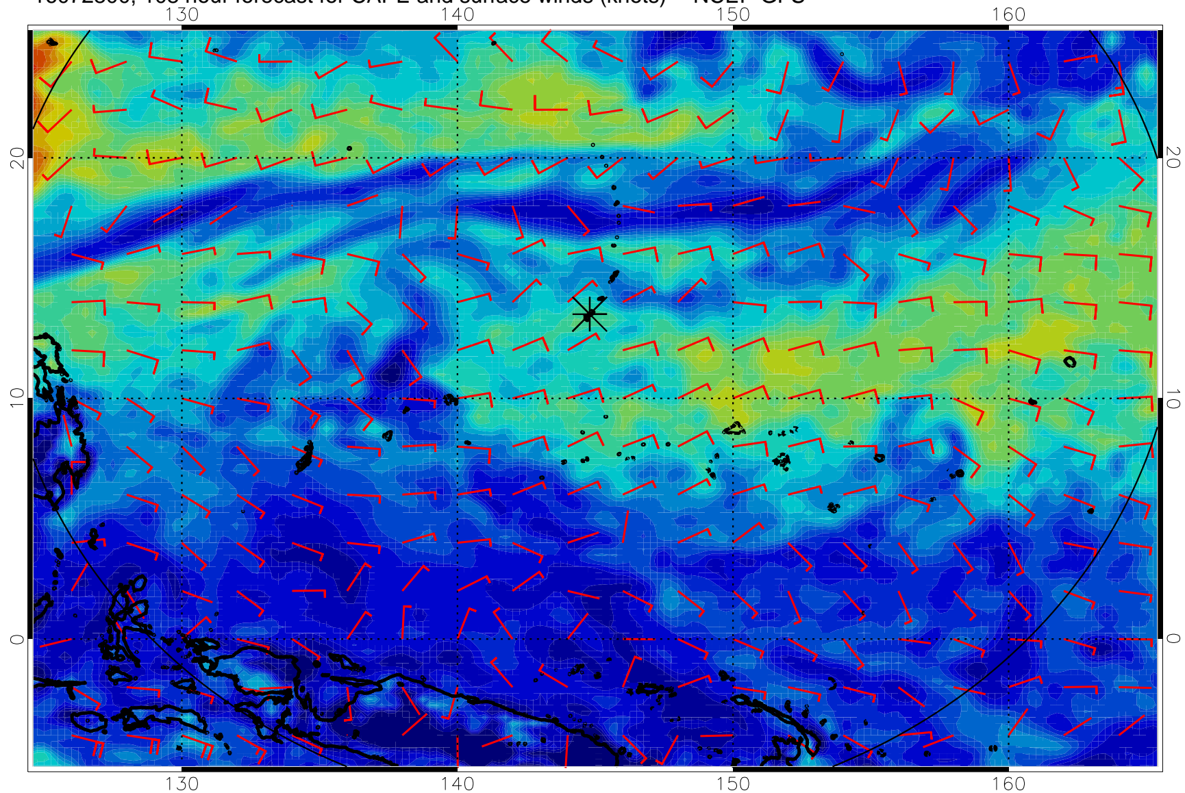
16072800, 108 hour forecast for CAPE and surface winds (knots) -- NCEP GFS
