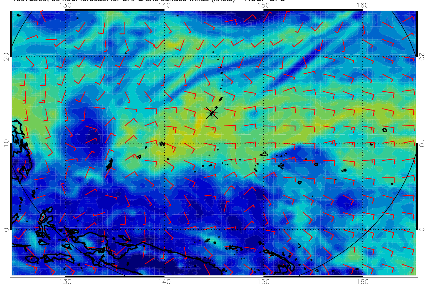
16072500, 36 hour forecast for CAPE and surface winds (knots) -- NCEP GFS
