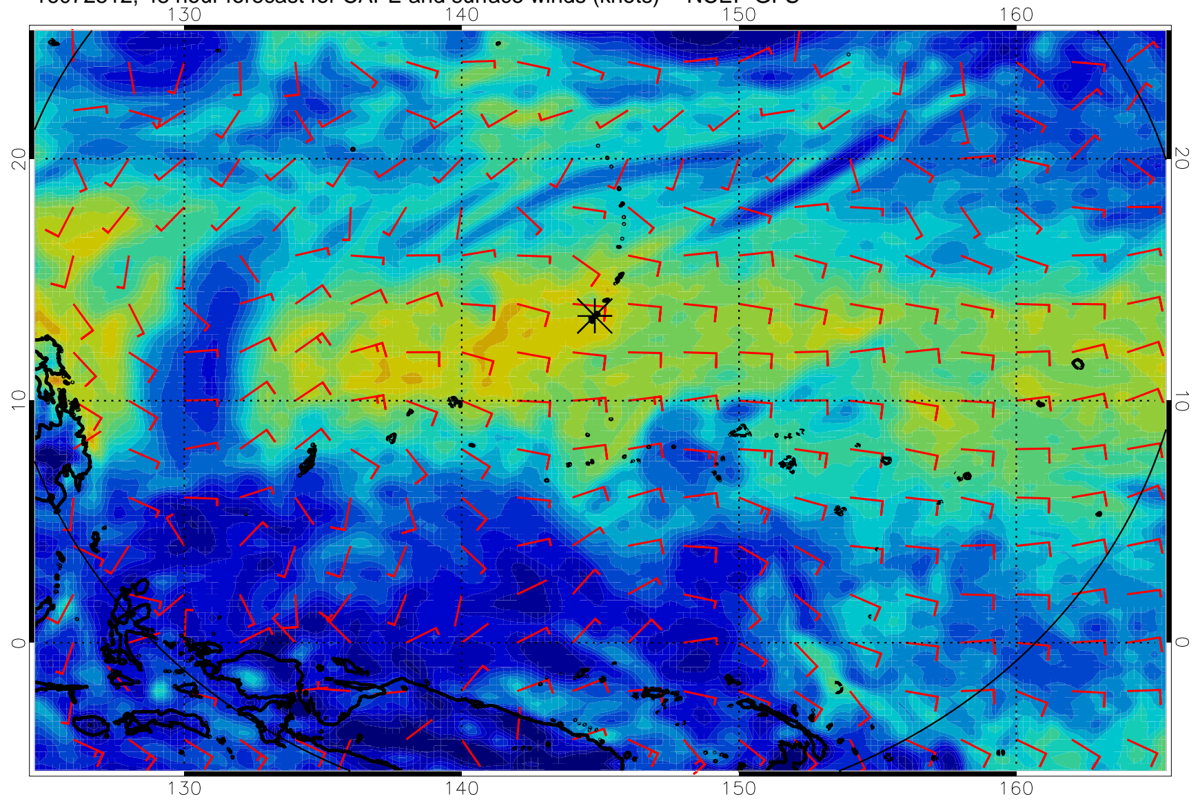
16072512, 48 hour forecast for CAPE and surface winds (knots) -- NCEP GFS
