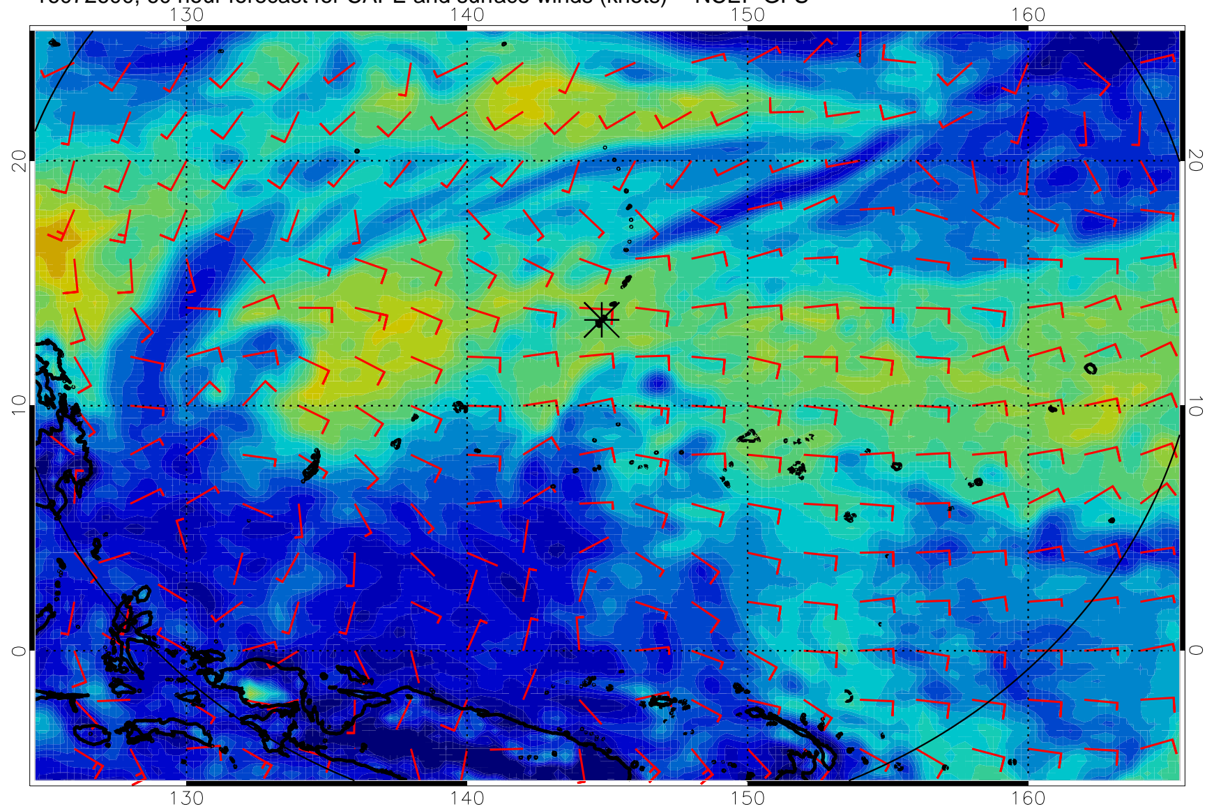
16072600, 60 hour forecast for CAPE and surface winds (knots) -- NCEP GFS
