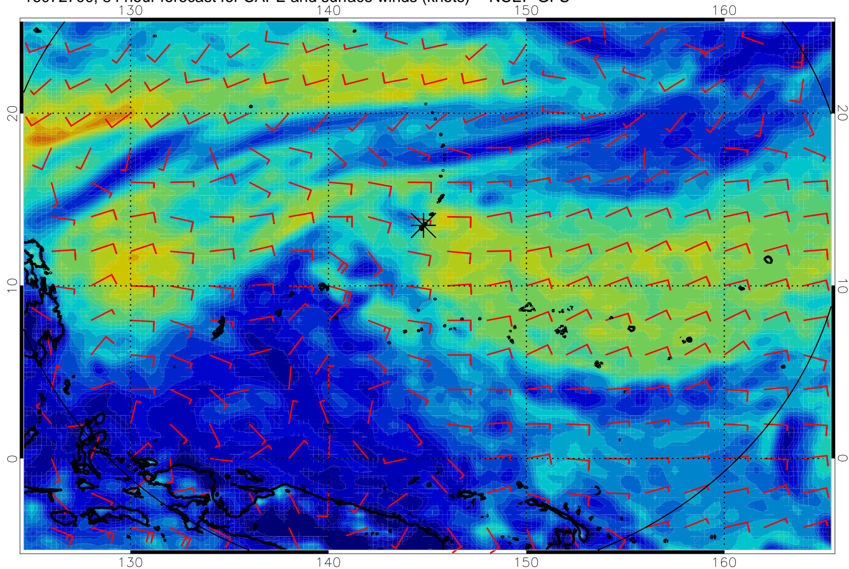
16072700, 84 hour forecast for CAPE and surface winds (knots) -- NCEP GFS
