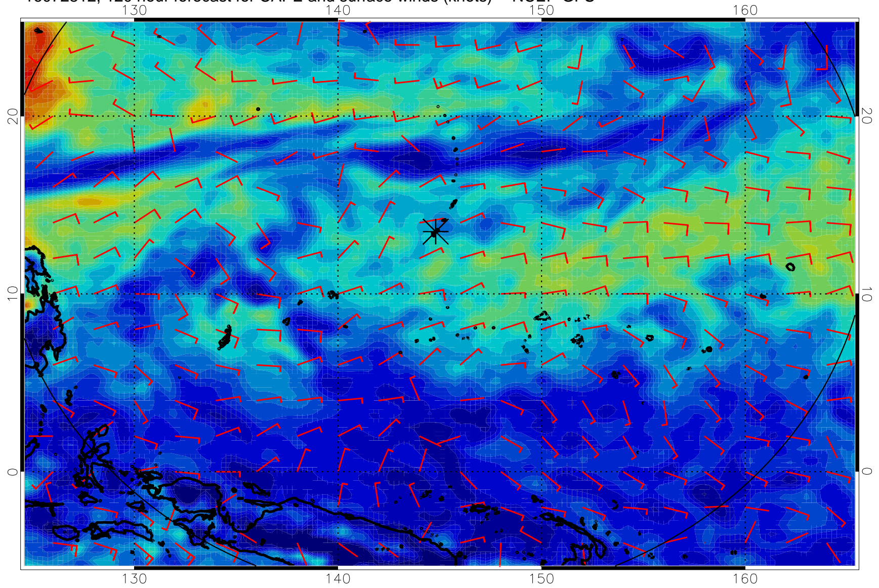
16072812, 120 hour forecast for CAPE and surface winds (knots) -- NCEP GFS
