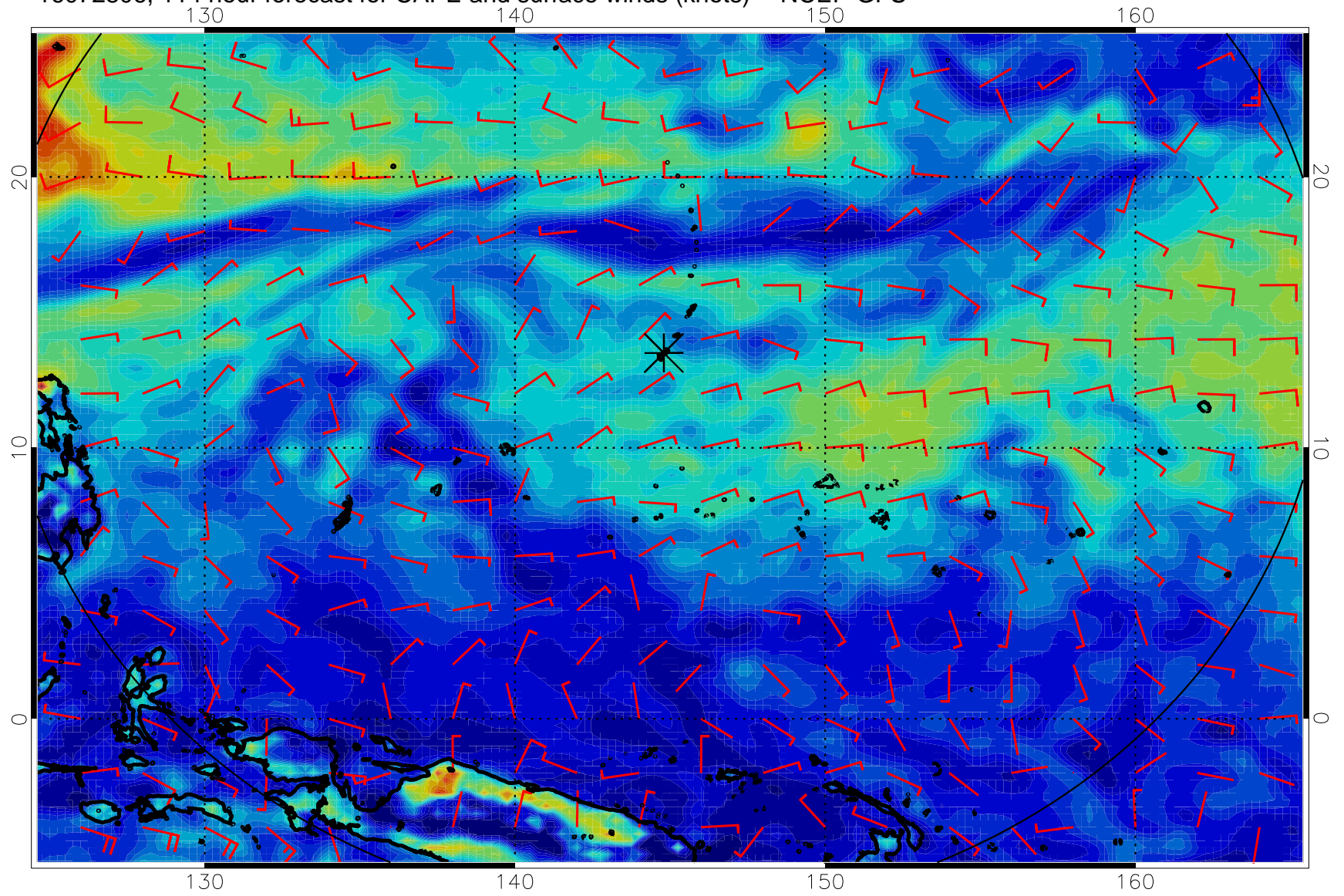
16072806, 114 hour forecast for CAPE and surface winds (knots) -- NCEP GFS
