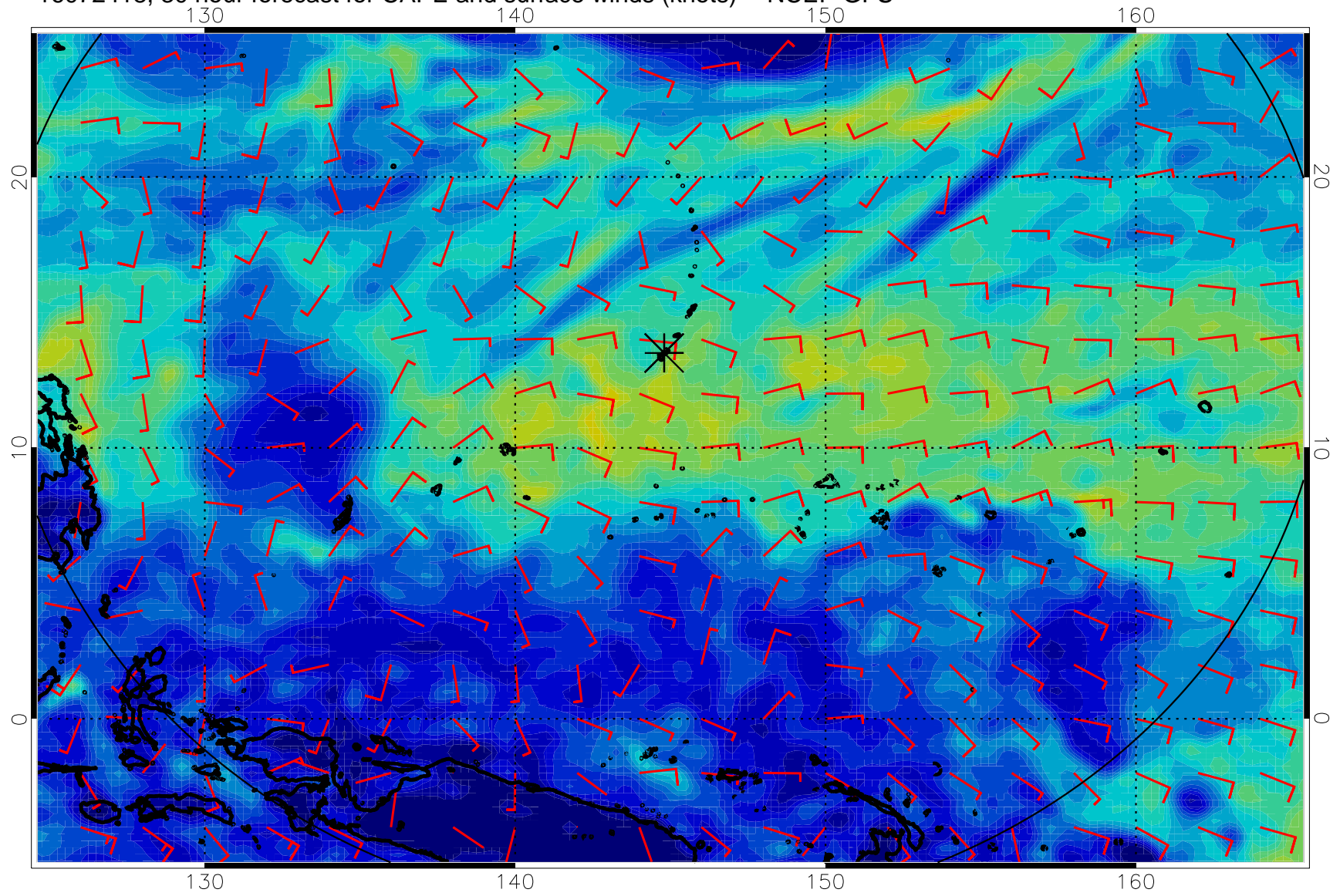
16072418, 30 hour forecast for CAPE and surface winds (knots) -- NCEP GFS
