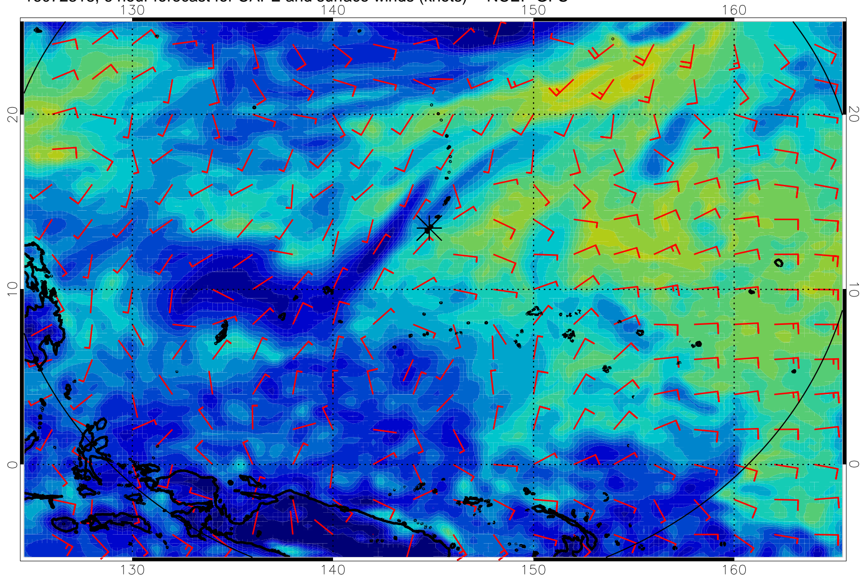
16072318, 6 hour forecast for CAPE and surface winds (knots) -- NCEP GFS
