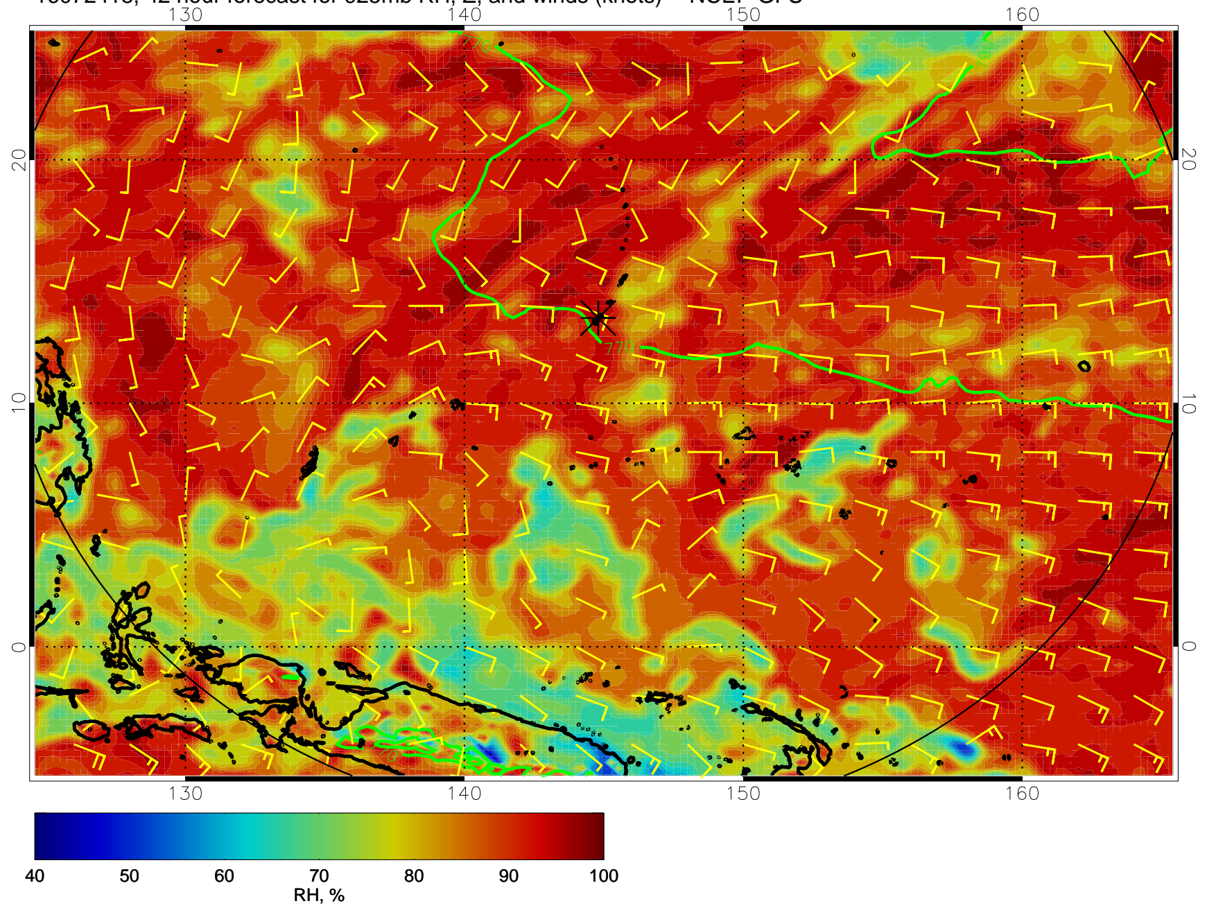
16072418, 42 hour forecast for 925mb RH, Z, and winds (knots) -- NCEP GFS
