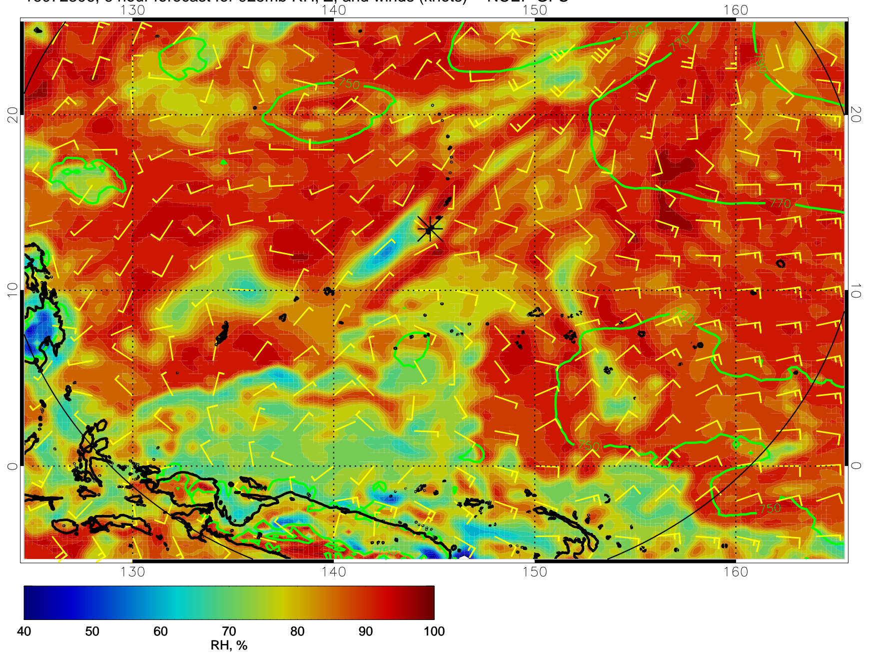
16072306, 6 hour forecast for 925mb RH, Z, and winds (knots) -- NCEP GFS
