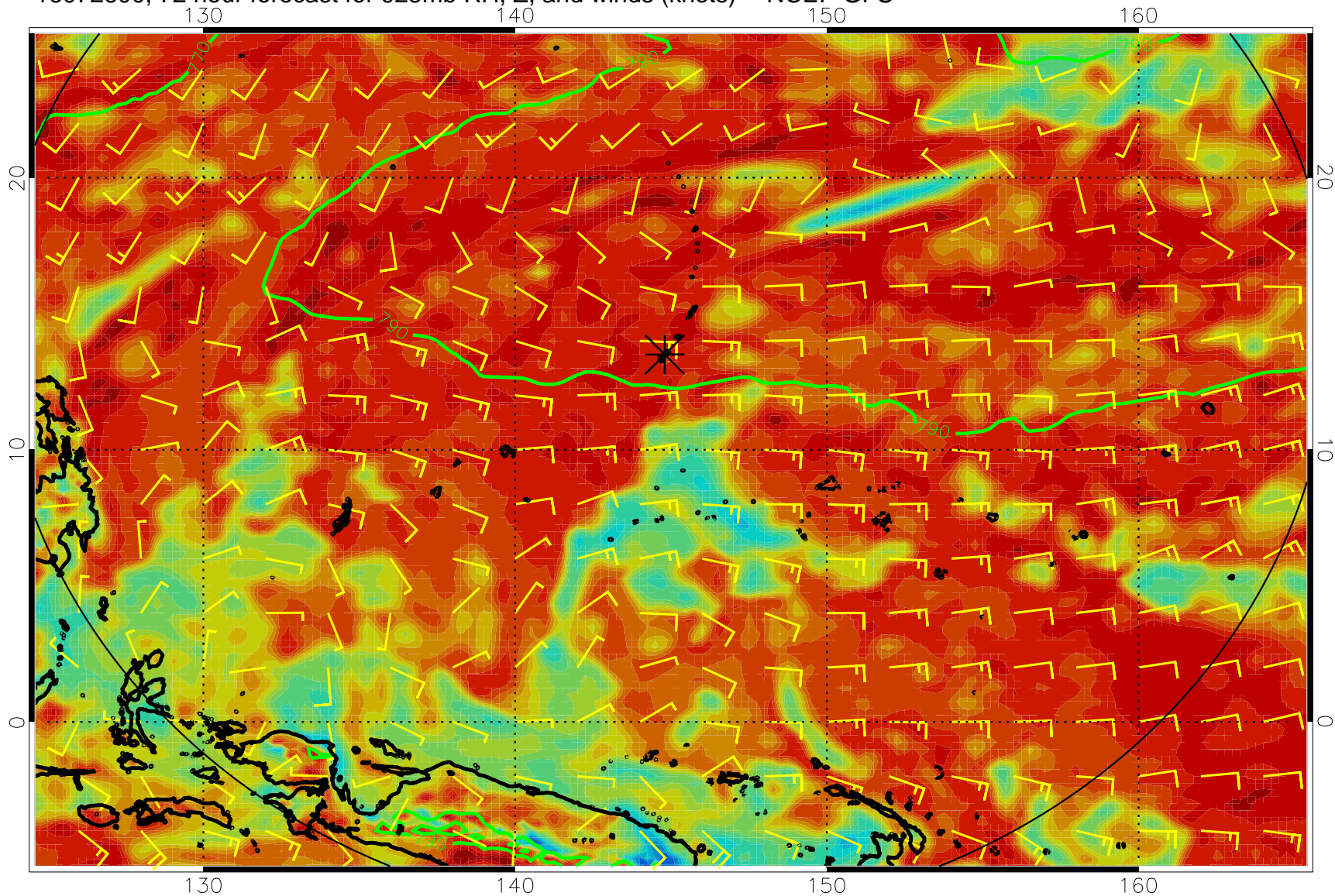
16072600, 72 hour forecast for 925mb RH, Z, and winds (knots) -- NCEP GFS
