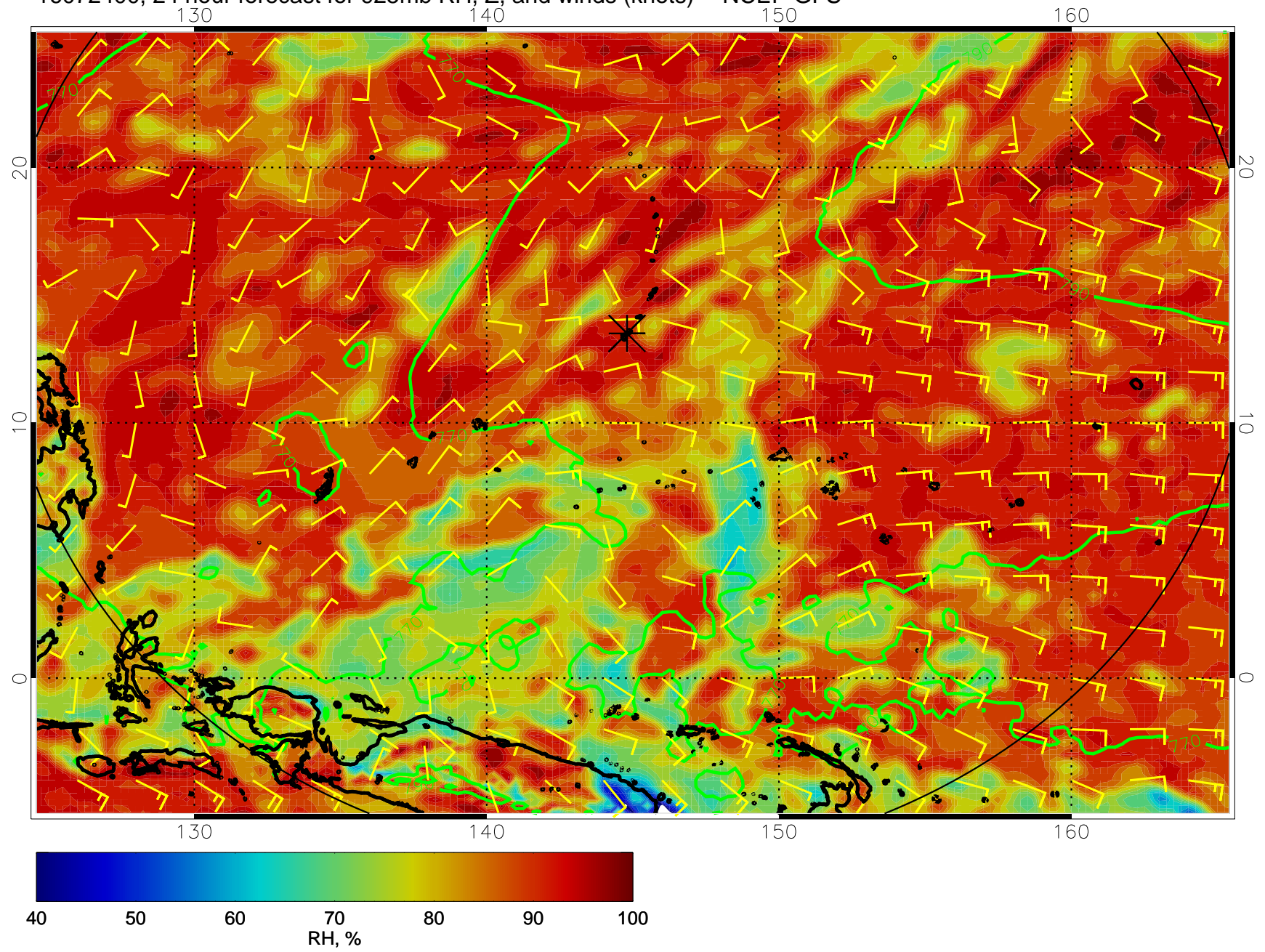
16072400, 24 hour forecast for 925mb RH, Z, and winds (knots) -- NCEP GFS
