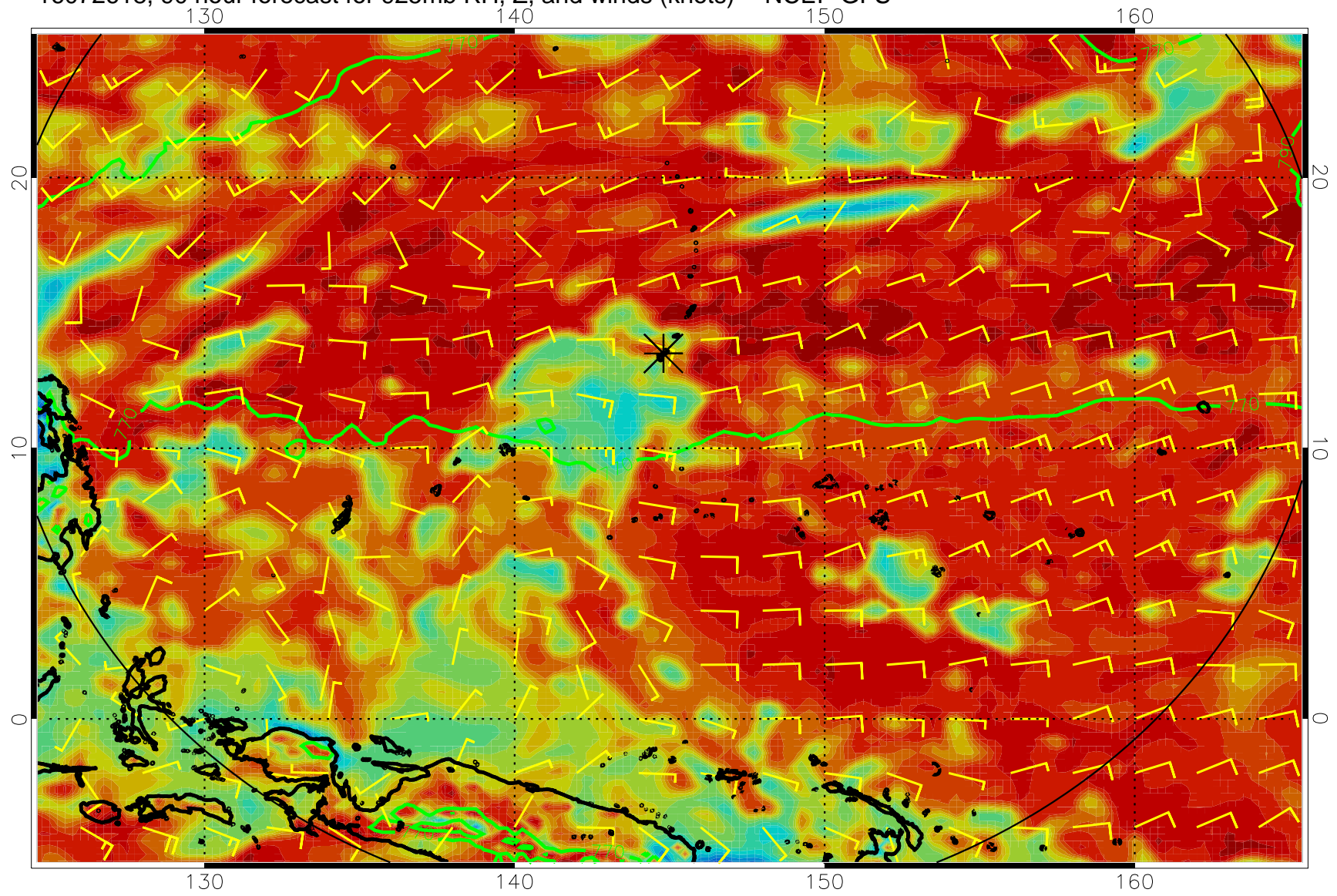
16072618, 90 hour forecast for 925mb RH, Z, and winds (knots) -- NCEP GFS
