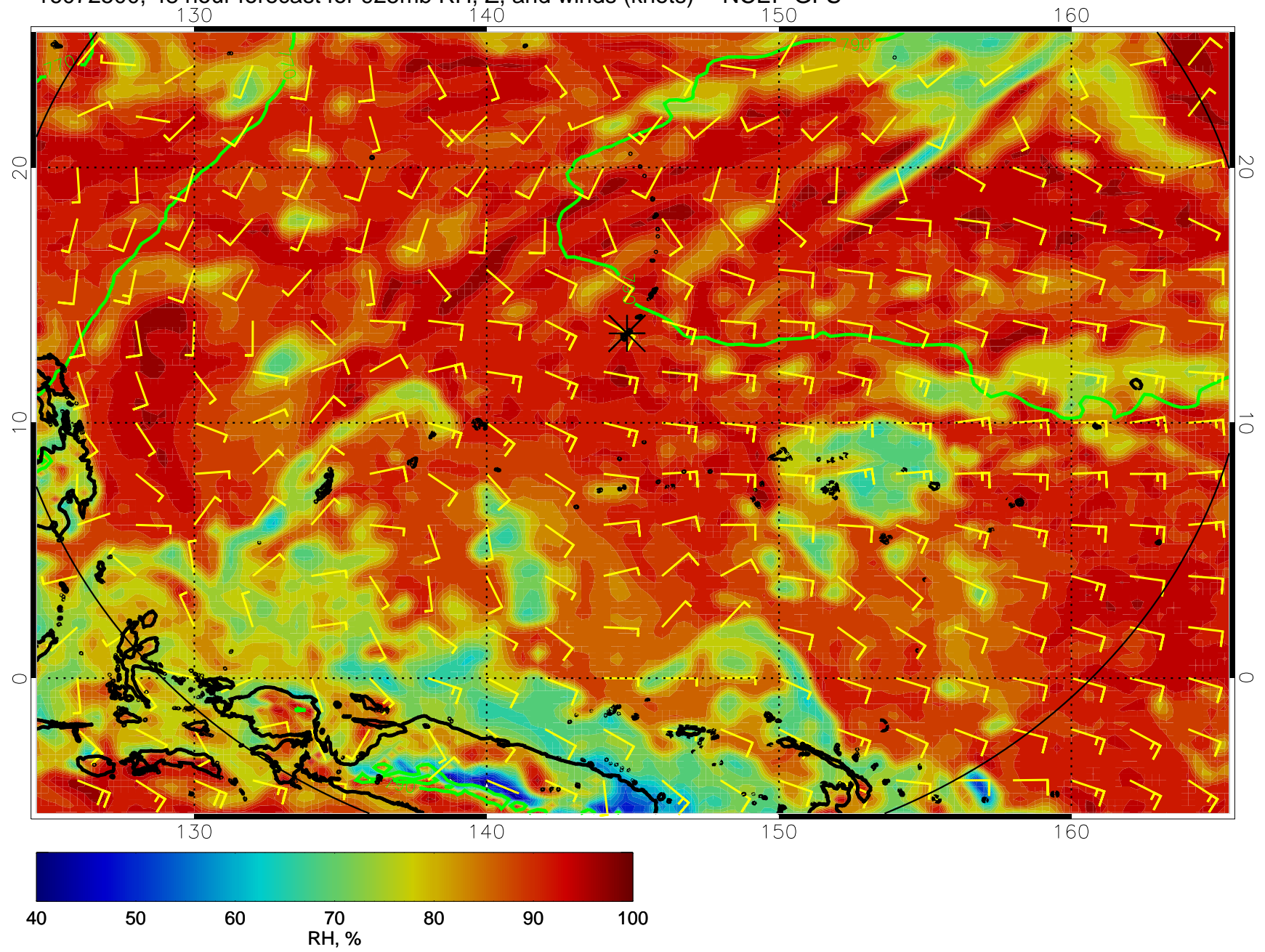
16072500, 48 hour forecast for 925mb RH, Z, and winds (knots) -- NCEP GFS
