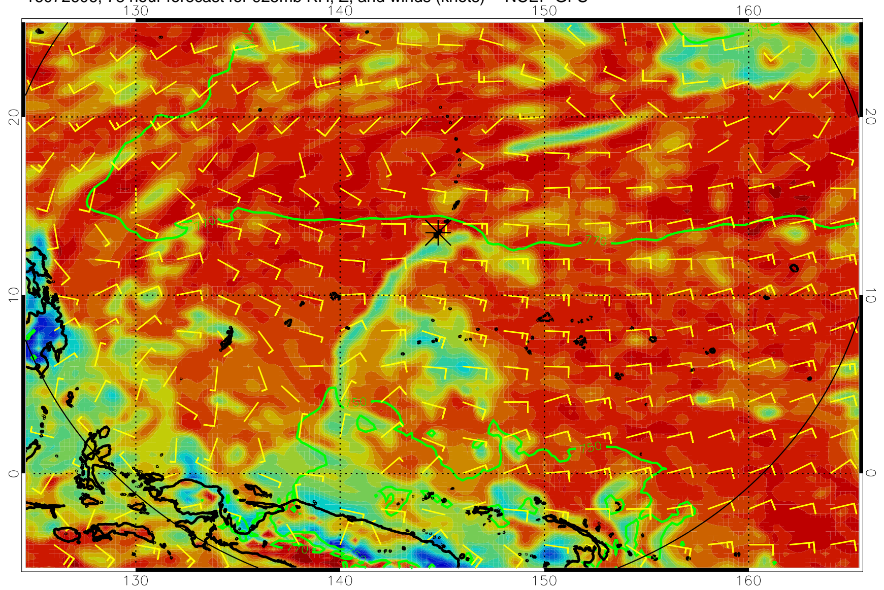
16072606, 78 hour forecast for 925mb RH, Z, and winds (knots) -- NCEP GFS
