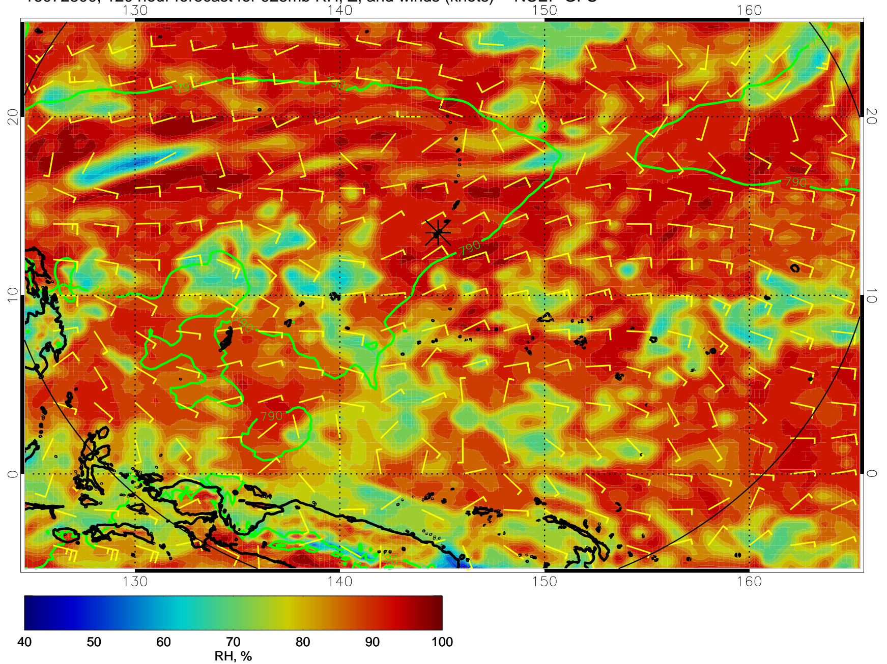
16072800, 120 hour forecast for 925mb RH, Z, and winds (knots) -- NCEP GFS
