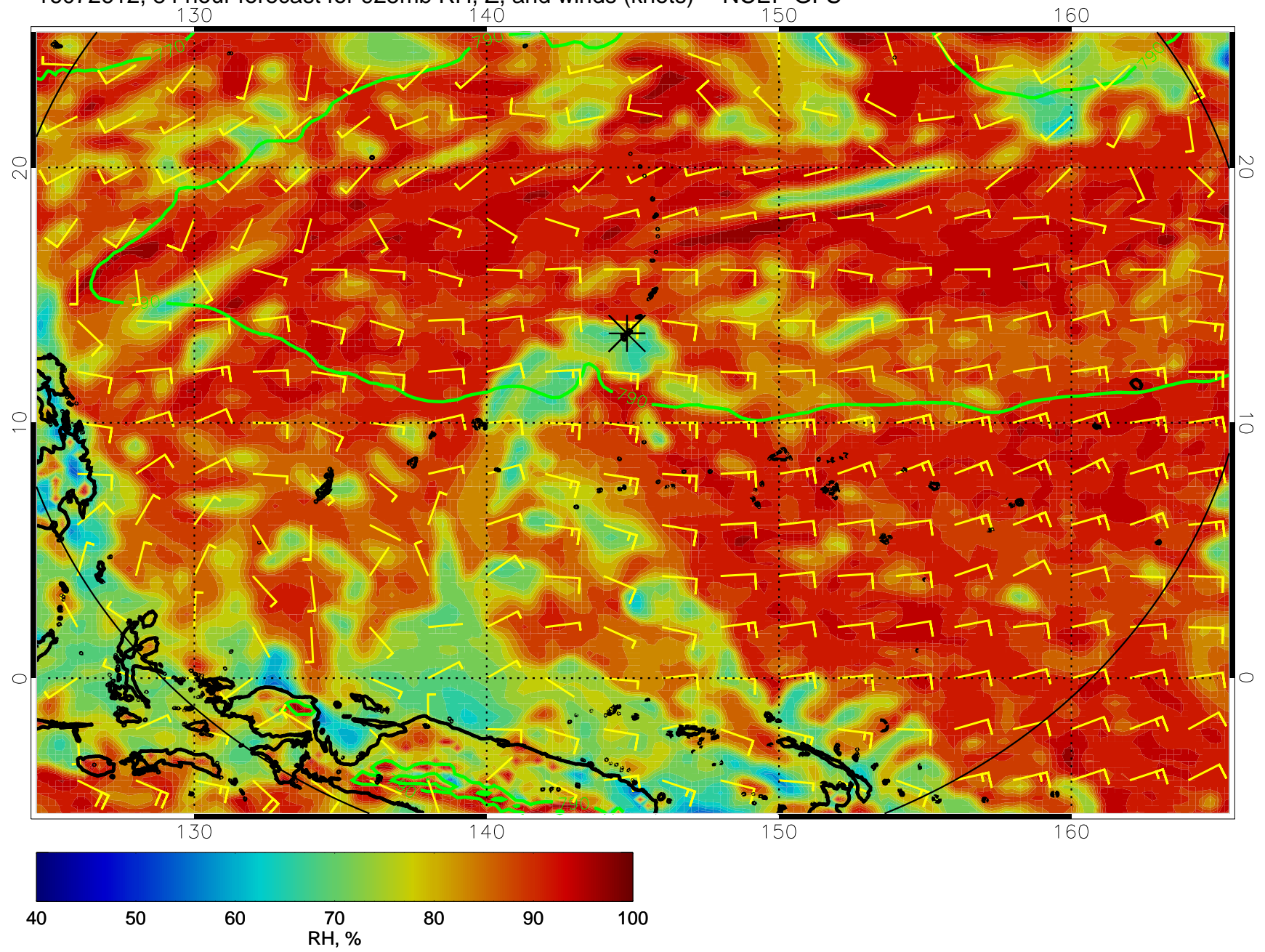
16072612, 84 hour forecast for 925mb RH, Z, and winds (knots) -- NCEP GFS
