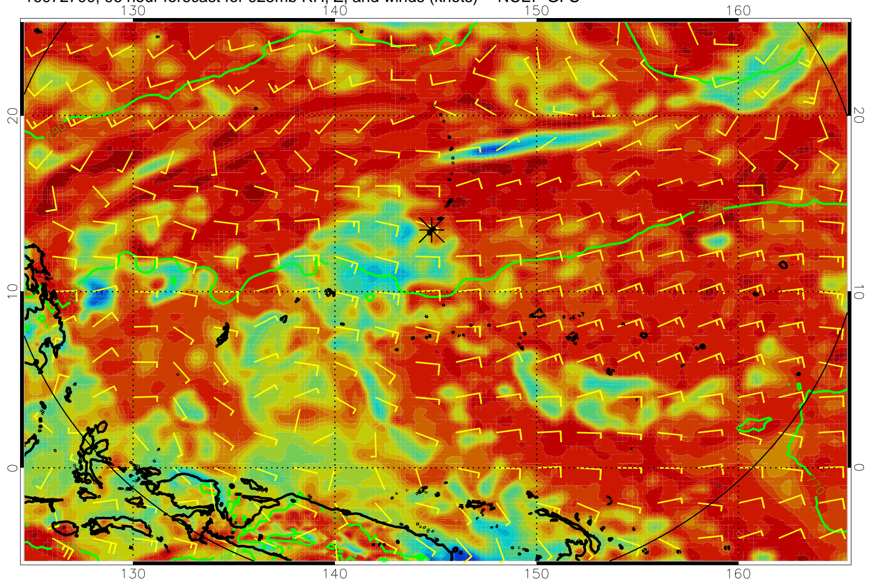
16072700, 96 hour forecast for 925mb RH, Z, and winds (knots) -- NCEP GFS
