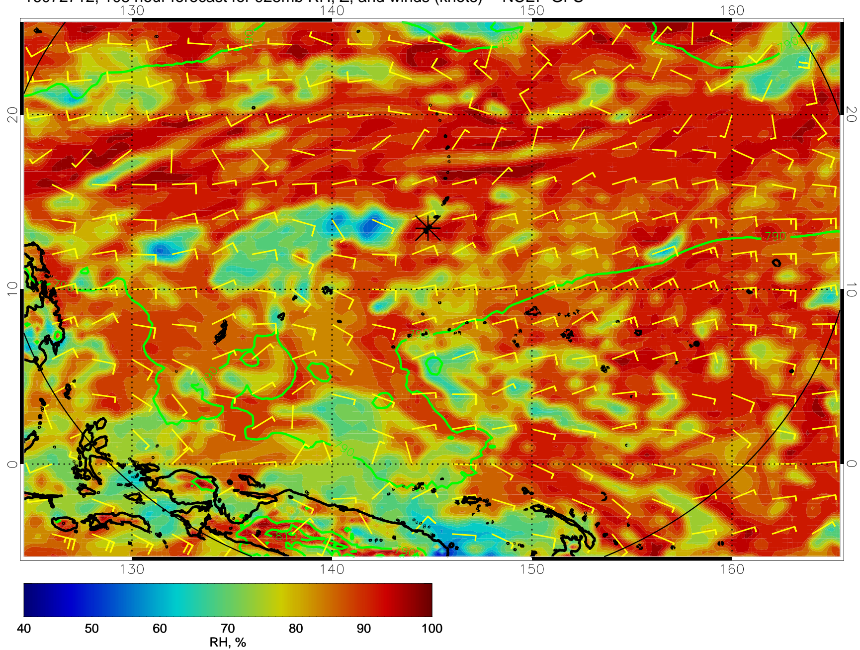
16072712, 108 hour forecast for 925mb RH, Z, and winds (knots) -- NCEP GFS
