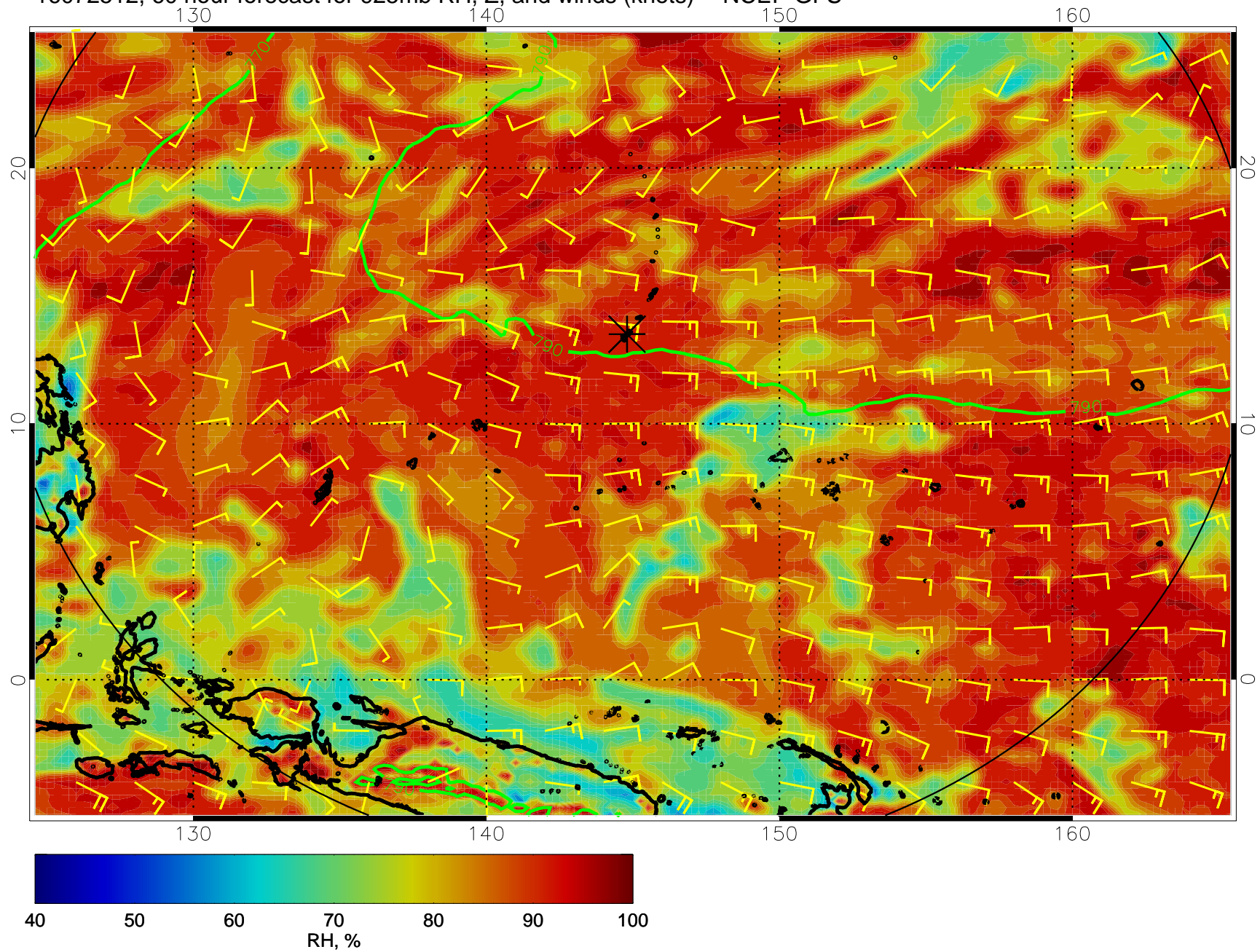
16072512, 60 hour forecast for 925mb RH, Z, and winds (knots) -- NCEP GFS
