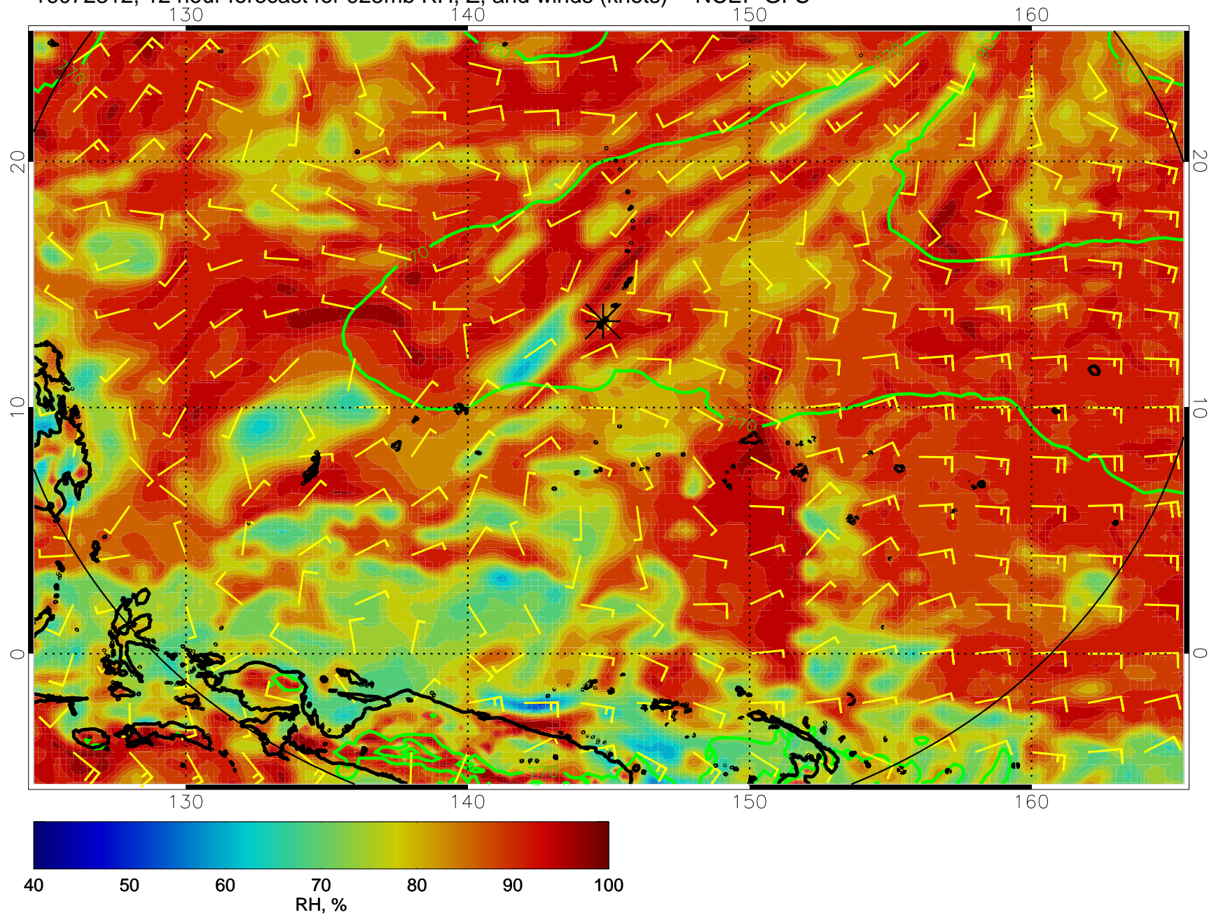
16072312, 12 hour forecast for 925mb RH, Z, and winds (knots) -- NCEP GFS
