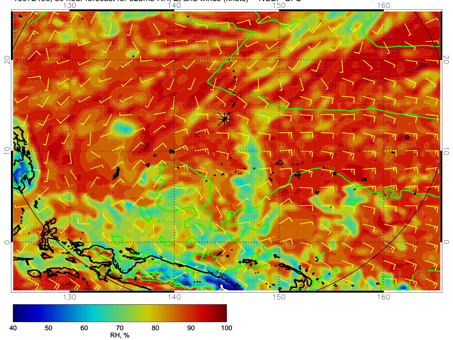
16072406, 30 hour forecast for 925mb RH, Z, and winds (knots) -- NCEP GFS
