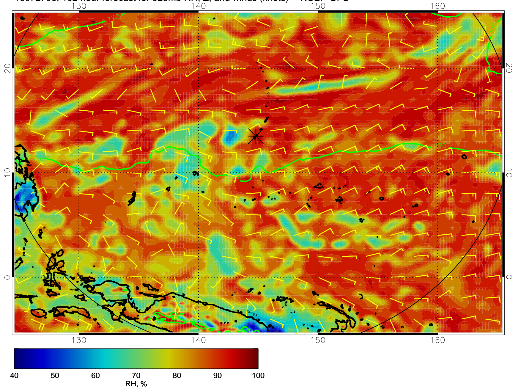
16072706, 102 hour forecast for 925mb RH, Z, and winds (knots) -- NCEP GFS
