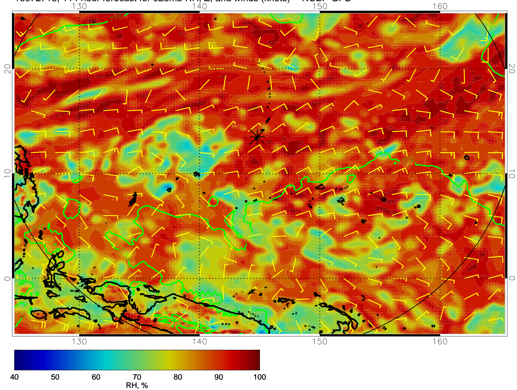
16072718, 114 hour forecast for 925mb RH, Z, and winds (knots) -- NCEP GFS
