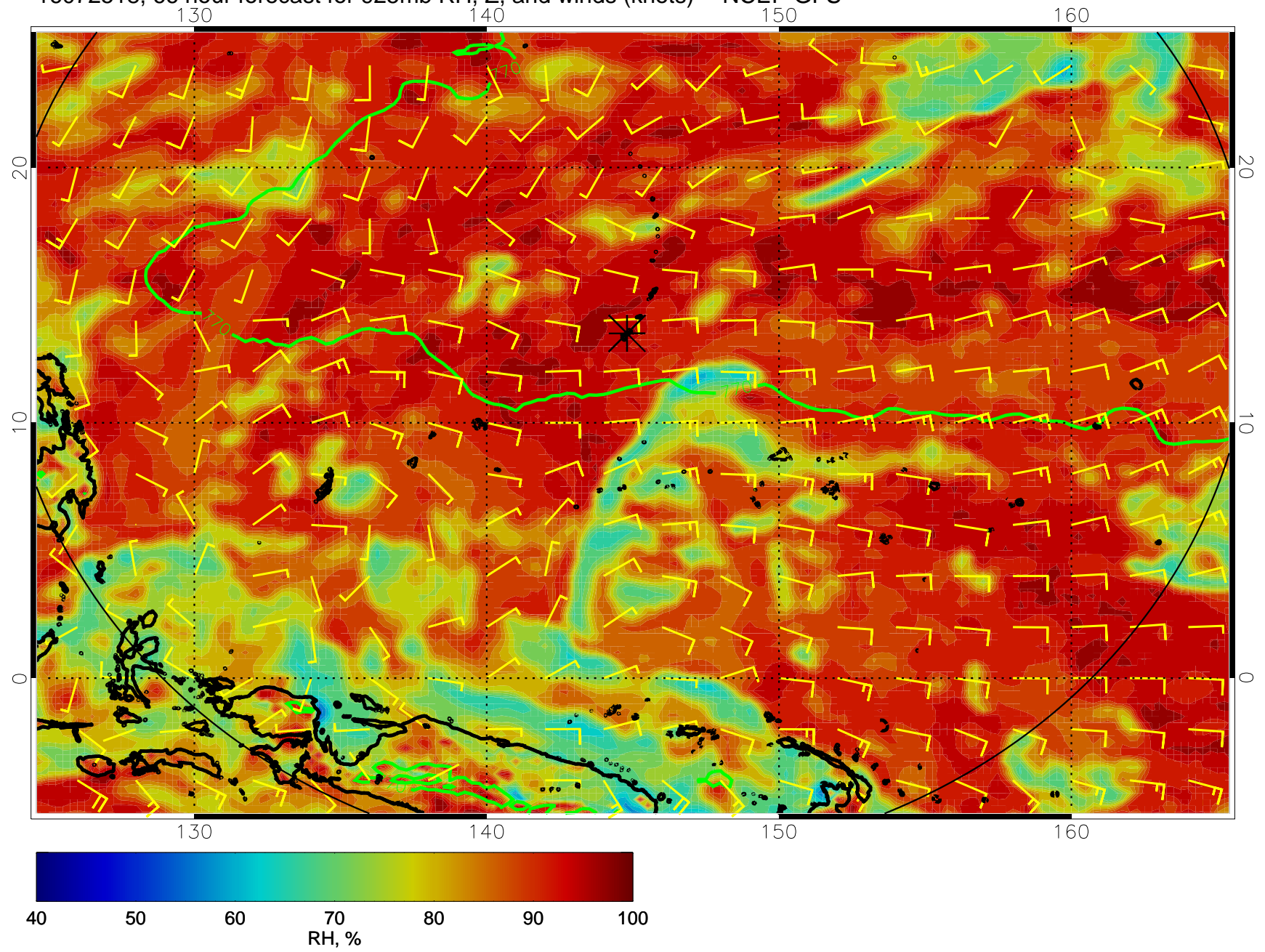
16072518, 66 hour forecast for 925mb RH, Z, and winds (knots) -- NCEP GFS
