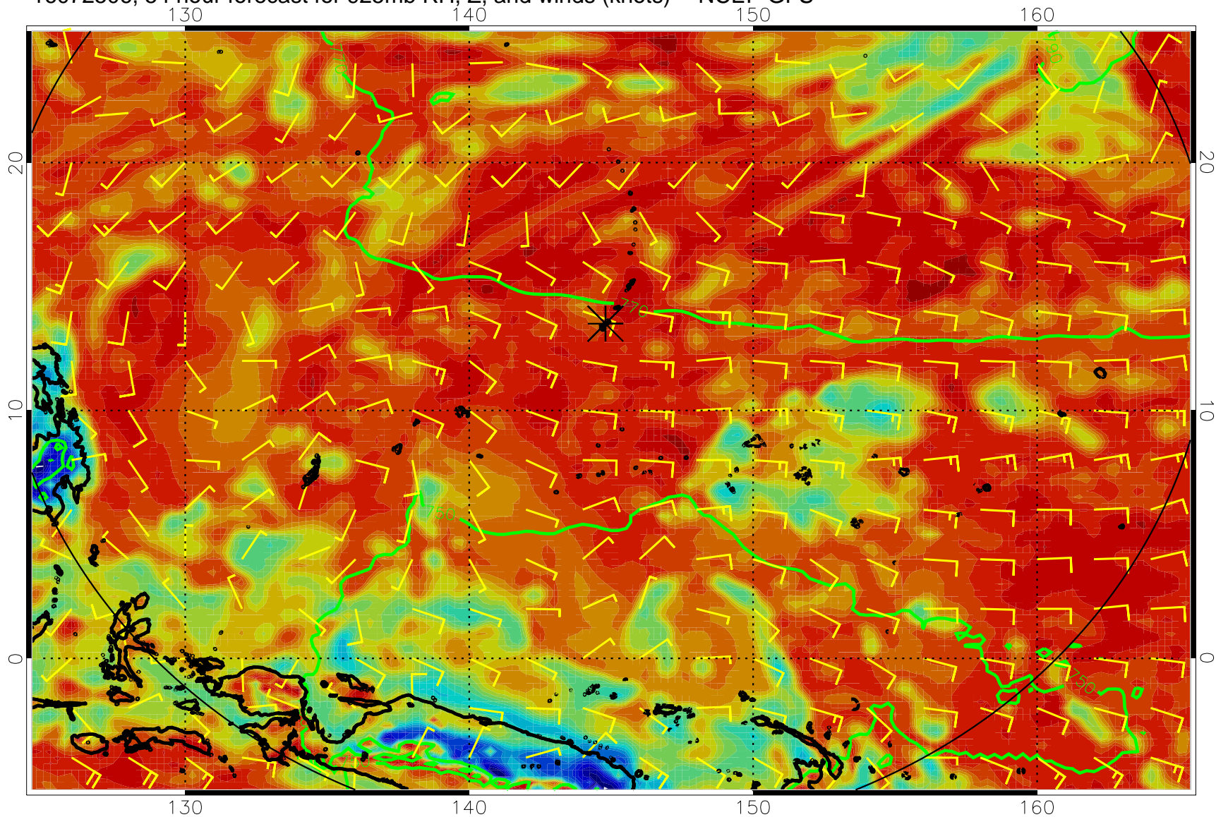
16072506, 54 hour forecast for 925mb RH, Z, and winds (knots) -- NCEP GFS
