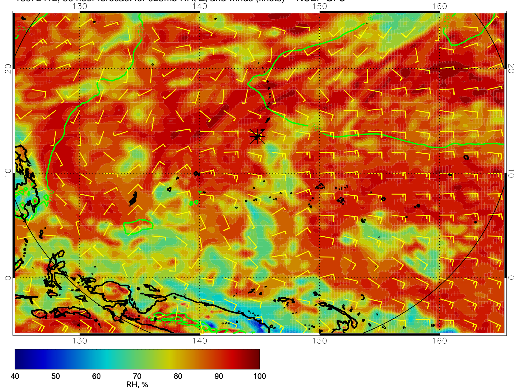
16072412, 36 hour forecast for 925mb RH, Z, and winds (knots) -- NCEP GFS
