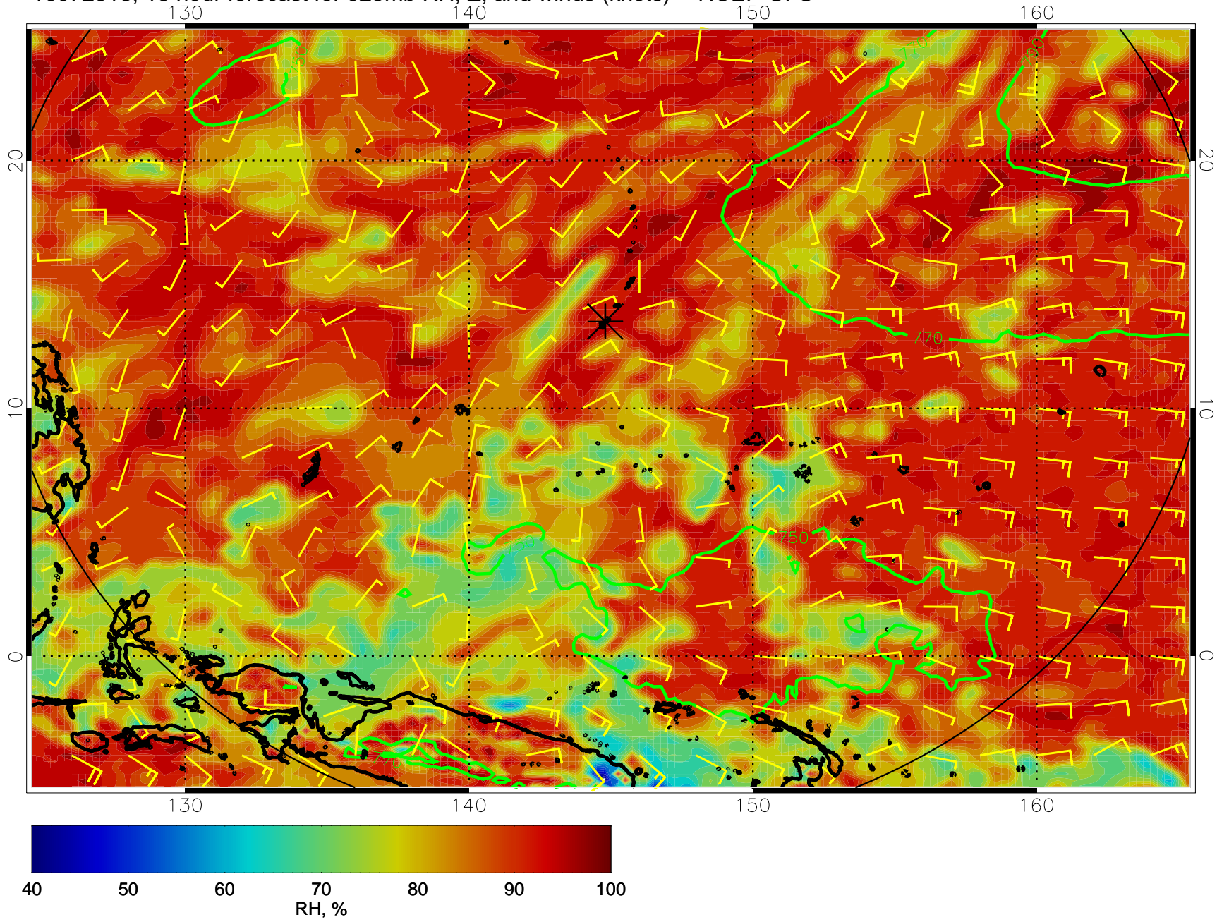
16072318, 18 hour forecast for 925mb RH, Z, and winds (knots) -- NCEP GFS
