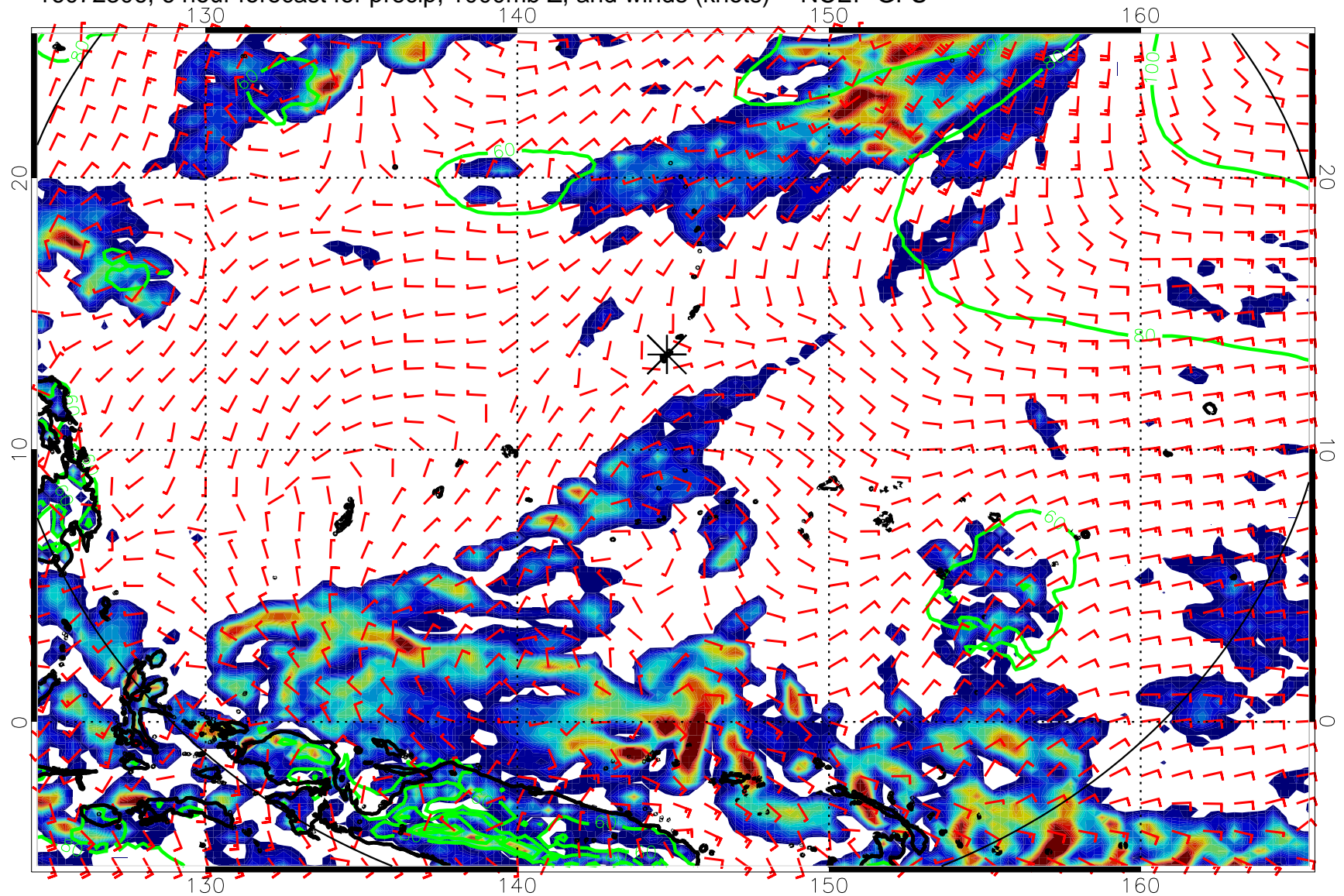
16072306, 6 hour forecast for precip, 1000mb Z, and winds (knots) -- NCEP GFS
