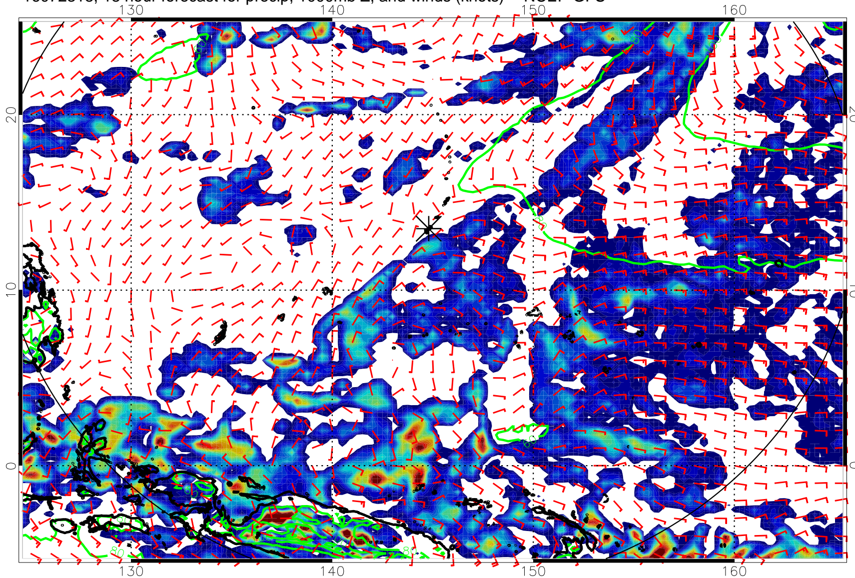
16072318, 18 hour forecast for precip, 1000mb Z, and winds (knots) -- NCEP GFS
