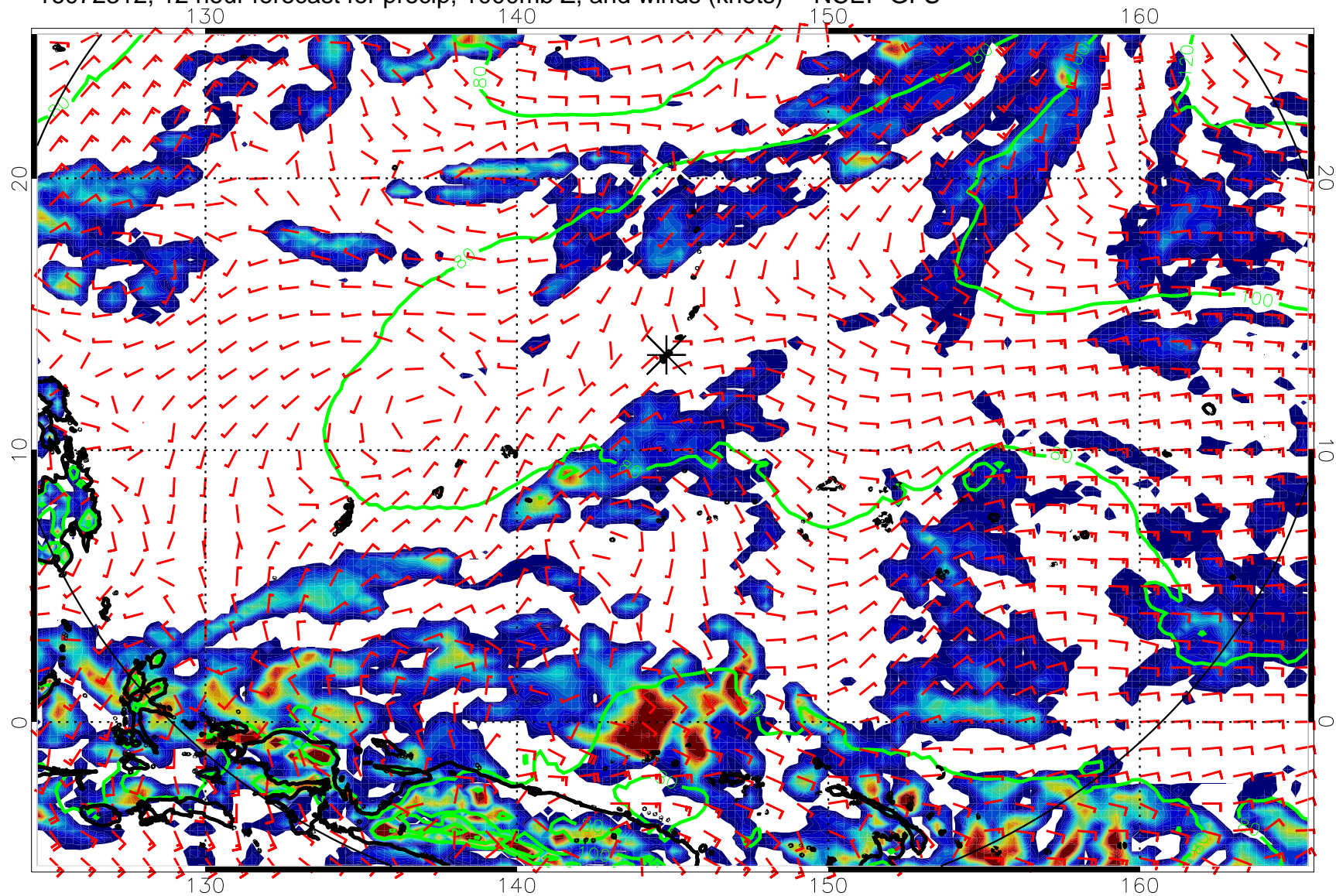
16072312, 12 hour forecast for precip, 1000mb Z, and winds (knots) -- NCEP GFS
