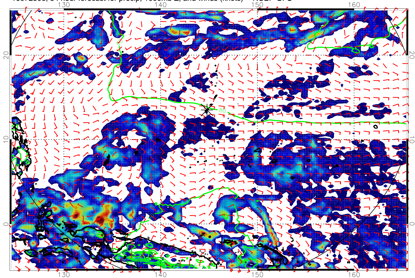
16072506, 54 hour forecast for precip, 1000mb Z, and winds (knots) -- NCEP GFS
