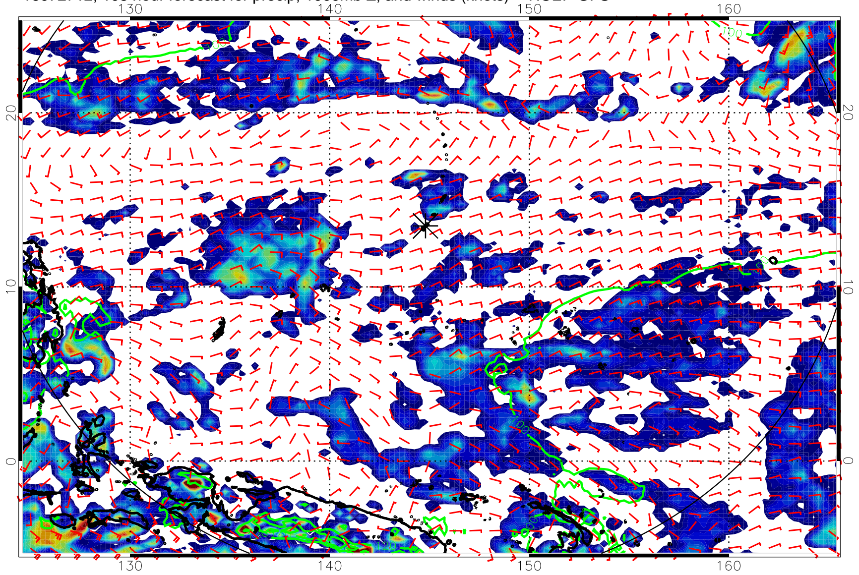
16072712, 108 hour forecast for precip, 1000mb Z, and winds (knots) -- NCEP GFS
