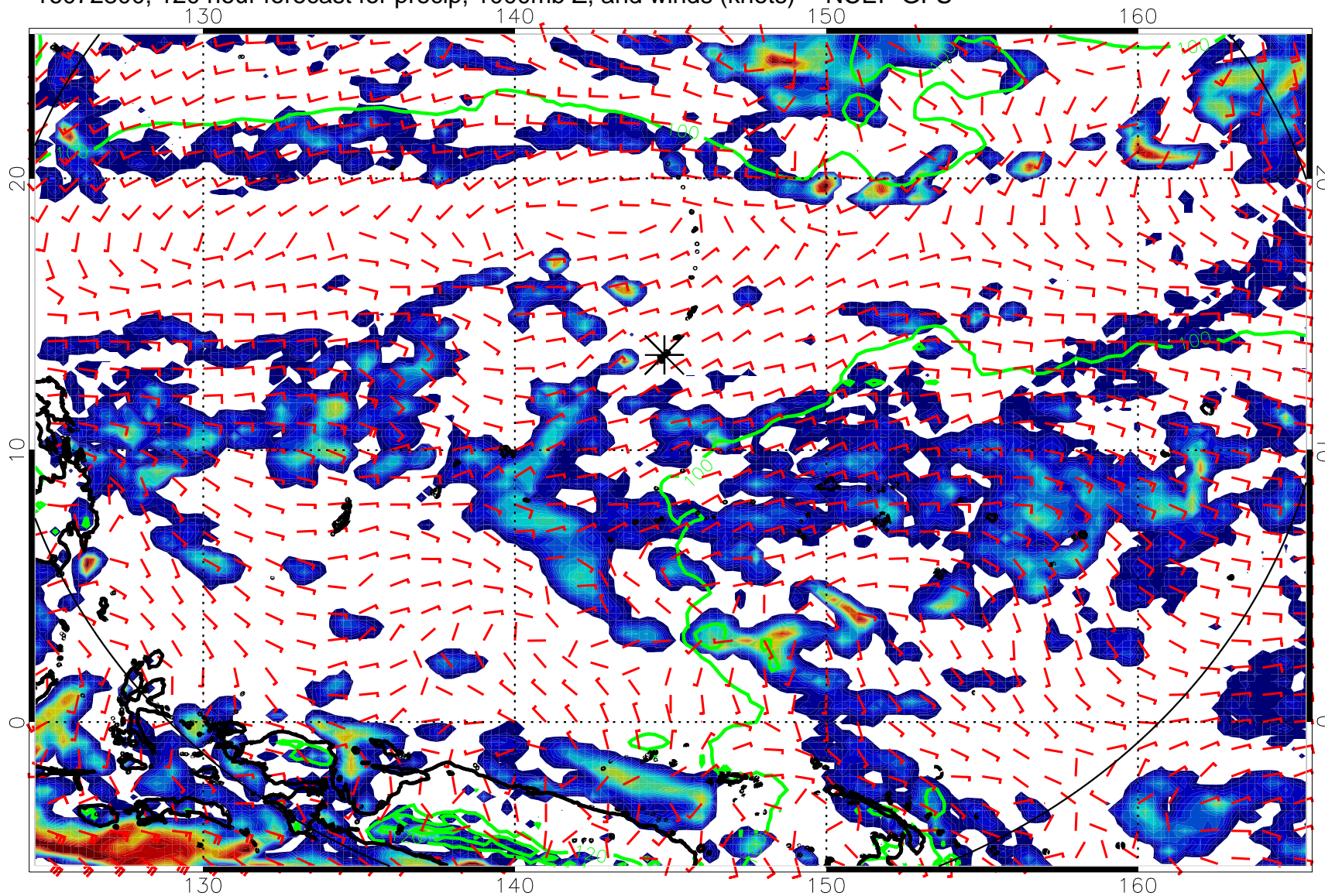
16072800, 120 hour forecast for precip, 1000mb Z, and winds (knots) -- NCEP GFS
