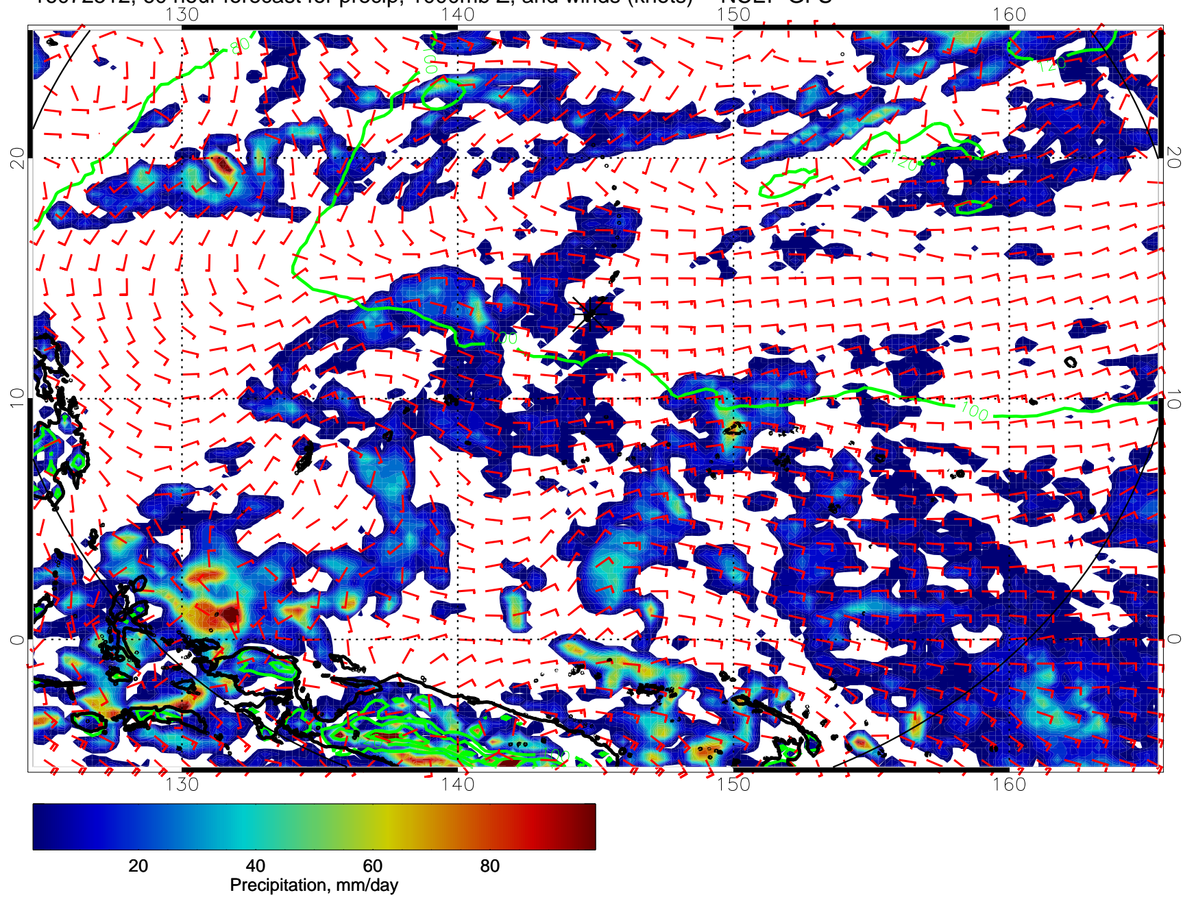
16072512, 60 hour forecast for precip, 1000mb Z, and winds (knots) -- NCEP GFS
