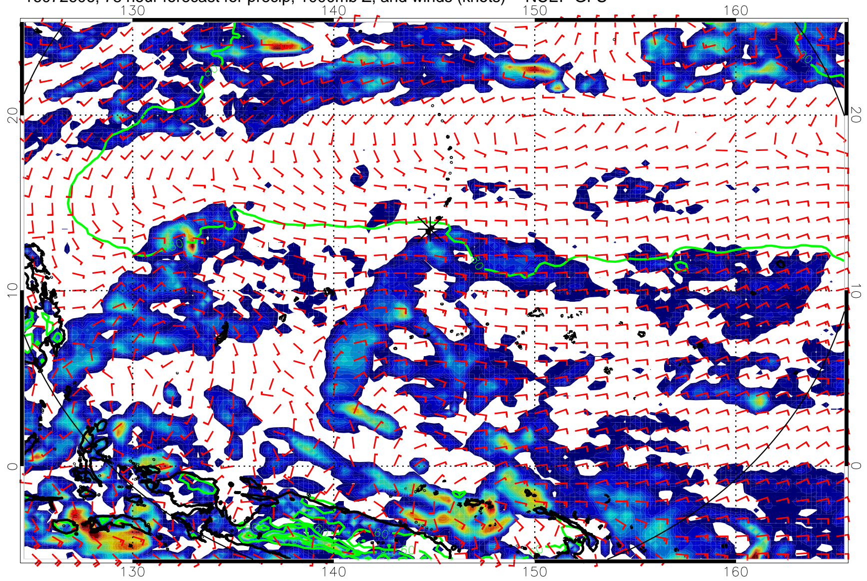
16072606, 78 hour forecast for precip, 1000mb Z, and winds (knots) -- NCEP GFS
