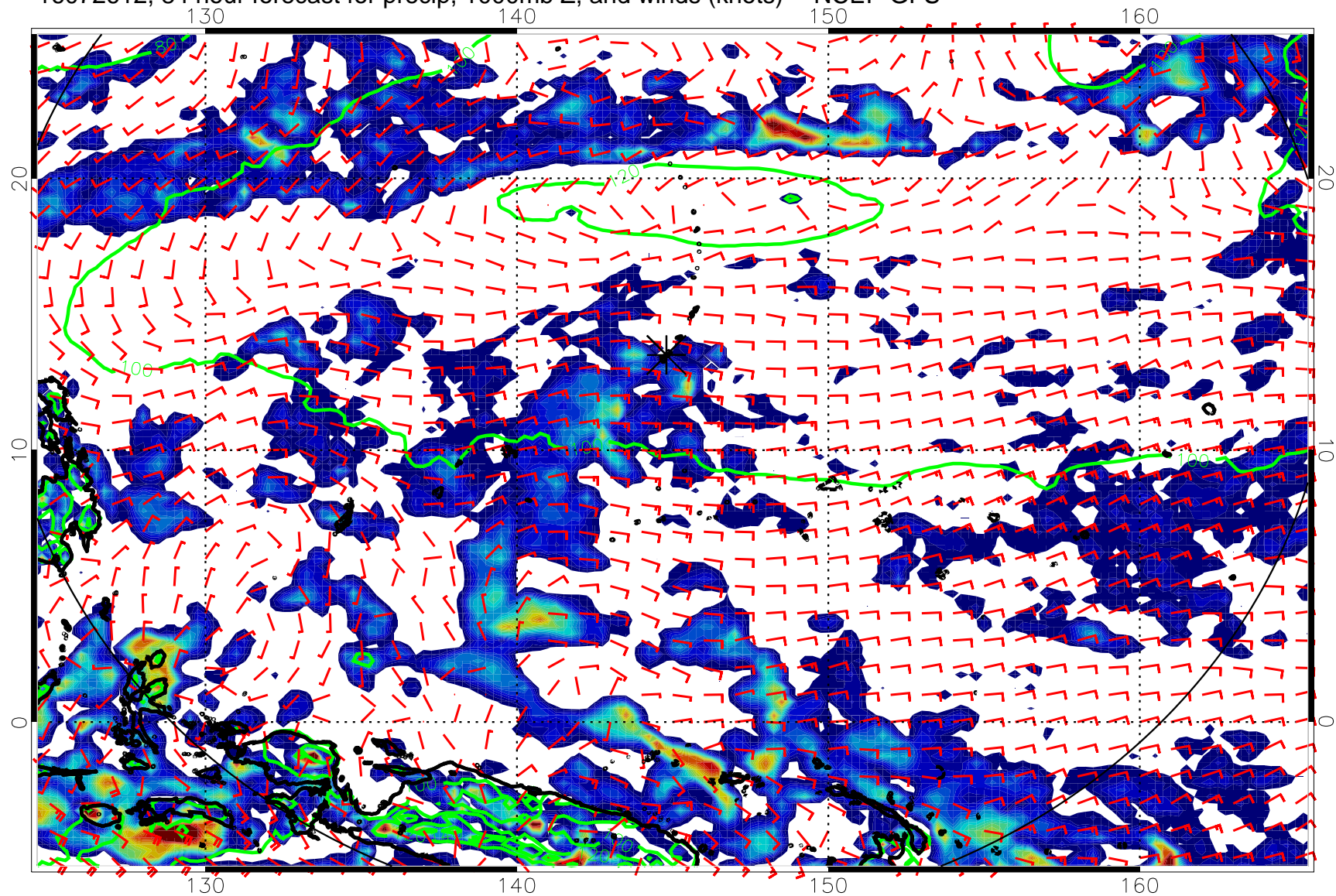
16072612, 84 hour forecast for precip, 1000mb Z, and winds (knots) -- NCEP GFS
