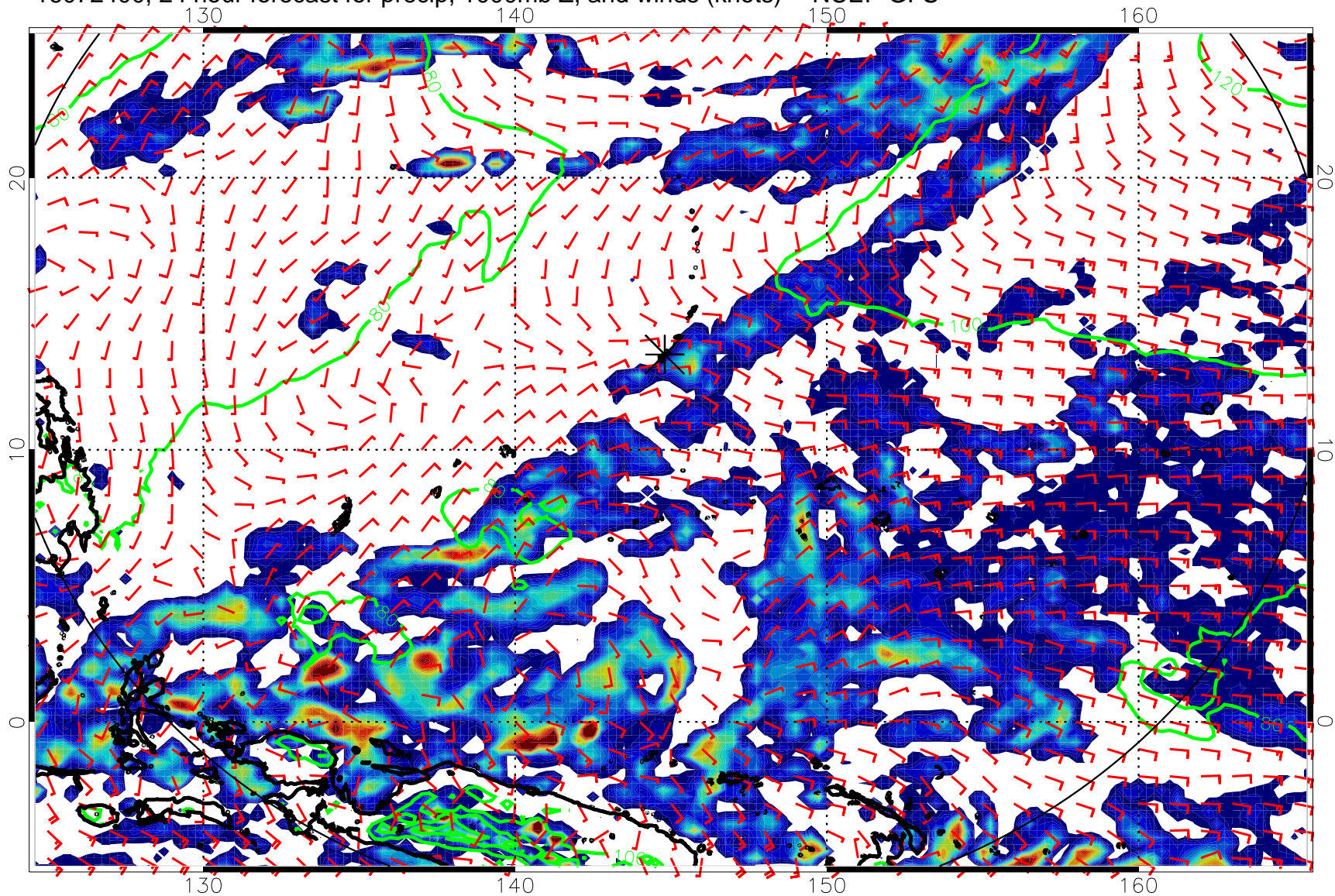
16072400, 24 hour forecast for precip, 1000mb Z, and winds (knots) -- NCEP GFS
