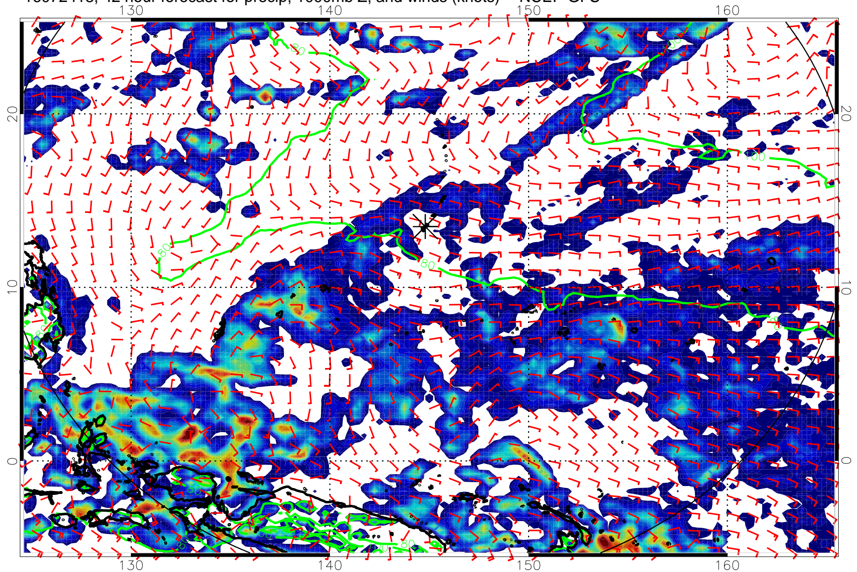
16072418, 42 hour forecast for precip, 1000mb Z, and winds (knots) -- NCEP GFS
