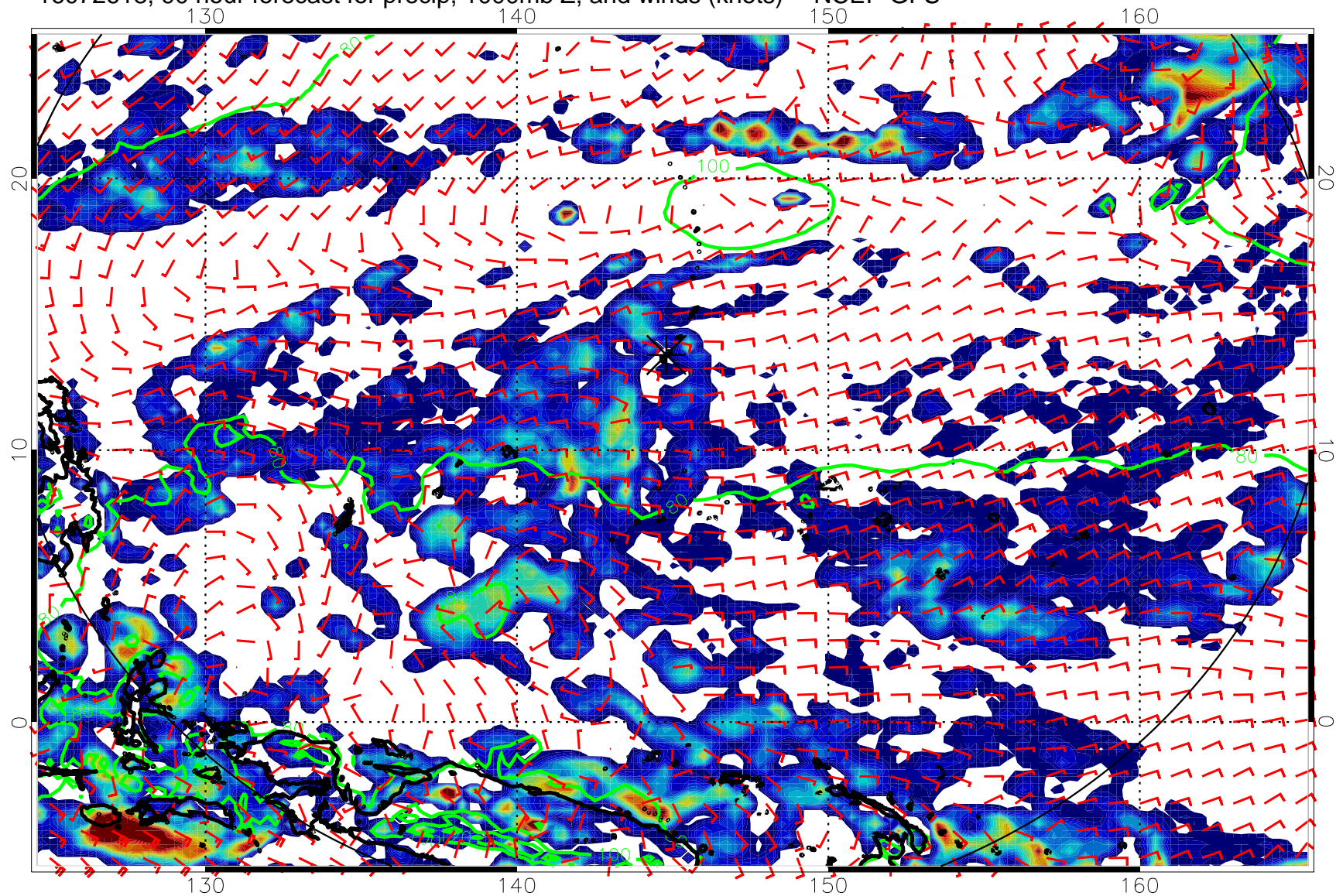
16072618, 90 hour forecast for precip, 1000mb Z, and winds (knots) -- NCEP GFS
