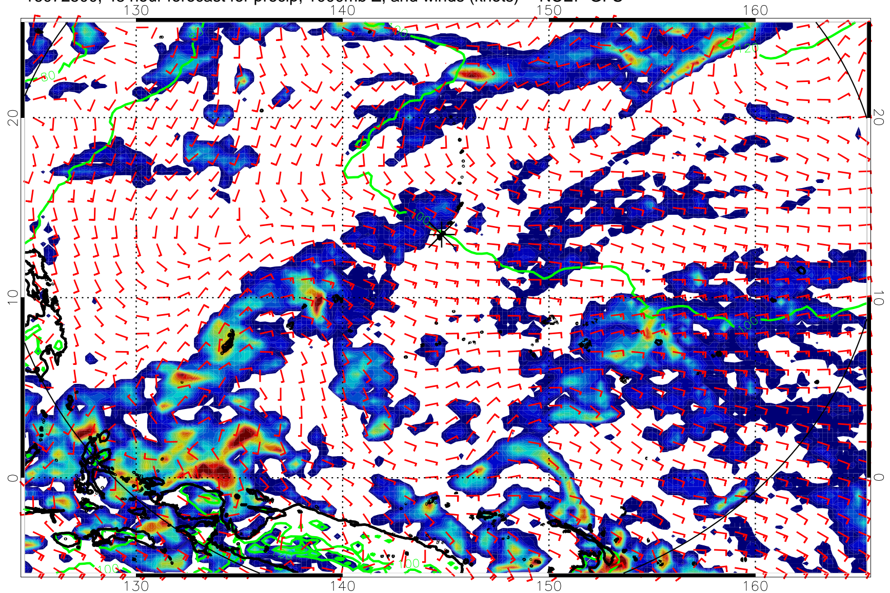
16072500, 48 hour forecast for precip, 1000mb Z, and winds (knots) -- NCEP GFS
