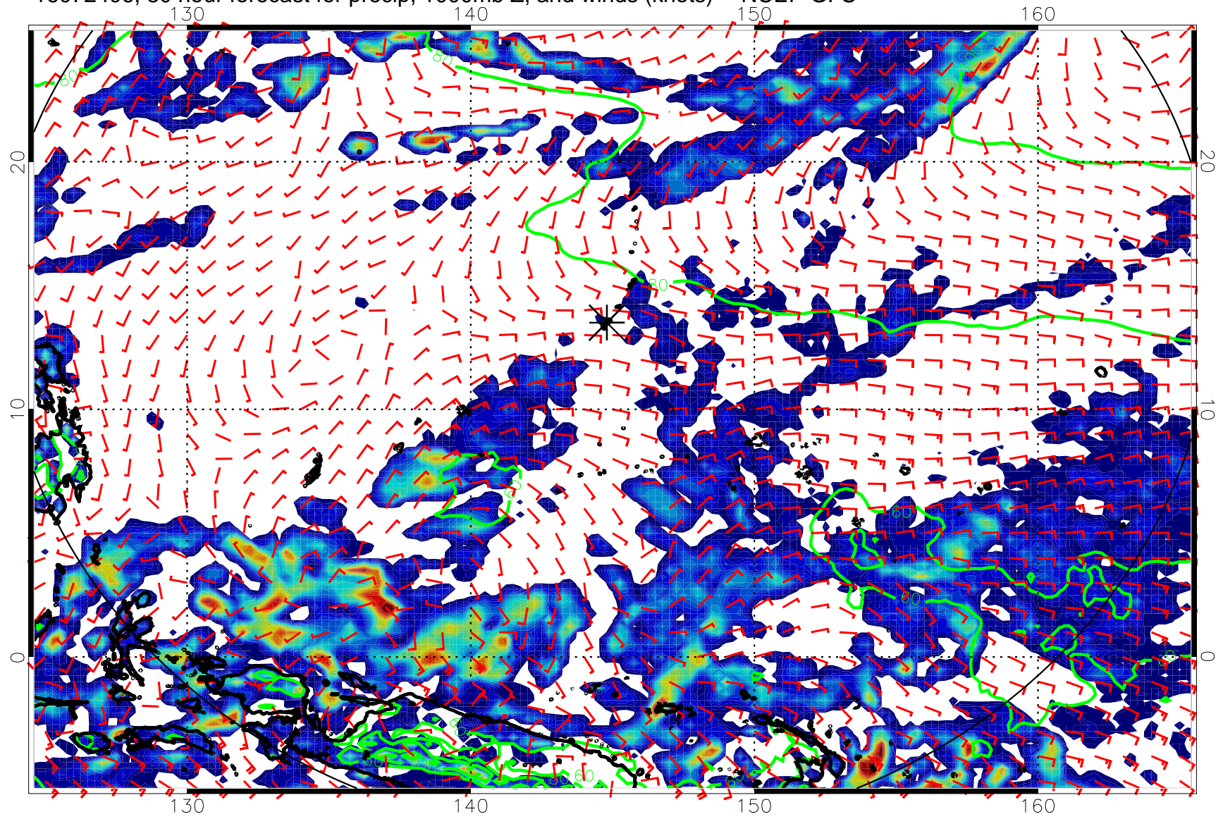
16072406, 30 hour forecast for precip, 1000mb Z, and winds (knots) -- NCEP GFS
