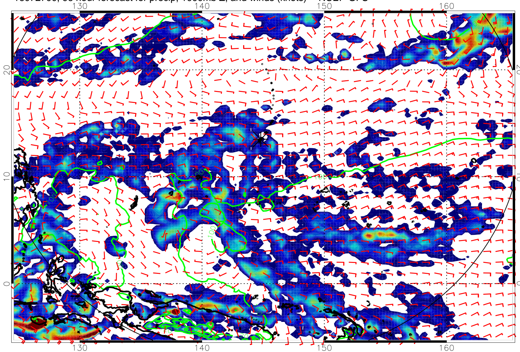
16072700, 96 hour forecast for precip, 1000mb Z, and winds (knots) -- NCEP GFS
