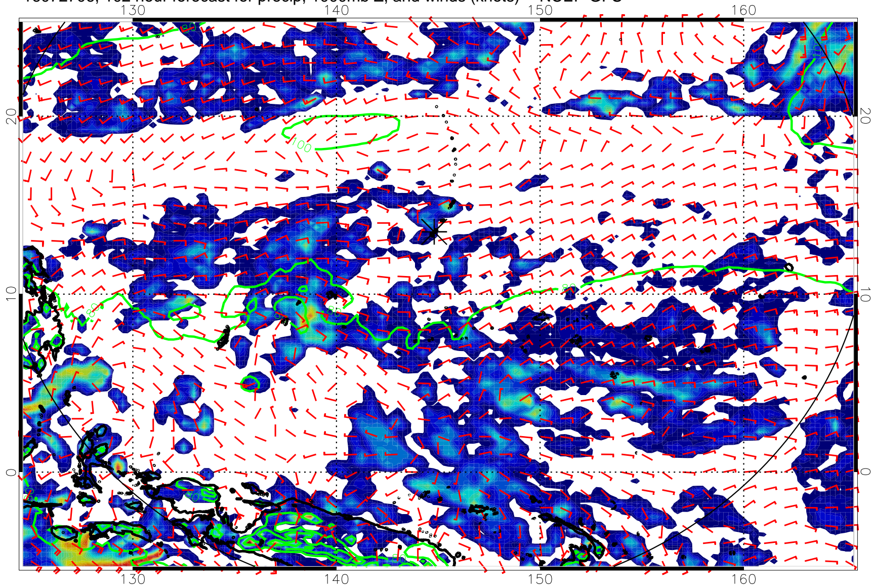
16072706, 102 hour forecast for precip, 1000mb Z, and winds (knots) -- NCEP GFS
