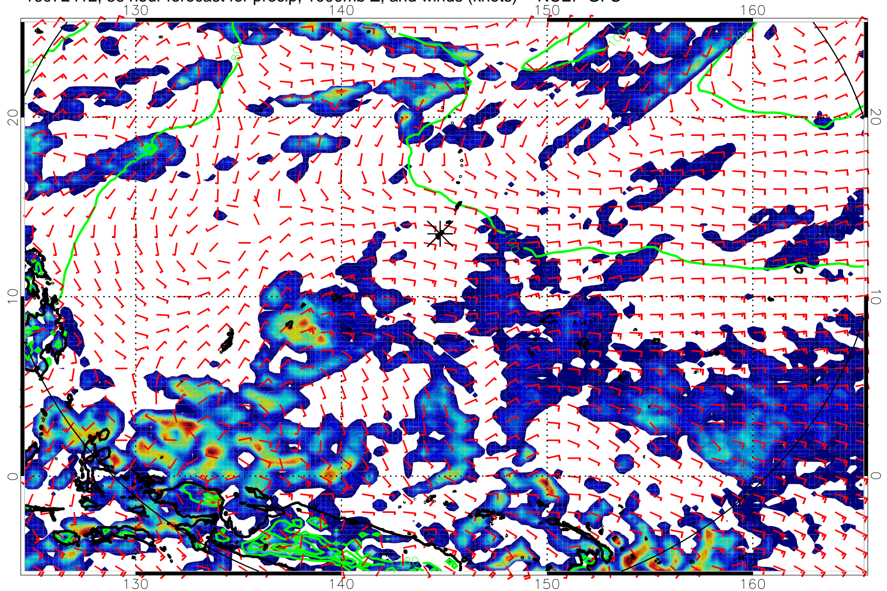
16072412, 36 hour forecast for precip, 1000mb Z, and winds (knots) -- NCEP GFS
