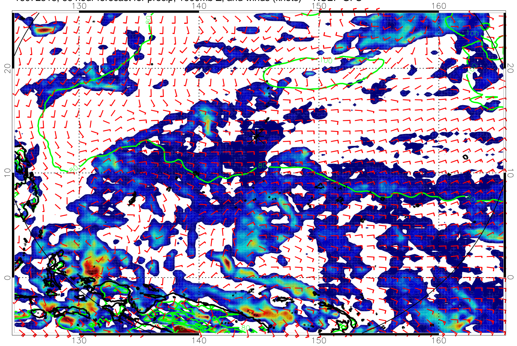
16072518, 66 hour forecast for precip, 1000mb Z, and winds (knots) -- NCEP GFS
