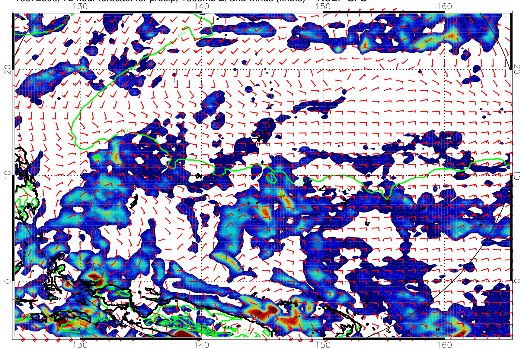
16072600, 72 hour forecast for precip, 1000mb Z, and winds (knots) -- NCEP GFS
