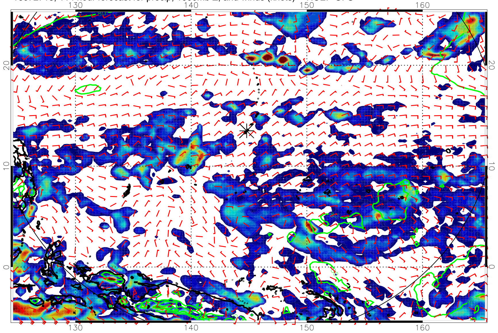
16072718, 114 hour forecast for precip, 1000mb Z, and winds (knots) -- NCEP GFS
