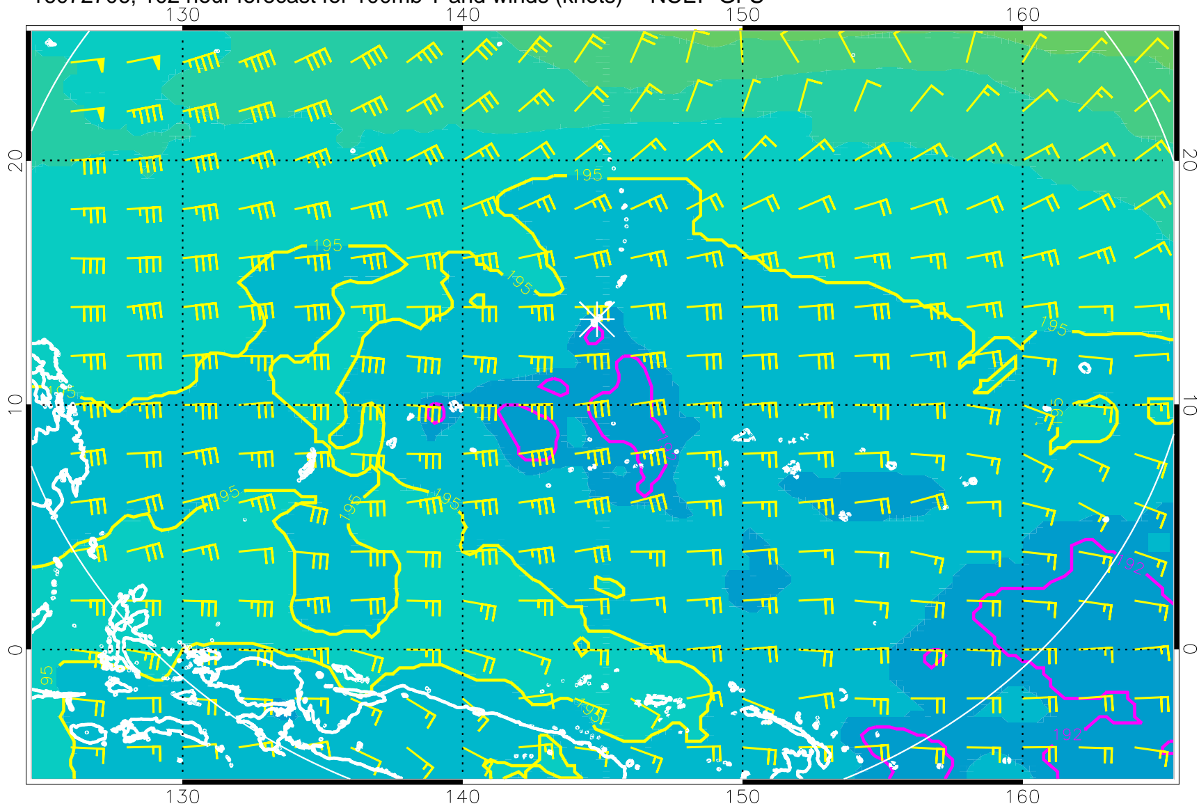
16072706, 102 hour forecast for 100mb T and winds (knots) -- NCEP GFS
