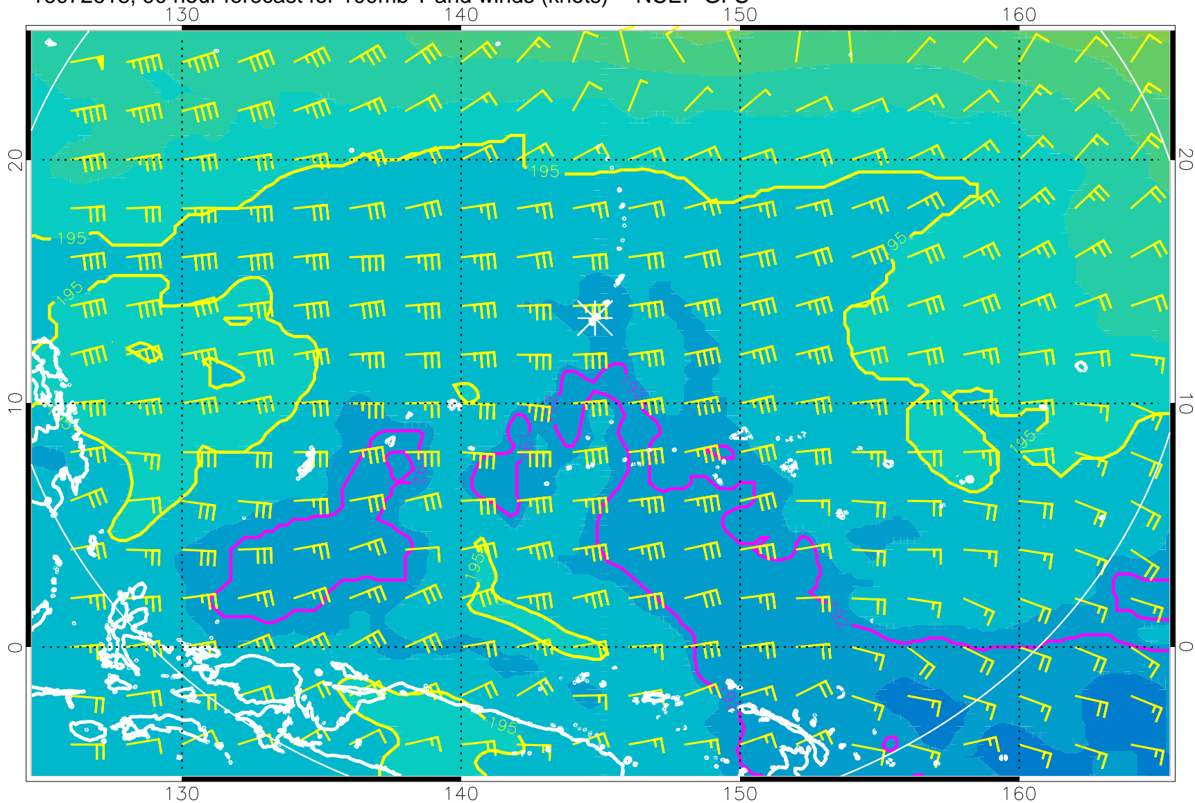
16072618, 90 hour forecast for 100mb T and winds (knots) -- NCEP GFS
