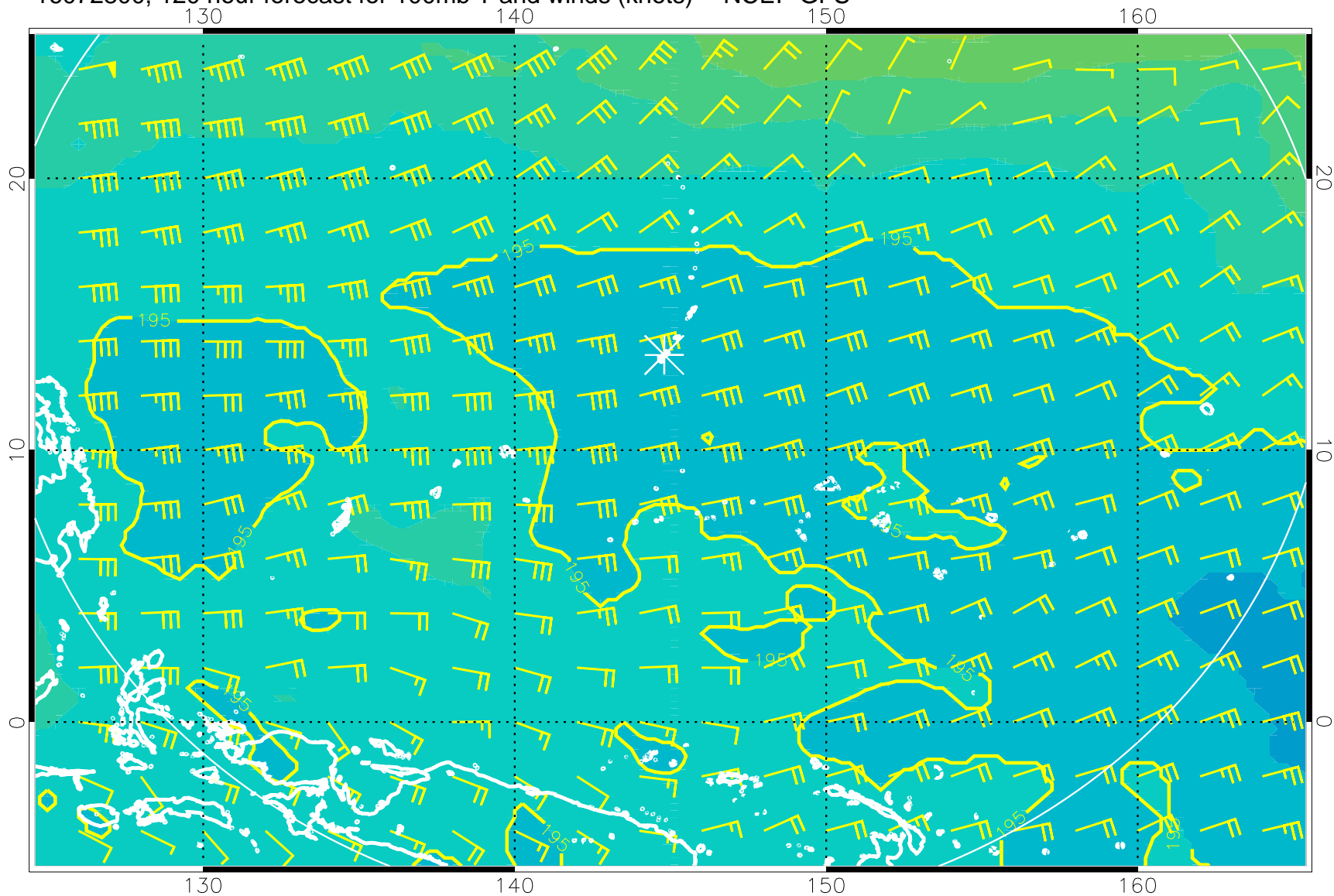
16072800, 120 hour forecast for 100mb T and winds (knots) -- NCEP GFS
