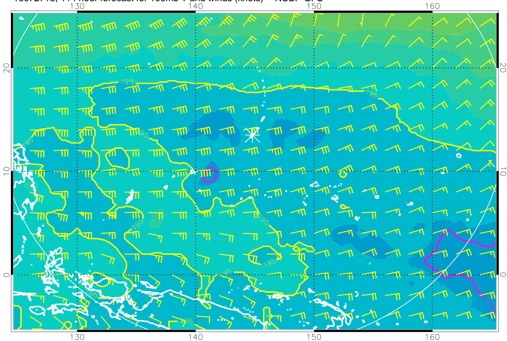
16072718, 114 hour forecast for 100mb T and winds (knots) -- NCEP GFS
