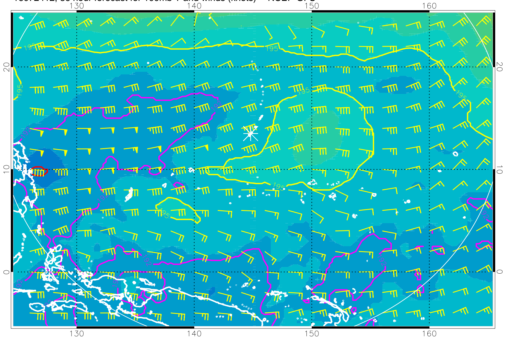
16072412, 36 hour forecast for 100mb T and winds (knots) -- NCEP GFS
