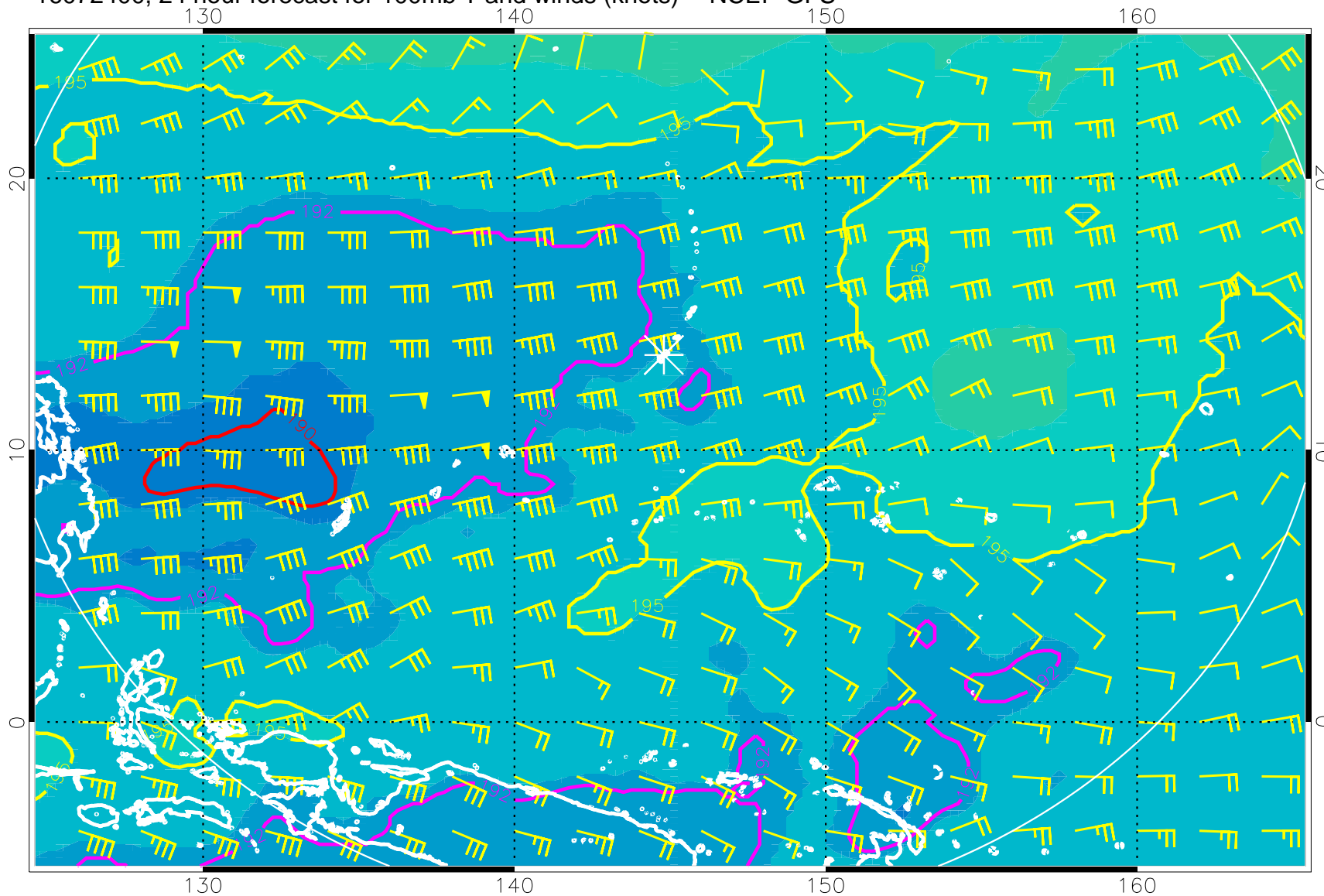
16072400, 24 hour forecast for 100mb T and winds (knots) -- NCEP GFS
