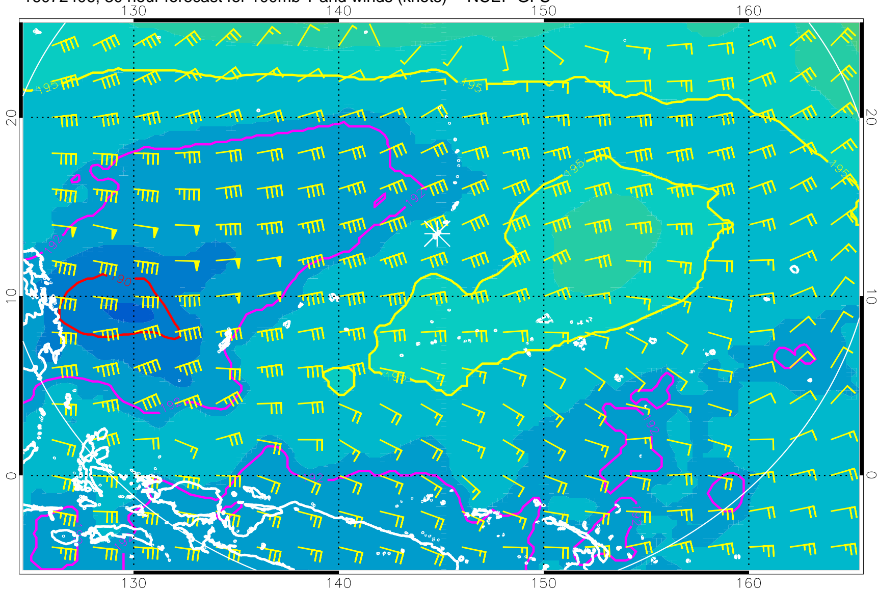
16072406, 30 hour forecast for 100mb T and winds (knots) -- NCEP GFS
