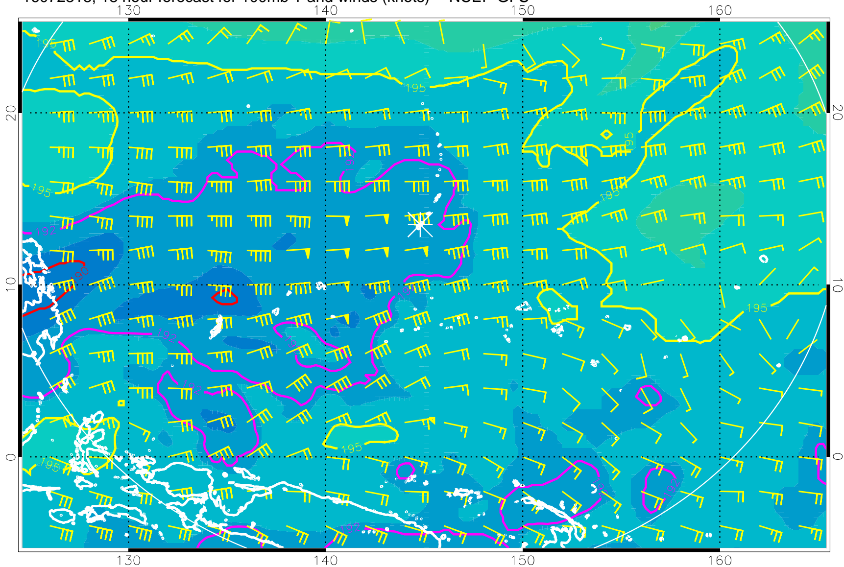
16072318, 18 hour forecast for 100mb T and winds (knots) -- NCEP GFS
