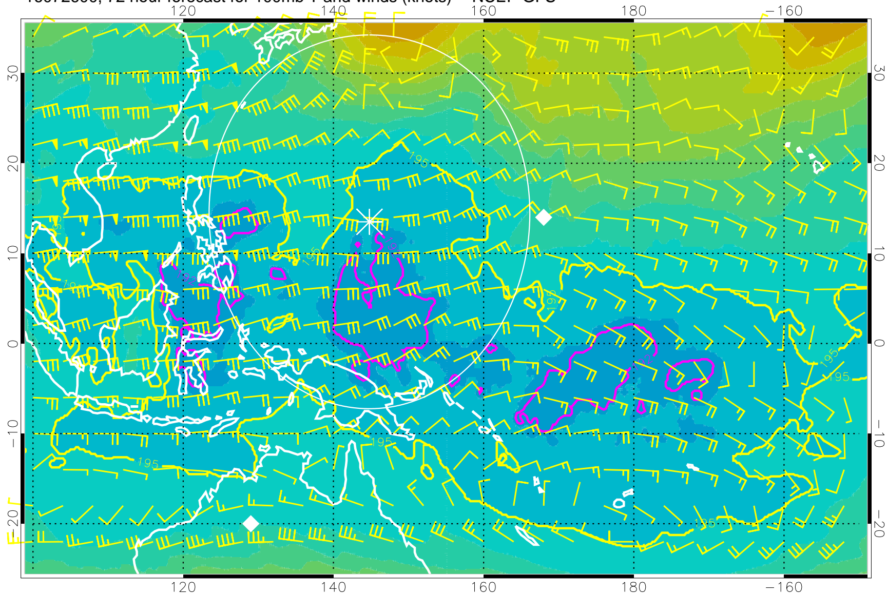
16072600, 72 hour forecast for 100mb T and winds (knots) -- NCEP GFS
