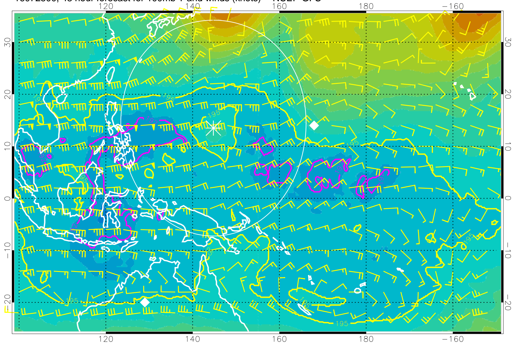
16072500, 48 hour forecast for 100mb T and winds (knots) -- NCEP GFS
