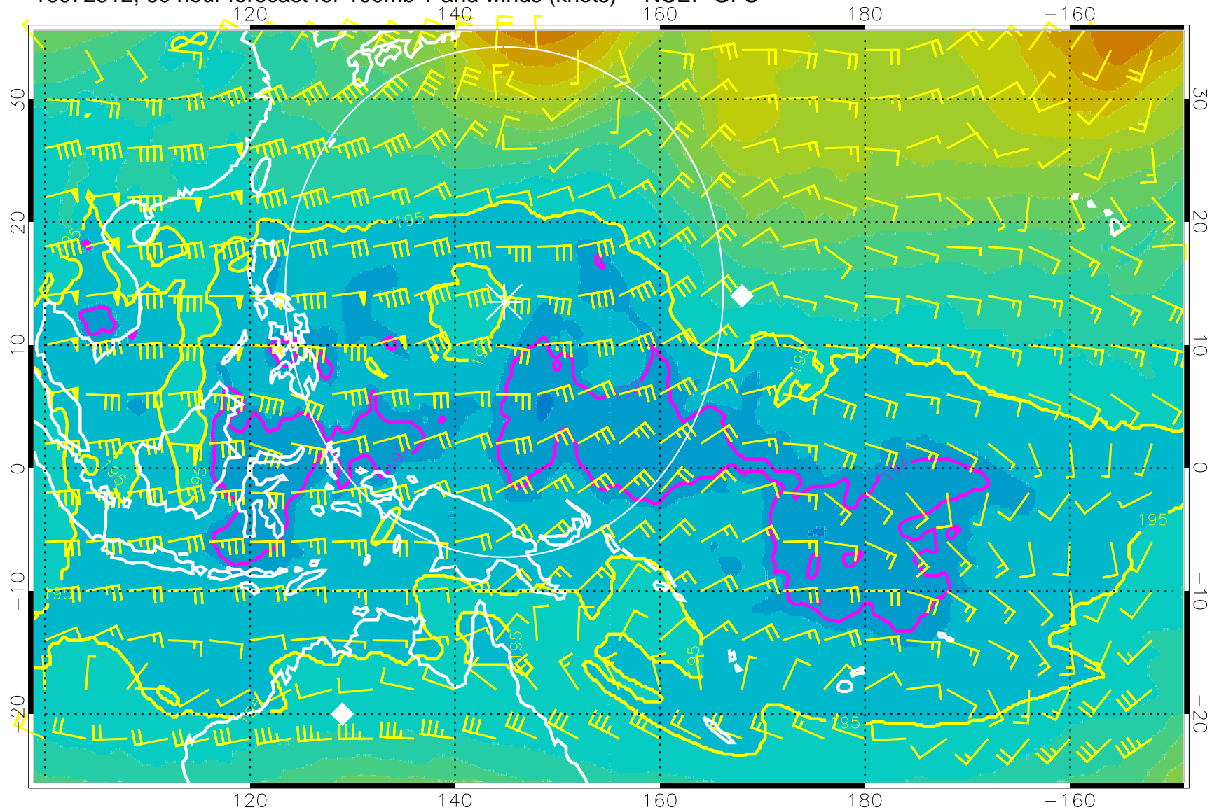
16072512, 60 hour forecast for 100mb T and winds (knots) -- NCEP GFS
