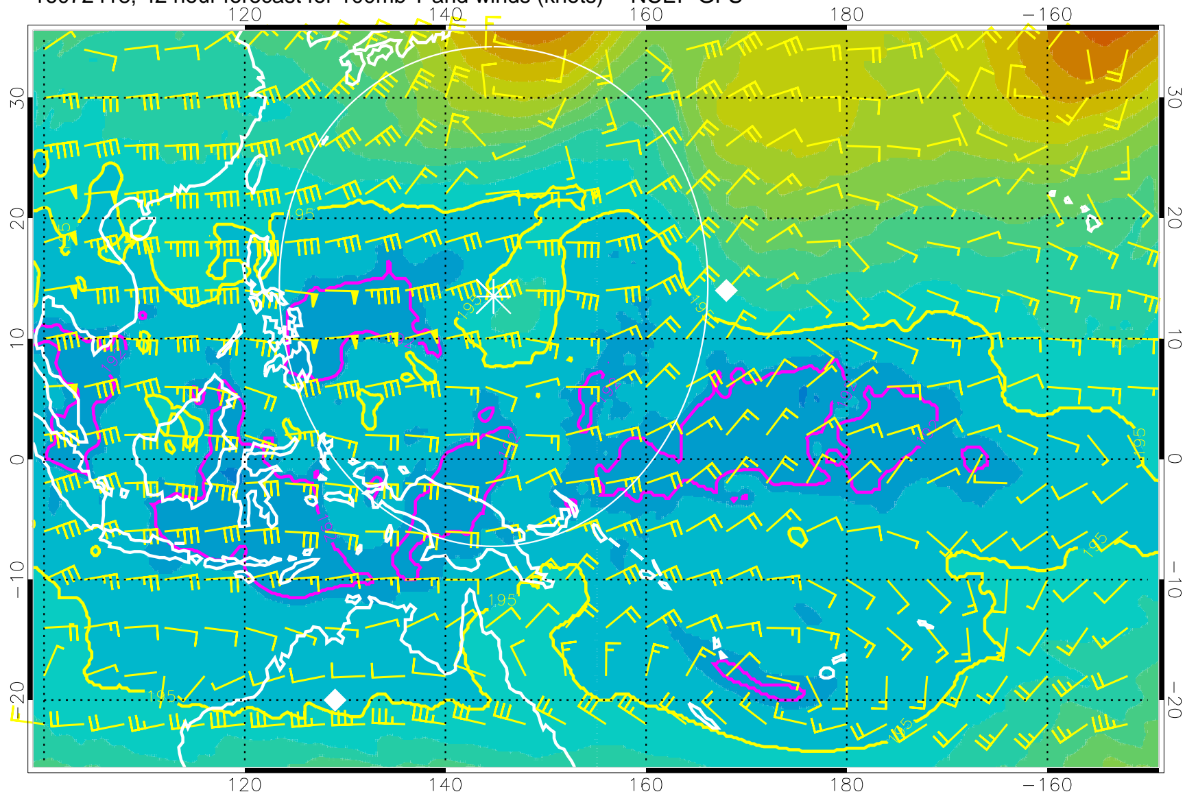
16072418, 42 hour forecast for 100mb T and winds (knots) -- NCEP GFS
