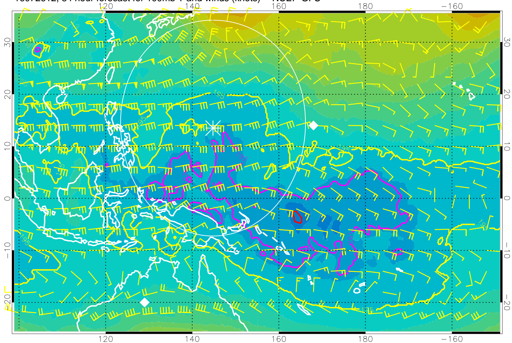
16072612, 84 hour forecast for 100mb T and winds (knots) -- NCEP GFS
