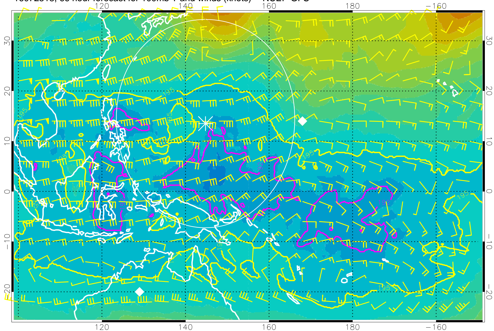
16072518, 66 hour forecast for 100mb T and winds (knots) -- NCEP GFS
