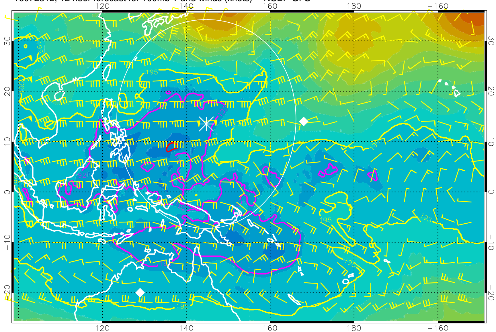
16072312, 12 hour forecast for 100mb T and winds (knots) -- NCEP GFS
