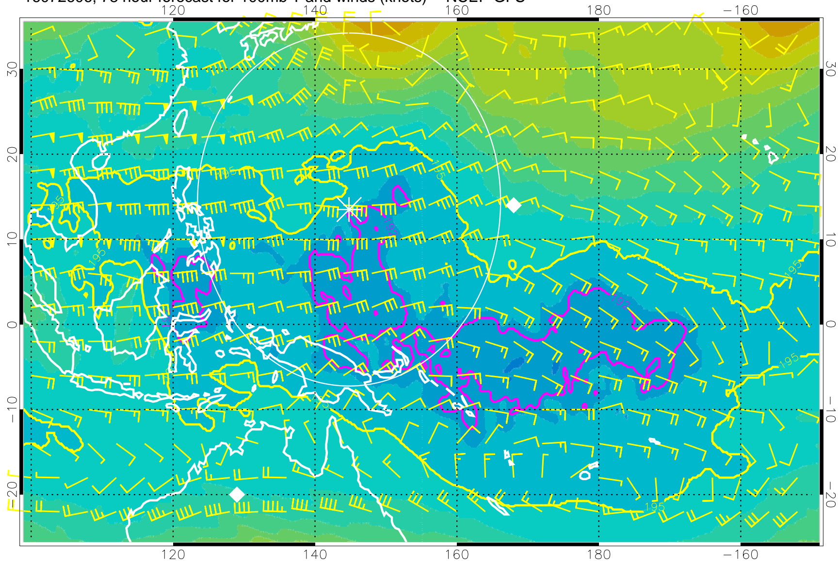
16072606, 78 hour forecast for 100mb T and winds (knots) -- NCEP GFS
