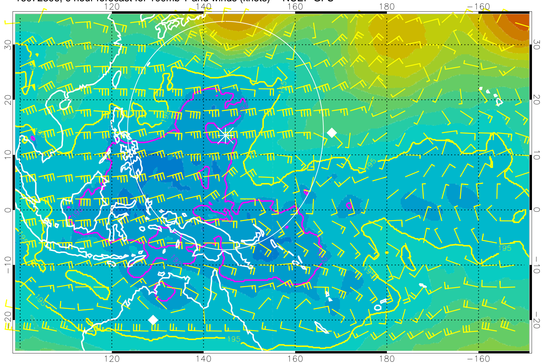
16072306, 6 hour forecast for 100mb T and winds (knots) -- NCEP GFS
