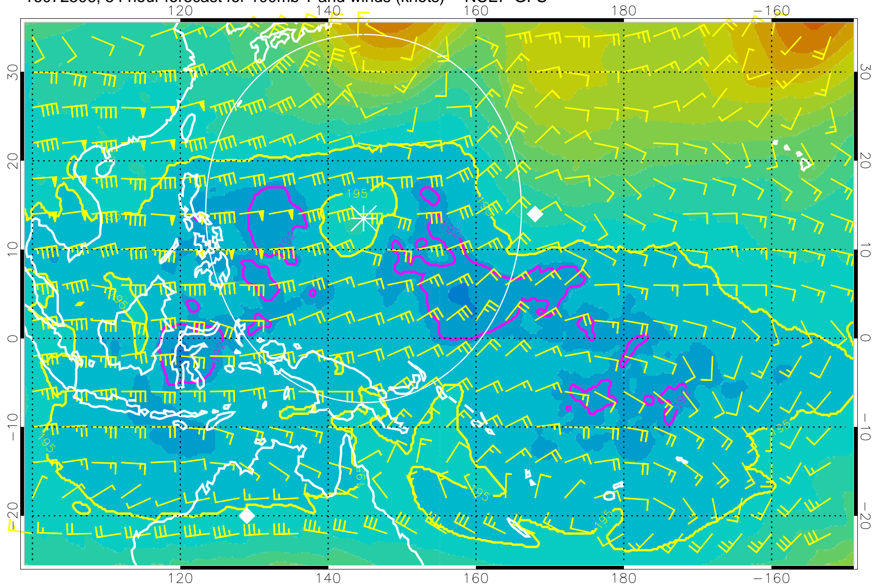
16072506, 54 hour forecast for 100mb T and winds (knots) -- NCEP GFS
