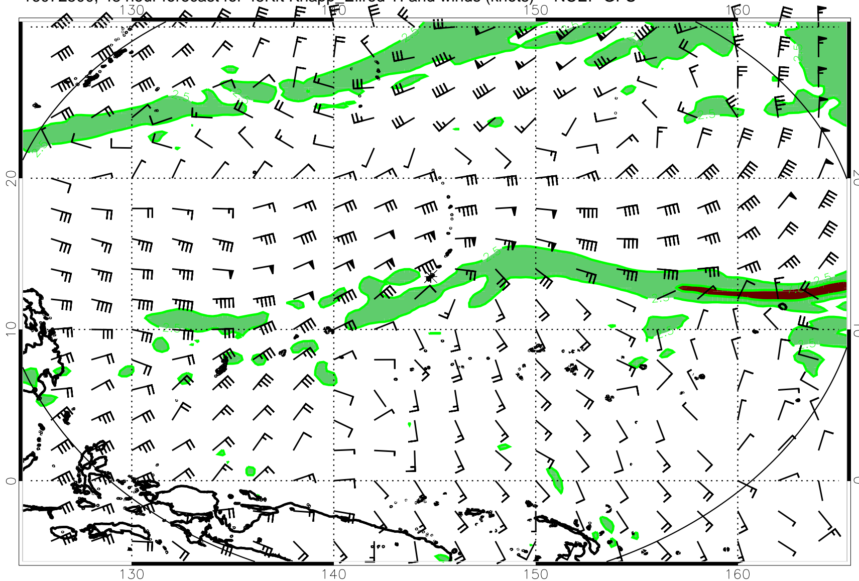
16072500, 48 hour forecast for 45Kft Knapp_Ellrod TI and winds (knots) -- NCEP GFS
