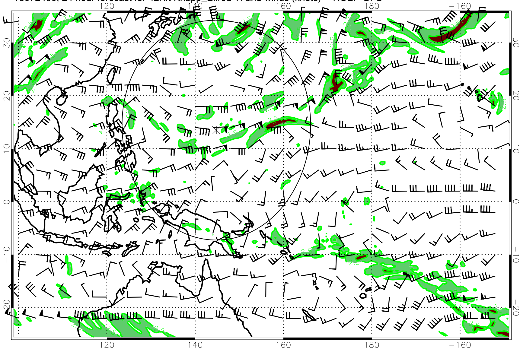
16072400, 24 hour forecast for 42Kft Knapp_Ellrod TI and winds (knots) -- NCEP GFS
