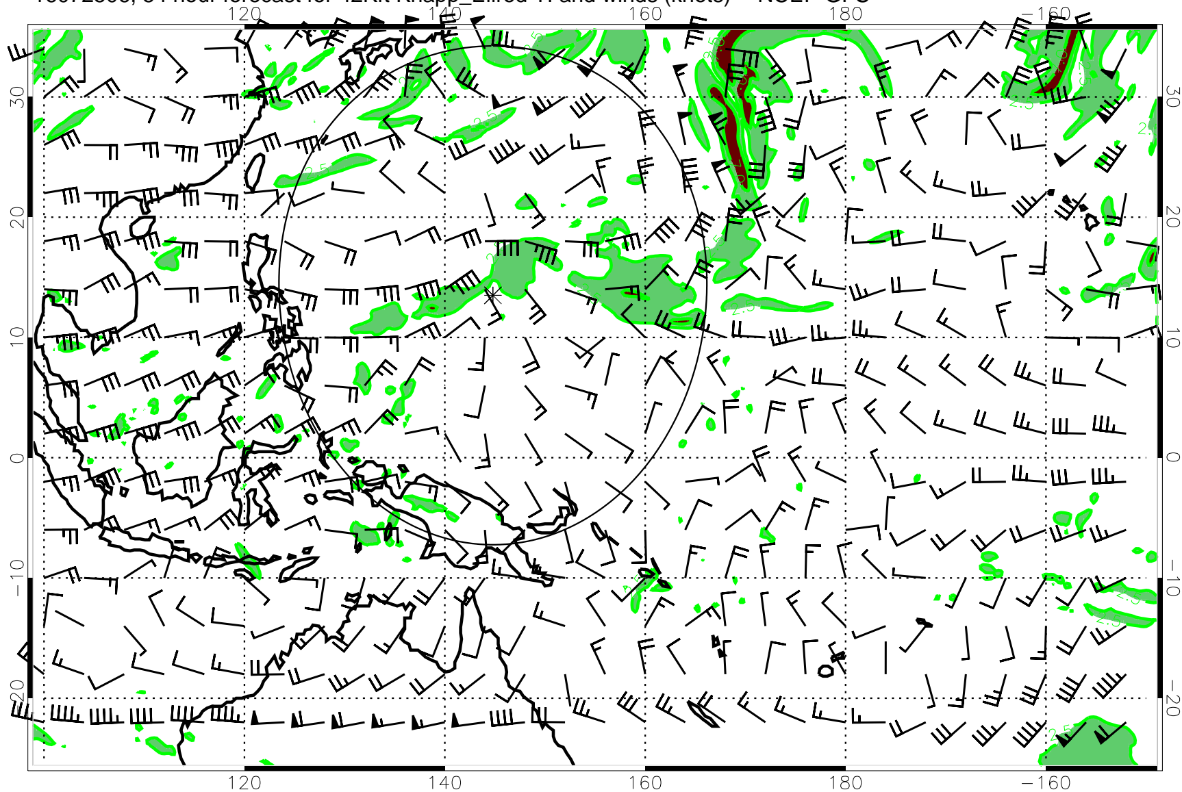
16072506, 54 hour forecast for 42Kft Knapp_Ellrod TI and winds (knots) -- NCEP GFS
